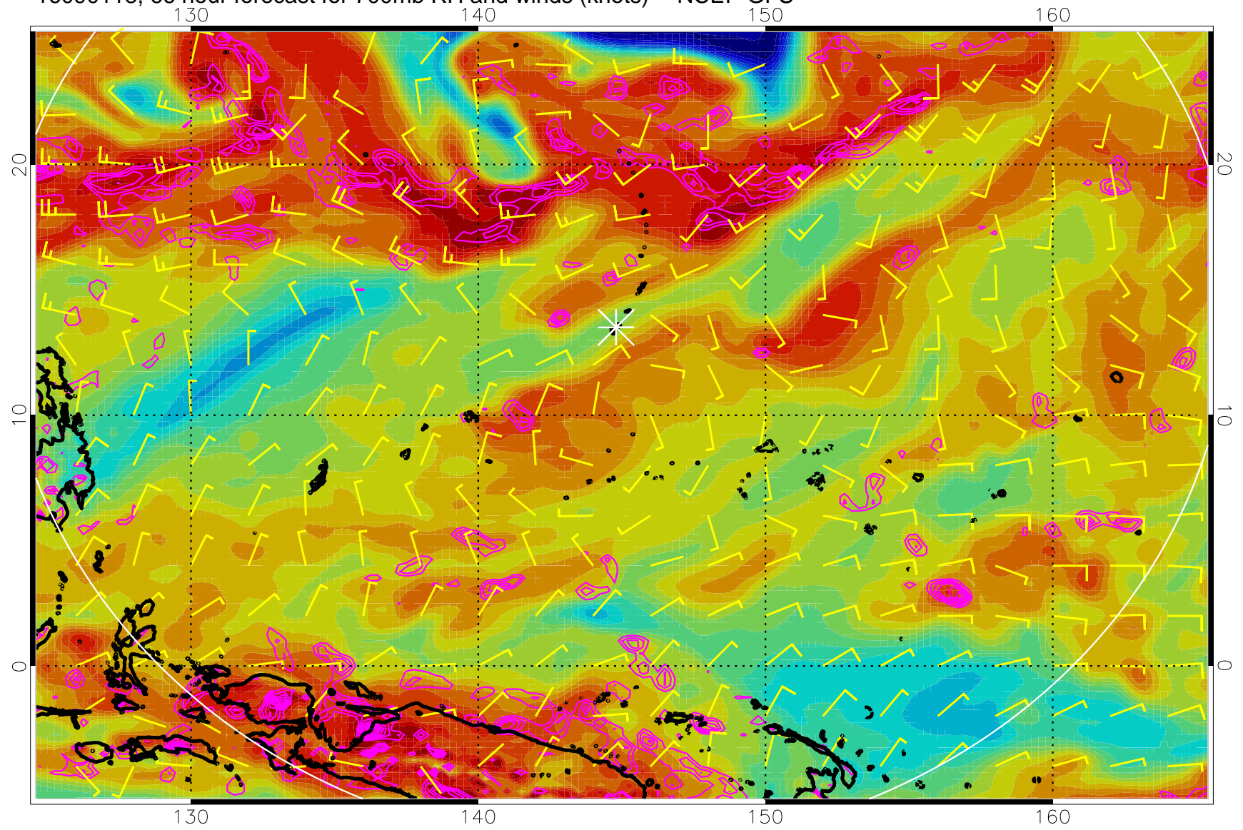
16090118, 66 hour forecast for 700mb RH and winds (knots) -- NCEP GFS
