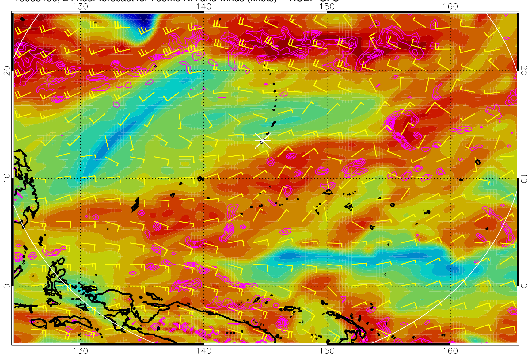
16083100, 24 hour forecast for 700mb RH and winds (knots) -- NCEP GFS
