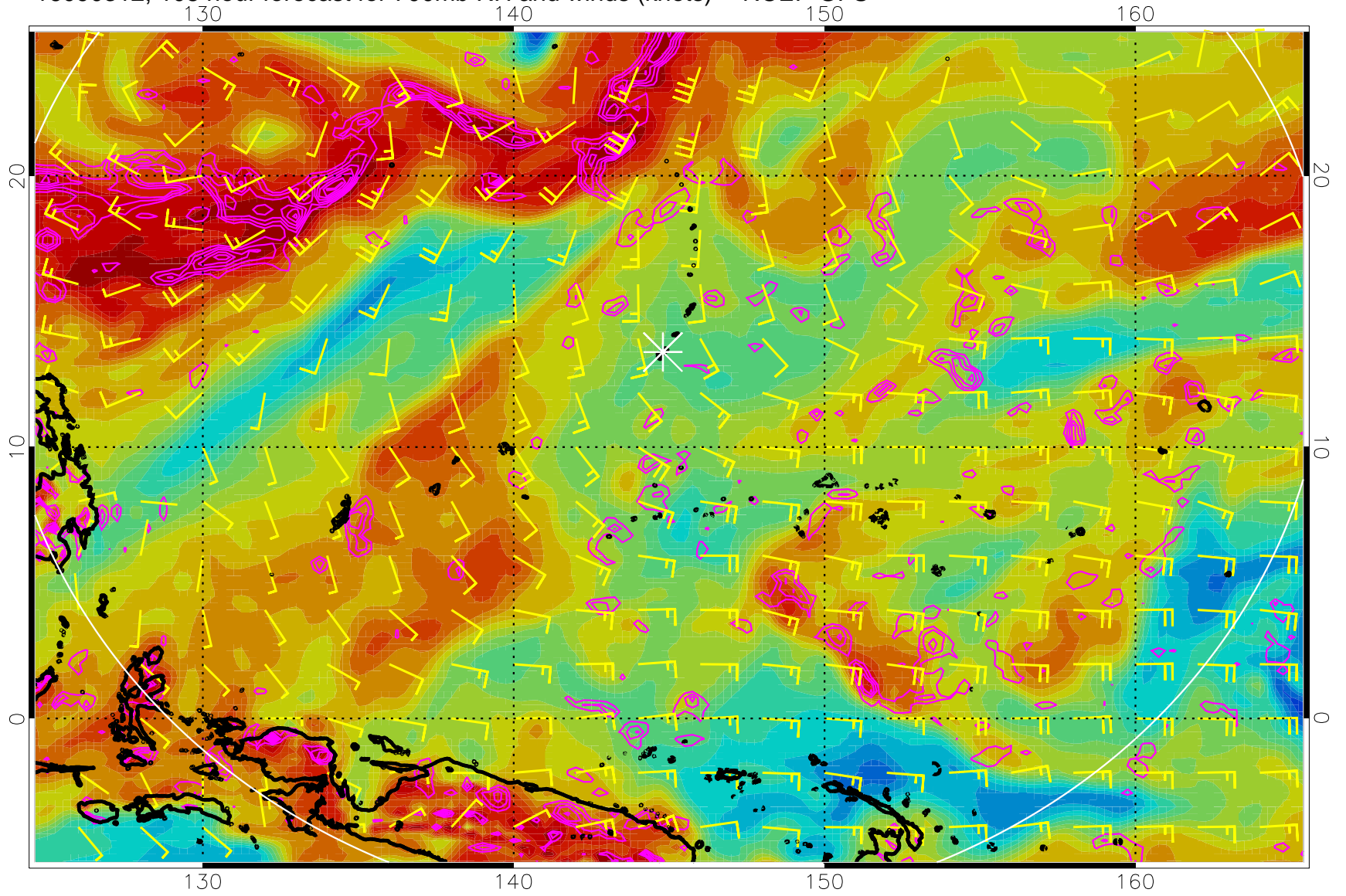
16090312, 108 hour forecast for 700mb RH and winds (knots) -- NCEP GFS
