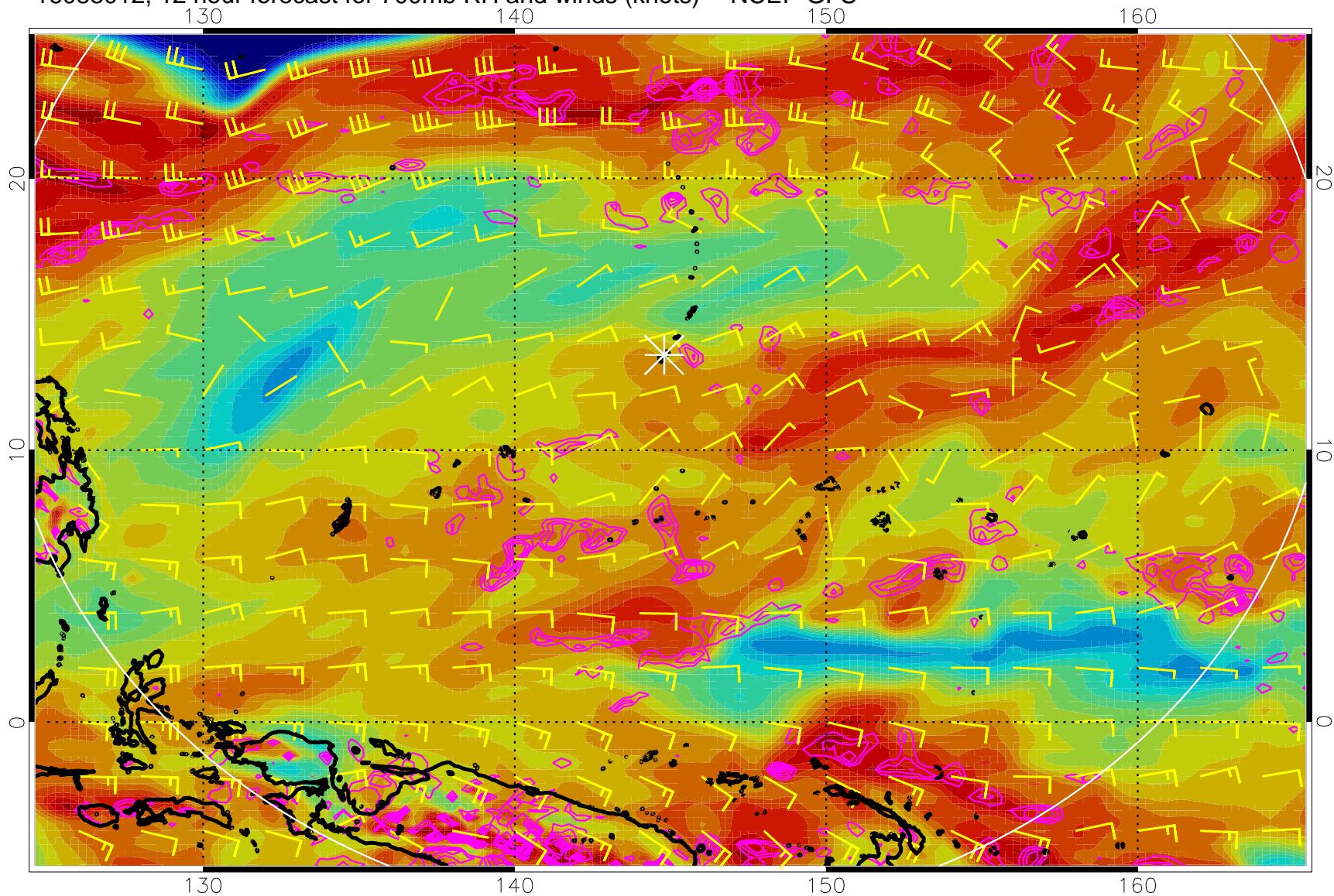
16083012, 12 hour forecast for 700mb RH and winds (knots) -- NCEP GFS
