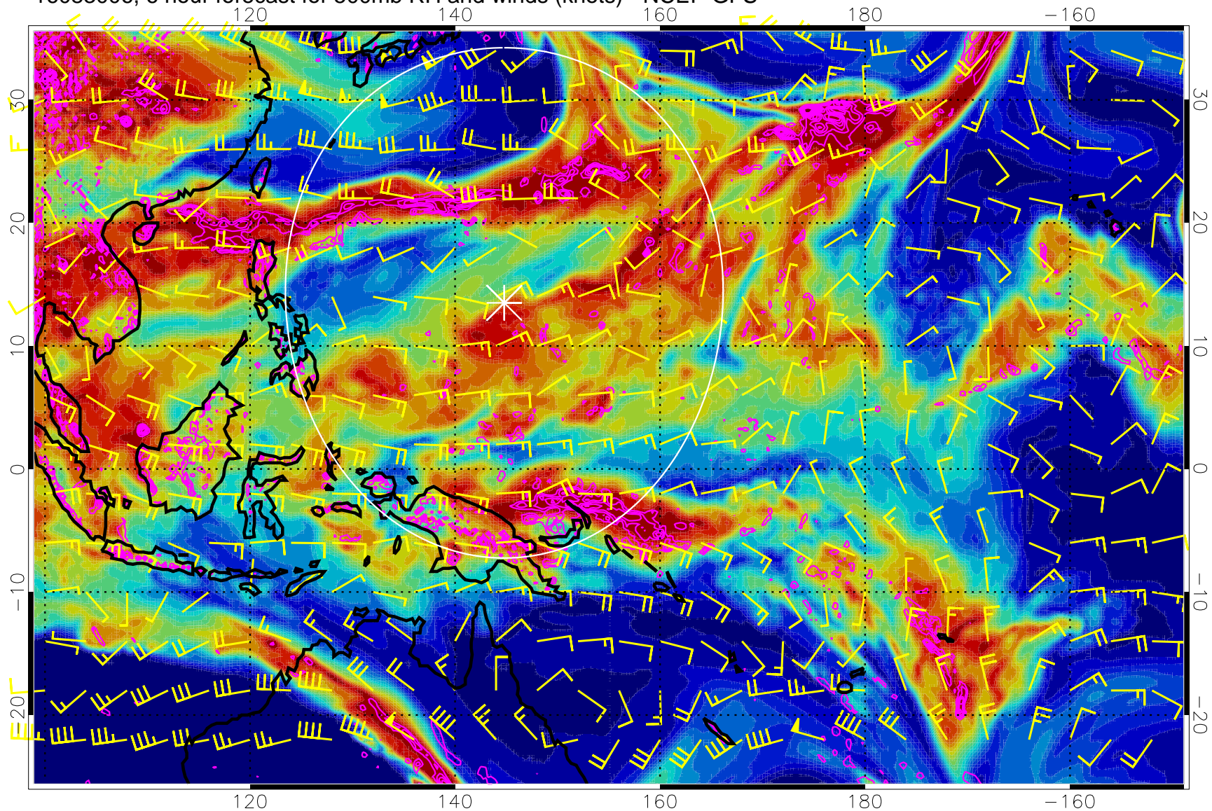
16083006, 6 hour forecast for 500mb RH and winds (knots) - NCEP GFS
