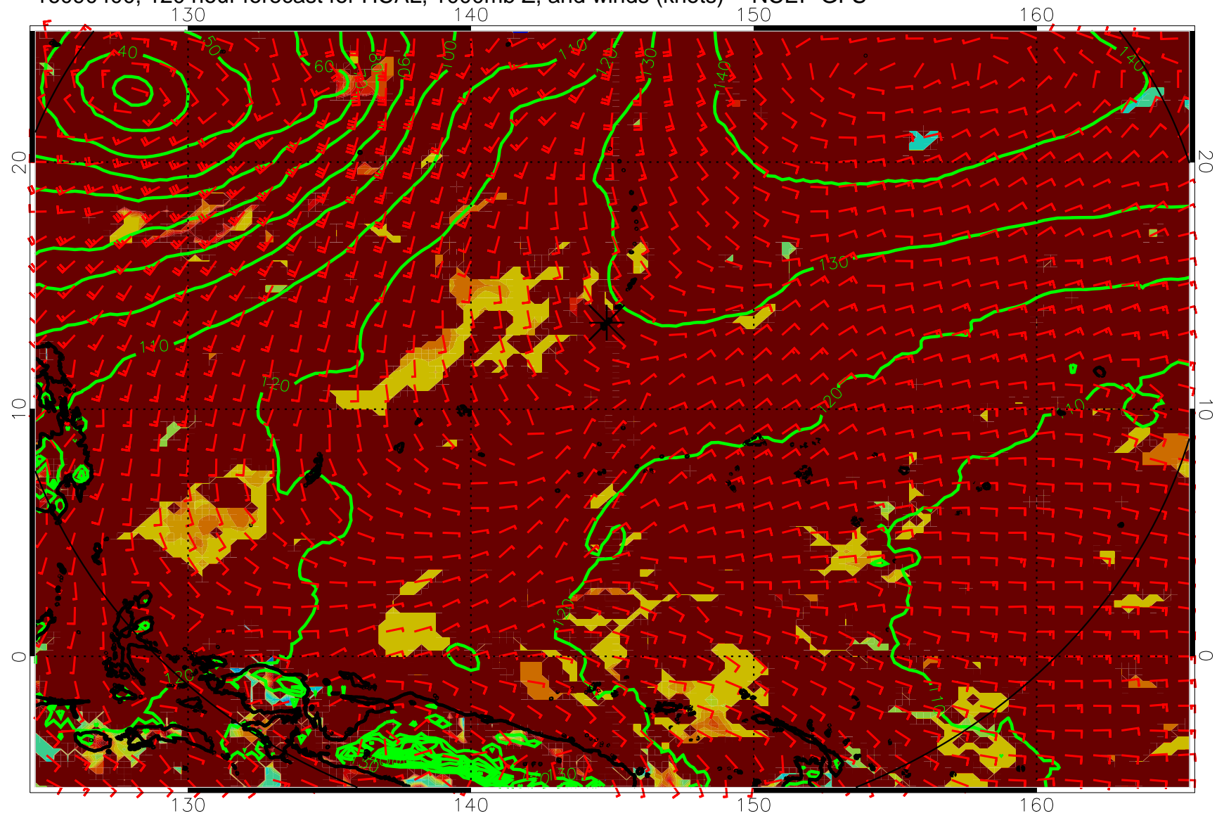
16090400, 120 hour forecast for HCAL, 1000mb Z, and winds (knots) -- NCEP GFS
