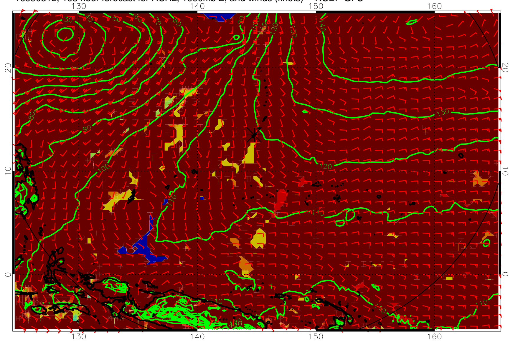
16090312, 108 hour forecast for HCAL, 1000mb Z, and winds (knots) -- NCEP GFS
