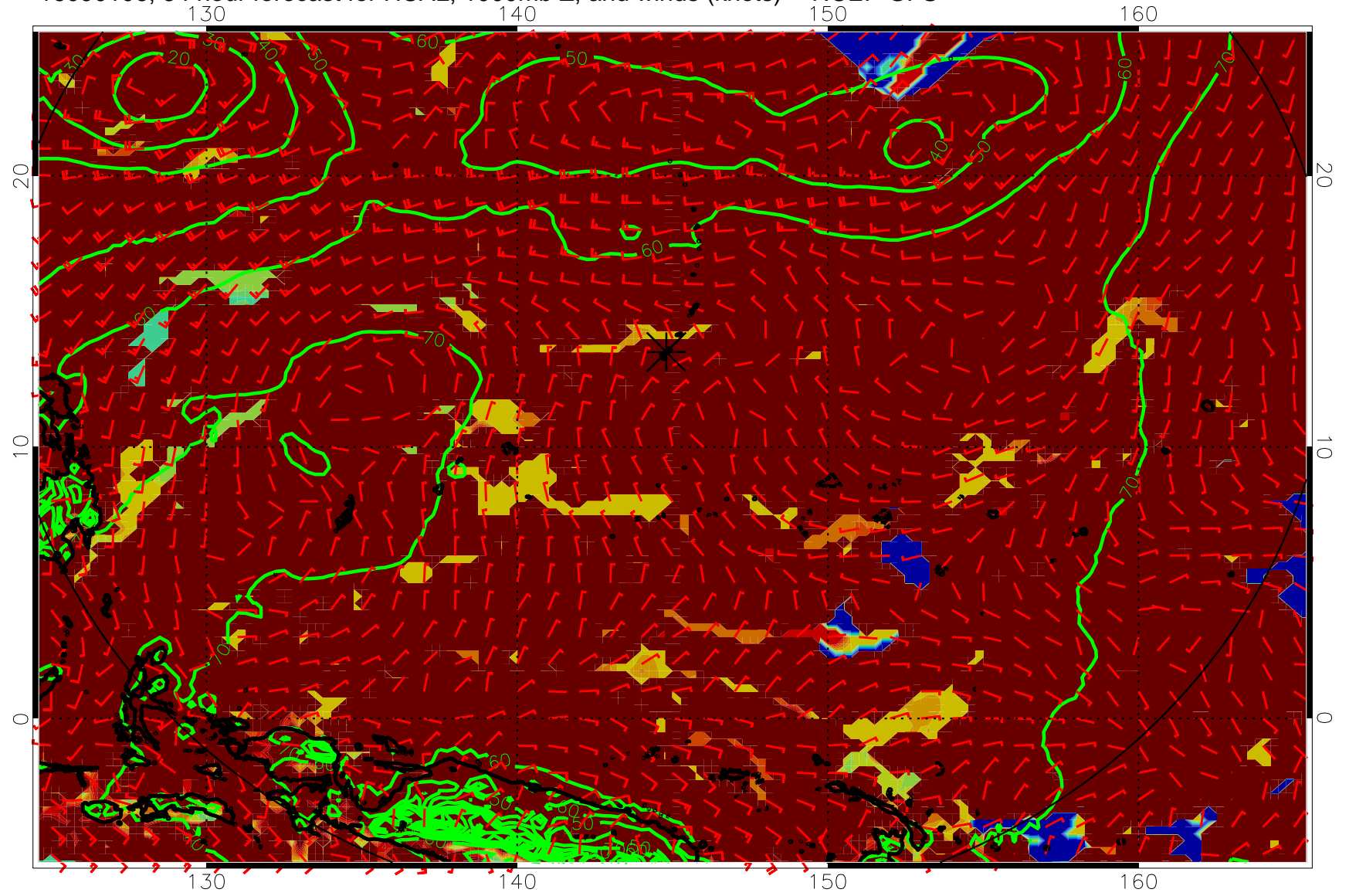
16090106, 54 hour forecast for HCAL, 1000mb Z, and winds (knots) -- NCEP GFS
