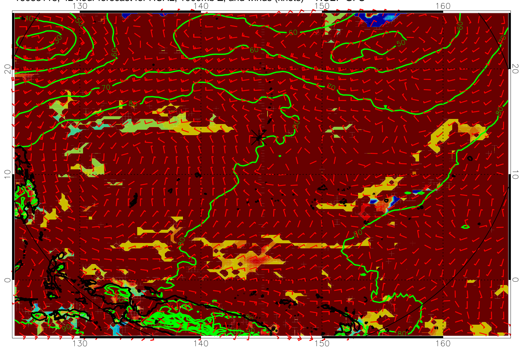
16083118, 42 hour forecast for HCAL, 1000mb Z, and winds (knots) -- NCEP GFS
