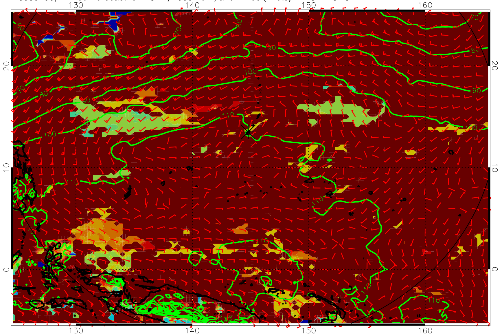
16083100, 24 hour forecast for HCAL, 1000mb Z, and winds (knots) -- NCEP GFS
