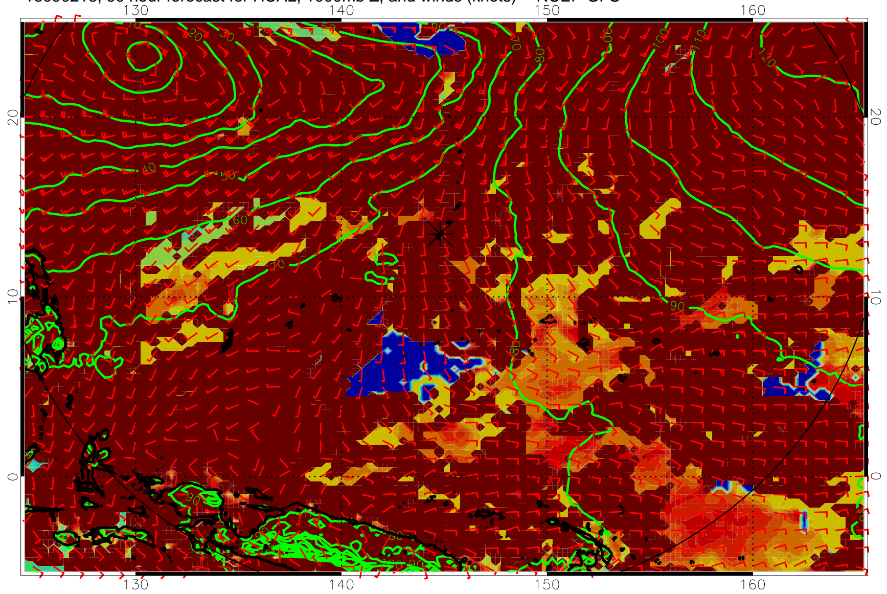
16090218, 90 hour forecast for HCAL, 1000mb Z, and winds (knots) -- NCEP GFS
