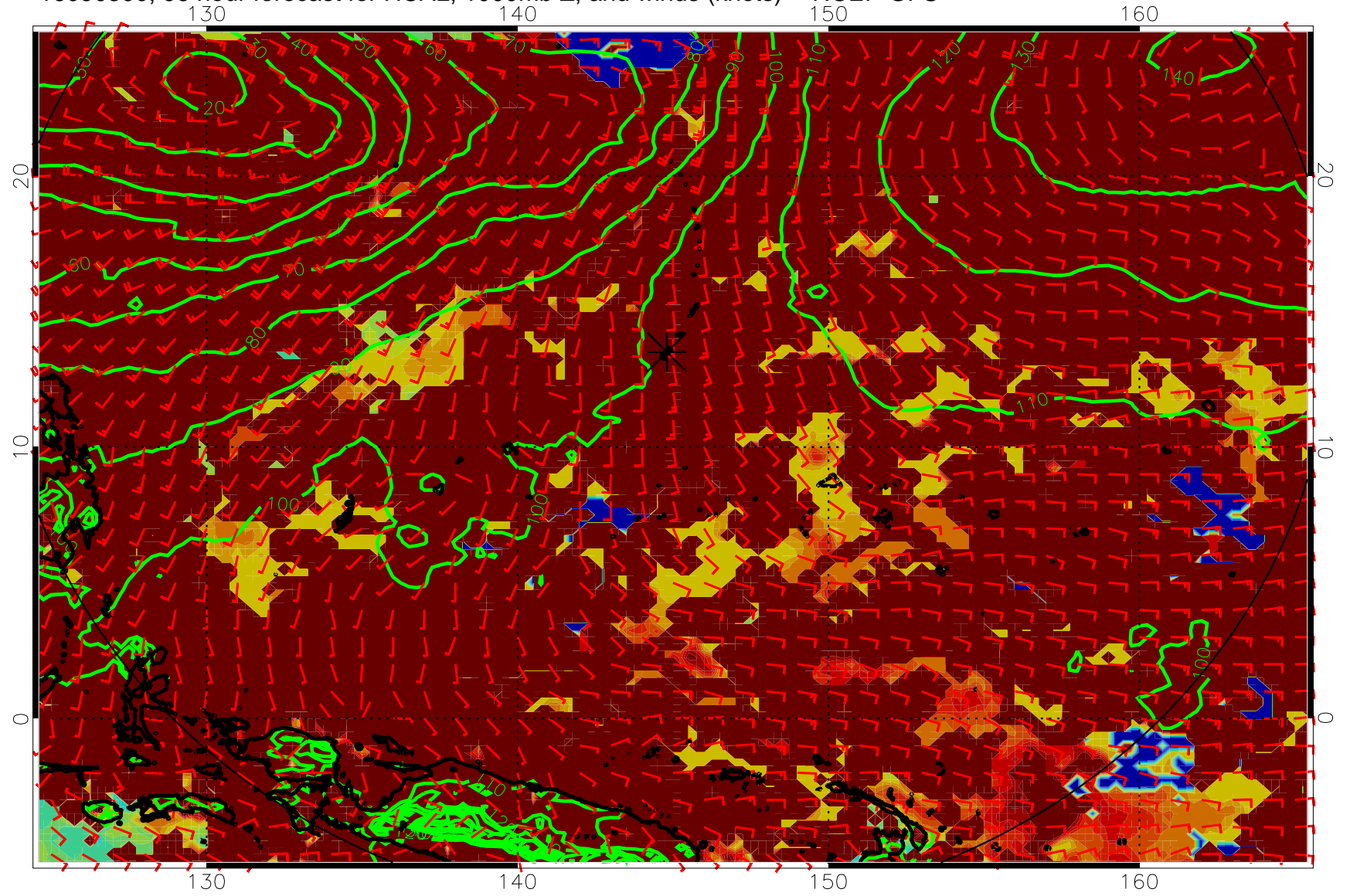
16090300, 96 hour forecast for HCAL, 1000mb Z, and winds (knots) -- NCEP GFS
