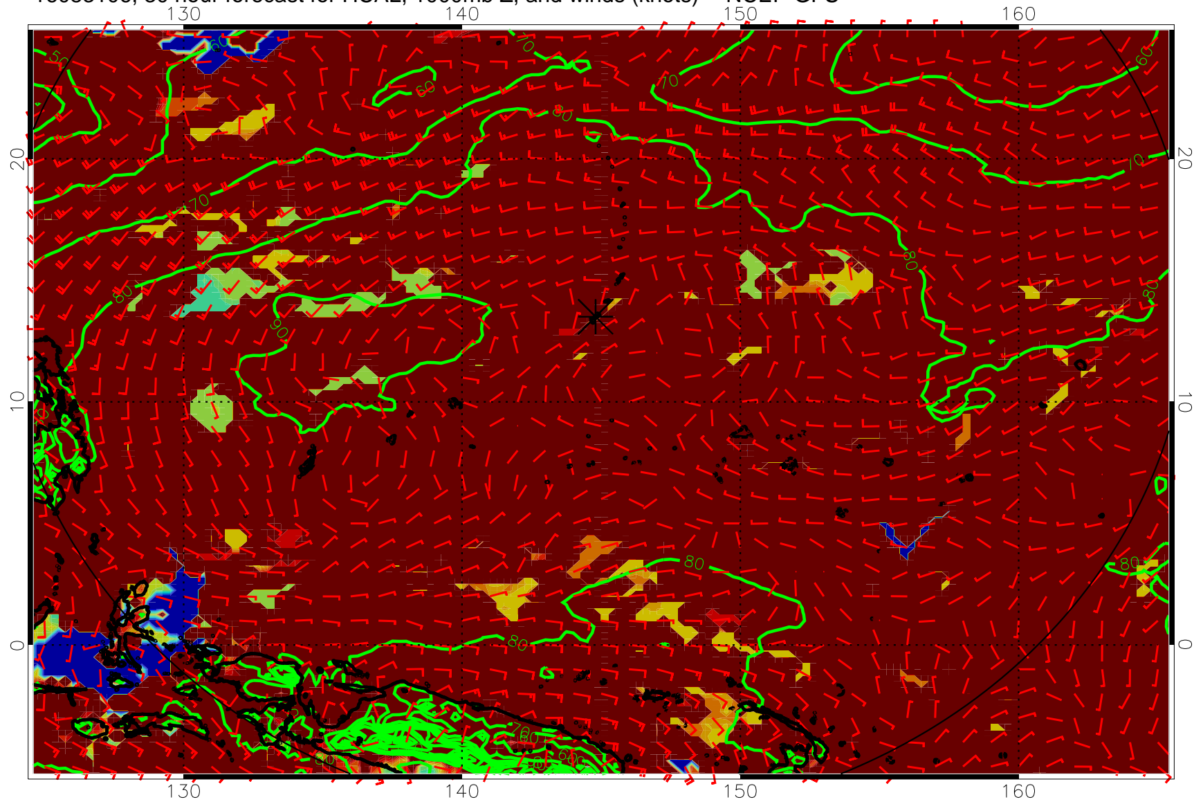
16083106, 30 hour forecast for HCAL, 1000mb Z, and winds (knots) -- NCEP GFS
