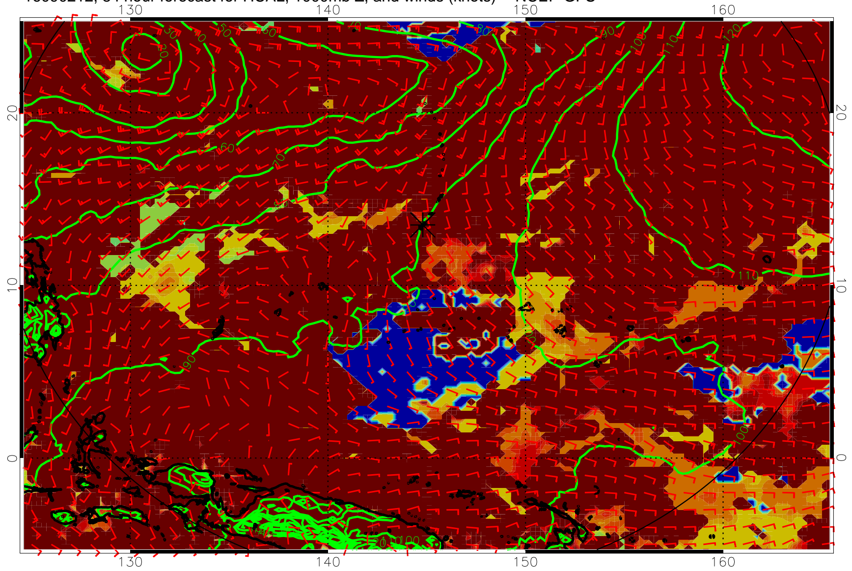
16090212, 84 hour forecast for HCAL, 1000mb Z, and winds (knots) -- NCEP GFS
