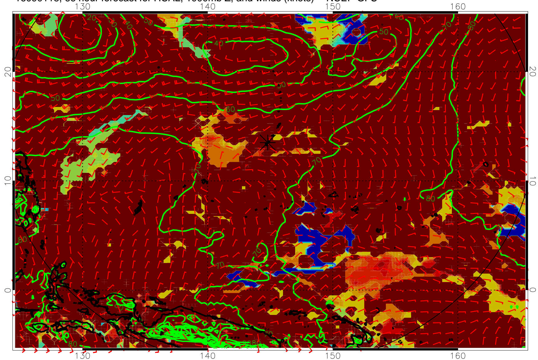
16090118, 66 hour forecast for HCAL, 1000mb Z, and winds (knots) -- NCEP GFS
