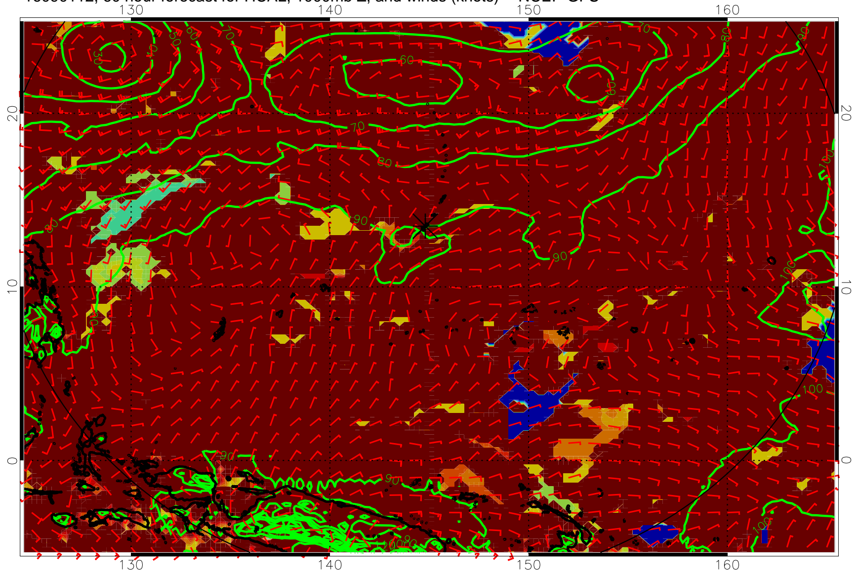
16090112, 60 hour forecast for HCAL, 1000mb Z, and winds (knots) -- NCEP GFS
