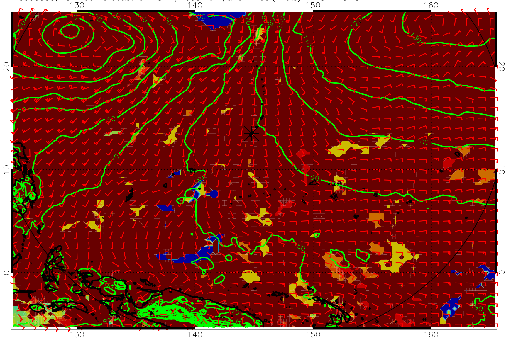
16090306, 102 hour forecast for HCAL, 1000mb Z, and winds (knots) -- NCEP GFS
