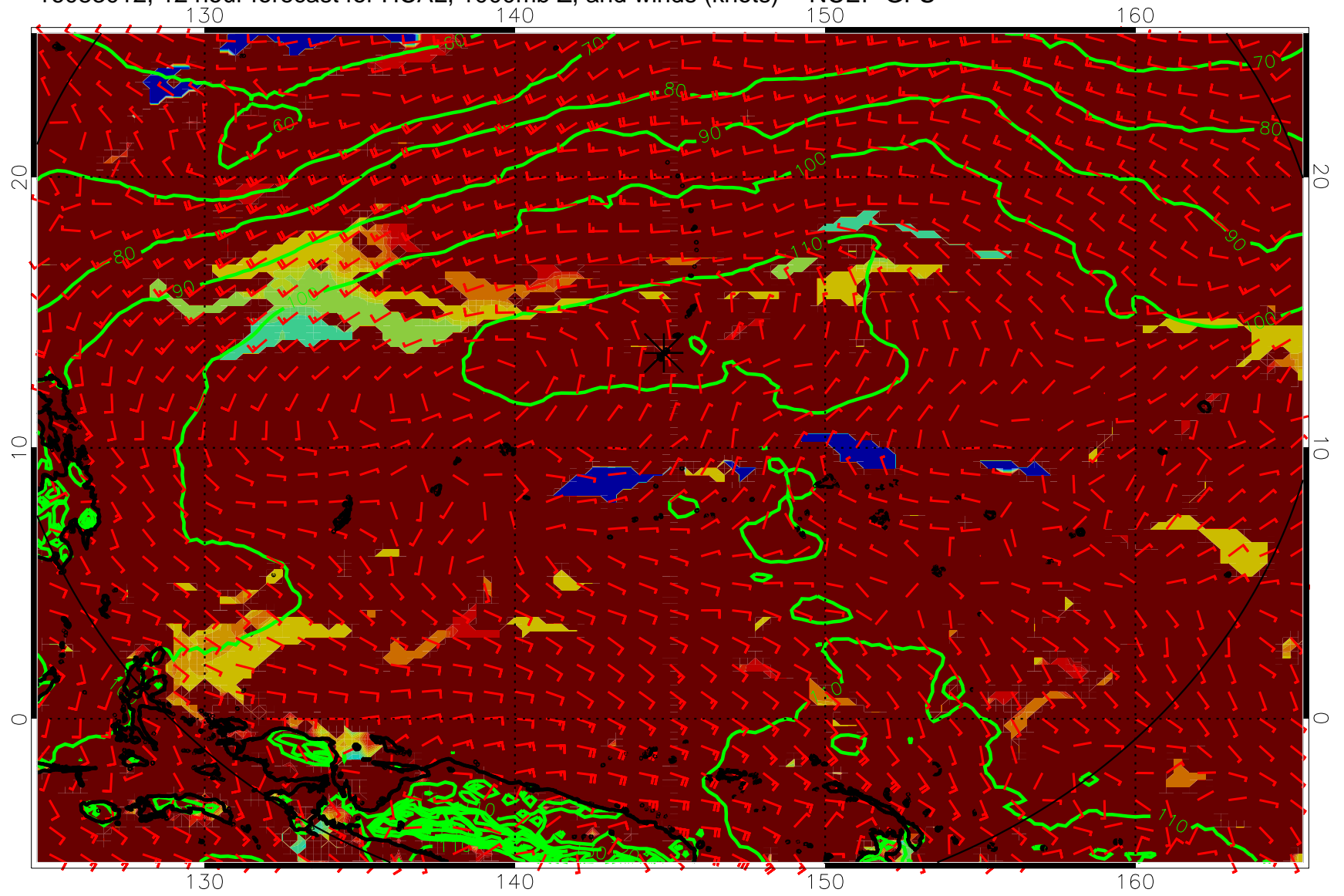
16083012, 12 hour forecast for HCAL, 1000mb Z, and winds (knots) -- NCEP GFS
