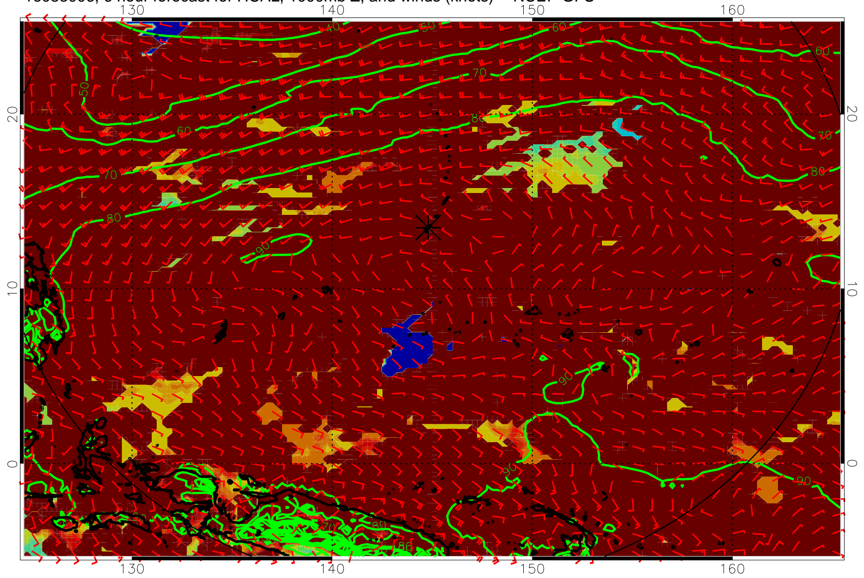
16083006, 6 hour forecast for HCAL, 1000mb Z, and winds (knots) -- NCEP GFS
