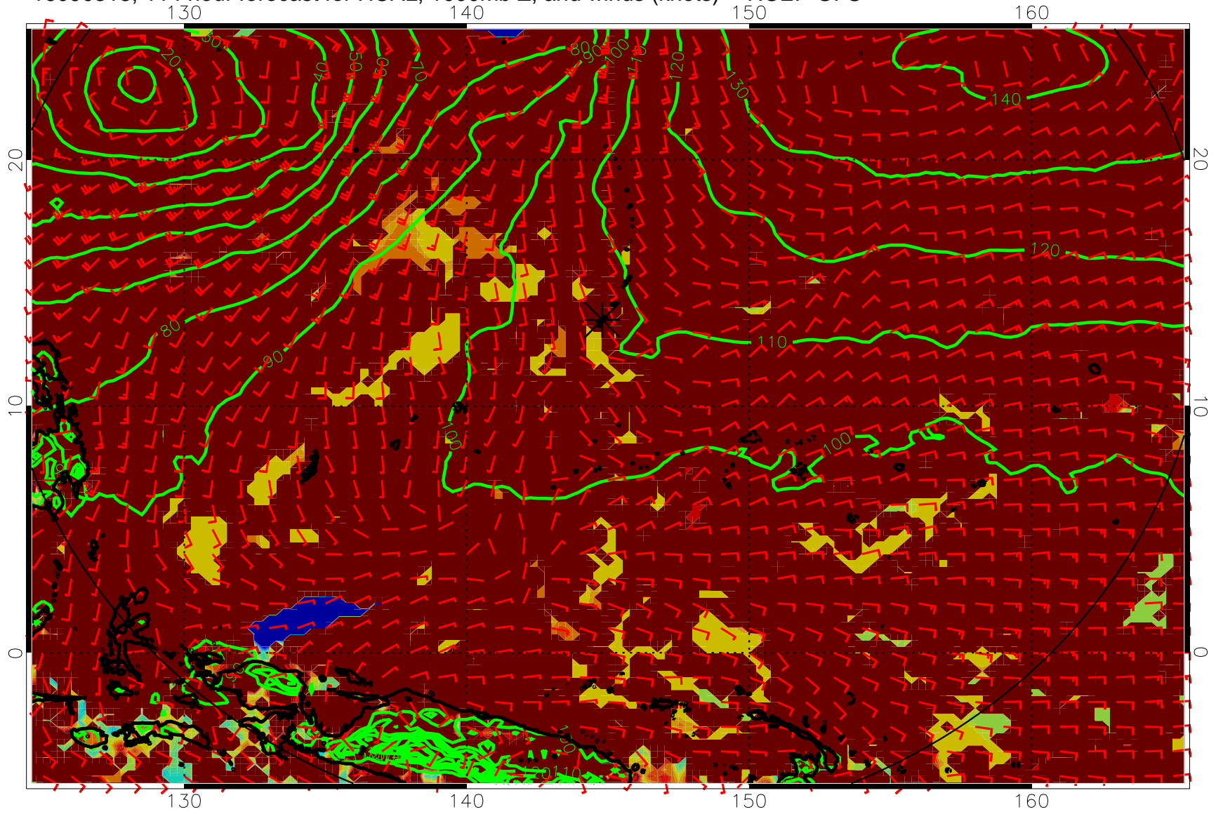
16090318, 114 hour forecast for HCAL, 1000mb Z, and winds (knots) -- NCEP GFS
