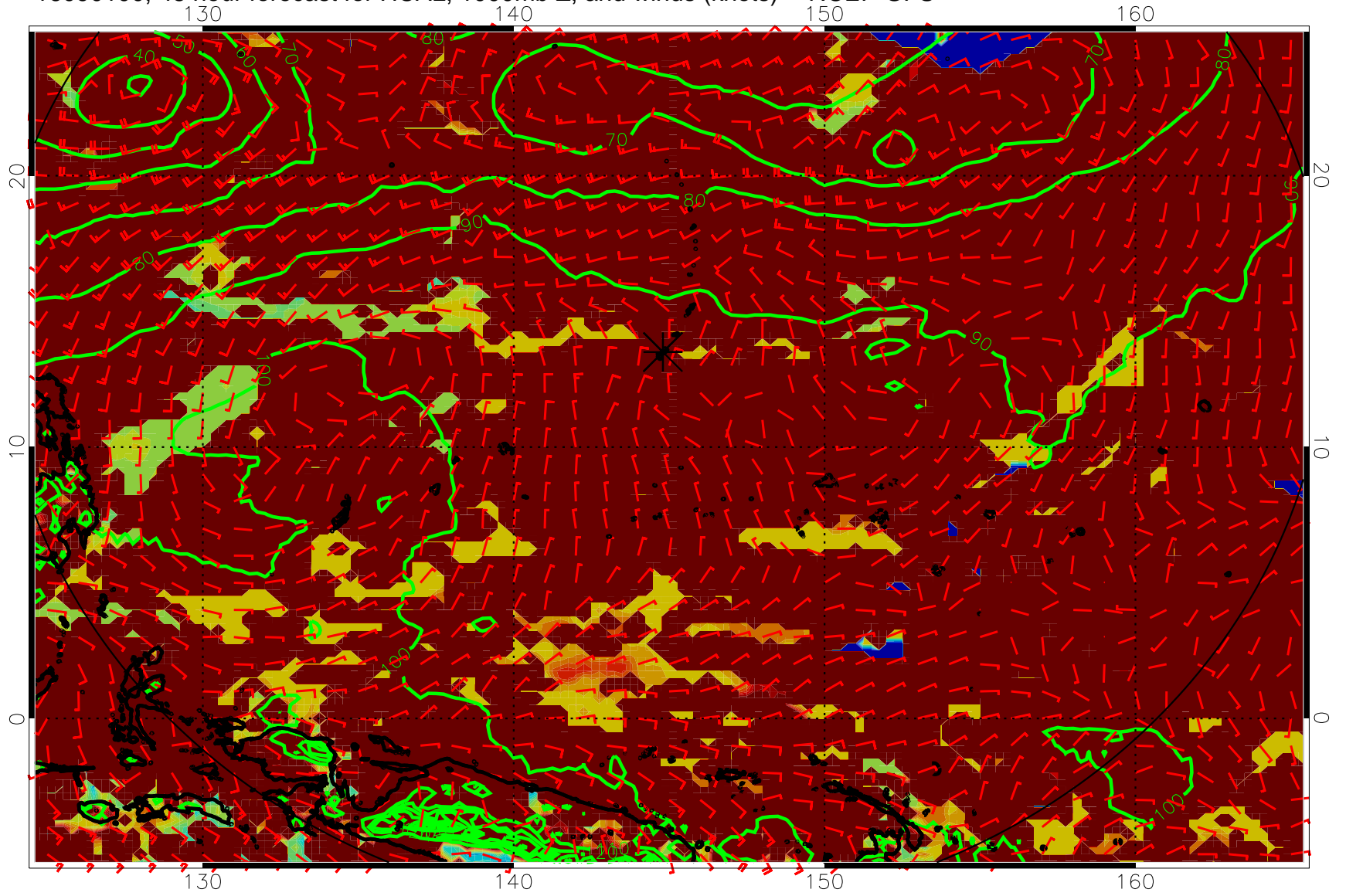
16090100, 48 hour forecast for HCAL, 1000mb Z, and winds (knots) -- NCEP GFS
