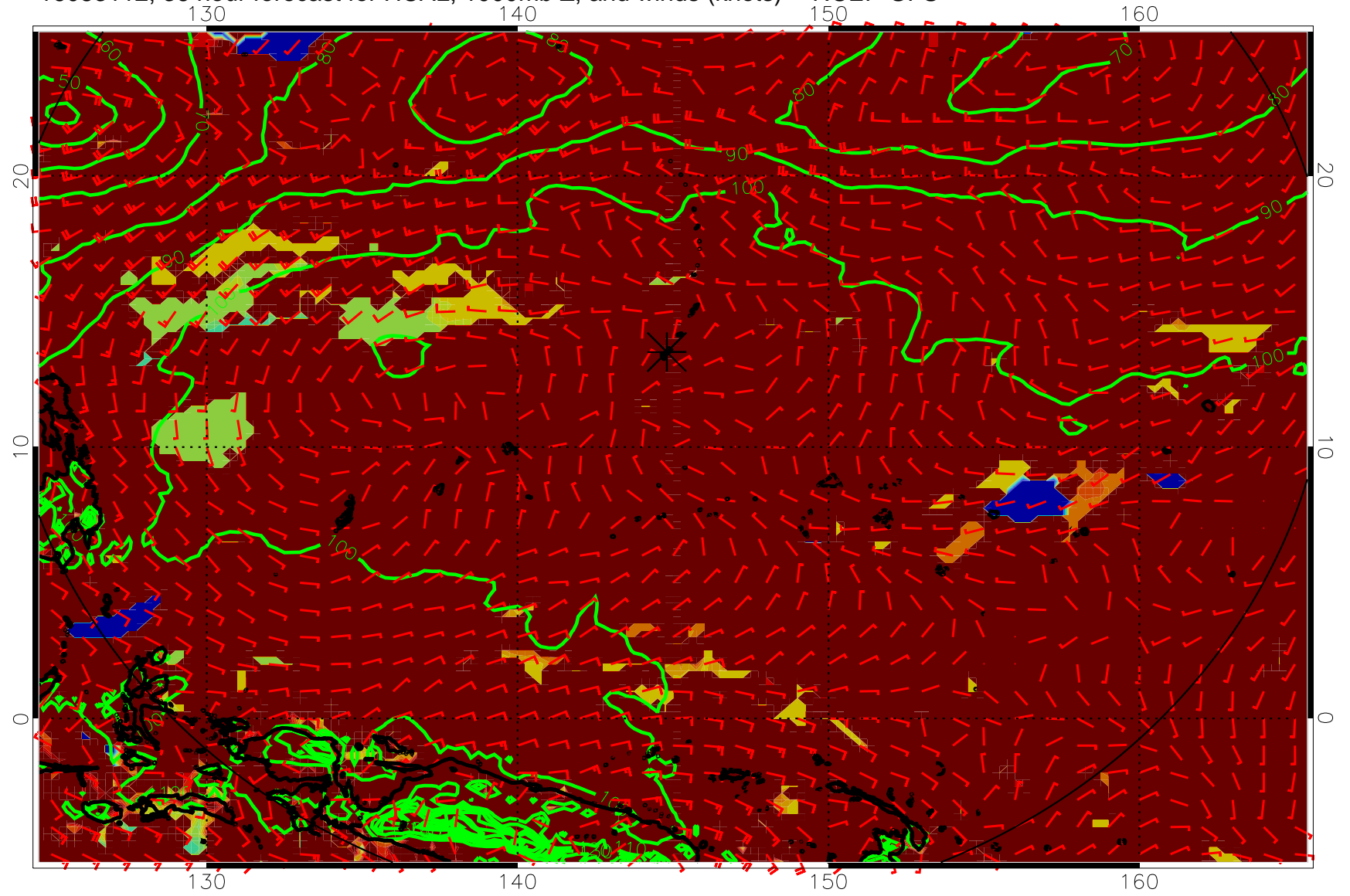
16083112, 36 hour forecast for HCAL, 1000mb Z, and winds (knots) -- NCEP GFS
