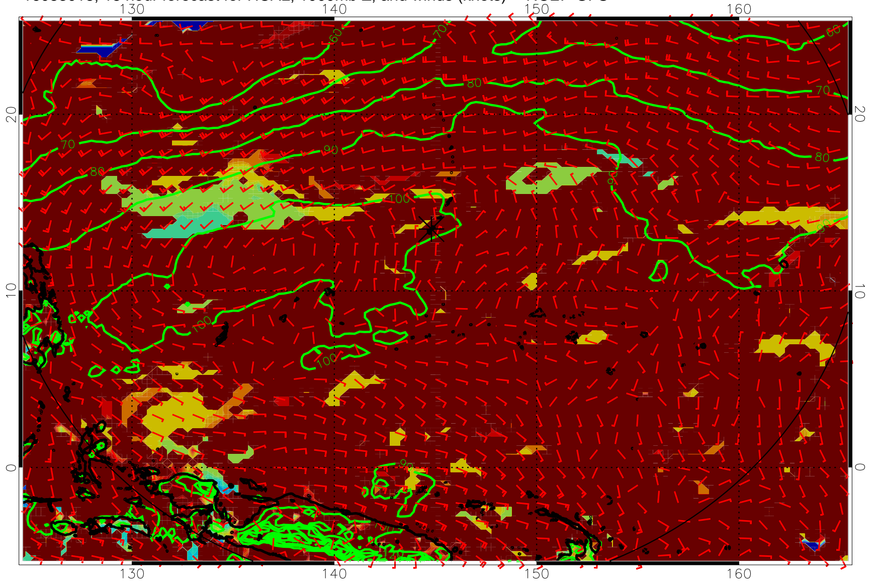
16083018, 18 hour forecast for HCAL, 1000mb Z, and winds (knots) -- NCEP GFS
