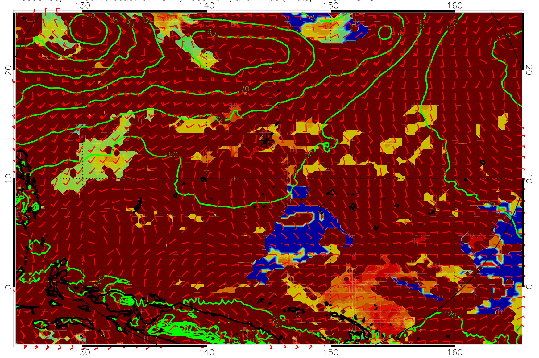
16090200, 72 hour forecast for HCAL, 1000mb Z, and winds (knots) -- NCEP GFS
