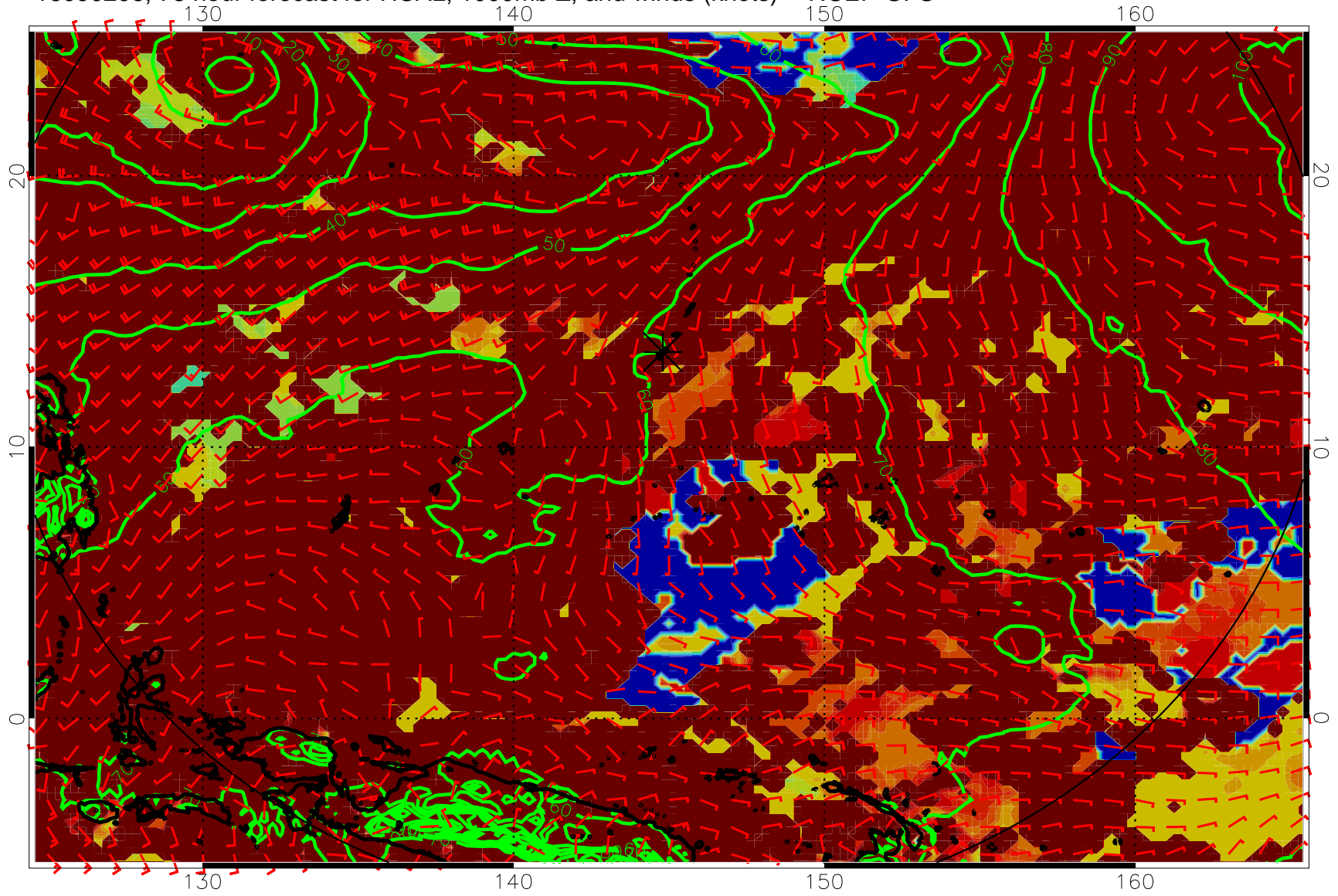
16090206, 78 hour forecast for HCAL, 1000mb Z, and winds (knots) -- NCEP GFS
