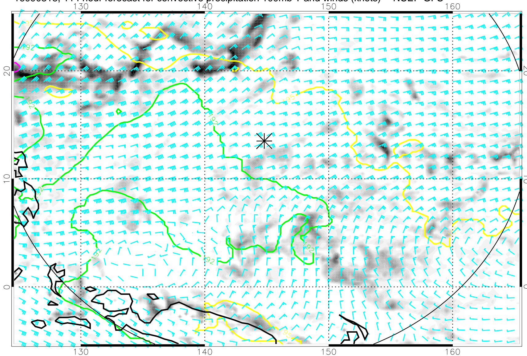
16090318, 114 hour forecast for convective precipitation 100mb T and winds (knots) -- NCEP GFS
