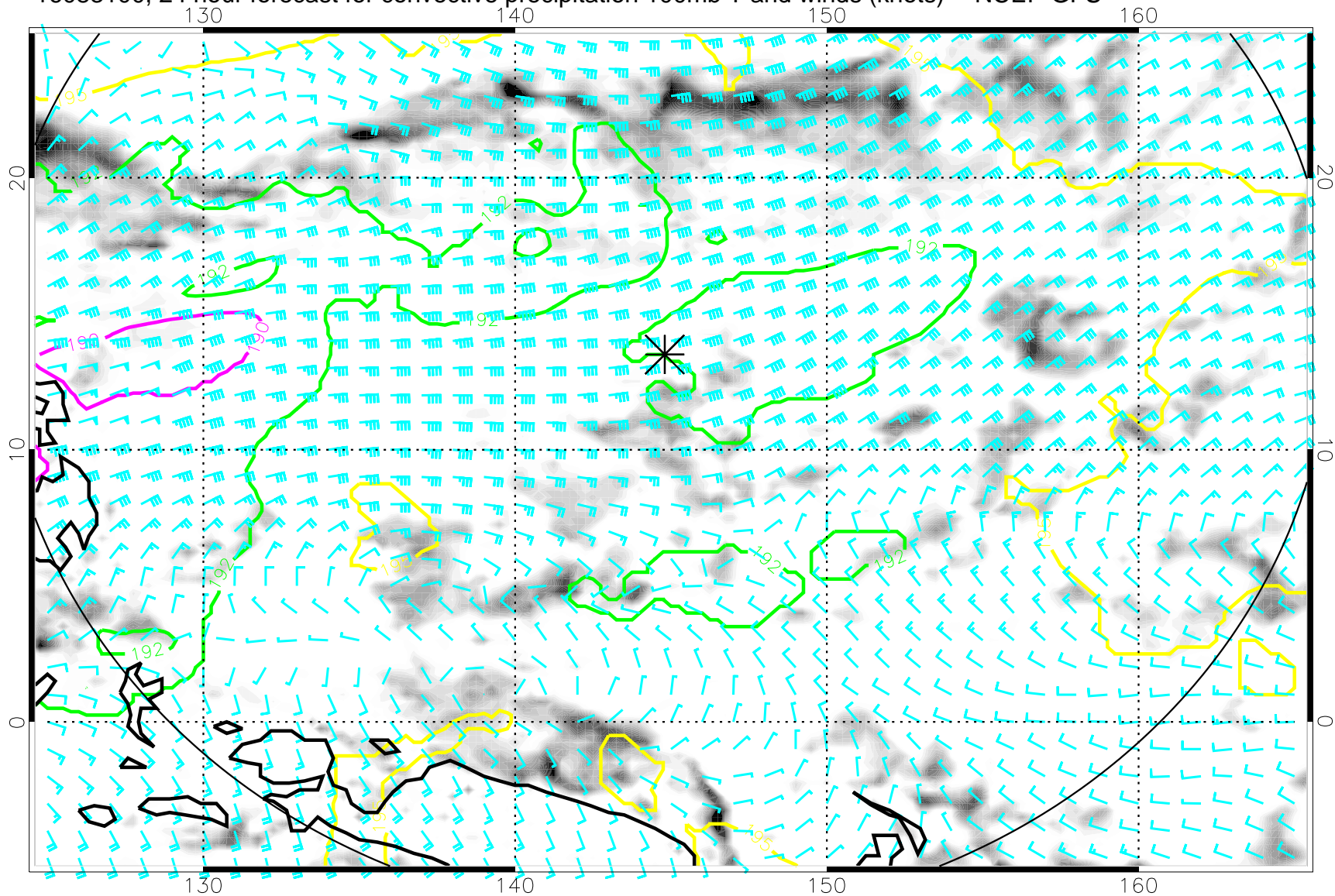
16083100, 24 hour forecast for convective precipitation 100mb T and winds (knots) -- NCEP GFS
