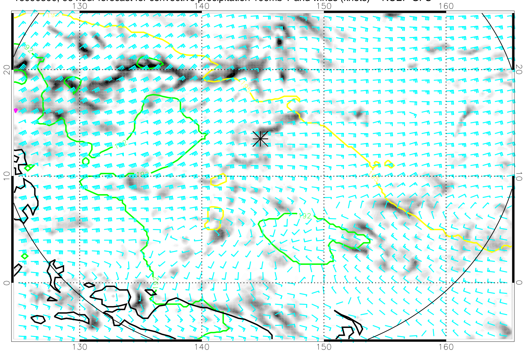
16090300, 96 hour forecast for convective precipitation 100mb T and winds (knots) -- NCEP GFS
