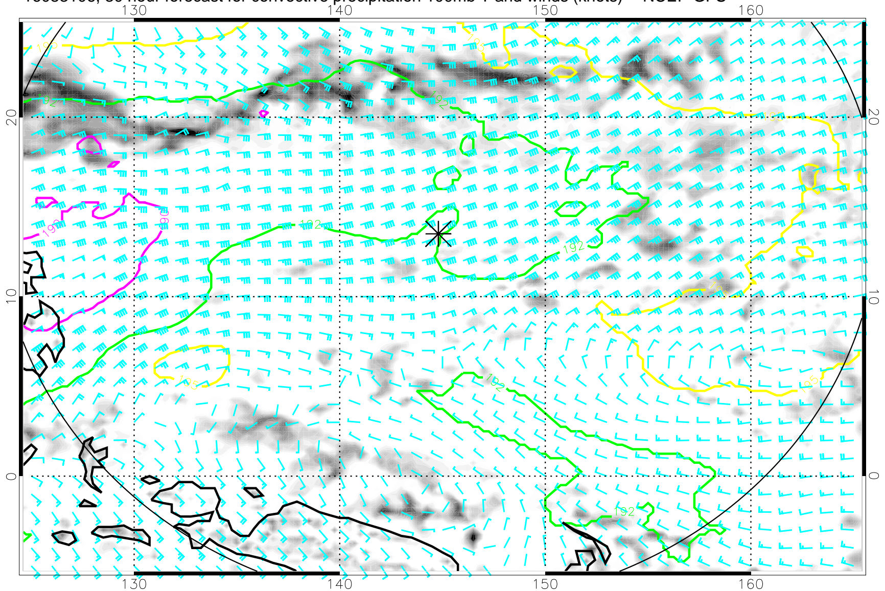
16083106, 30 hour forecast for convective precipitation 100mb T and winds (knots) -- NCEP GFS
