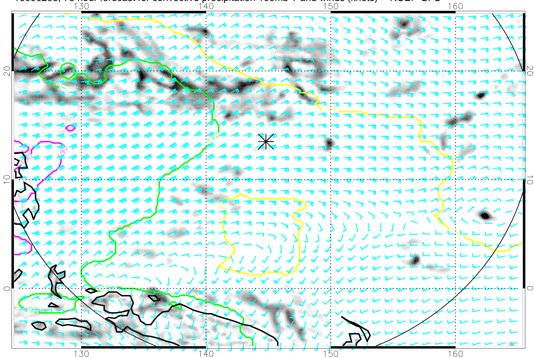
16090206, 78 hour forecast for convective precipitation 100mb T and winds (knots) -- NCEP GFS
