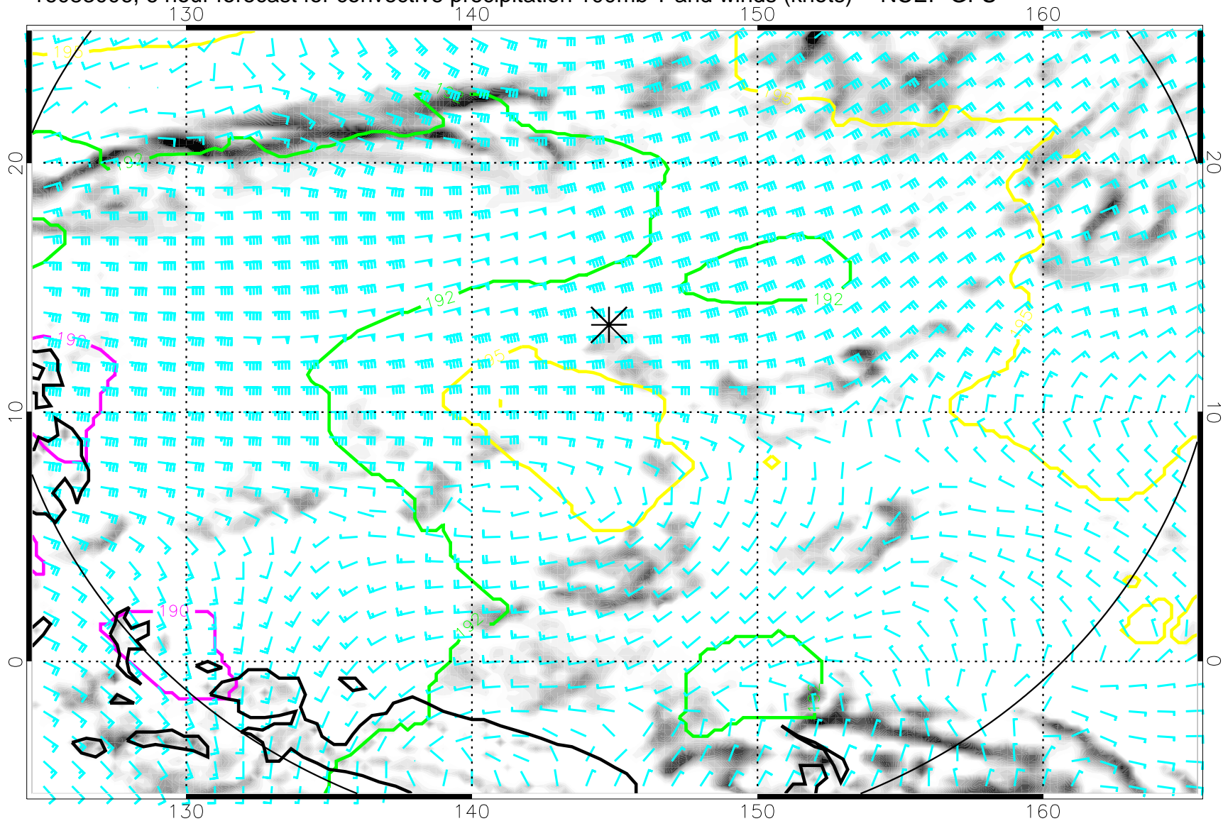
16083006, 6 hour forecast for convective precipitation 100mb T and winds (knots) -- NCEP GFS
