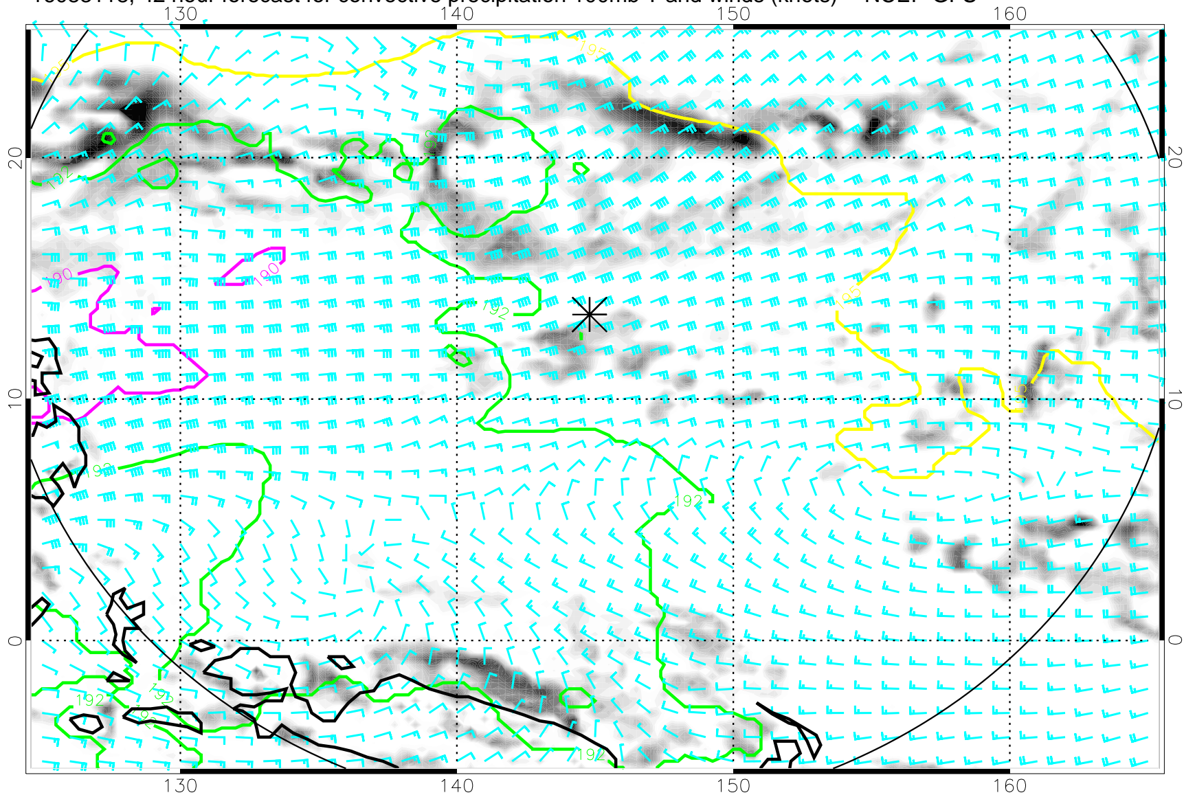
16083118, 42 hour forecast for convective precipitation 100mb T and winds (knots) -- NCEP GFS
