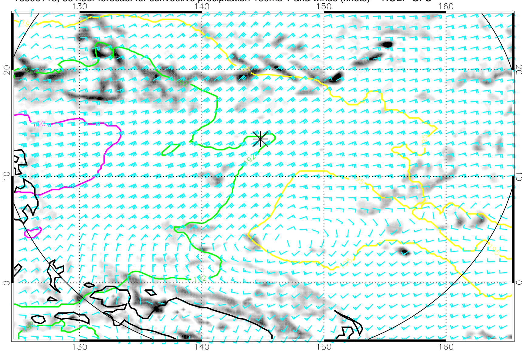
16090118, 66 hour forecast for convective precipitation 100mb T and winds (knots) -- NCEP GFS
