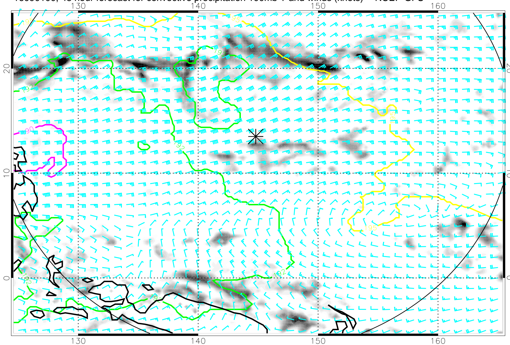
16090100, 48 hour forecast for convective precipitation 100mb T and winds (knots) -- NCEP GFS
