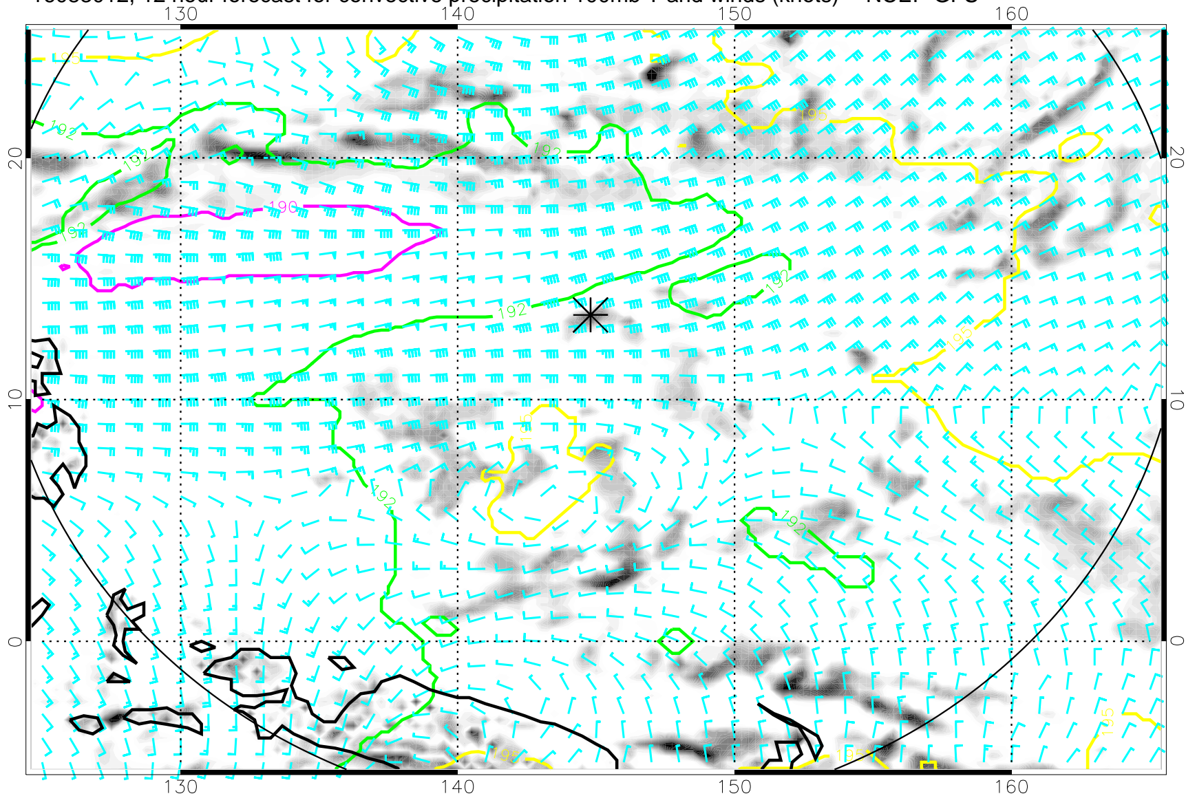
16083012, 12 hour forecast for convective precipitation 100mb T and winds (knots) -- NCEP GFS
