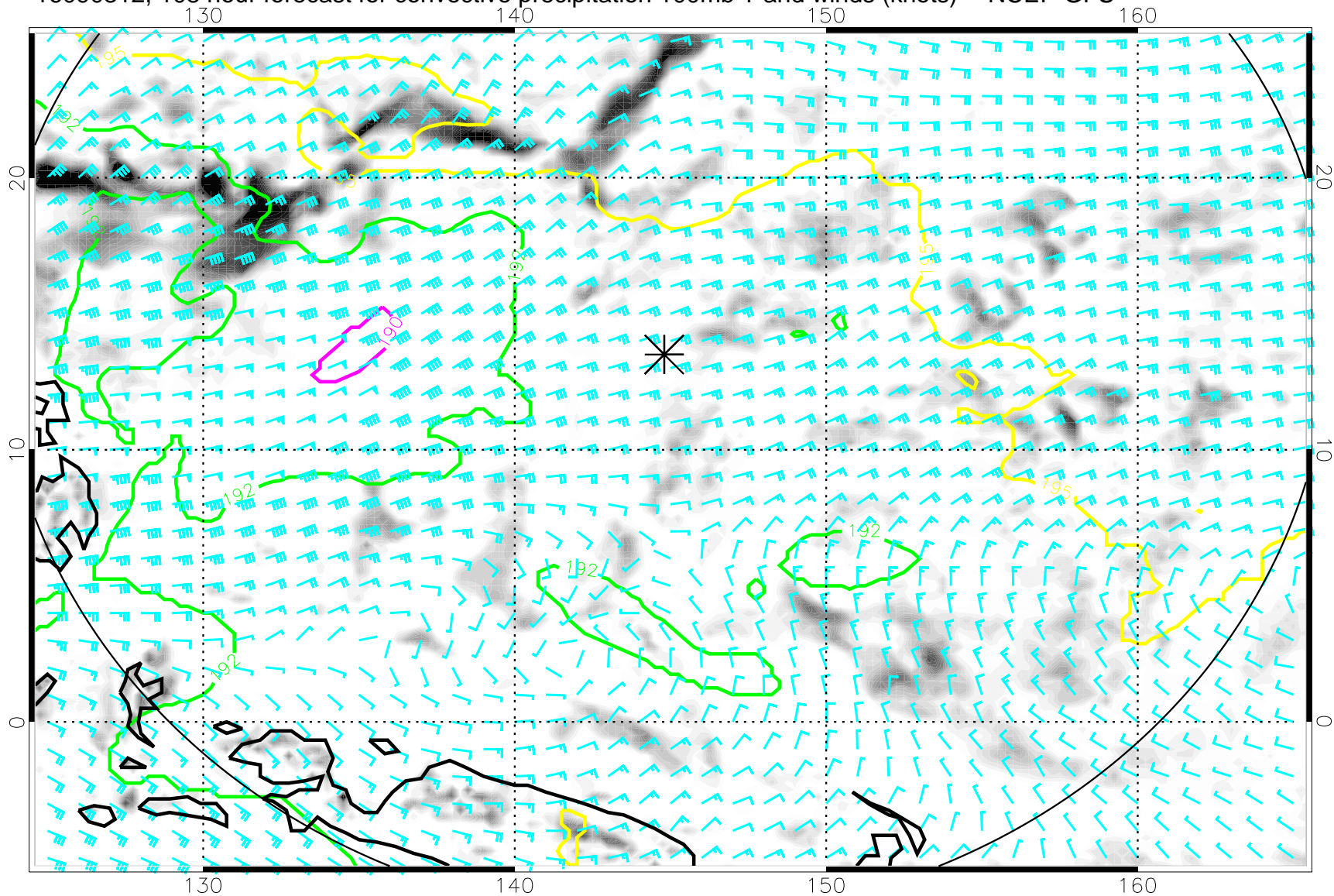
16090312, 108 hour forecast for convective precipitation 100mb T and winds (knots) -- NCEP GFS
