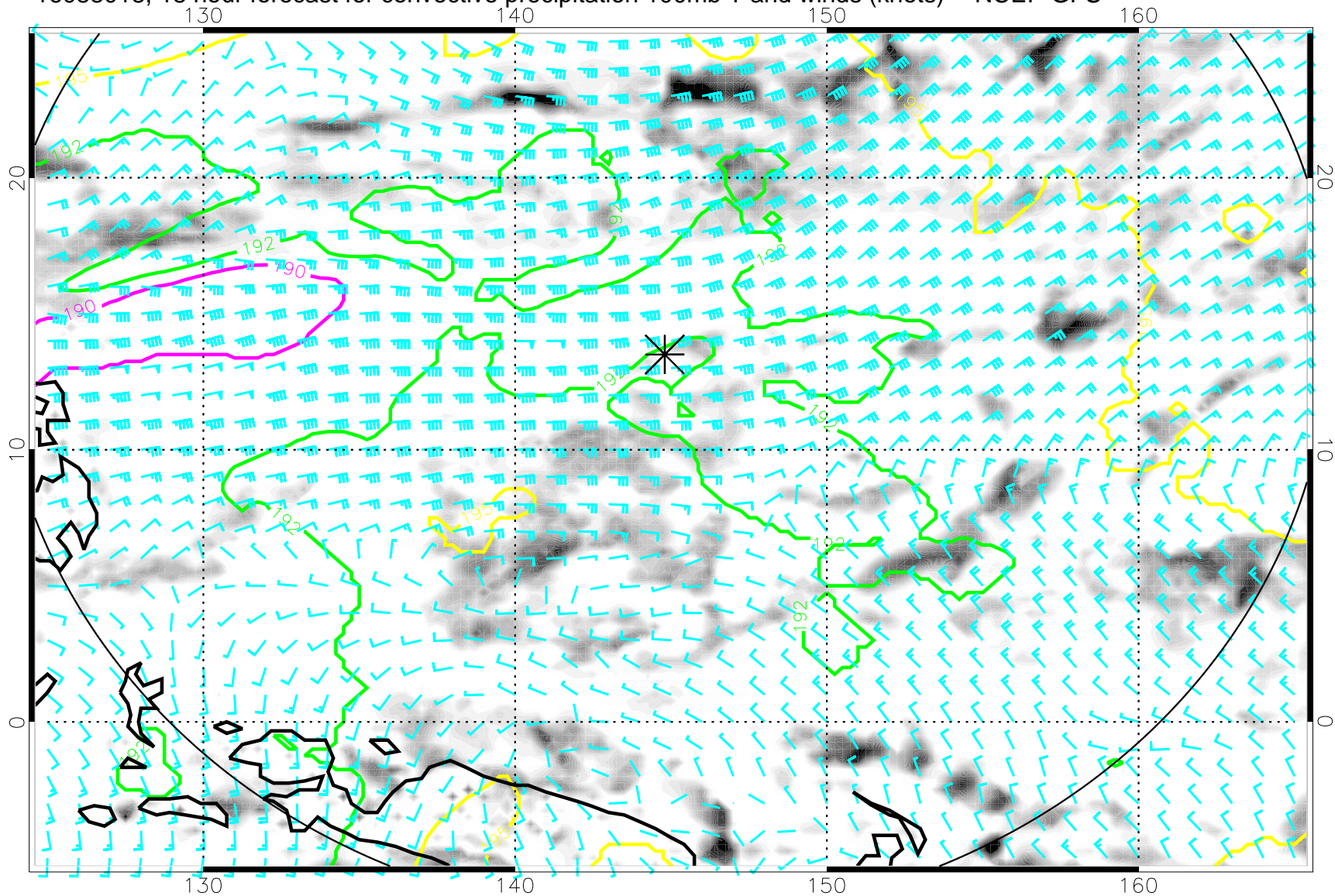
16083018, 18 hour forecast for convective precipitation 100mb T and winds (knots) -- NCEP GFS
