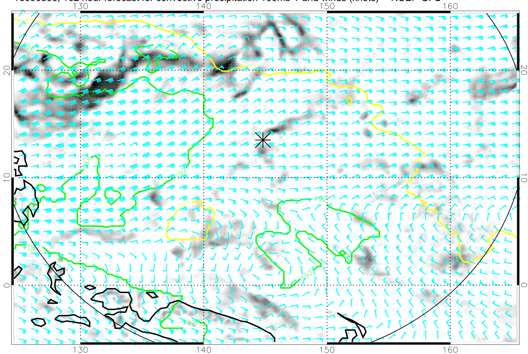
16090306, 102 hour forecast for convective precipitation 100mb T and winds (knots) -- NCEP GFS
