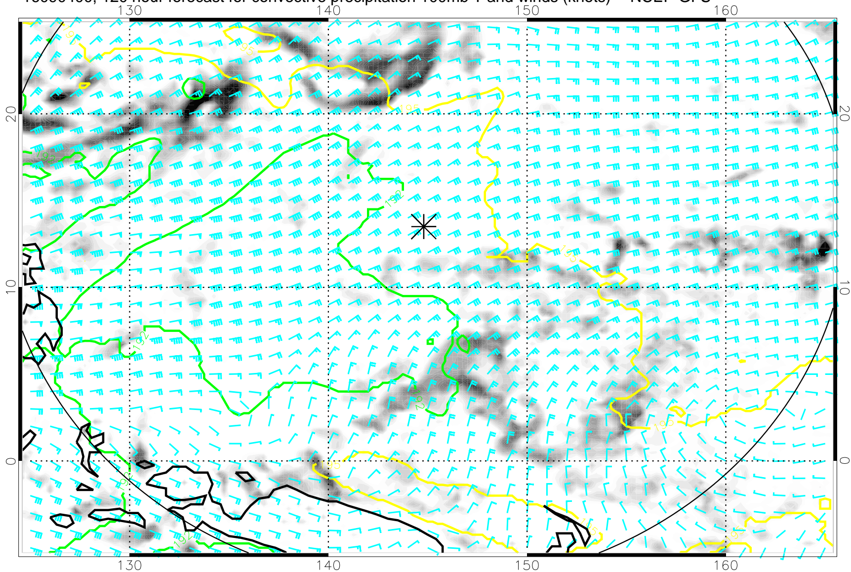
16090400, 120 hour forecast for convective precipitation 100mb T and winds (knots) -- NCEP GFS
