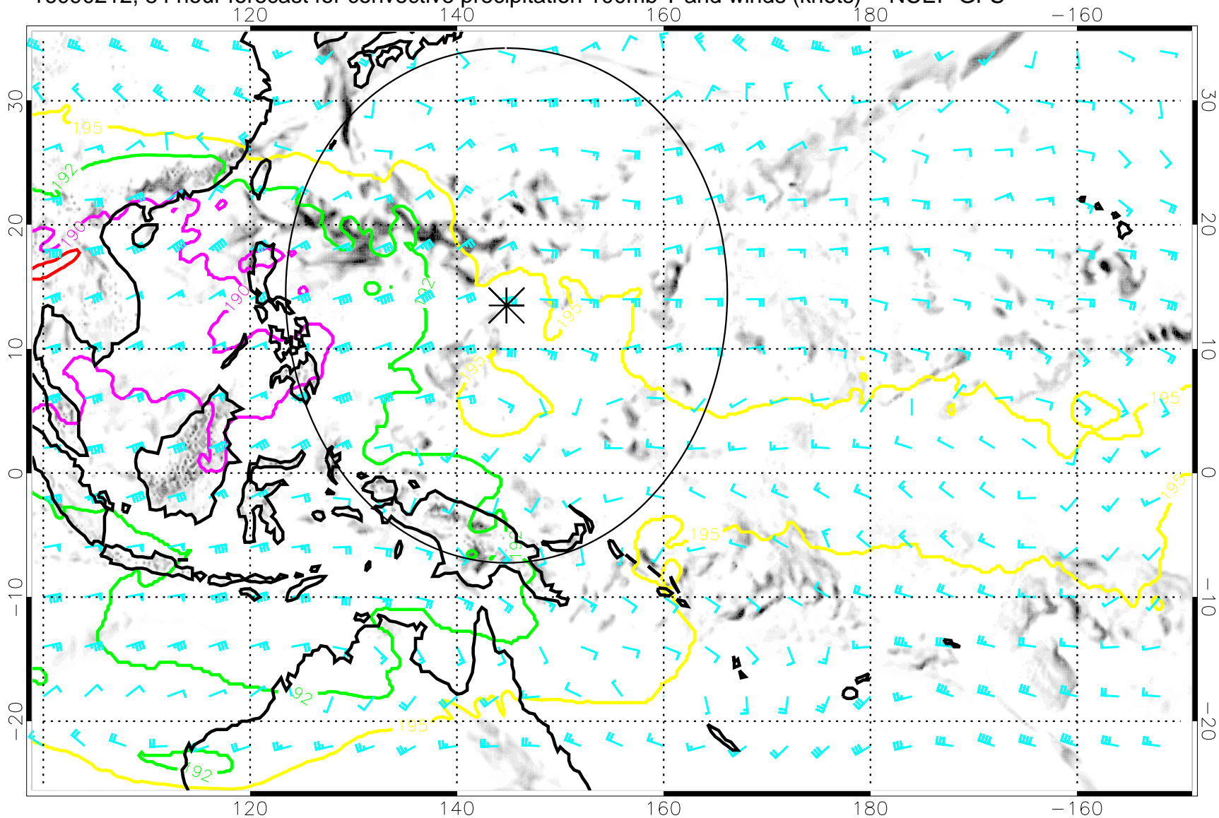
16090212, 84 hour forecast for convective precipitation 100mb T and winds (knots) -- NCEP GFS
