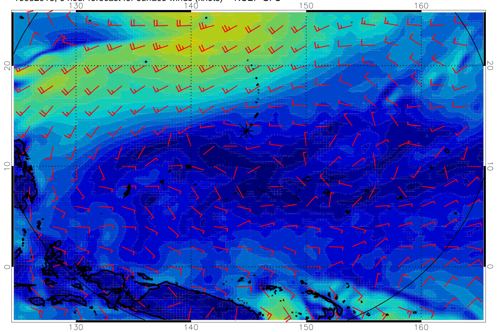
16082918, 6 hour forecast for surface winds (knots) -- NCEP GFS
