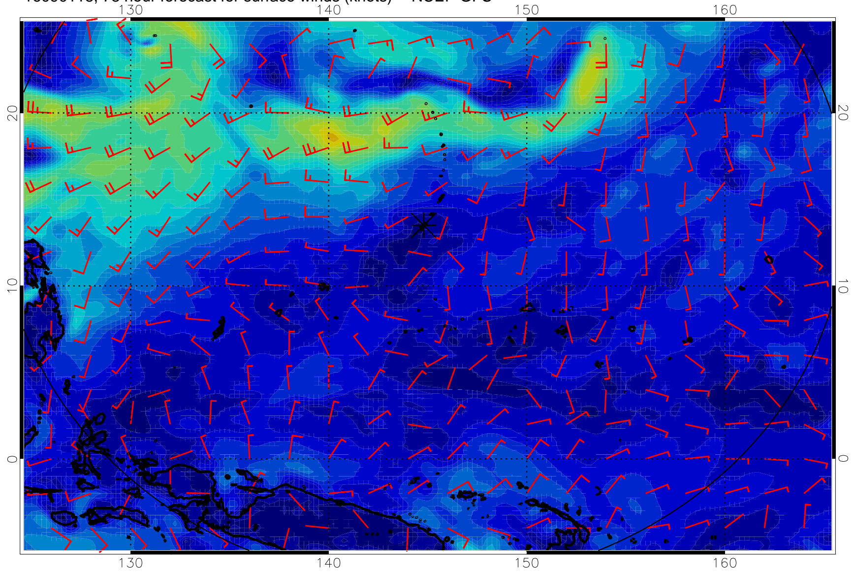
16090118, 78 hour forecast for surface winds (knots) -- NCEP GFS
