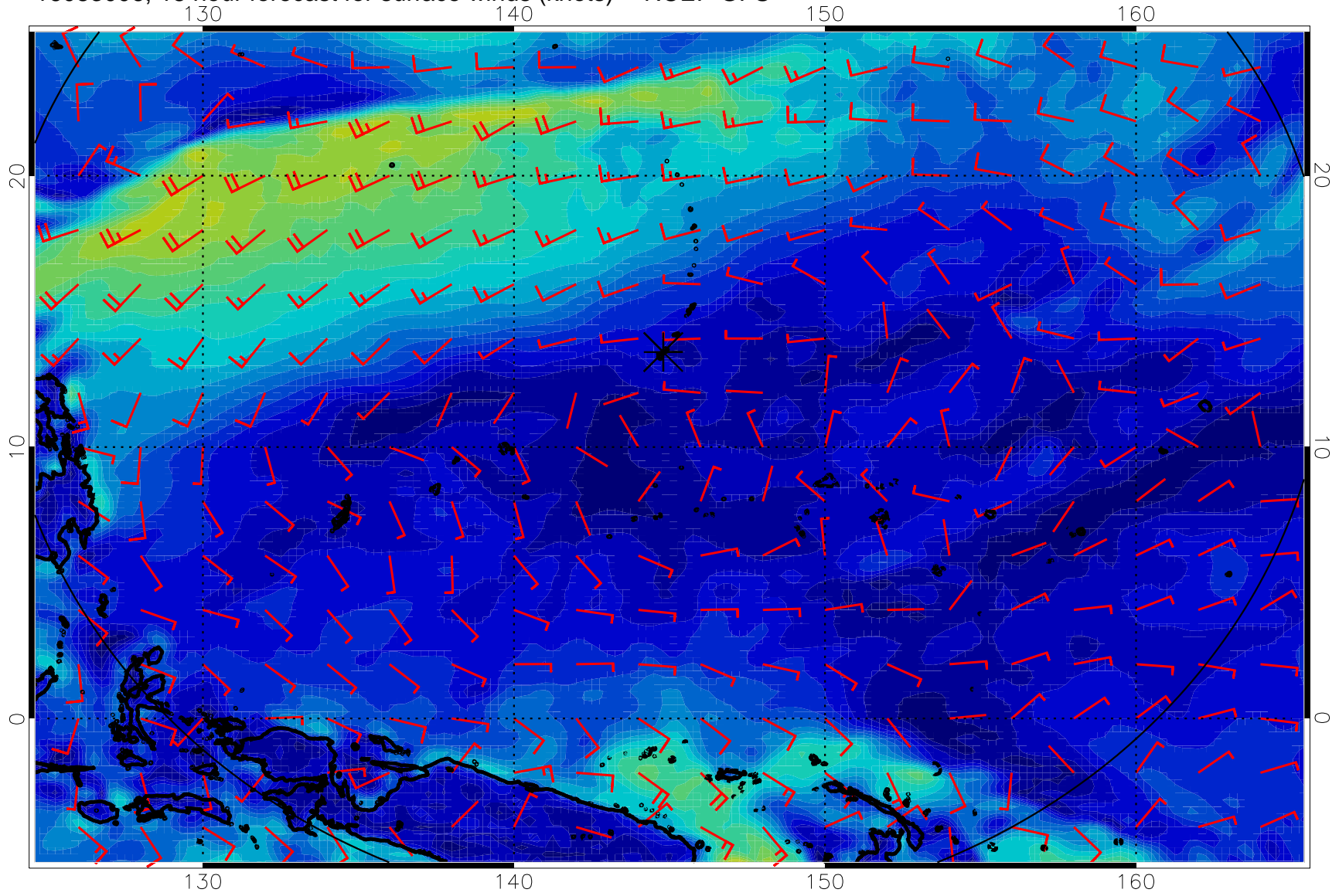
16083006, 18 hour forecast for surface winds (knots) -- NCEP GFS
