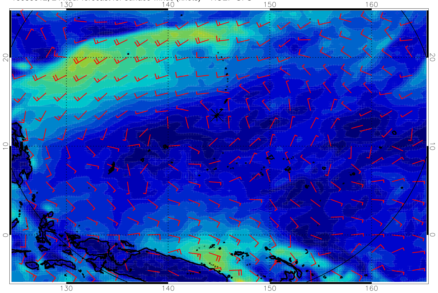
16083012, 24 hour forecast for surface winds (knots) -- NCEP GFS
