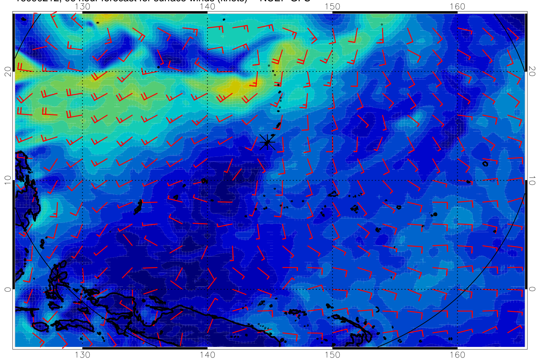
16090212, 96 hour forecast for surface winds (knots) -- NCEP GFS
