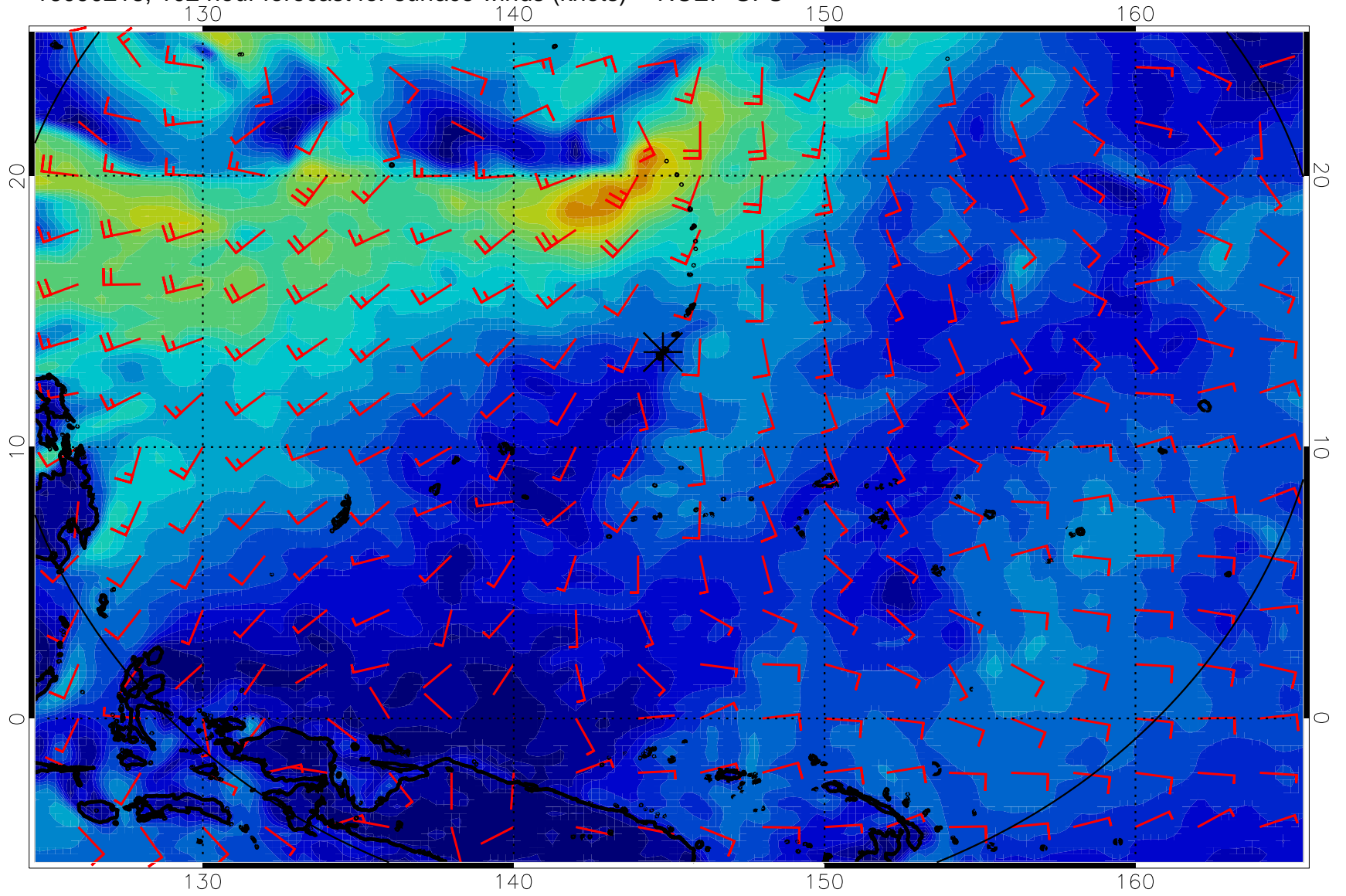
16090218, 102 hour forecast for surface winds (knots) -- NCEP GFS
