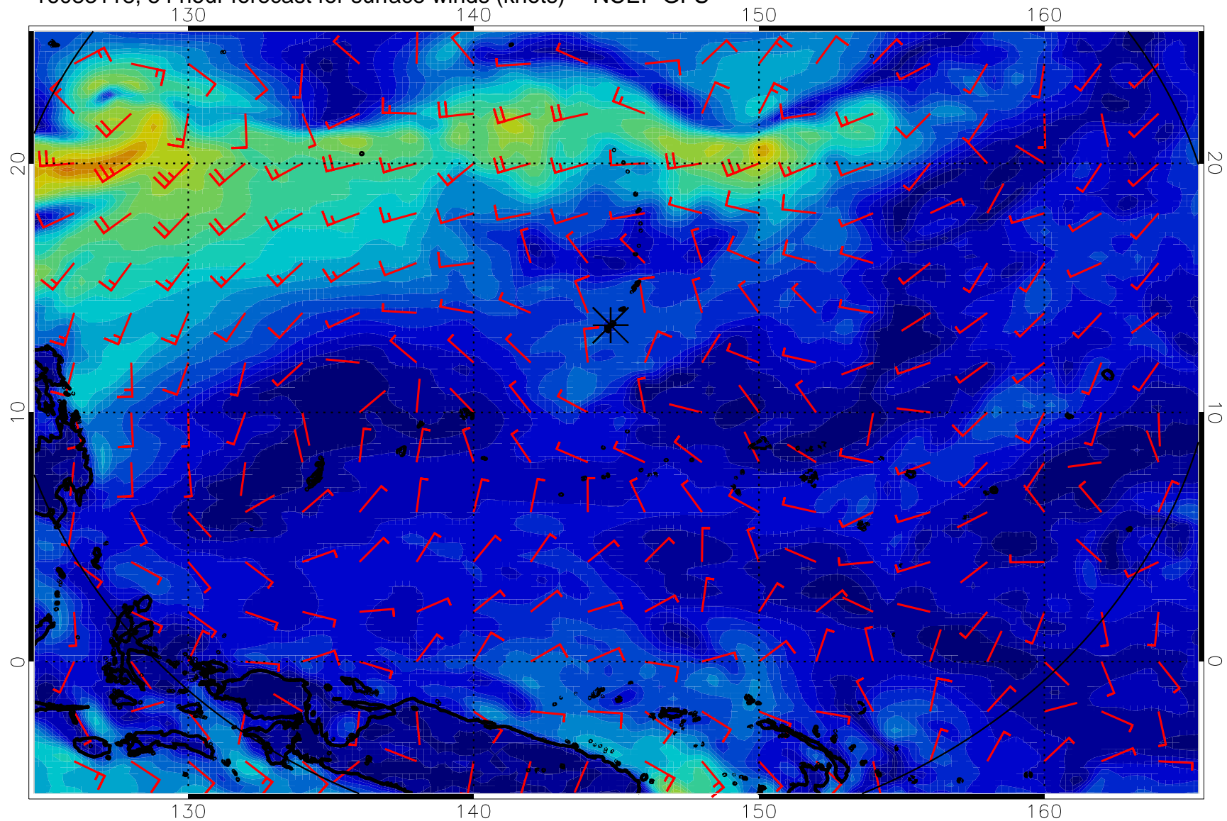
16083118, 54 hour forecast for surface winds (knots) -- NCEP GFS
