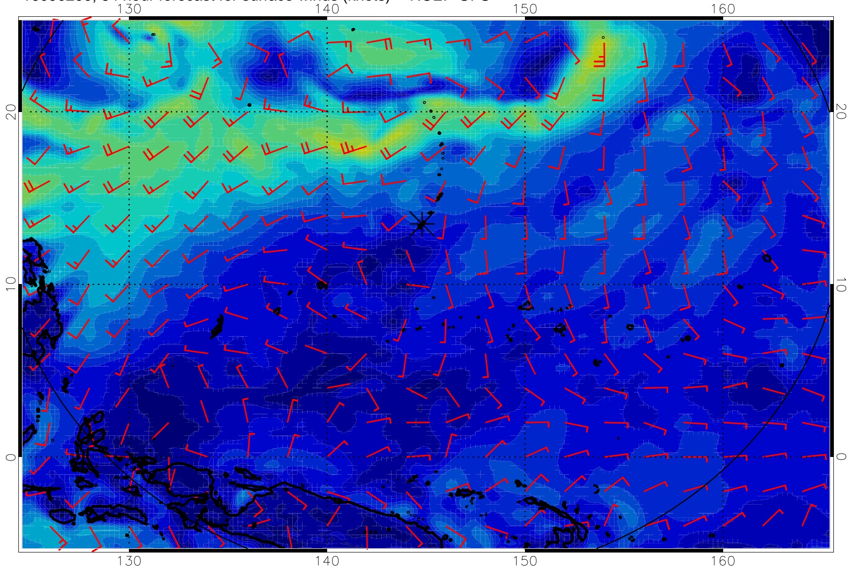
16090200, 84 hour forecast for surface winds (knots) -- NCEP GFS
