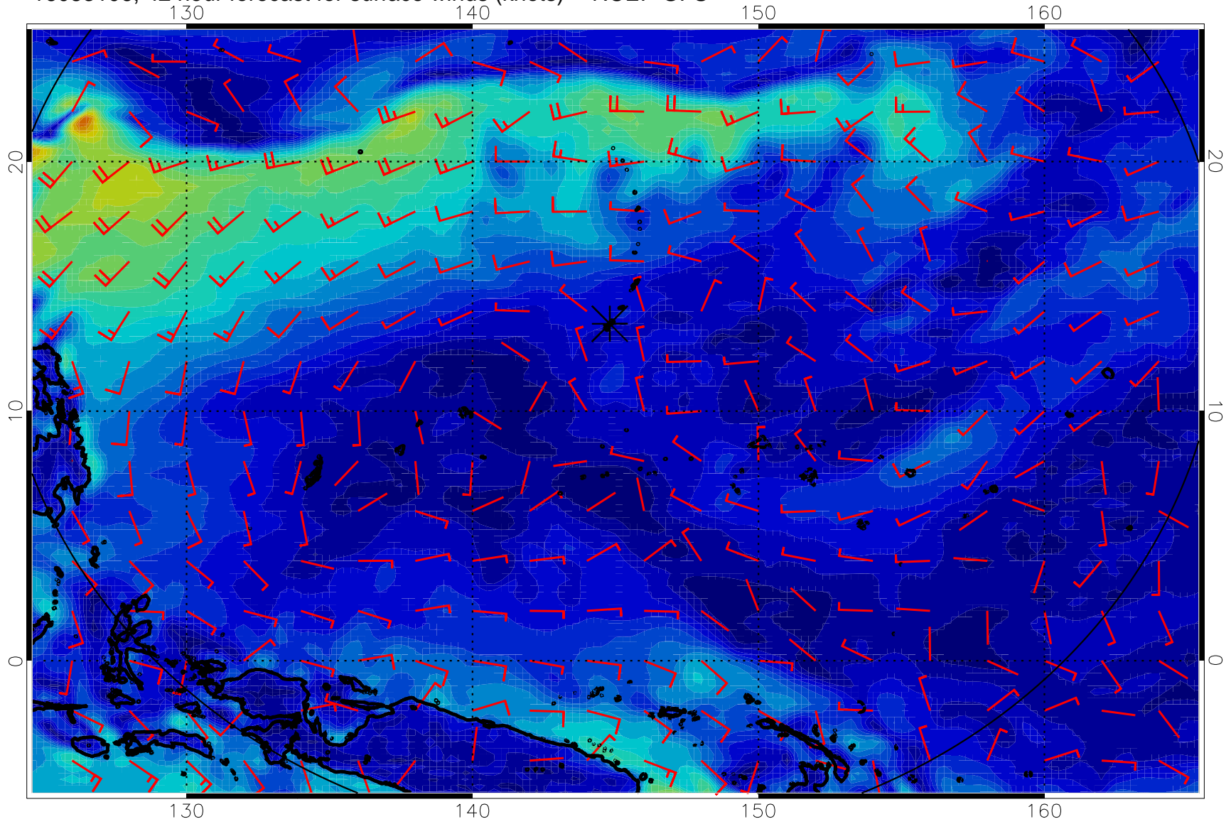
16083106, 42 hour forecast for surface winds (knots) -- NCEP GFS
