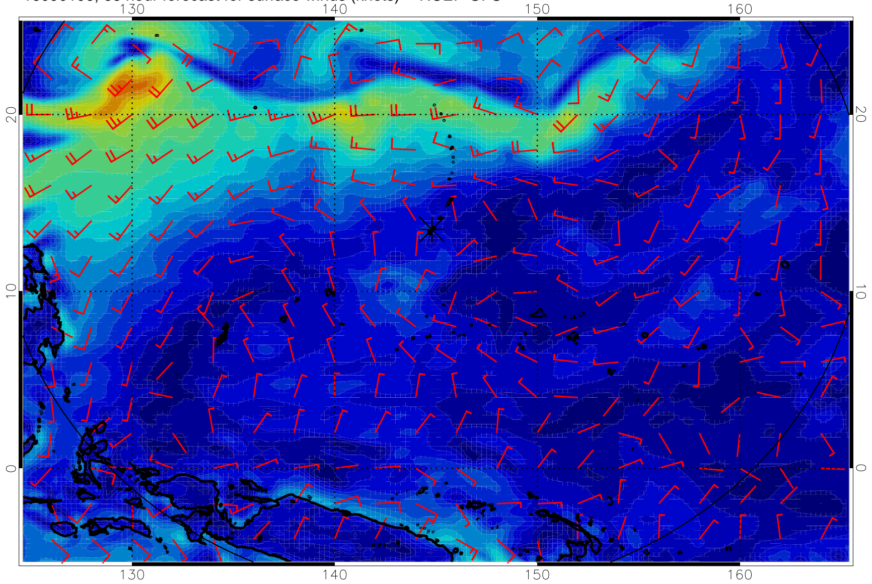
16090106, 66 hour forecast for surface winds (knots) -- NCEP GFS
