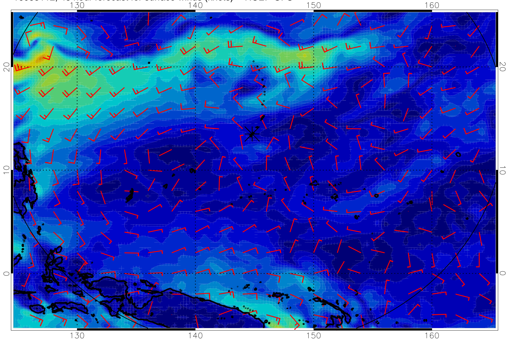
16083112, 48 hour forecast for surface winds (knots) -- NCEP GFS
