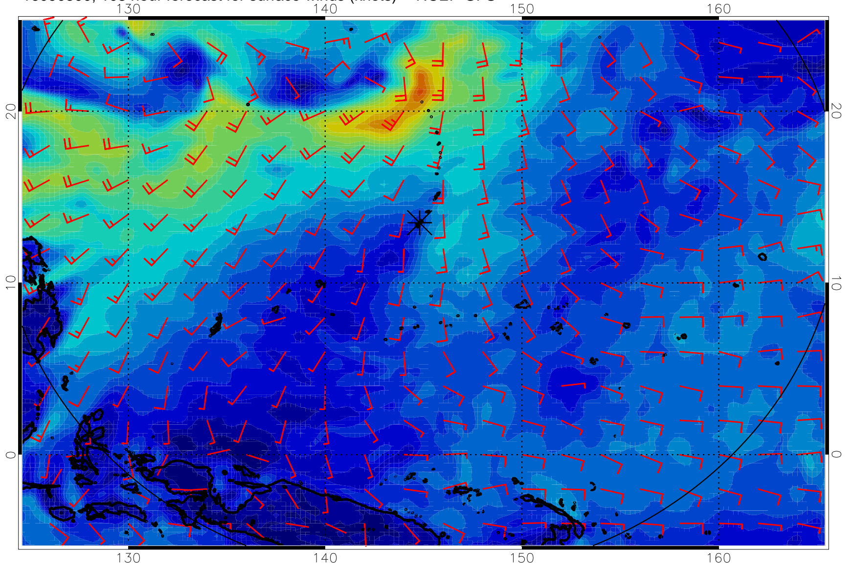
16090300, 108 hour forecast for surface winds (knots) -- NCEP GFS
