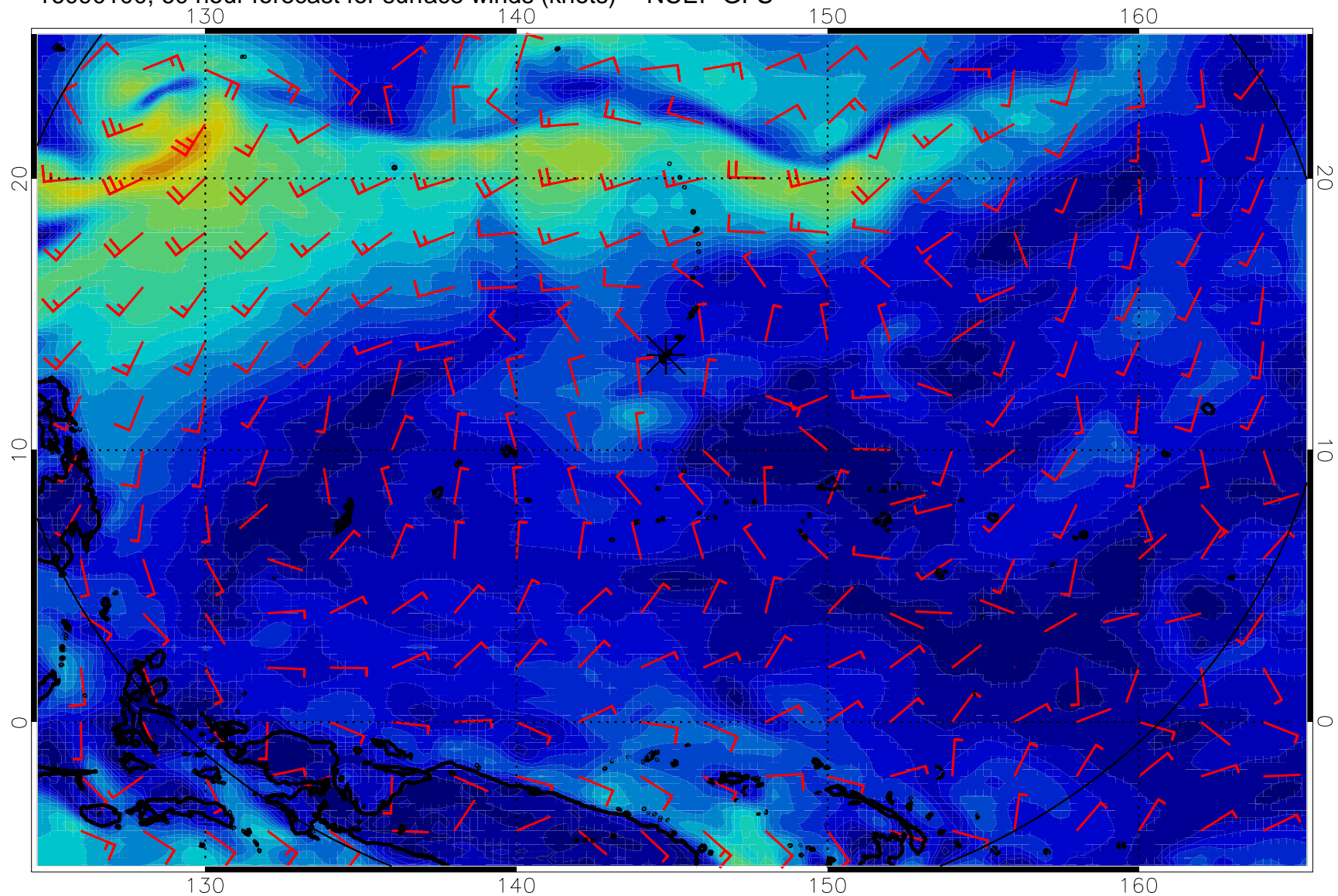
16090100, 60 hour forecast for surface winds (knots) -- NCEP GFS
