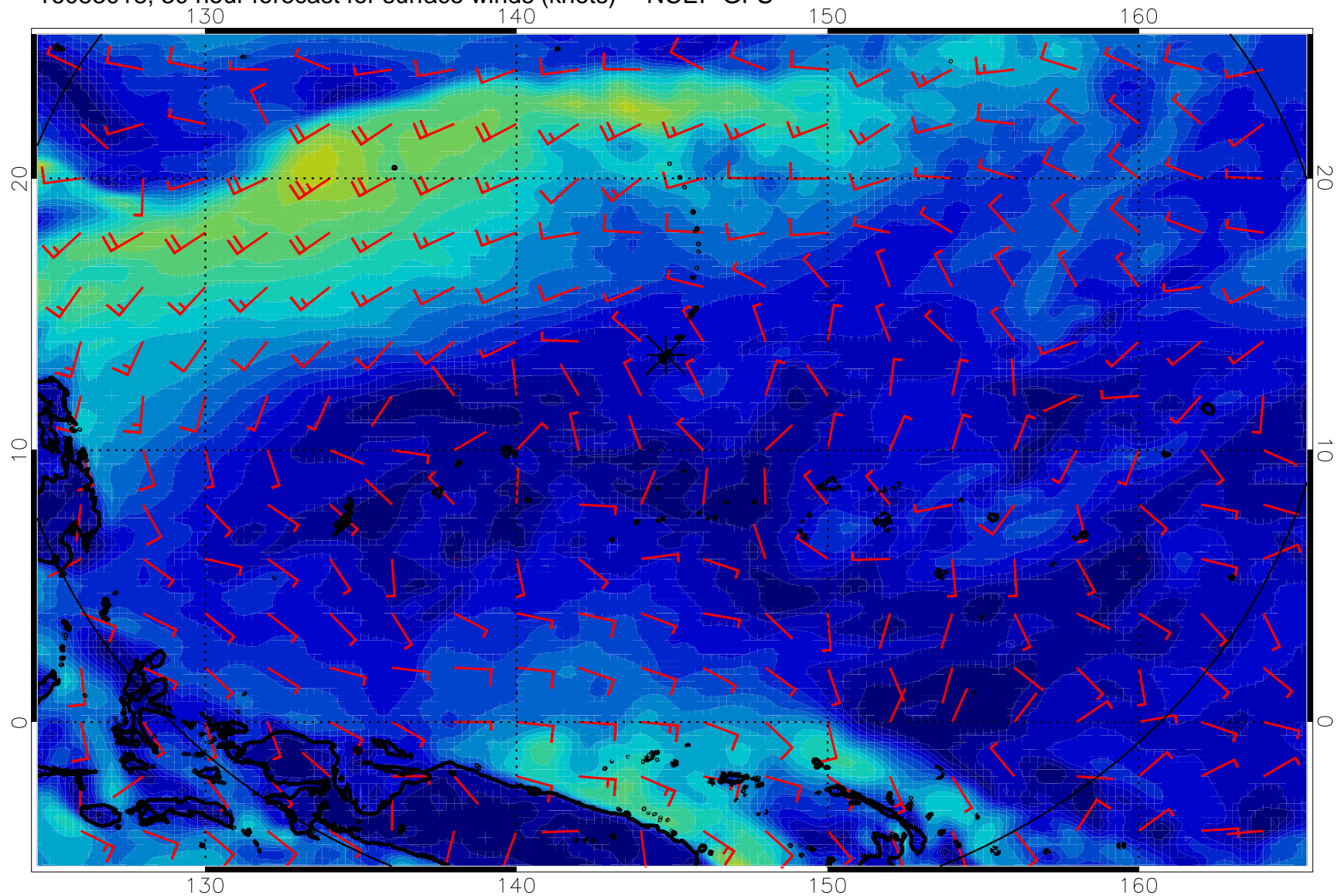
16083018, 30 hour forecast for surface winds (knots) -- NCEP GFS
