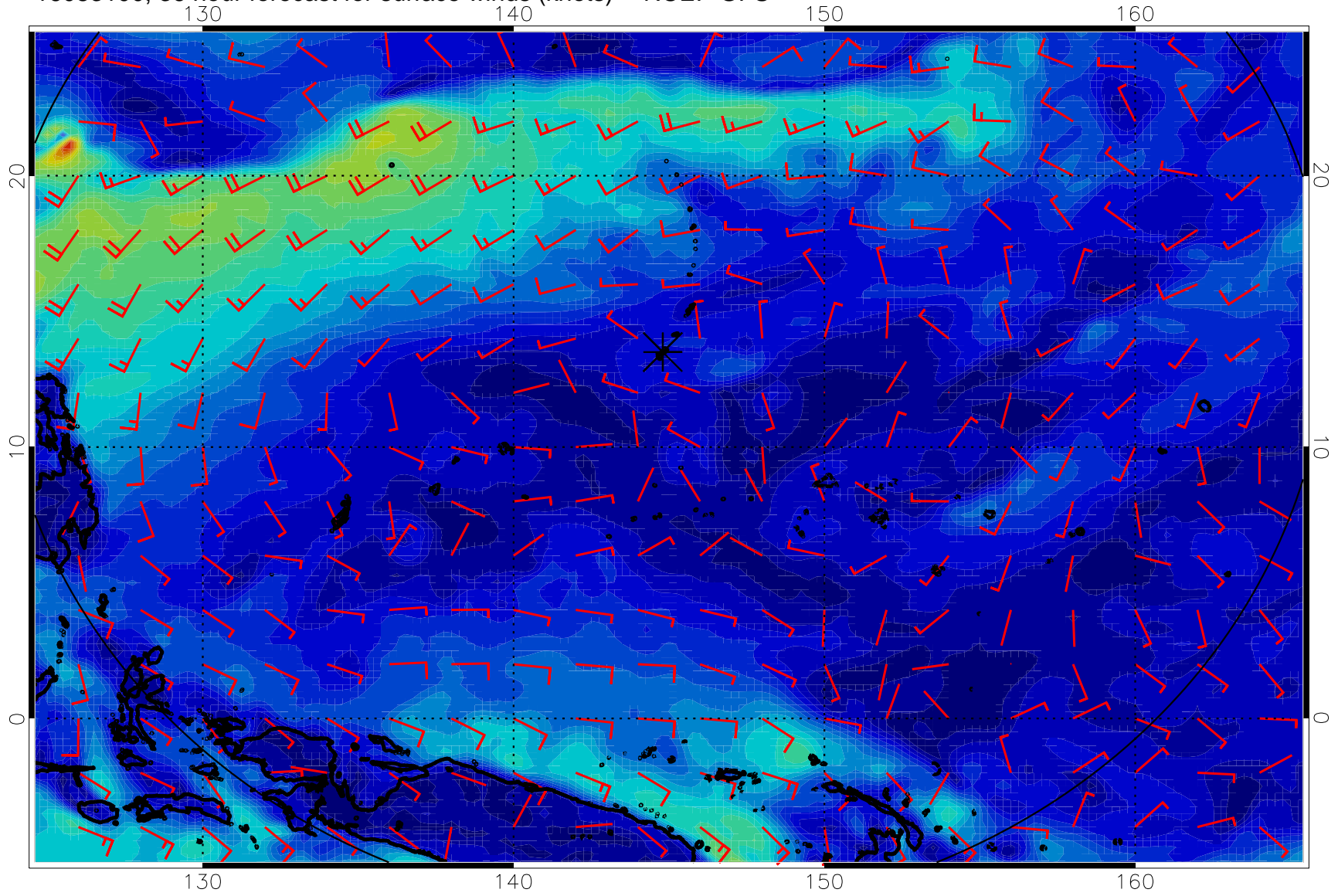
16083100, 36 hour forecast for surface winds (knots) -- NCEP GFS
