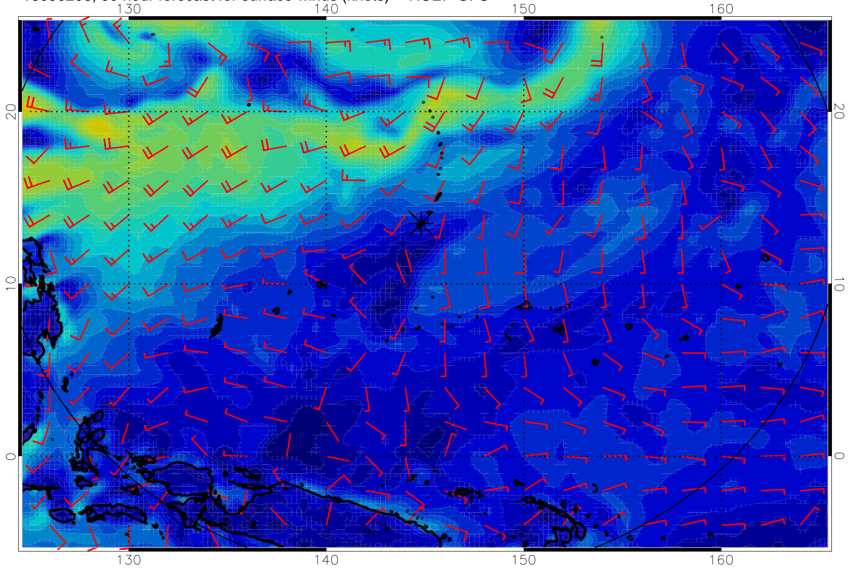
16090206, 90 hour forecast for surface winds (knots) -- NCEP GFS
