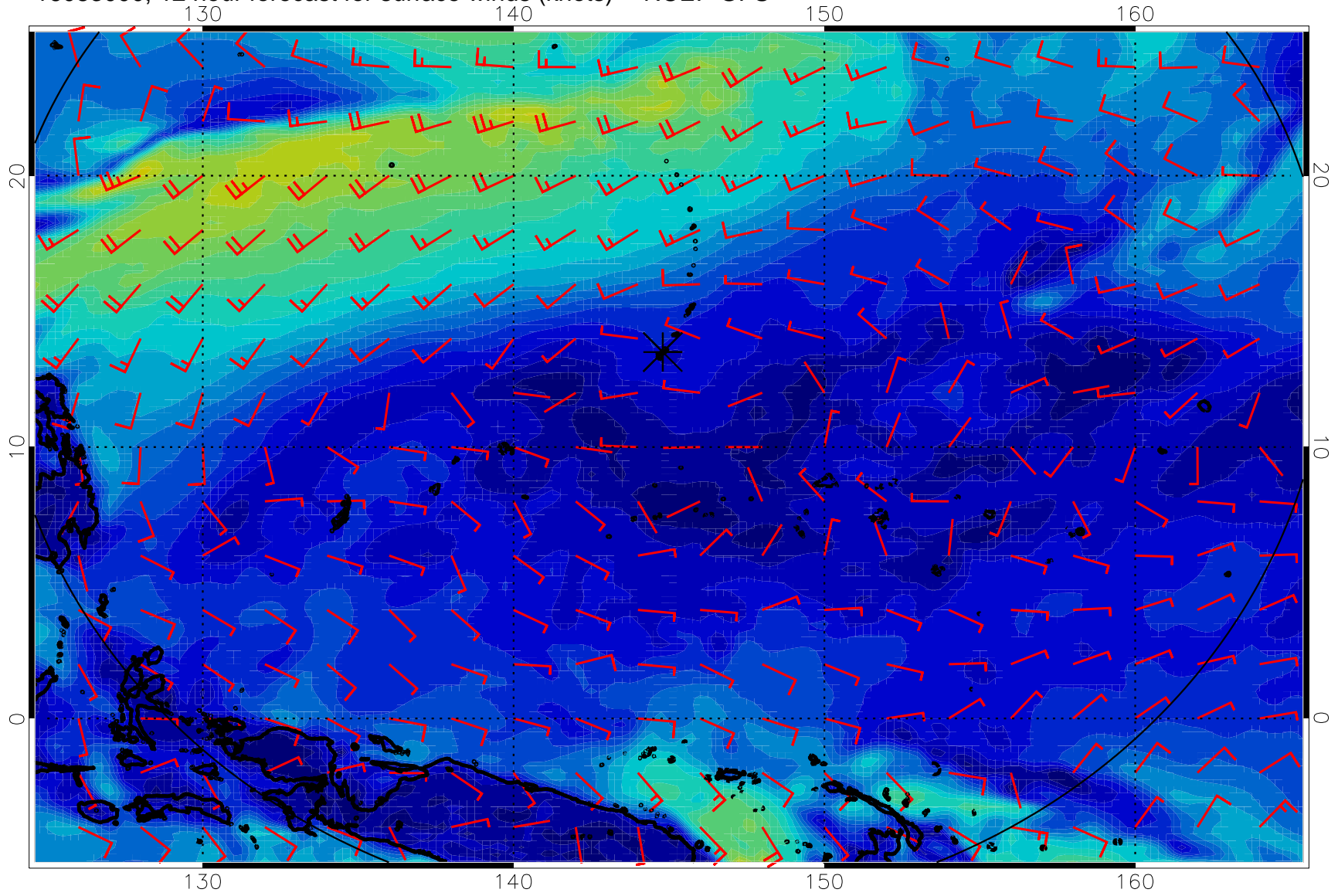
16083000, 12 hour forecast for surface winds (knots) -- NCEP GFS
