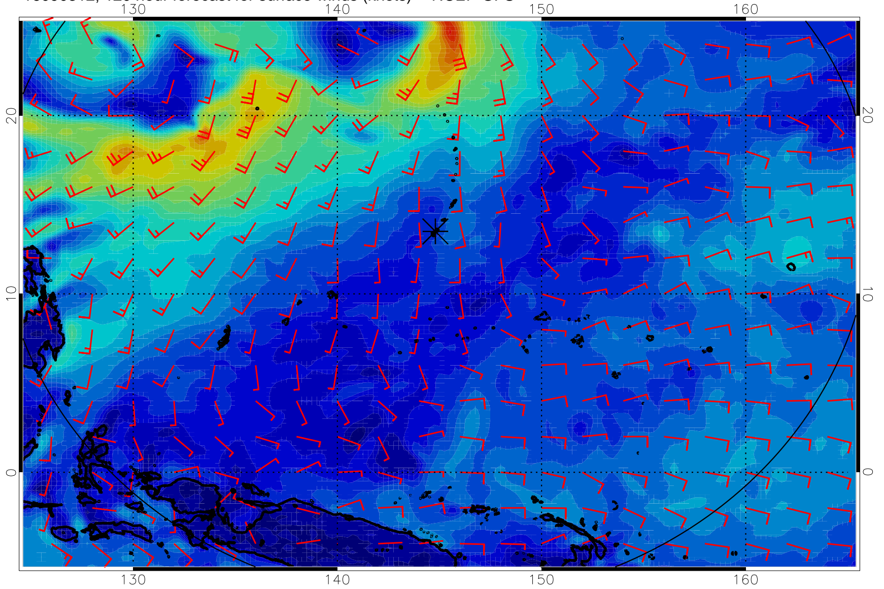
16090312, 120 hour forecast for surface winds (knots) -- NCEP GFS
