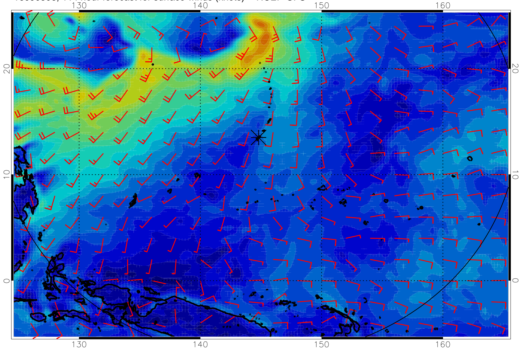
16090306, 114 hour forecast for surface winds (knots) -- NCEP GFS
