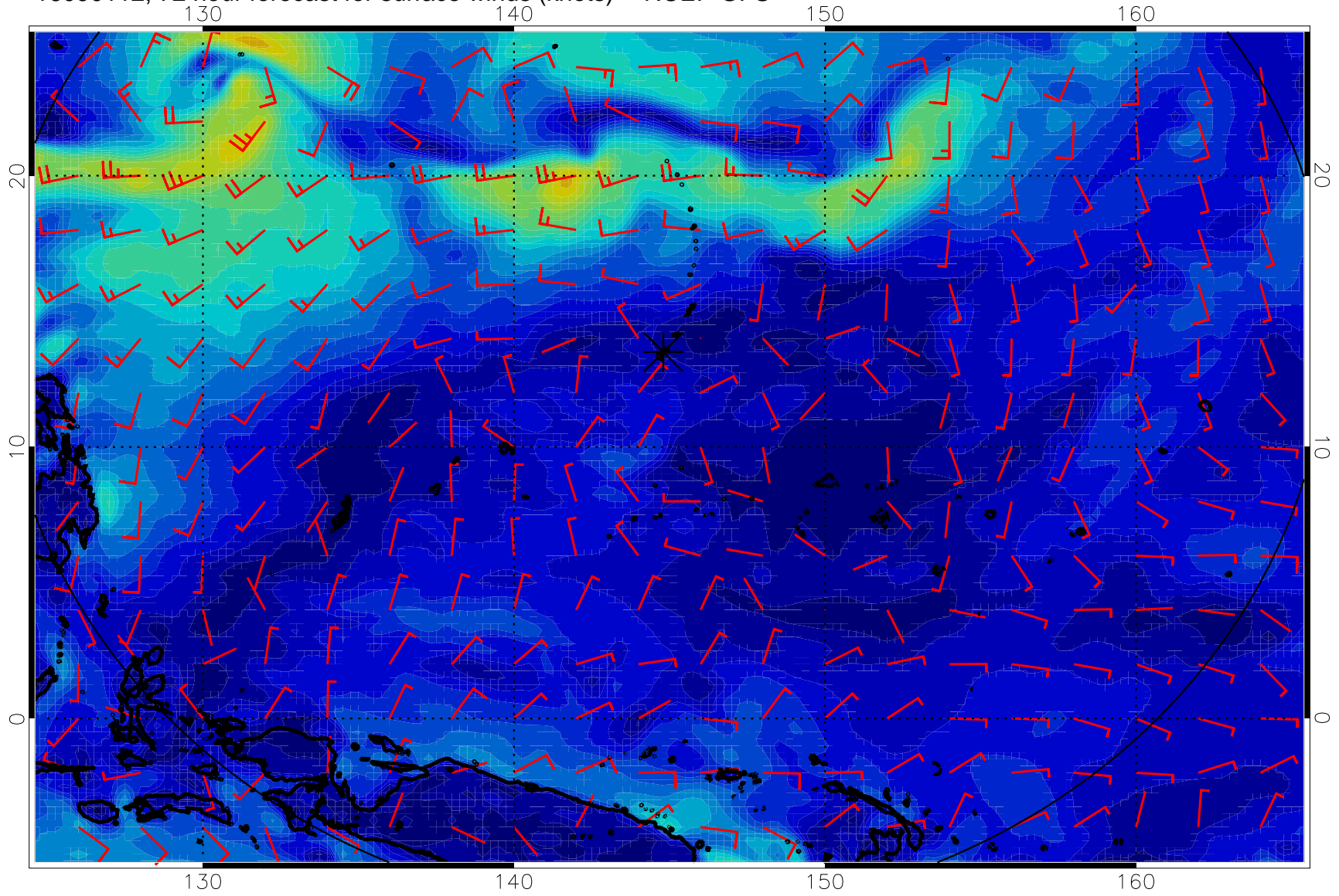
16090112, 72 hour forecast for surface winds (knots) -- NCEP GFS
