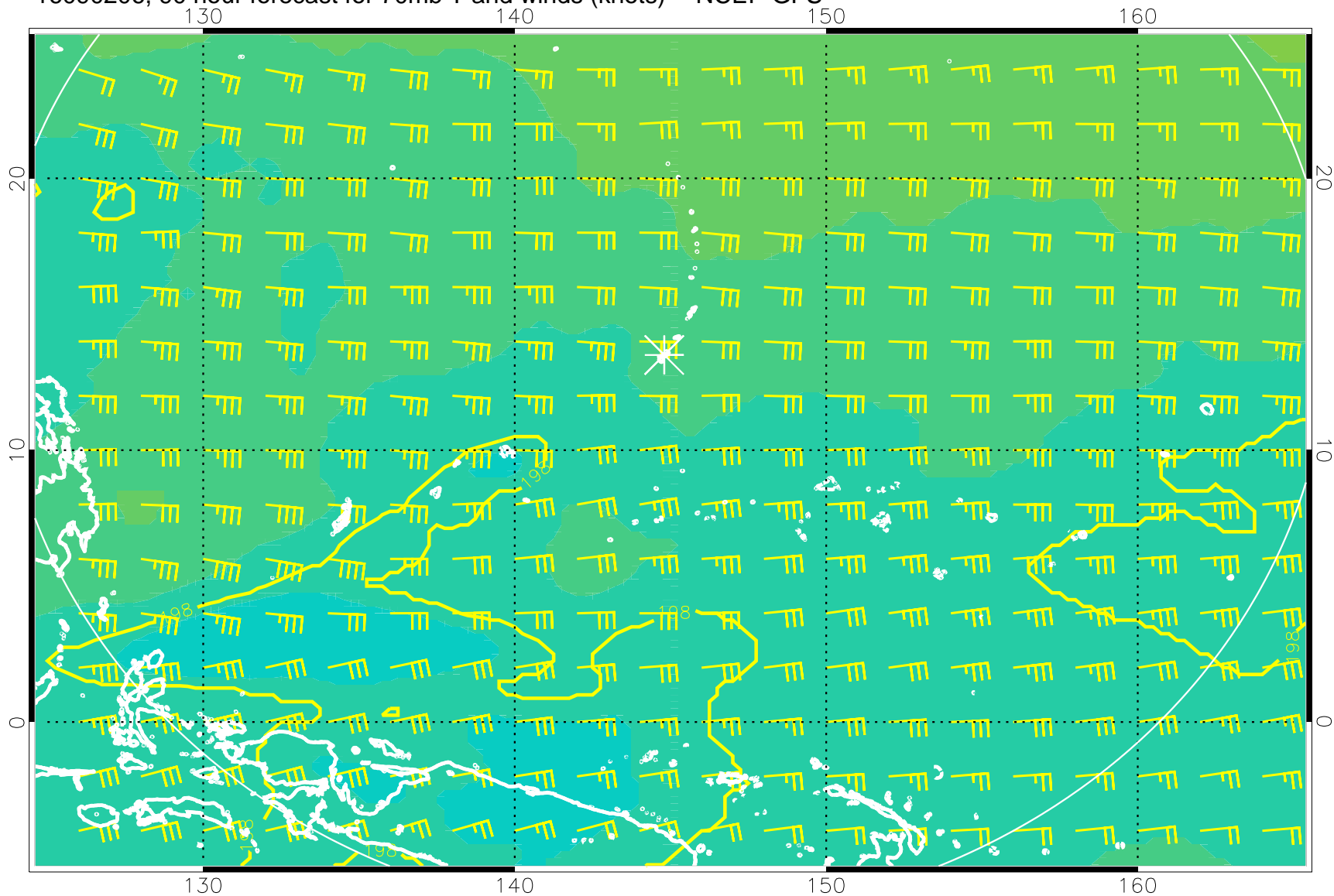
16090206, 90 hour forecast for 70mb T and winds (knots) -- NCEP GFS
