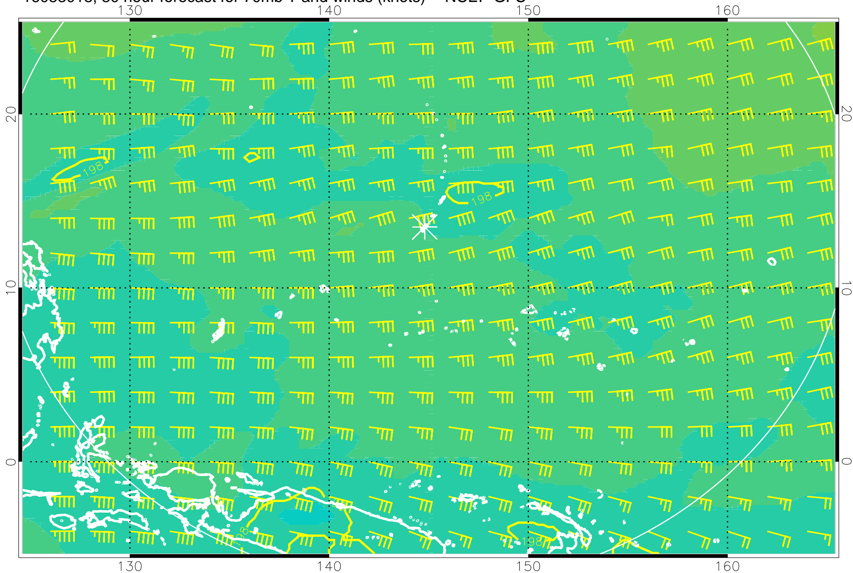
16083018, 30 hour forecast for 70mb T and winds (knots) -- NCEP GFS
