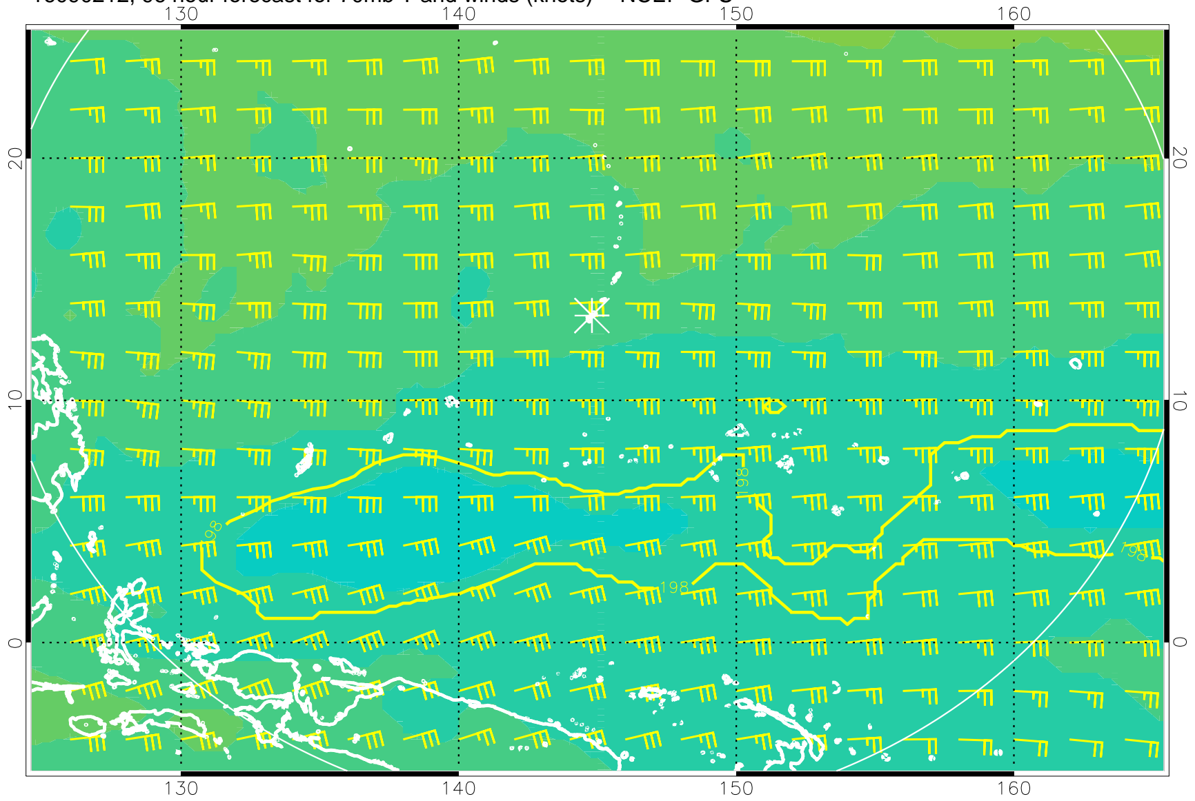
16090212, 96 hour forecast for 70mb T and winds (knots) -- NCEP GFS
