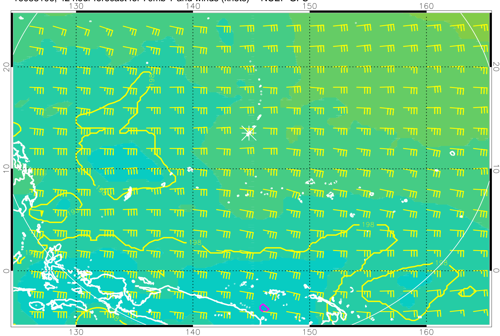
16083106, 42 hour forecast for 70mb T and winds (knots) -- NCEP GFS
