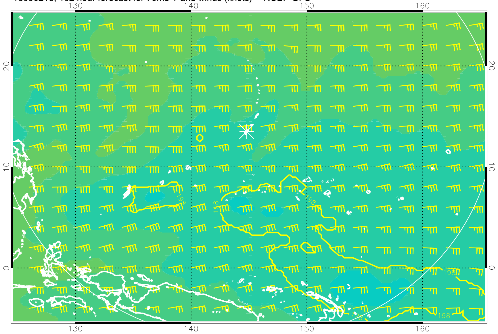
16090218, 102 hour forecast for 70mb T and winds (knots) -- NCEP GFS
