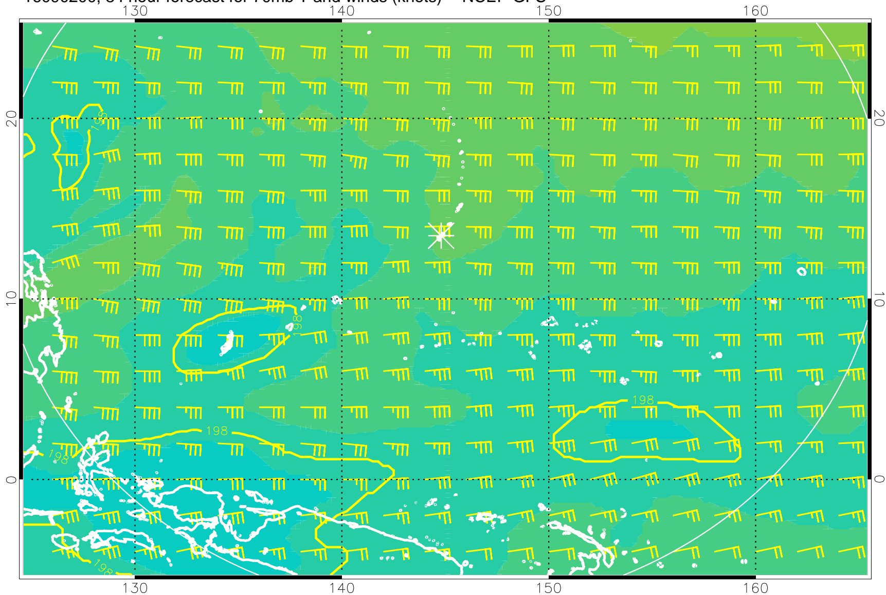
16090200, 84 hour forecast for 70mb T and winds (knots) -- NCEP GFS
