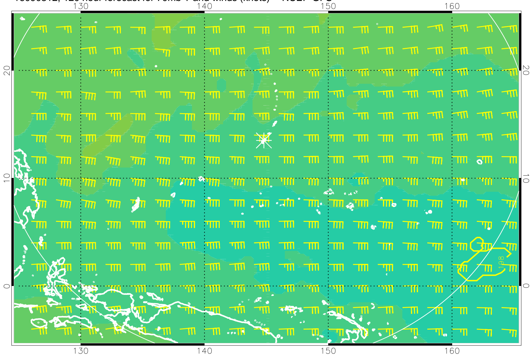
16090312, 120 hour forecast for 70mb T and winds (knots) -- NCEP GFS
