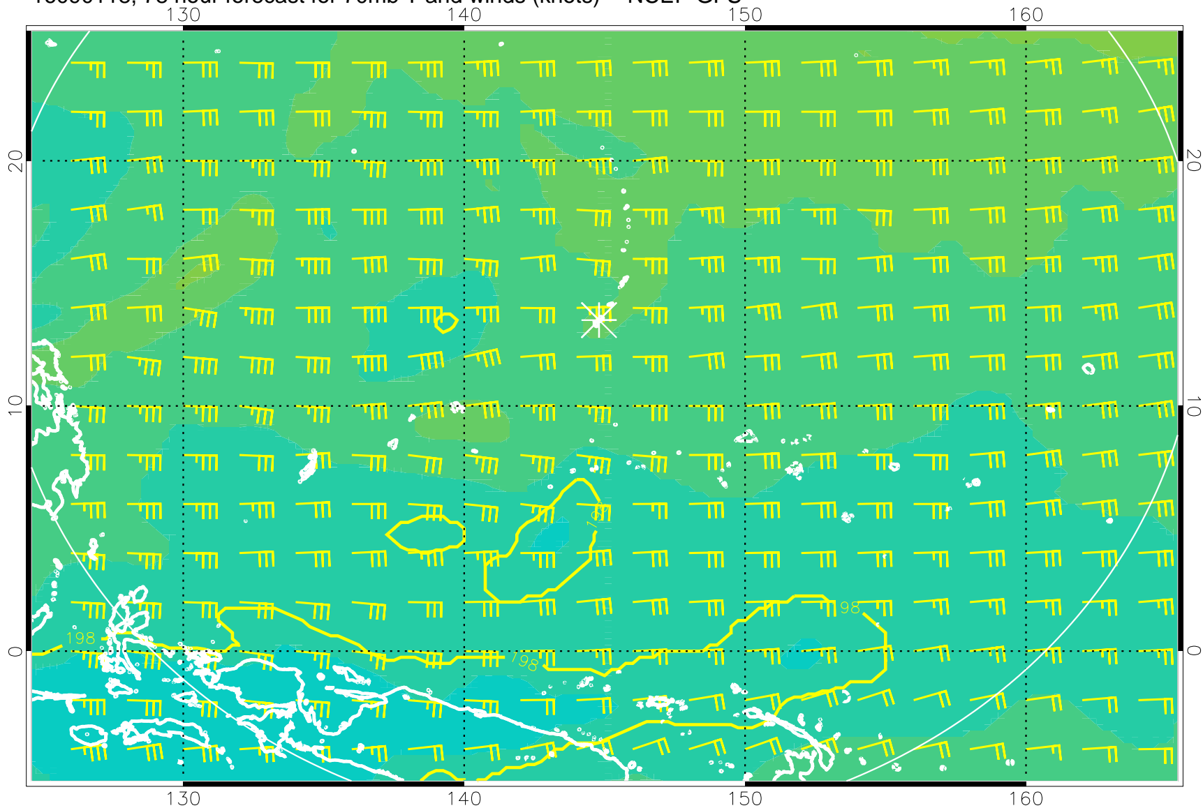
16090118, 78 hour forecast for 70mb T and winds (knots) -- NCEP GFS
