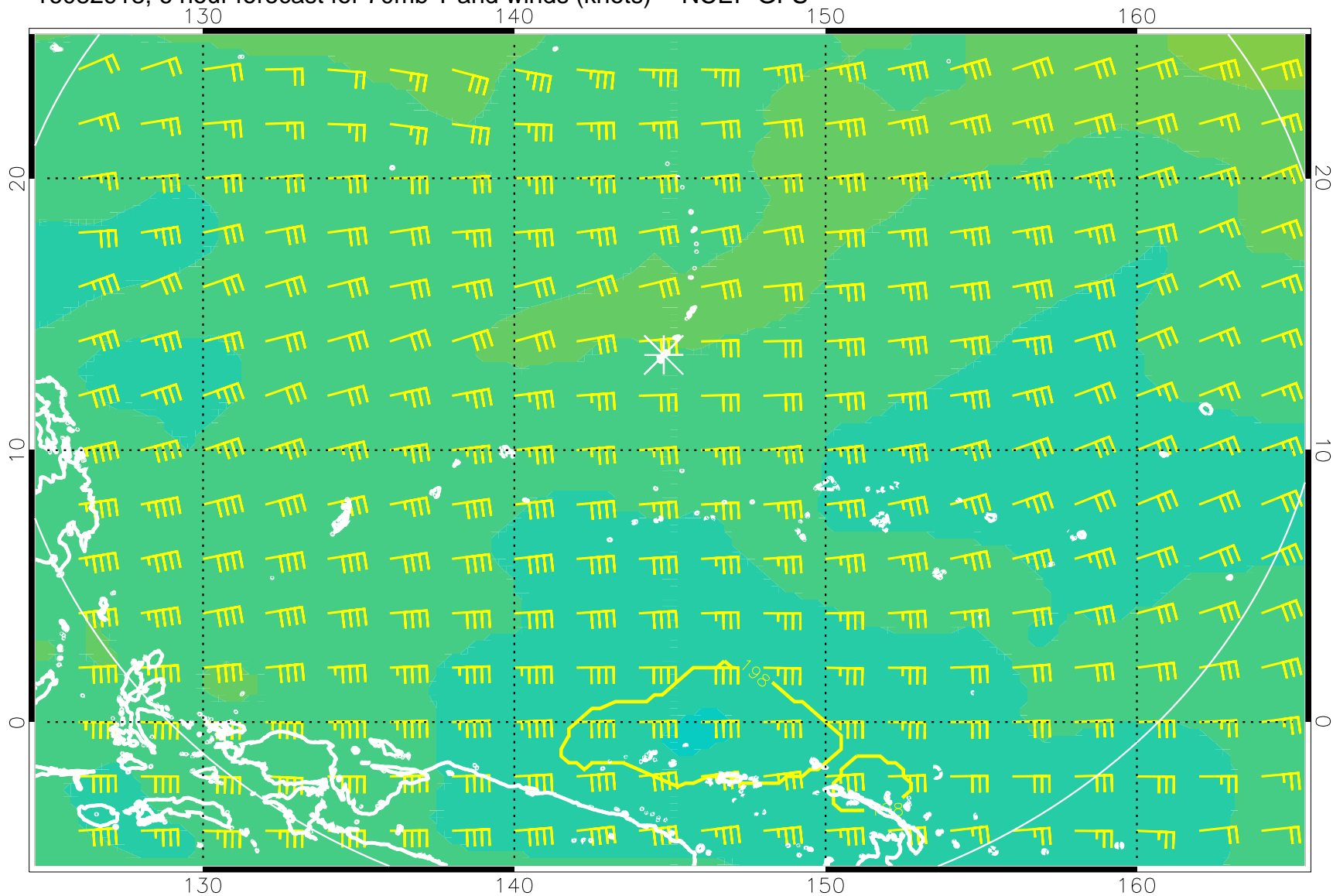
16082918, 6 hour forecast for 70mb T and winds (knots) -- NCEP GFS
