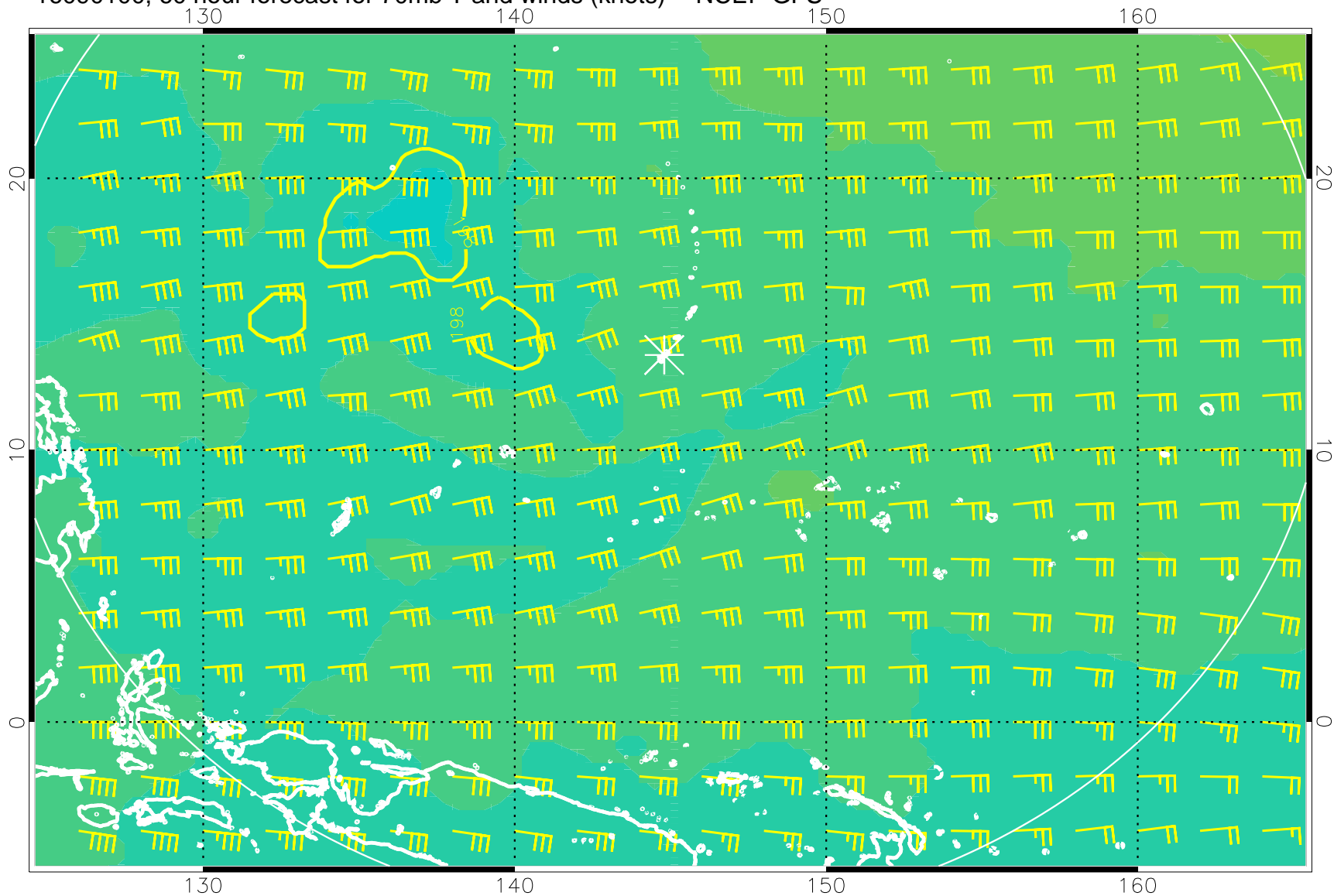
16090100, 60 hour forecast for 70mb T and winds (knots) -- NCEP GFS
