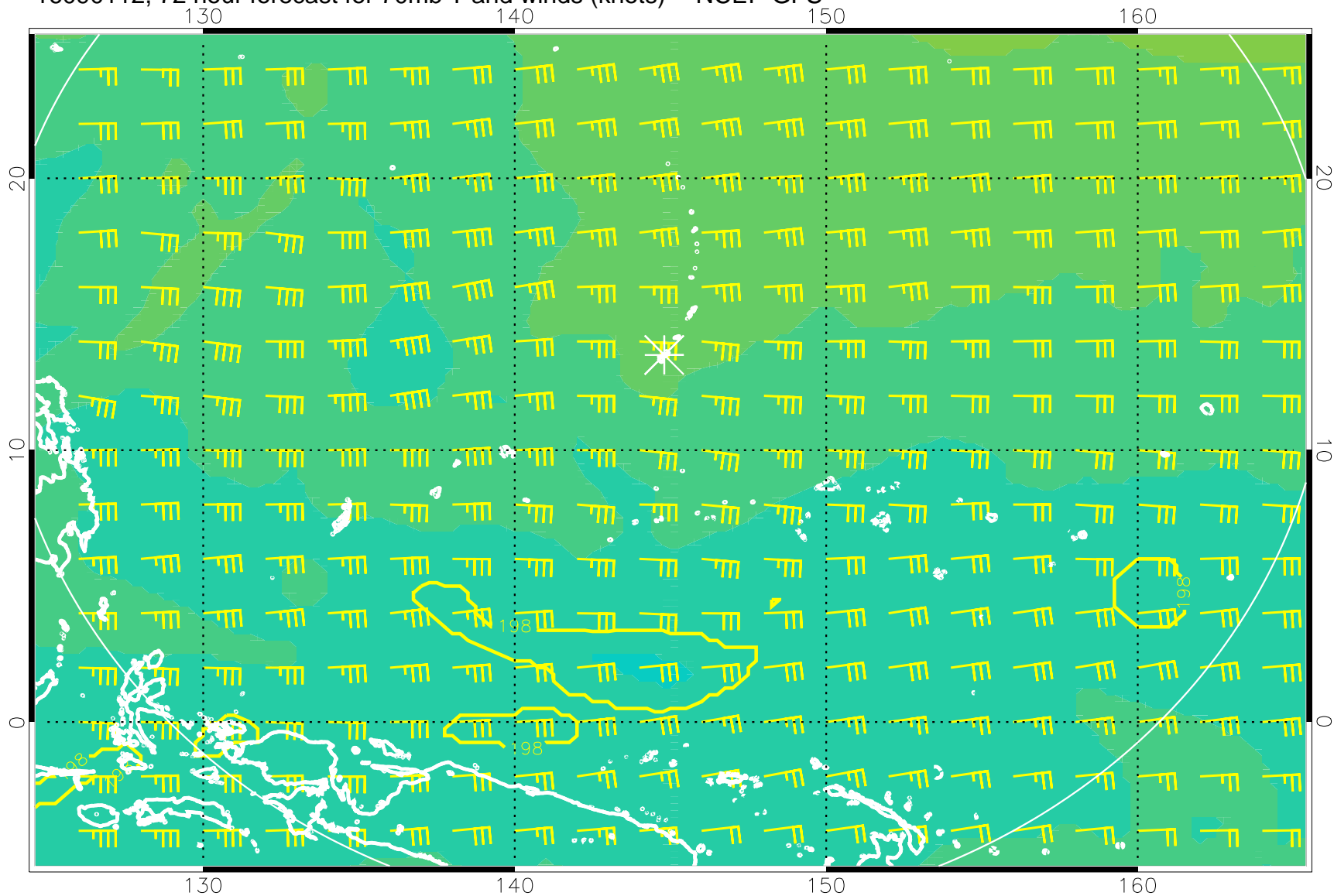
16090112, 72 hour forecast for 70mb T and winds (knots) -- NCEP GFS
