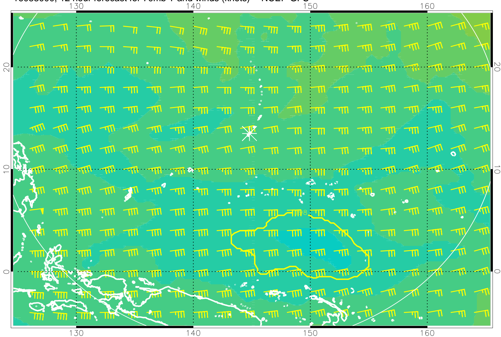
16083000, 12 hour forecast for 70mb T and winds (knots) -- NCEP GFS
