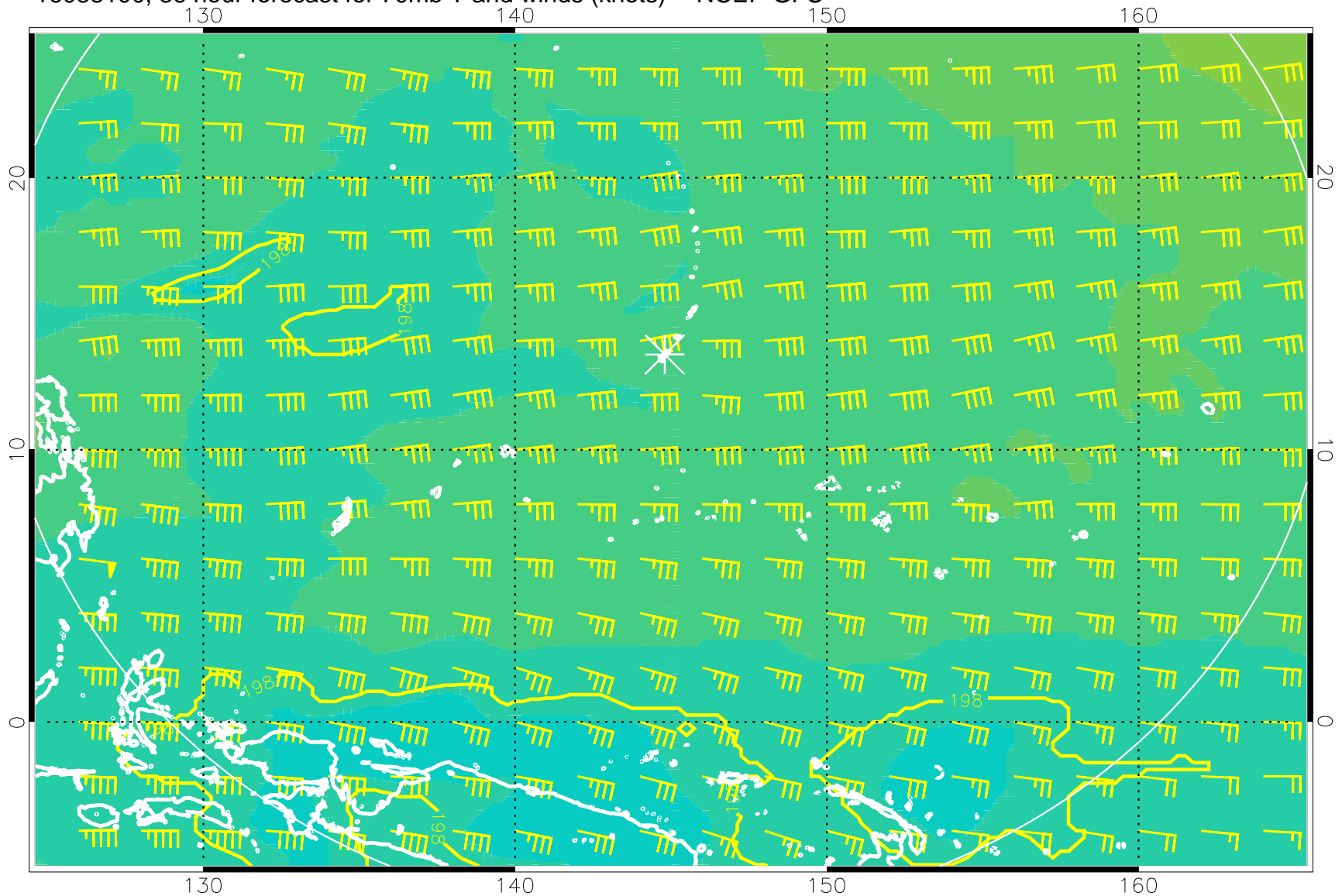
16083100, 36 hour forecast for 70mb T and winds (knots) -- NCEP GFS
