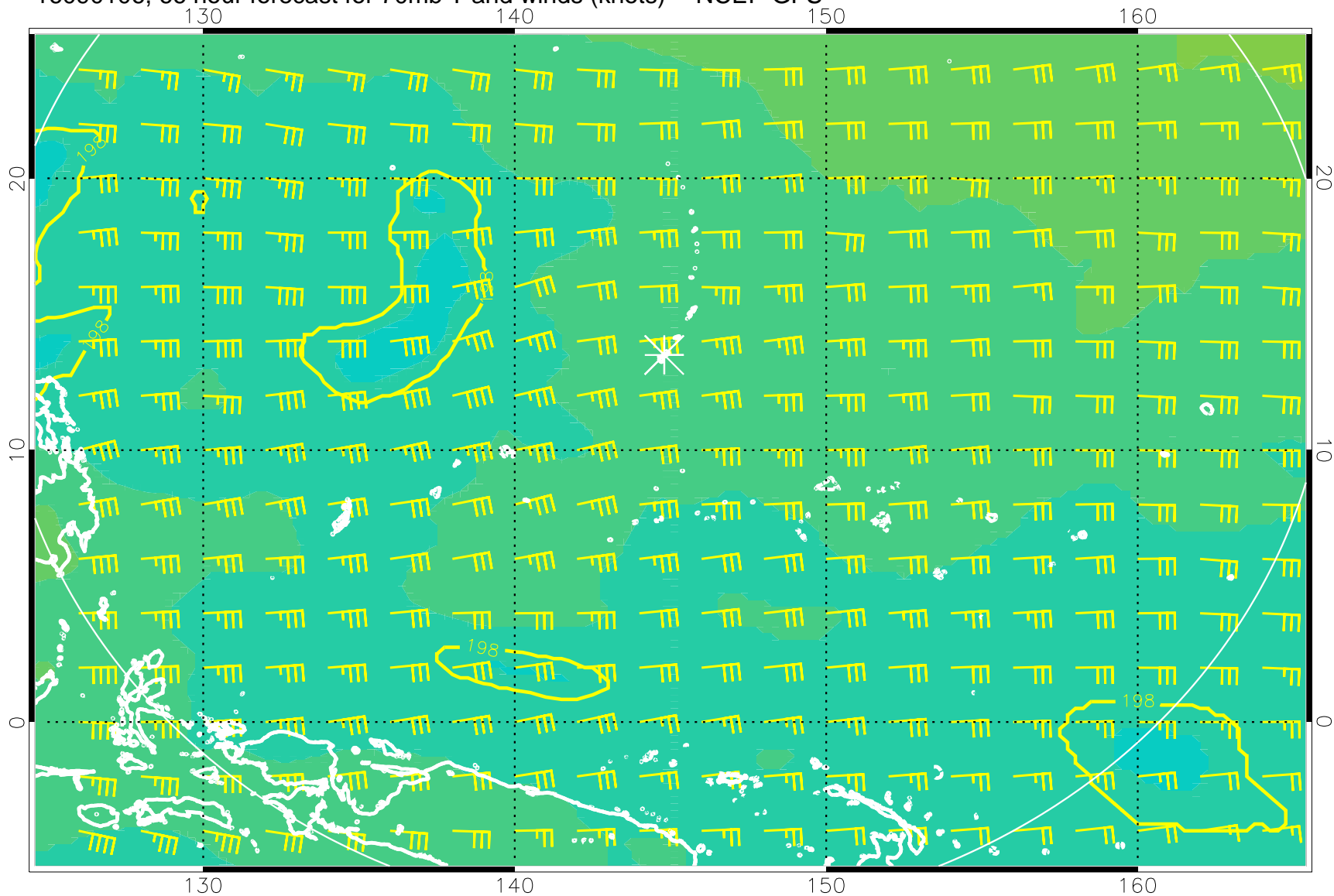
16090106, 66 hour forecast for 70mb T and winds (knots) -- NCEP GFS
