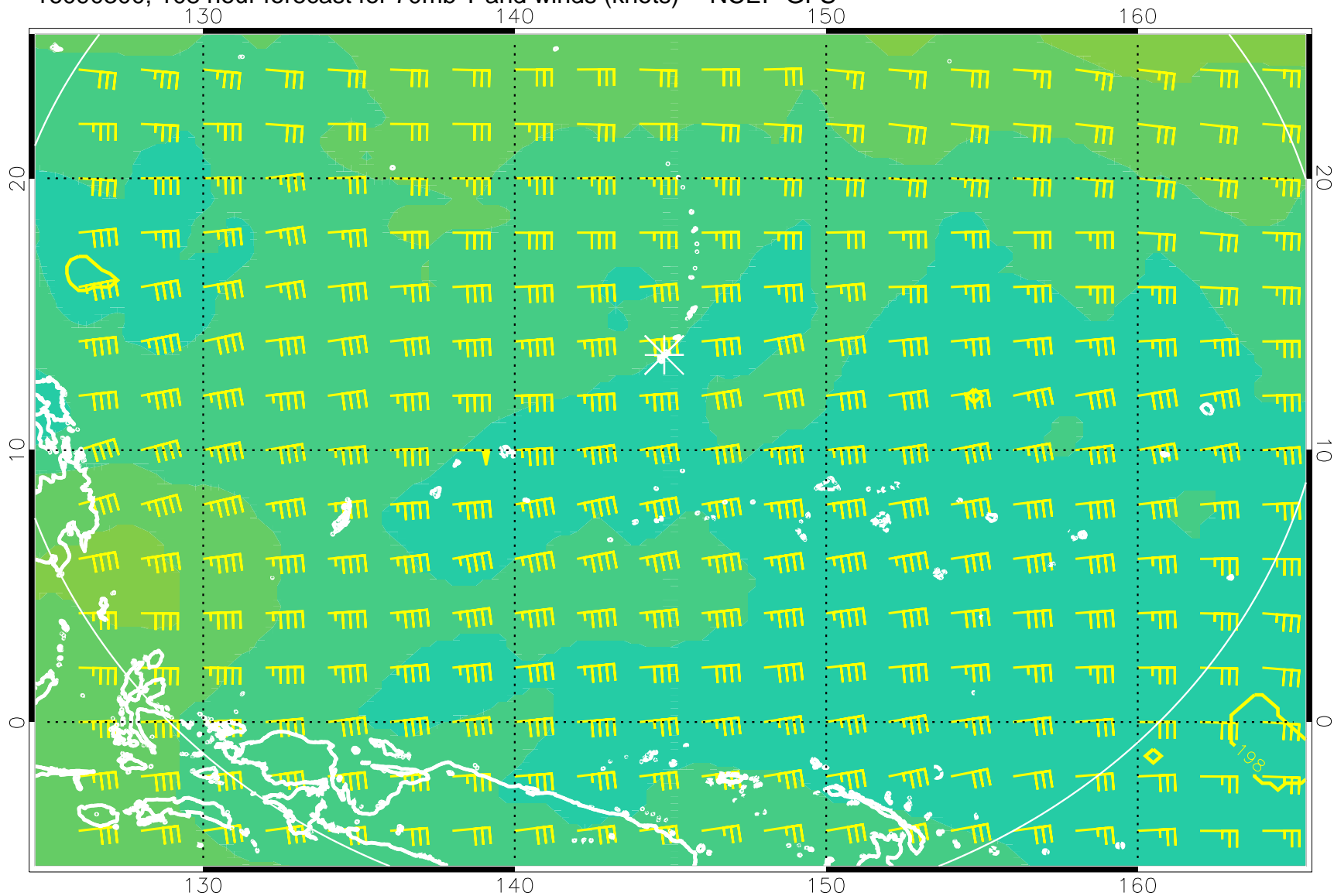
16090300, 108 hour forecast for 70mb T and winds (knots) -- NCEP GFS
