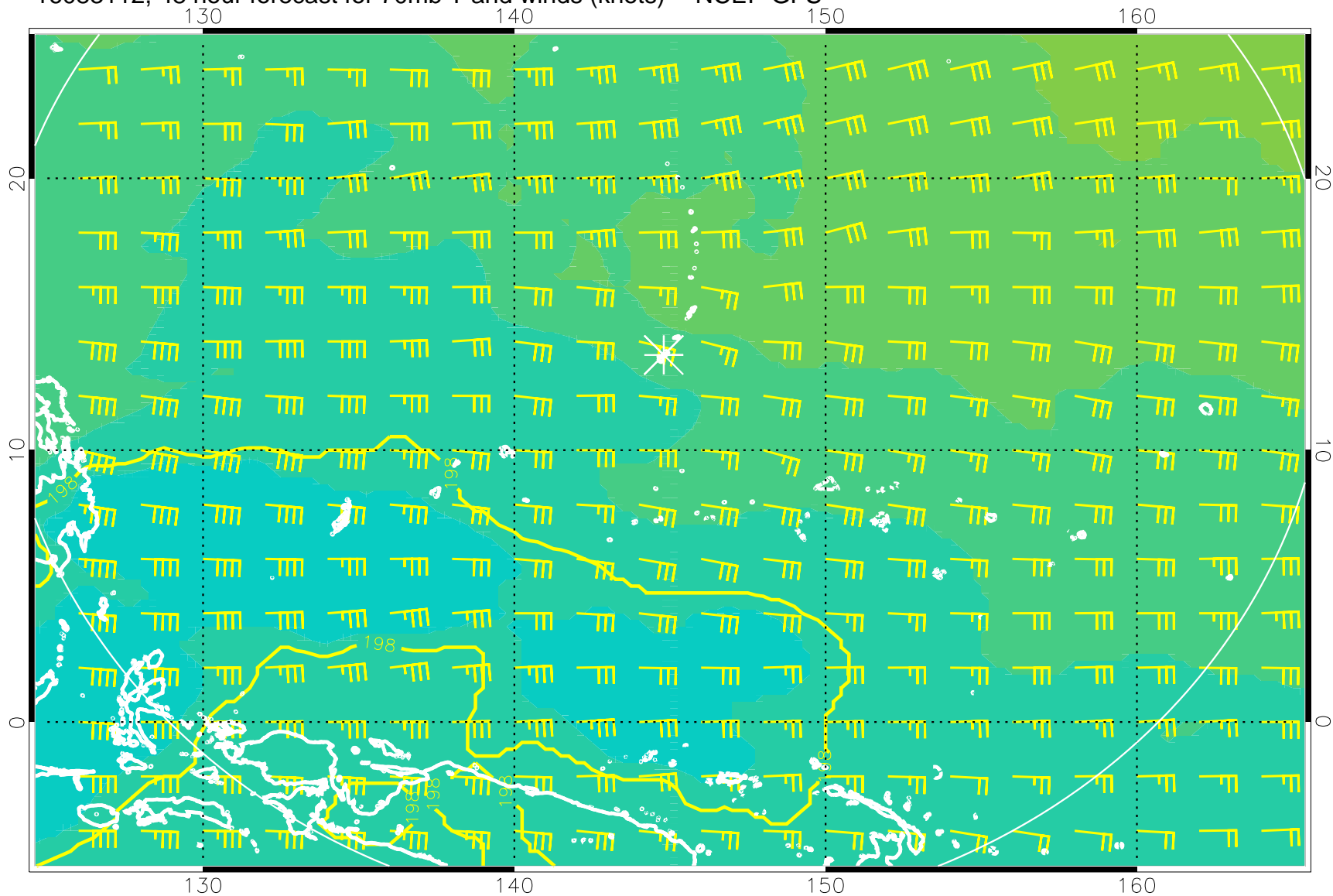
16083112, 48 hour forecast for 70mb T and winds (knots) -- NCEP GFS
