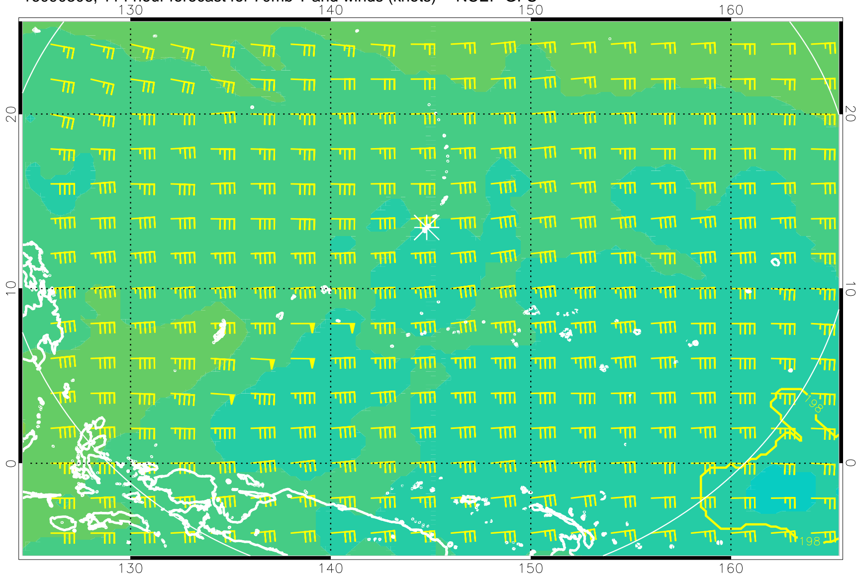
16090306, 114 hour forecast for 70mb T and winds (knots) -- NCEP GFS
