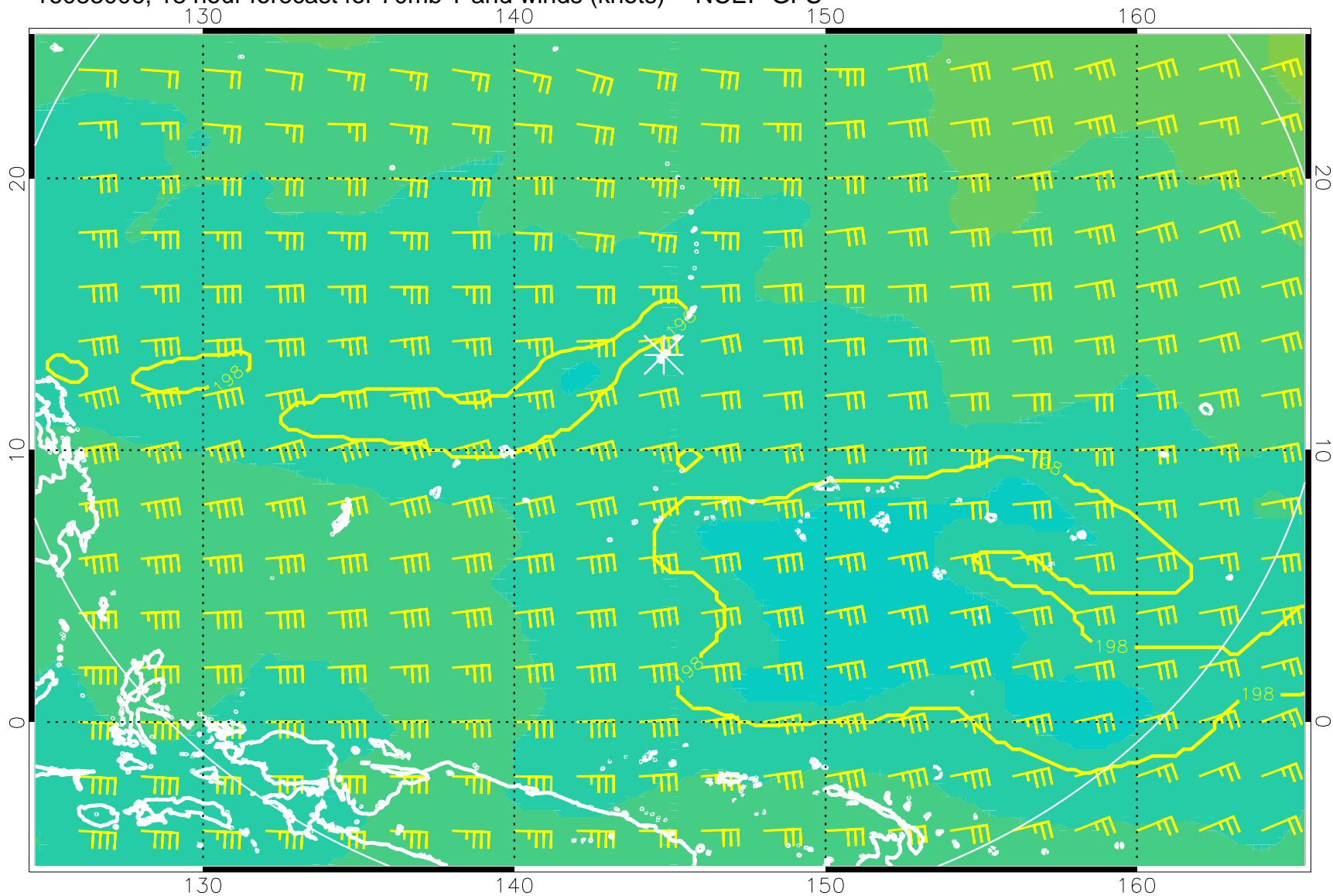
16083006, 18 hour forecast for 70mb T and winds (knots) -- NCEP GFS
