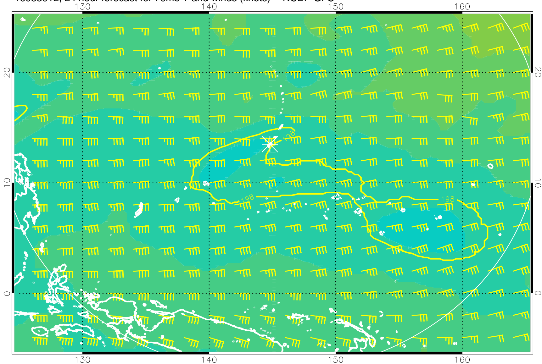
16083012, 24 hour forecast for 70mb T and winds (knots) -- NCEP GFS
