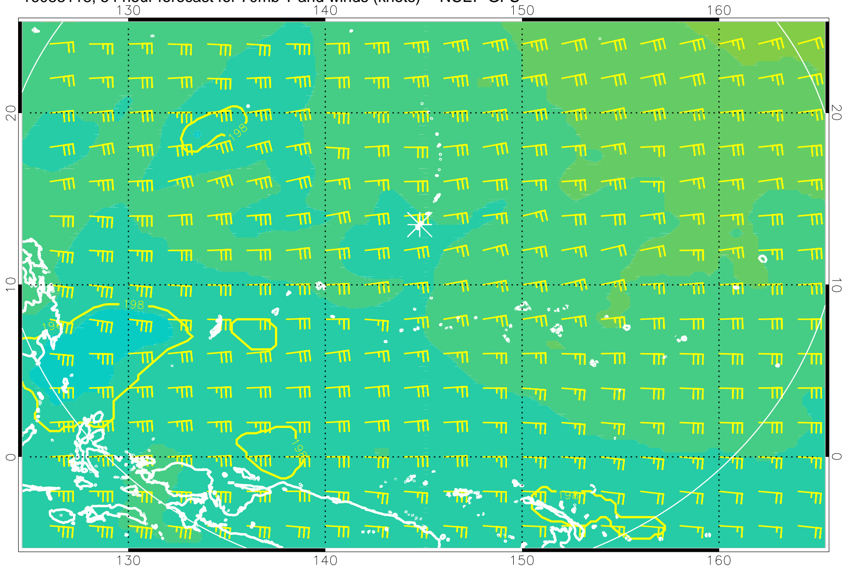
16083118, 54 hour forecast for 70mb T and winds (knots) -- NCEP GFS
