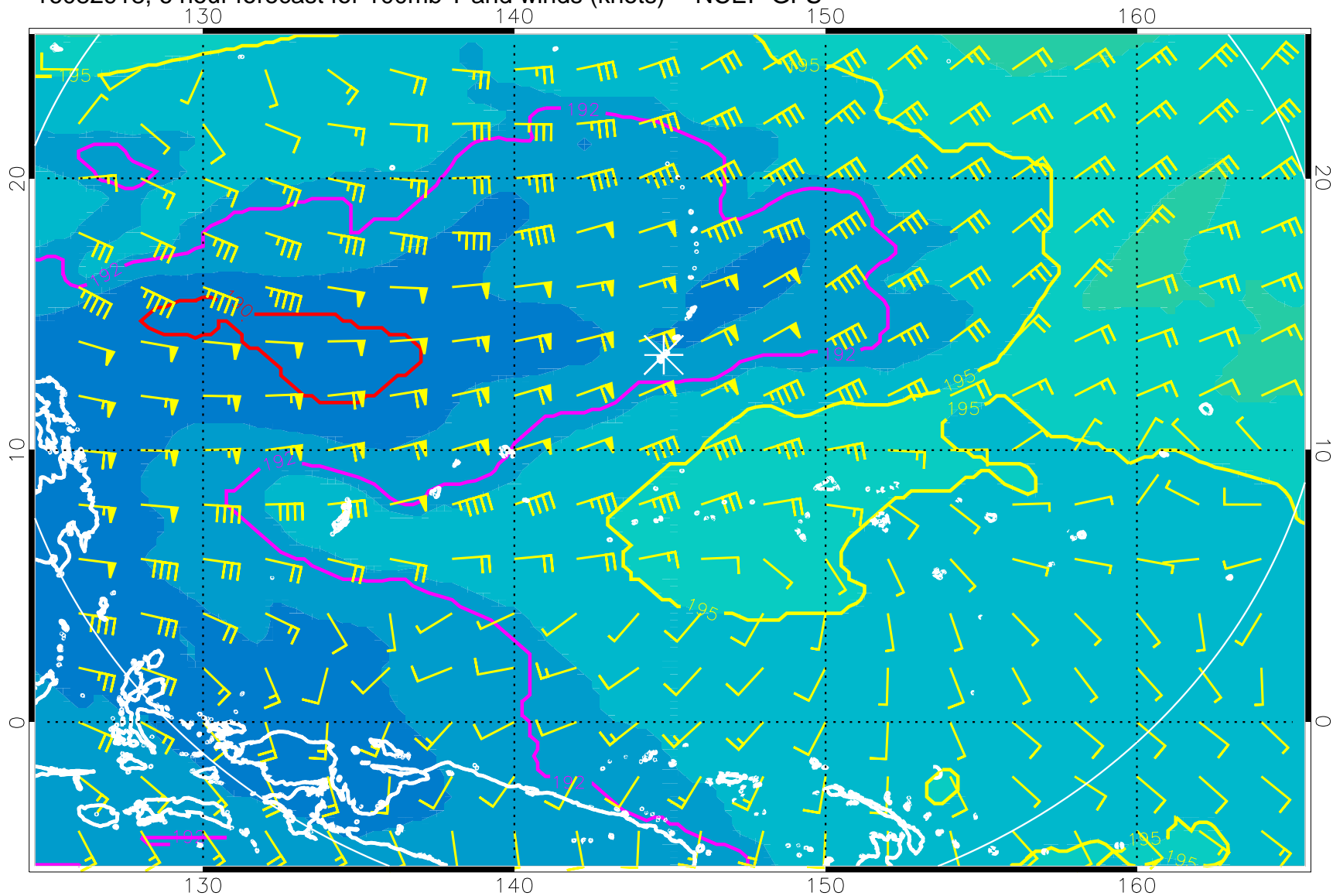
16082918, 6 hour forecast for 100mb T and winds (knots) -- NCEP GFS
