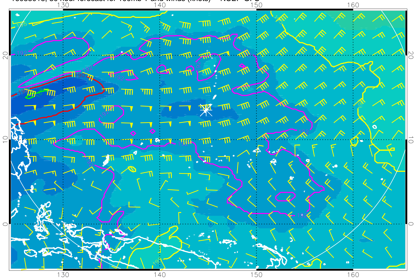
16083018, 30 hour forecast for 100mb T and winds (knots) -- NCEP GFS
