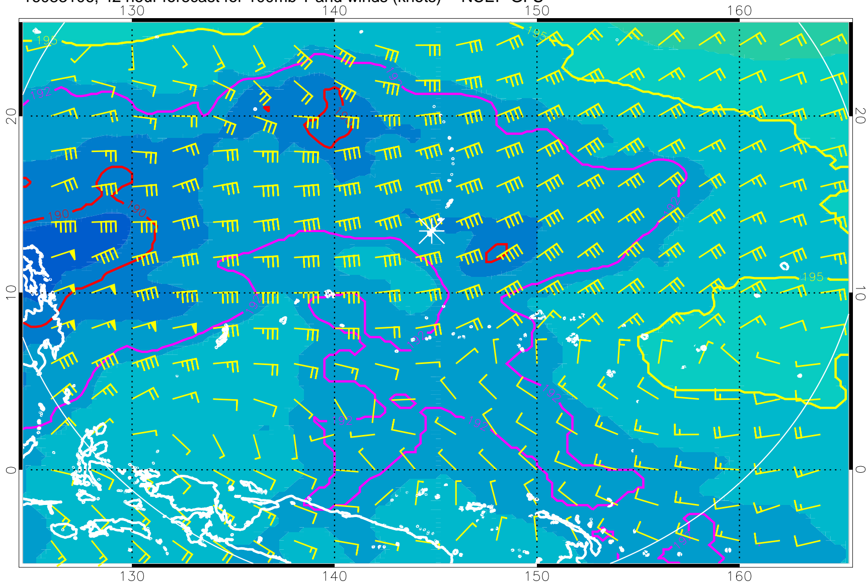
16083106, 42 hour forecast for 100mb T and winds (knots) -- NCEP GFS
