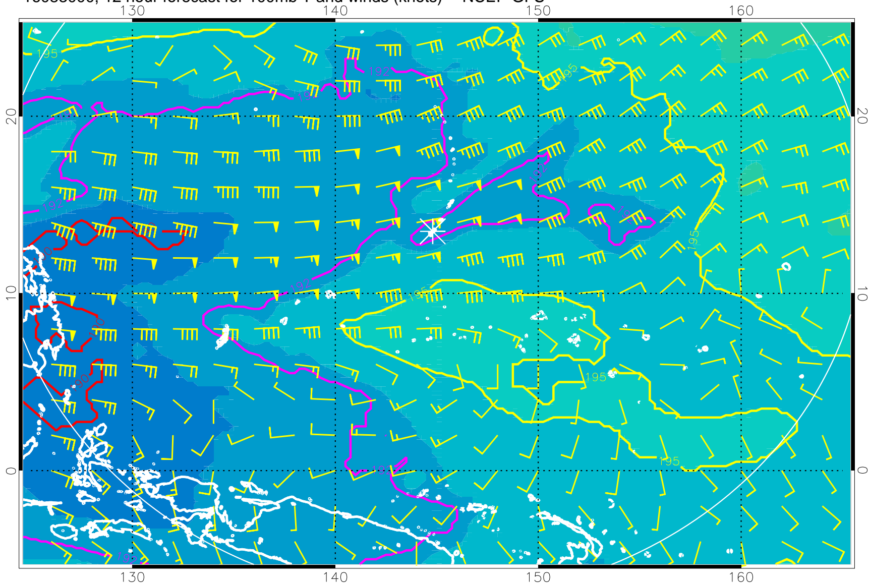
16083000, 12 hour forecast for 100mb T and winds (knots) -- NCEP GFS
