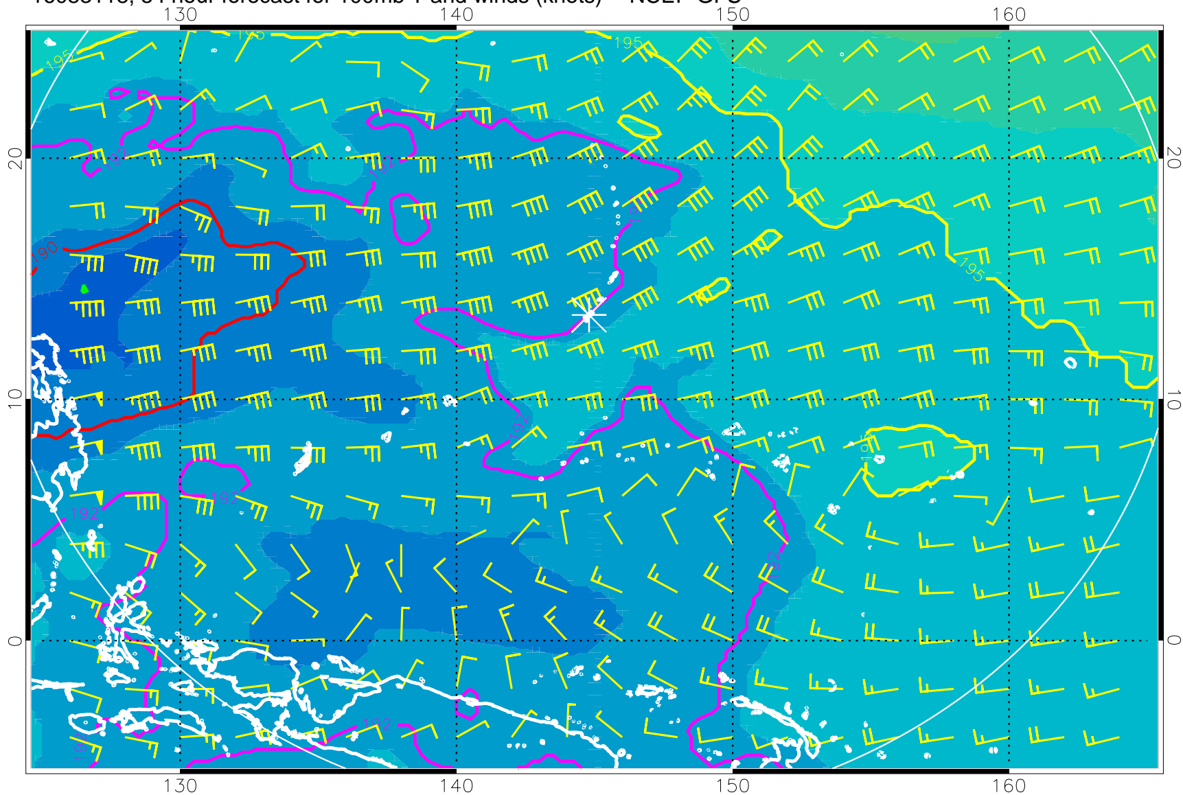
16083118, 54 hour forecast for 100mb T and winds (knots) -- NCEP GFS
