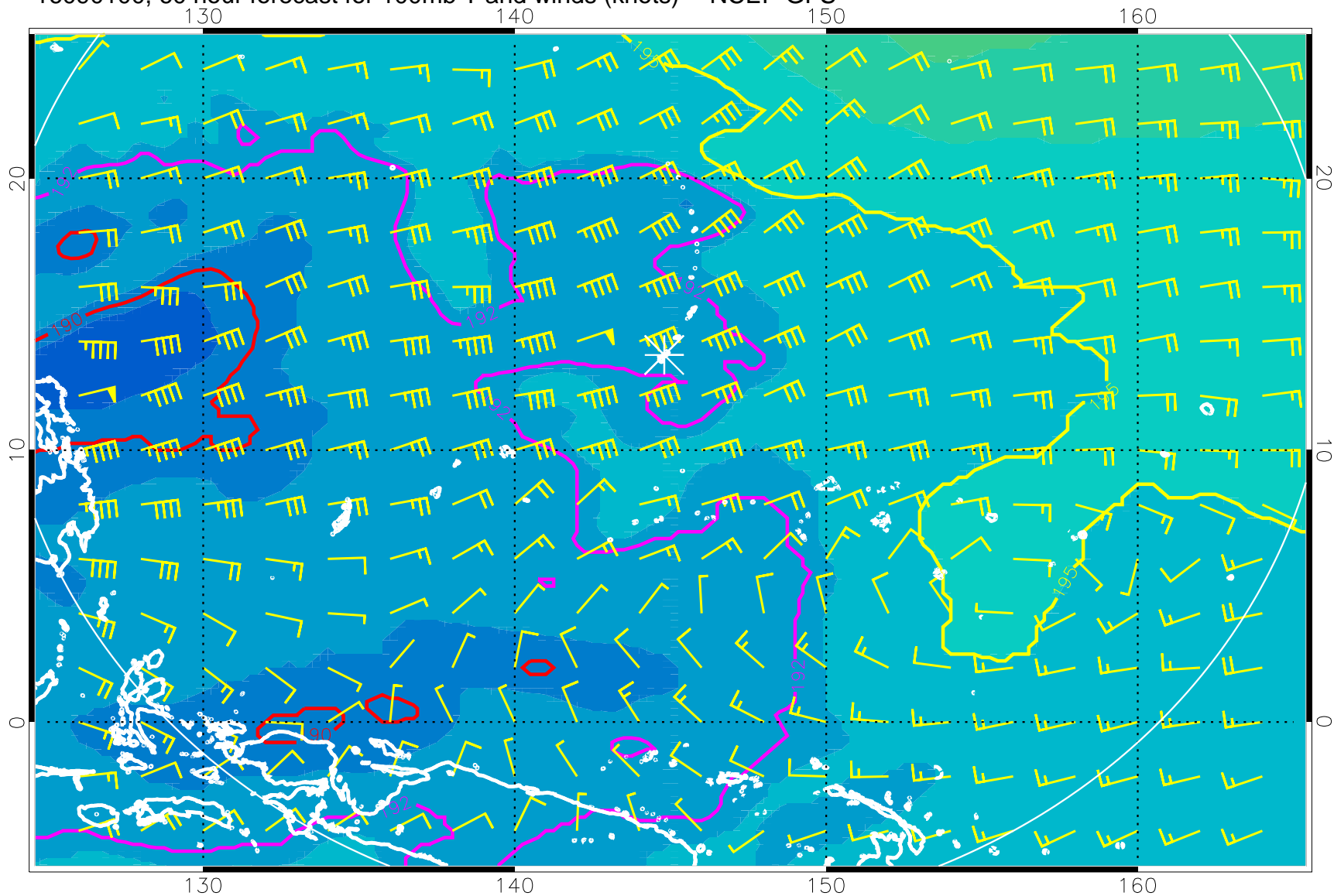
16090100, 60 hour forecast for 100mb T and winds (knots) -- NCEP GFS
