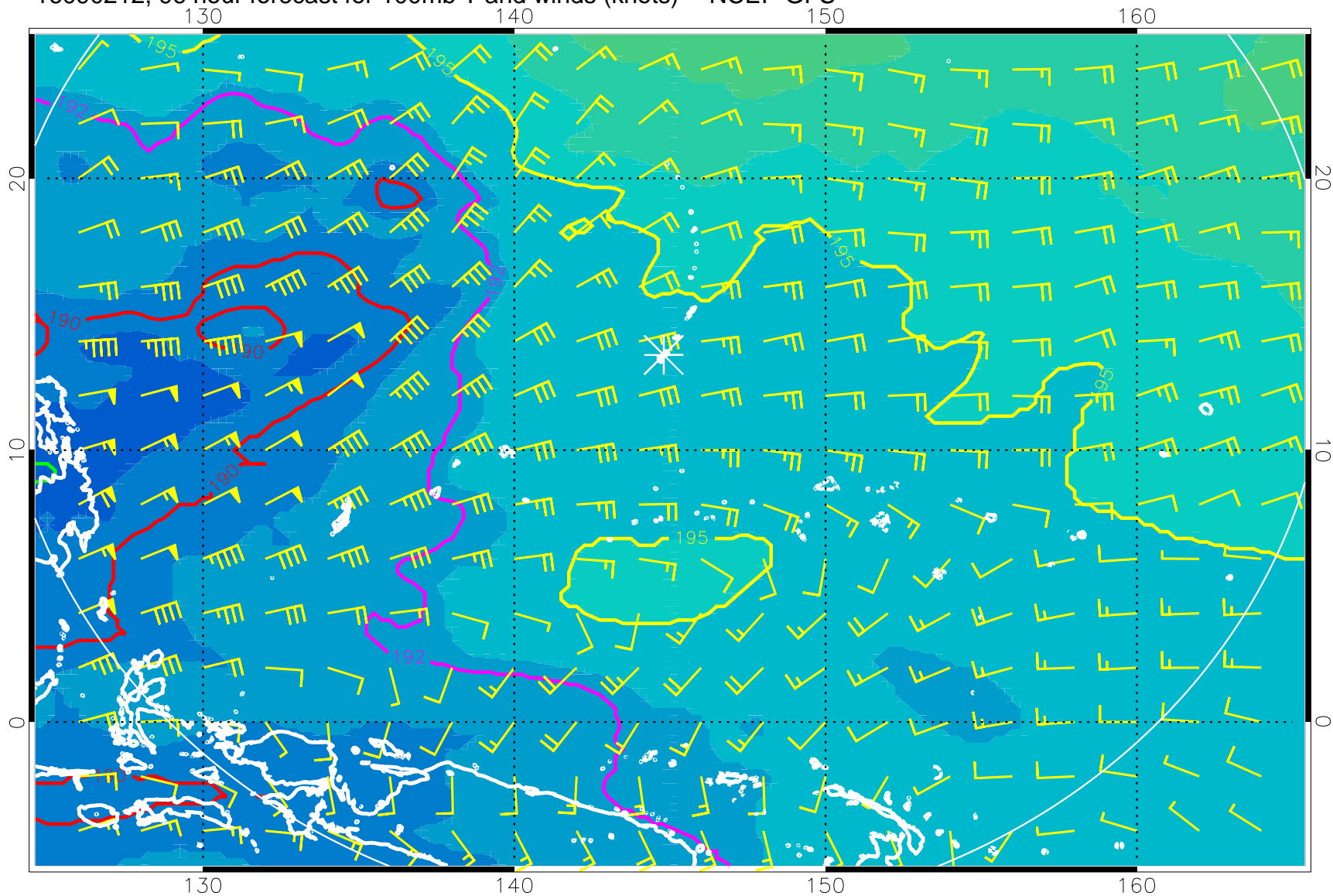
16090212, 96 hour forecast for 100mb T and winds (knots) -- NCEP GFS
