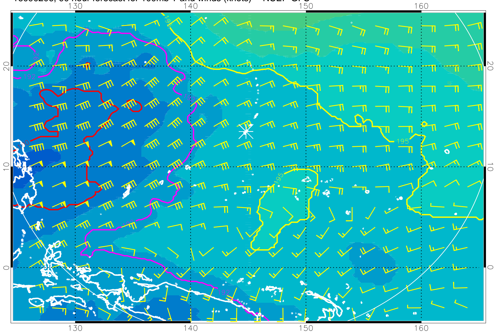
16090206, 90 hour forecast for 100mb T and winds (knots) -- NCEP GFS
