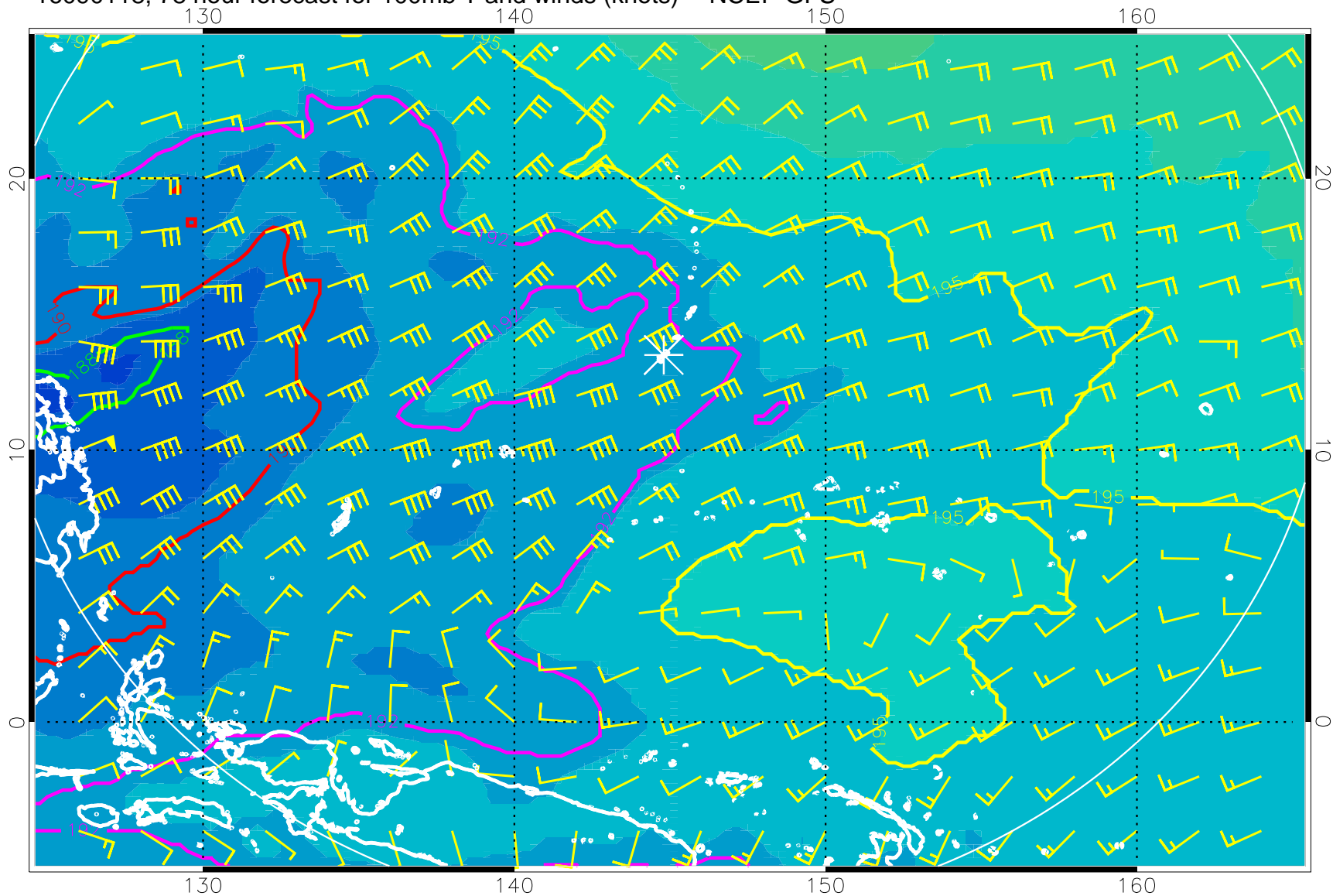
16090118, 78 hour forecast for 100mb T and winds (knots) -- NCEP GFS
