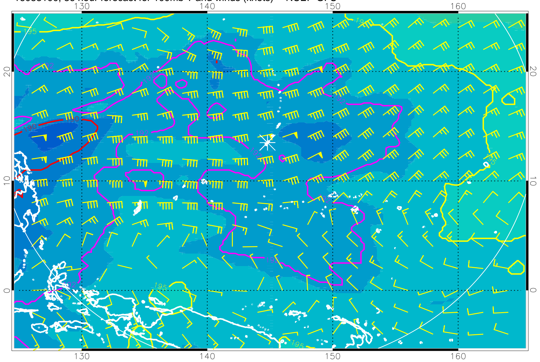
16083100, 36 hour forecast for 100mb T and winds (knots) -- NCEP GFS
