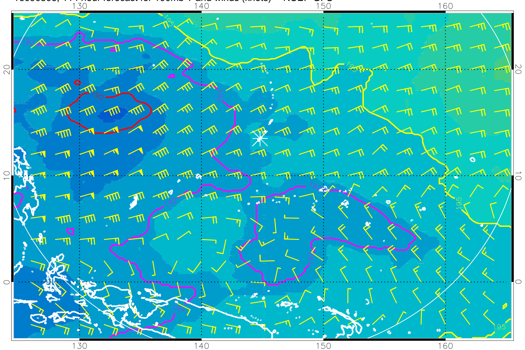
16090306, 114 hour forecast for 100mb T and winds (knots) -- NCEP GFS
