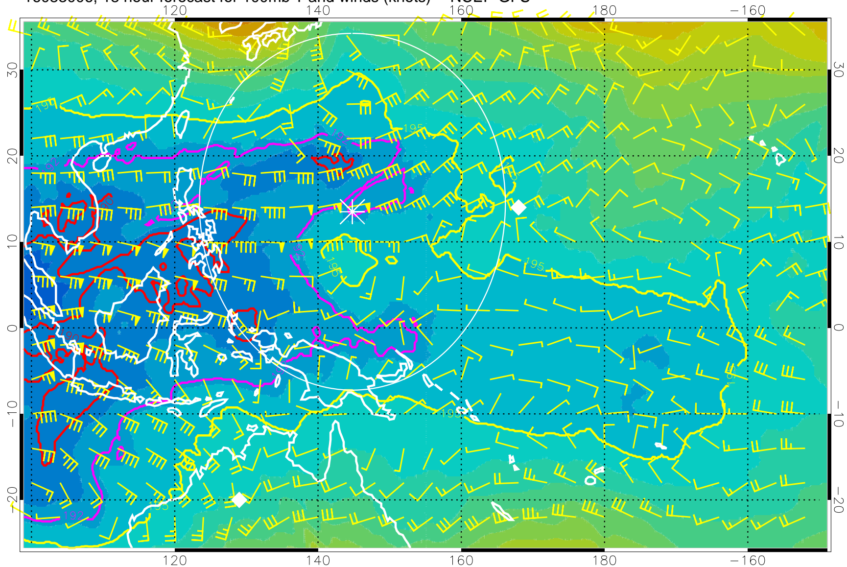
16083006, 18 hour forecast for 100mb T and winds (knots) -- NCEP GFS
