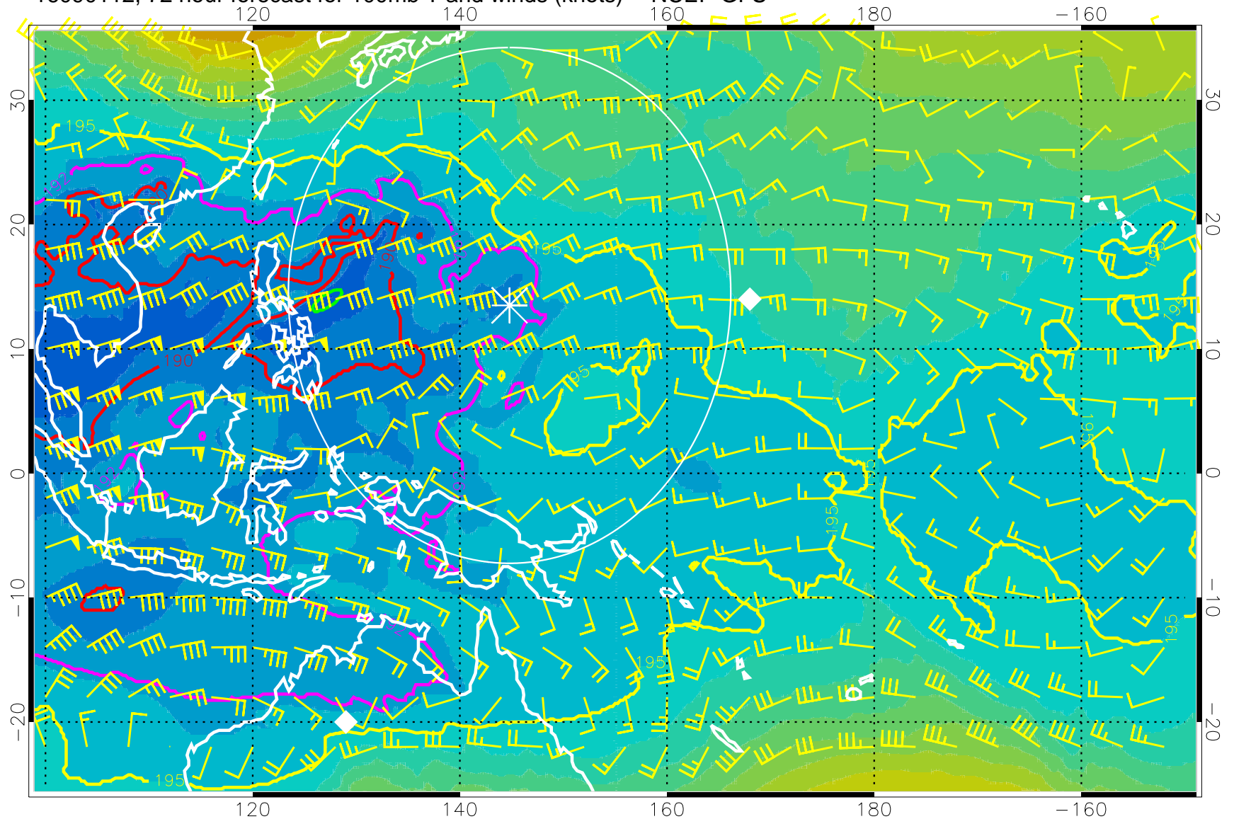
16090112, 72 hour forecast for 100mb T and winds (knots) -- NCEP GFS
