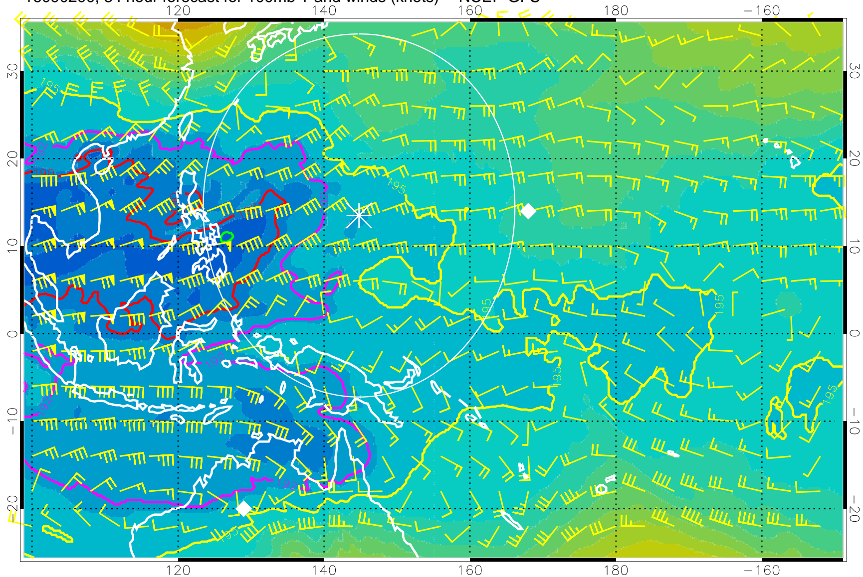
16090200, 84 hour forecast for 100mb T and winds (knots) -- NCEP GFS
