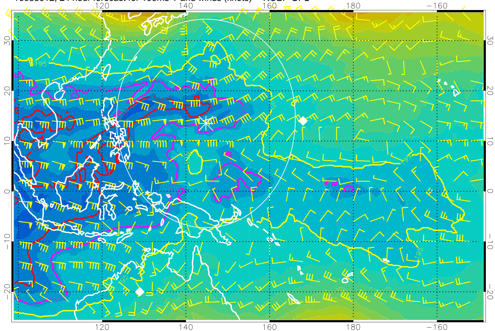
16083012, 24 hour forecast for 100mb T and winds (knots) -- NCEP GFS
