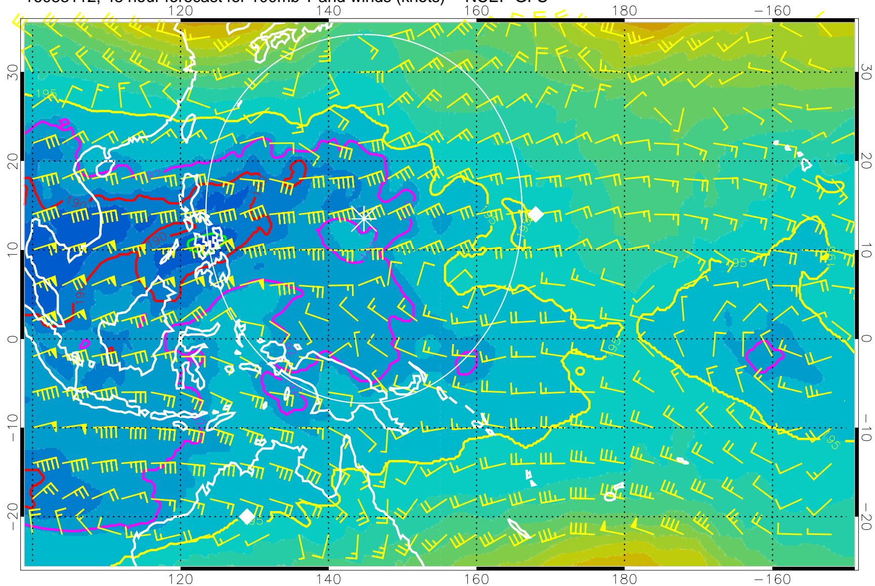
16083112, 48 hour forecast for 100mb T and winds (knots) -- NCEP GFS
