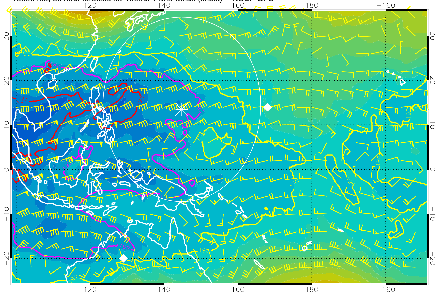
16090106, 66 hour forecast for 100mb T and winds (knots) -- NCEP GFS
