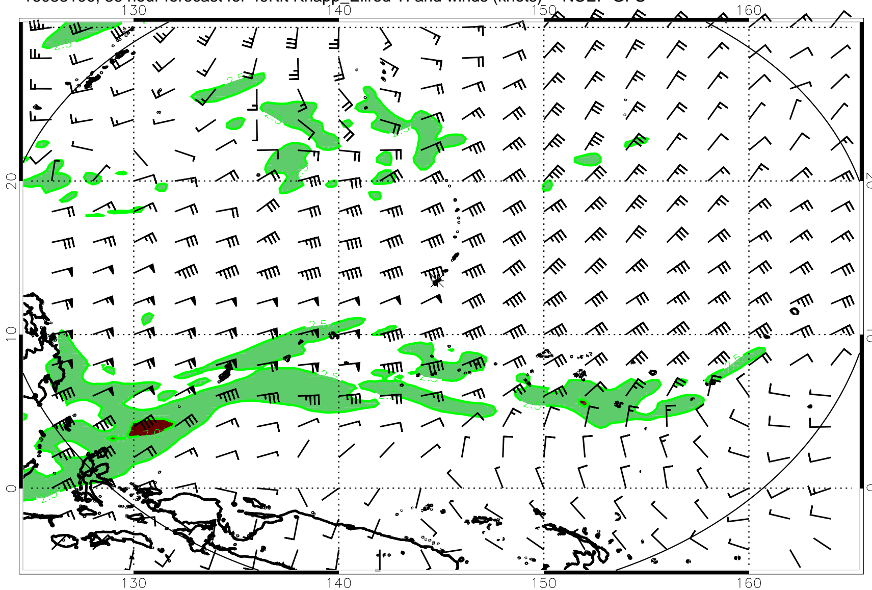
16083100, 36 hour forecast for 49Kft Knapp_Ellrod TI and winds (knots) -- NCEP GFS
