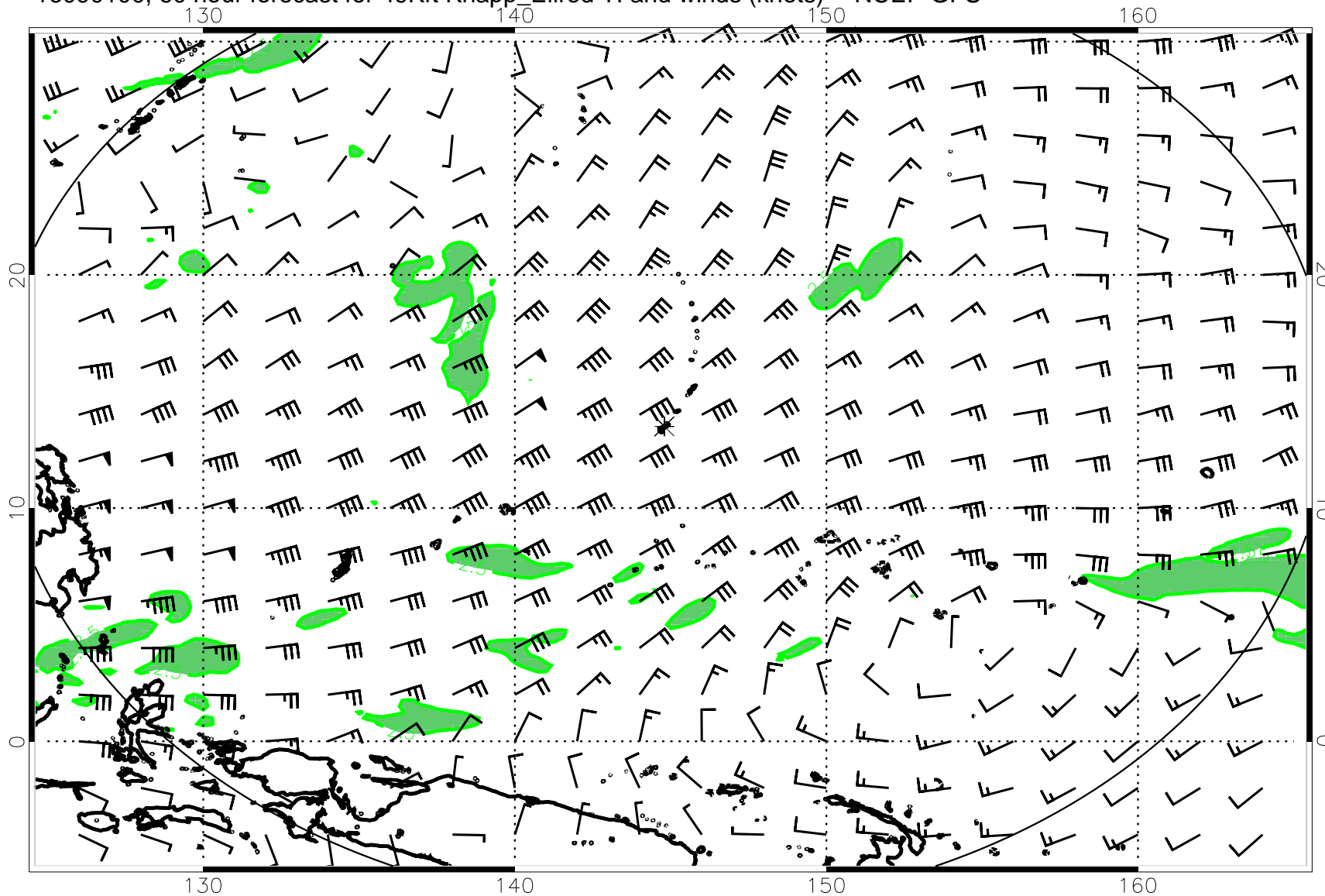
16090100, 60 hour forecast for 49Kft Knapp_Ellrod TI and winds (knots) -- NCEP GFS
