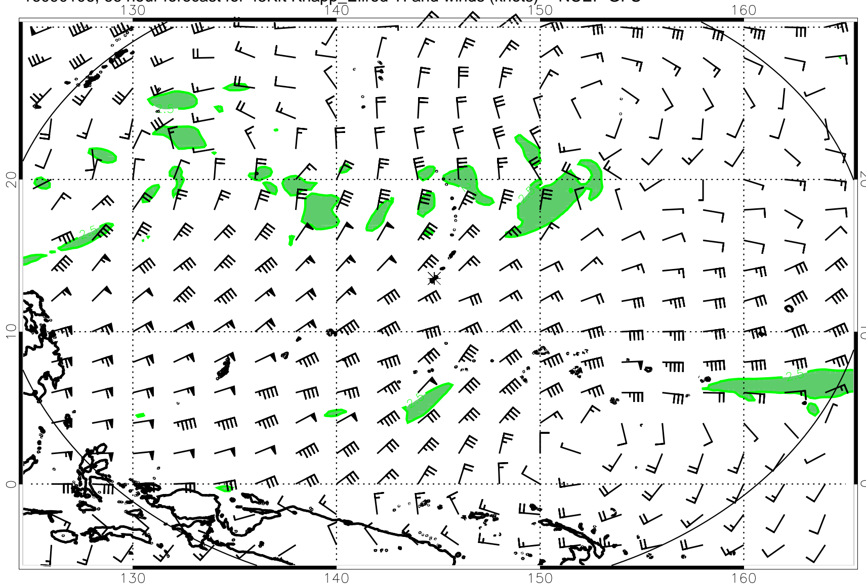
16090106, 66 hour forecast for 45Kft Knapp_Ellrod TI and winds (knots) -- NCEP GFS
