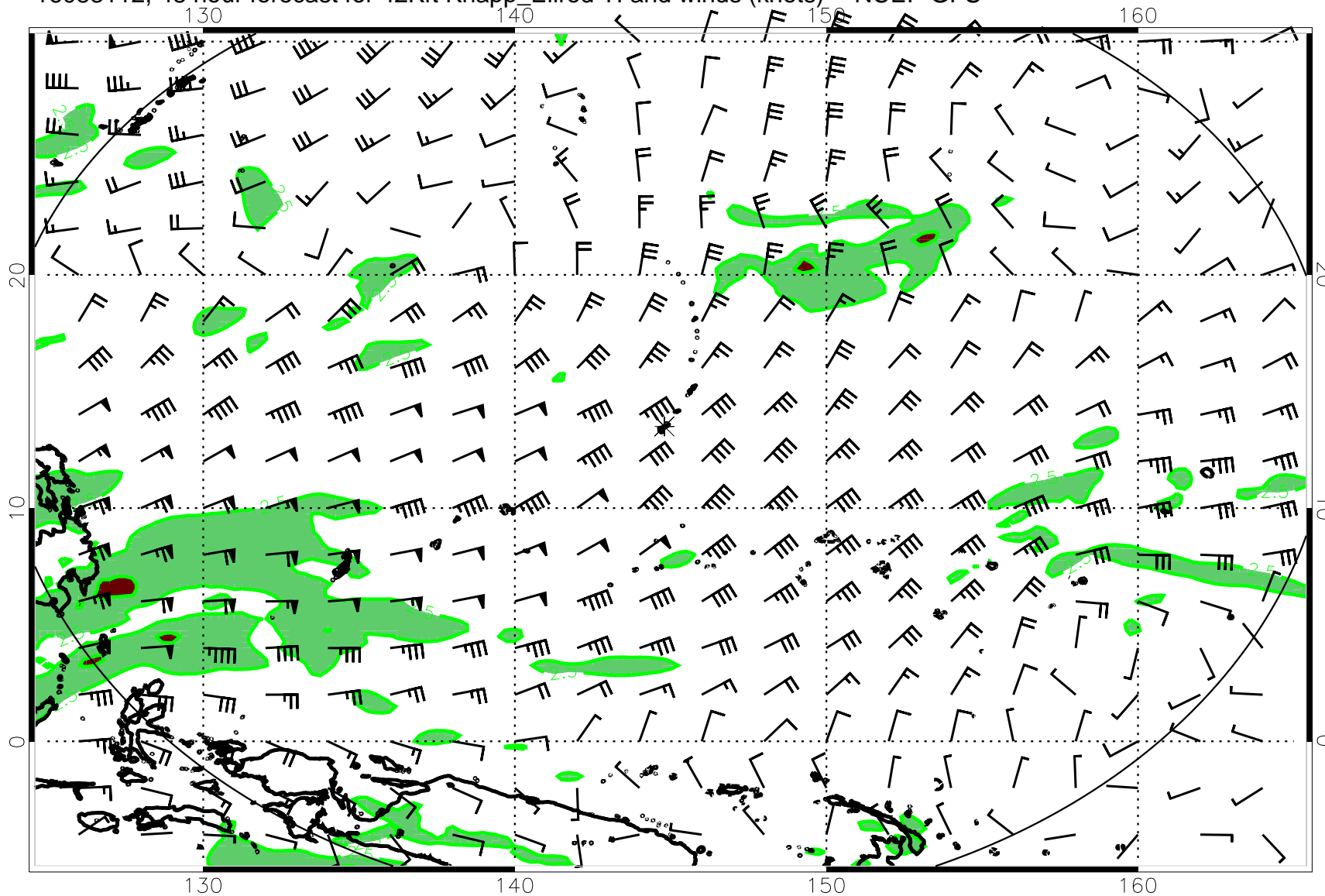
16083112, 48 hour forecast for 42Kft Knapp_Ellrod TI and winds (knots) -- NCEP GFS
