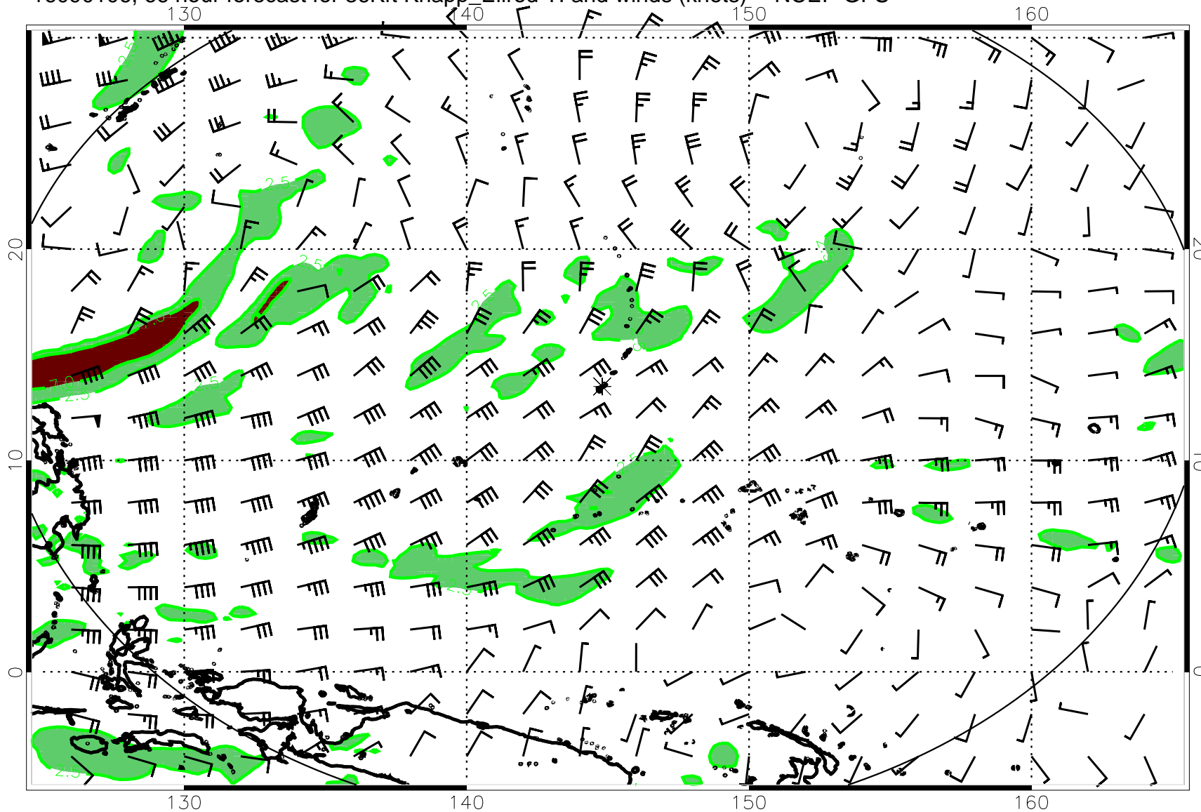
16090106, 66 hour forecast for 36Kft Knapp_Ellrod TI and winds (knots) -- NCEP GFS
