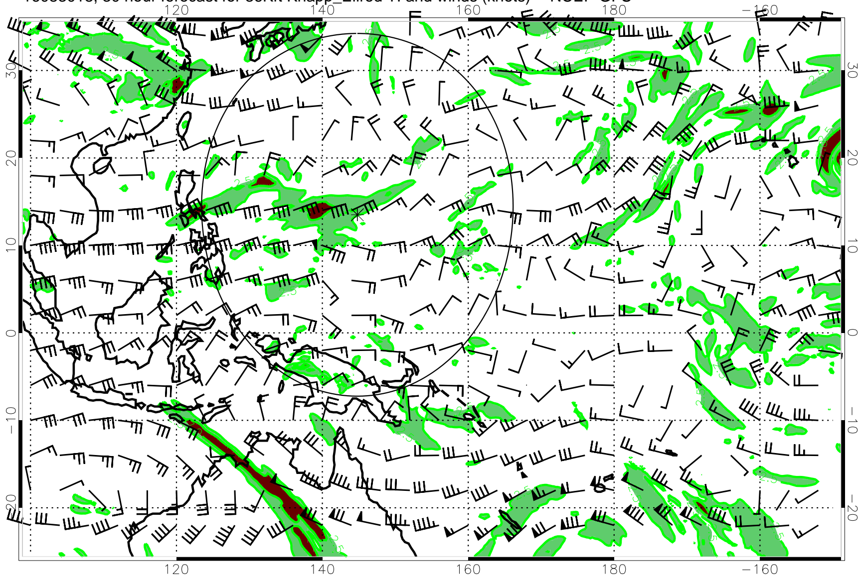
16083018, 30 hour forecast for 36Kft Knapp_Ellrod TI and winds (knots) -- NCEP GFS
