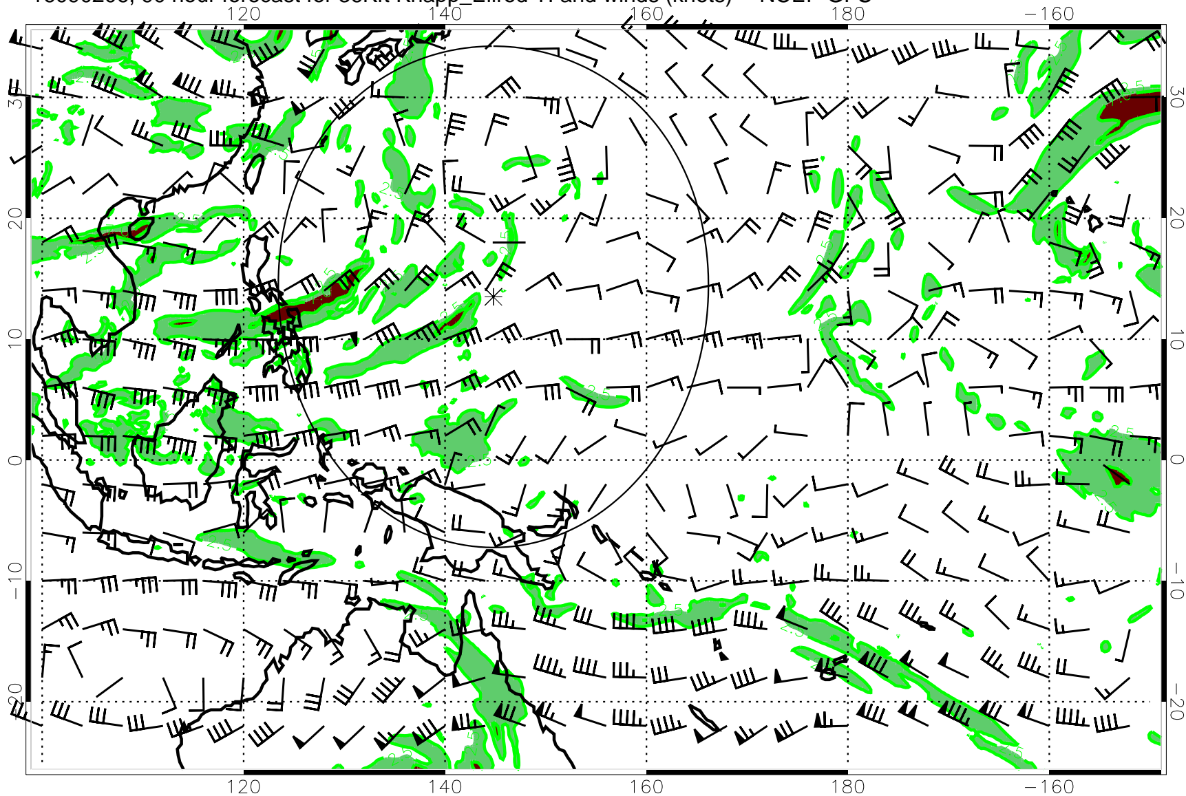
16090206, 90 hour forecast for 36Kft Knapp_Ellrod TI and winds (knots) -- NCEP GFS
