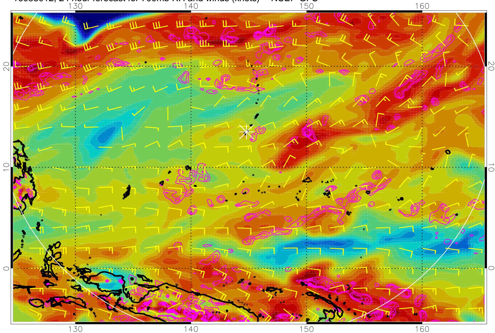
16083012, 24 hour forecast for 700mb RH and winds (knots) -- NCEP GFS
