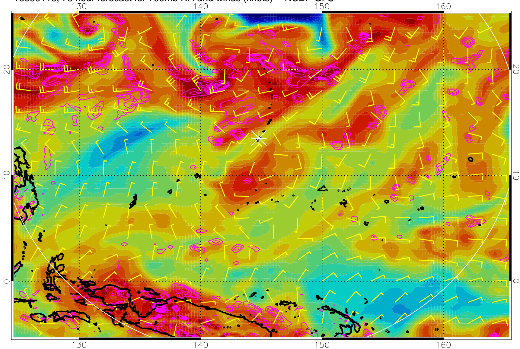
16090118, 78 hour forecast for 700mb RH and winds (knots) -- NCEP GFS
