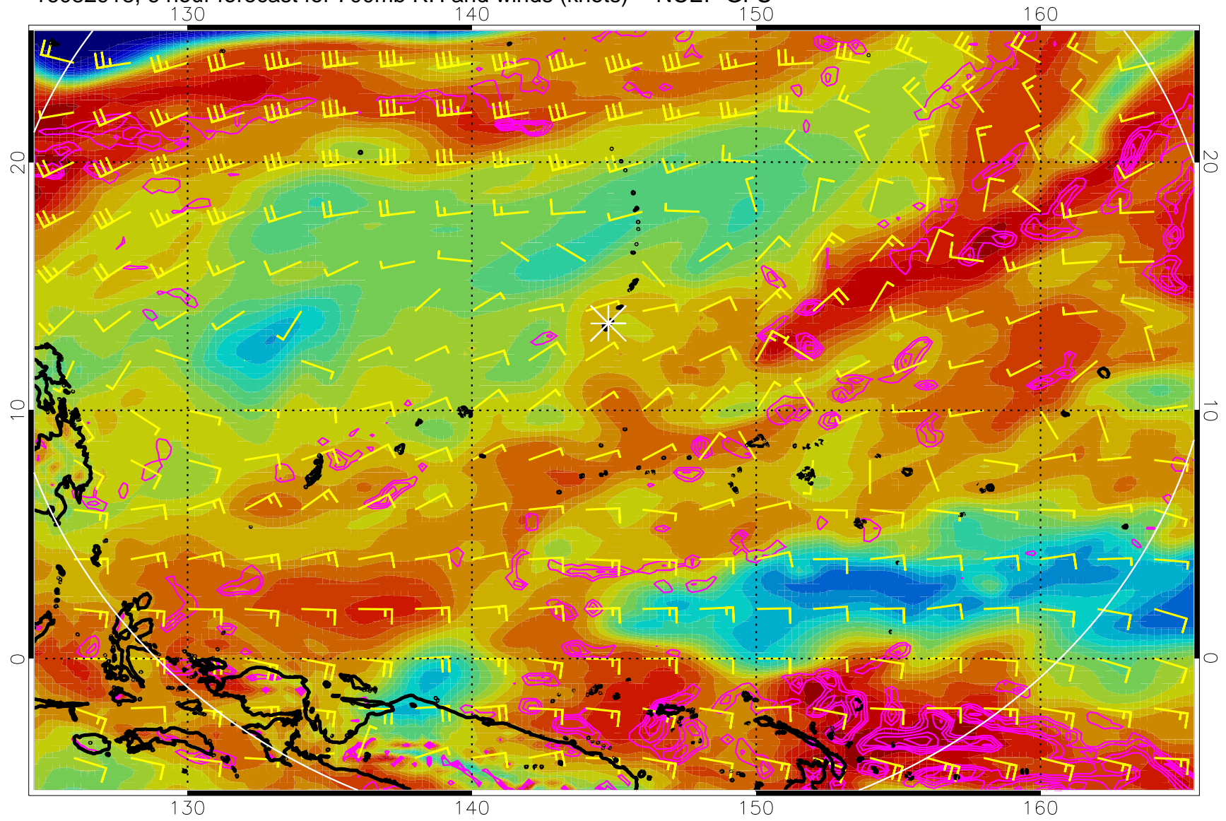
16082918, 6 hour forecast for 700mb RH and winds (knots) -- NCEP GFS
