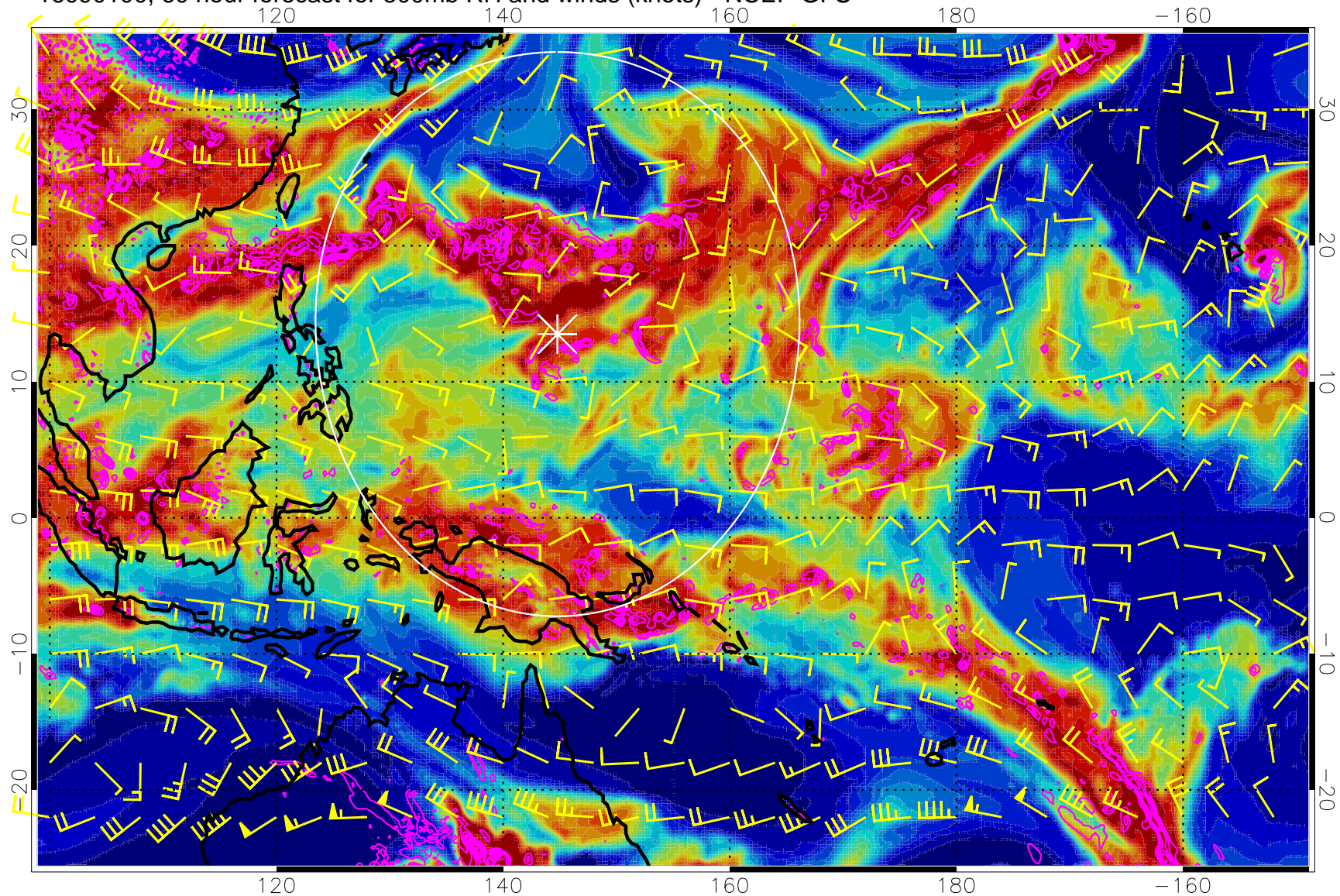
16090100, 60 hour forecast for 500mb RH and winds (knots) - NCEP GFS
