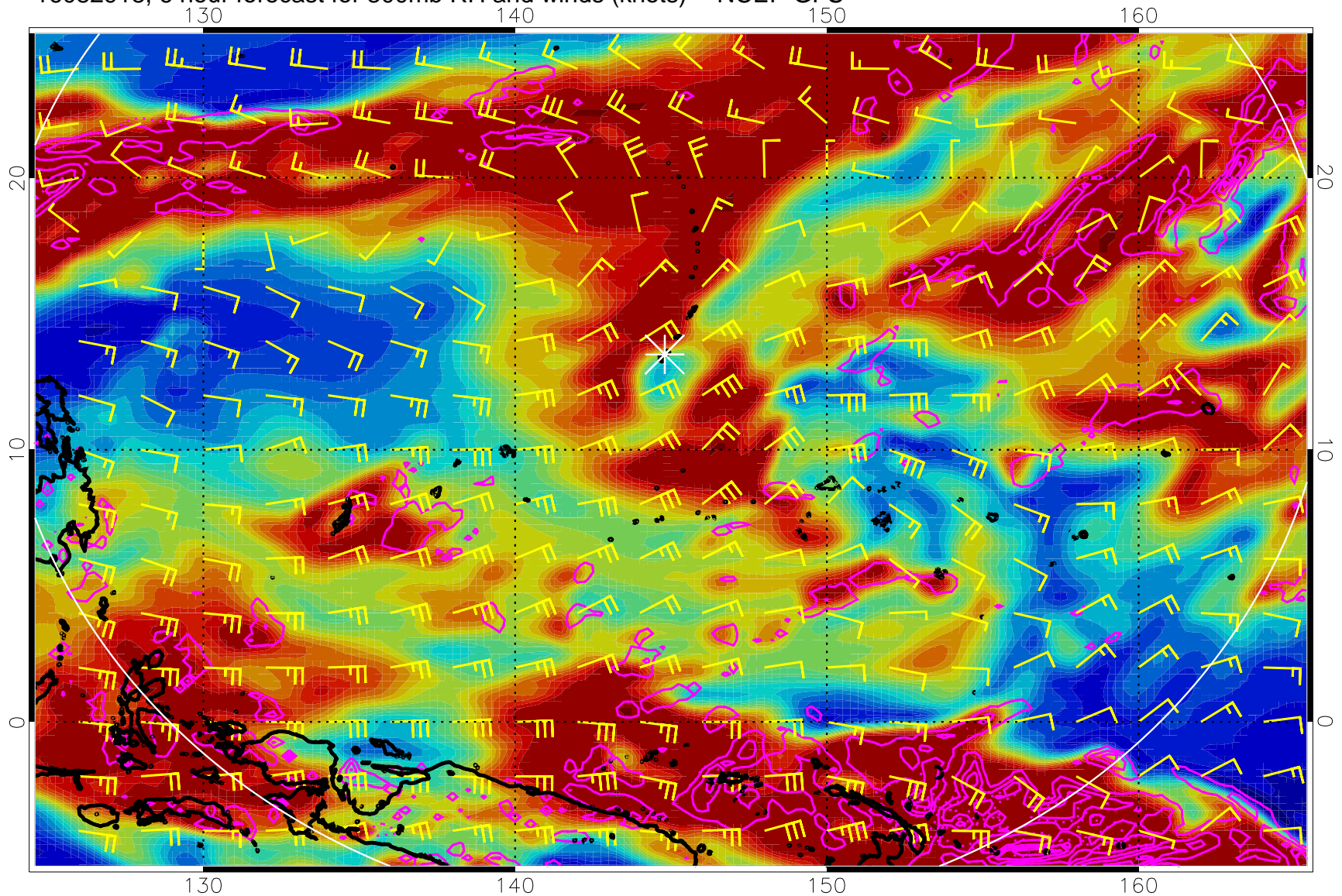
16082918, 6 hour forecast for 300mb RH and winds (knots) -- NCEP GFS
