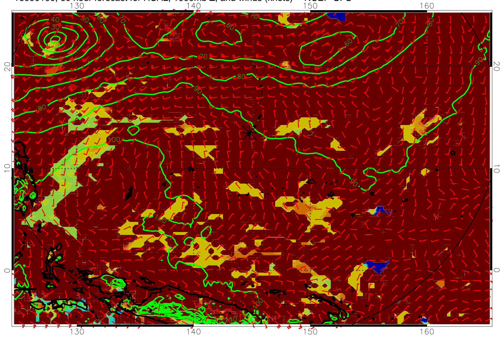
16090100, 60 hour forecast for HCAL, 1000mb Z, and winds (knots) -- NCEP GFS
