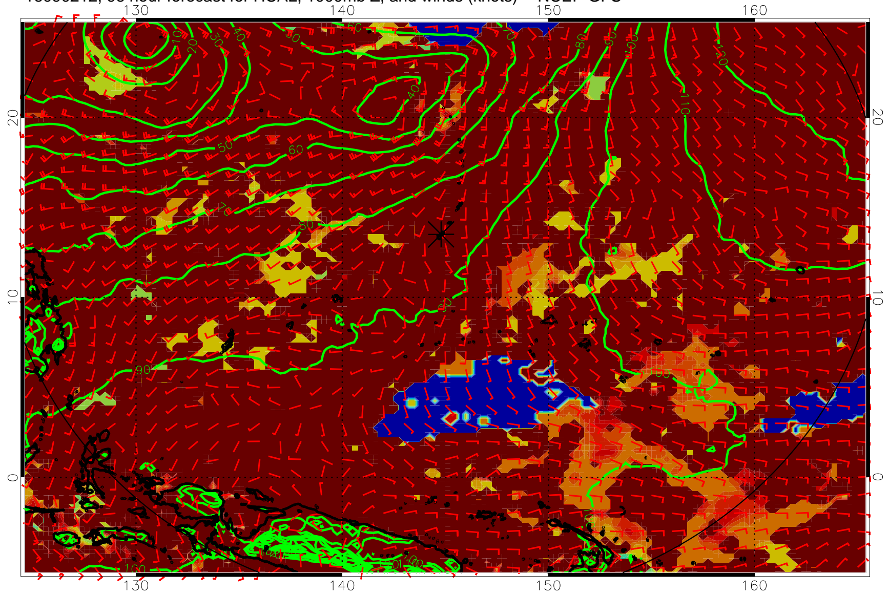
16090212, 96 hour forecast for HCAL, 1000mb Z, and winds (knots) -- NCEP GFS
