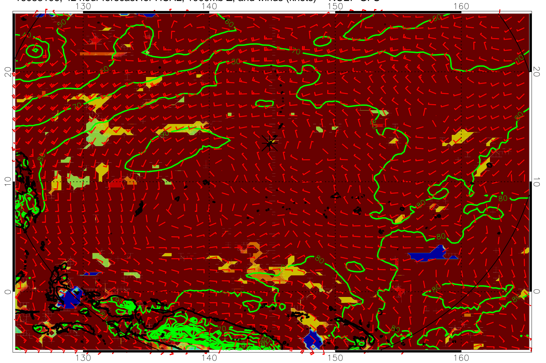
16083106, 42 hour forecast for HCAL, 1000mb Z, and winds (knots) -- NCEP GFS
