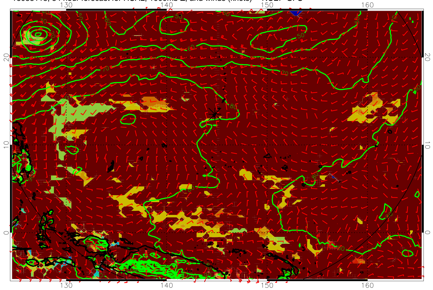
16083118, 54 hour forecast for HCAL, 1000mb Z, and winds (knots) -- NCEP GFS
