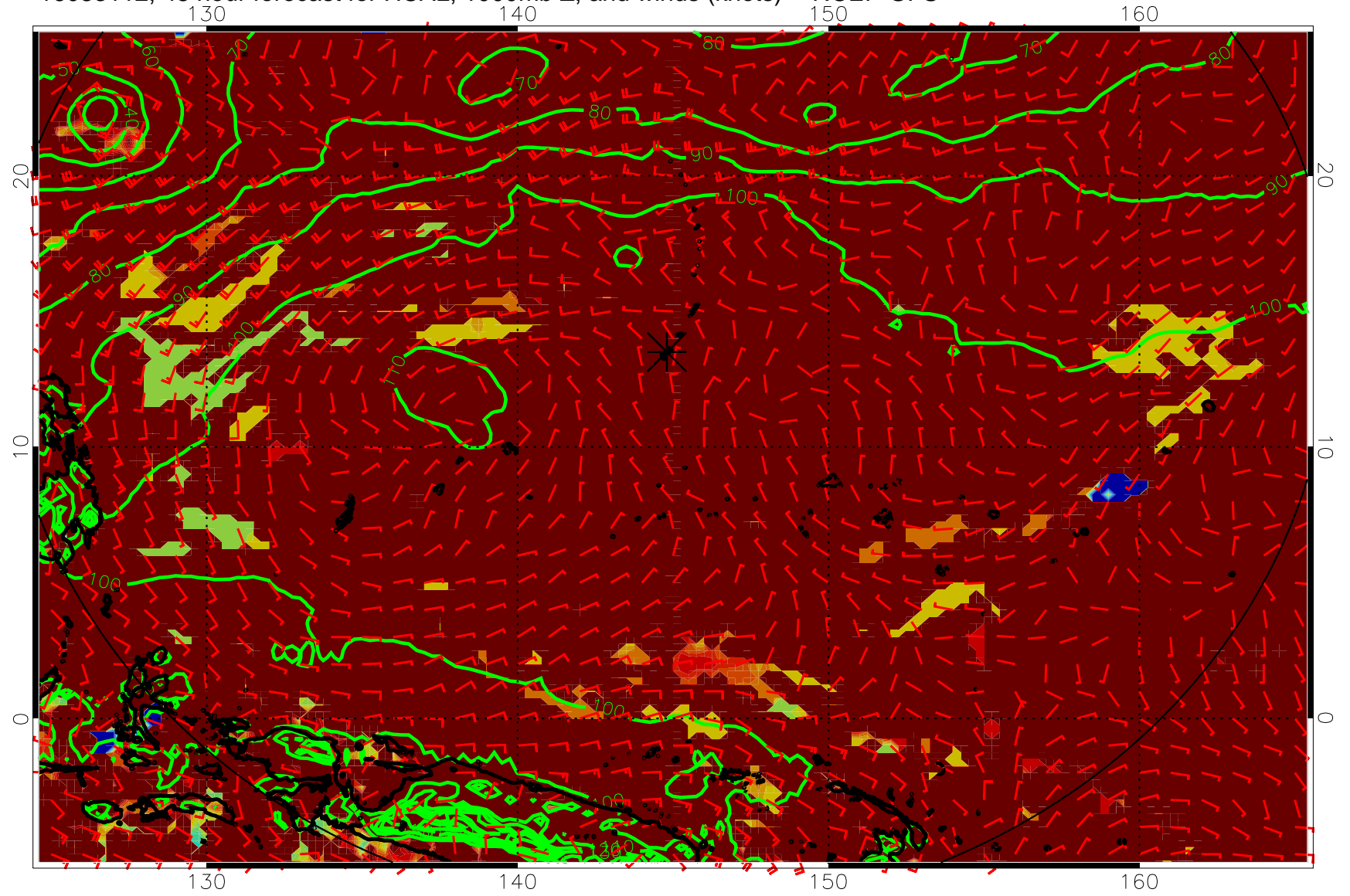
16083112, 48 hour forecast for HCAL, 1000mb Z, and winds (knots) -- NCEP GFS
