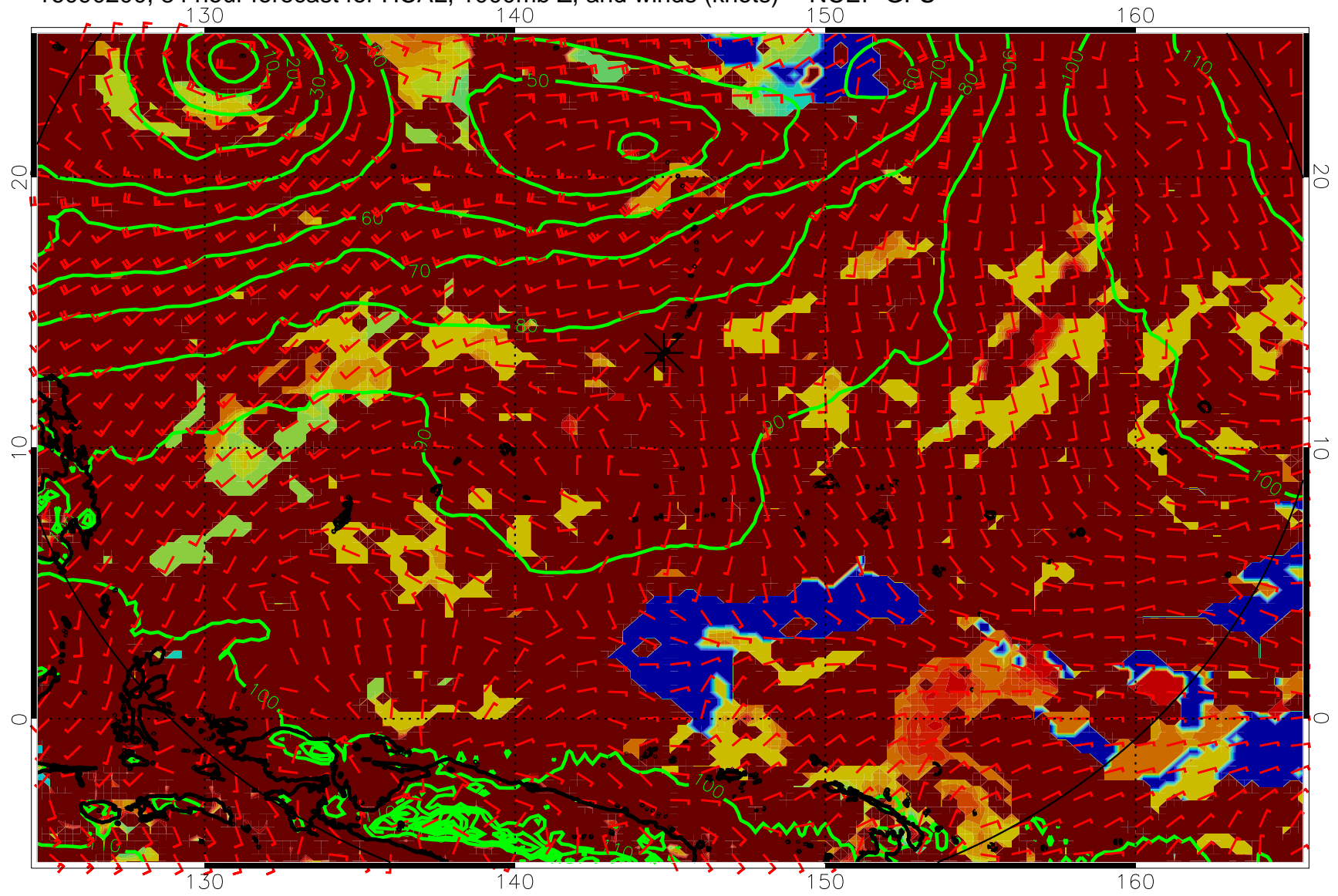
16090200, 84 hour forecast for HCAL, 1000mb Z, and winds (knots) -- NCEP GFS
