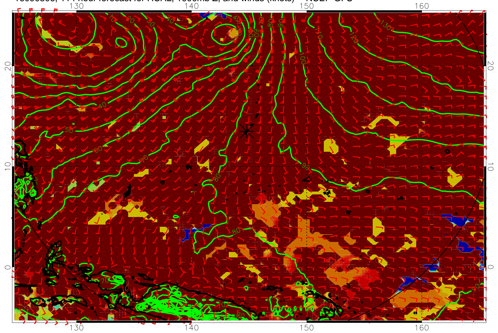
16090306, 114 hour forecast for HCAL, 1000mb Z, and winds (knots) -- NCEP GFS
