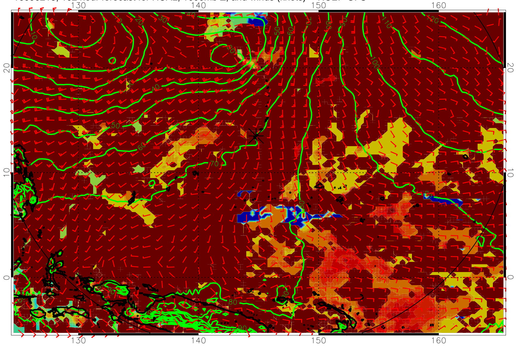
16090218, 102 hour forecast for HCAL, 1000mb Z, and winds (knots) -- NCEP GFS
