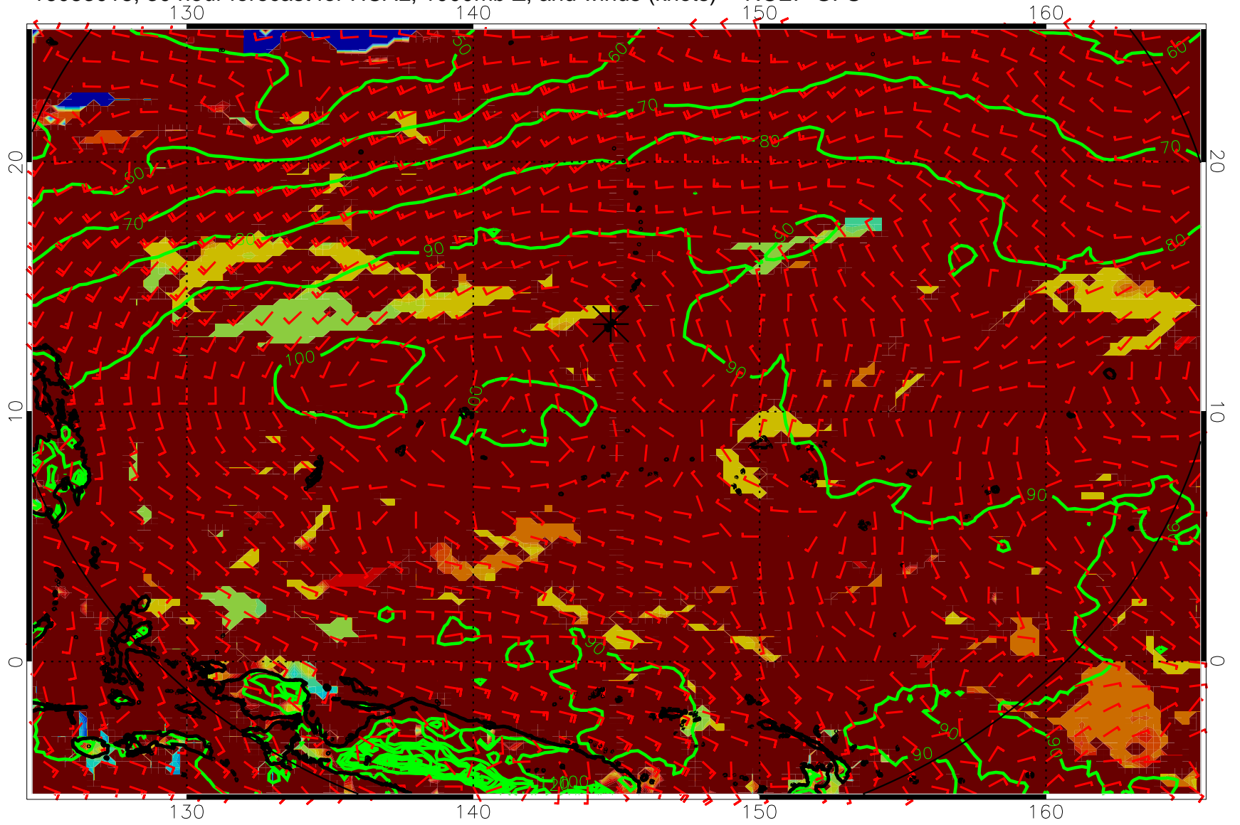
16083018, 30 hour forecast for HCAL, 1000mb Z, and winds (knots) -- NCEP GFS
