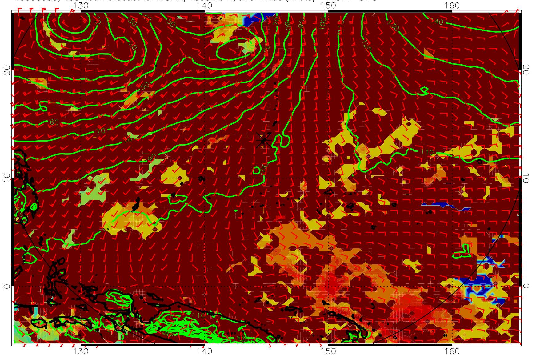
16090300, 108 hour forecast for HCAL, 1000mb Z, and winds (knots) -- NCEP GFS
