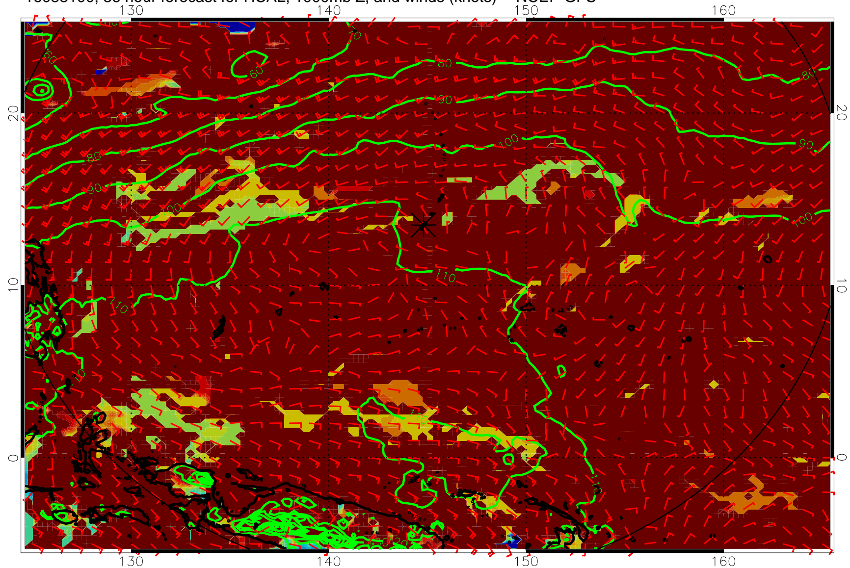
16083100, 36 hour forecast for HCAL, 1000mb Z, and winds (knots) -- NCEP GFS
