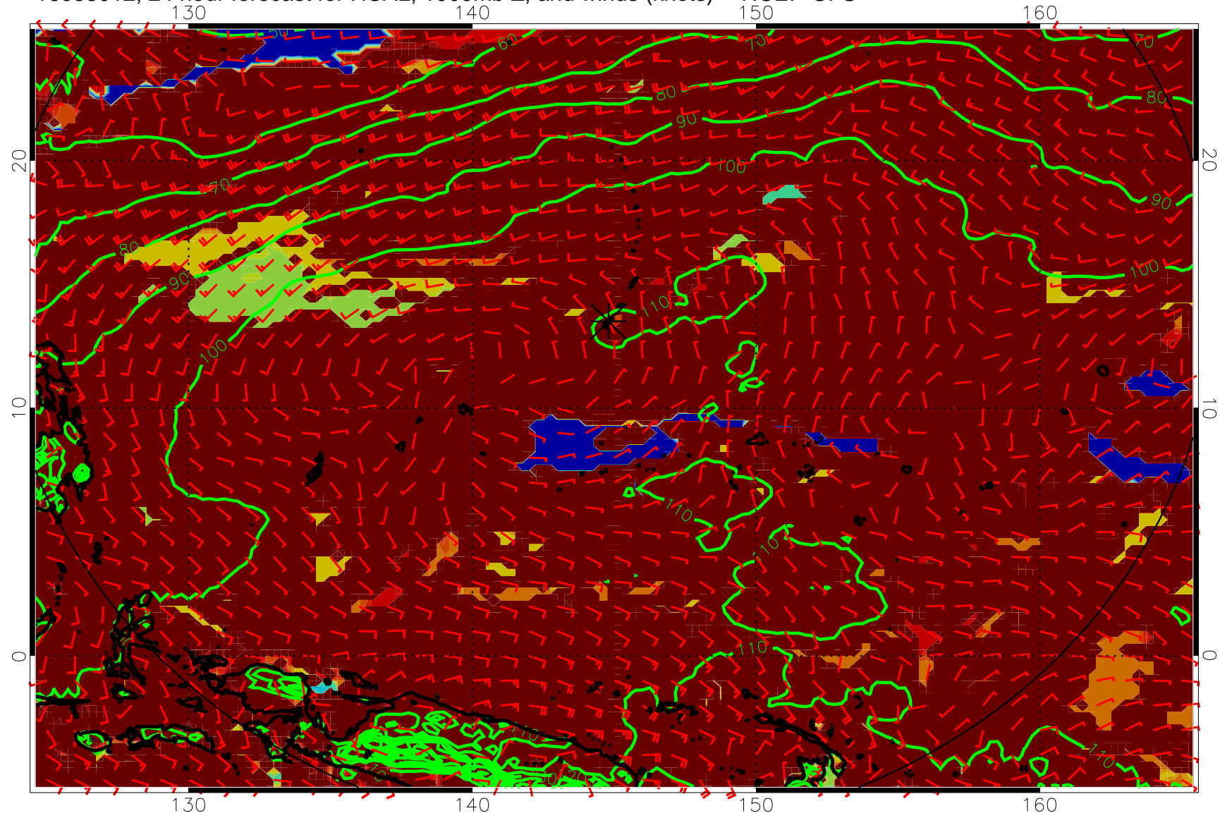
16083012, 24 hour forecast for HCAL, 1000mb Z, and winds (knots) -- NCEP GFS
