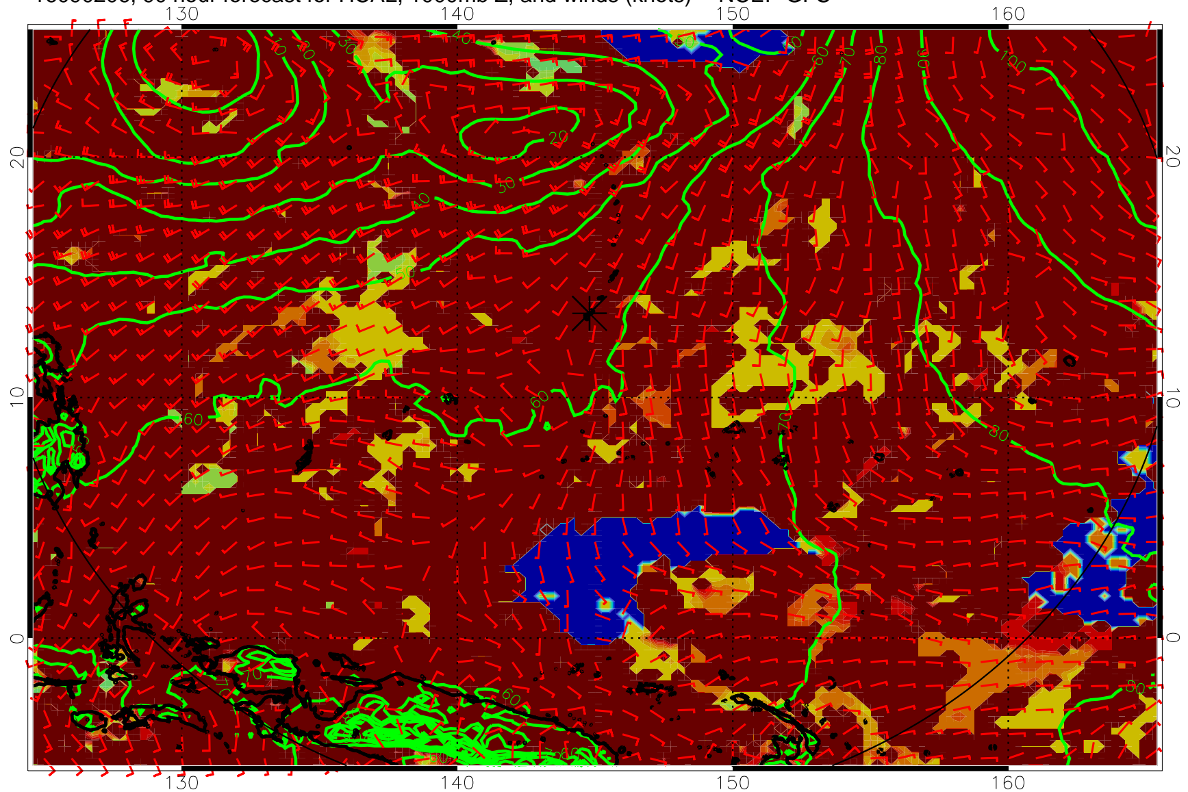
16090206, 90 hour forecast for HCAL, 1000mb Z, and winds (knots) -- NCEP GFS
