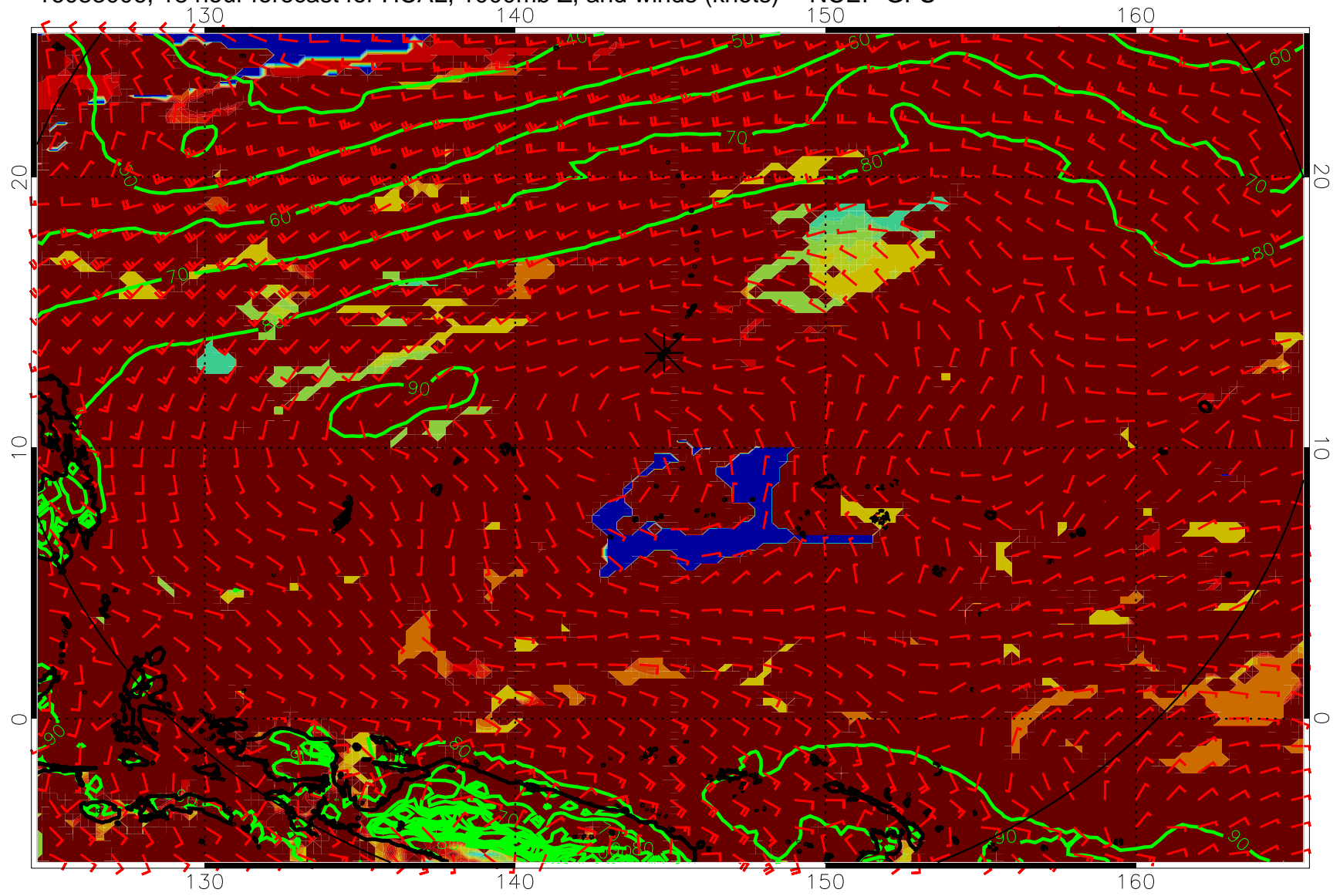
16083006, 18 hour forecast for HCAL, 1000mb Z, and winds (knots) -- NCEP GFS
