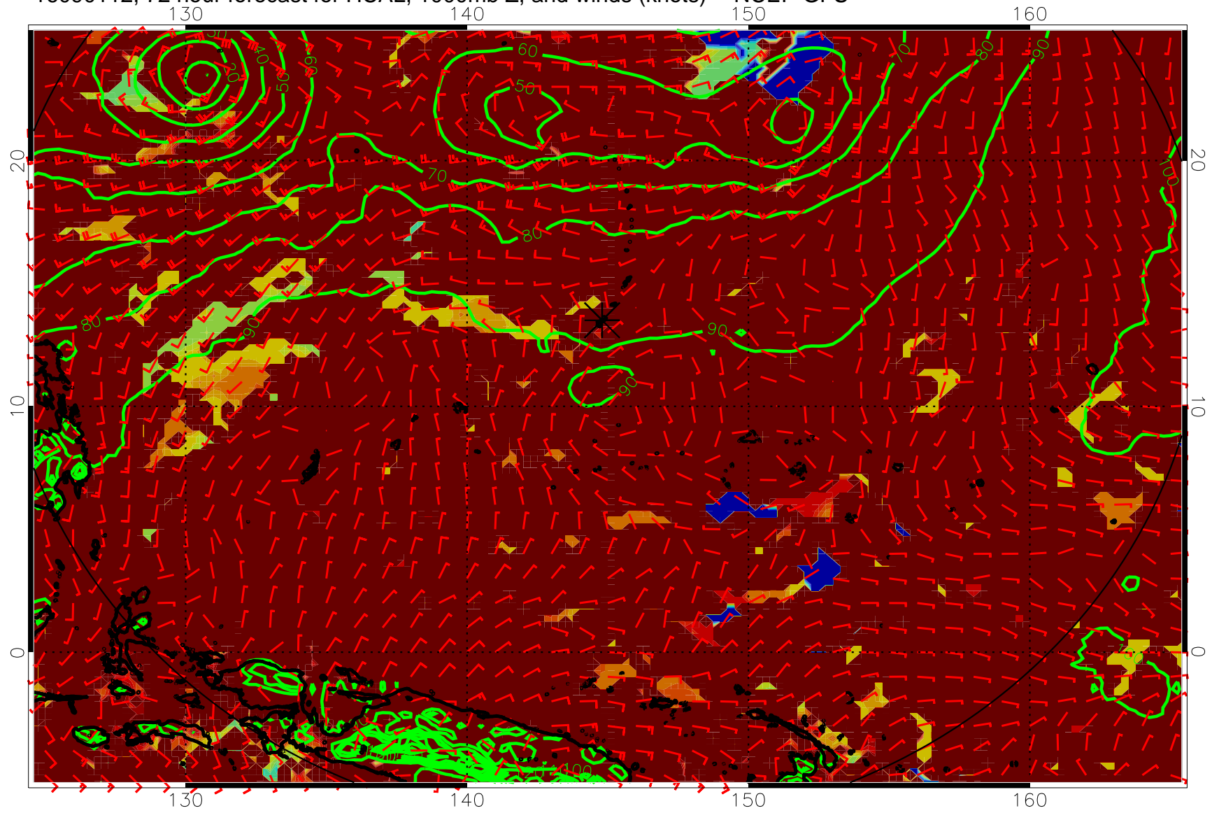
16090112, 72 hour forecast for HCAL, 1000mb Z, and winds (knots) -- NCEP GFS
