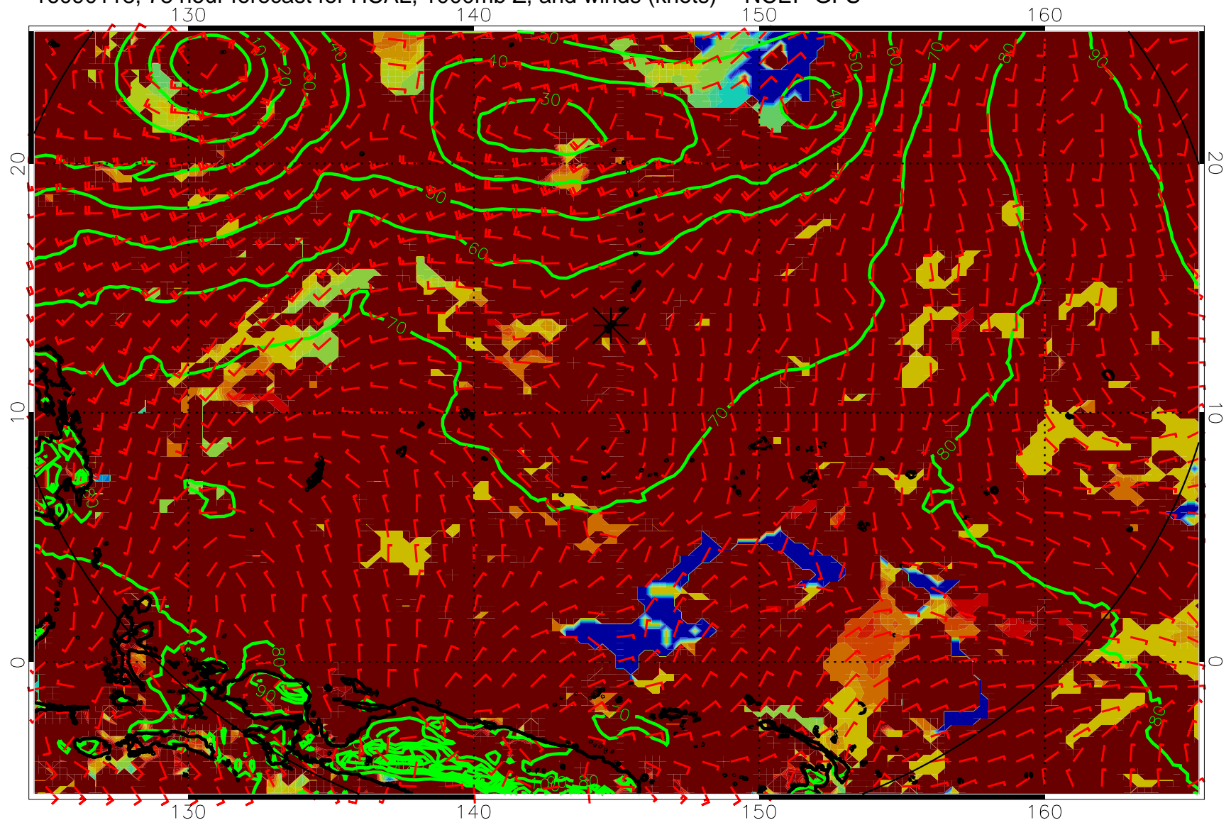
16090118, 78 hour forecast for HCAL, 1000mb Z, and winds (knots) -- NCEP GFS
