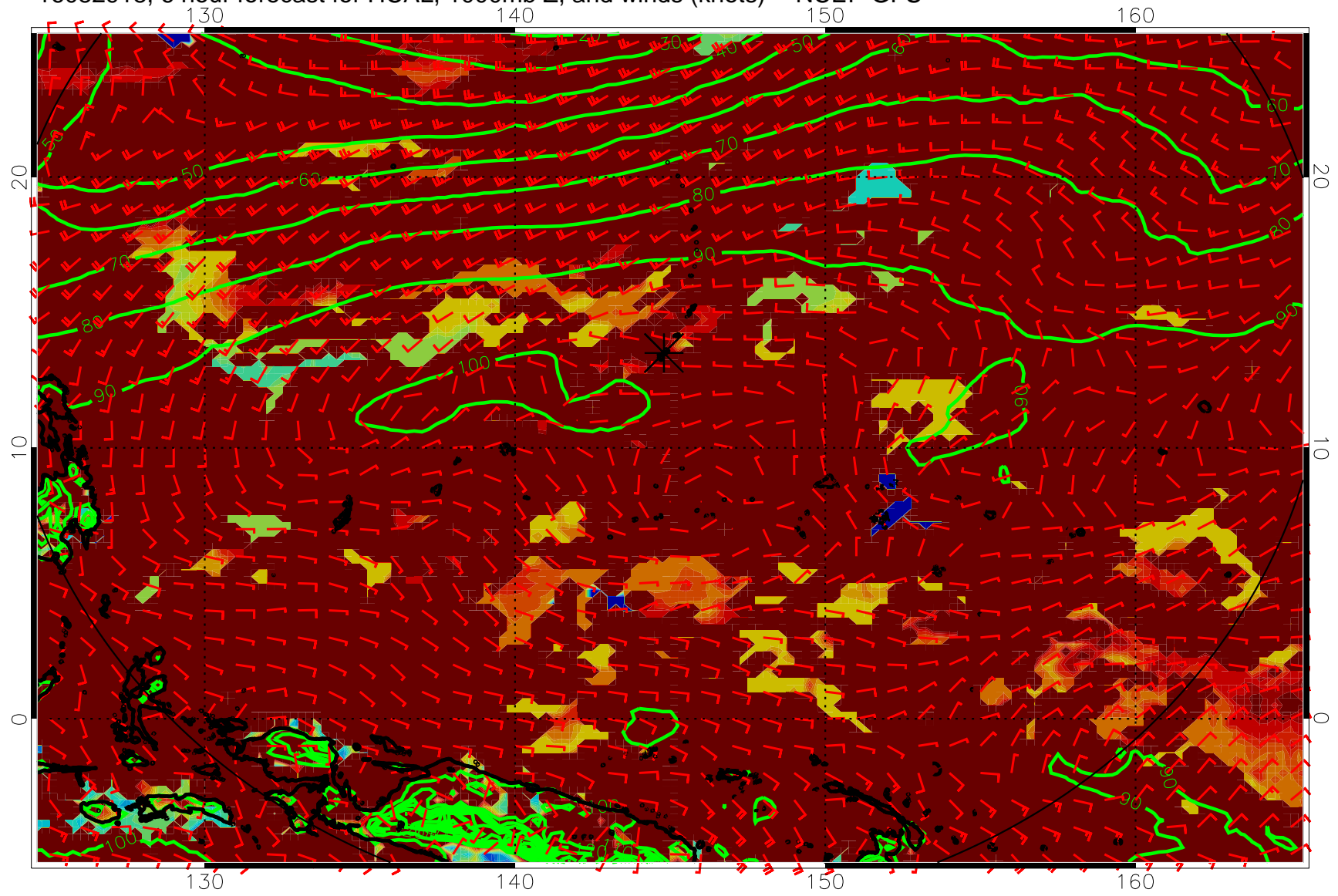
16082918, 6 hour forecast for HCAL, 1000mb Z, and winds (knots) -- NCEP GFS
