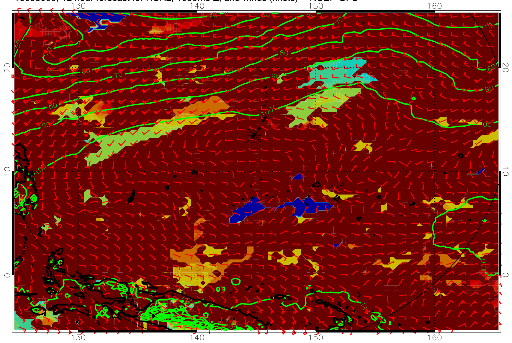
16083000, 12 hour forecast for HCAL, 1000mb Z, and winds (knots) -- NCEP GFS
