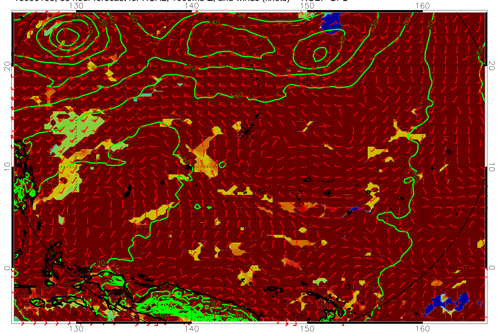
16090106, 66 hour forecast for HCAL, 1000mb Z, and winds (knots) -- NCEP GFS
