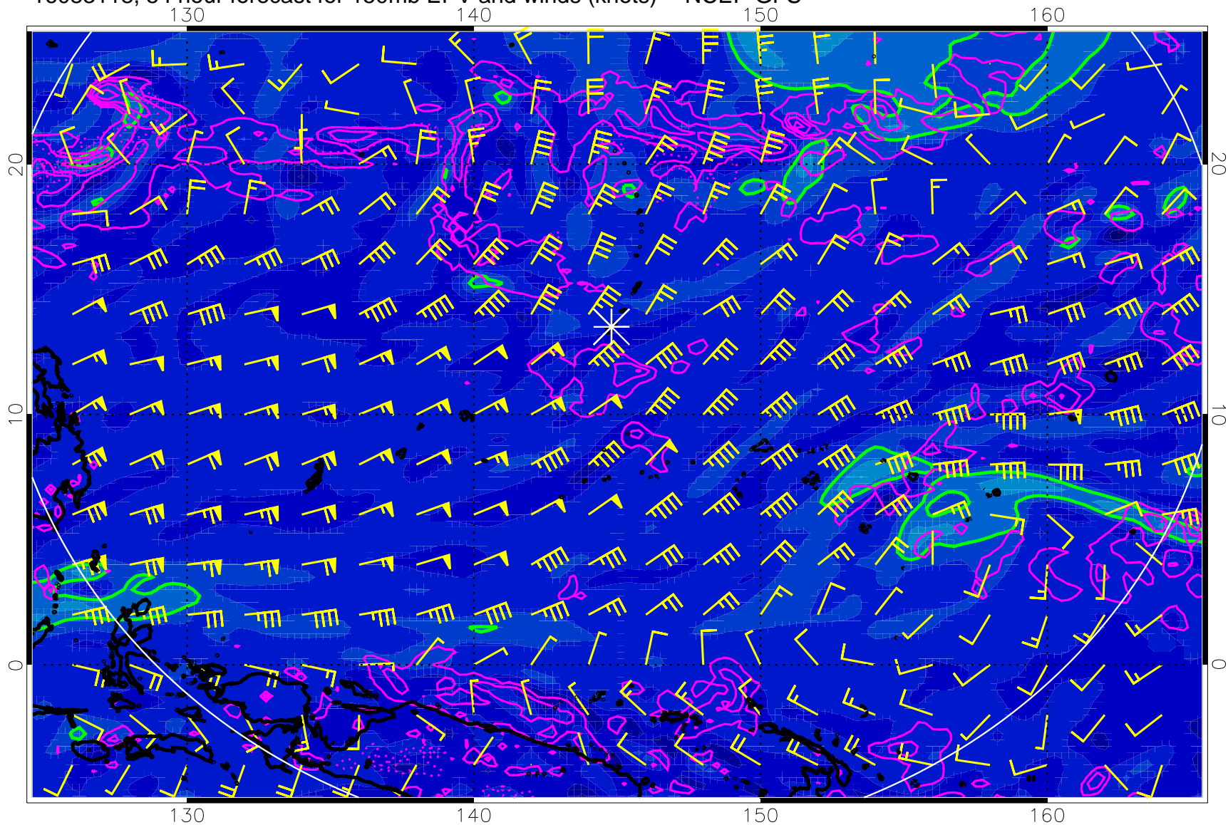
16083118, 54 hour forecast for 150mb EPV and winds (knots) -- NCEP GFS
