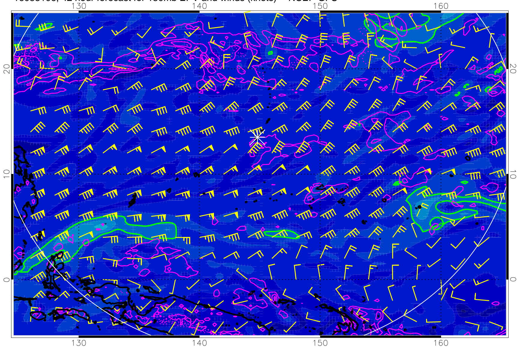
16083106, 42 hour forecast for 150mb EPV and winds (knots) -- NCEP GFS
