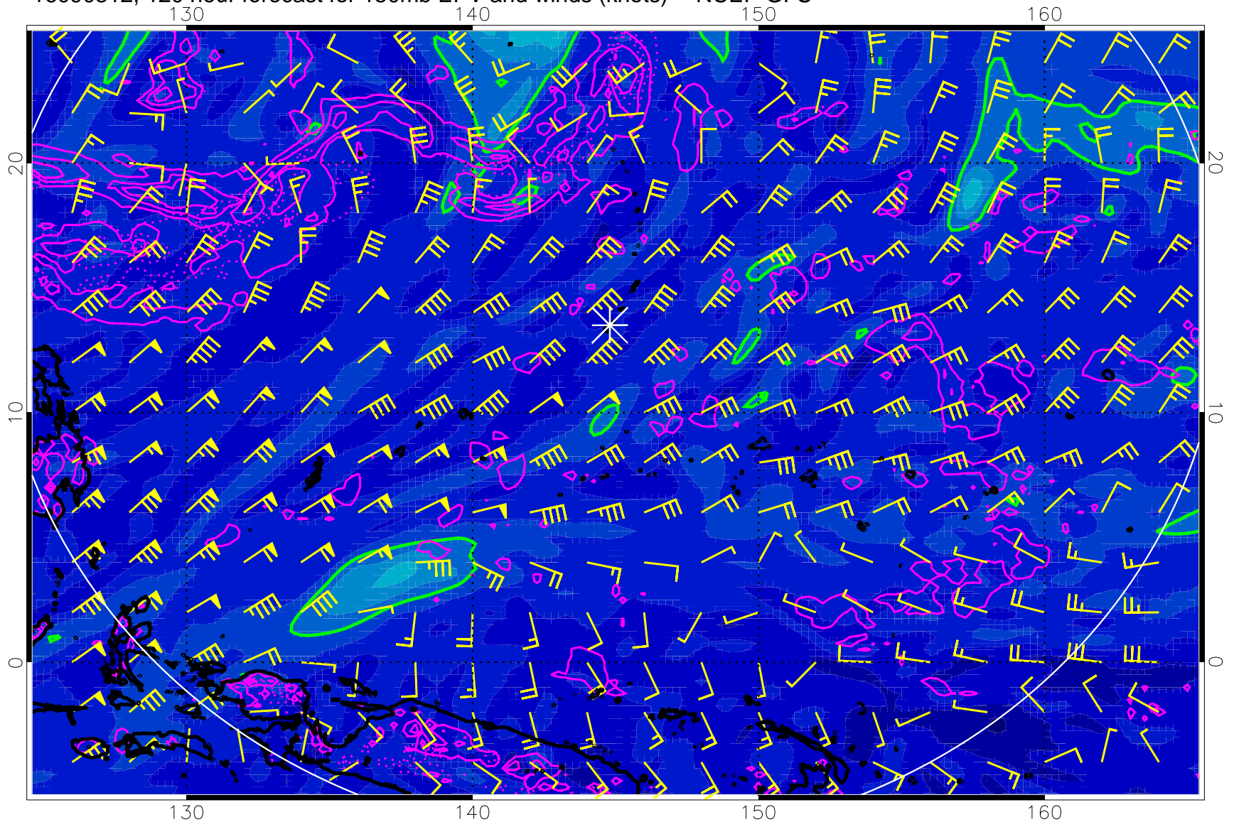
16090312, 120 hour forecast for 150mb EPV and winds (knots) -- NCEP GFS
