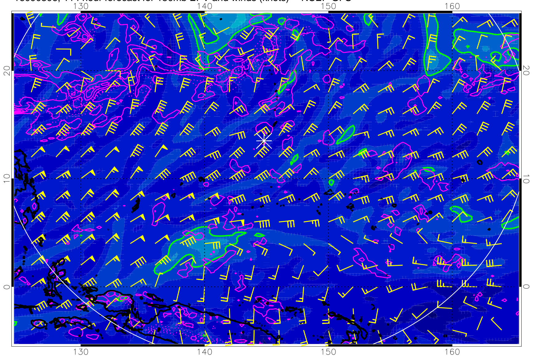
16090306, 114 hour forecast for 150mb EPV and winds (knots) -- NCEP GFS
