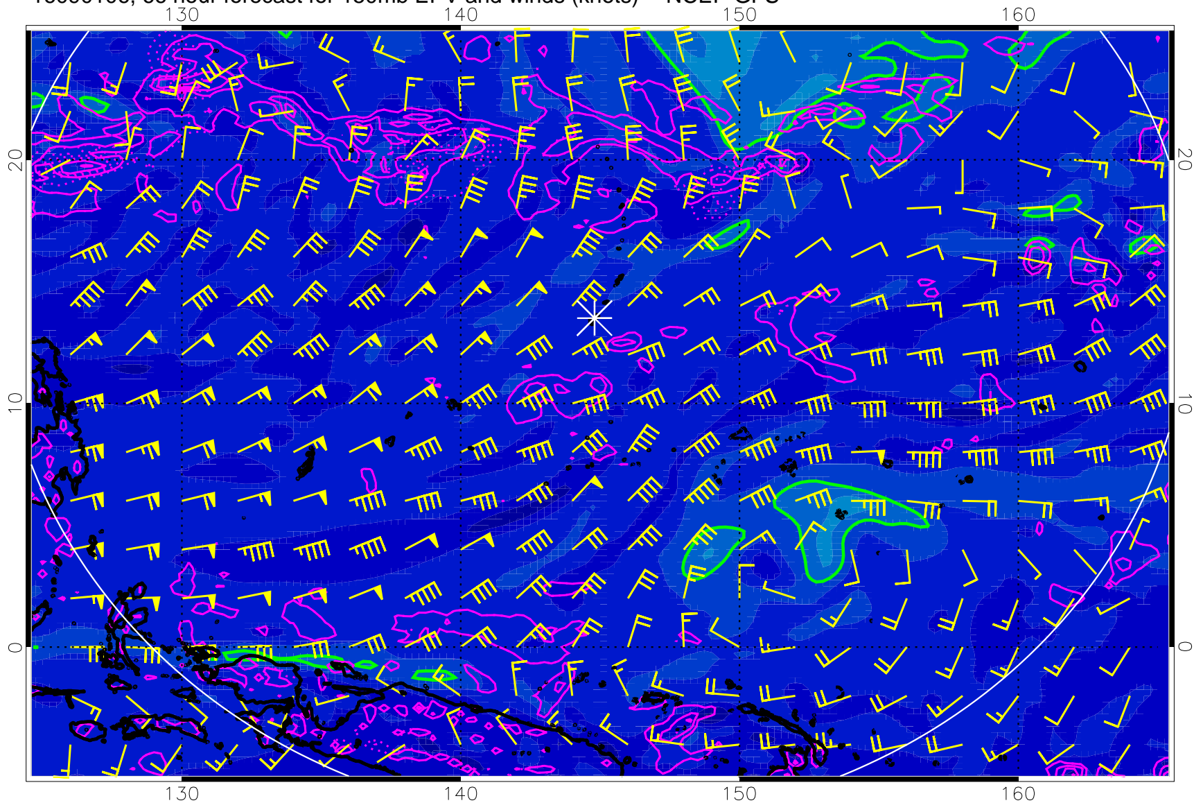
16090106, 66 hour forecast for 150mb EPV and winds (knots) -- NCEP GFS
