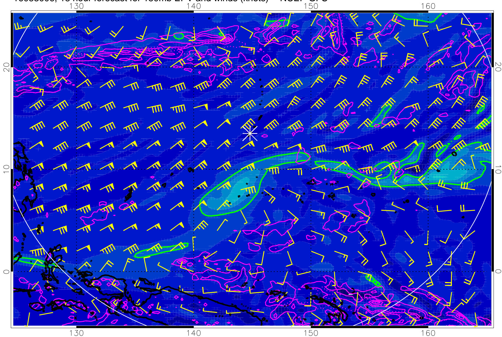
16083006, 18 hour forecast for 150mb EPV and winds (knots) -- NCEP GFS
