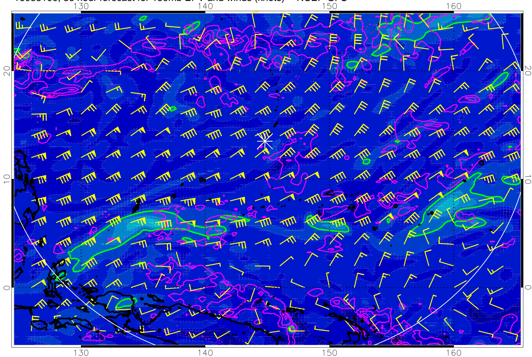
16083100, 36 hour forecast for 150mb EPV and winds (knots) -- NCEP GFS
