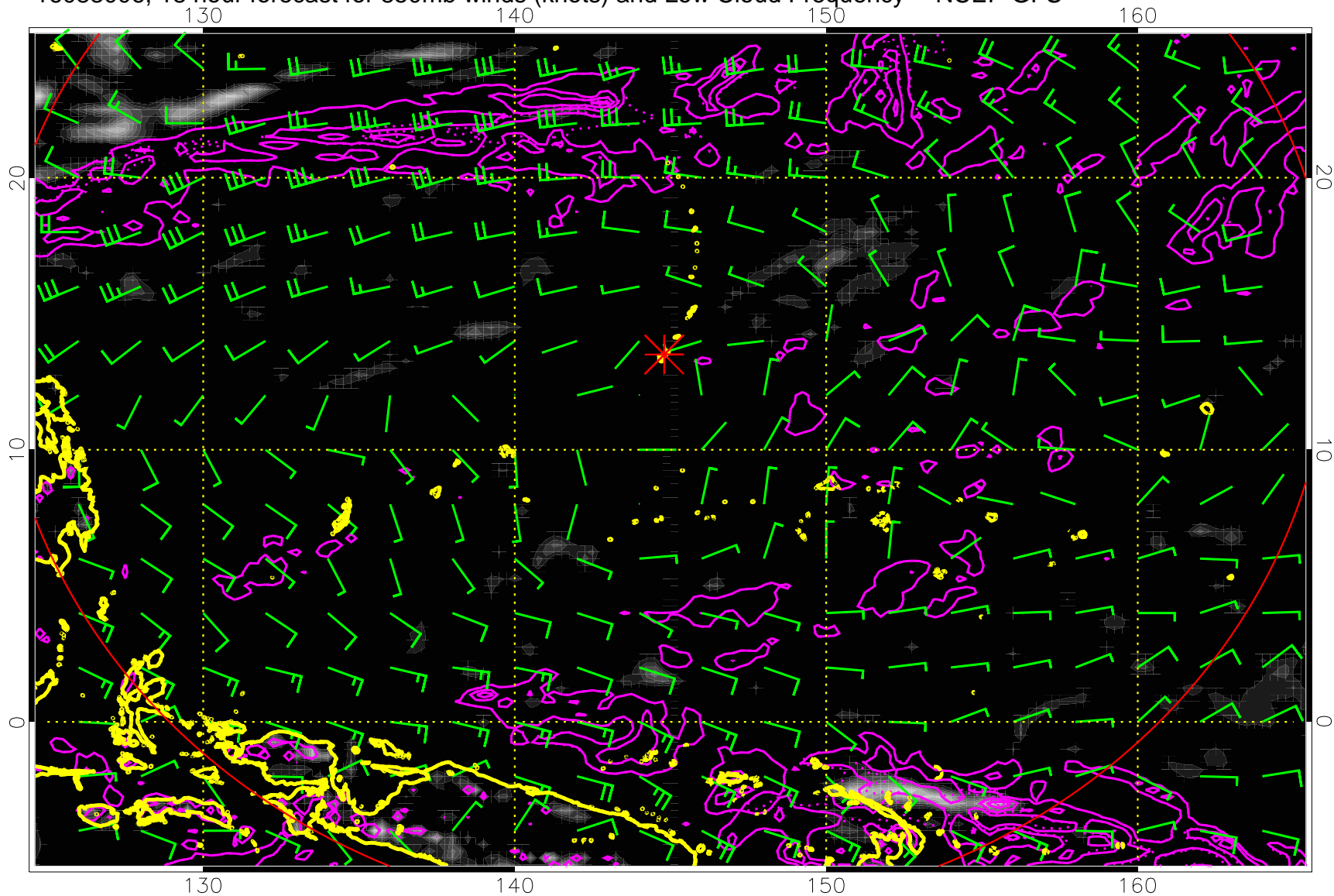
16083006, 18 hour forecast for 850mb winds (knots) and Low Cloud Frequency -- NCEP GFS
