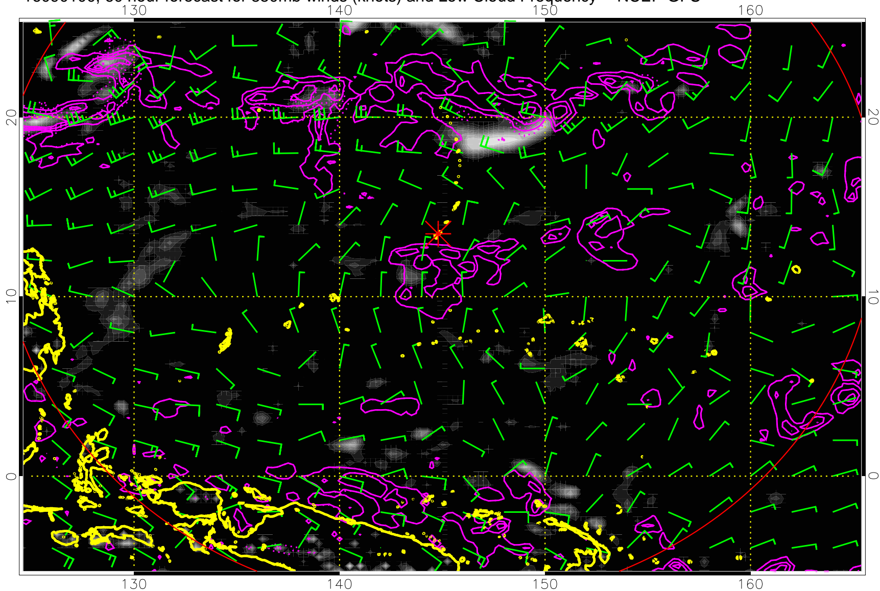
16090100, 60 hour forecast for 850mb winds (knots) and Low Cloud Frequency -- NCEP GFS
