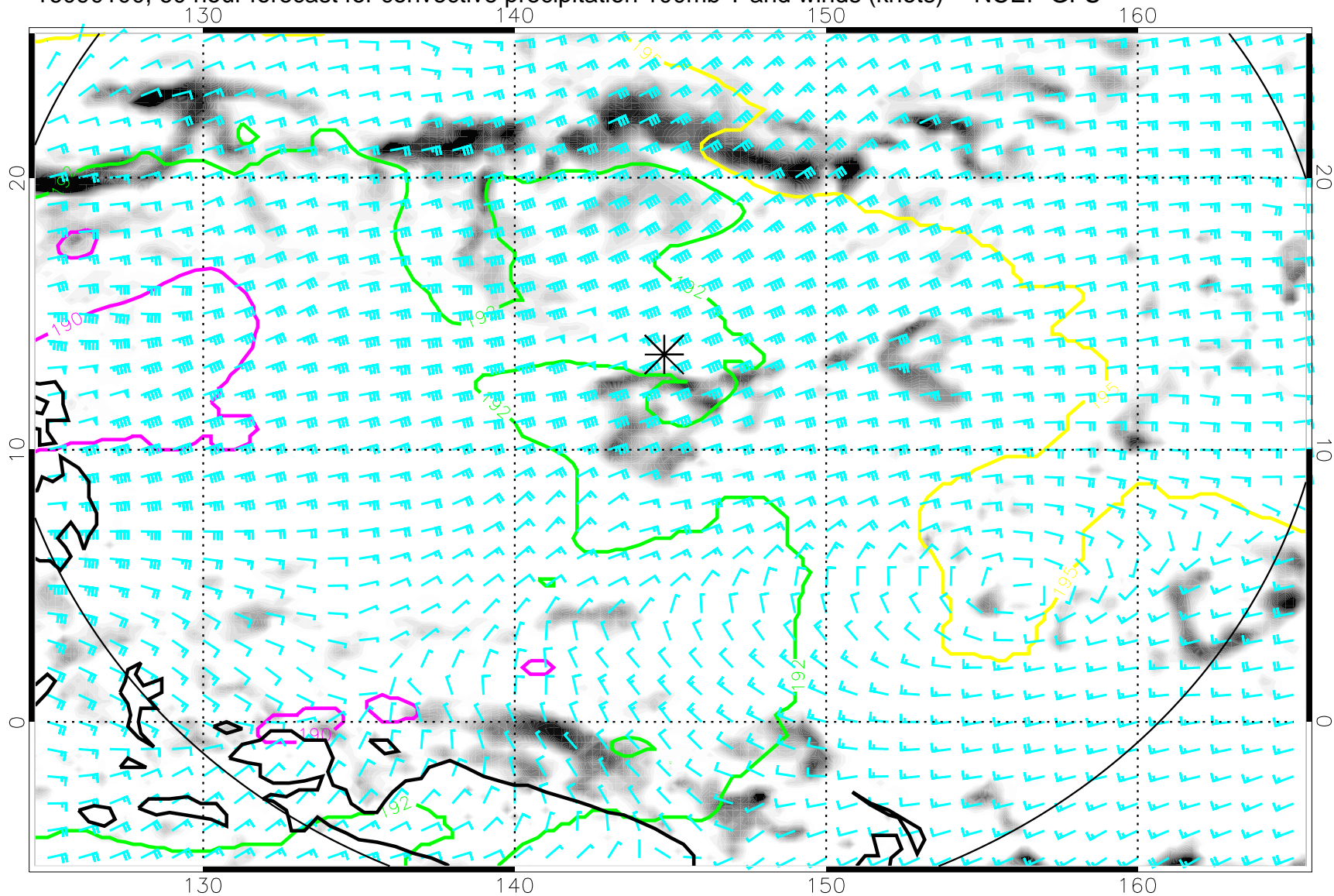
16090100, 60 hour forecast for convective precipitation 100mb T and winds (knots) -- NCEP GFS
