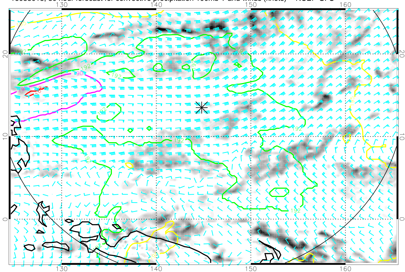
16083018, 30 hour forecast for convective precipitation 100mb T and winds (knots) -- NCEP GFS
