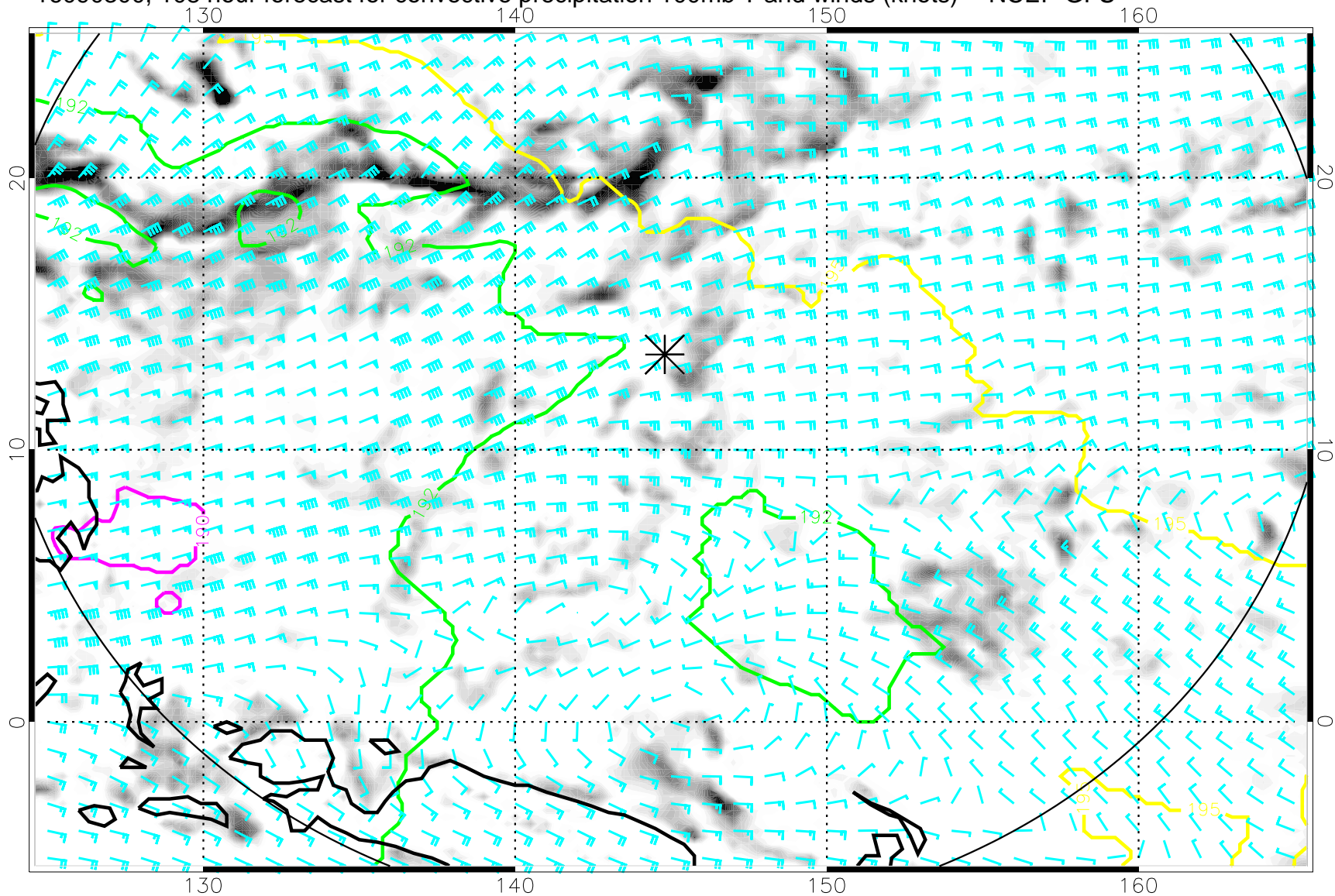
16090300, 108 hour forecast for convective precipitation 100mb T and winds (knots) -- NCEP GFS
