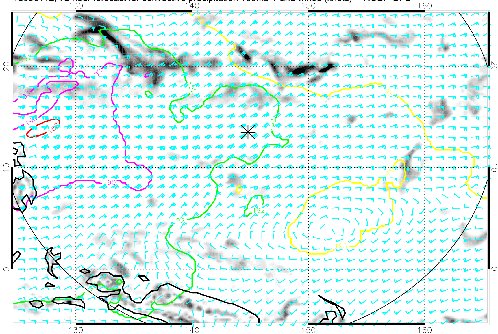
16090112, 72 hour forecast for convective precipitation 100mb T and winds (knots) -- NCEP GFS
