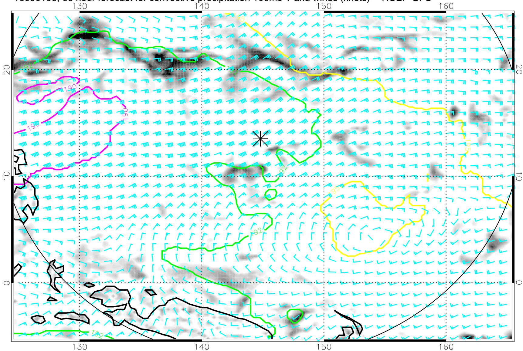
16090106, 66 hour forecast for convective precipitation 100mb T and winds (knots) -- NCEP GFS
