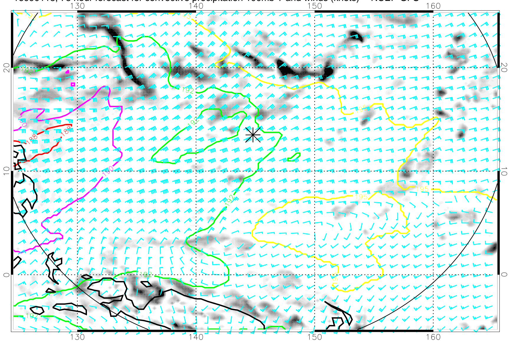
16090118, 78 hour forecast for convective precipitation 100mb T and winds (knots) -- NCEP GFS
