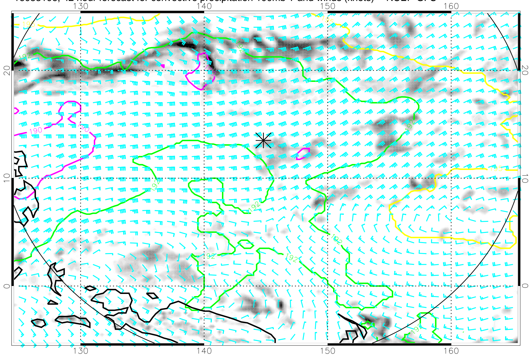
16083106, 42 hour forecast for convective precipitation 100mb T and winds (knots) -- NCEP GFS
