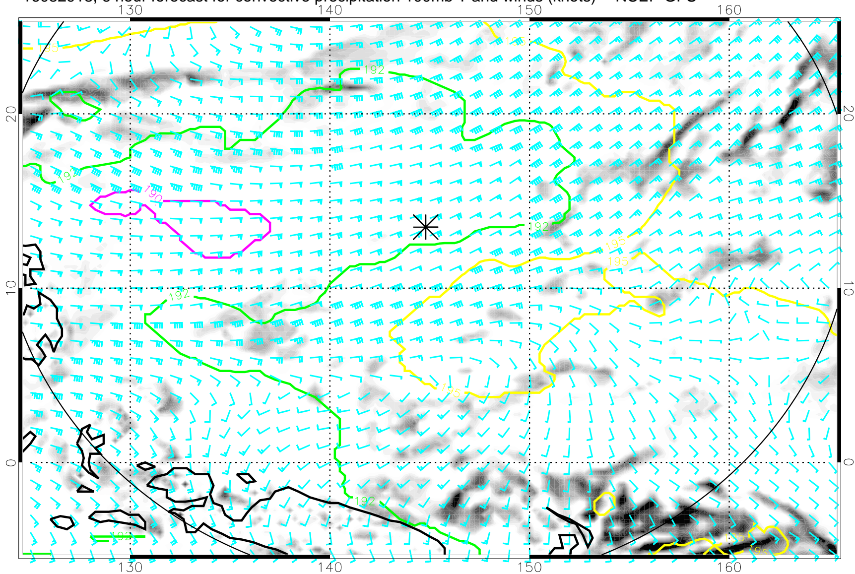
16082918, 6 hour forecast for convective precipitation 100mb T and winds (knots) -- NCEP GFS
