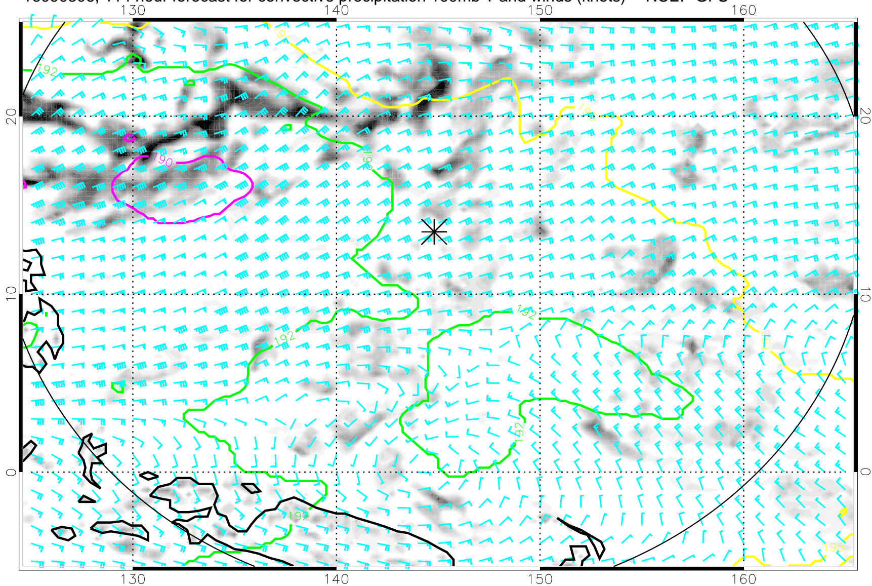
16090306, 114 hour forecast for convective precipitation 100mb T and winds (knots) -- NCEP GFS
