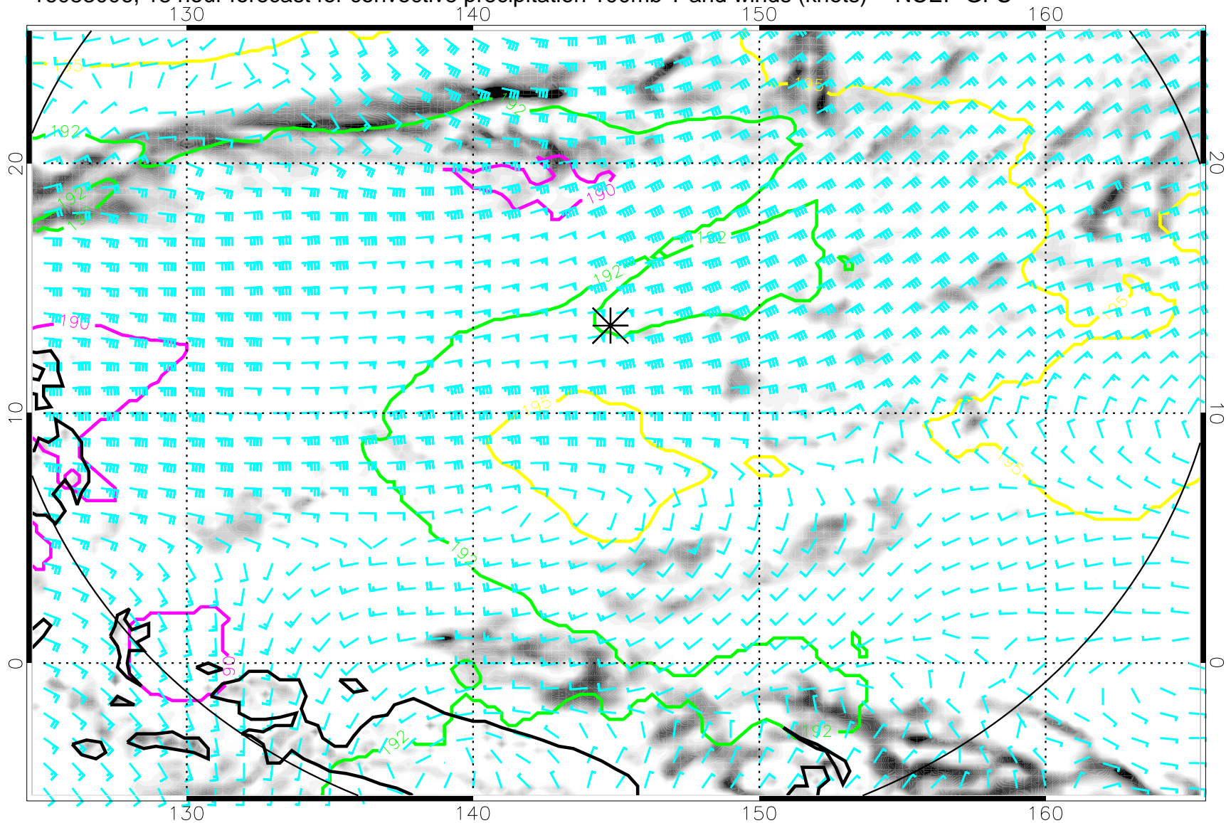
16083006, 18 hour forecast for convective precipitation 100mb T and winds (knots) -- NCEP GFS
