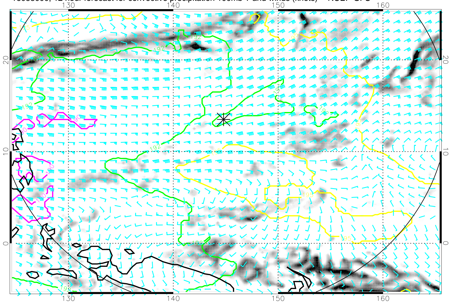
16083000, 12 hour forecast for convective precipitation 100mb T and winds (knots) -- NCEP GFS
