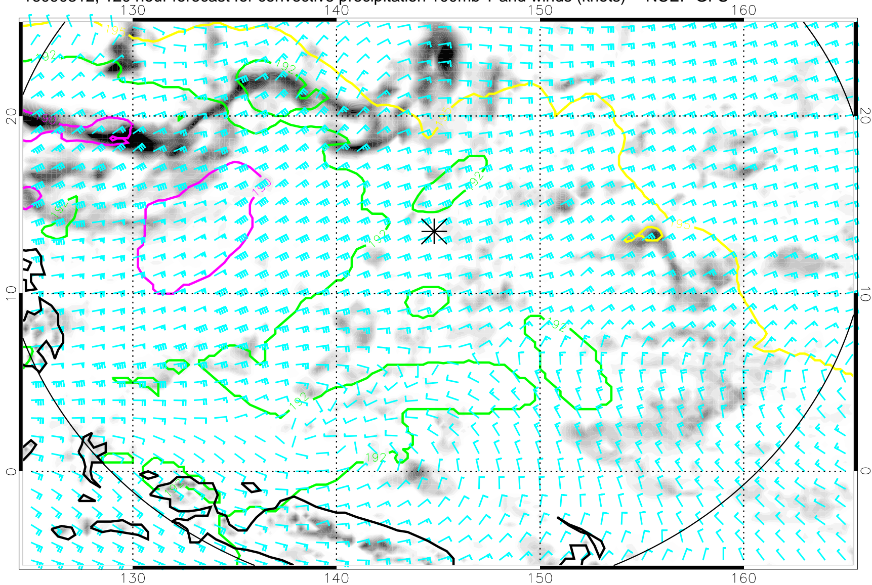
16090312, 120 hour forecast for convective precipitation 100mb T and winds (knots) -- NCEP GFS
