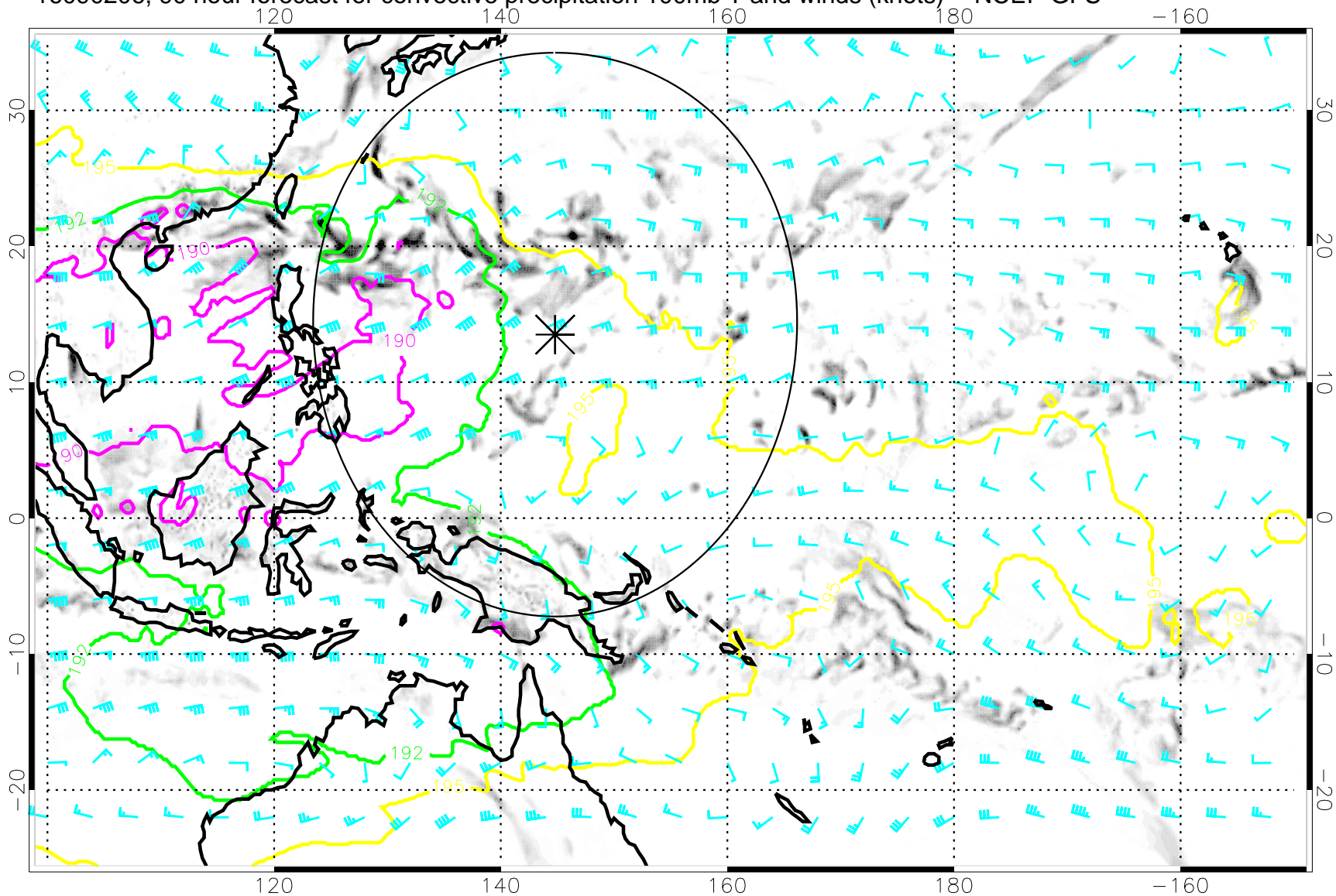
16090206, 90 hour forecast for convective precipitation 100mb T and winds (knots) -- NCEP GFS
