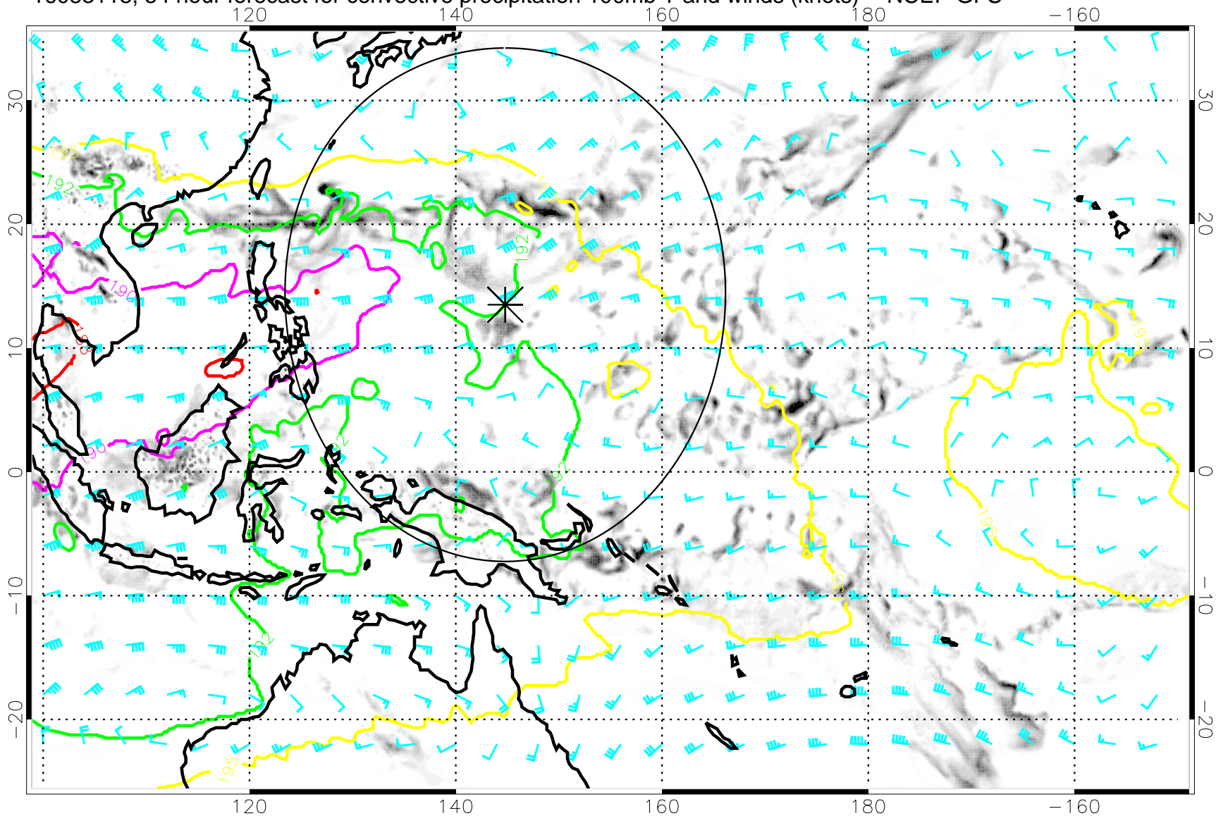
16083118, 54 hour forecast for convective precipitation 100mb T and winds (knots) -- NCEP GFS
