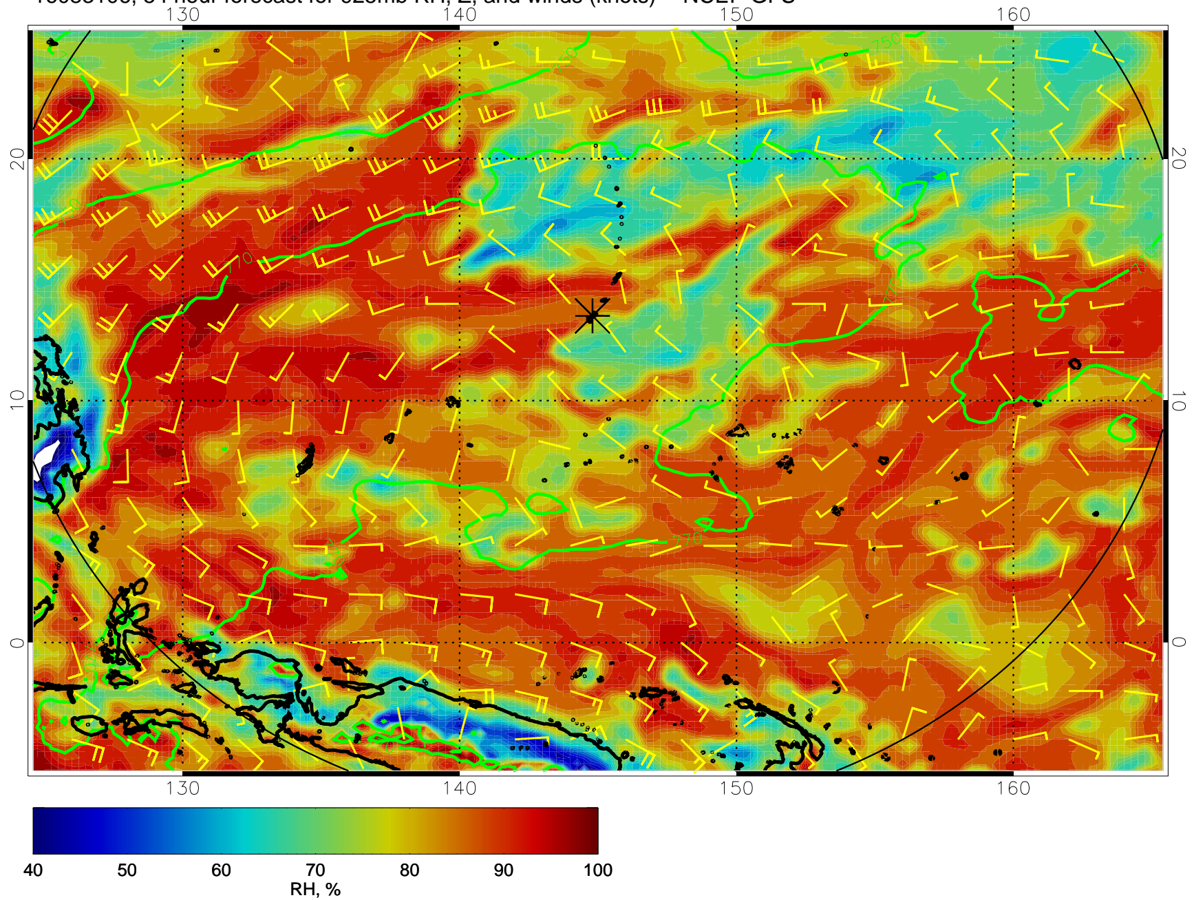
16083106, 54 hour forecast for 925mb RH, Z, and winds (knots) -- NCEP GFS
