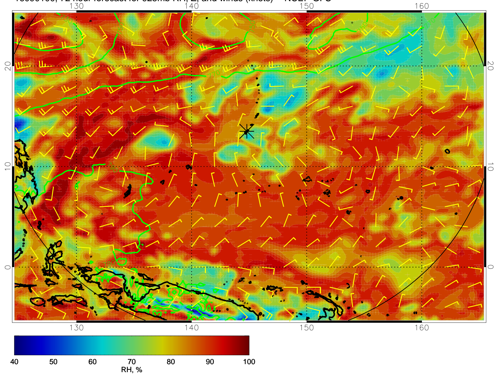
16090100, 72 hour forecast for 925mb RH, Z, and winds (knots) -- NCEP GFS
