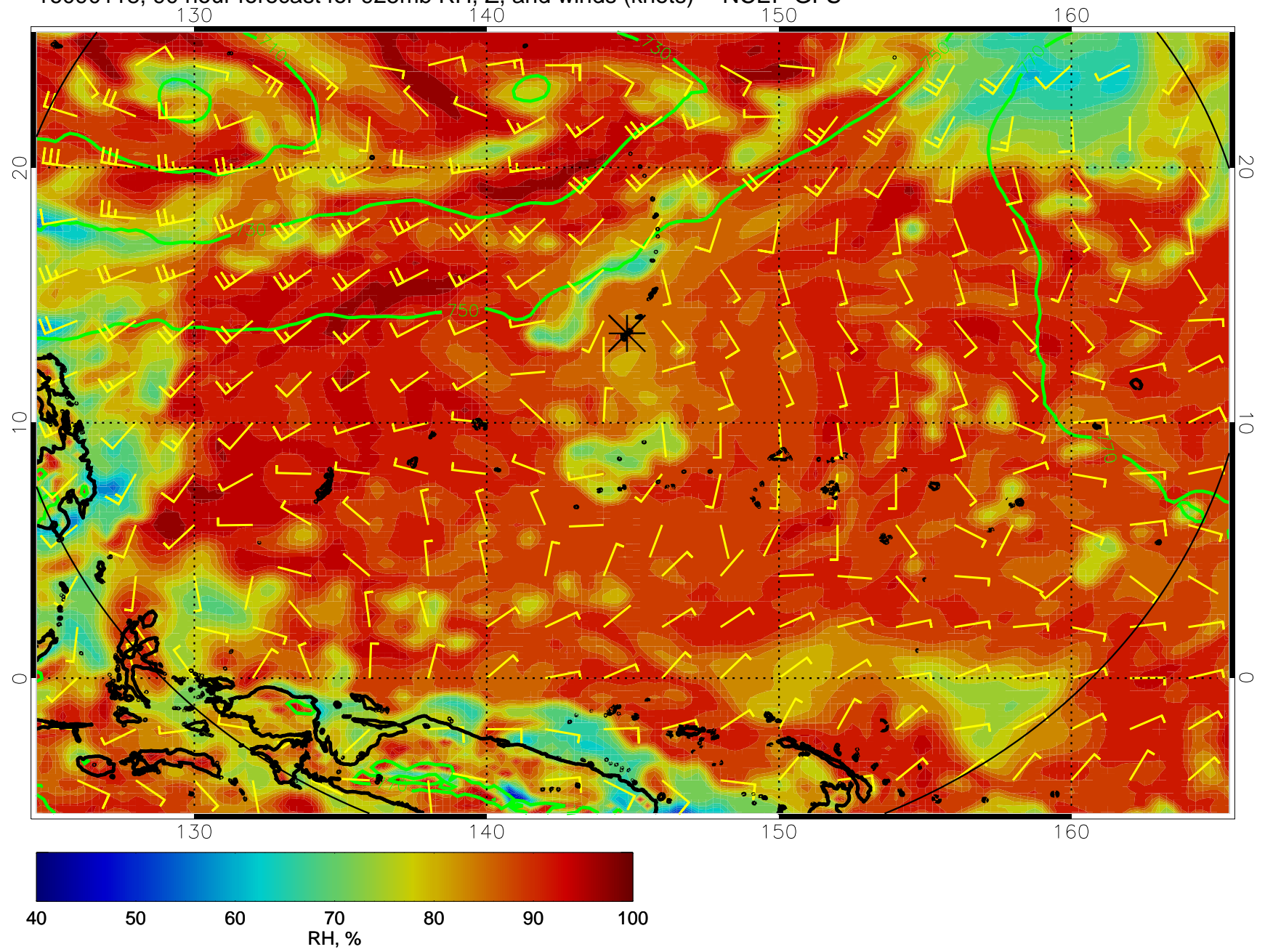
16090118, 90 hour forecast for 925mb RH, Z, and winds (knots) -- NCEP GFS
