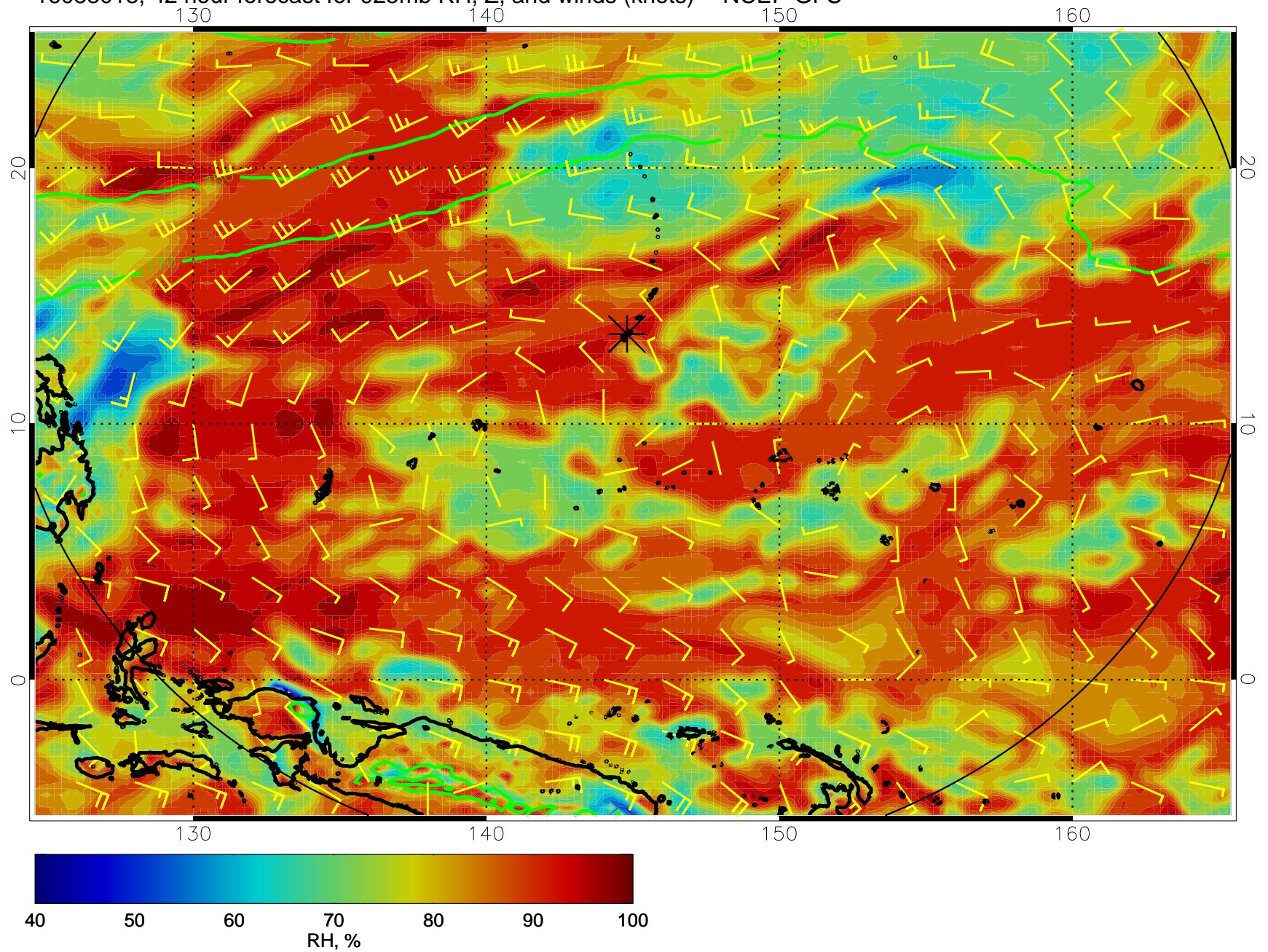
16083018, 42 hour forecast for 925mb RH, Z, and winds (knots) -- NCEP GFS
