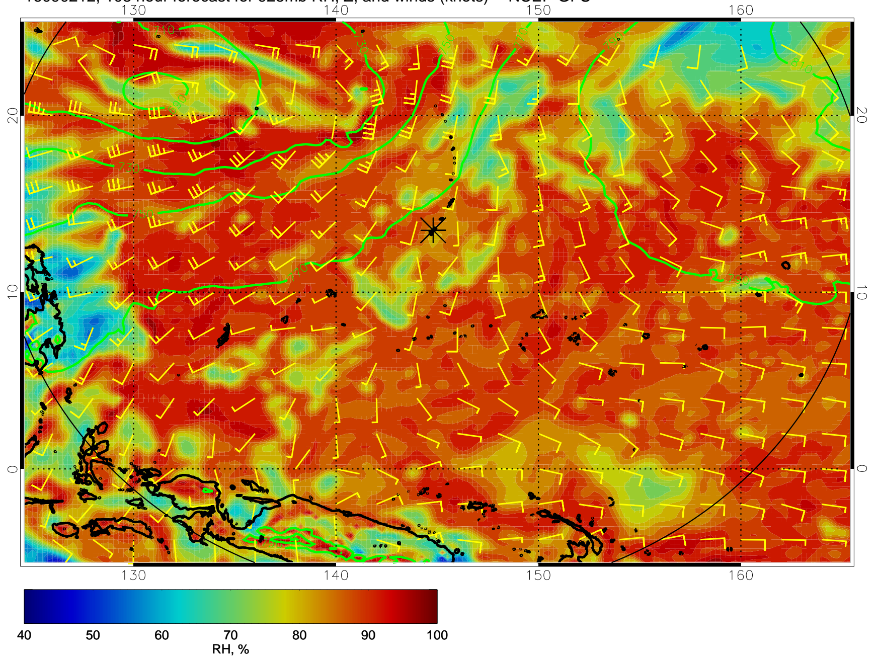
16090212, 108 hour forecast for 925mb RH, Z, and winds (knots) -- NCEP GFS
