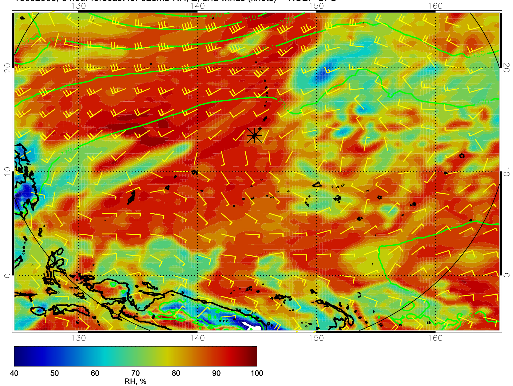
16082906, 6 hour forecast for 925mb RH, Z, and winds (knots) -- NCEP GFS
