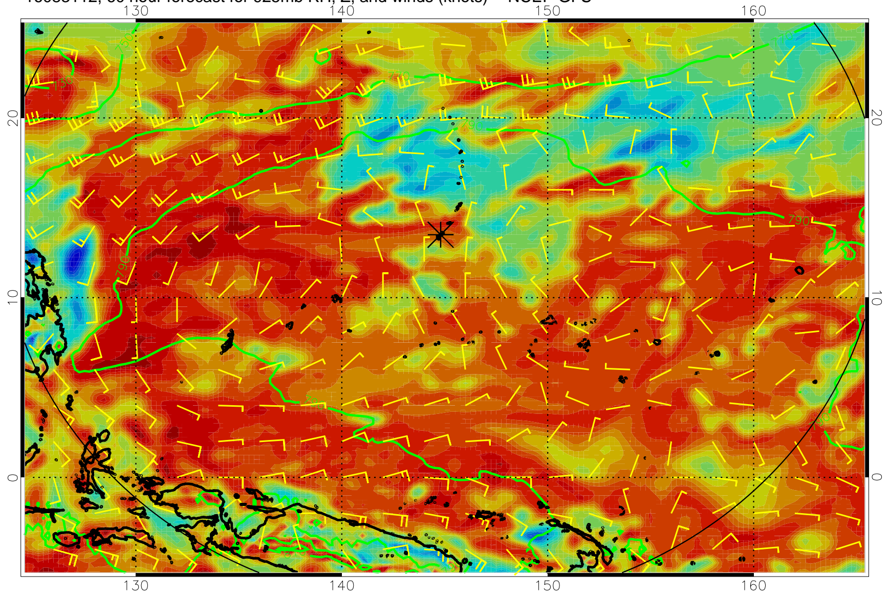
16083112, 60 hour forecast for 925mb RH, Z, and winds (knots) -- NCEP GFS
