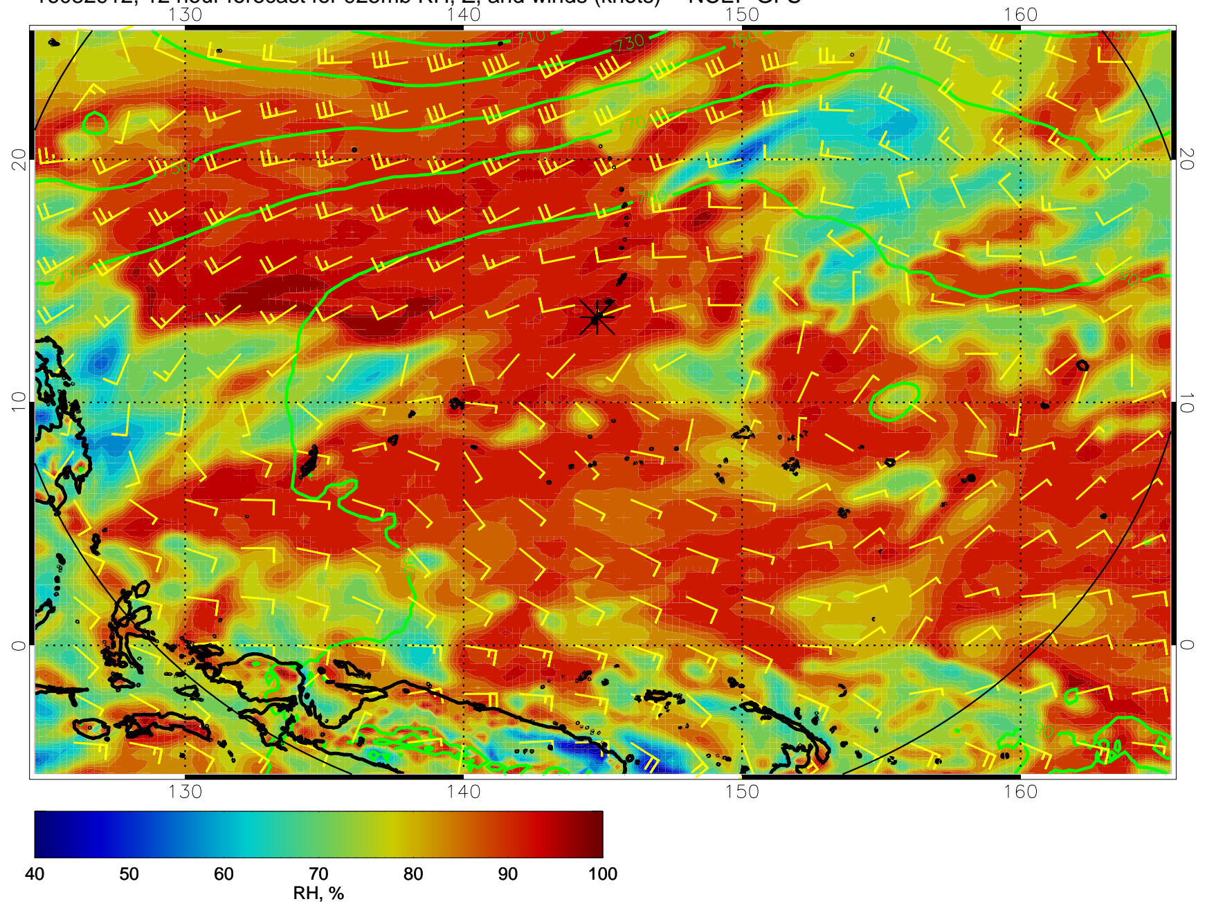
16082912, 12 hour forecast for 925mb RH, Z, and winds (knots) -- NCEP GFS
