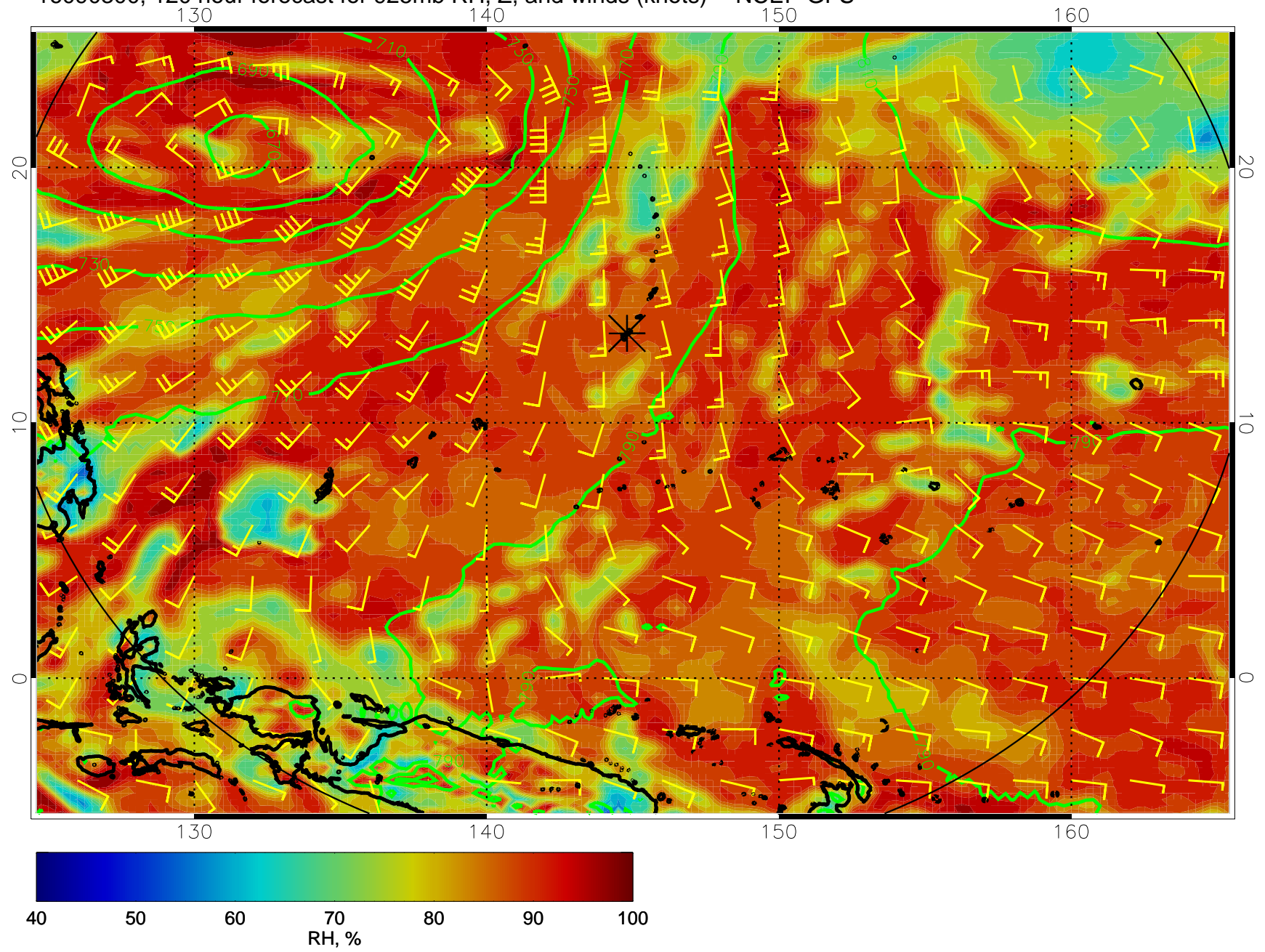
16090300, 120 hour forecast for 925mb RH, Z, and winds (knots) -- NCEP GFS
