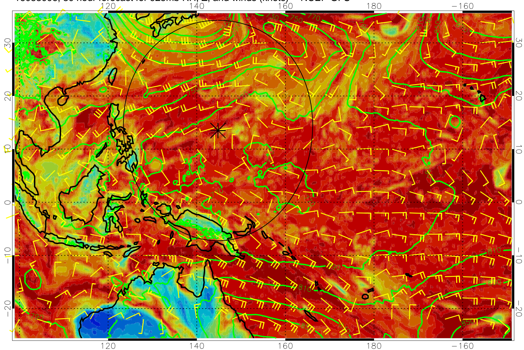
16083006, 30 hour forecast for 925mb RH, Z, and winds (knots) -- NCEP GFS
