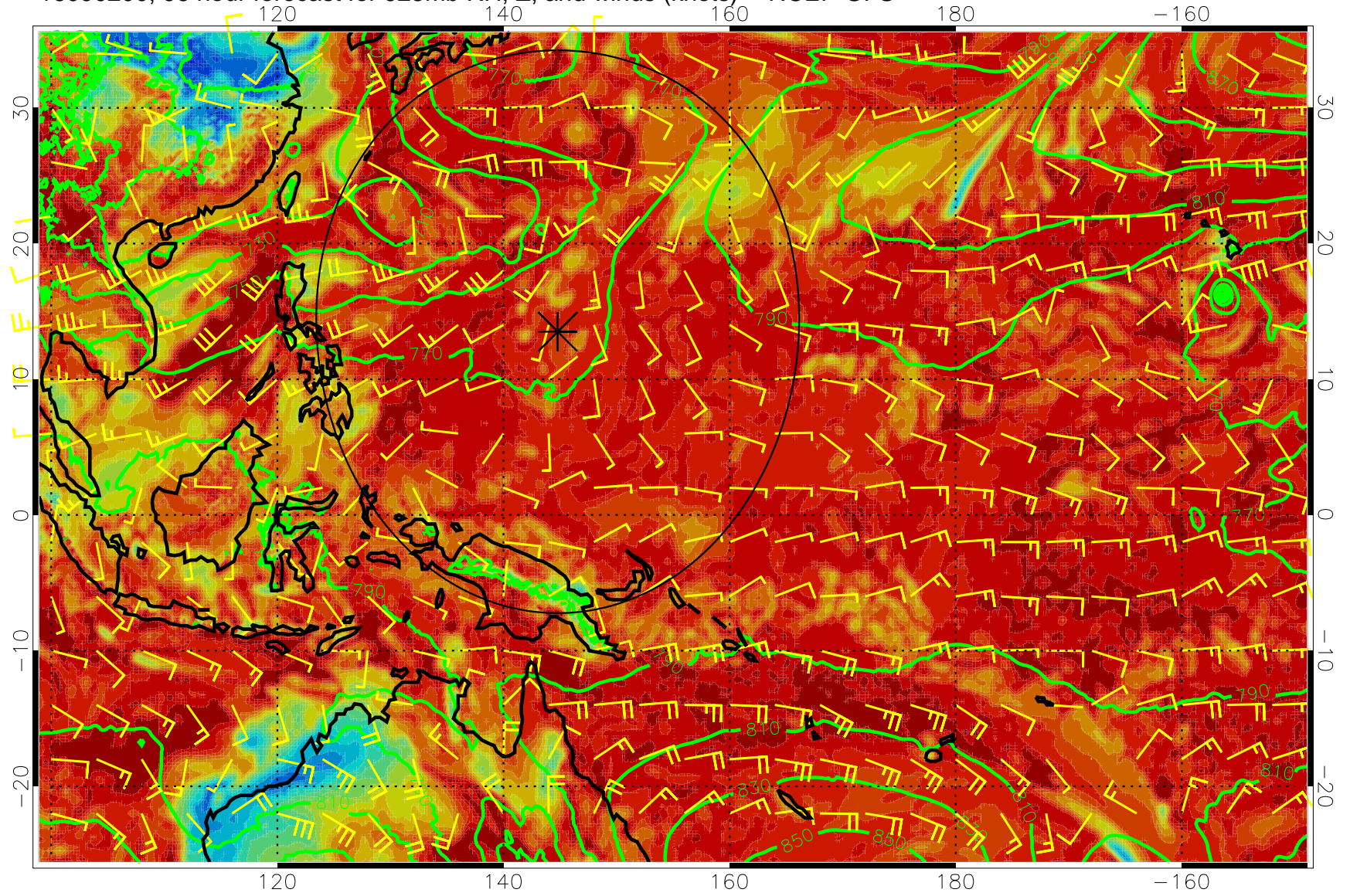
16090200, 96 hour forecast for 925mb RH, Z, and winds (knots) -- NCEP GFS
