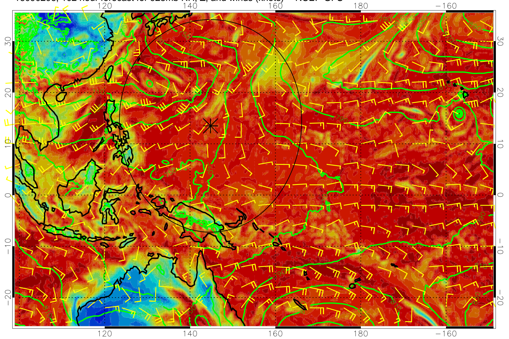
16090206, 102 hour forecast for 925mb RH, Z, and winds (knots) -- NCEP GFS
