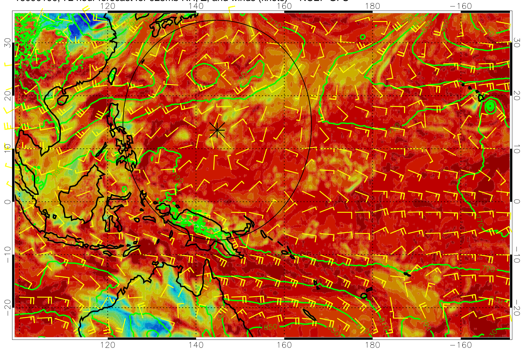
16090100, 72 hour forecast for 925mb RH, Z, and winds (knots) -- NCEP GFS
