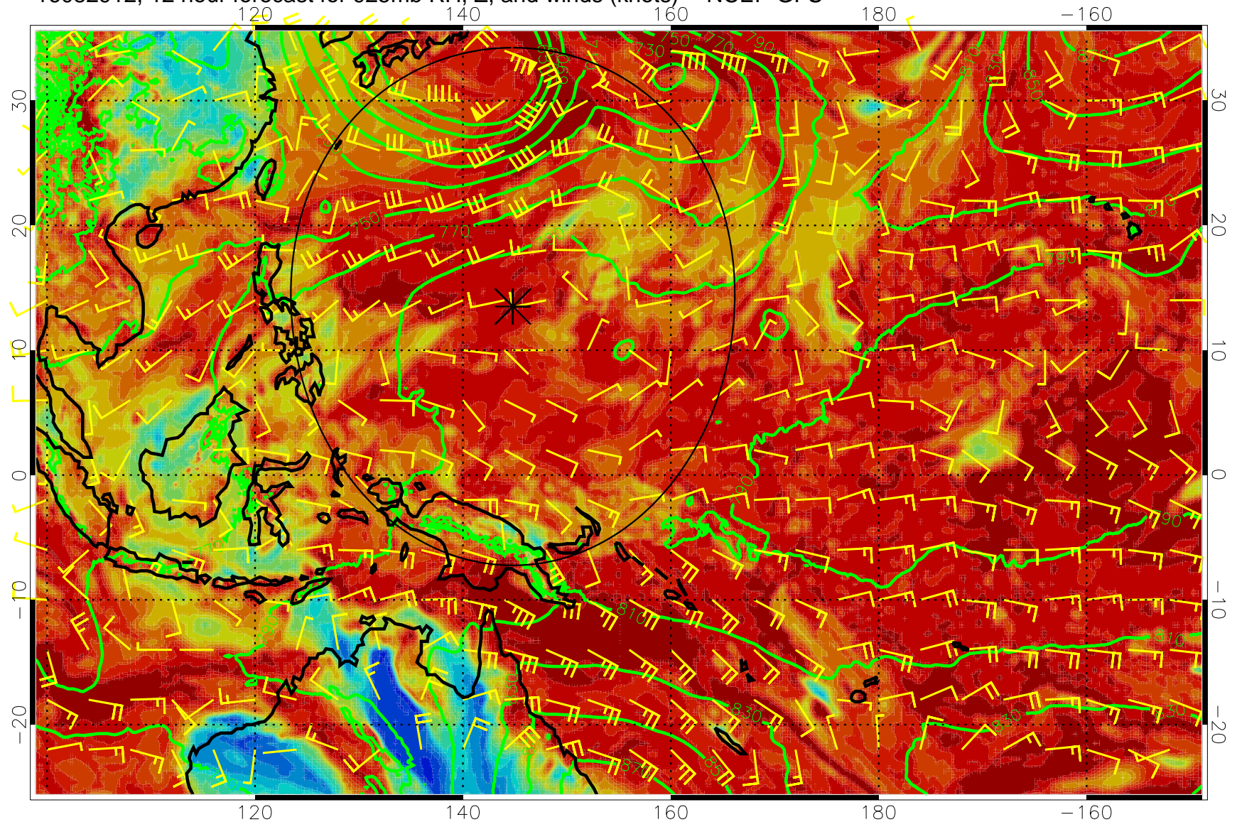
16082912, 12 hour forecast for 925mb RH, Z, and winds (knots) -- NCEP GFS
