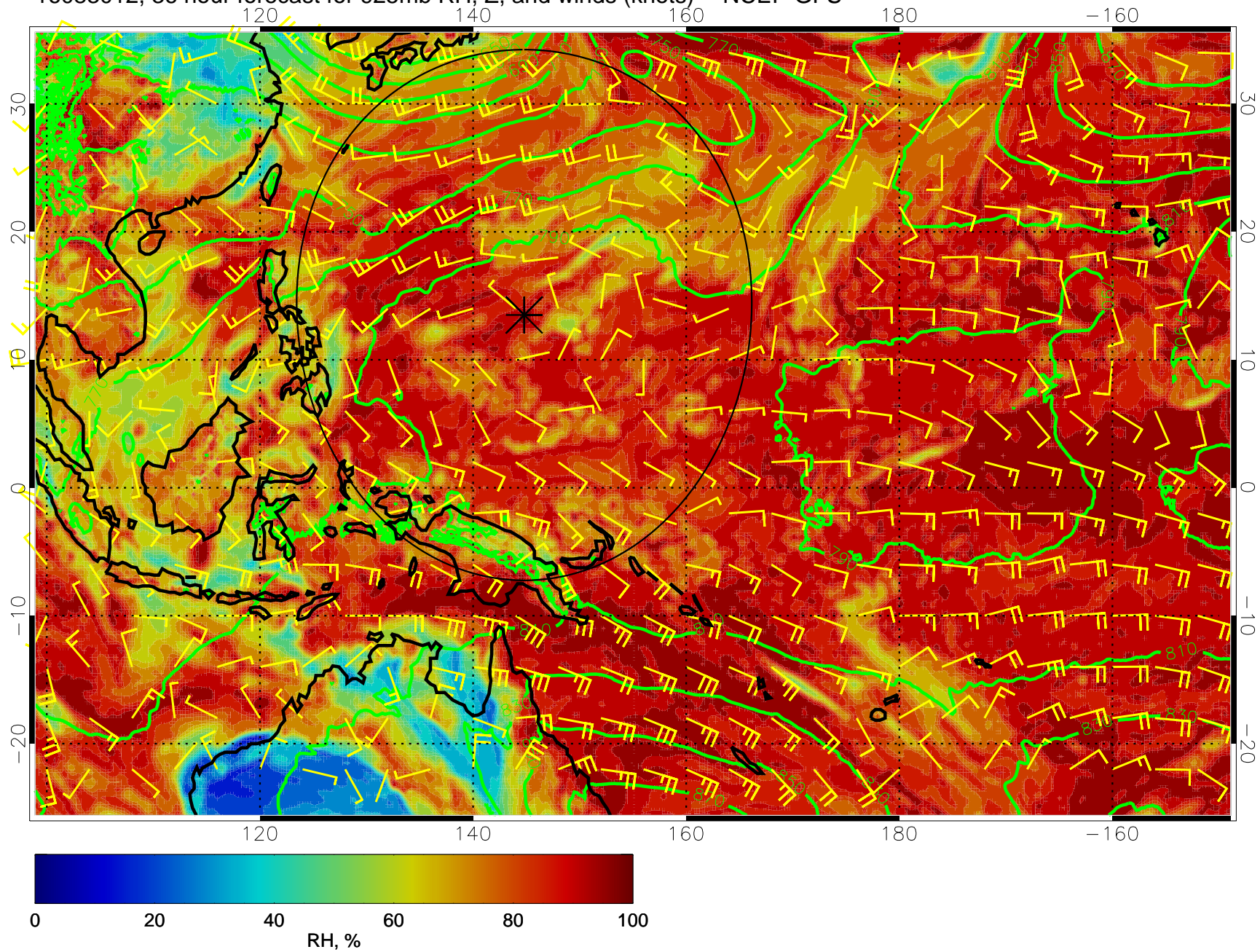
16083012, 36 hour forecast for 925mb RH, Z, and winds (knots) -- NCEP GFS
