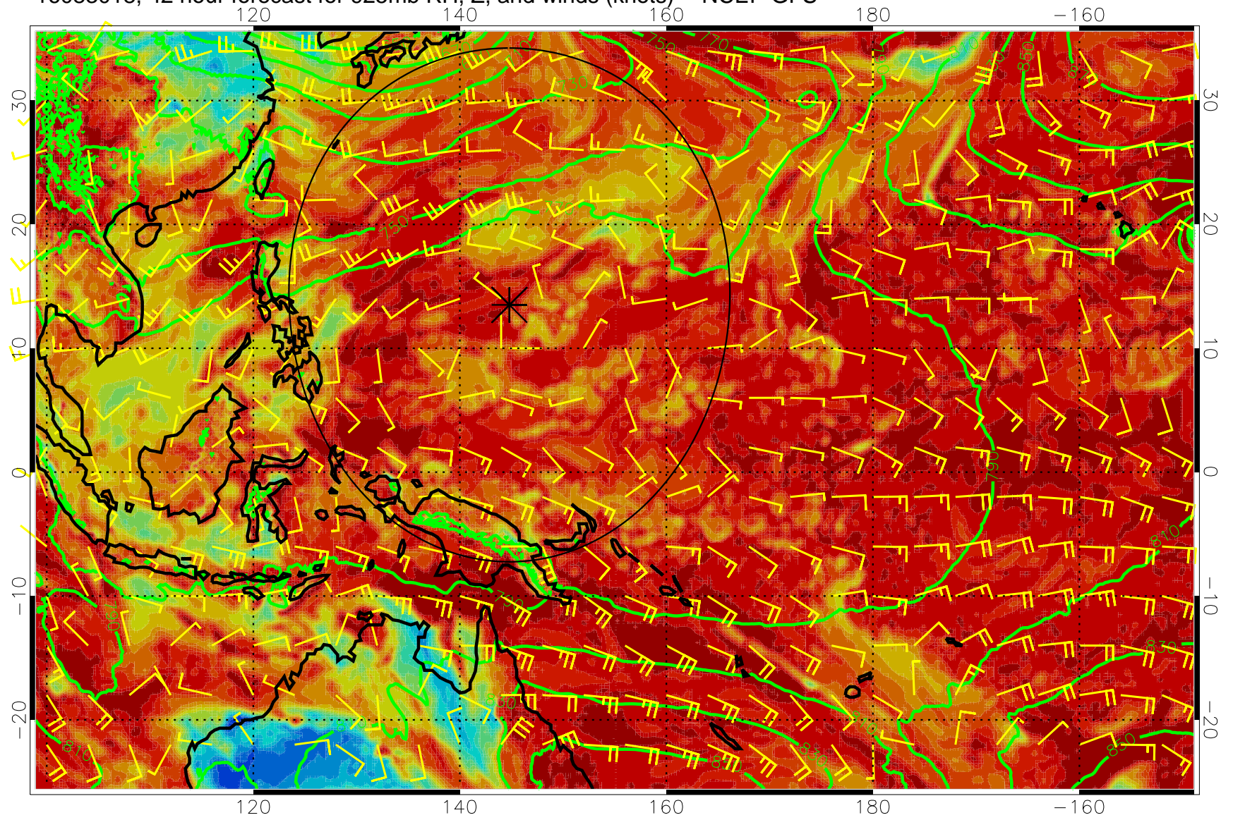
16083018, 42 hour forecast for 925mb RH, Z, and winds (knots) -- NCEP GFS
