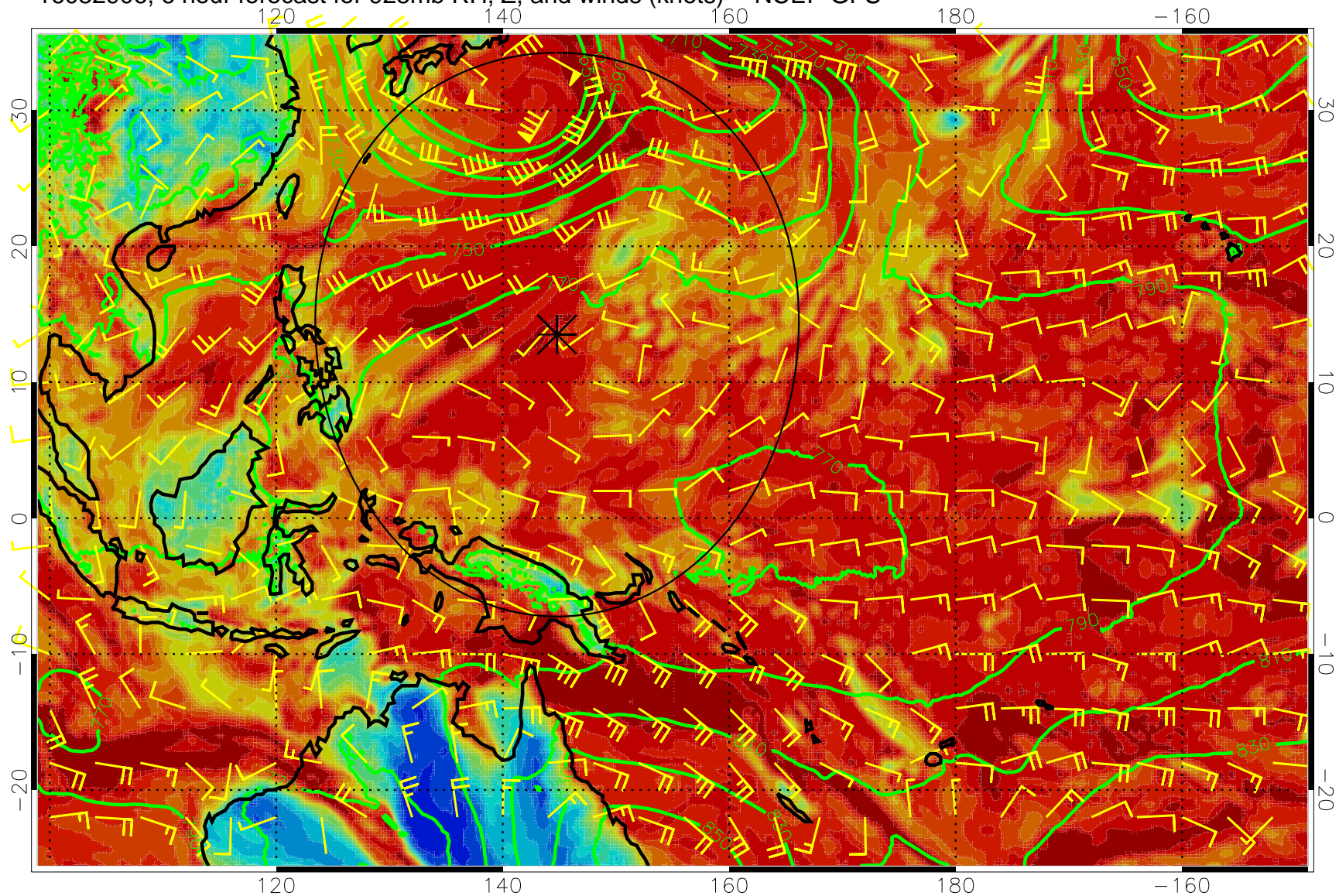
16082906, 6 hour forecast for 925mb RH, Z, and winds (knots) -- NCEP GFS
