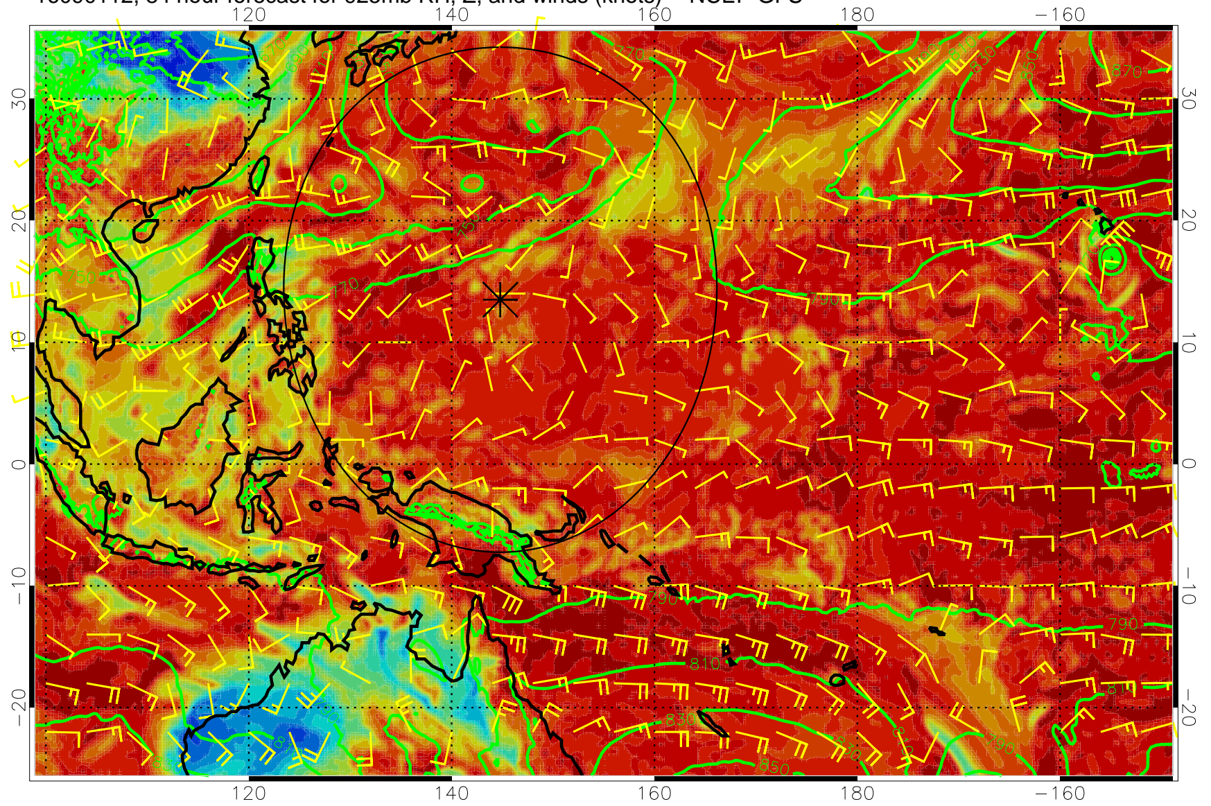
16090112, 84 hour forecast for 925mb RH, Z, and winds (knots) -- NCEP GFS
