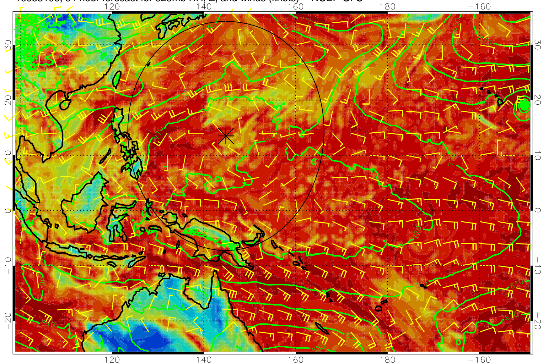
16083106, 54 hour forecast for 925mb RH, Z, and winds (knots) -- NCEP GFS
