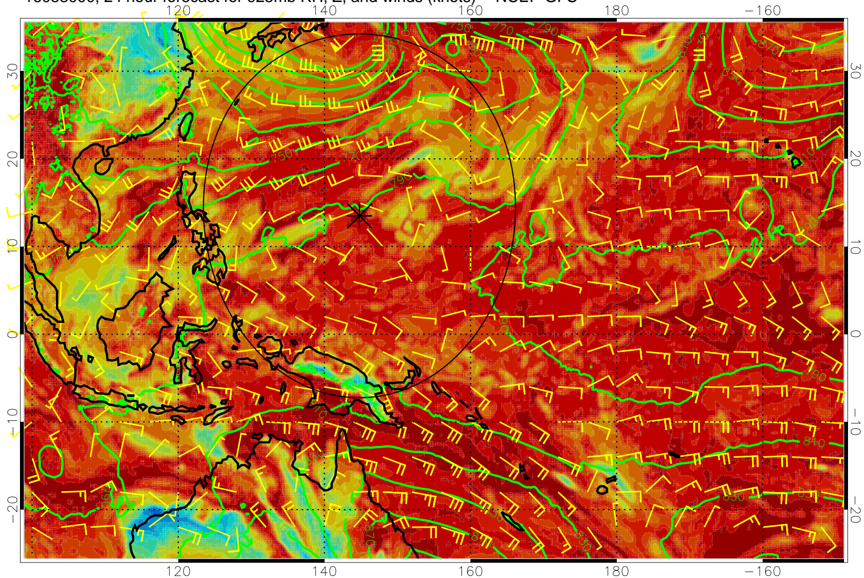
16083000, 24 hour forecast for 925mb RH, Z, and winds (knots) -- NCEP GFS
