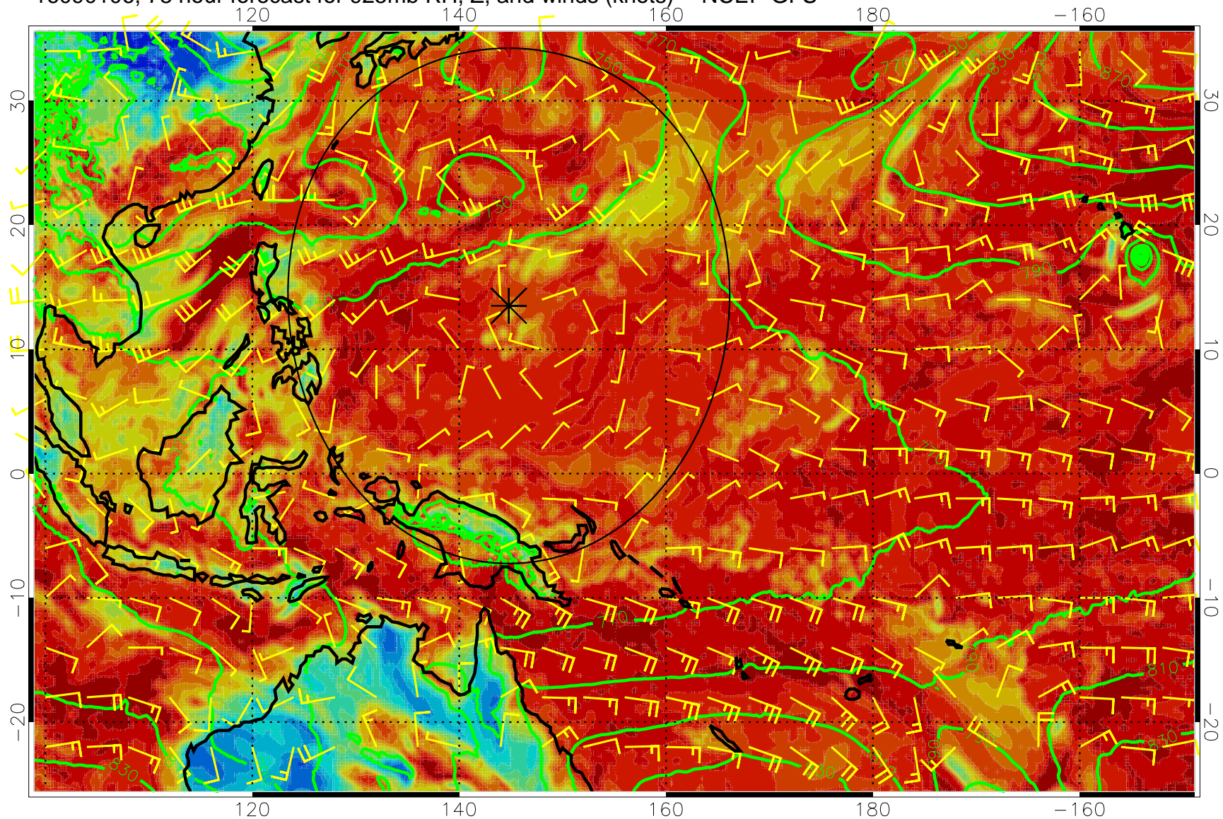
16090106, 78 hour forecast for 925mb RH, Z, and winds (knots) -- NCEP GFS
