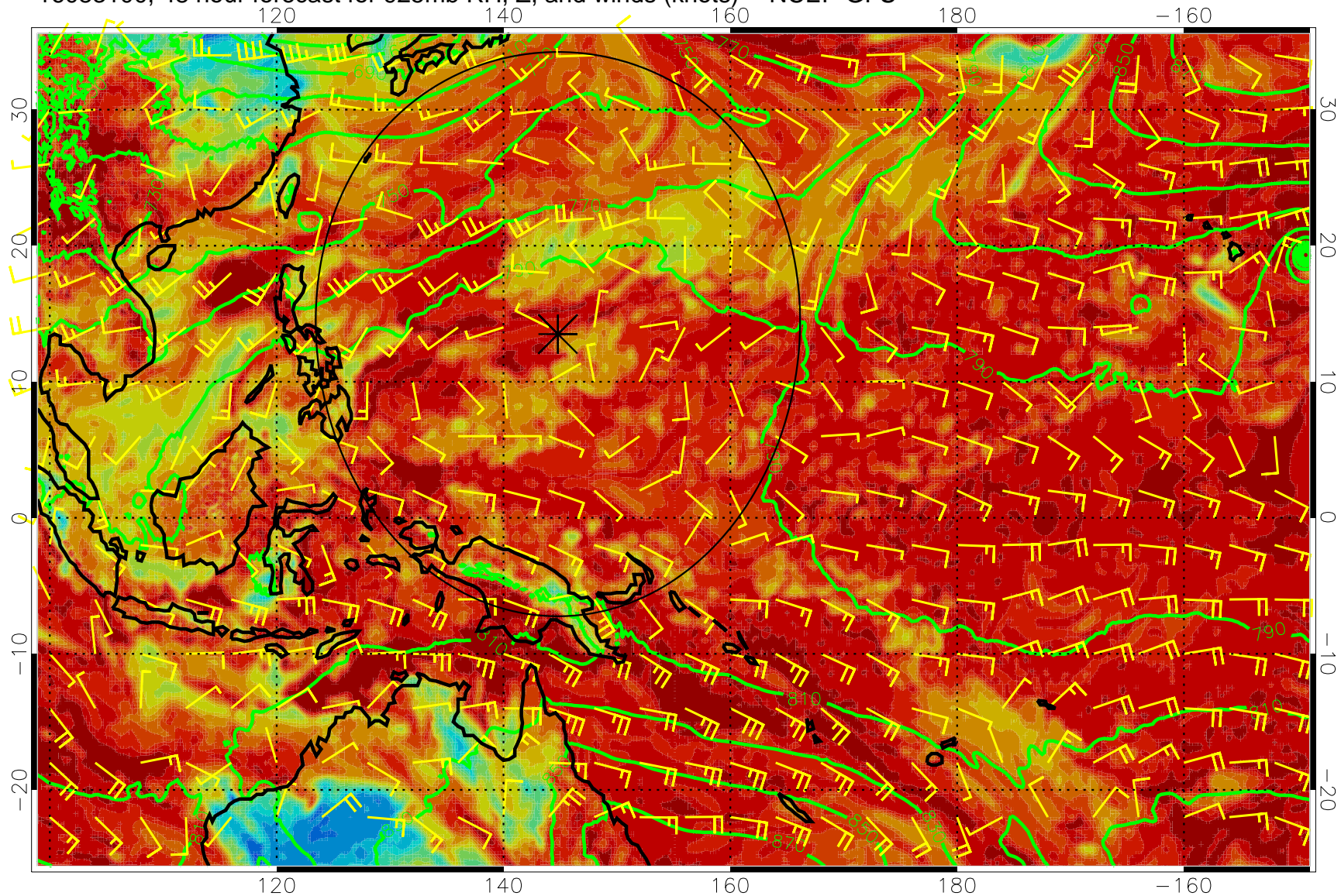
16083100, 48 hour forecast for 925mb RH, Z, and winds (knots) -- NCEP GFS
