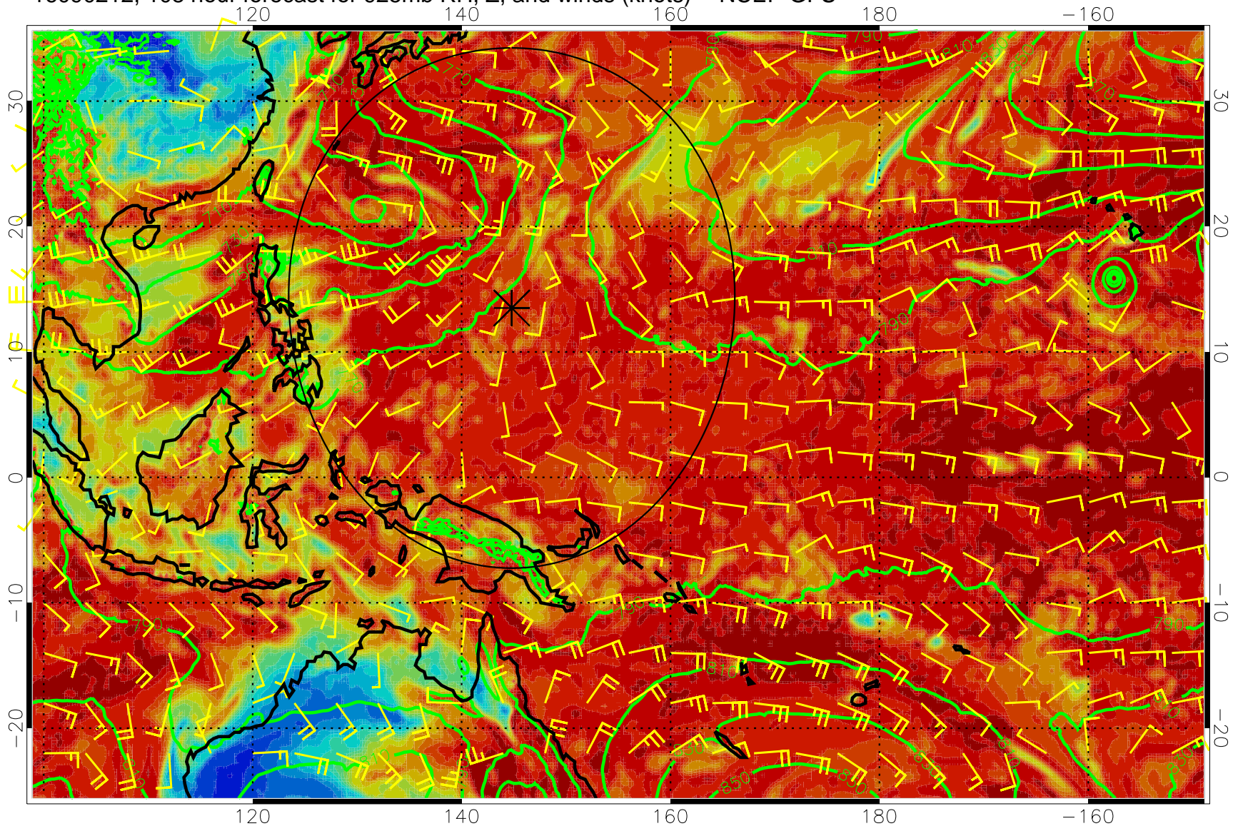
16090212, 108 hour forecast for 925mb RH, Z, and winds (knots) -- NCEP GFS
