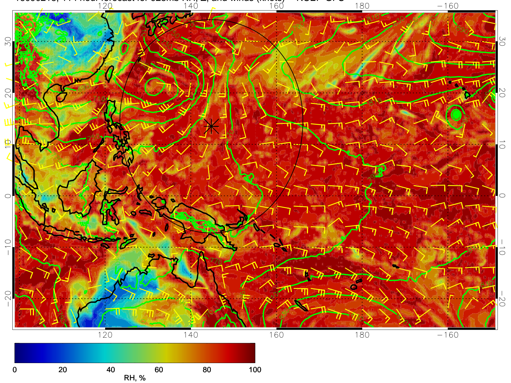
16090218, 114 hour forecast for 925mb RH, Z, and winds (knots) -- NCEP GFS
