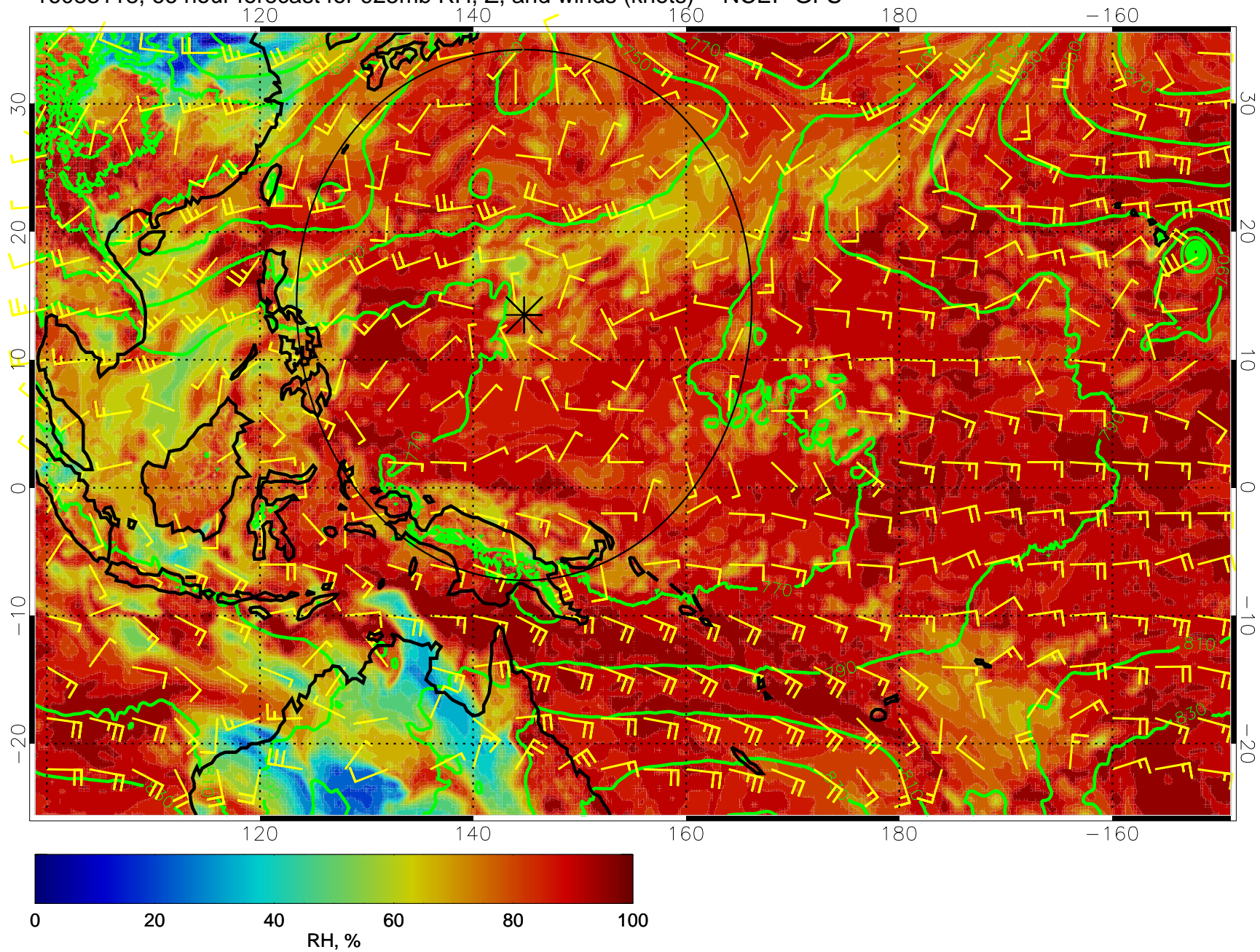
16083118, 66 hour forecast for 925mb RH, Z, and winds (knots) -- NCEP GFS
