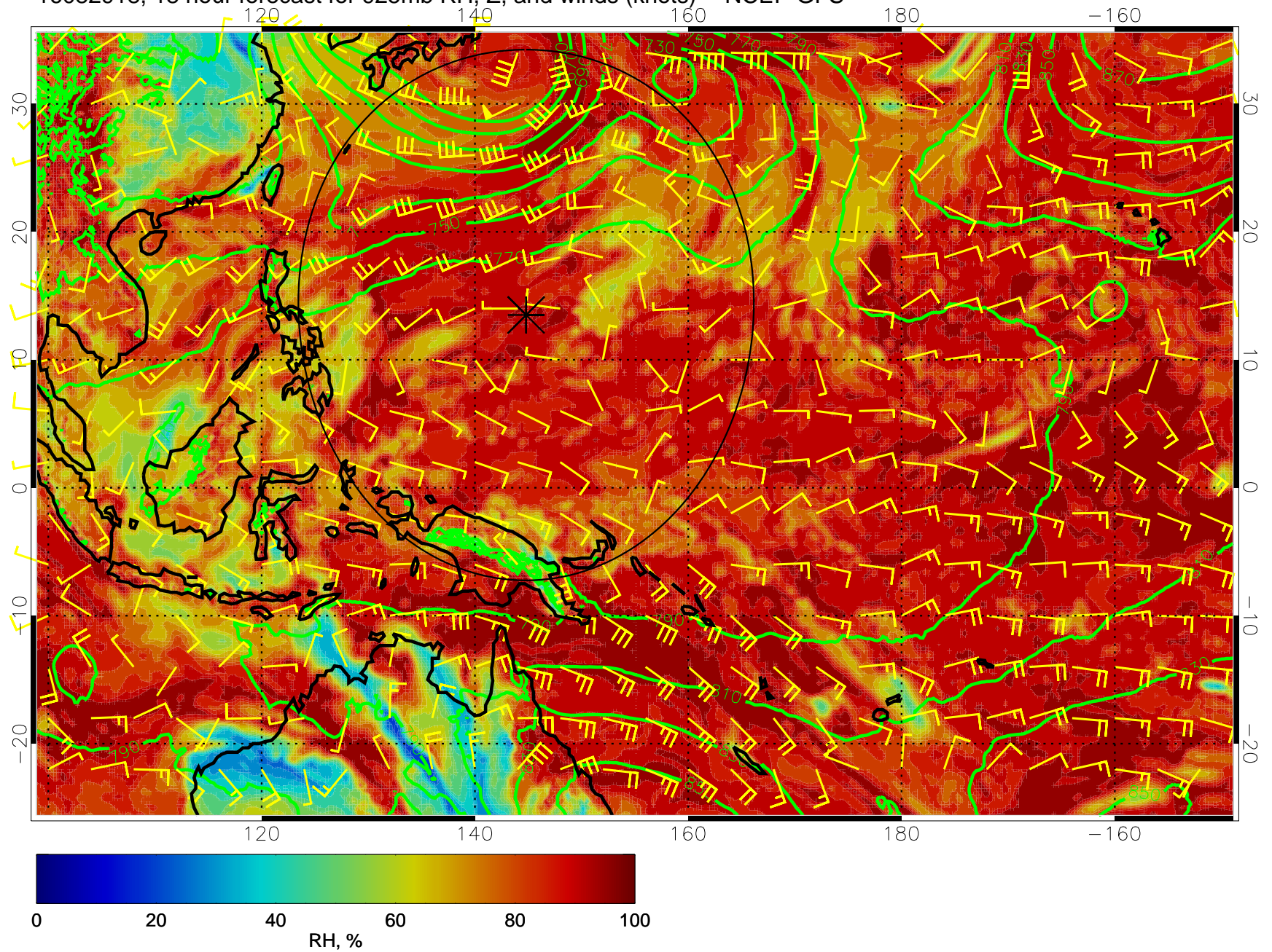
16082918, 18 hour forecast for 925mb RH, Z, and winds (knots) -- NCEP GFS
