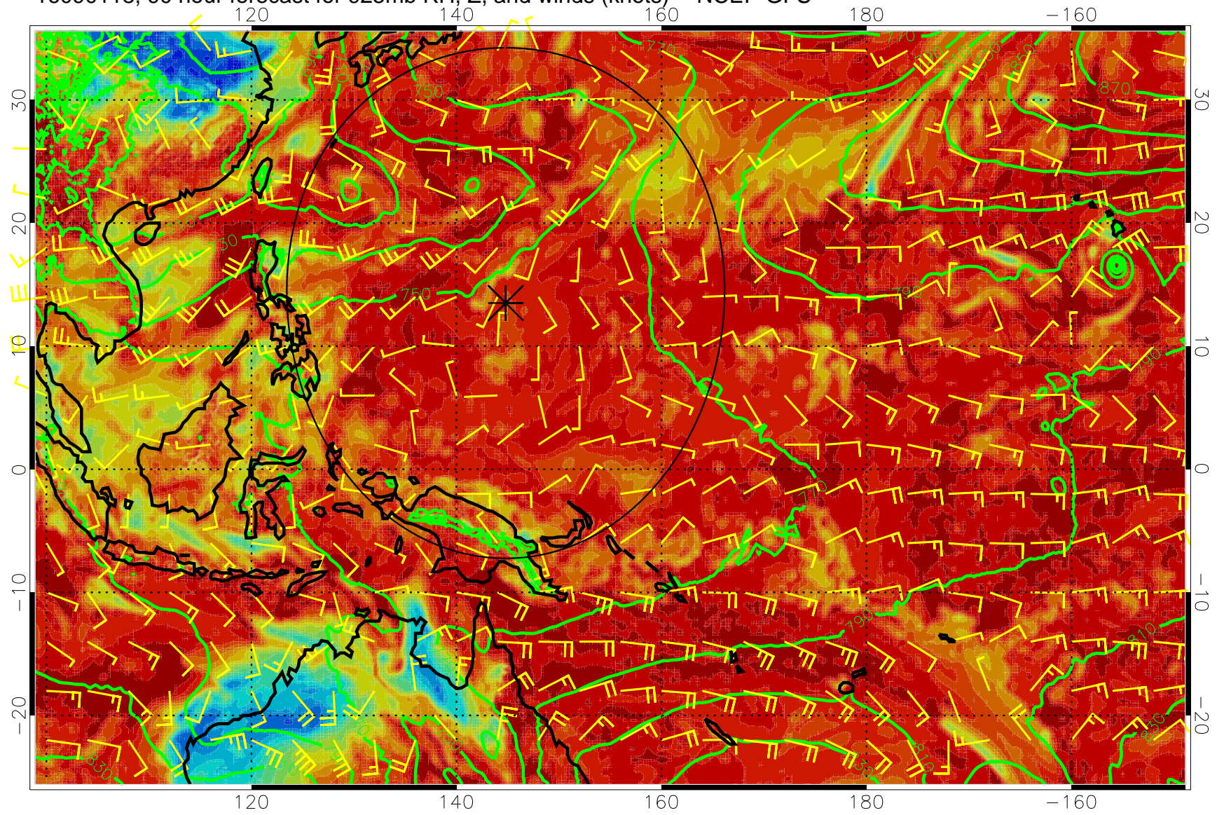
16090118, 90 hour forecast for 925mb RH, Z, and winds (knots) -- NCEP GFS
