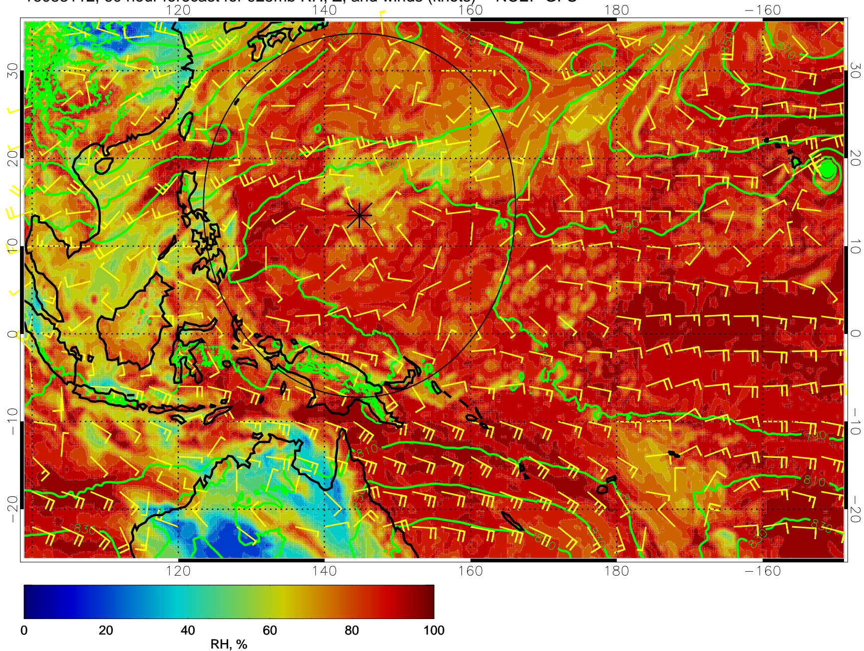
16083112, 60 hour forecast for 925mb RH, Z, and winds (knots) -- NCEP GFS
