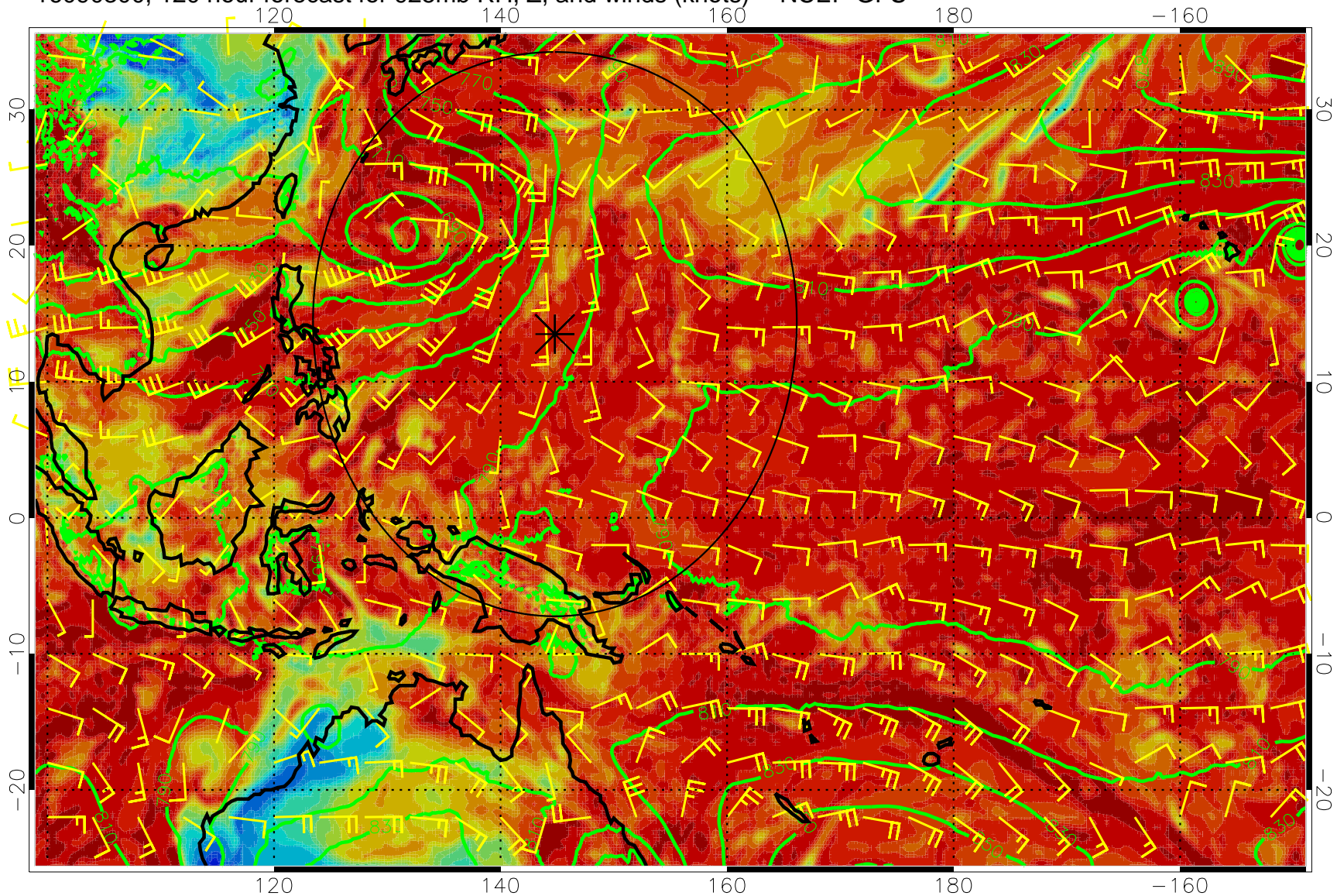
16090300, 120 hour forecast for 925mb RH, Z, and winds (knots) -- NCEP GFS
