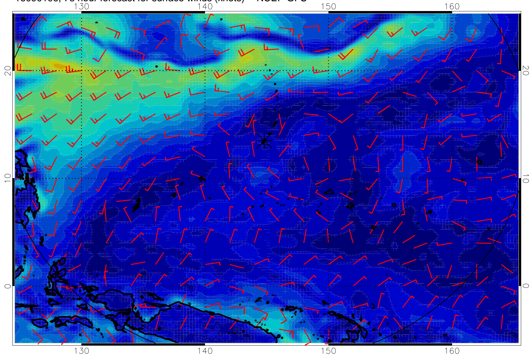
16090106, 78 hour forecast for surface winds (knots) -- NCEP GFS
