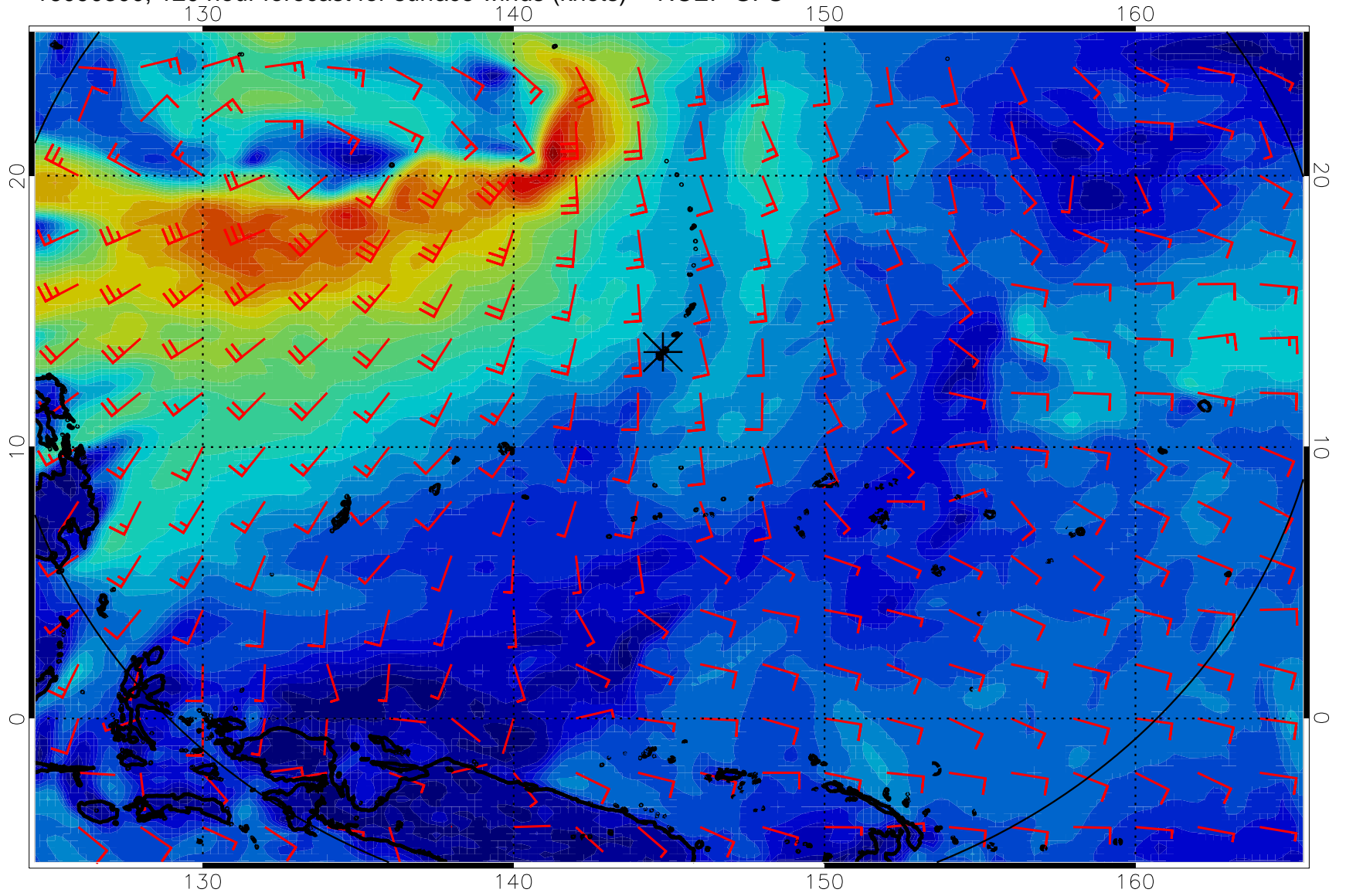
16090300, 120 hour forecast for surface winds (knots) -- NCEP GFS
