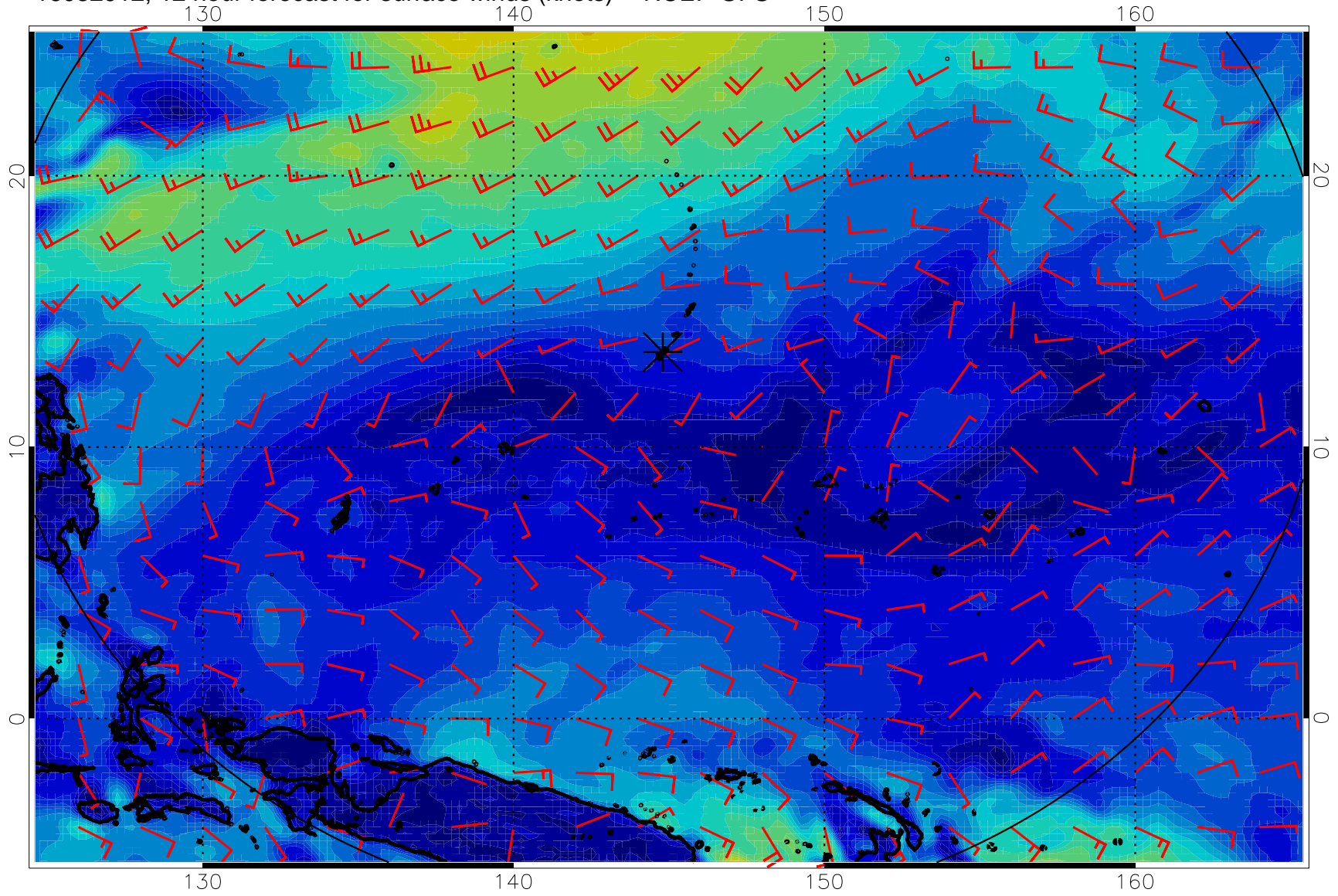
16082912, 12 hour forecast for surface winds (knots) -- NCEP GFS
