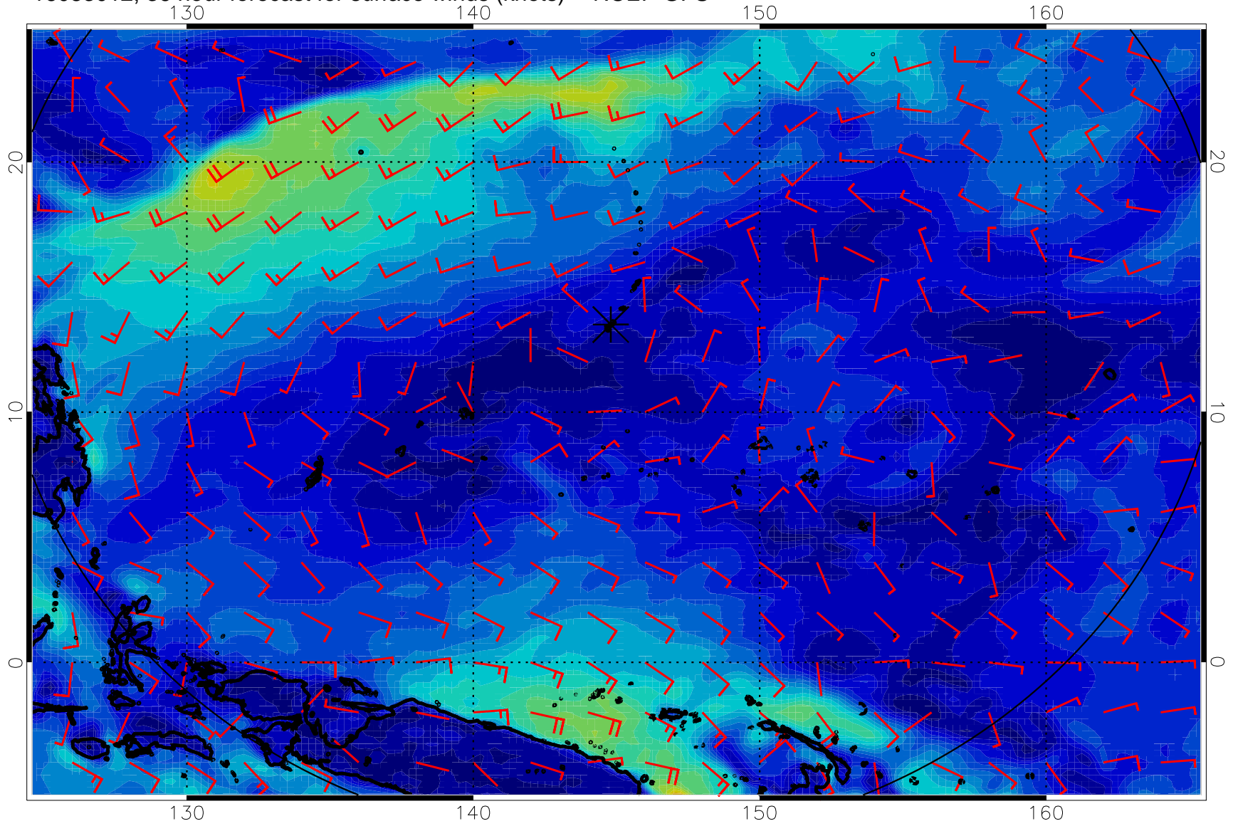
16083012, 36 hour forecast for surface winds (knots) -- NCEP GFS
