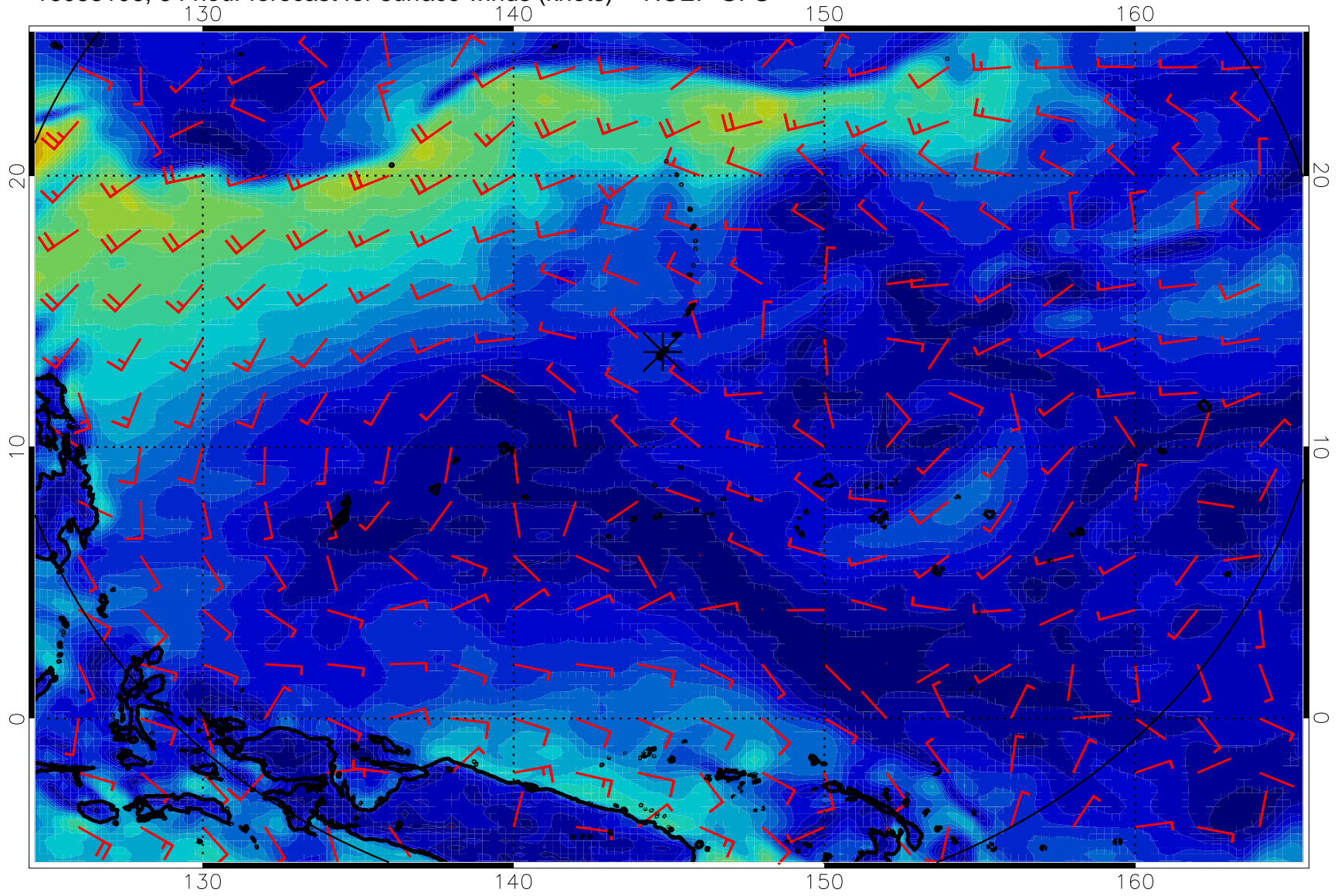
16083106, 54 hour forecast for surface winds (knots) -- NCEP GFS
