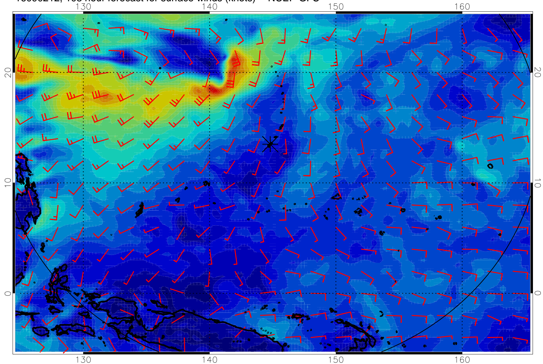
16090212, 108 hour forecast for surface winds (knots) -- NCEP GFS
