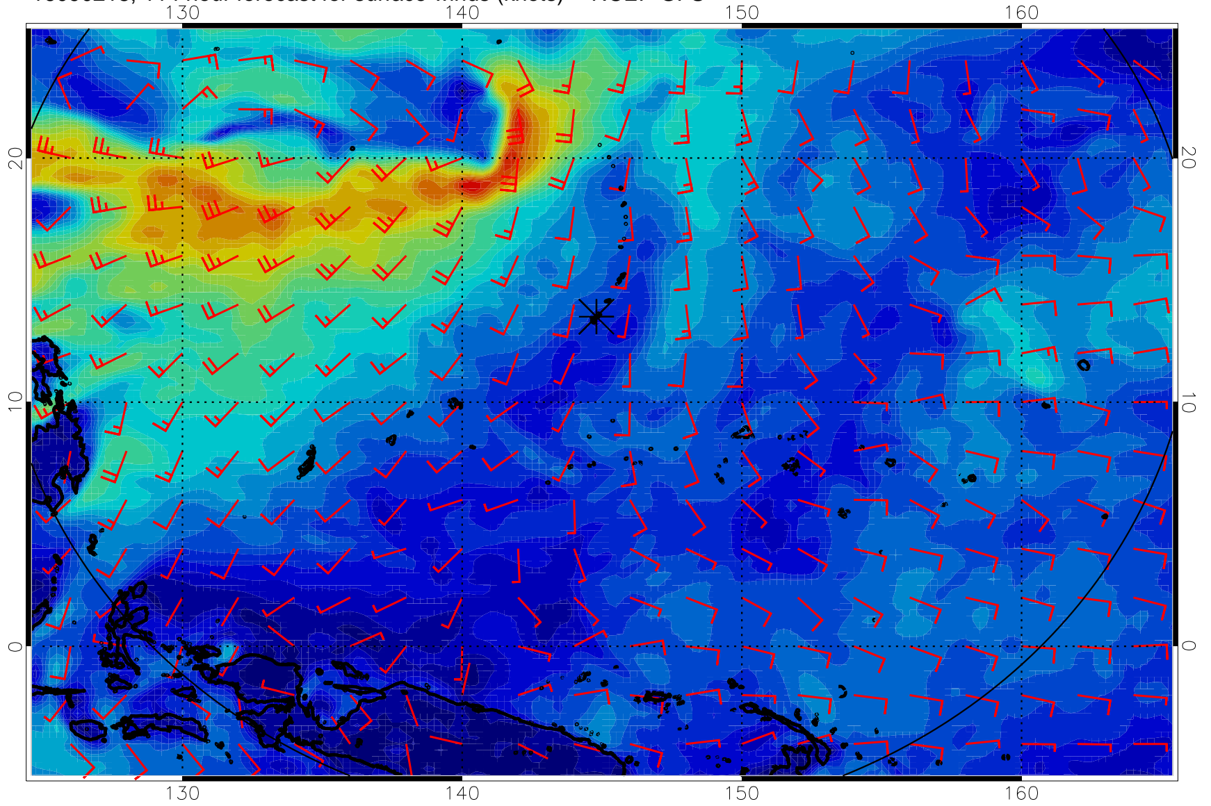
16090218, 114 hour forecast for surface winds (knots) -- NCEP GFS
