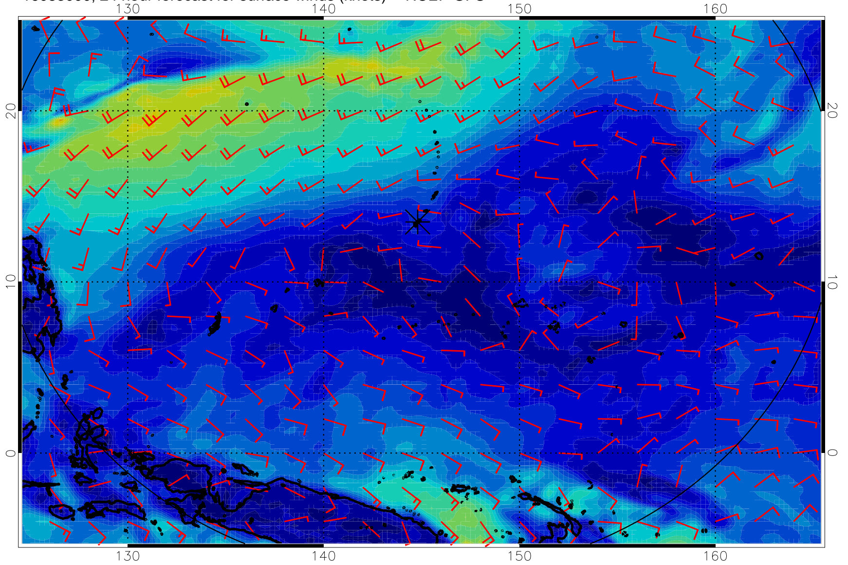
16083000, 24 hour forecast for surface winds (knots) -- NCEP GFS
