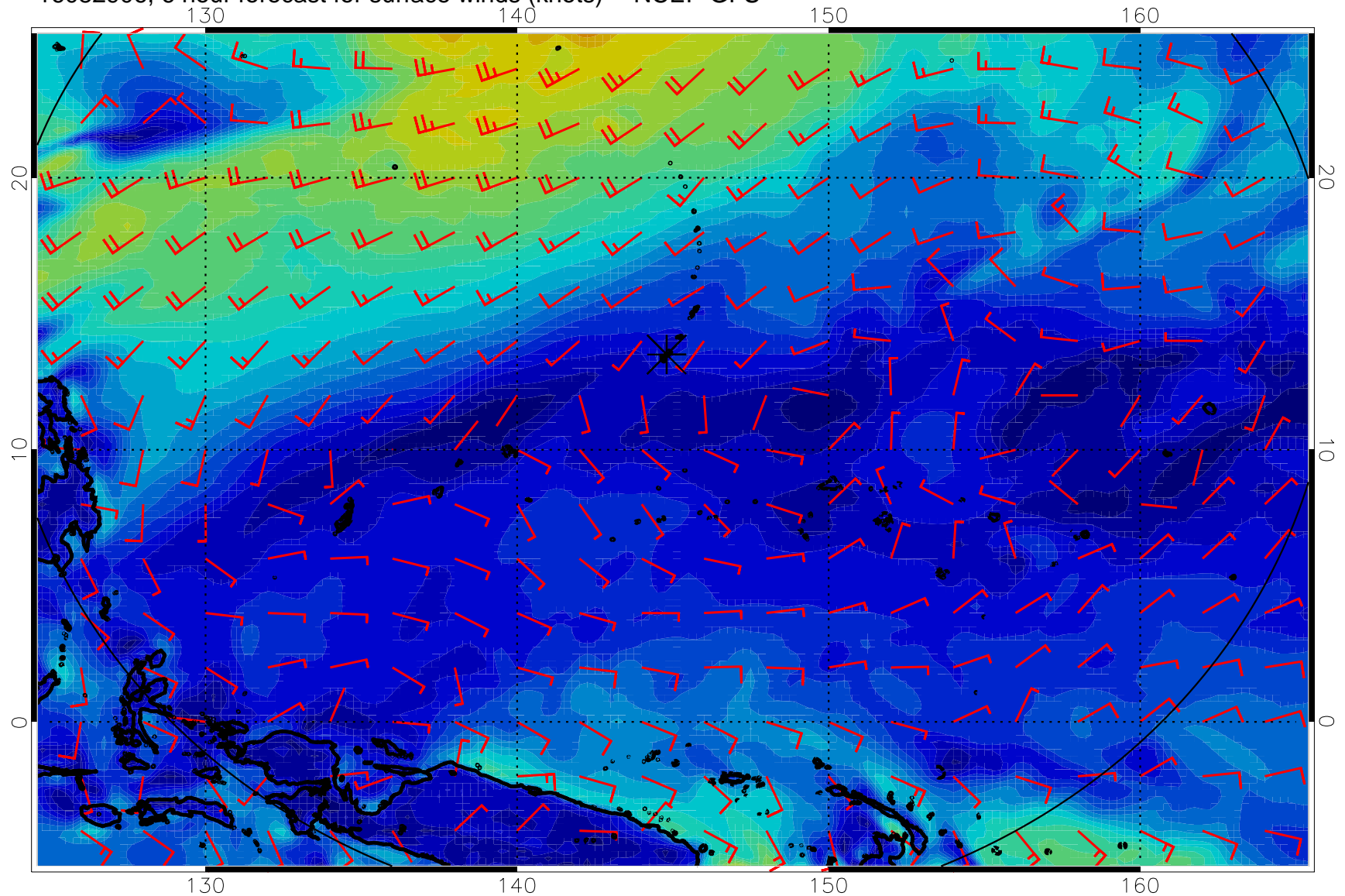
16082906, 6 hour forecast for surface winds (knots) -- NCEP GFS
