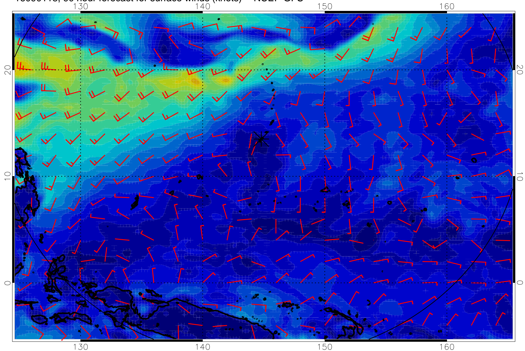
16090118, 90 hour forecast for surface winds (knots) -- NCEP GFS
