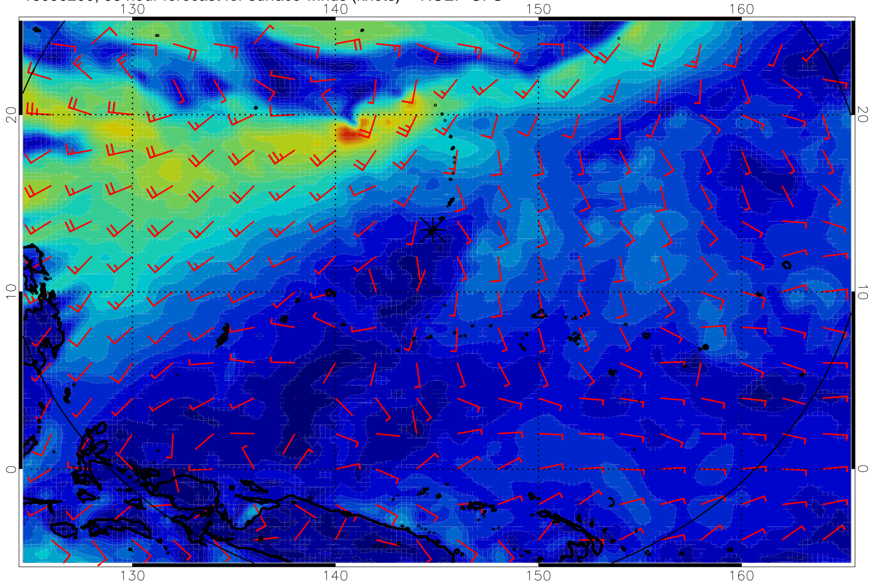
16090200, 96 hour forecast for surface winds (knots) -- NCEP GFS
