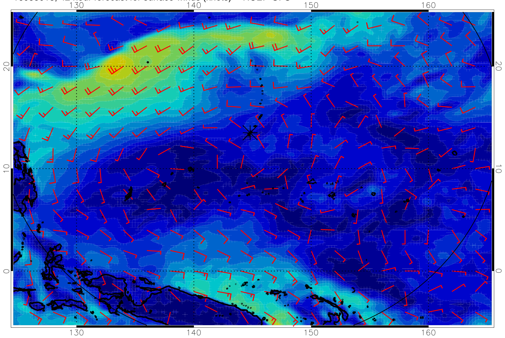
16083018, 42 hour forecast for surface winds (knots) -- NCEP GFS
