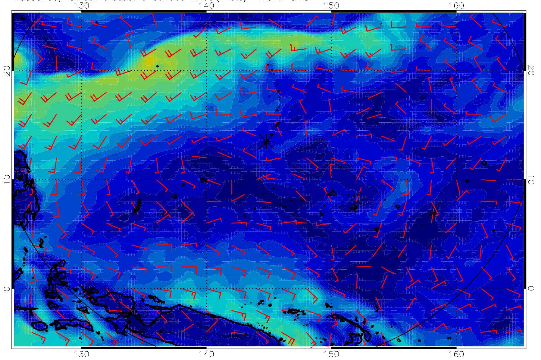
16083100, 48 hour forecast for surface winds (knots) -- NCEP GFS
