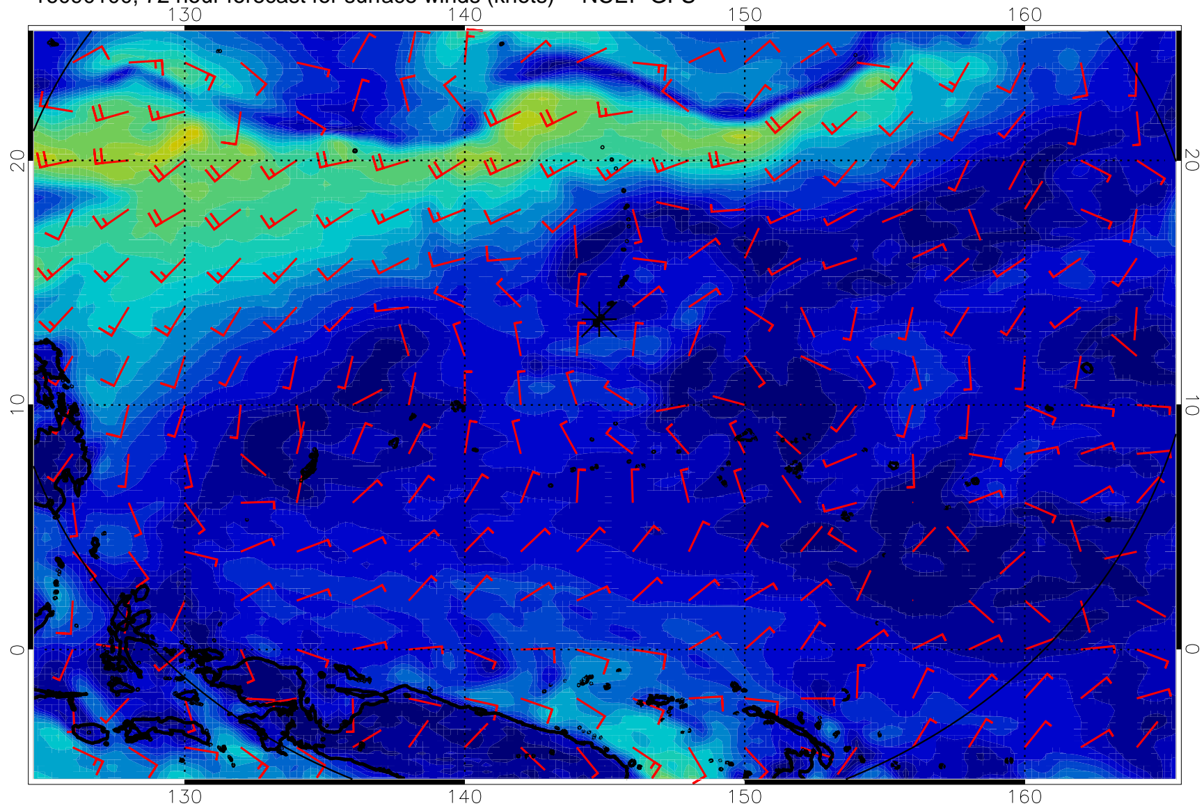
16090100, 72 hour forecast for surface winds (knots) -- NCEP GFS
