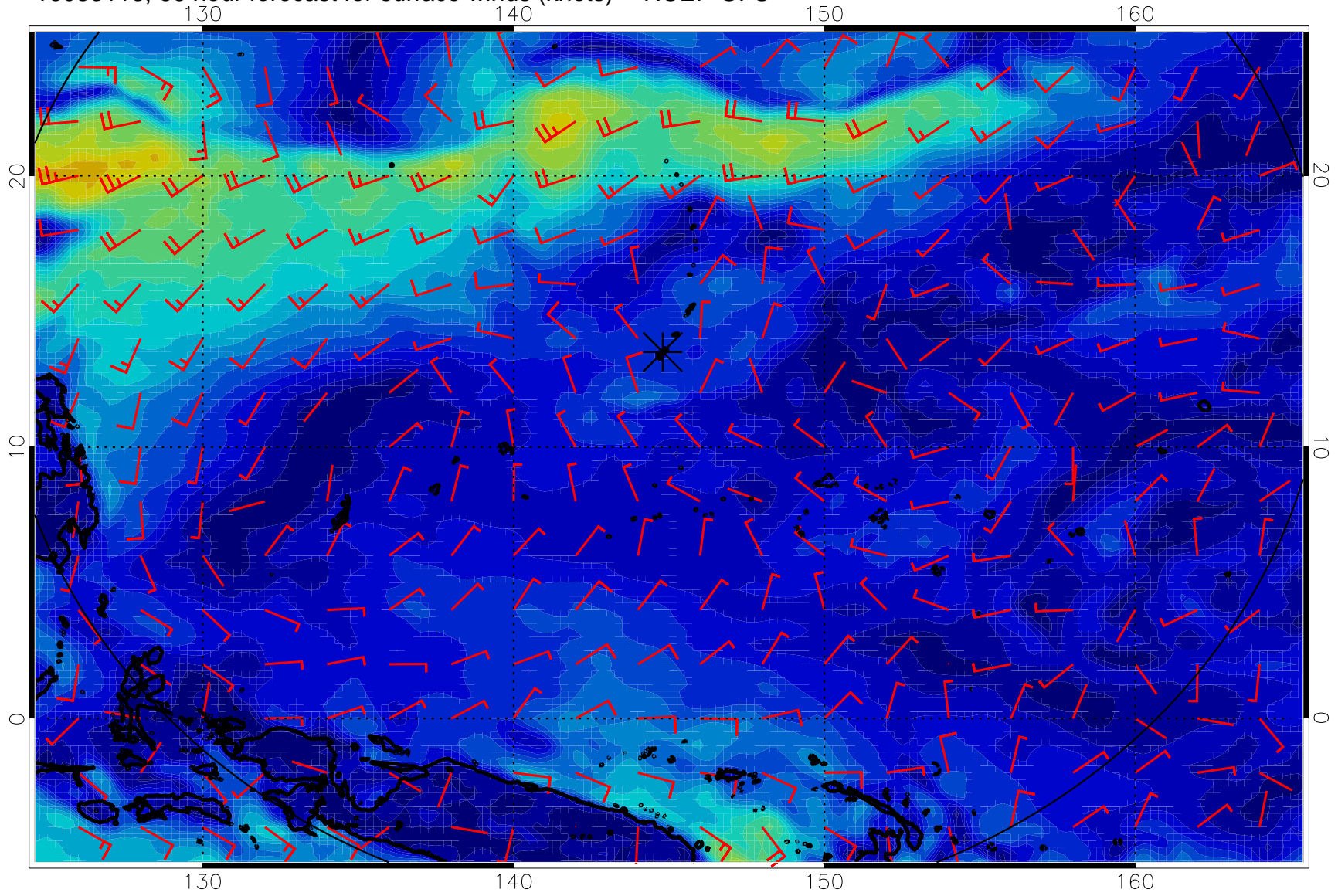
16083118, 66 hour forecast for surface winds (knots) -- NCEP GFS
