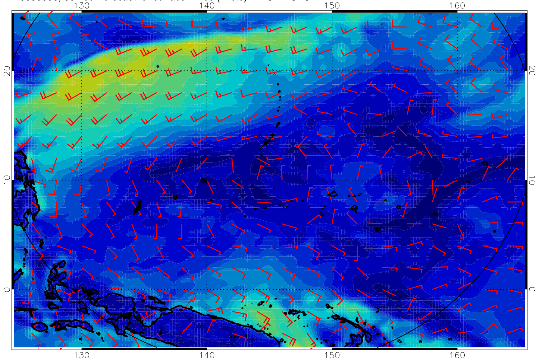
16083006, 30 hour forecast for surface winds (knots) -- NCEP GFS
