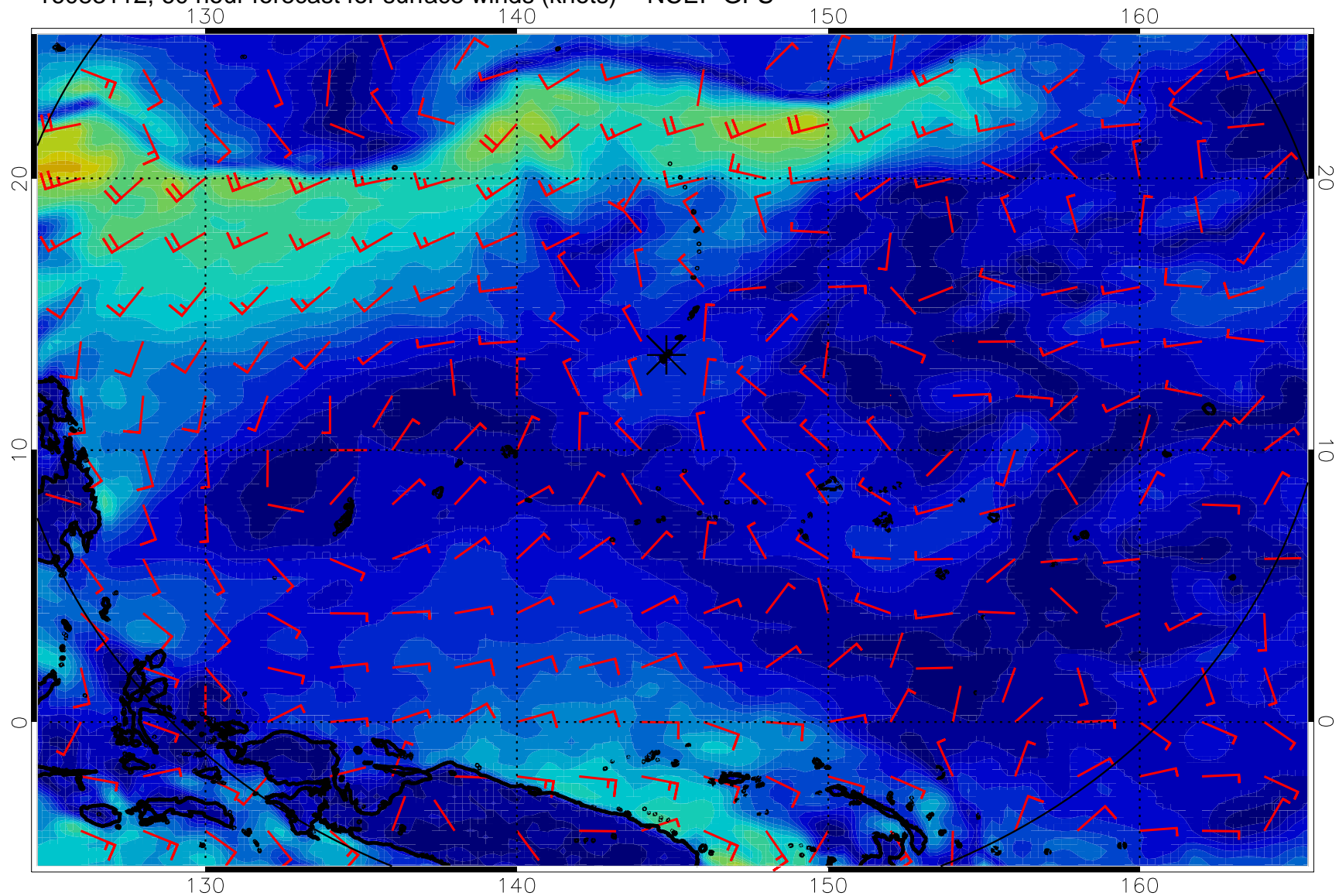
16083112, 60 hour forecast for surface winds (knots) -- NCEP GFS
