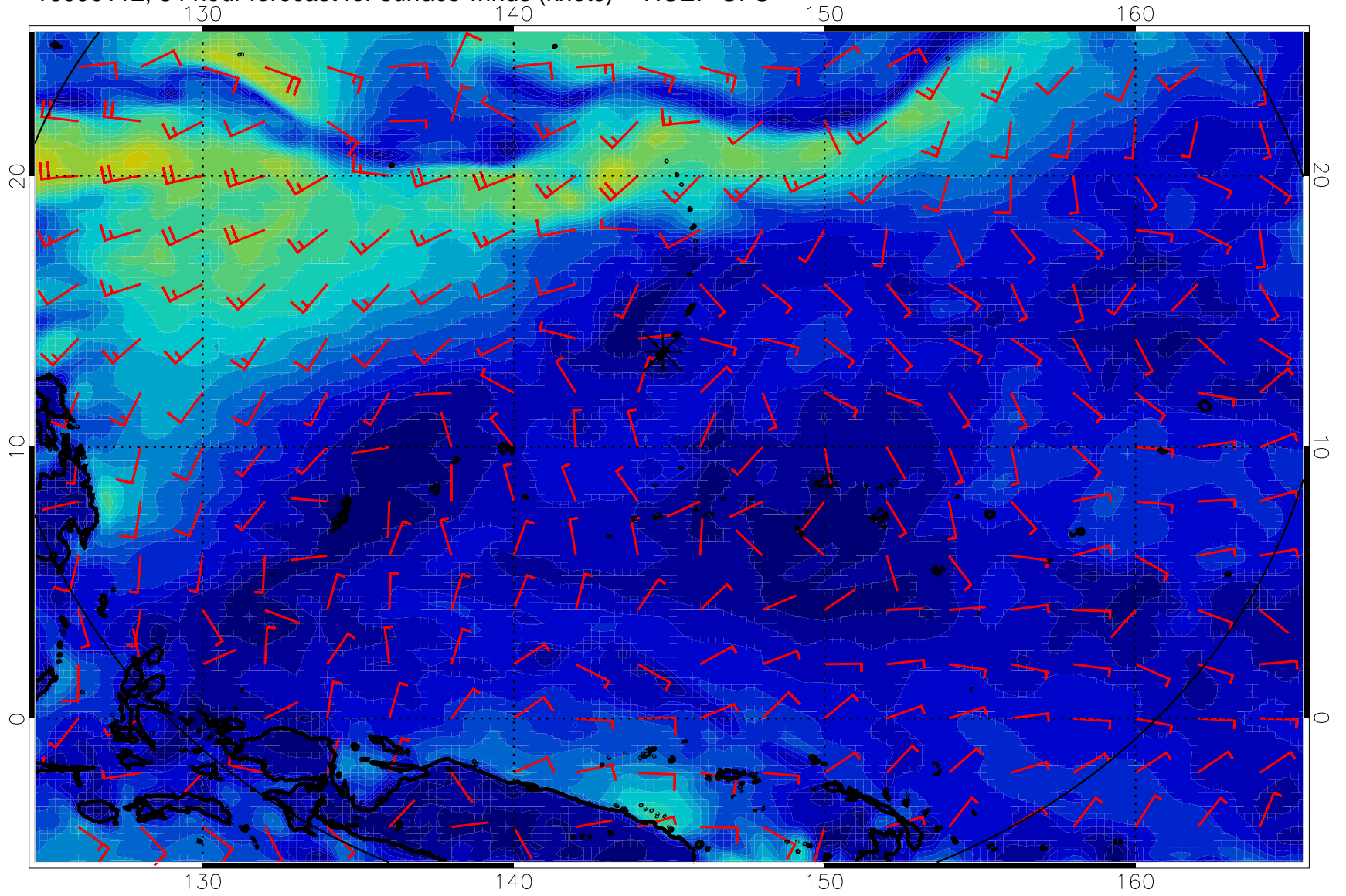
16090112, 84 hour forecast for surface winds (knots) -- NCEP GFS
