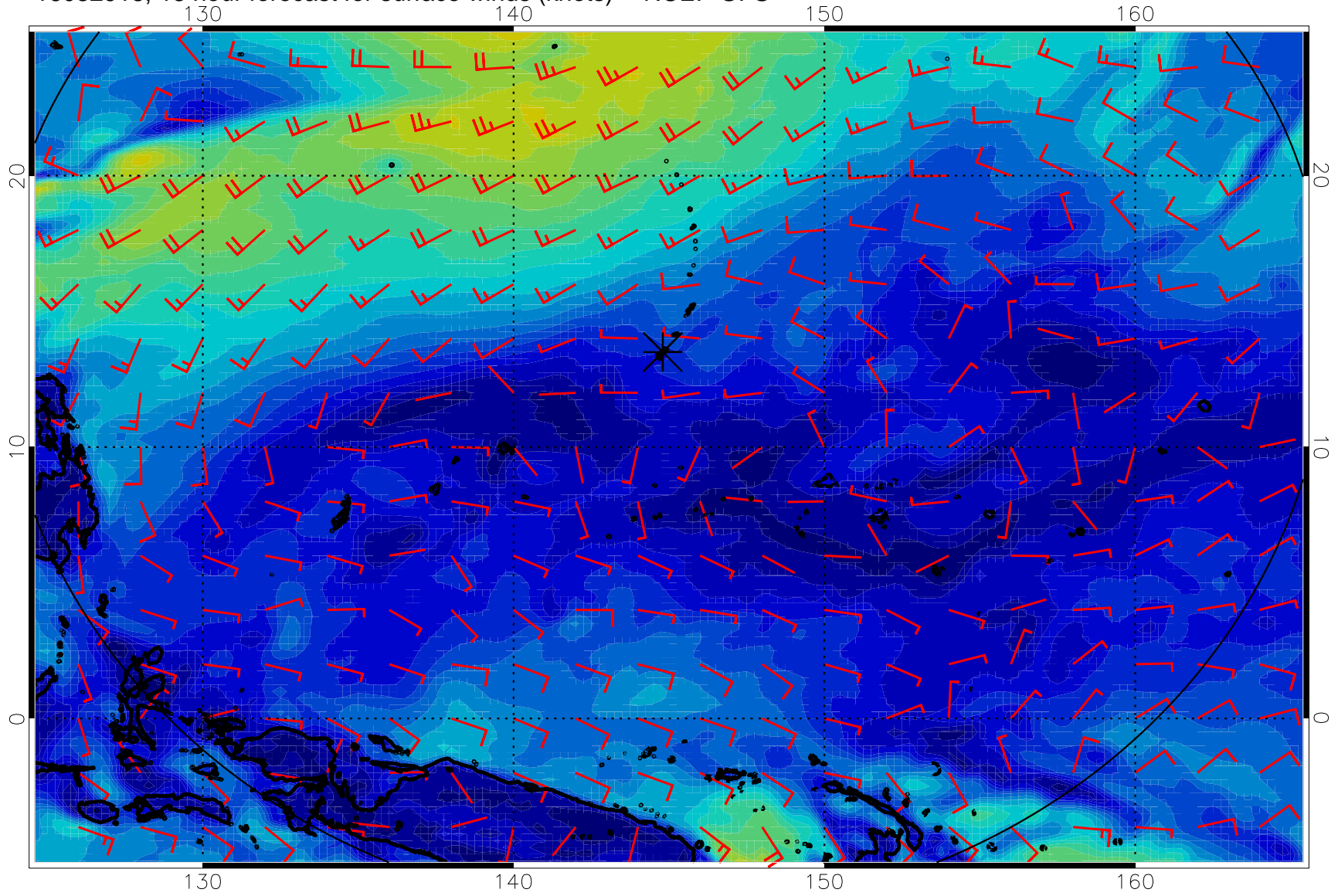
16082918, 18 hour forecast for surface winds (knots) -- NCEP GFS
