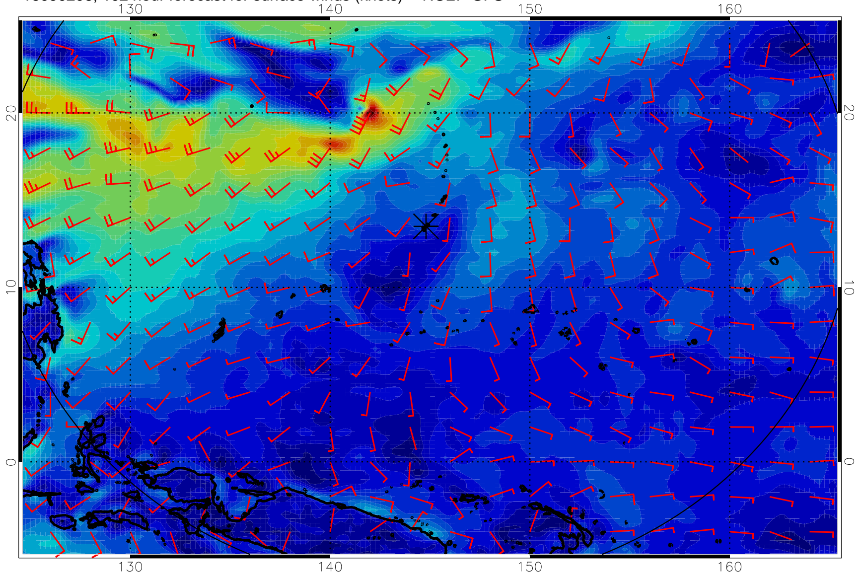
16090206, 102 hour forecast for surface winds (knots) -- NCEP GFS
