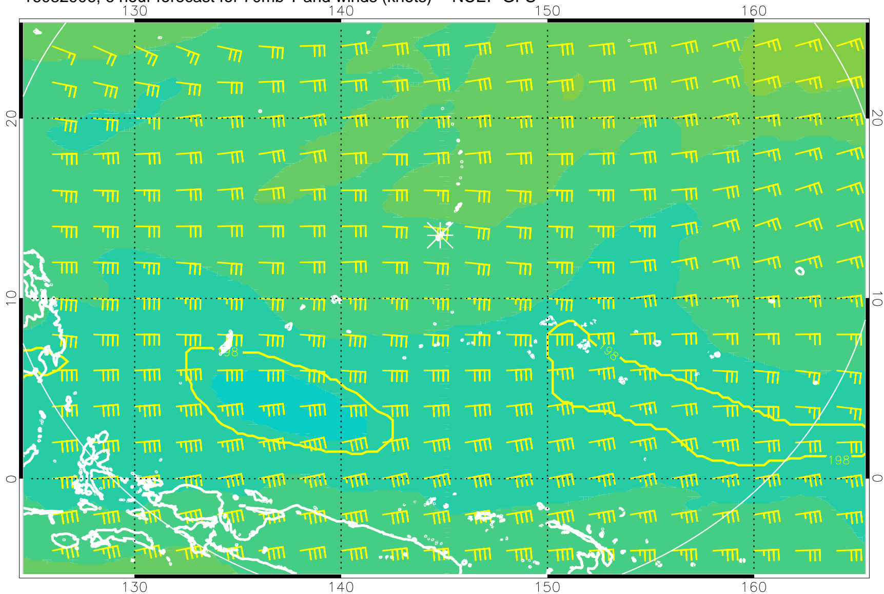
16082906, 6 hour forecast for 70mb T and winds (knots) -- NCEP GFS
