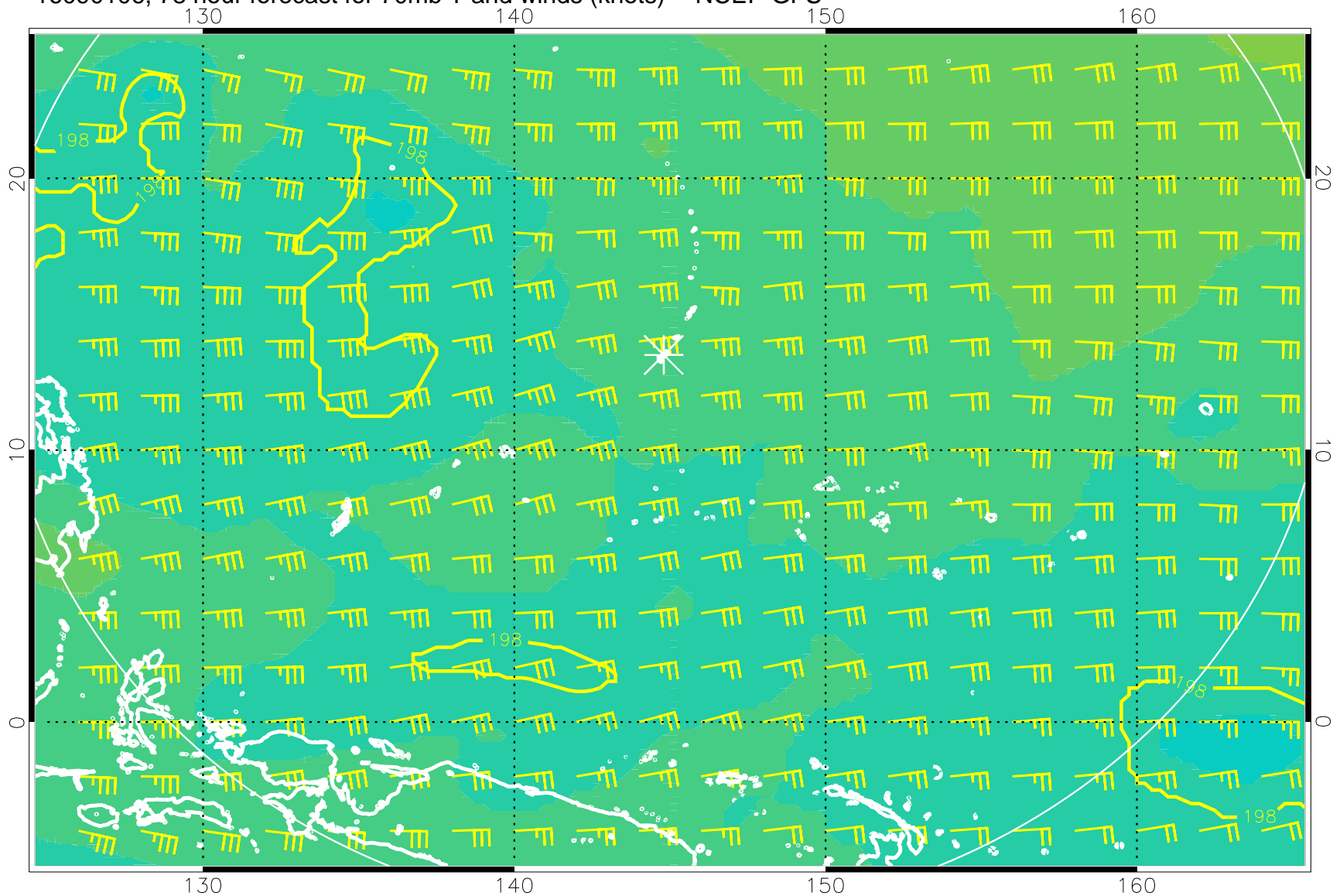
16090106, 78 hour forecast for 70mb T and winds (knots) -- NCEP GFS
