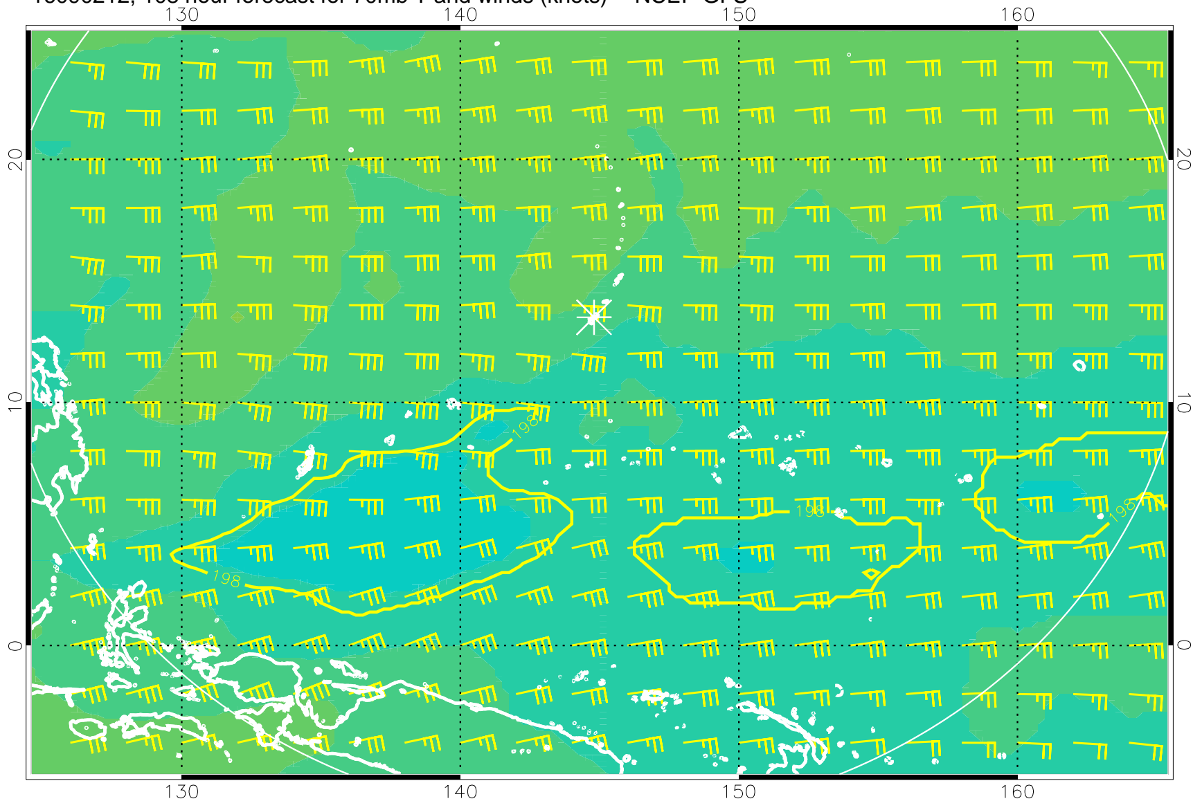
16090212, 108 hour forecast for 70mb T and winds (knots) -- NCEP GFS
