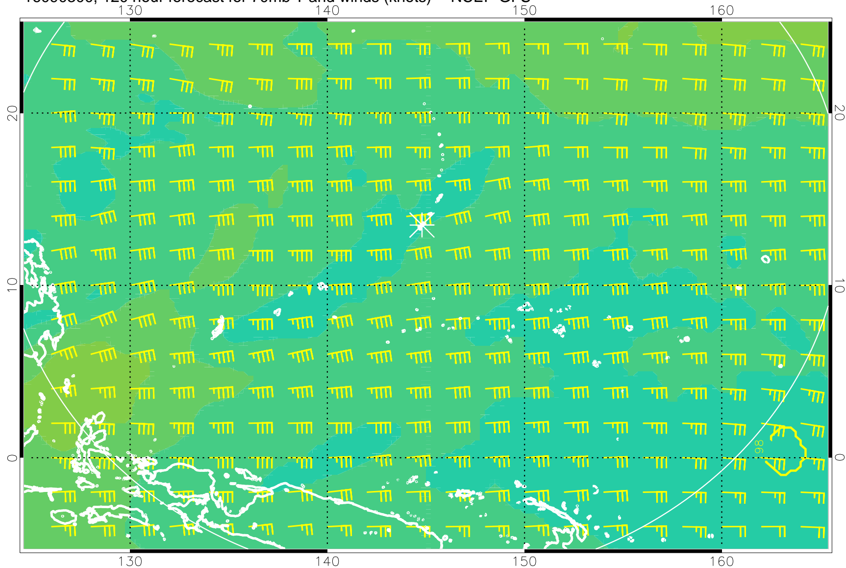
16090300, 120 hour forecast for 70mb T and winds (knots) -- NCEP GFS
