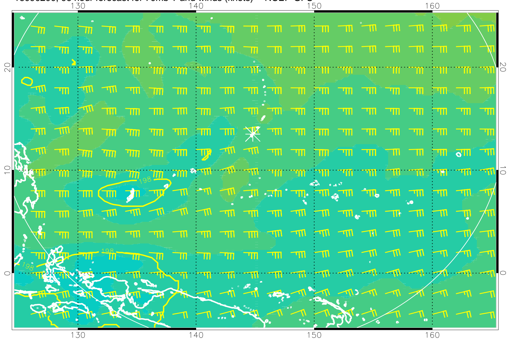
16090200, 96 hour forecast for 70mb T and winds (knots) -- NCEP GFS
