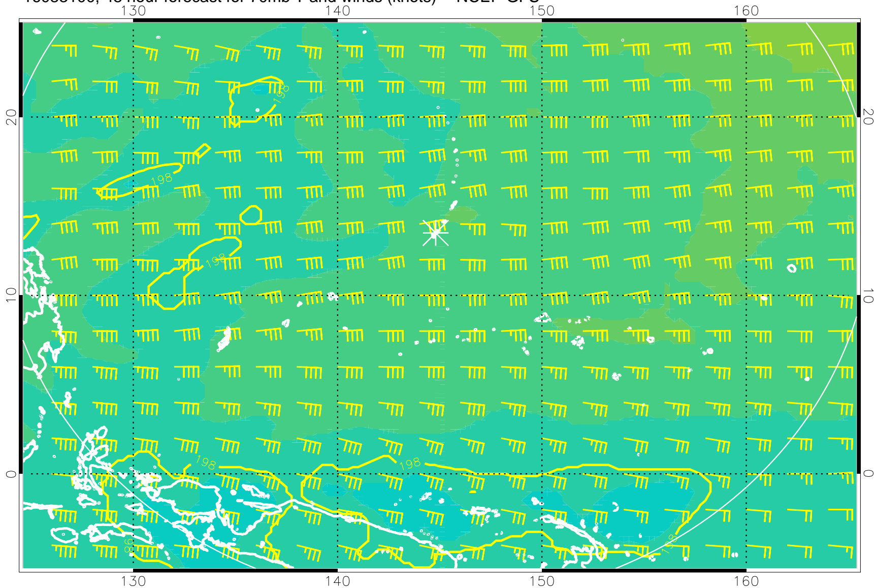
16083100, 48 hour forecast for 70mb T and winds (knots) -- NCEP GFS
