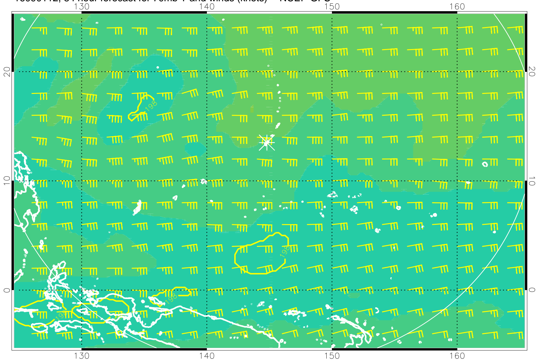
16090112, 84 hour forecast for 70mb T and winds (knots) -- NCEP GFS
