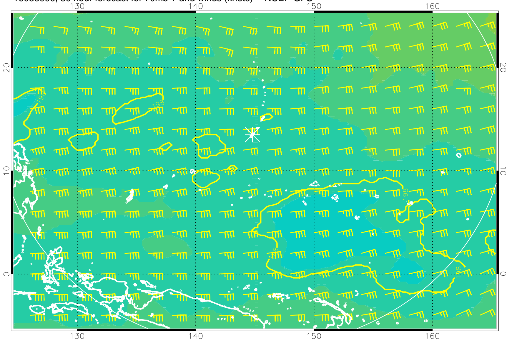
16083006, 30 hour forecast for 70mb T and winds (knots) -- NCEP GFS
