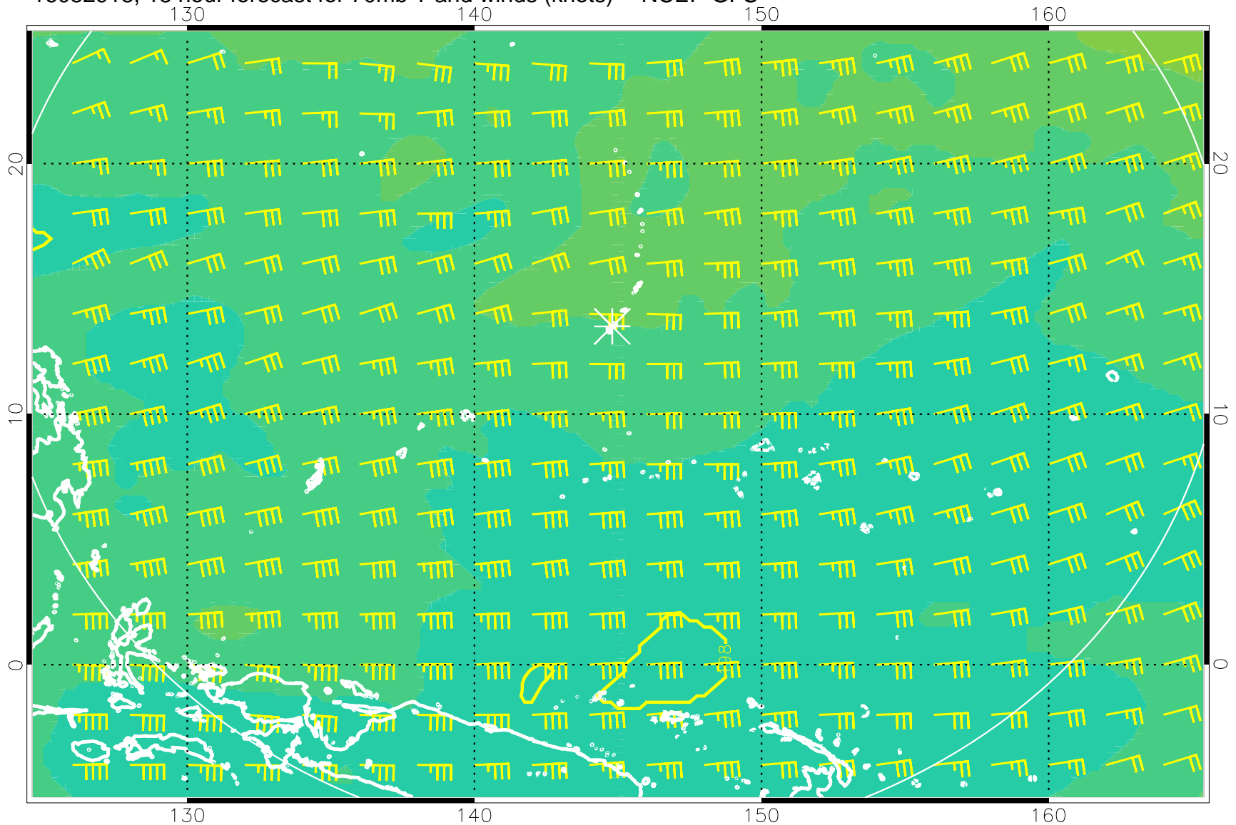
16082918, 18 hour forecast for 70mb T and winds (knots) -- NCEP GFS
