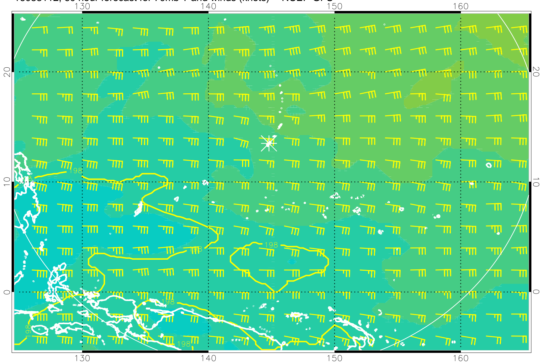
16083112, 60 hour forecast for 70mb T and winds (knots) -- NCEP GFS
