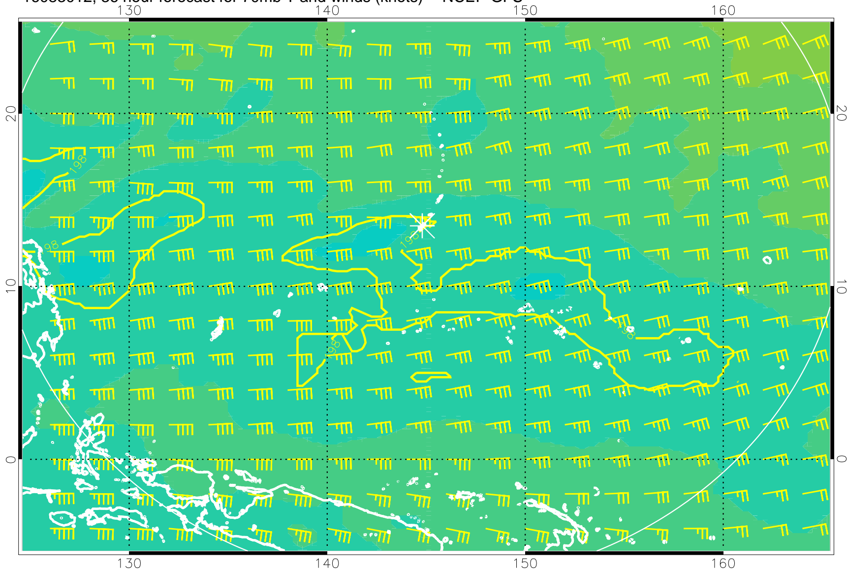
16083012, 36 hour forecast for 70mb T and winds (knots) -- NCEP GFS
