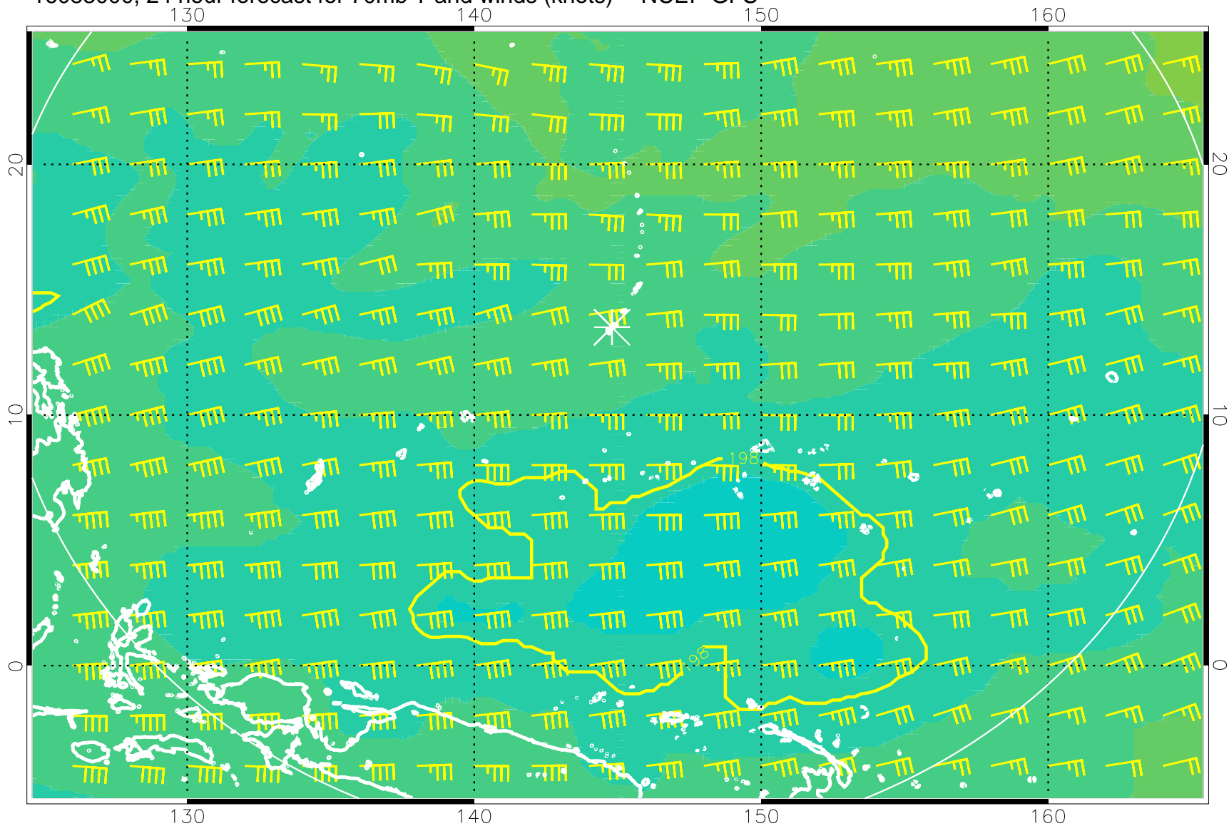
16083000, 24 hour forecast for 70mb T and winds (knots) -- NCEP GFS
