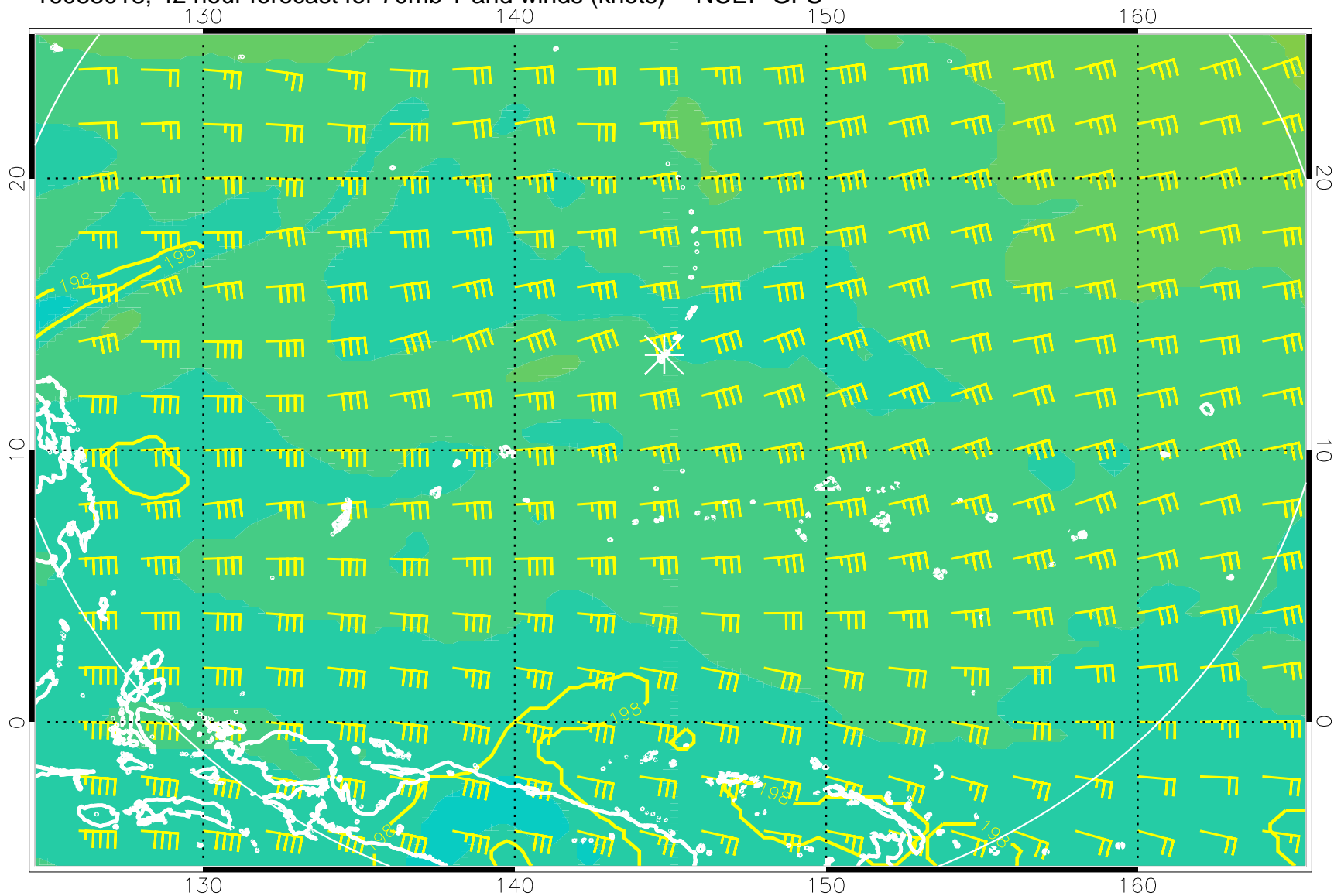
16083018, 42 hour forecast for 70mb T and winds (knots) -- NCEP GFS
