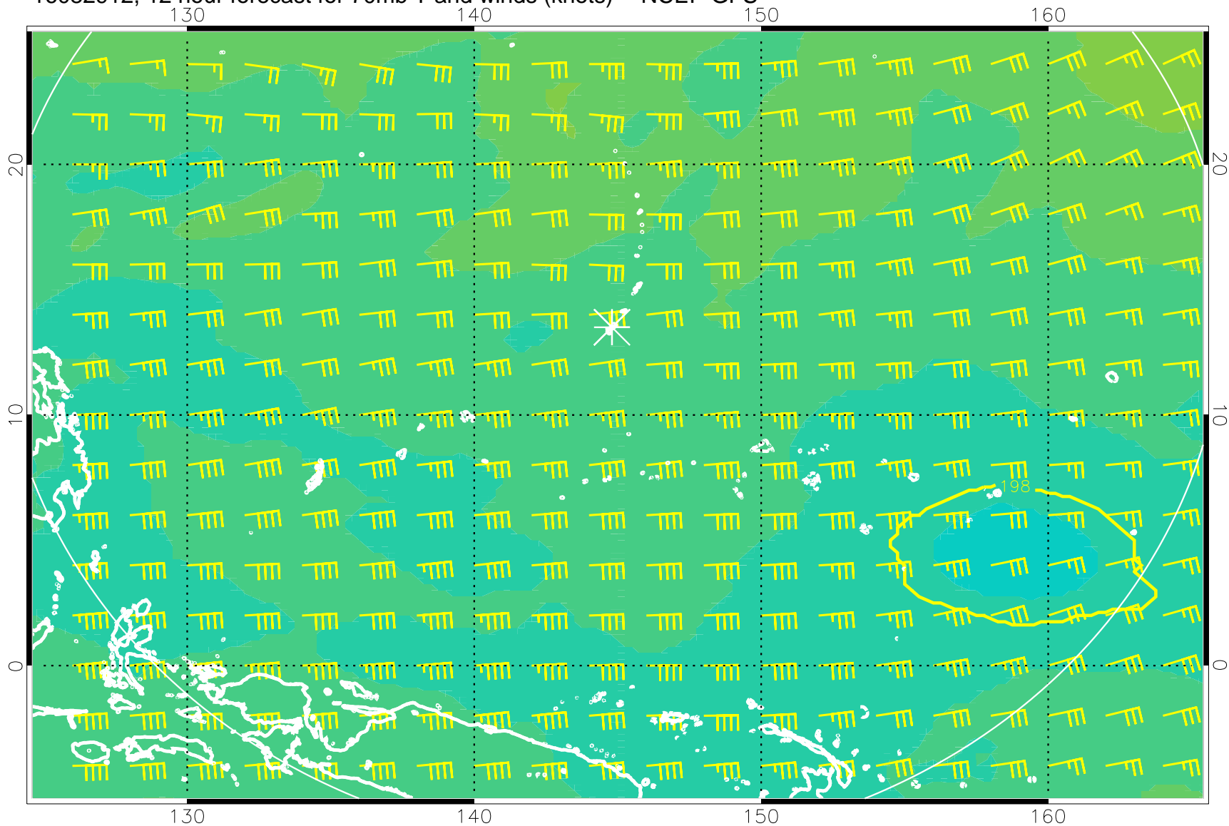
16082912, 12 hour forecast for 70mb T and winds (knots) -- NCEP GFS
