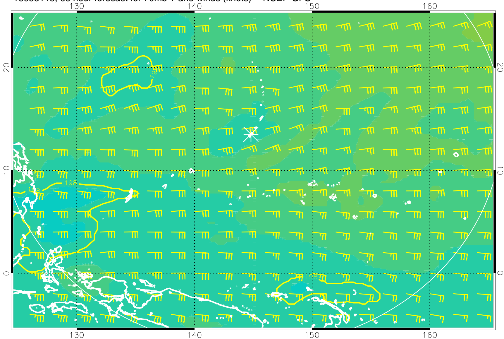
16083118, 66 hour forecast for 70mb T and winds (knots) -- NCEP GFS
