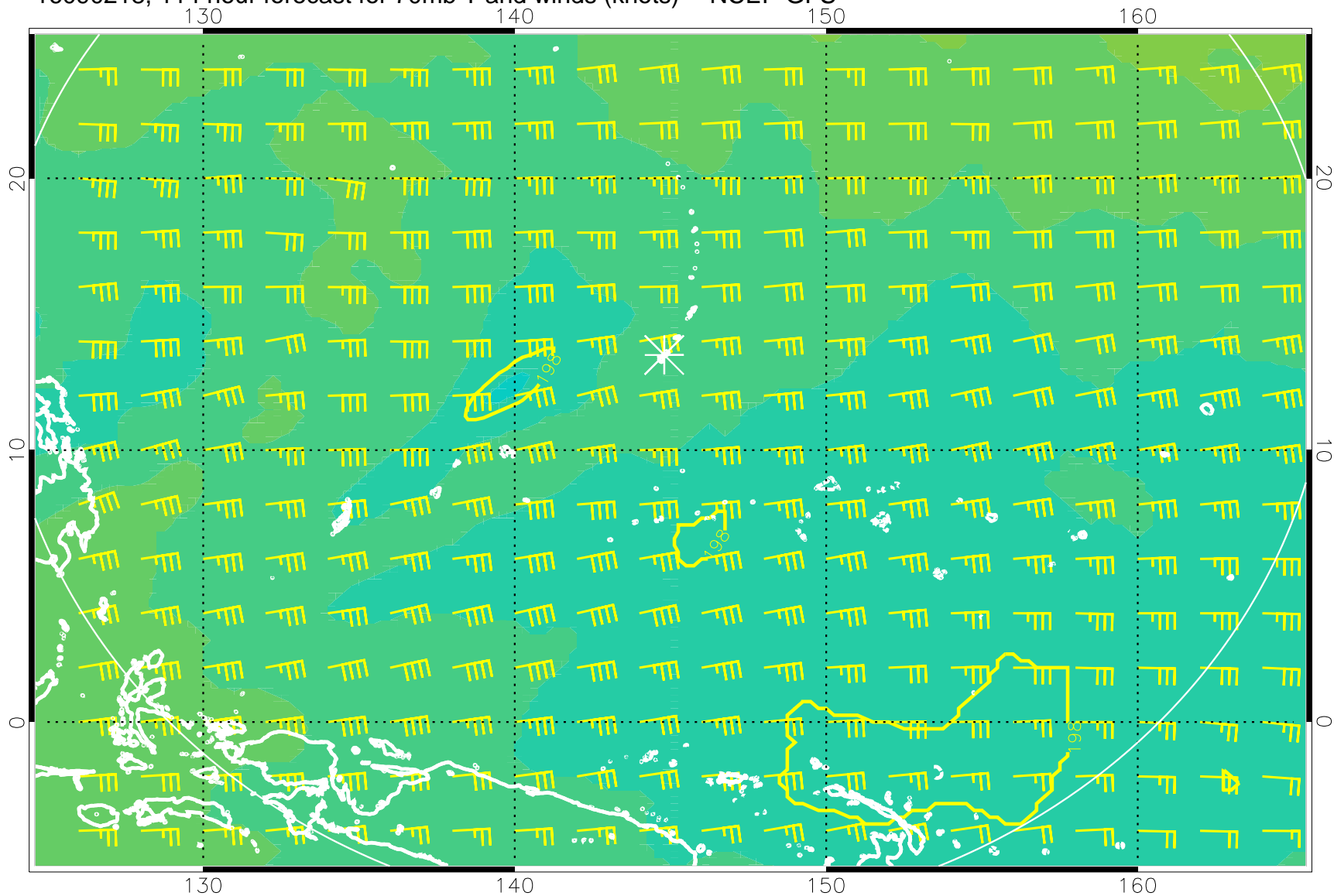
16090218, 114 hour forecast for 70mb T and winds (knots) -- NCEP GFS
