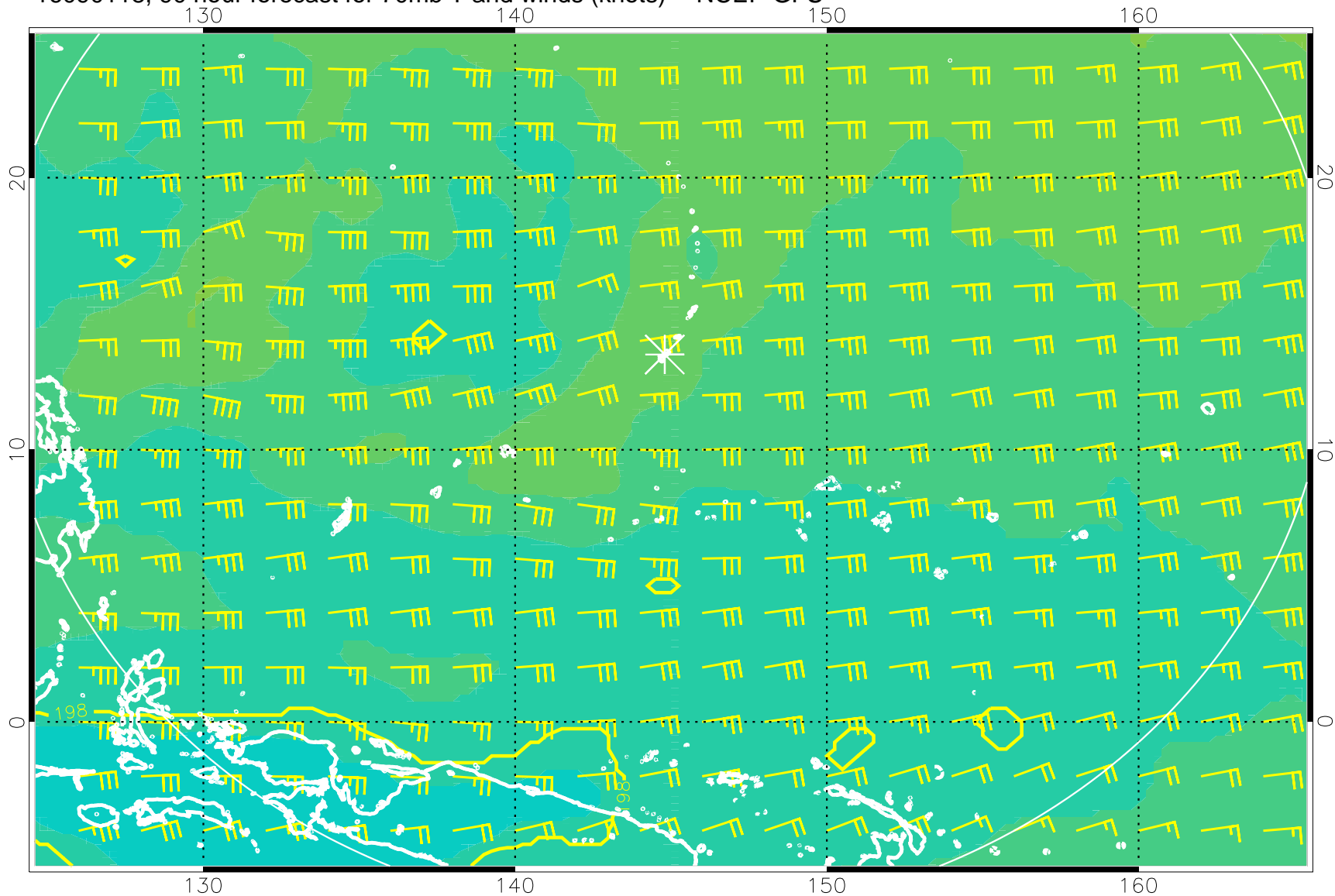
16090118, 90 hour forecast for 70mb T and winds (knots) -- NCEP GFS
