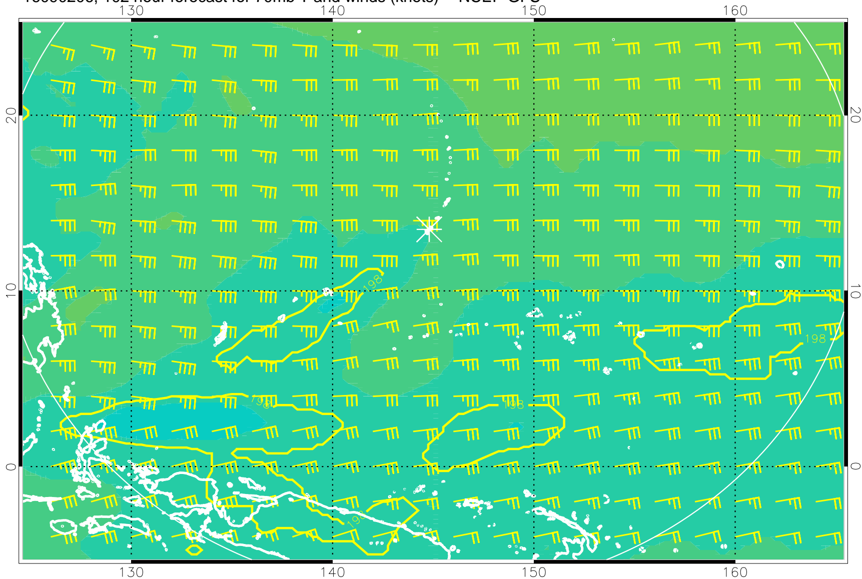
16090206, 102 hour forecast for 70mb T and winds (knots) -- NCEP GFS
