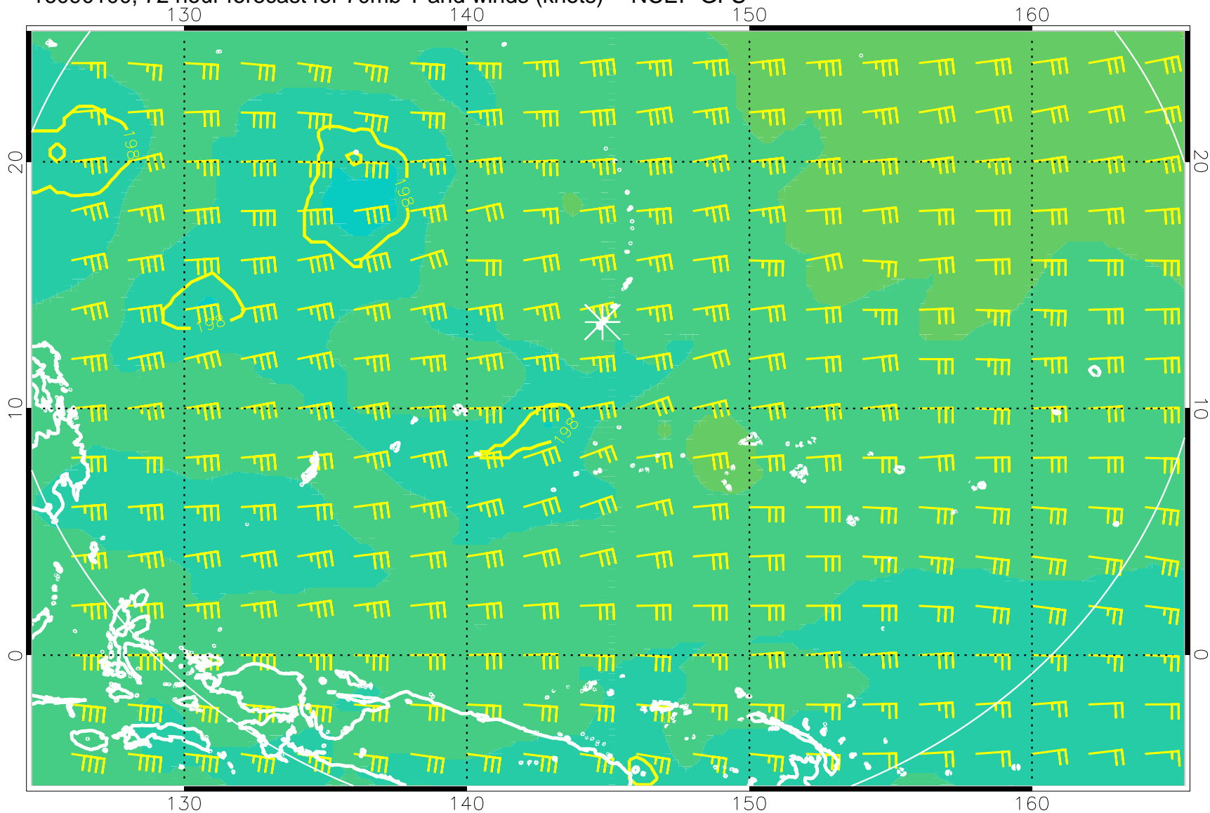
16090100, 72 hour forecast for 70mb T and winds (knots) -- NCEP GFS
