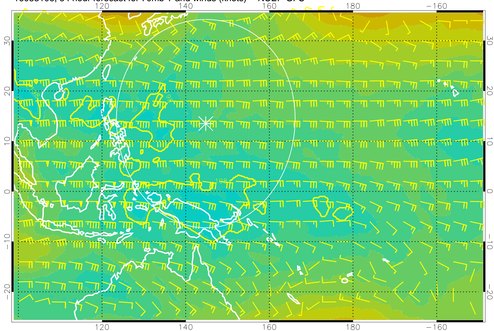
16083106, 54 hour forecast for 70mb T and winds (knots) -- NCEP GFS
