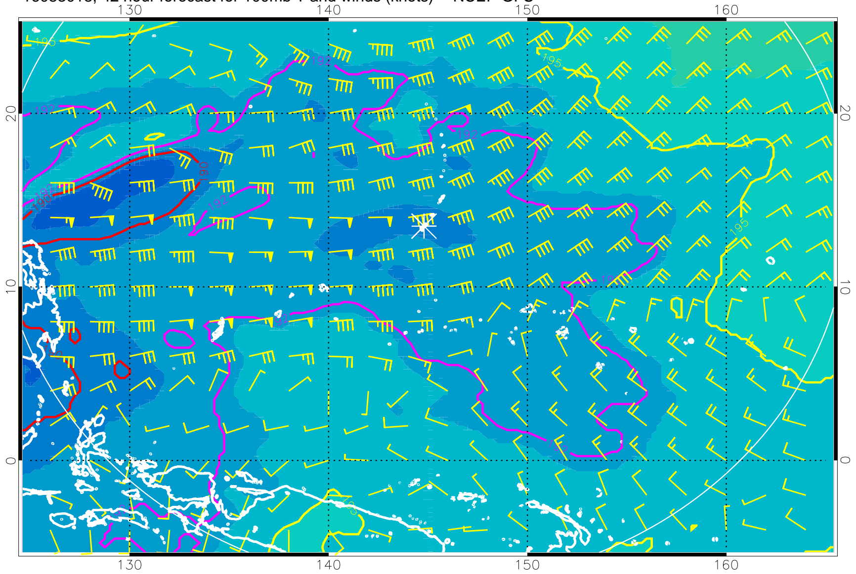
16083018, 42 hour forecast for 100mb T and winds (knots) -- NCEP GFS
