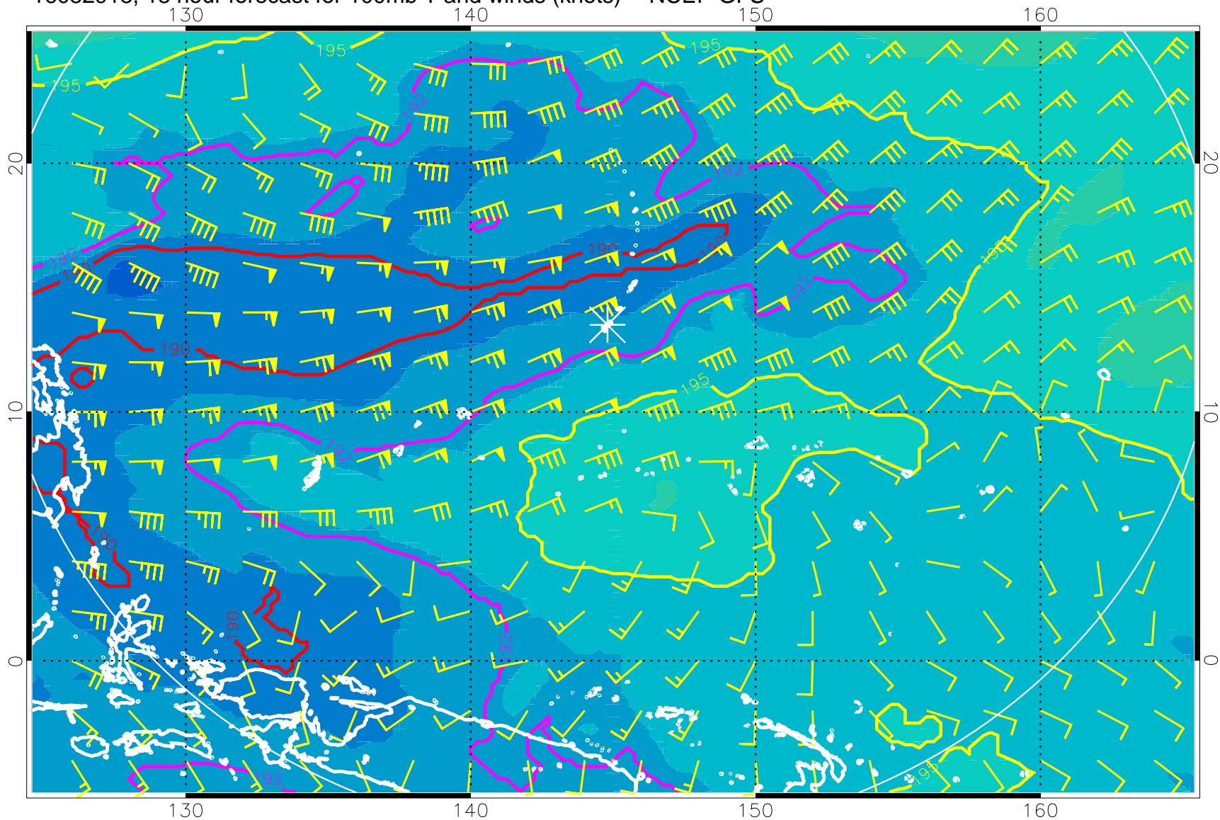
16082918, 18 hour forecast for 100mb T and winds (knots) -- NCEP GFS
