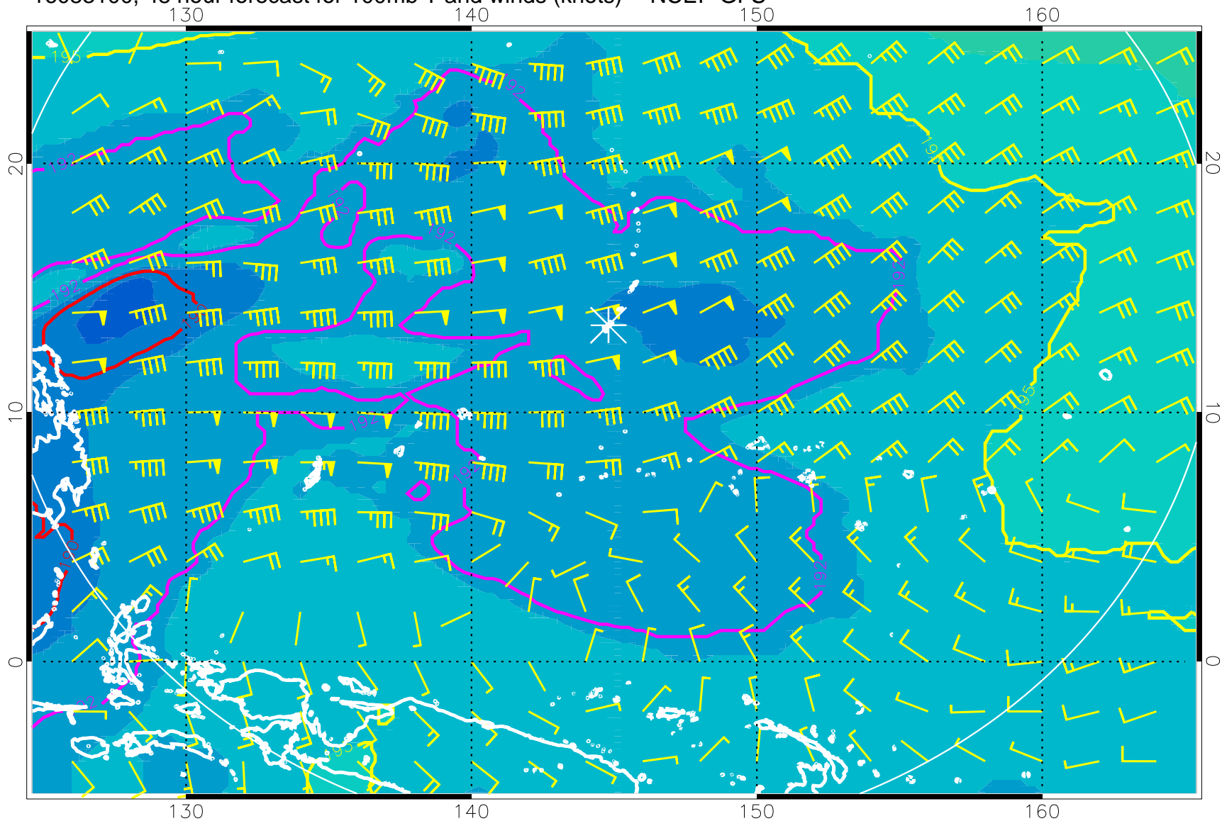
16083100, 48 hour forecast for 100mb T and winds (knots) -- NCEP GFS
