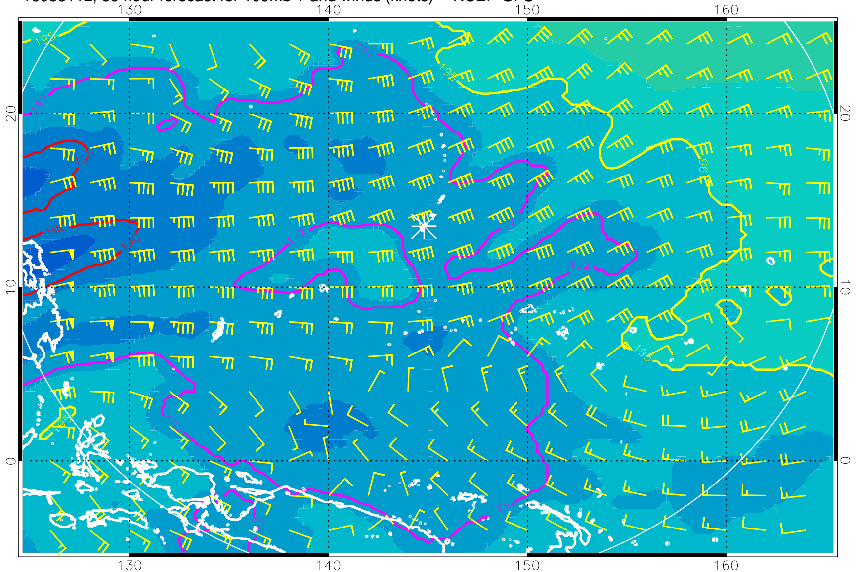
16083112, 60 hour forecast for 100mb T and winds (knots) -- NCEP GFS
