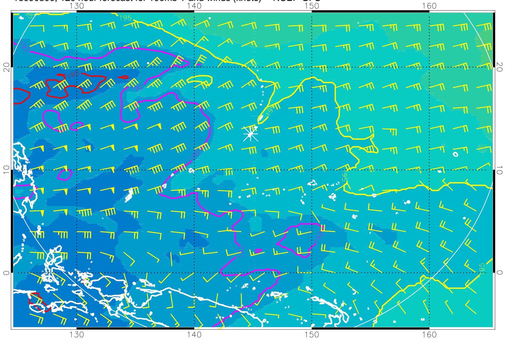
16090300, 120 hour forecast for 100mb T and winds (knots) -- NCEP GFS
