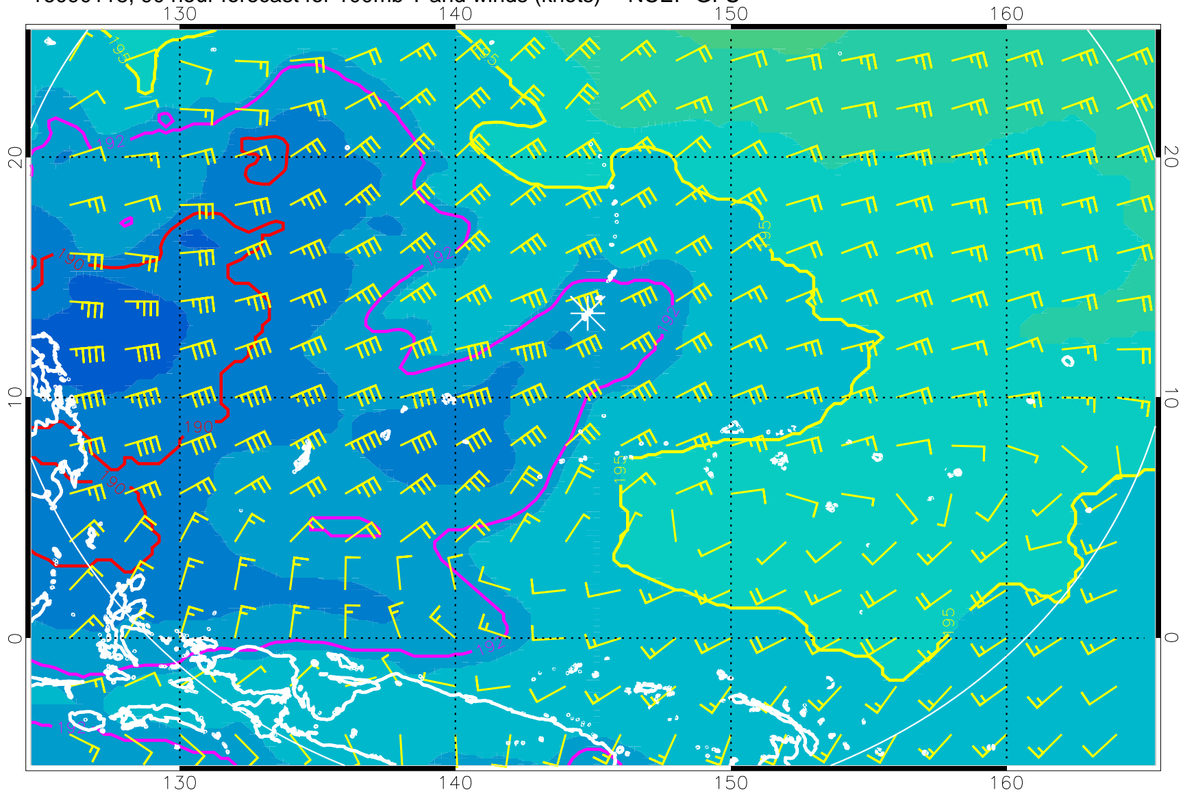
16090118, 90 hour forecast for 100mb T and winds (knots) -- NCEP GFS
