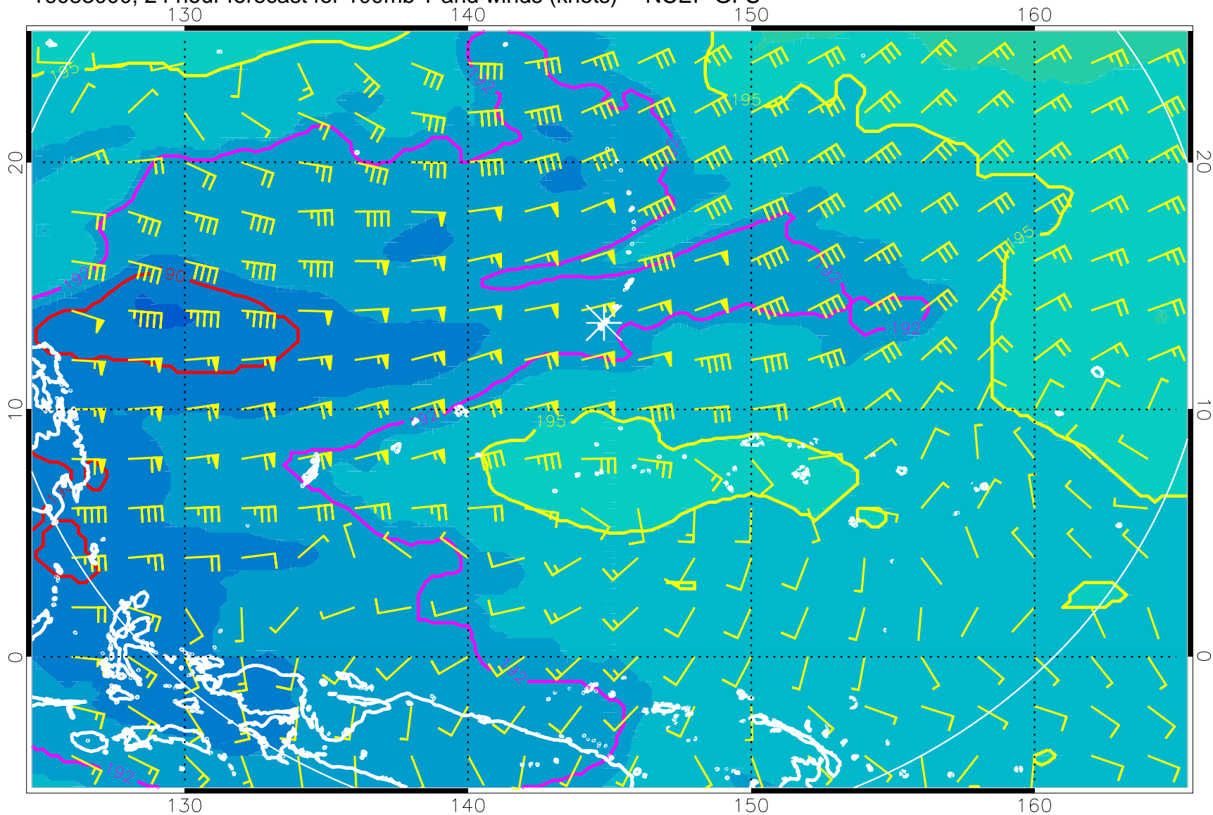
16083000, 24 hour forecast for 100mb T and winds (knots) -- NCEP GFS
