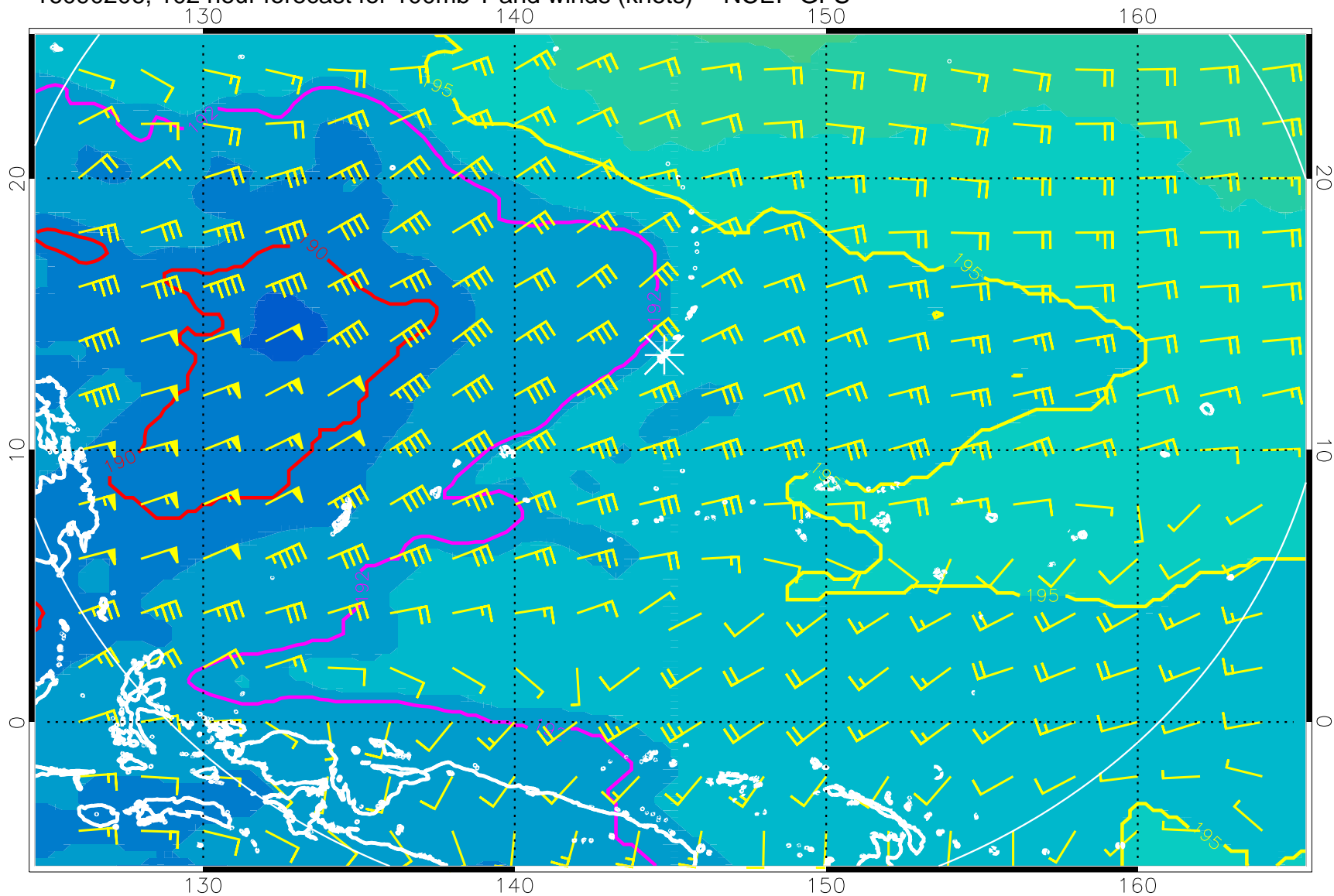
16090206, 102 hour forecast for 100mb T and winds (knots) -- NCEP GFS
