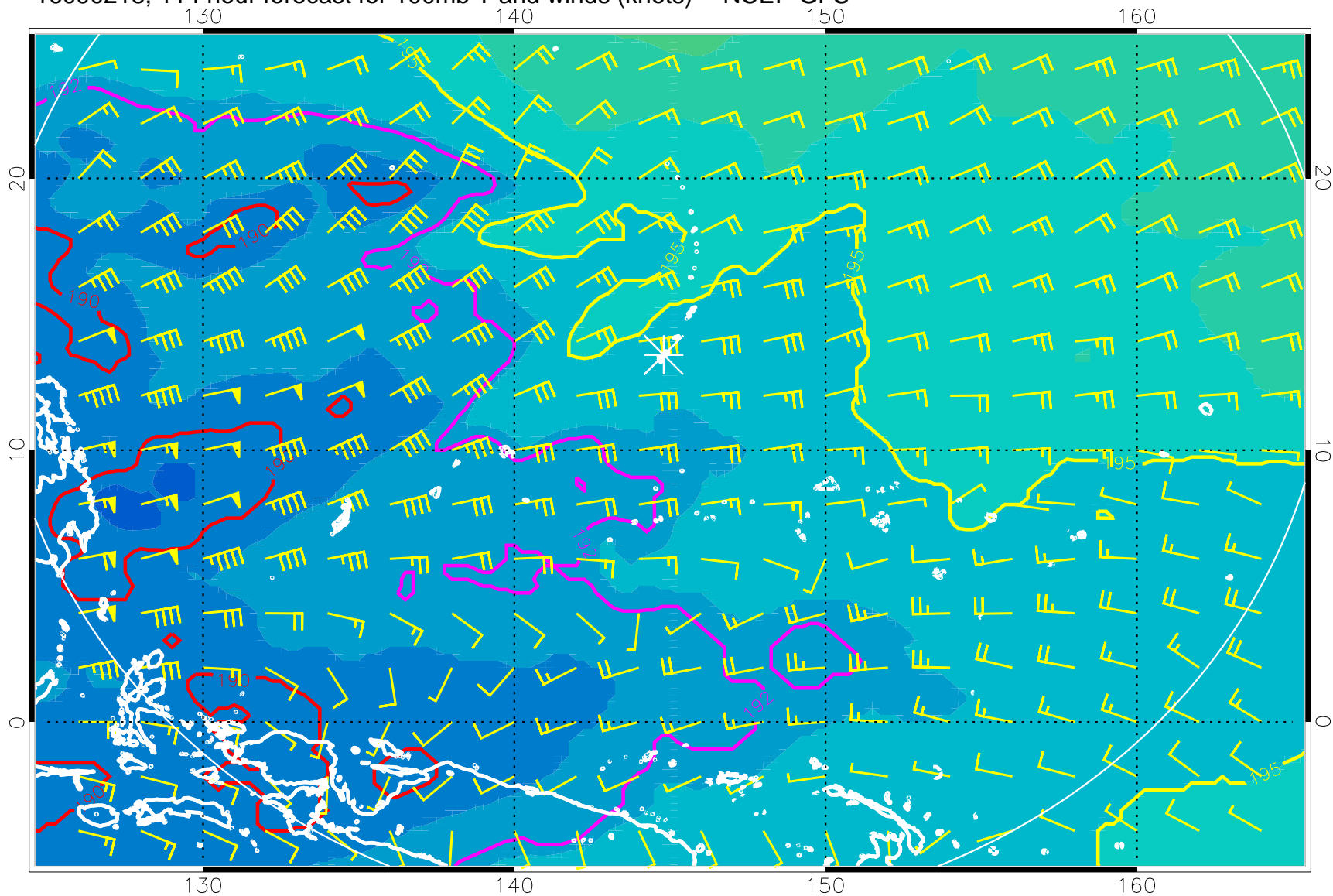
16090218, 114 hour forecast for 100mb T and winds (knots) -- NCEP GFS
