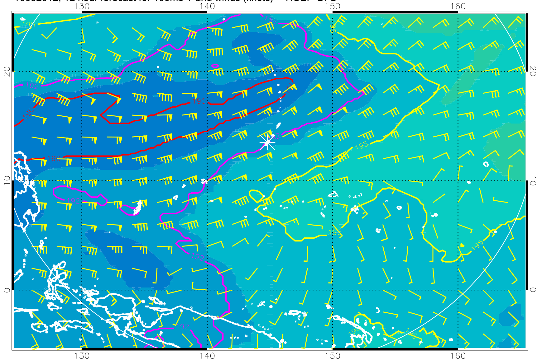
16082912, 12 hour forecast for 100mb T and winds (knots) -- NCEP GFS
