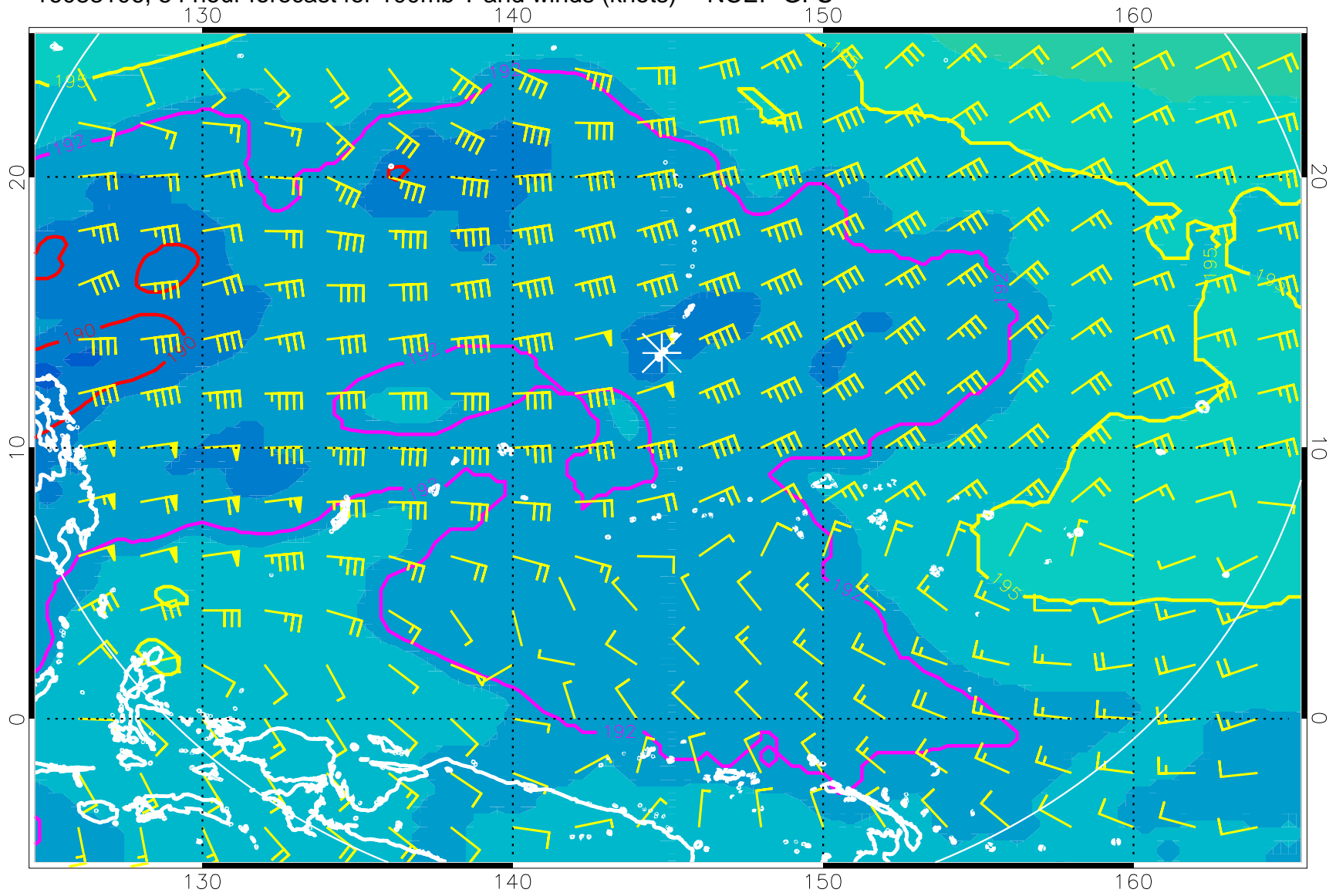
16083106, 54 hour forecast for 100mb T and winds (knots) -- NCEP GFS
