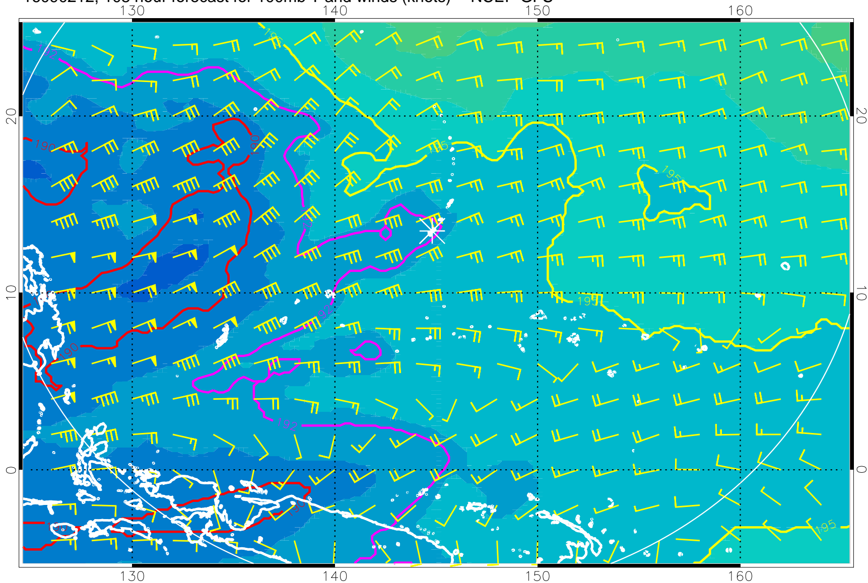
16090212, 108 hour forecast for 100mb T and winds (knots) -- NCEP GFS
