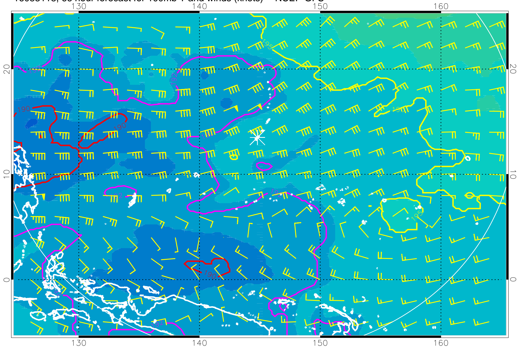
16083118, 66 hour forecast for 100mb T and winds (knots) -- NCEP GFS
