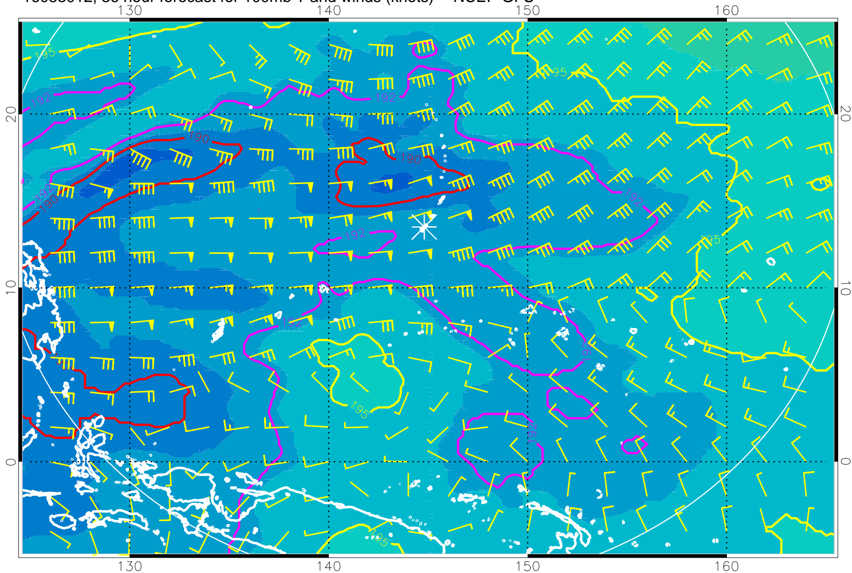
16083012, 36 hour forecast for 100mb T and winds (knots) -- NCEP GFS
