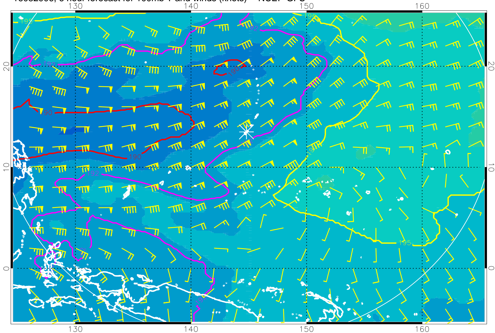
16082906, 6 hour forecast for 100mb T and winds (knots) -- NCEP GFS
