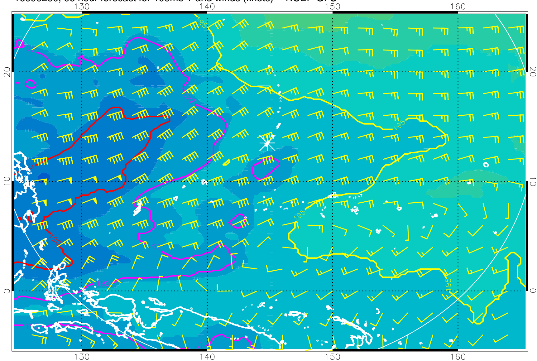
16090200, 96 hour forecast for 100mb T and winds (knots) -- NCEP GFS
