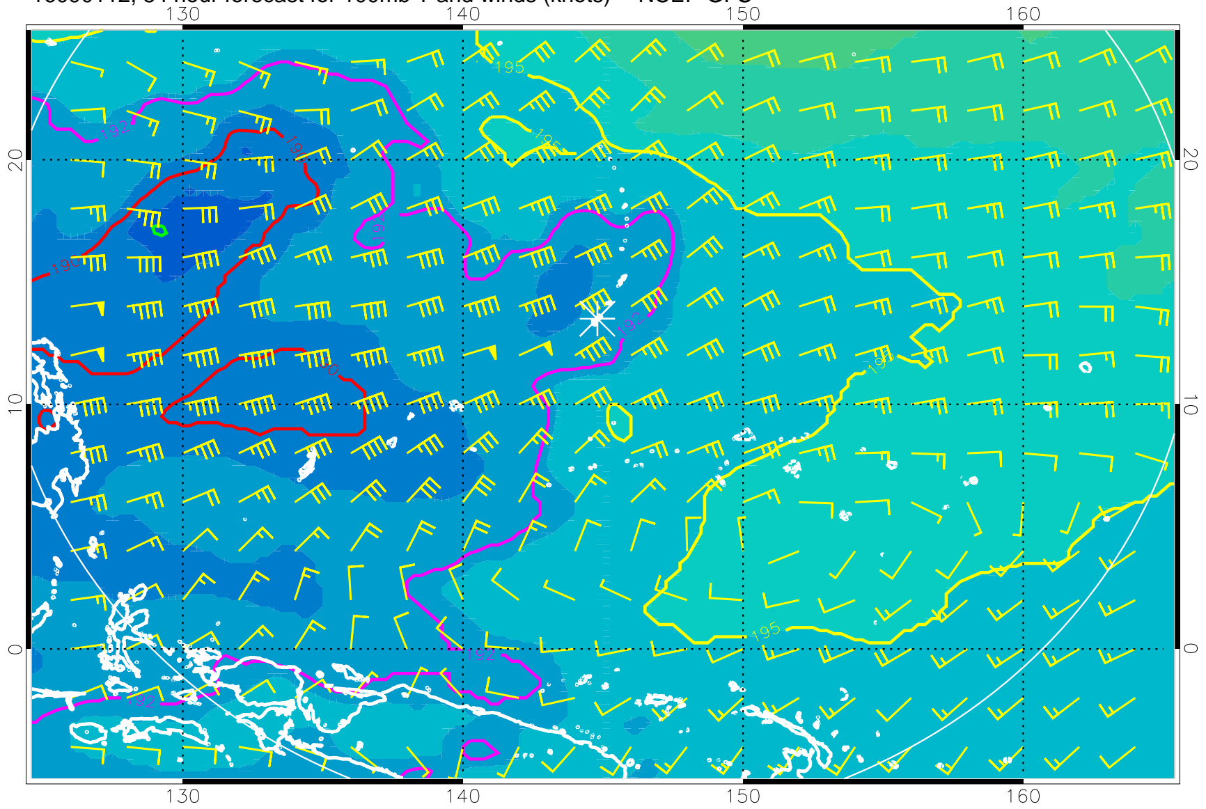
16090112, 84 hour forecast for 100mb T and winds (knots) -- NCEP GFS
