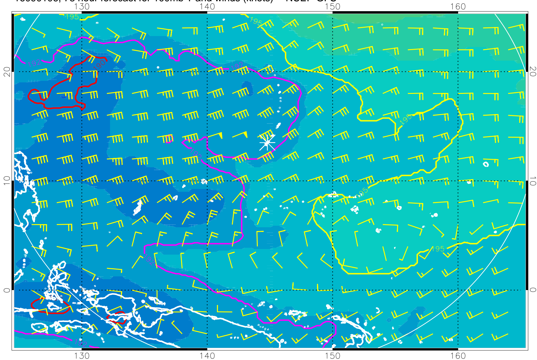
16090106, 78 hour forecast for 100mb T and winds (knots) -- NCEP GFS
