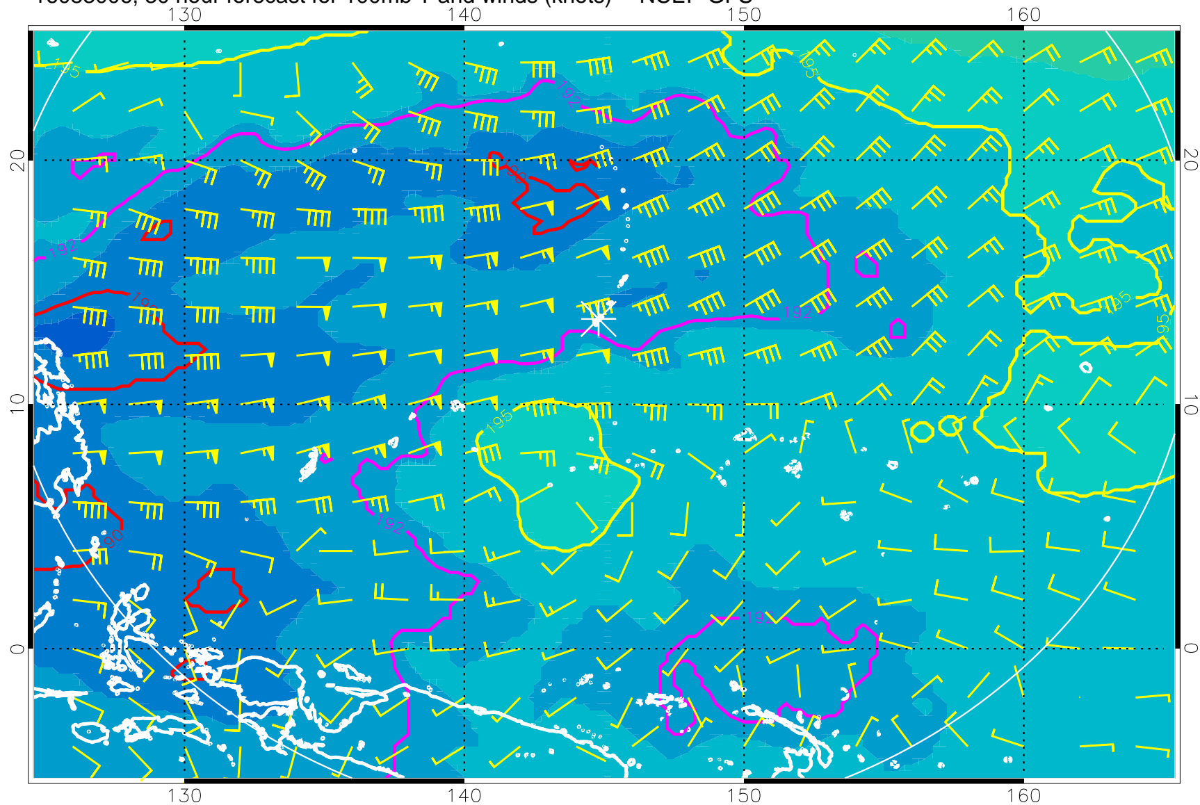
16083006, 30 hour forecast for 100mb T and winds (knots) -- NCEP GFS
