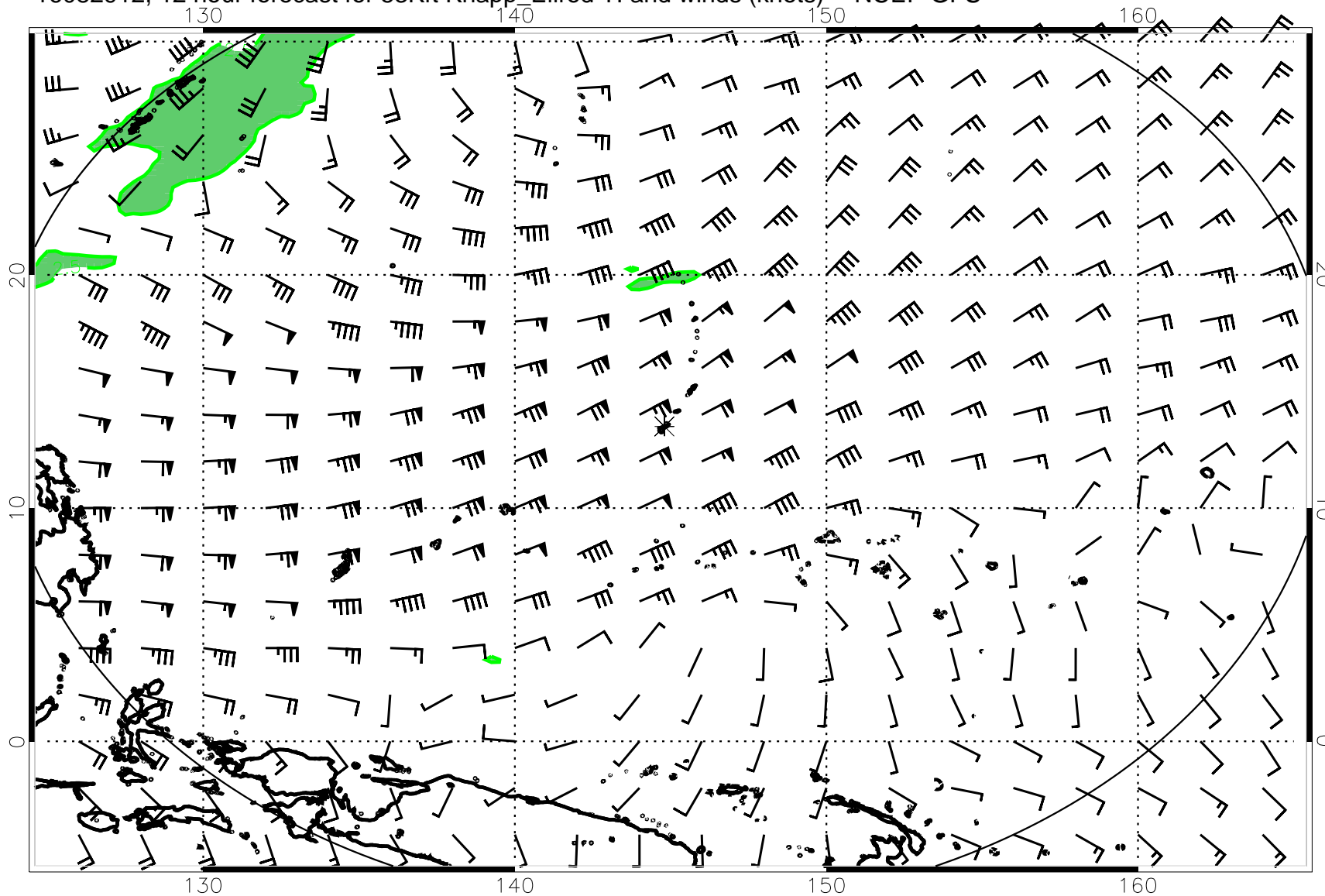
16082912, 12 hour forecast for 53Kft Knapp_Ellrod TI and winds (knots) -- NCEP GFS
