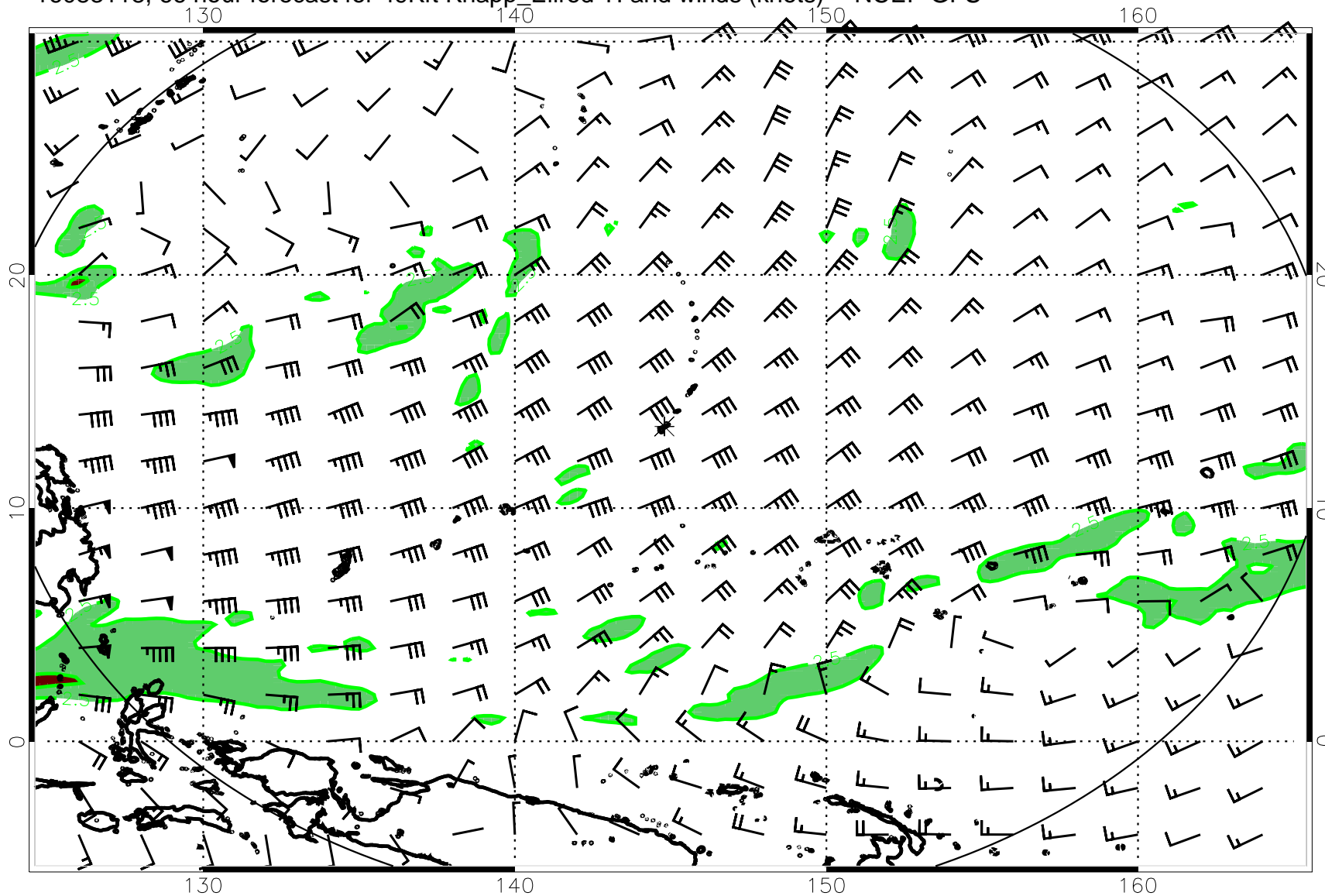
16083118, 66 hour forecast for 49Kft Knapp_Ellrod TI and winds (knots) -- NCEP GFS
