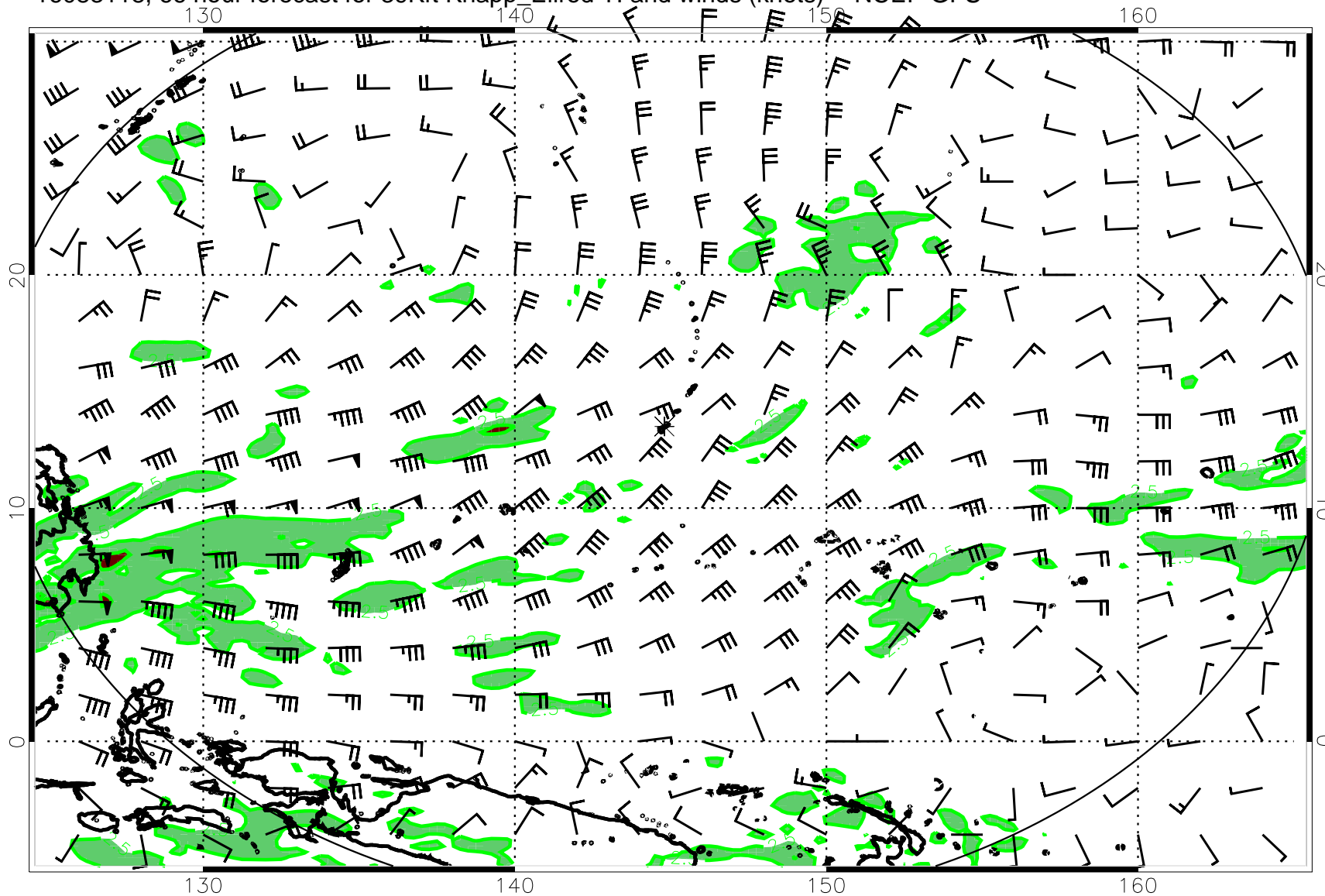
16083118, 66 hour forecast for 39Kft Knapp_Ellrod TI and winds (knots) -- NCEP GFS
