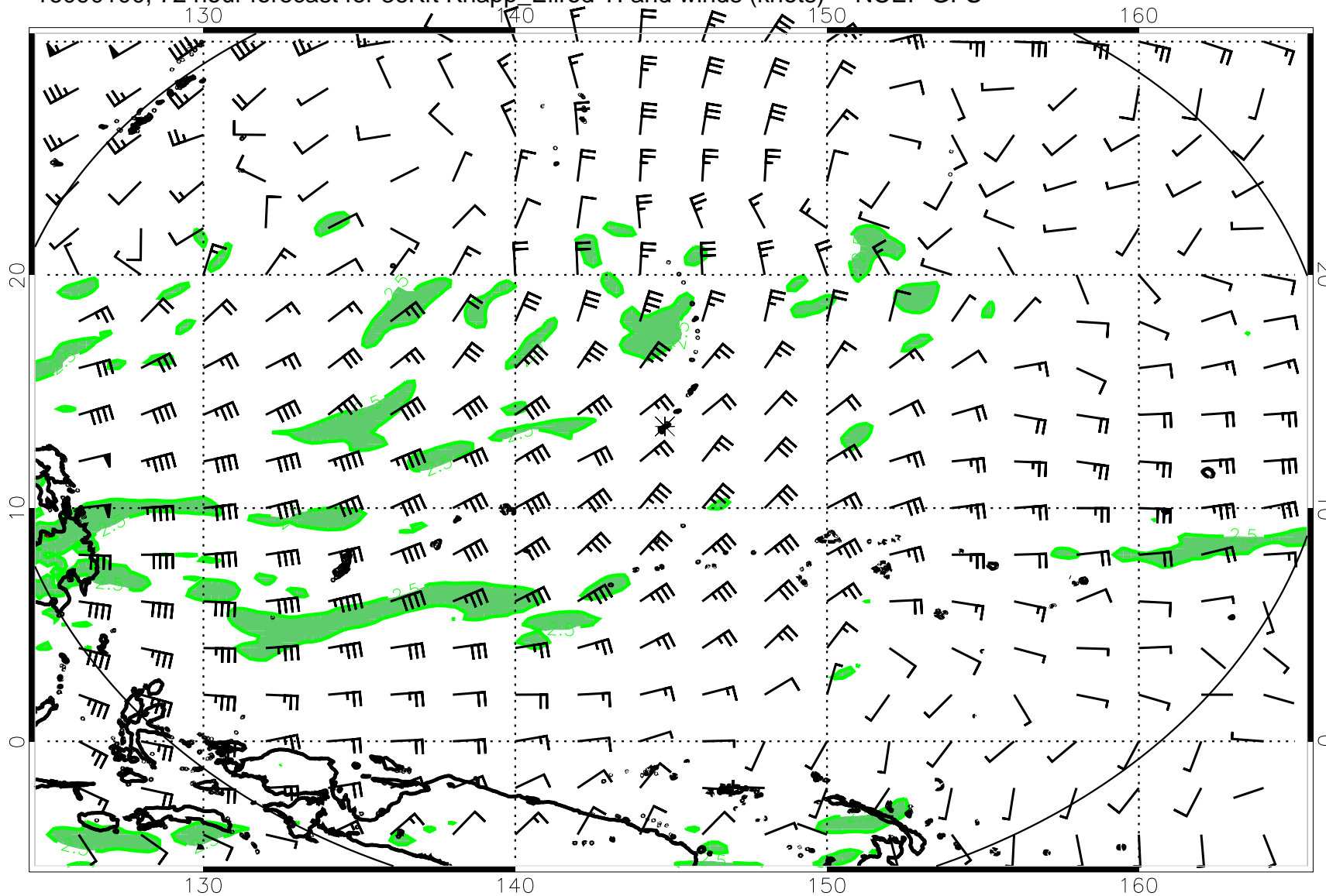
16090100, 72 hour forecast for 36Kft Knapp Ellrod TI and winds (knots) -- NCEP GFS
