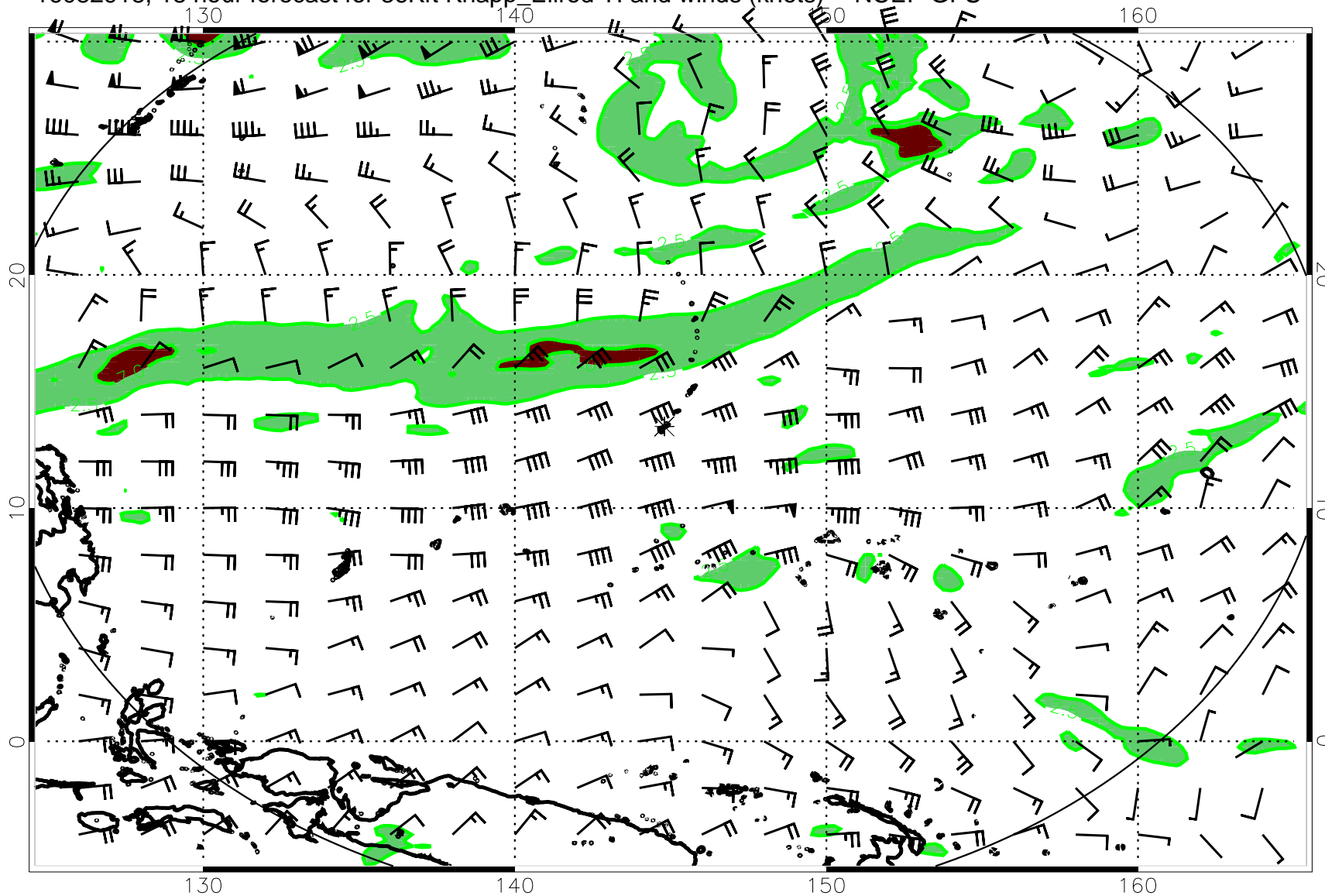
16082918, 18 hour forecast for 36Kft Knapp_Ellrod TI and winds (knots) -- NCEP GFS
