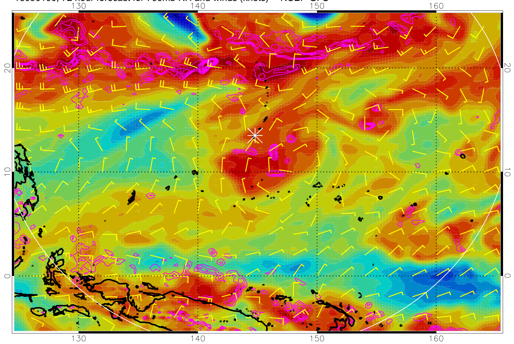
16090100, 72 hour forecast for 700mb RH and winds (knots) -- NCEP GFS
