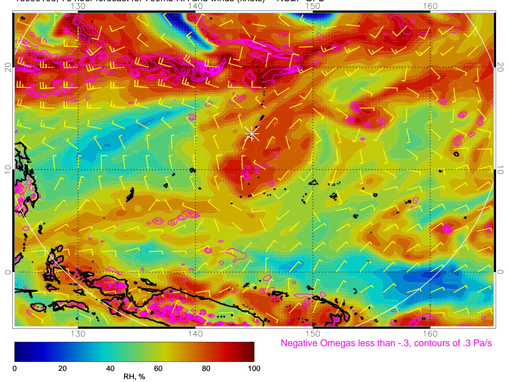
16090106, 78 hour forecast for 700mb RH and winds (knots) -- NCEP GFS
