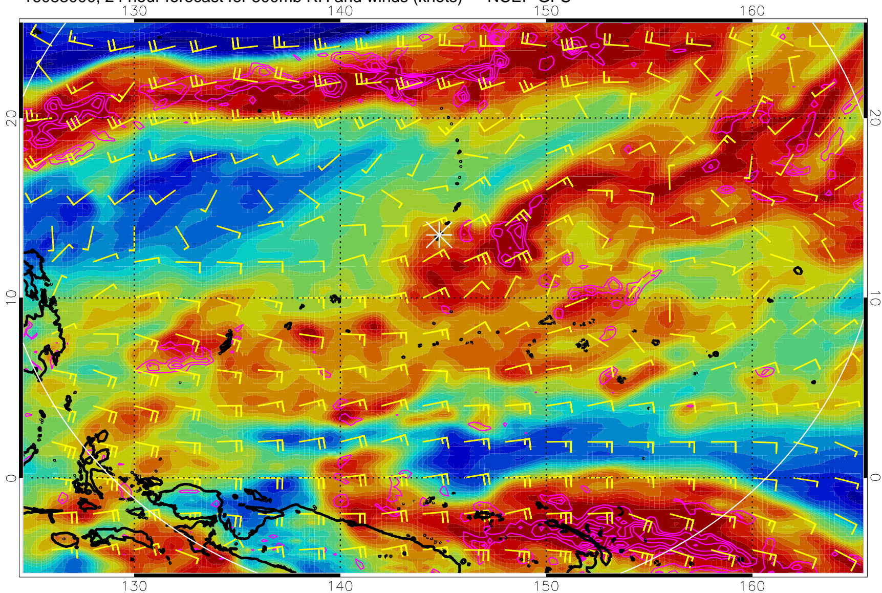
16083000, 24 hour forecast for 500mb RH and winds (knots) -- NCEP GFS
