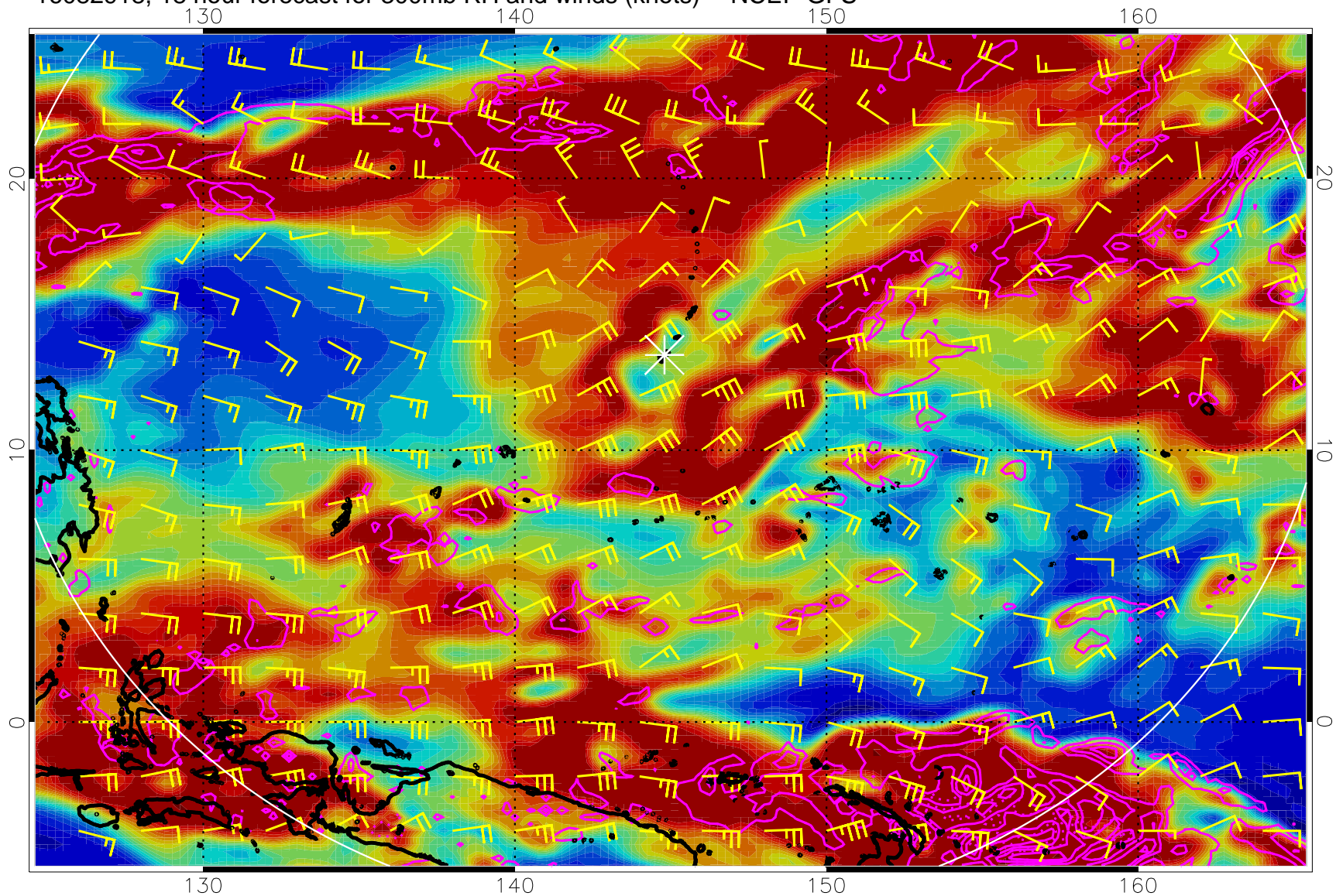
16082918, 18 hour forecast for 300mb RH and winds (knots) -- NCEP GFS
