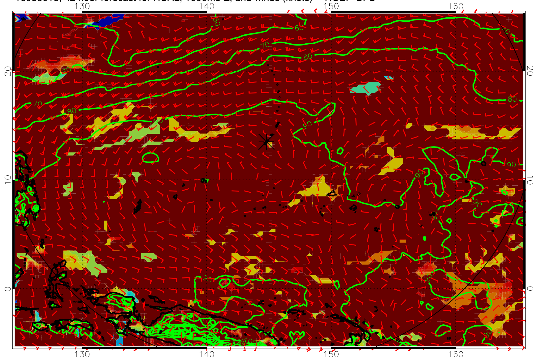
16083018, 42 hour forecast for HCAL, 1000mb Z, and winds (knots) -- NCEP GFS
