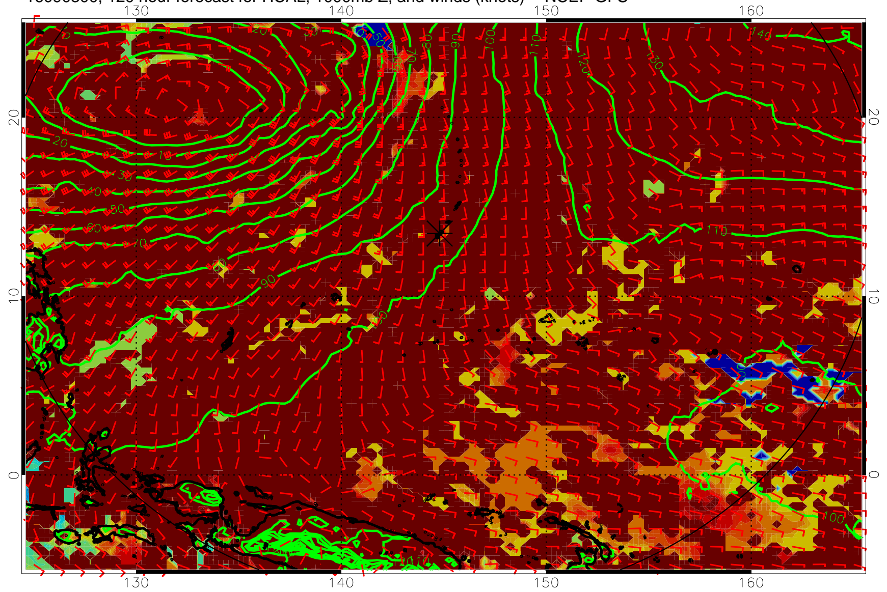
16090300, 120 hour forecast for HCAL, 1000mb Z, and winds (knots) -- NCEP GFS
