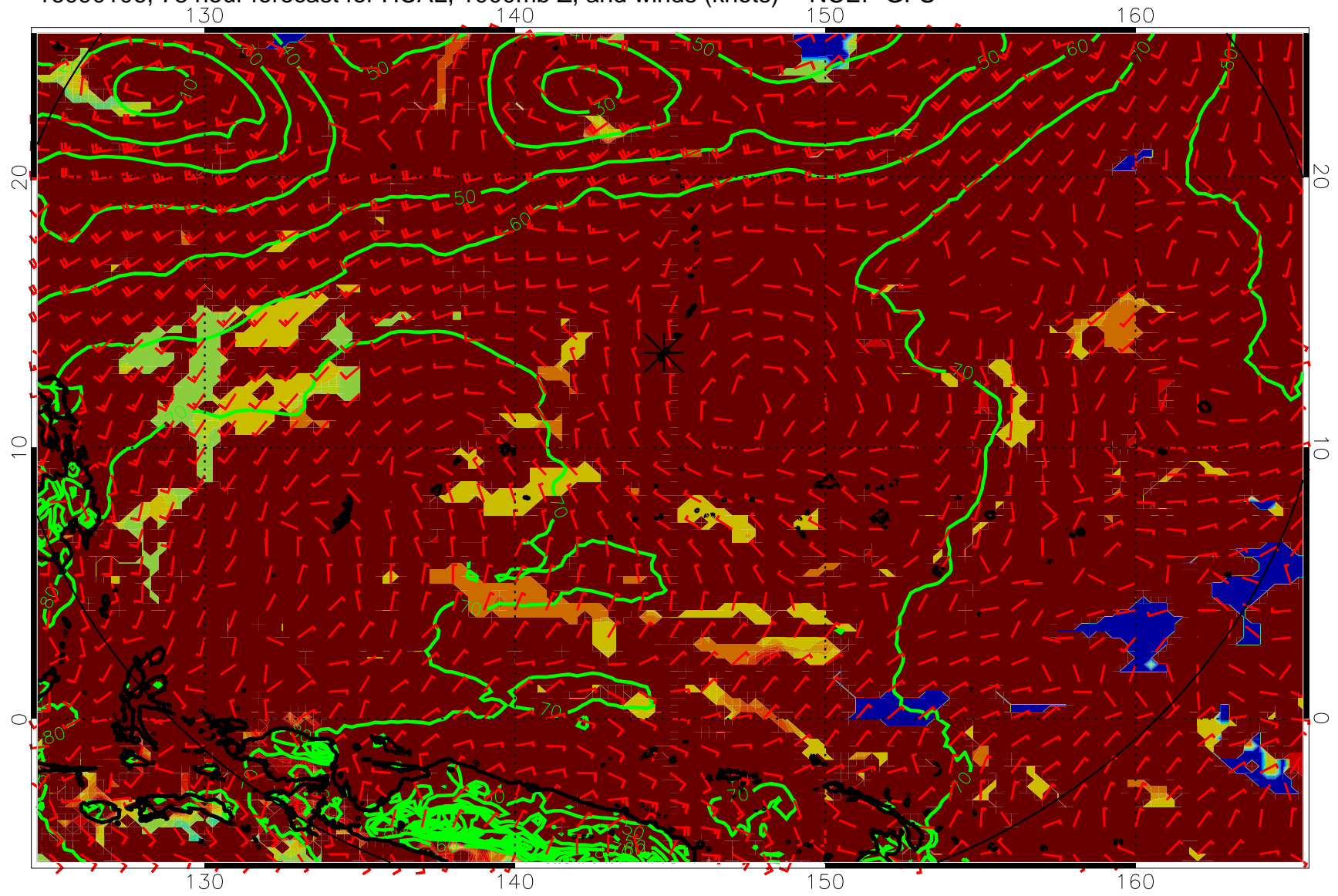
16090106, 78 hour forecast for HCAL, 1000mb Z, and winds (knots) -- NCEP GFS
