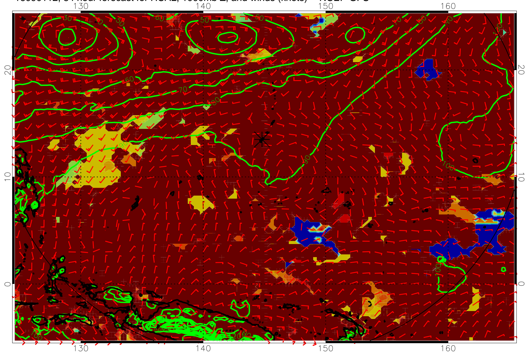
16090112, 84 hour forecast for HCAL, 1000mb Z, and winds (knots) -- NCEP GFS
