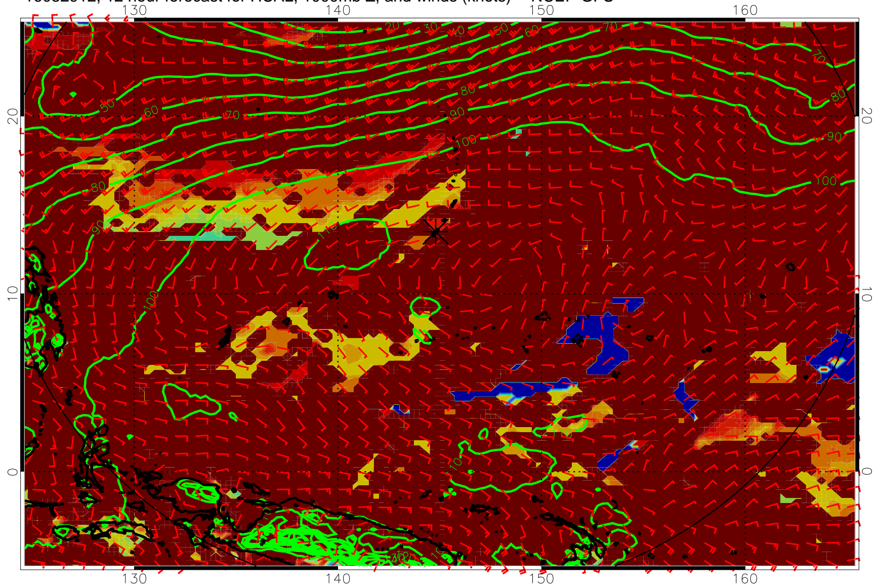
16082912, 12 hour forecast for HCAL, 1000mb Z, and winds (knots) -- NCEP GFS
