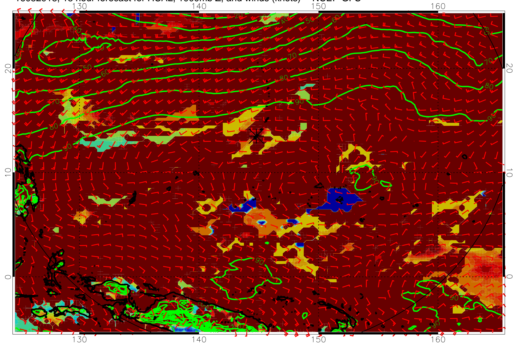
16082918, 18 hour forecast for HCAL, 1000mb Z, and winds (knots) -- NCEP GFS
