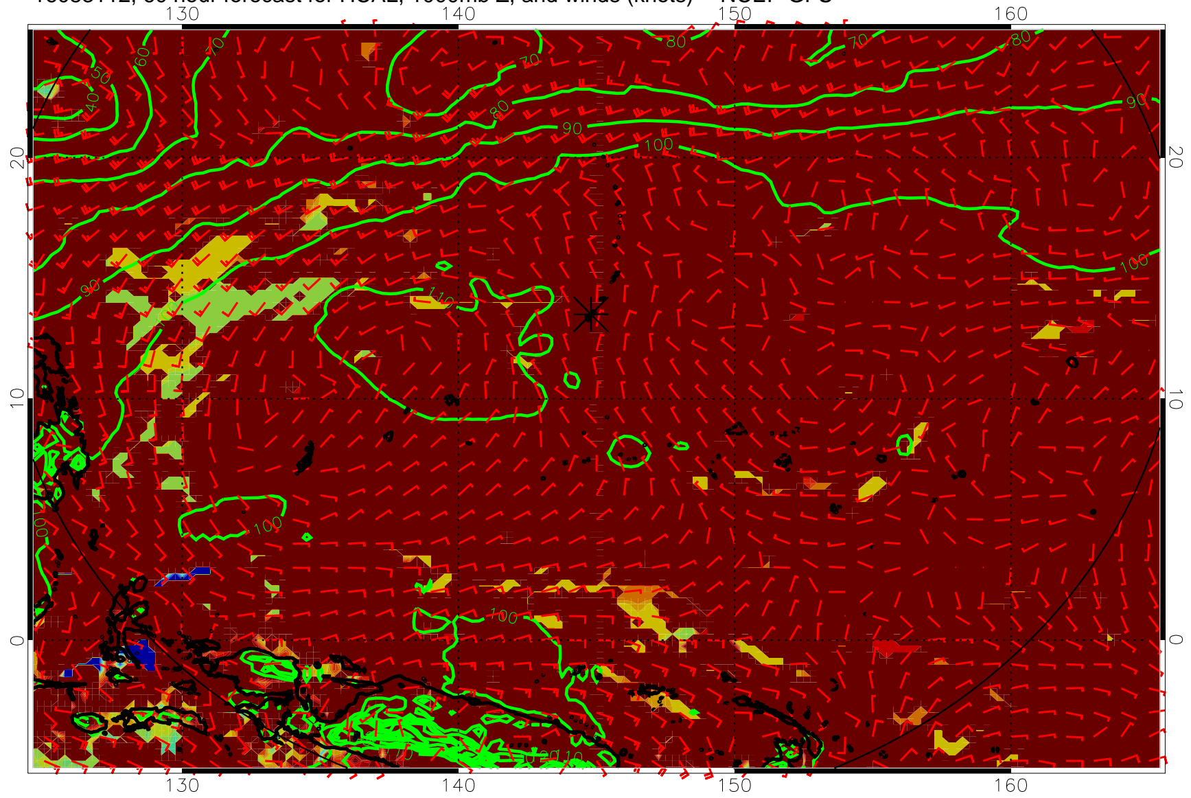
16083112, 60 hour forecast for HCAL, 1000mb Z, and winds (knots) -- NCEP GFS
