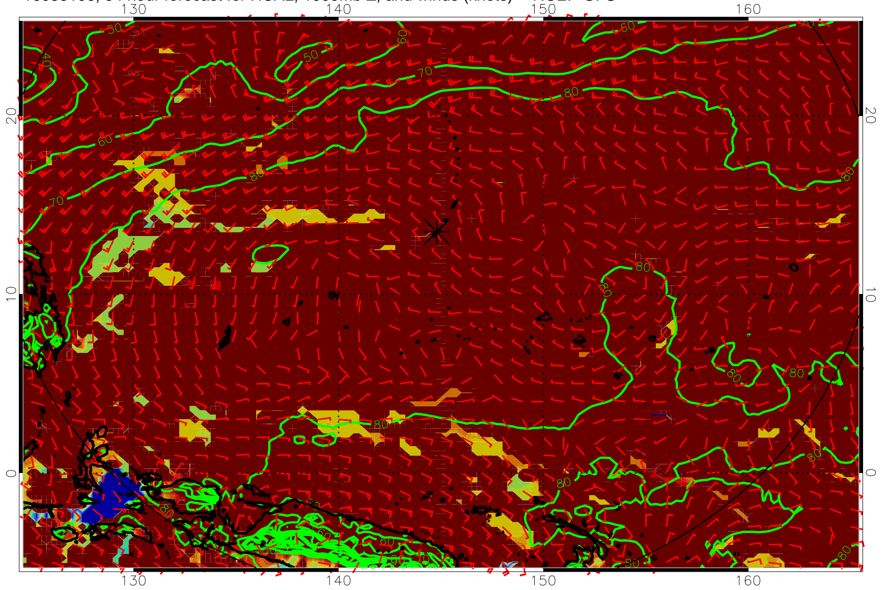
16083106, 54 hour forecast for HCAL, 1000mb Z, and winds (knots) -- NCEP GFS
