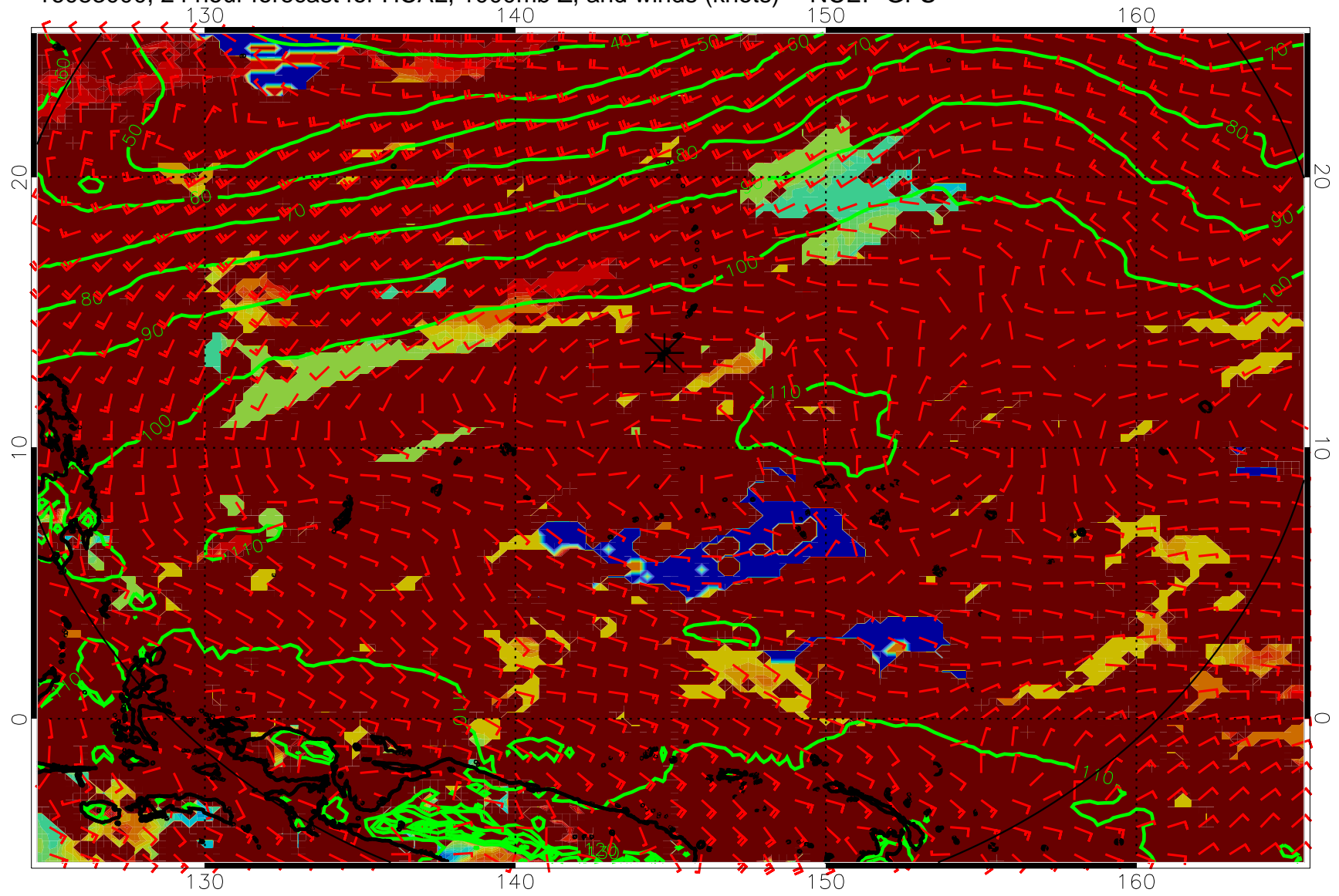
16083000, 24 hour forecast for HCAL, 1000mb Z, and winds (knots) -- NCEP GFS
