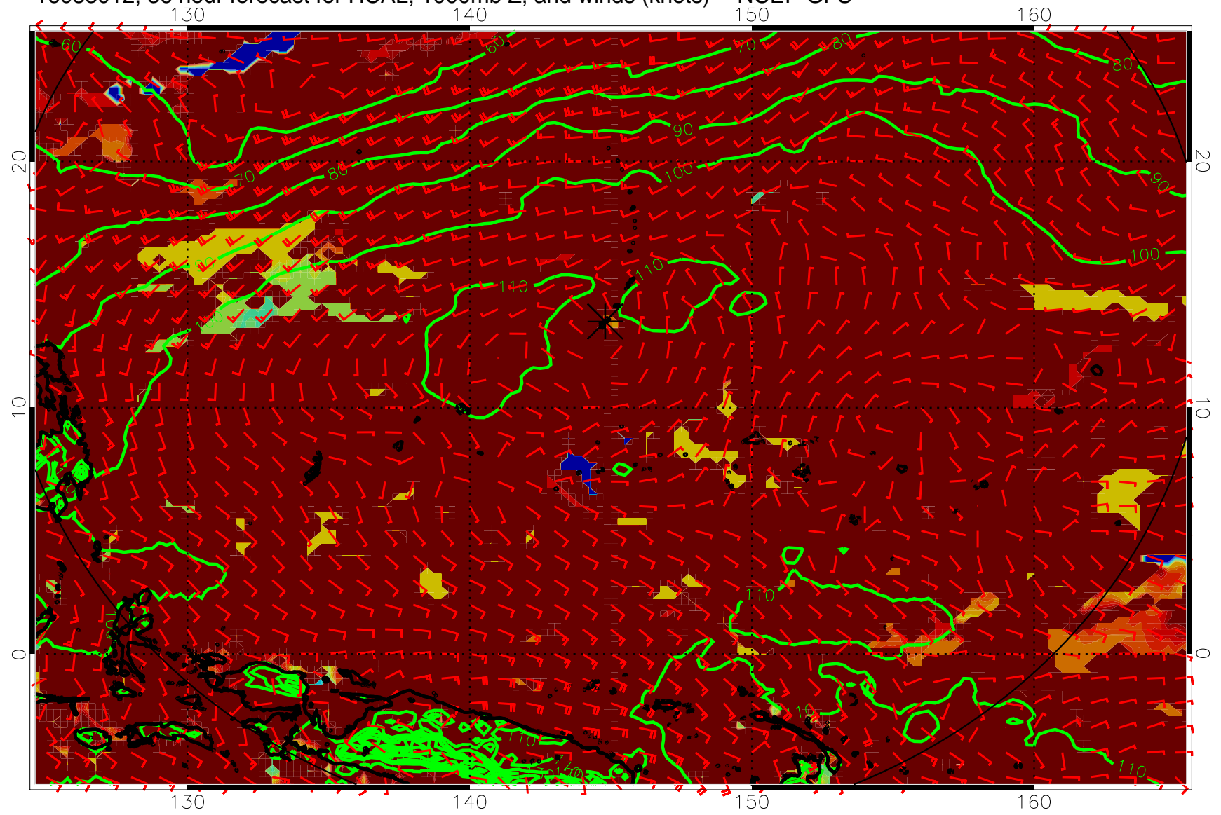
16083012, 36 hour forecast for HCAL, 1000mb Z, and winds (knots) -- NCEP GFS
