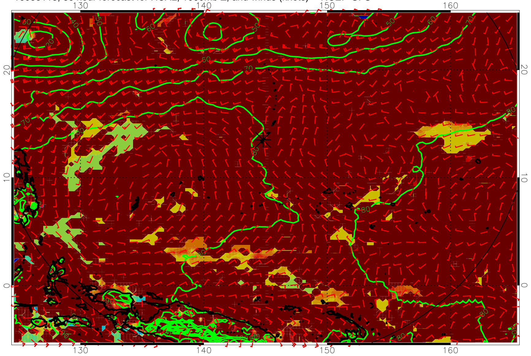
16083118, 66 hour forecast for HCAL, 1000mb Z, and winds (knots) -- NCEP GFS
