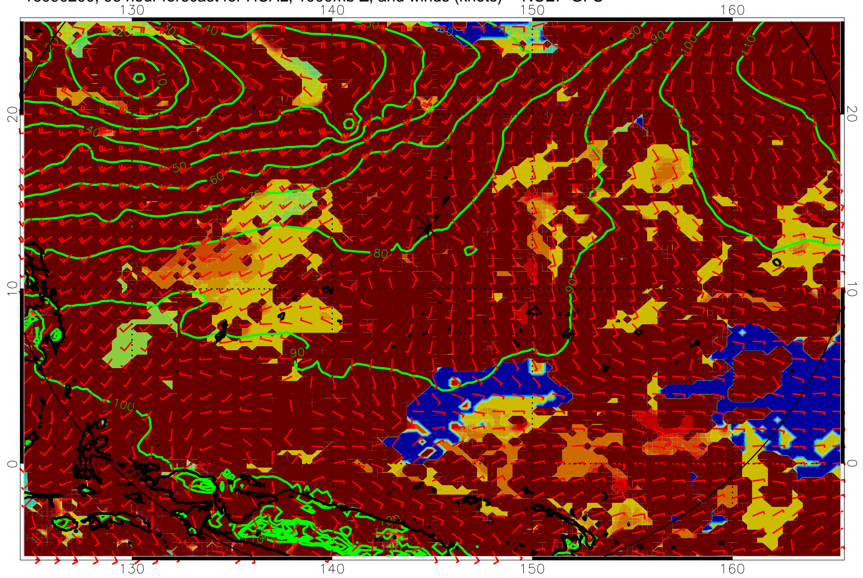
16090200, 96 hour forecast for HCAL, 1000mb Z, and winds (knots) -- NCEP GFS
