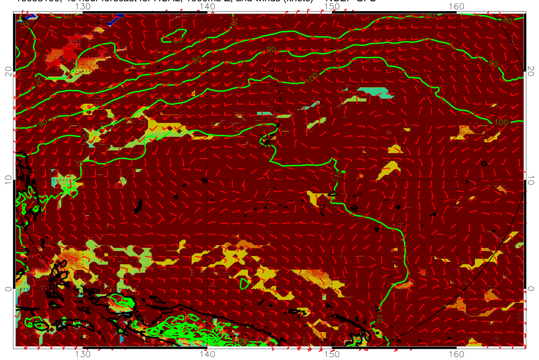
16083100, 48 hour forecast for HCAL, 1000mb Z, and winds (knots) -- NCEP GFS
