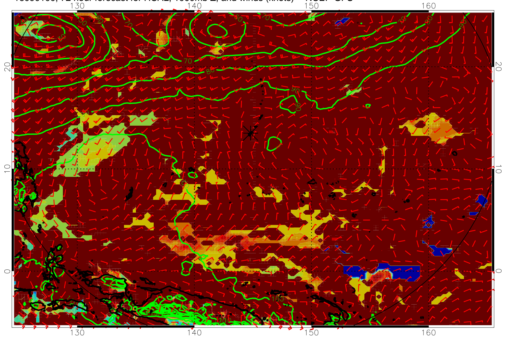
16090100, 72 hour forecast for HCAL, 1000mb Z, and winds (knots) -- NCEP GFS
