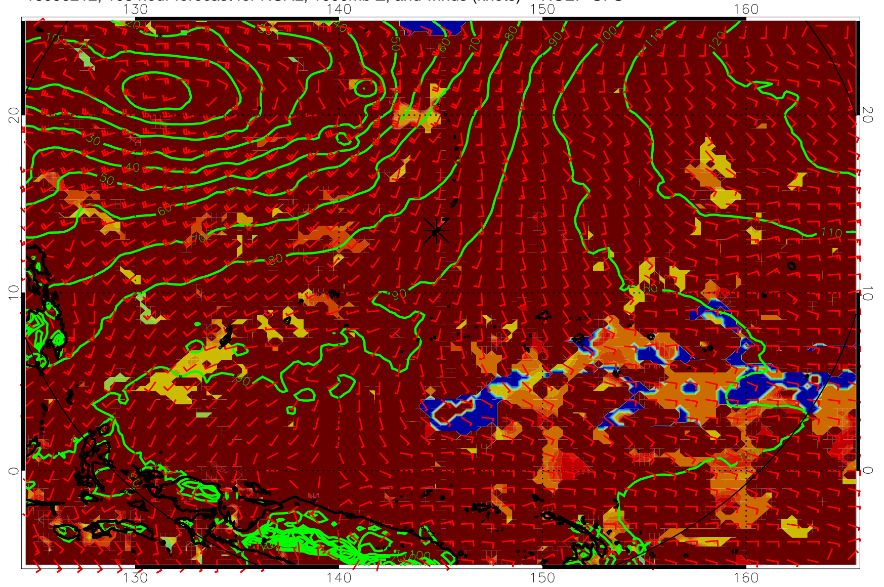
16090212, 108 hour forecast for HCAL, 1000mb Z, and winds (knots) -- NCEP GFS
