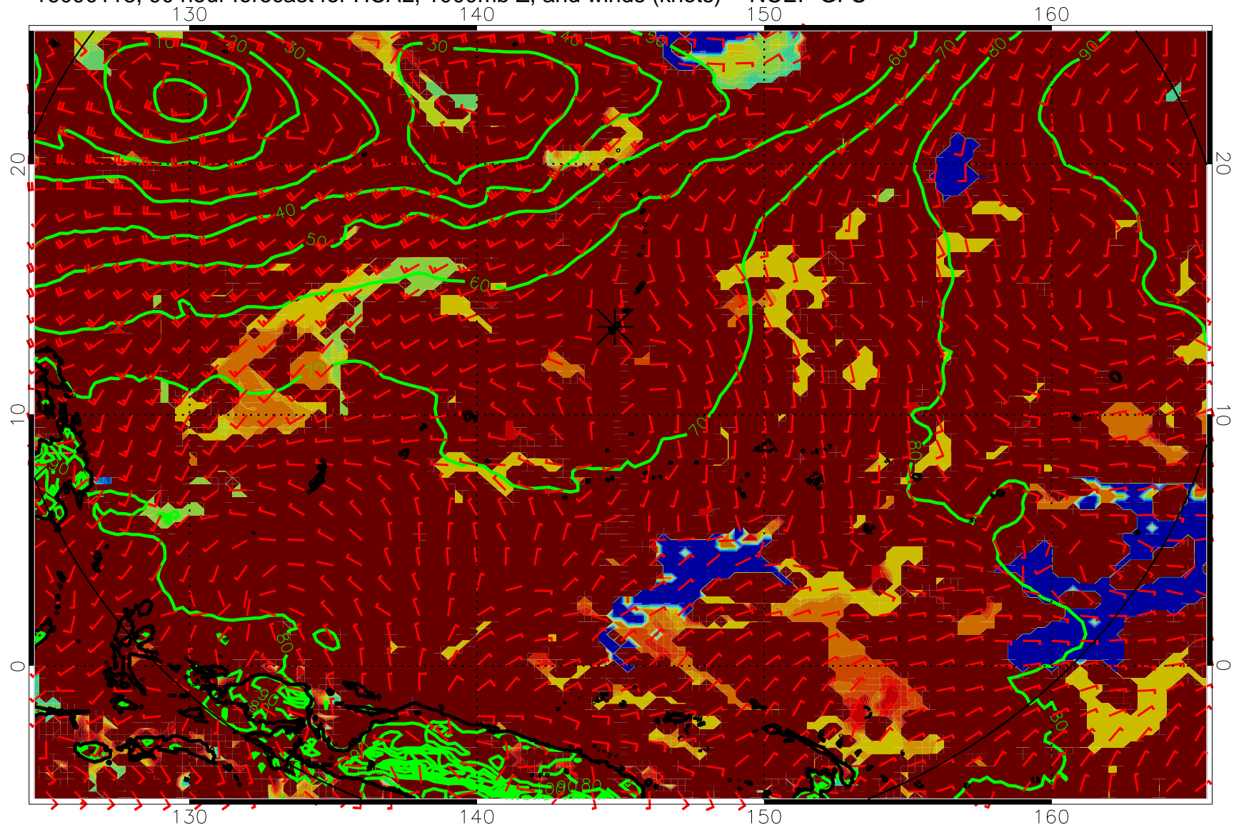
16090118, 90 hour forecast for HCAL, 1000mb Z, and winds (knots) -- NCEP GFS
