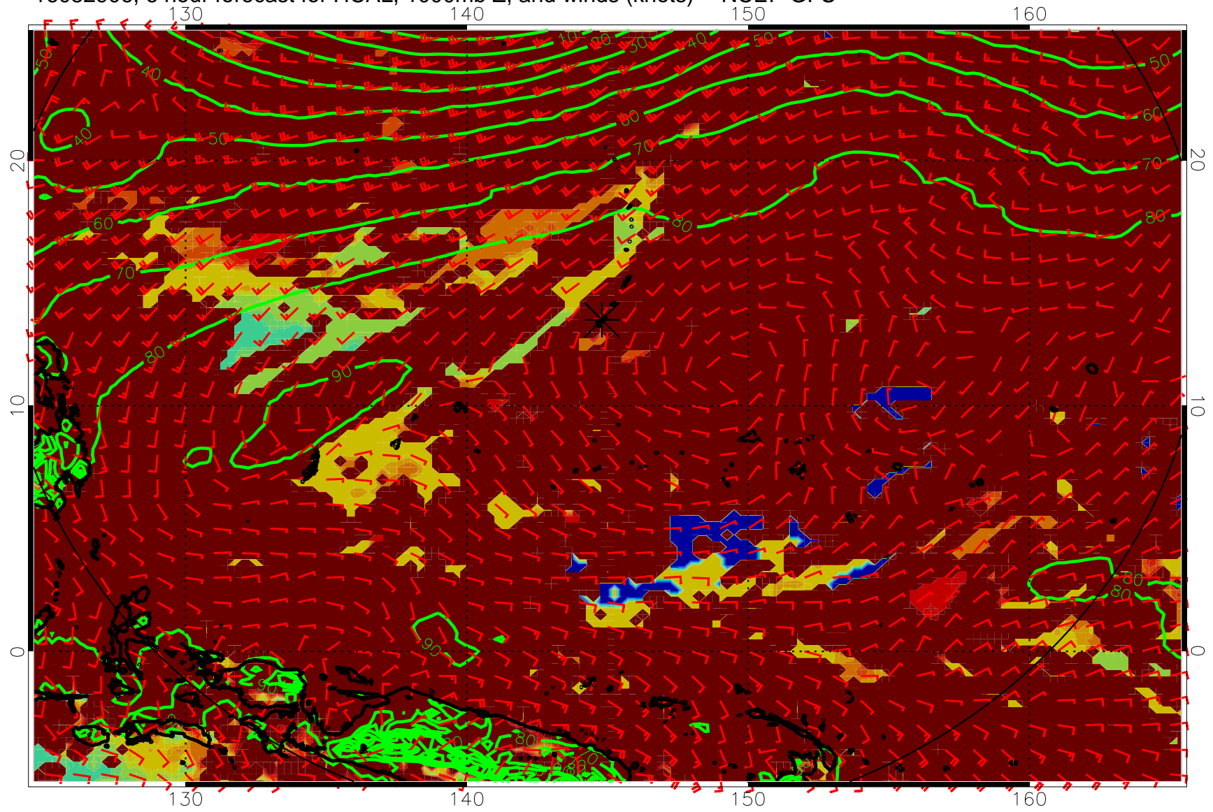
16082906, 6 hour forecast for HCAL, 1000mb Z, and winds (knots) -- NCEP GFS
