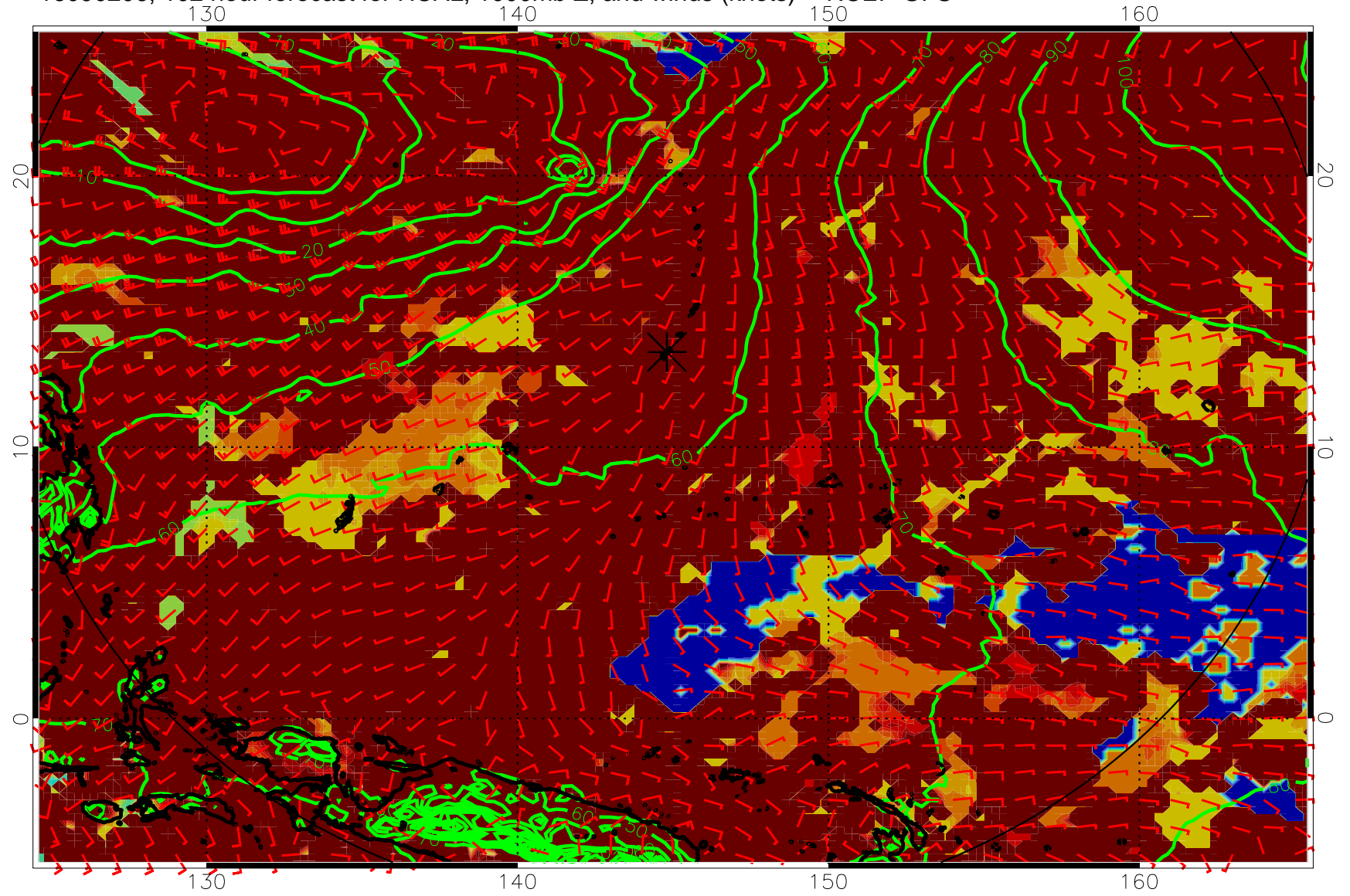
16090206, 102 hour forecast for HCAL, 1000mb Z, and winds (knots) -- NCEP GFS
