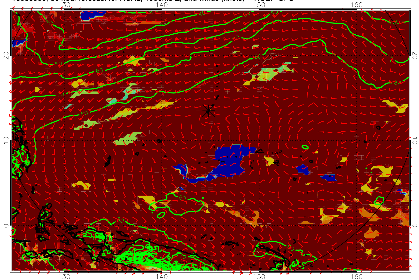
16083006, 30 hour forecast for HCAL, 1000mb Z, and winds (knots) -- NCEP GFS
