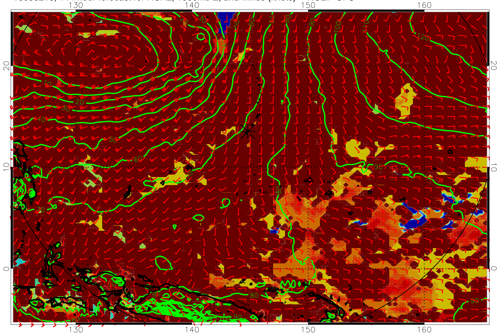
16090218, 114 hour forecast for HCAL, 1000mb Z, and winds (knots) -- NCEP GFS
