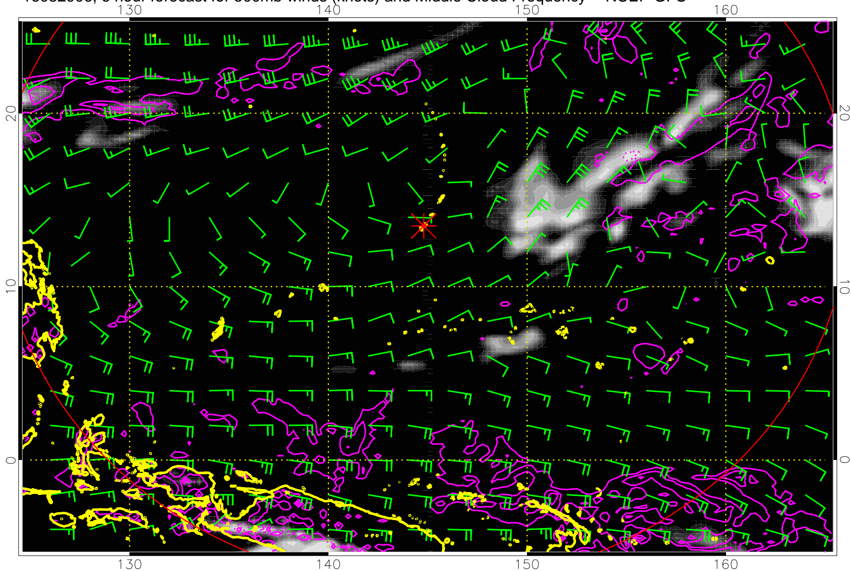
16082906, 6 hour forecast for 500mb winds (knots) and Middle Cloud Frequency -- NCEP GFS
