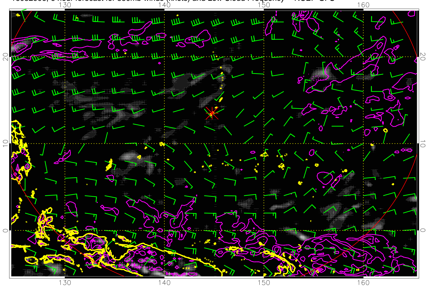
16082906, 6 hour forecast for 850mb winds (knots) and Low Cloud Frequency -- NCEP GFS
