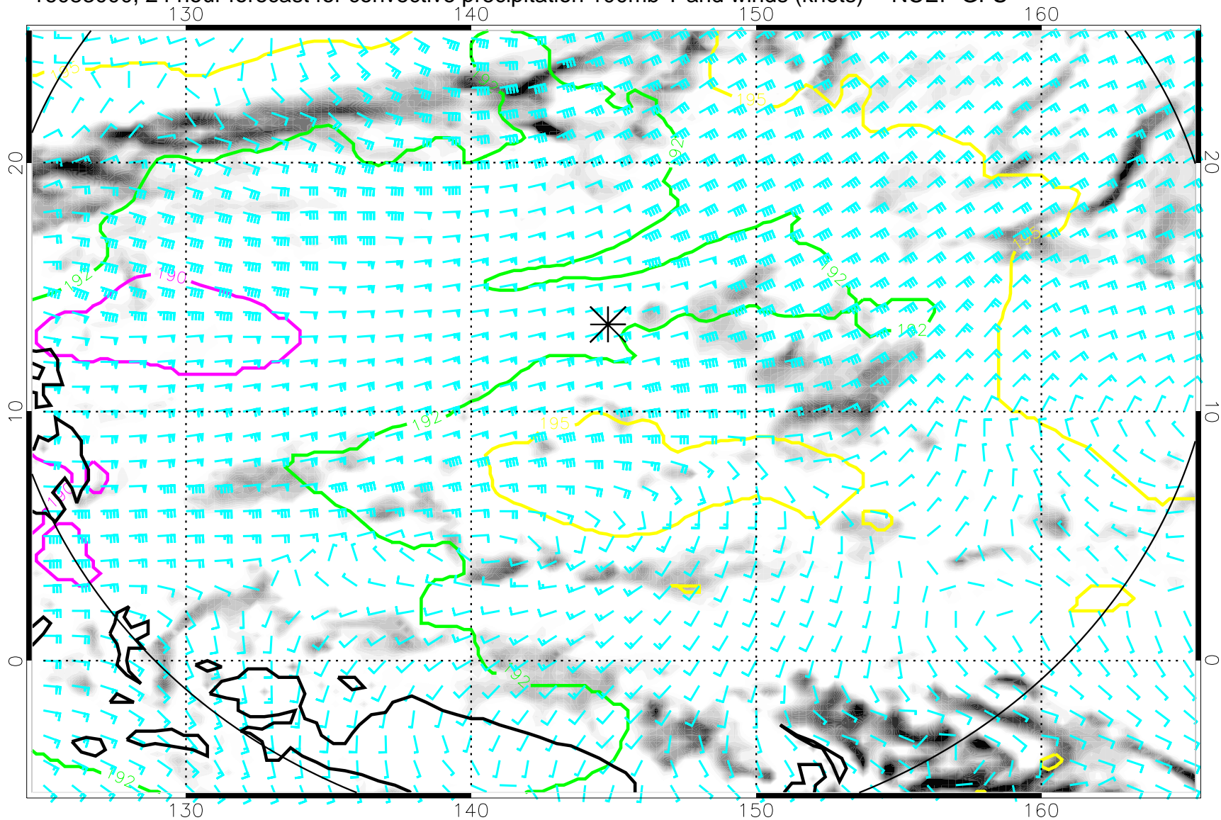
16083000, 24 hour forecast for convective precipitation 100mb T and winds (knots) -- NCEP GFS
