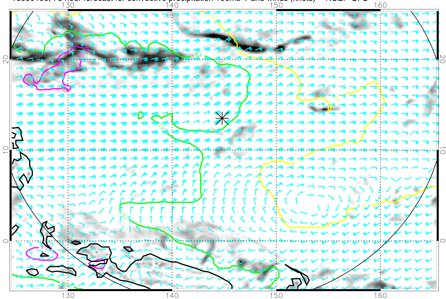
16090106, 78 hour forecast for convective precipitation 100mb T and winds (knots) -- NCEP GFS
