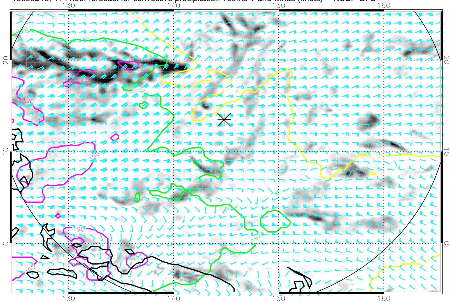
16090218, 114 hour forecast for convective precipitation 100mb T and winds (knots) -- NCEP GFS
