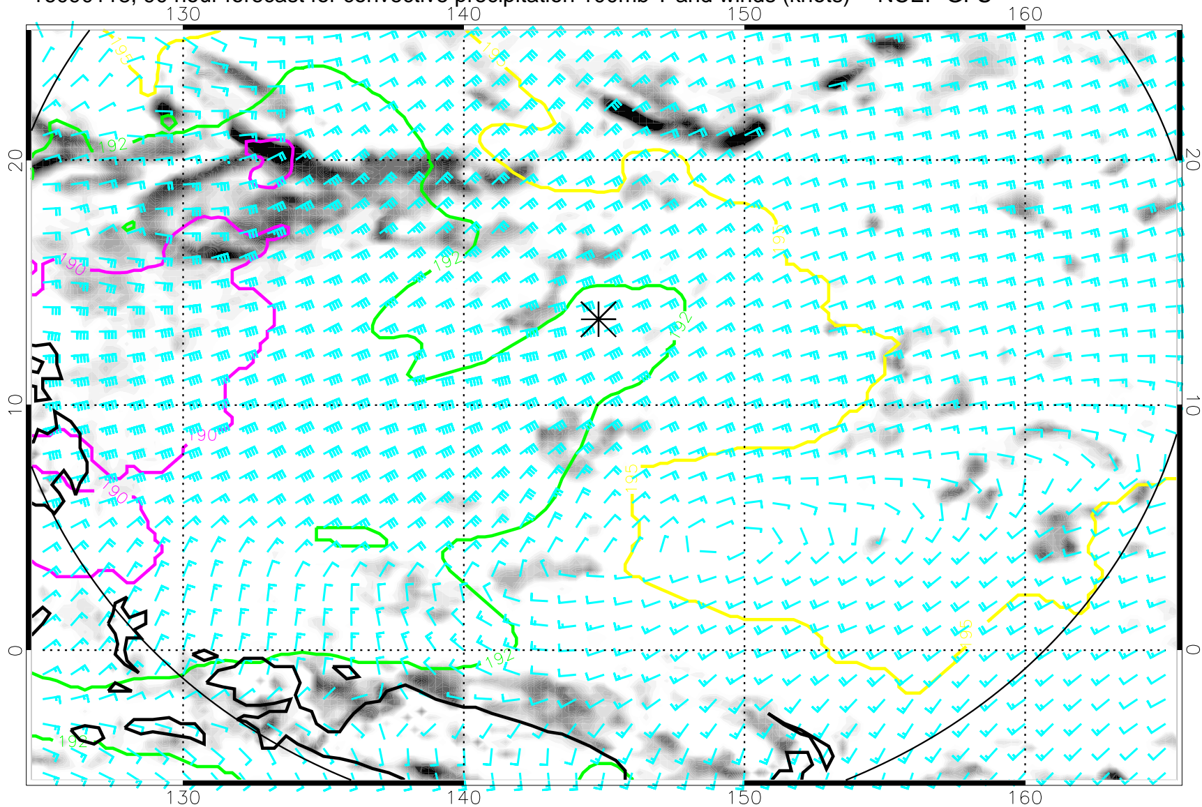
16090118, 90 hour forecast for convective precipitation 100mb T and winds (knots) -- NCEP GFS
