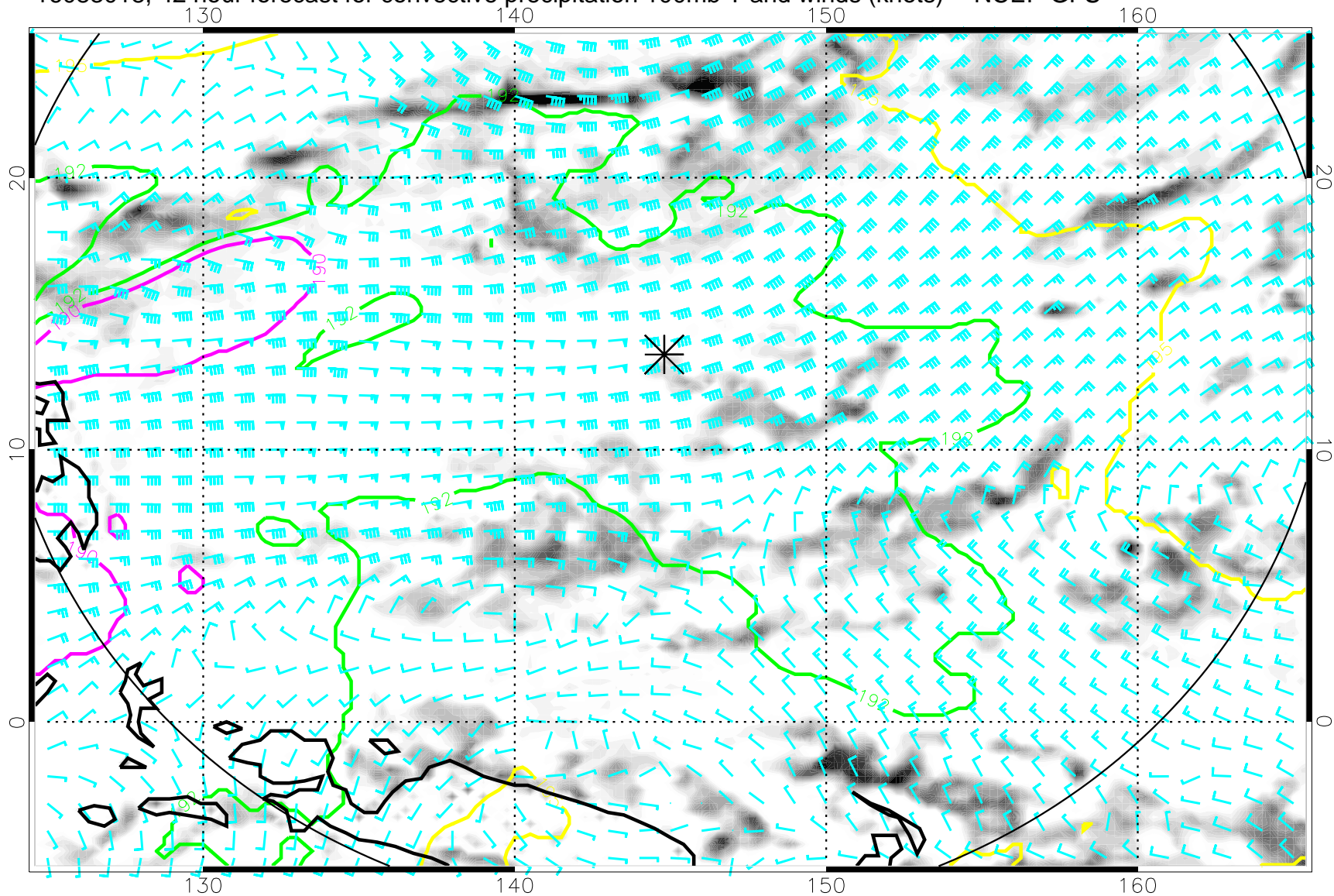
16083018, 42 hour forecast for convective precipitation 100mb T and winds (knots) -- NCEP GFS
