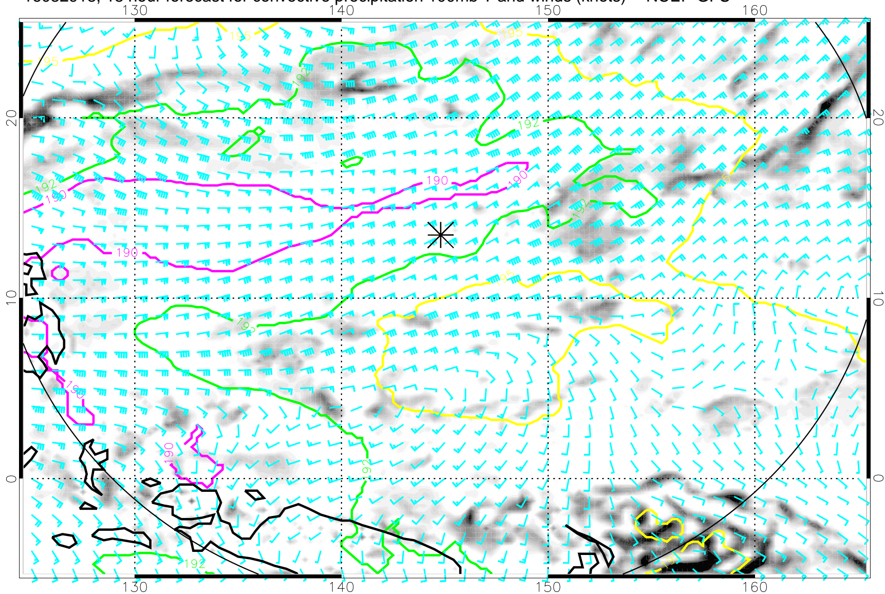
16082918, 18 hour forecast for convective precipitation 100mb T and winds (knots) -- NCEP GFS
