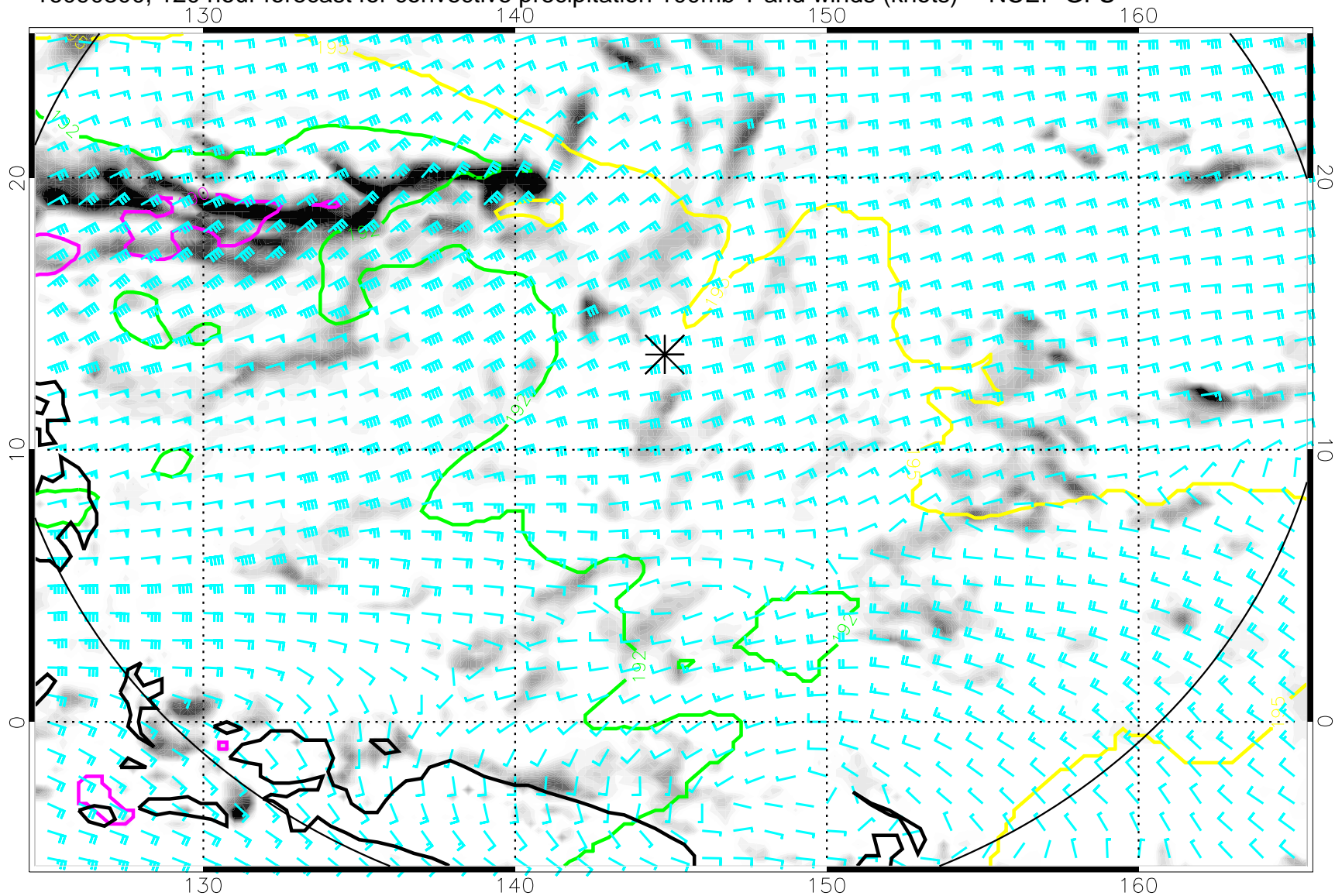
16090300, 120 hour forecast for convective precipitation 100mb T and winds (knots) -- NCEP GFS
