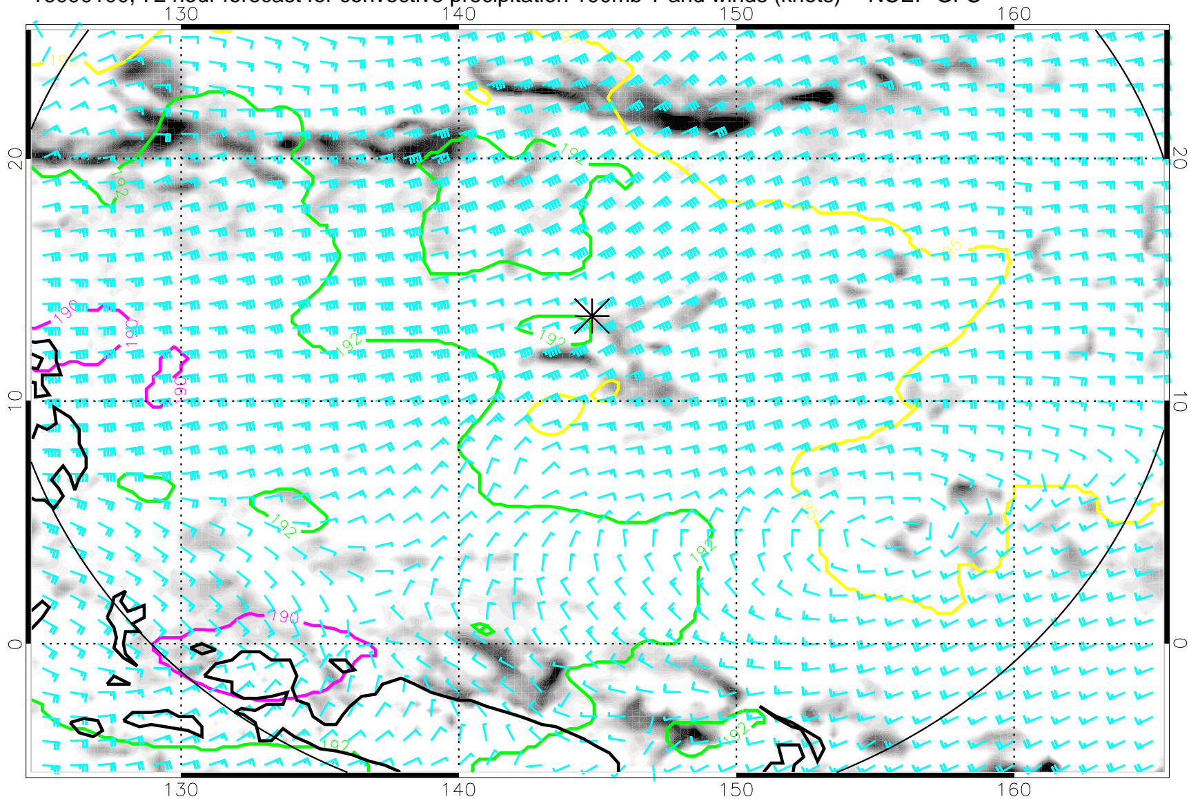
16090100, 72 hour forecast for convective precipitation 100mb T and winds (knots) -- NCEP GFS
