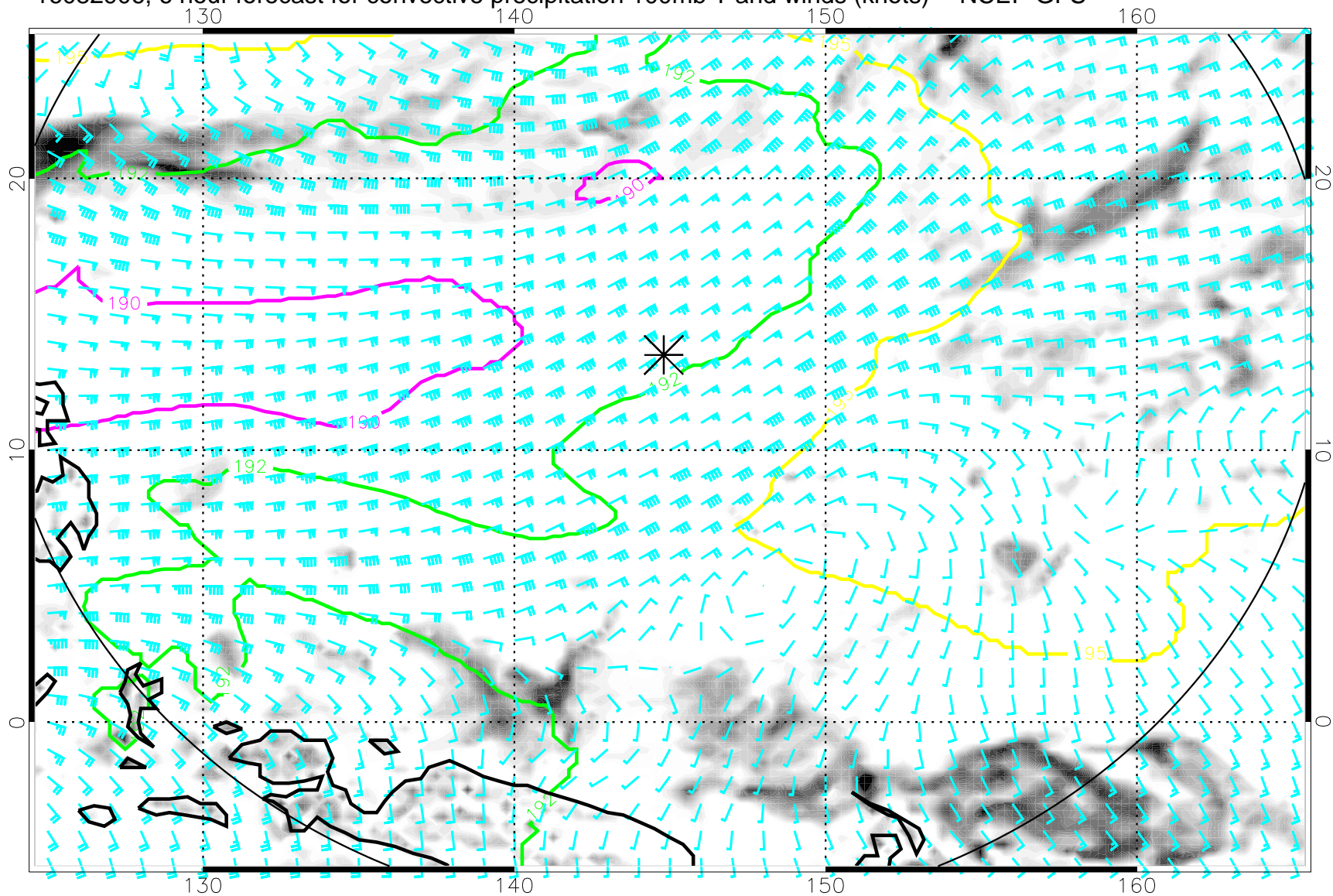
16082906, 6 hour forecast for convective precipitation 100mb T and winds (knots) -- NCEP GFS
