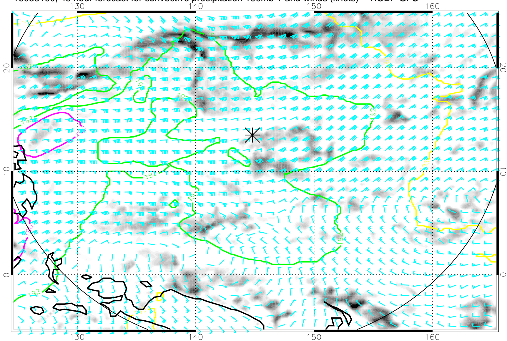
16083100, 48 hour forecast for convective precipitation 100mb T and winds (knots) -- NCEP GFS
