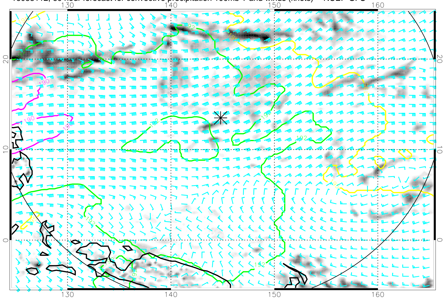
16083112, 60 hour forecast for convective precipitation 100mb T and winds (knots) -- NCEP GFS
