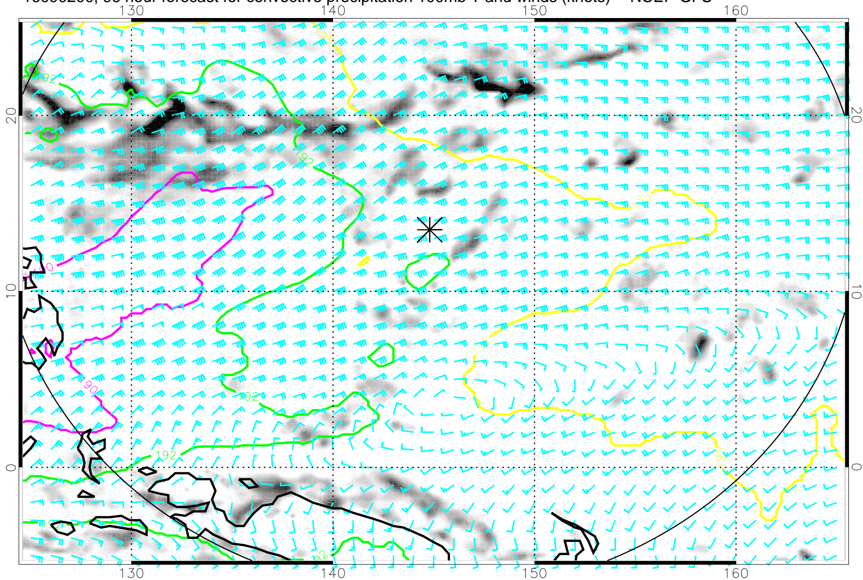
16090200, 96 hour forecast for convective precipitation 100mb T and winds (knots) -- NCEP GFS
