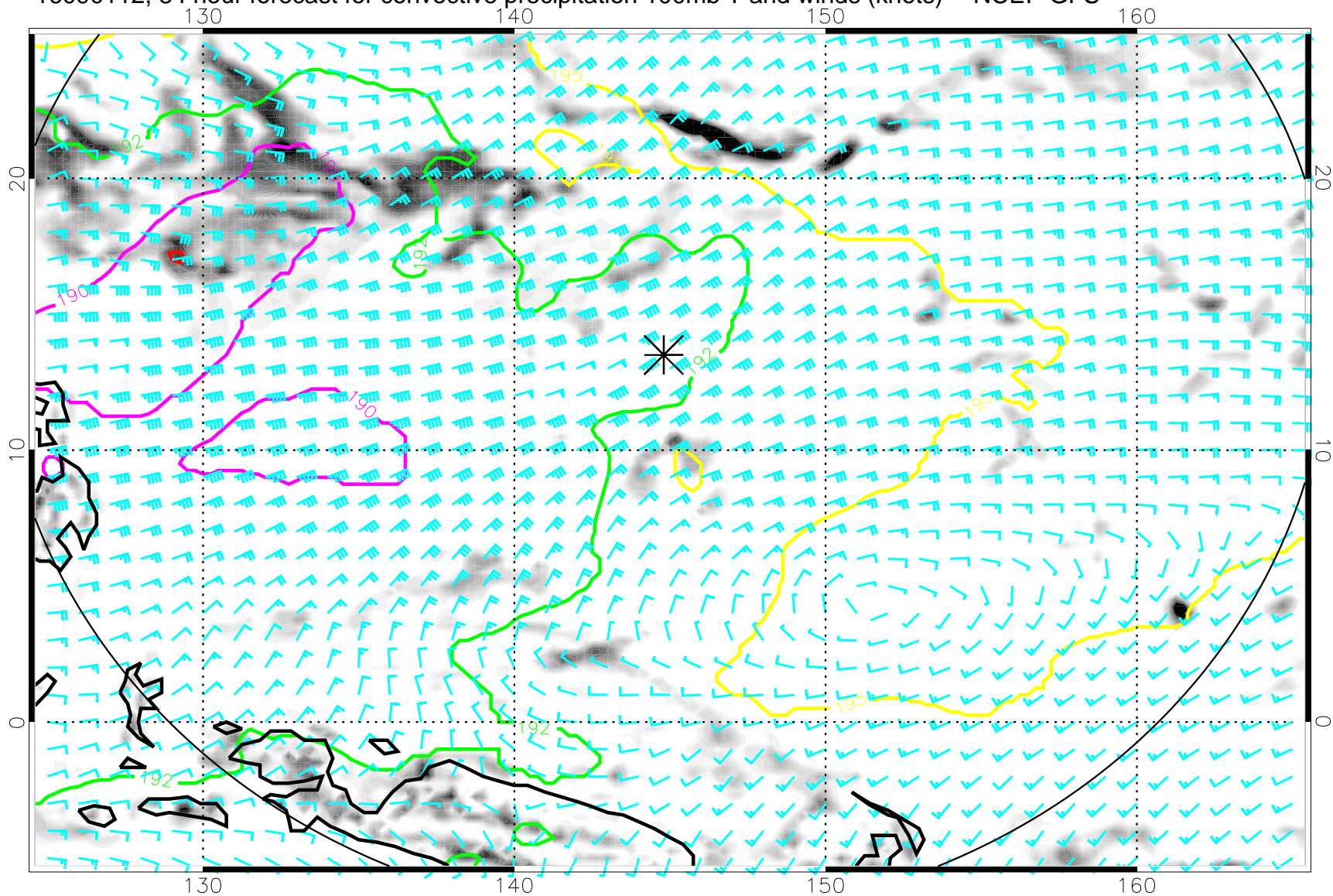
16090112, 84 hour forecast for convective precipitation 100mb T and winds (knots) -- NCEP GFS
