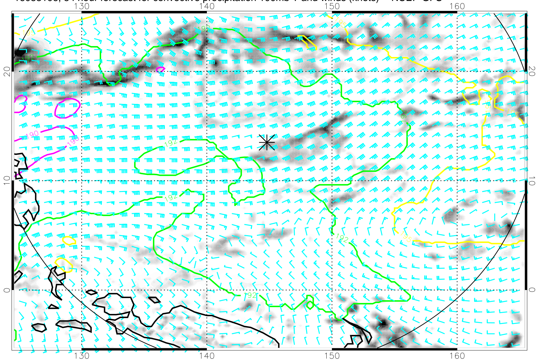
16083106, 54 hour forecast for convective precipitation 100mb T and winds (knots) -- NCEP GFS
