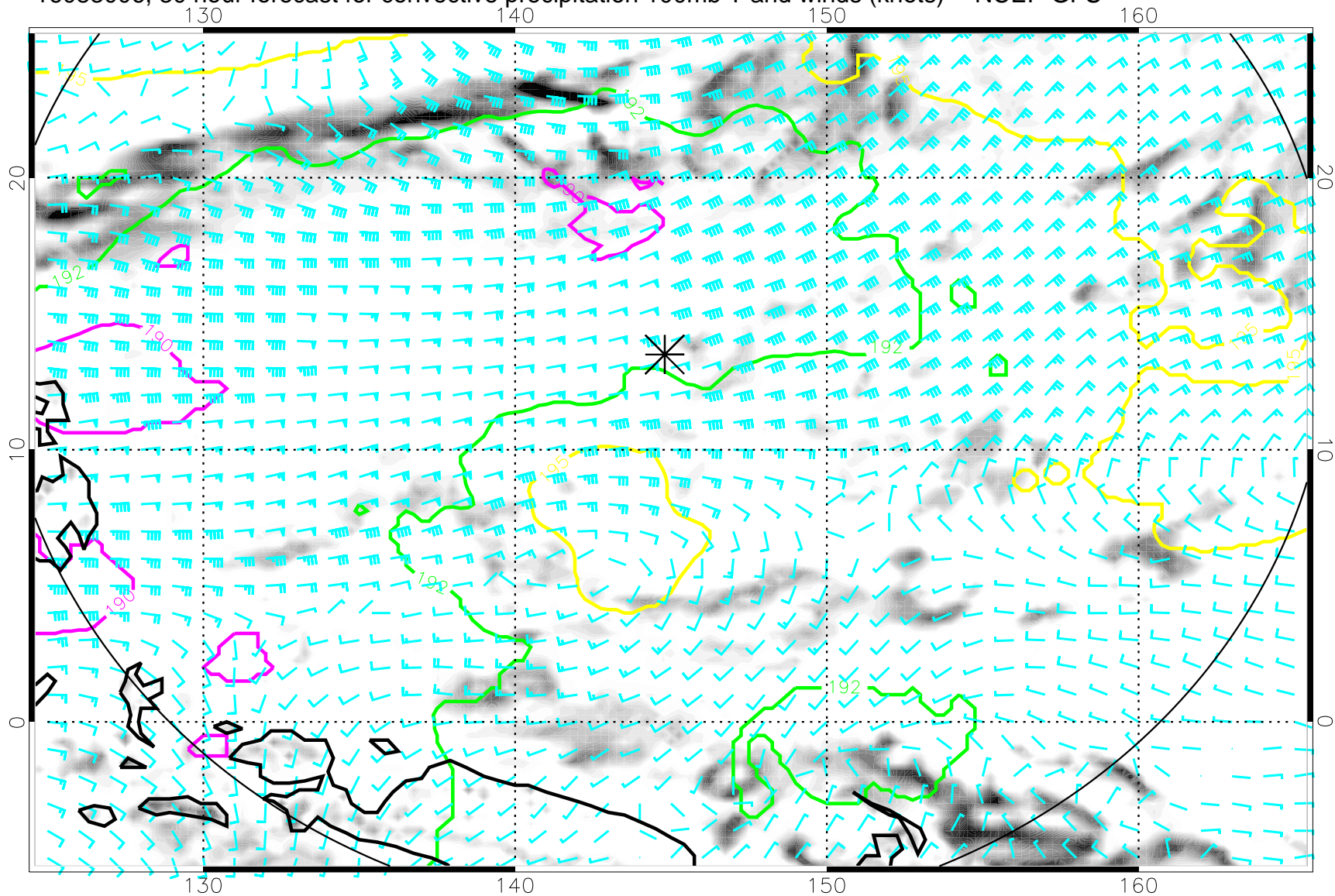
16083006, 30 hour forecast for convective precipitation 100mb T and winds (knots) -- NCEP GFS
