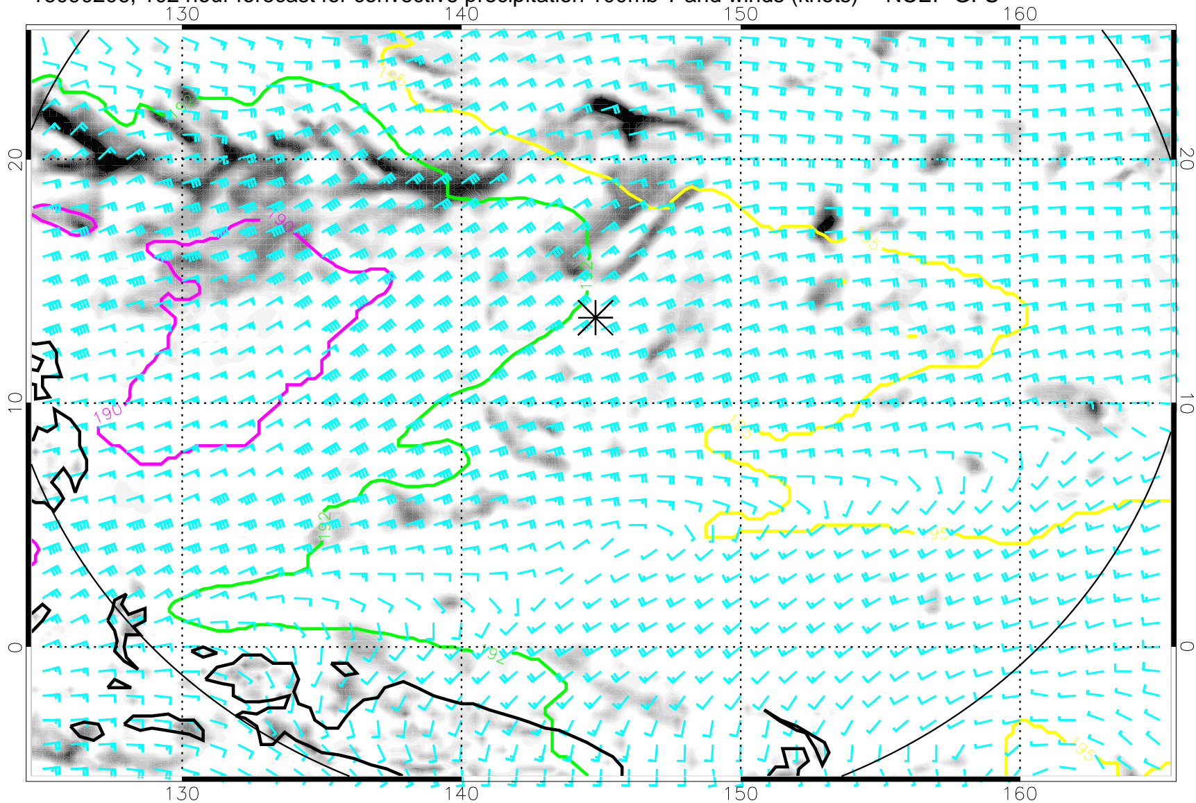
16090206, 102 hour forecast for convective precipitation 100mb T and winds (knots) -- NCEP GFS
