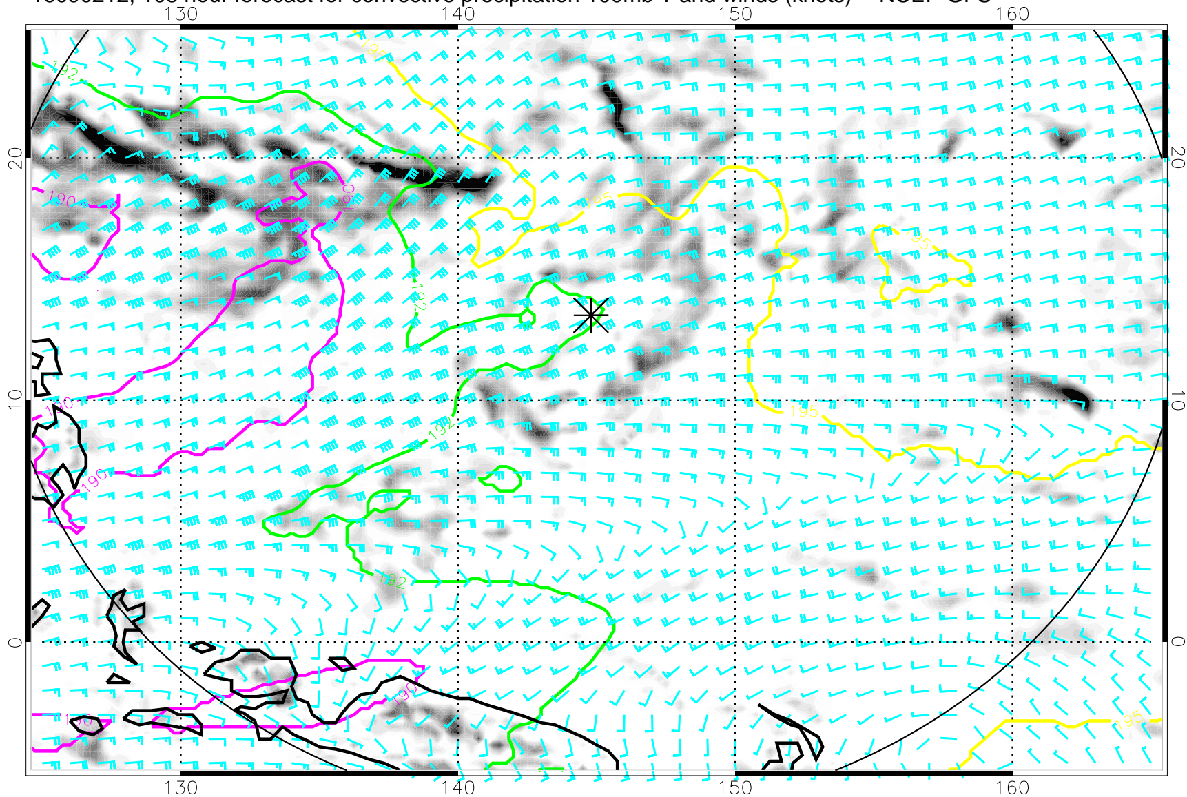
16090212, 108 hour forecast for convective precipitation 100mb T and winds (knots) -- NCEP GFS
