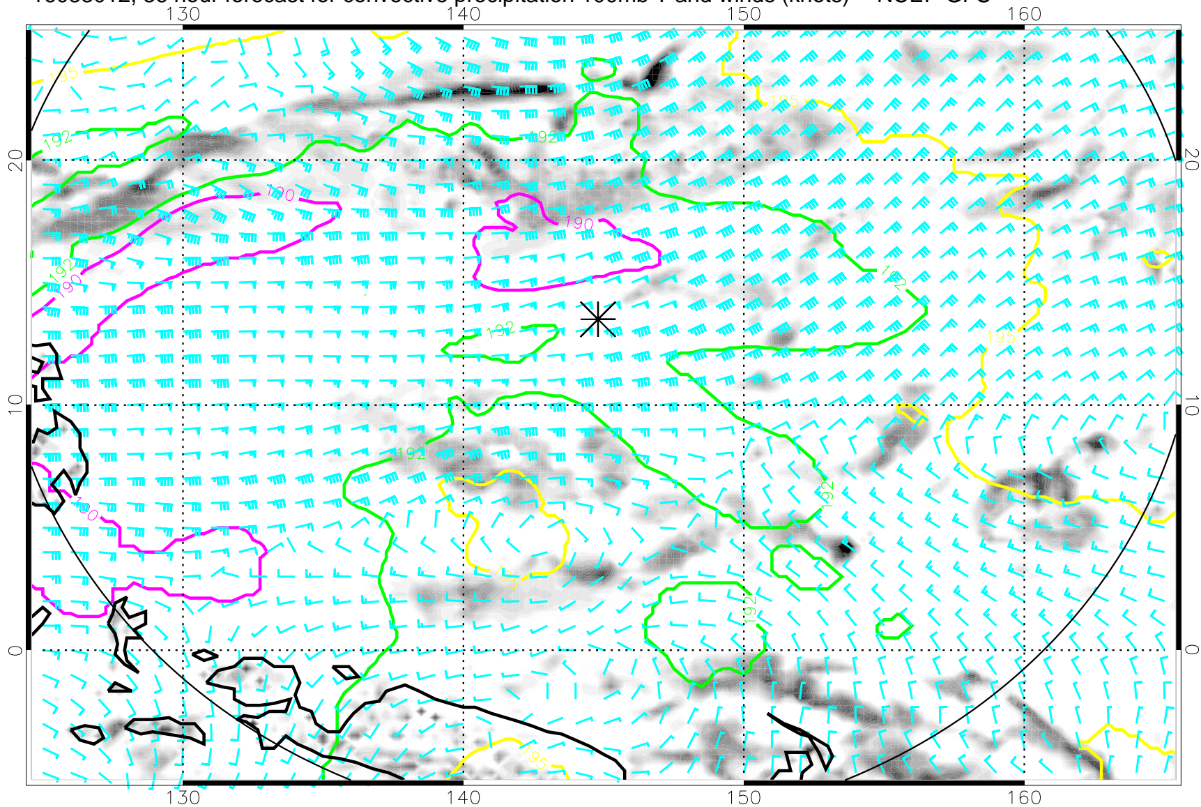
16083012, 36 hour forecast for convective precipitation 100mb T and winds (knots) -- NCEP GFS
