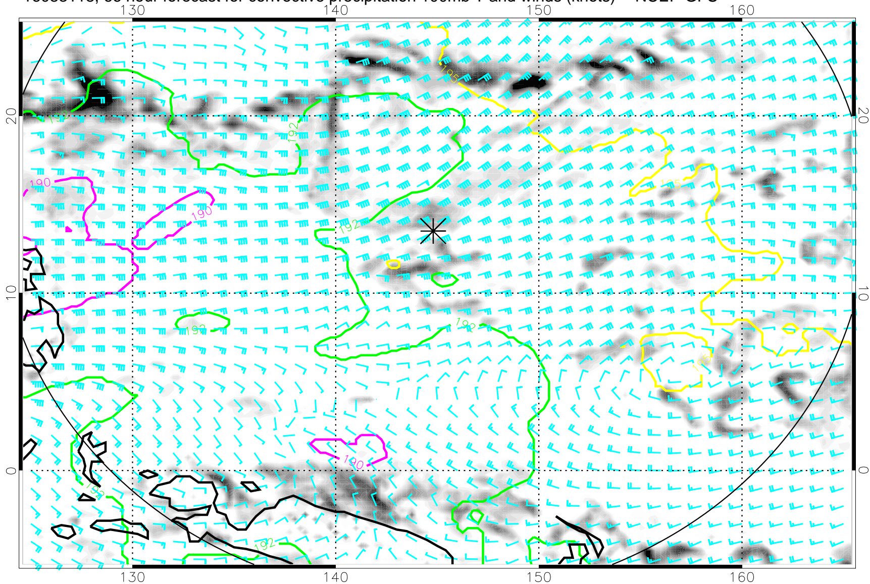
16083118, 66 hour forecast for convective precipitation 100mb T and winds (knots) -- NCEP GFS
