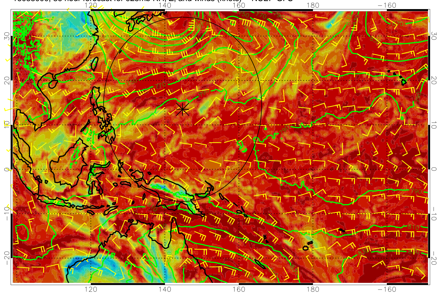
16083000, 36 hour forecast for 925mb RH, Z, and winds (knots) -- NCEP GFS
