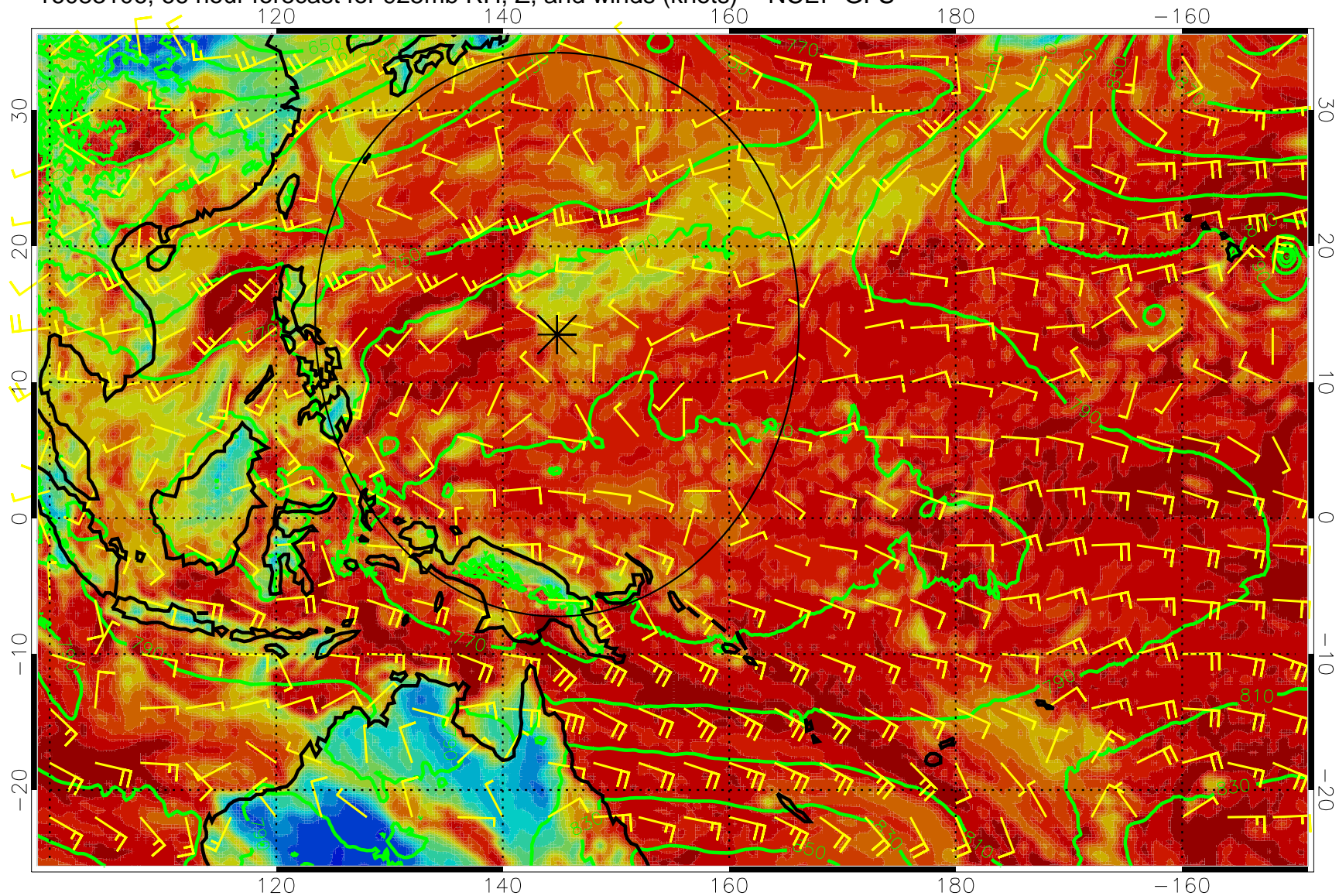
16083106, 66 hour forecast for 925mb RH, Z, and winds (knots) -- NCEP GFS
