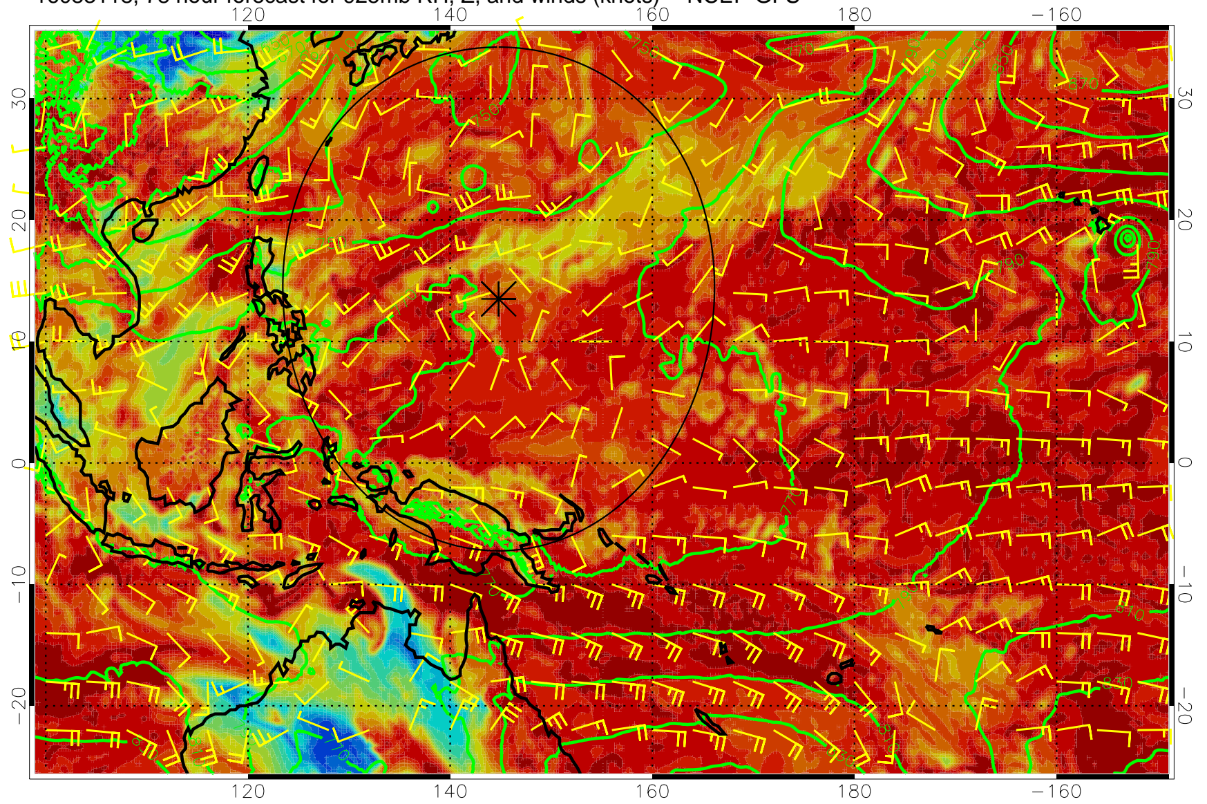
16083118, 78 hour forecast for 925mb RH, Z, and winds (knots) -- NCEP GFS
