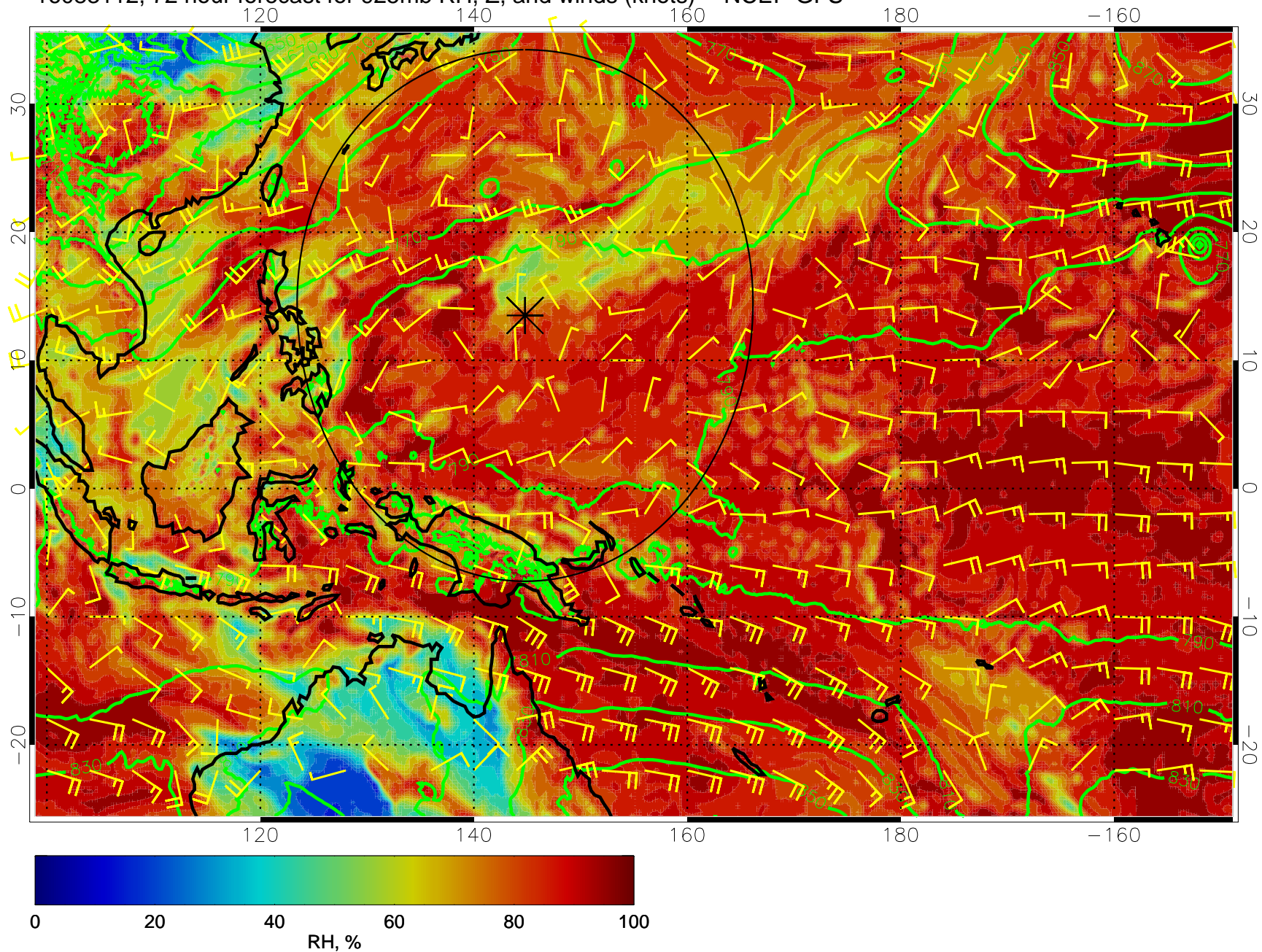
16083112, 72 hour forecast for 925mb RH, Z, and winds (knots) -- NCEP GFS
