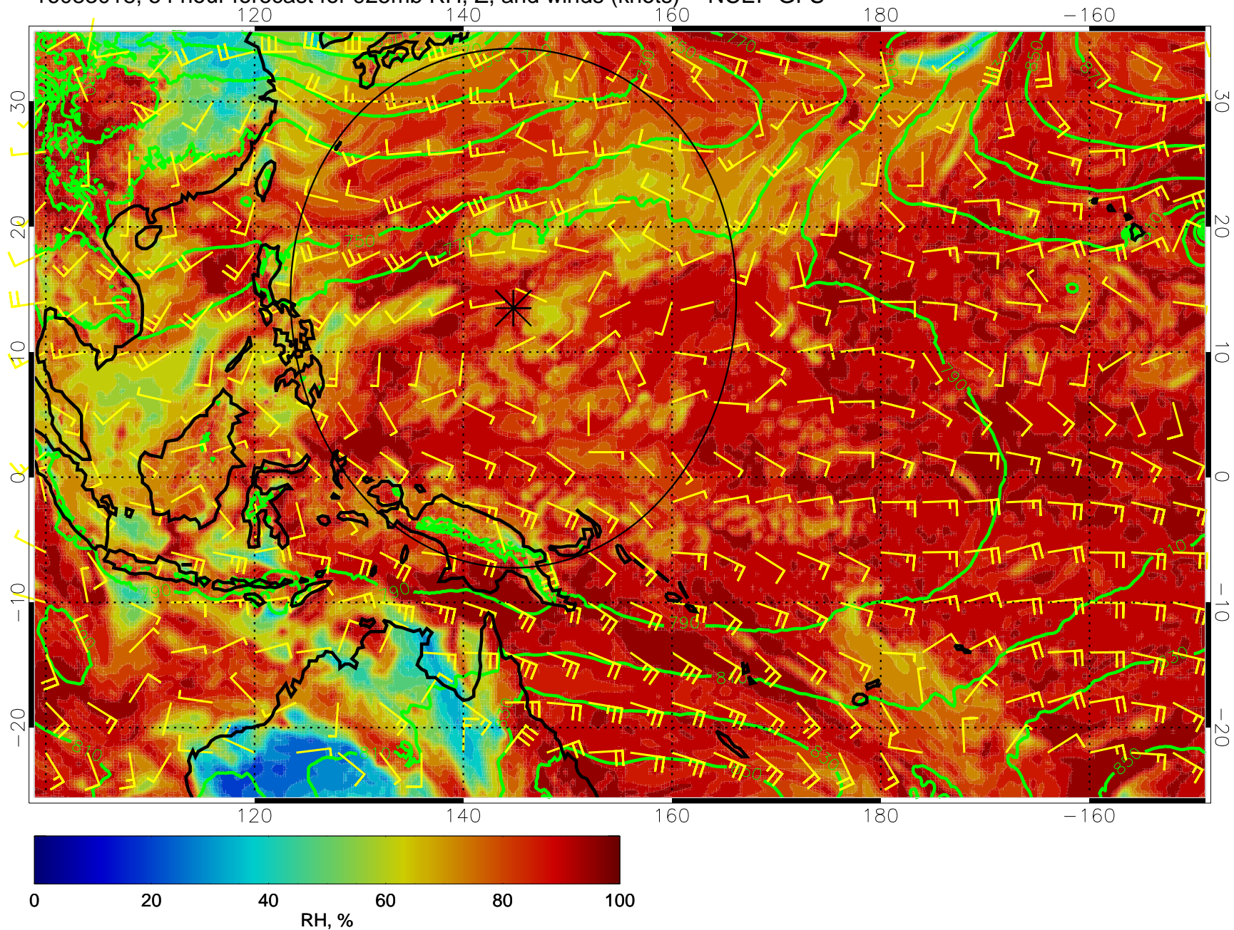
16083018, 54 hour forecast for 925mb RH, Z, and winds (knots) -- NCEP GFS
