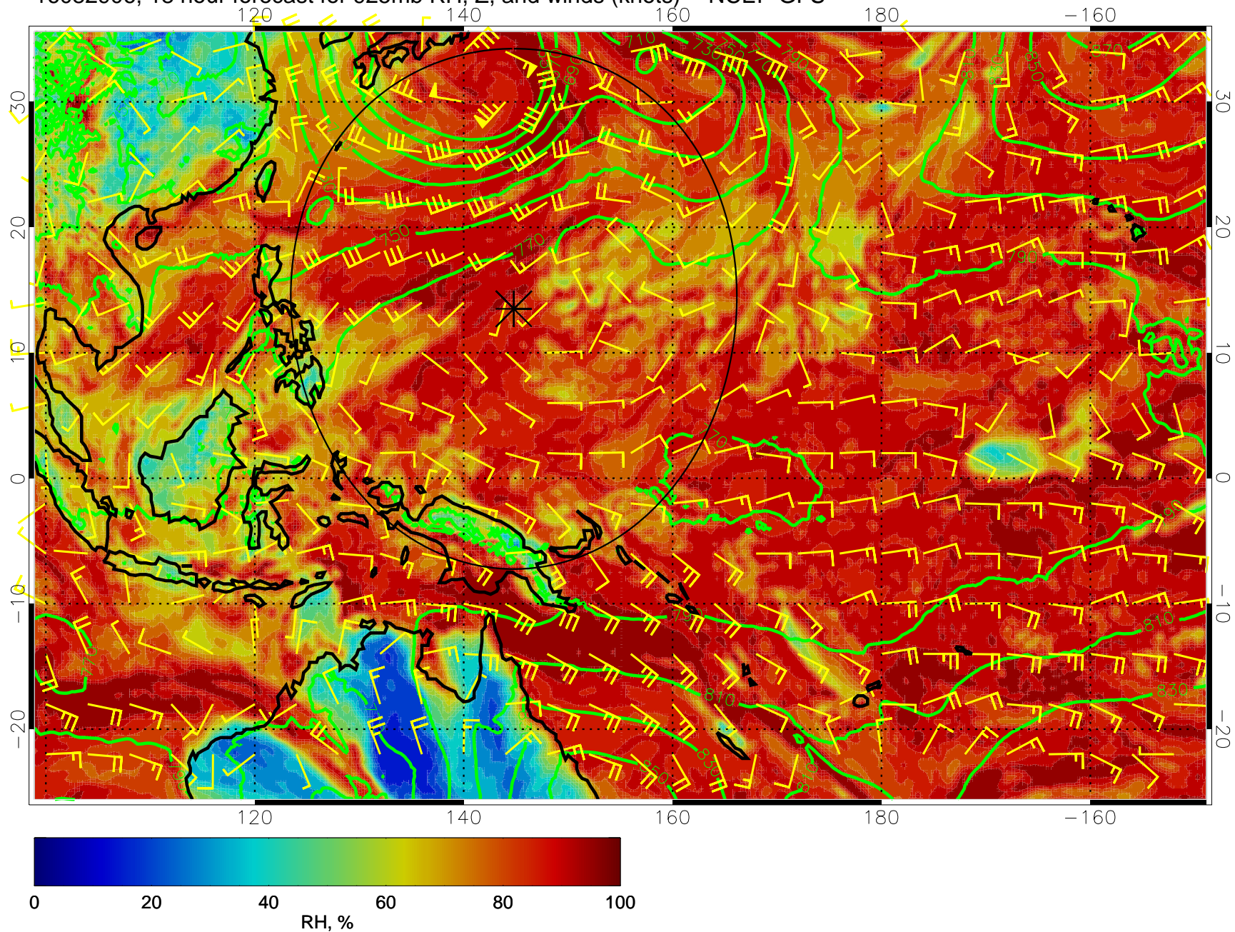
16082906, 18 hour forecast for 925mb RH, Z, and winds (knots) -- NCEP GFS
