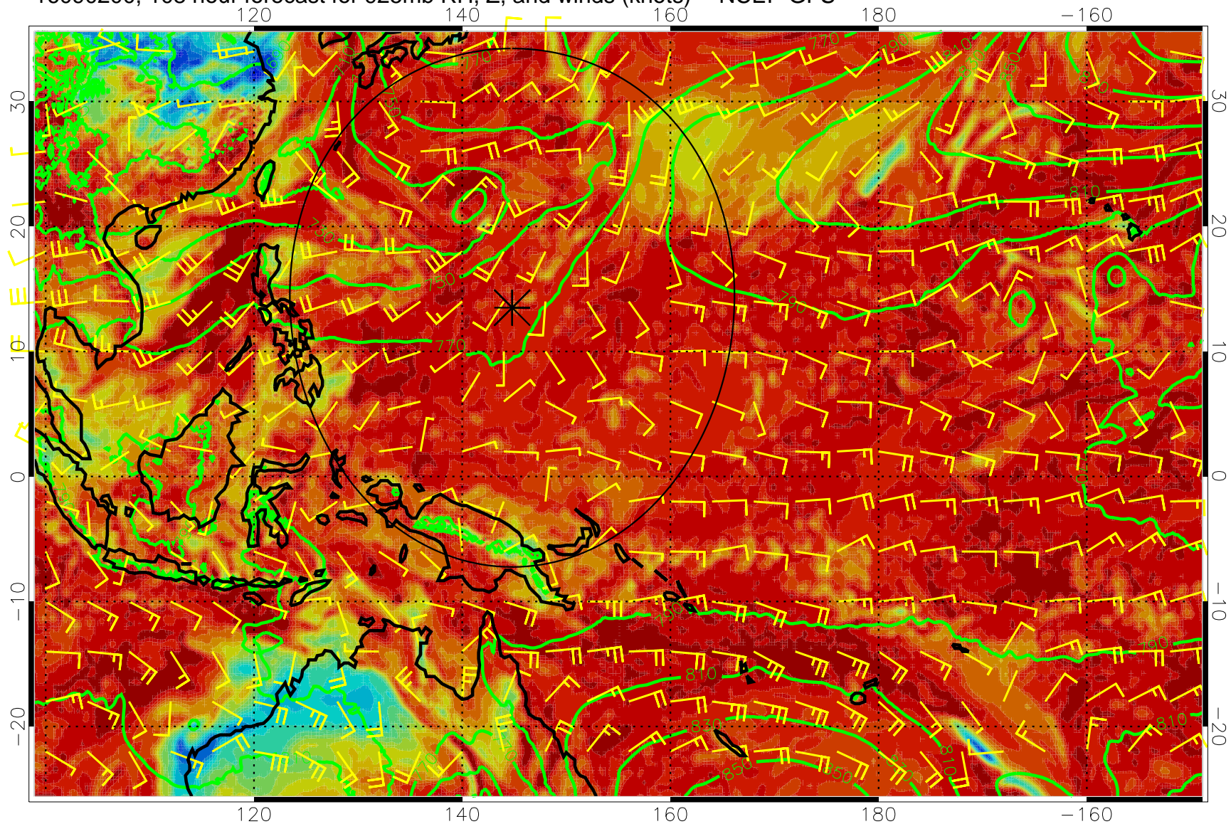
16090200, 108 hour forecast for 925mb RH, Z, and winds (knots) -- NCEP GFS
