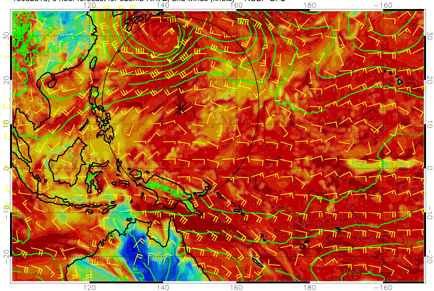
16082818, 6 hour forecast for 925mb RH, Z, and winds (knots) -- NCEP GFS
