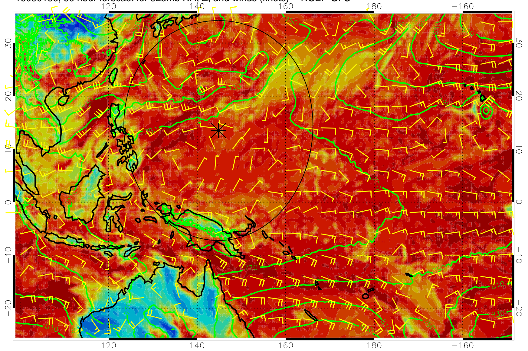
16090106, 90 hour forecast for 925mb RH, Z, and winds (knots) -- NCEP GFS
