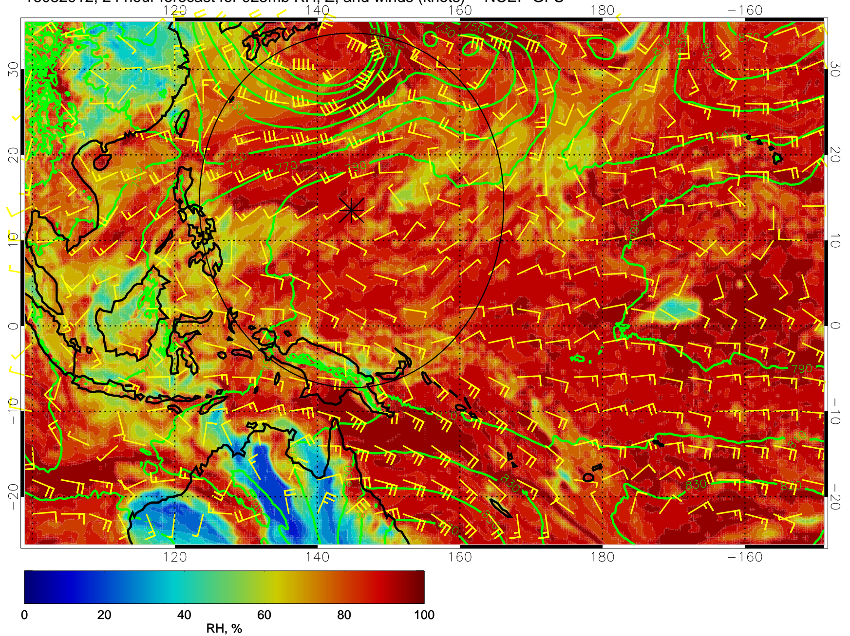
16082912, 24 hour forecast for 925mb RH, Z, and winds (knots) -- NCEP GFS
