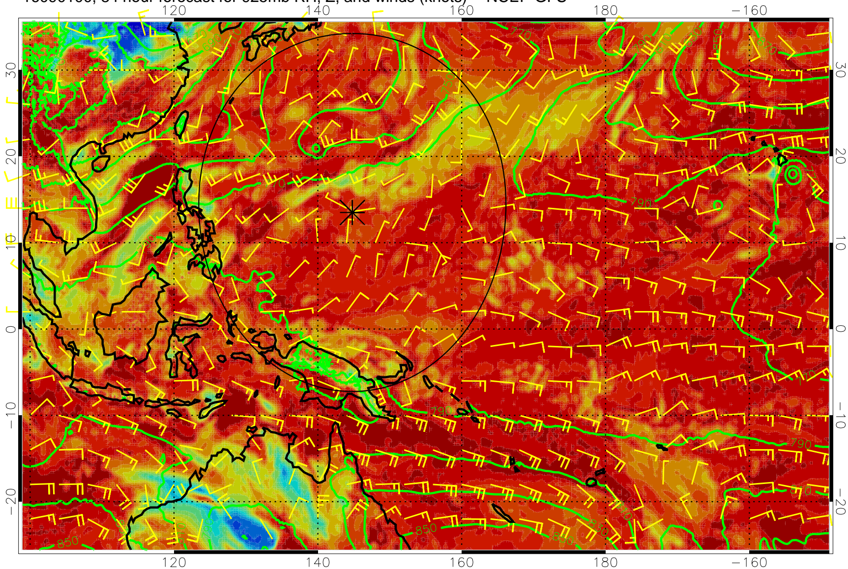
16090100, 84 hour forecast for 925mb RH, Z, and winds (knots) -- NCEP GFS
