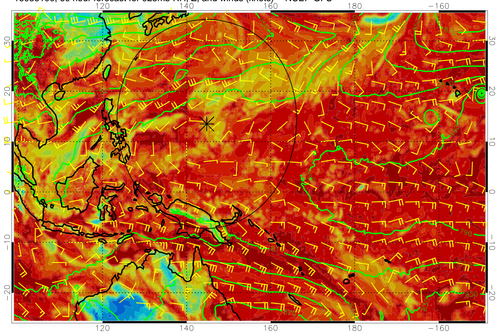
16083100, 60 hour forecast for 925mb RH, Z, and winds (knots) -- NCEP GFS
