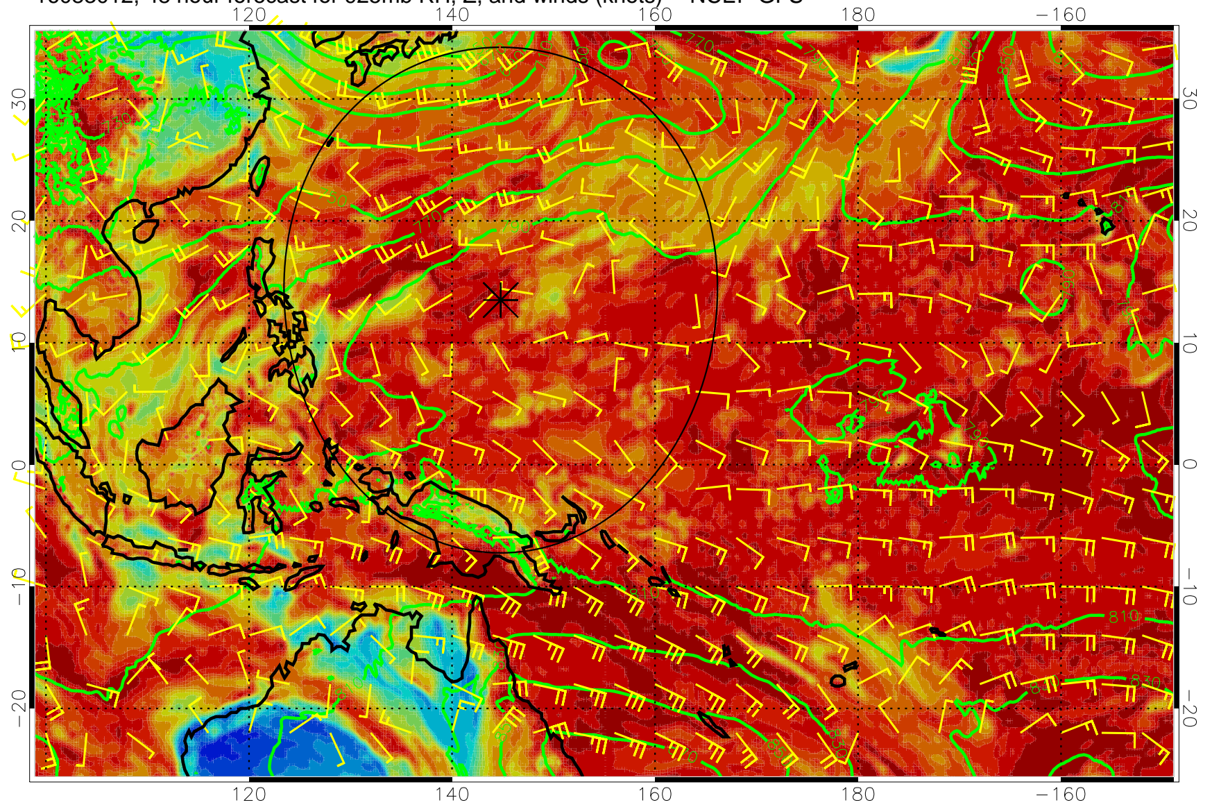
16083012, 48 hour forecast for 925mb RH, Z, and winds (knots) -- NCEP GFS
