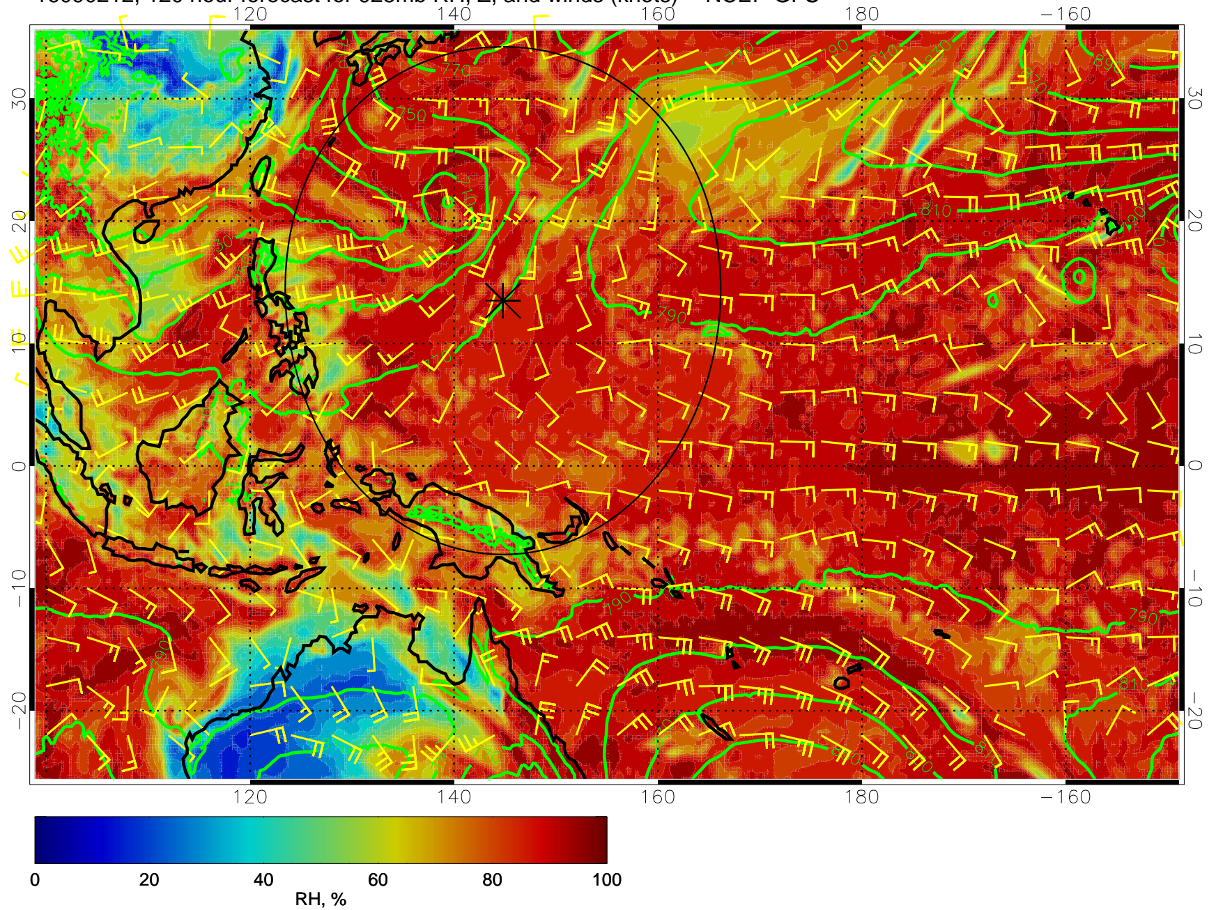
16090212, 120 hour forecast for 925mb RH, Z, and winds (knots) -- NCEP GFS
