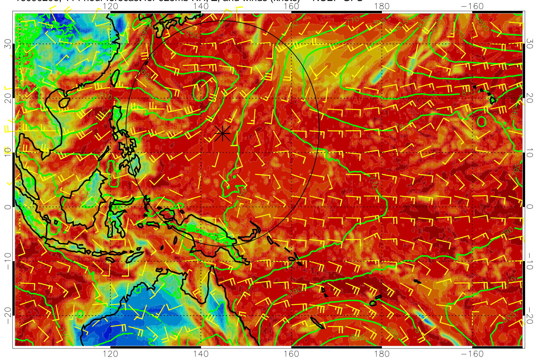
16090206, 114 hour forecast for 925mb RH, Z, and winds (knots) -- NCEP GFS
