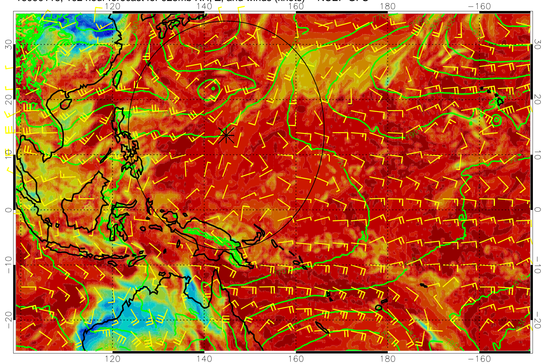
16090118, 102 hour forecast for 925mb RH, Z, and winds (knots) -- NCEP GFS
