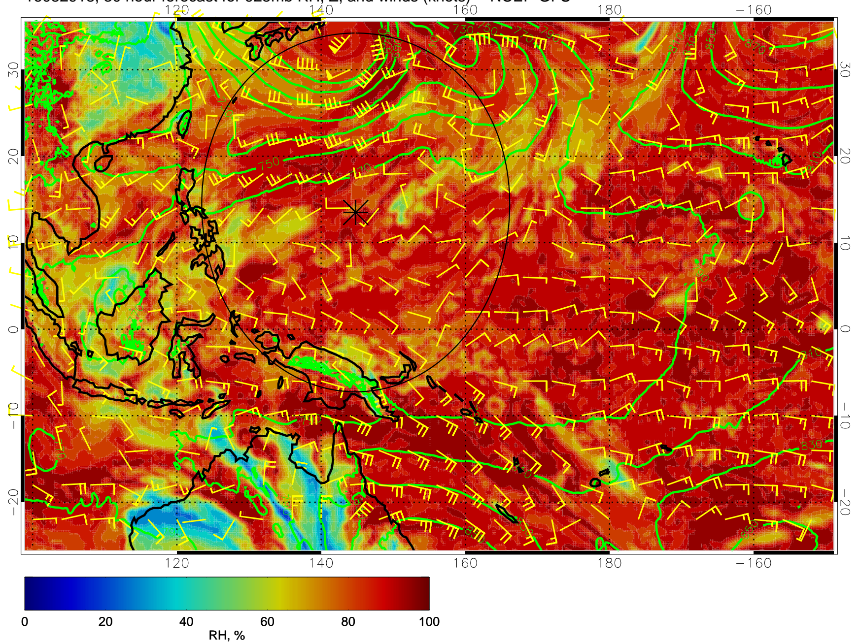
16082918, 30 hour forecast for 925mb RH, Z, and winds (knots) -- NCEP GFS
