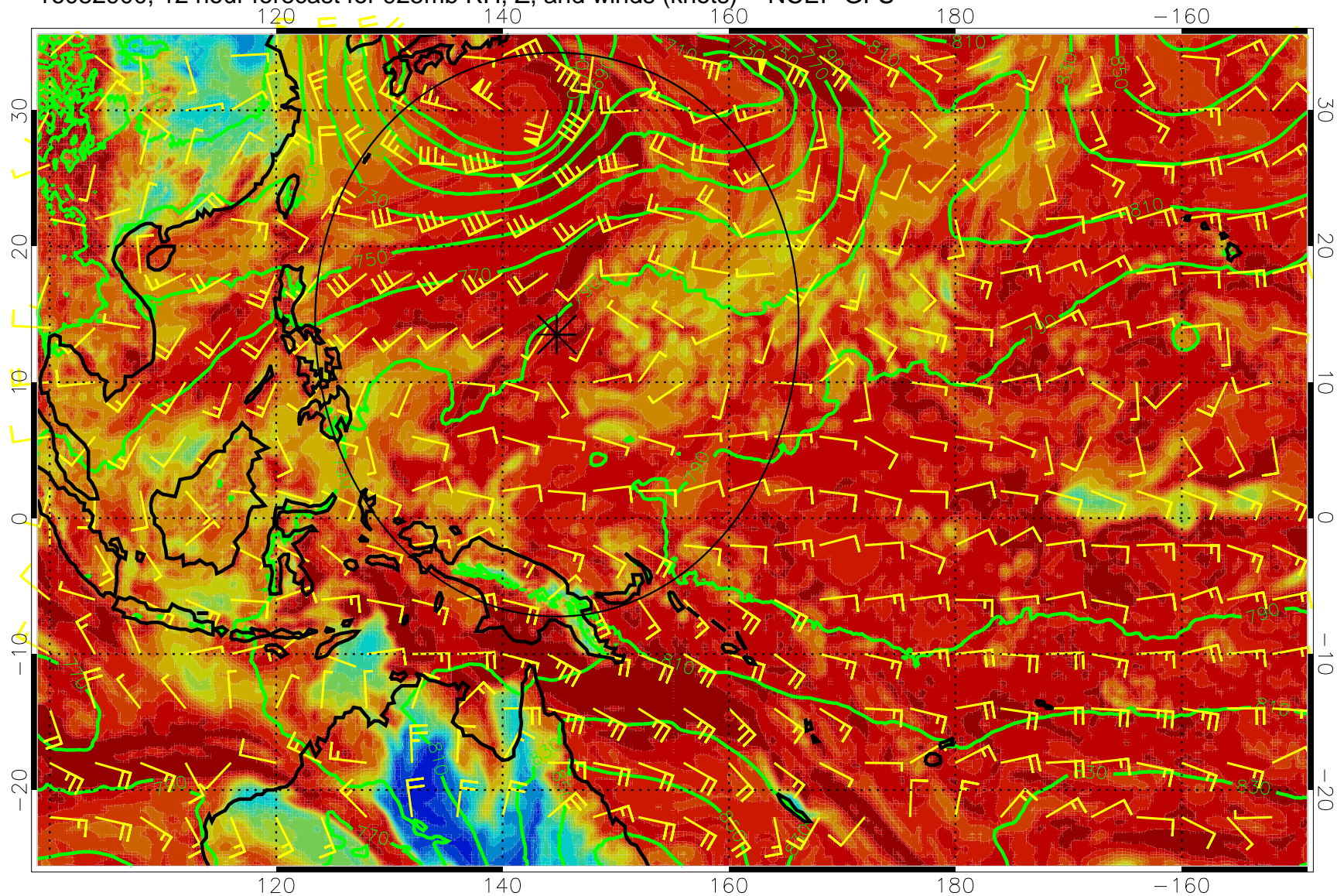
16082900, 12 hour forecast for 925mb RH, Z, and winds (knots) -- NCEP GFS
