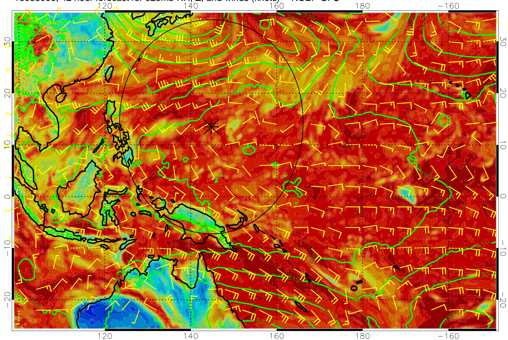
16083006, 42 hour forecast for 925mb RH, Z, and winds (knots) -- NCEP GFS
