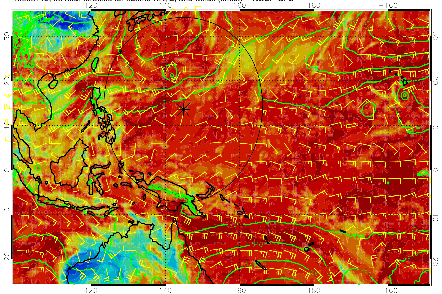
16090112, 96 hour forecast for 925mb RH, Z, and winds (knots) -- NCEP GFS
