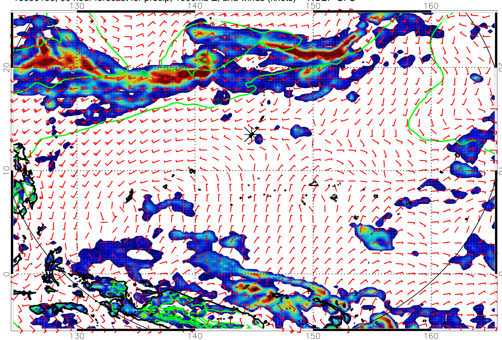
16090106, 90 hour forecast for precip, 1000mb Z, and winds (knots) -- NCEP GFS
