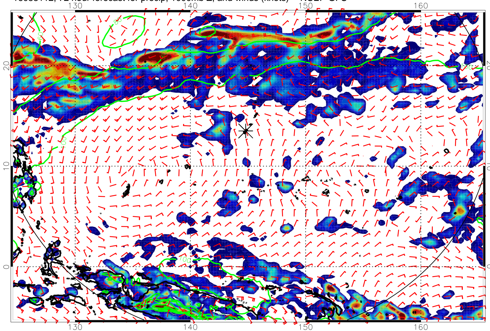
16083112, 72 hour forecast for precip, 1000mb Z, and winds (knots) -- NCEP GFS
