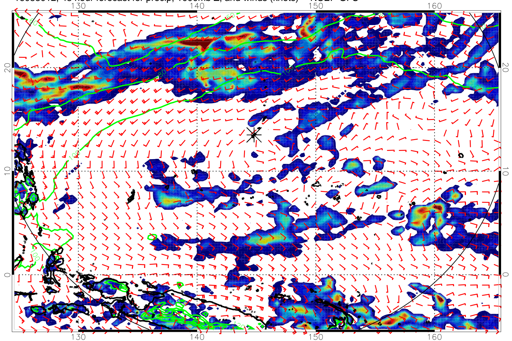
16083012, 48 hour forecast for precip, 1000mb Z, and winds (knots) -- NCEP GFS
