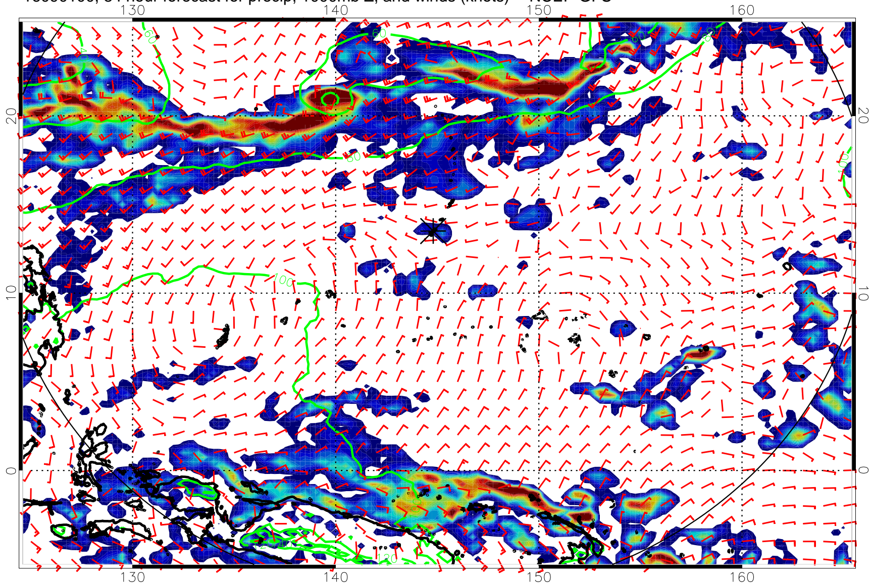
16090100, 84 hour forecast for precip, 1000mb Z, and winds (knots) -- NCEP GFS
