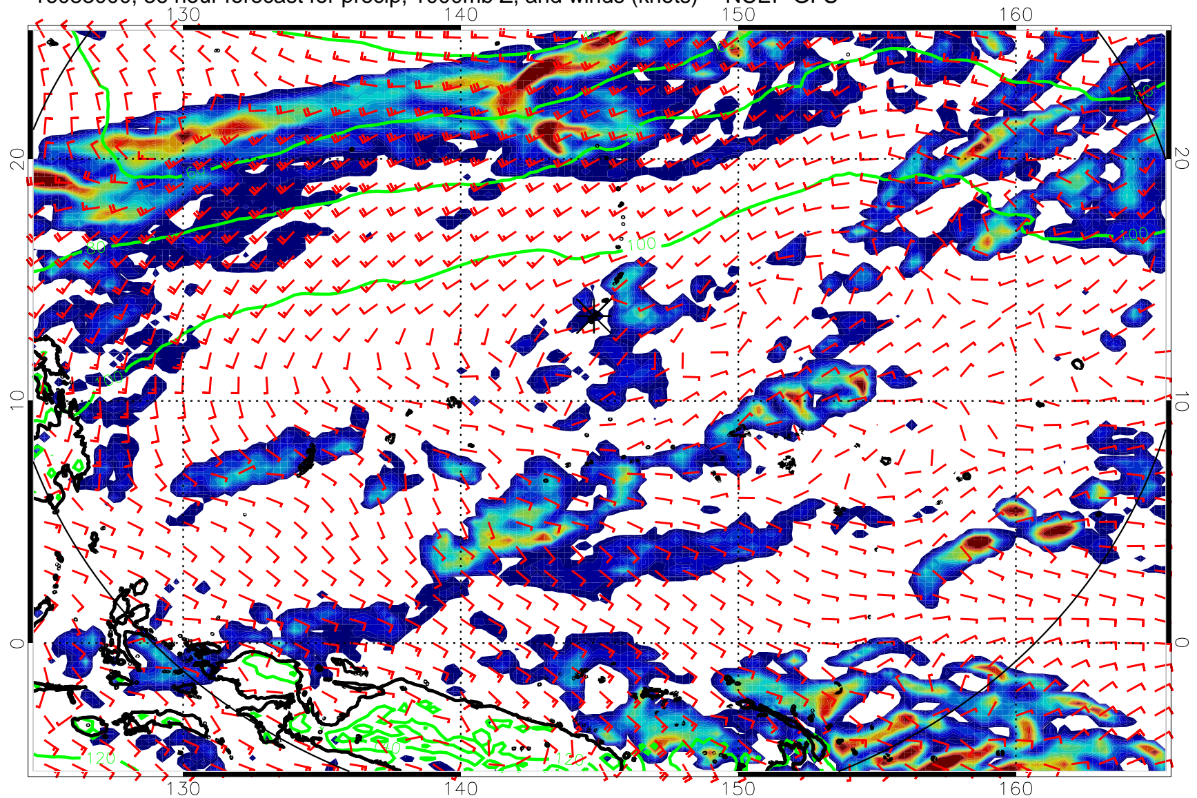
16083000, 36 hour forecast for precip, 1000mb Z, and winds (knots) -- NCEP GFS
