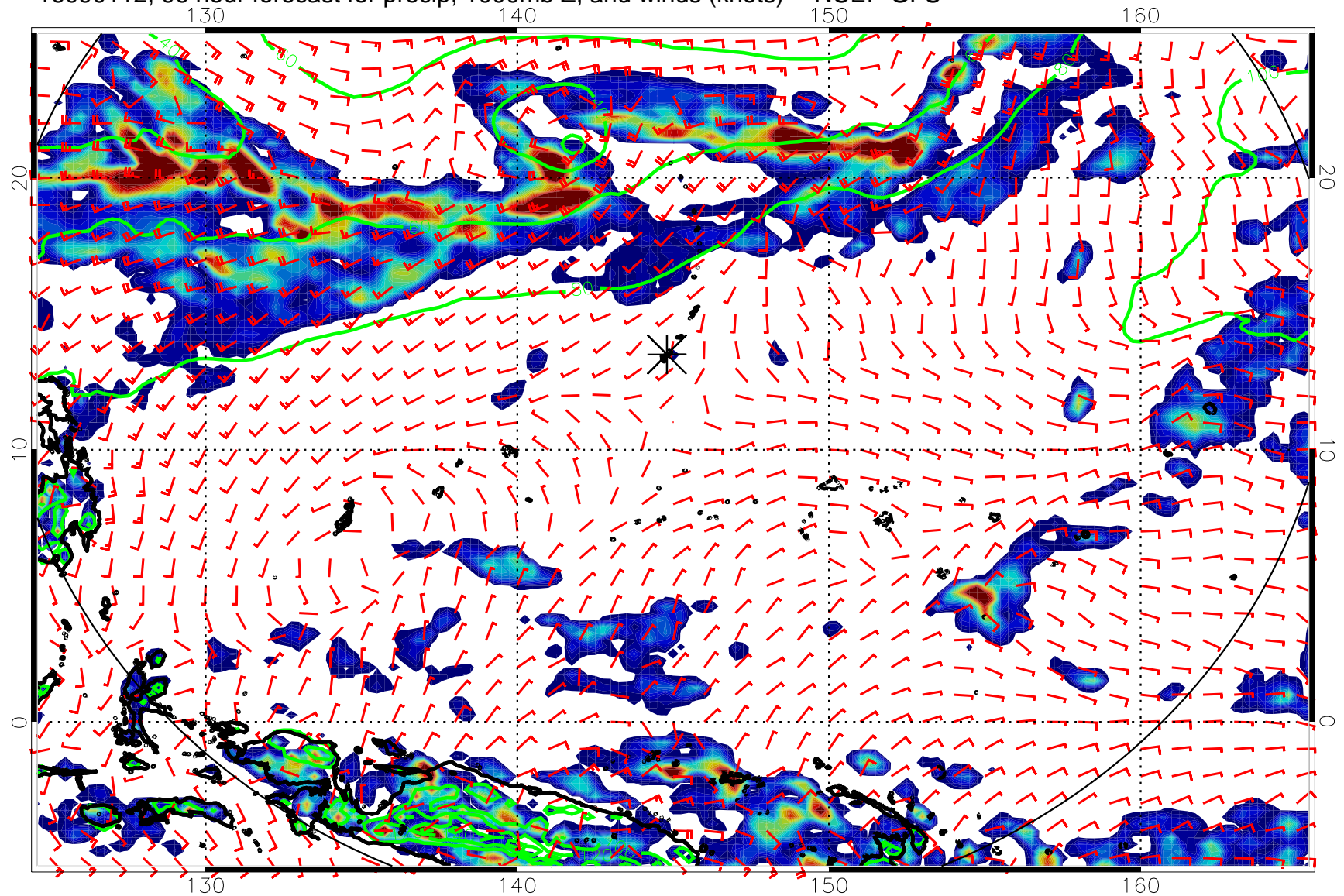
16090112, 96 hour forecast for precip, 1000mb Z, and winds (knots) -- NCEP GFS
