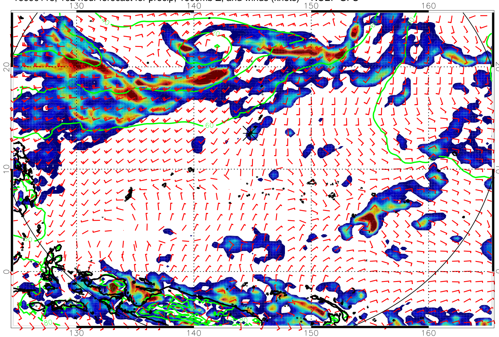
16090118, 102 hour forecast for precip, 1000mb Z, and winds (knots) -- NCEP GFS
