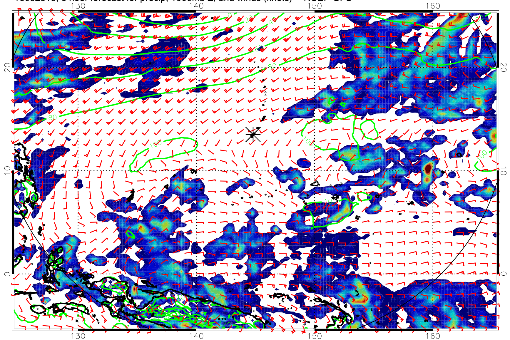
16082818, 6 hour forecast for precip, 1000mb Z, and winds (knots) -- NCEP GFS
