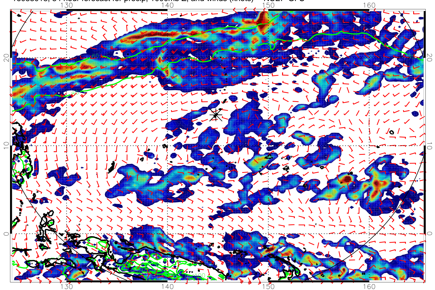
16083018, 54 hour forecast for precip, 1000mb Z, and winds (knots) -- NCEP GFS
