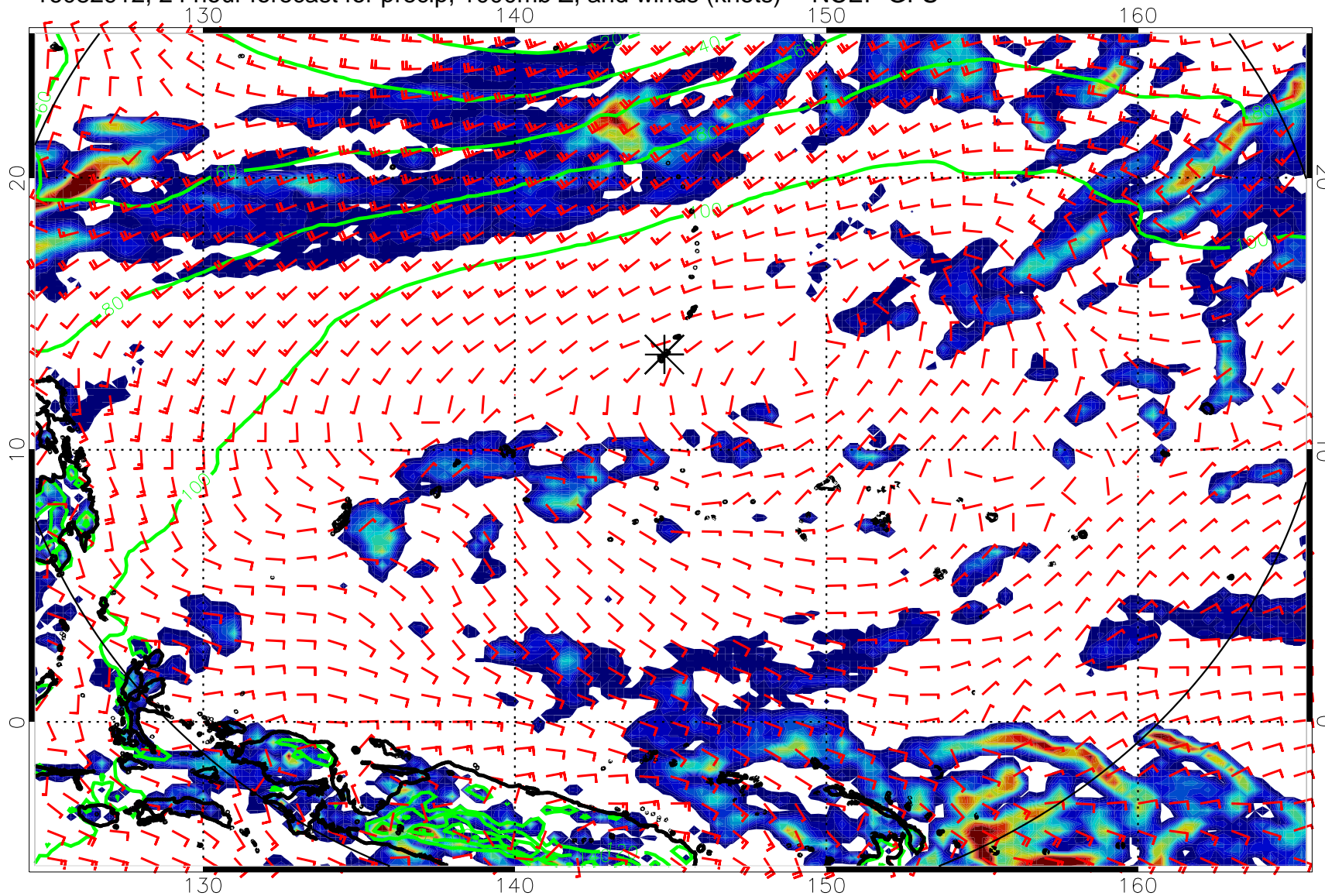
16082912, 24 hour forecast for precip, 1000mb Z, and winds (knots) -- NCEP GFS
