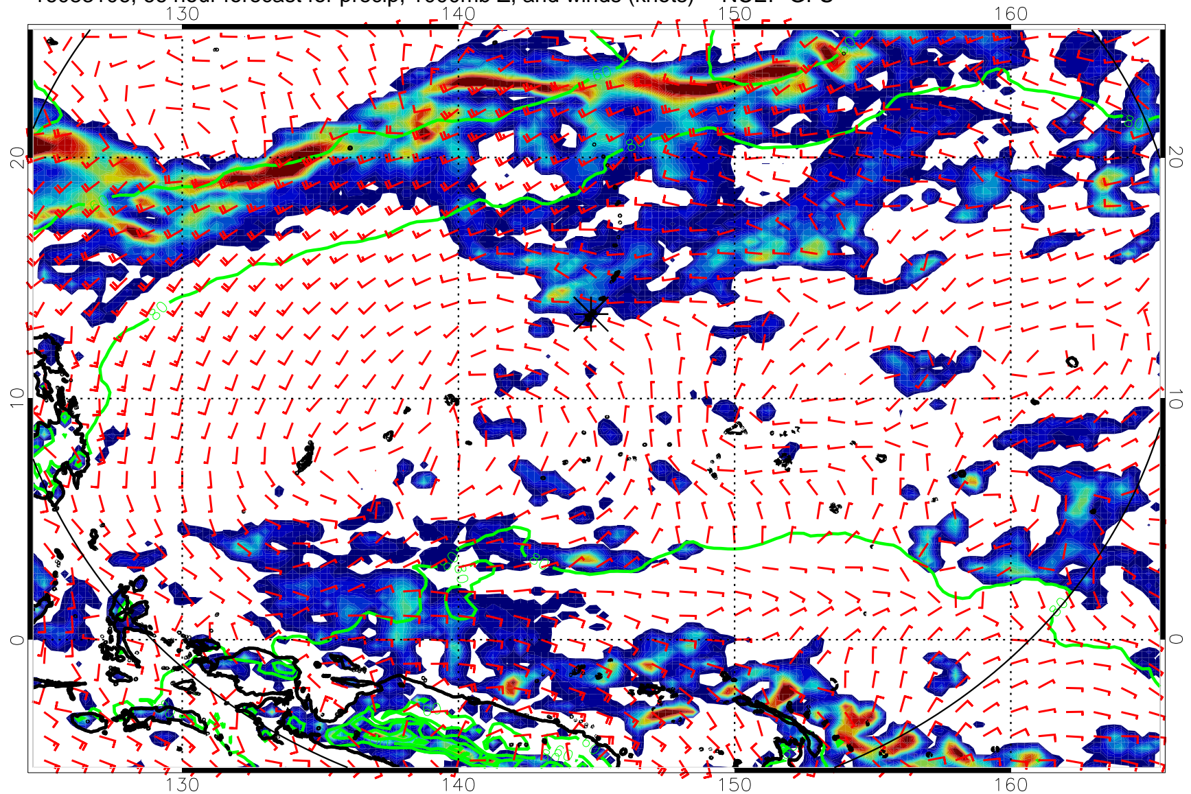
16083106, 66 hour forecast for precip, 1000mb Z, and winds (knots) -- NCEP GFS
