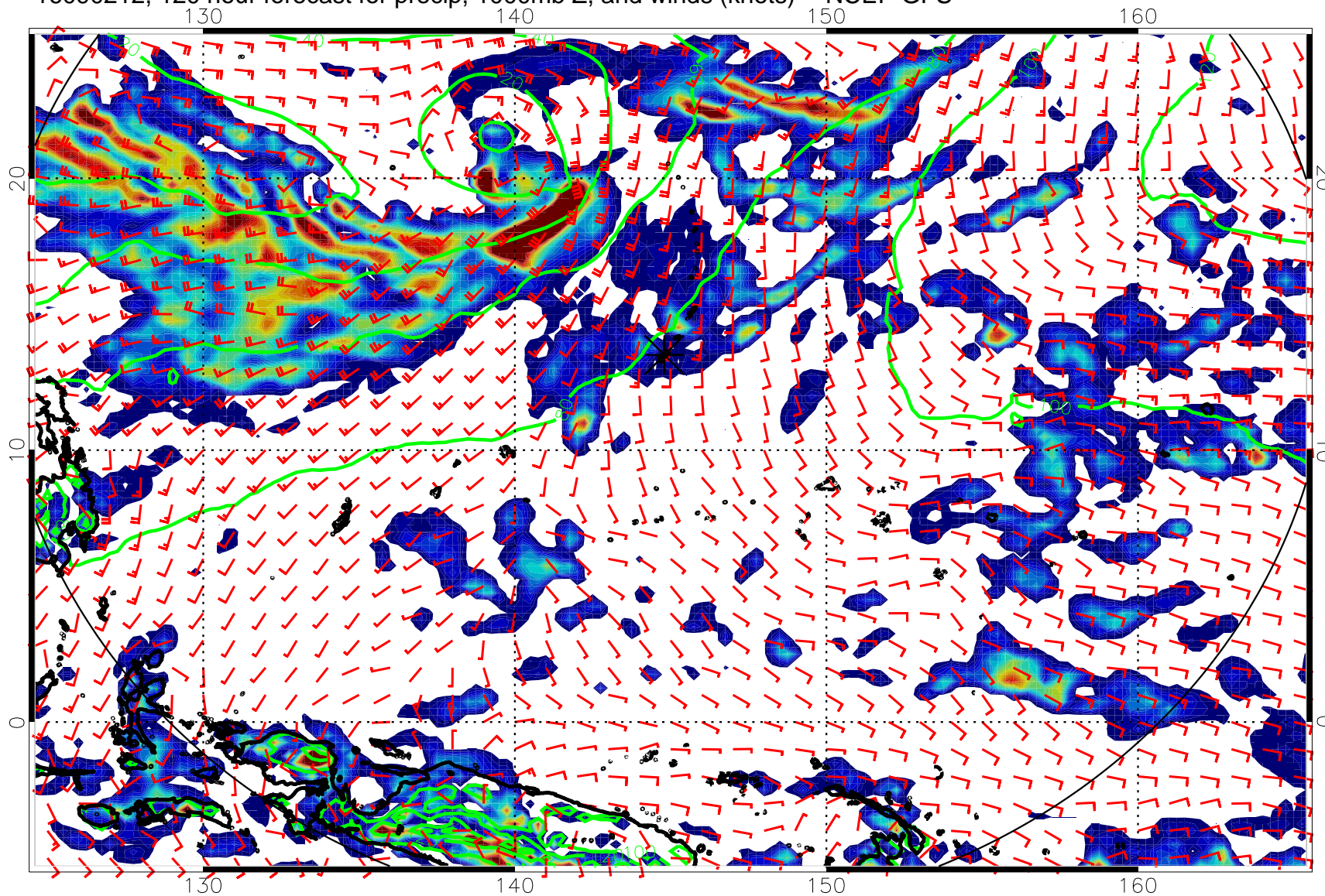
16090212, 120 hour forecast for precip, 1000mb Z, and winds (knots) -- NCEP GFS
