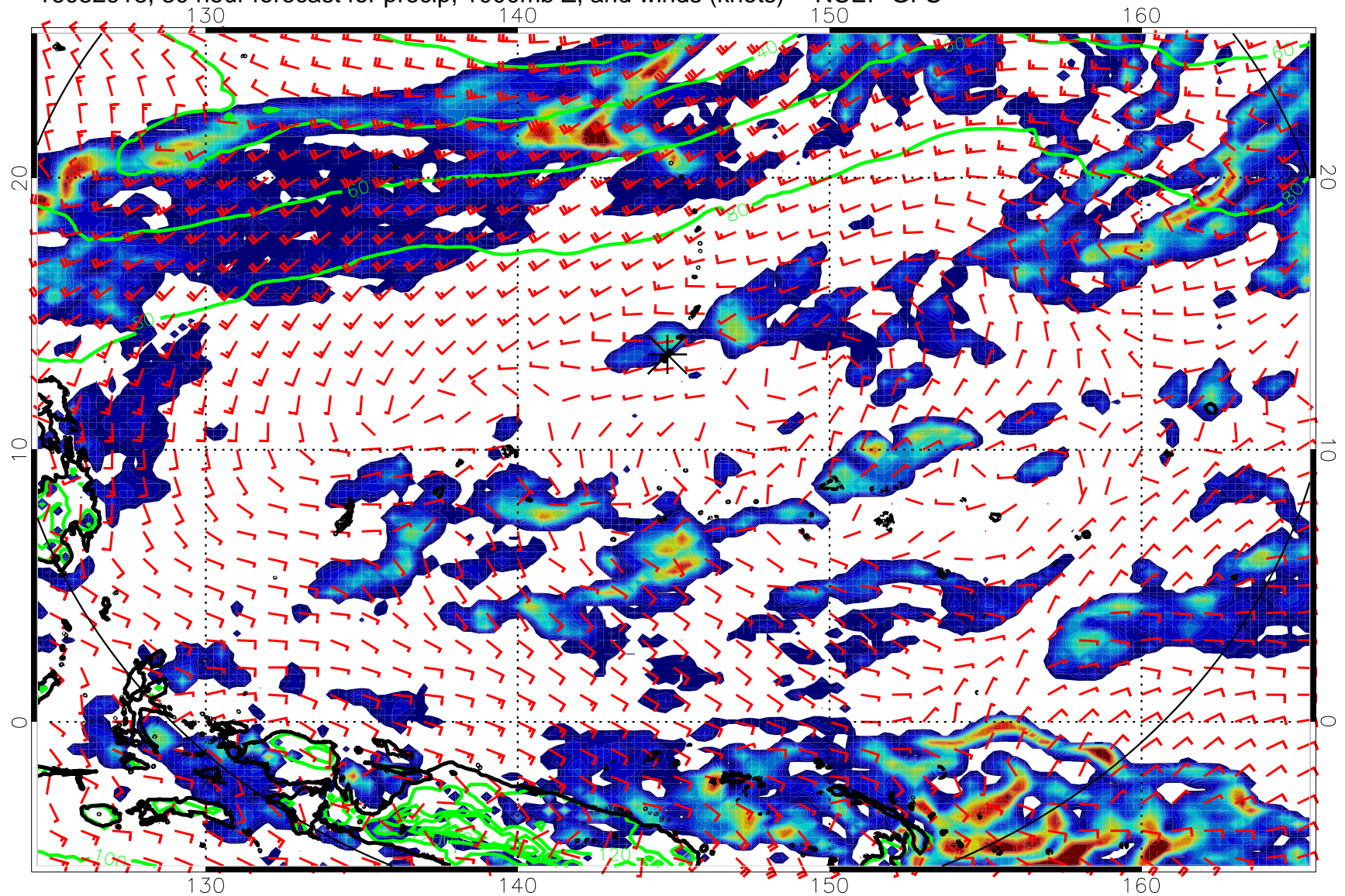
16082918, 30 hour forecast for precip, 1000mb Z, and winds (knots) -- NCEP GFS
