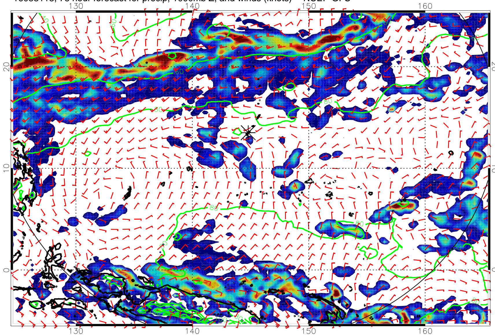
16083118, 78 hour forecast for precip, 1000mb Z, and winds (knots) -- NCEP GFS
