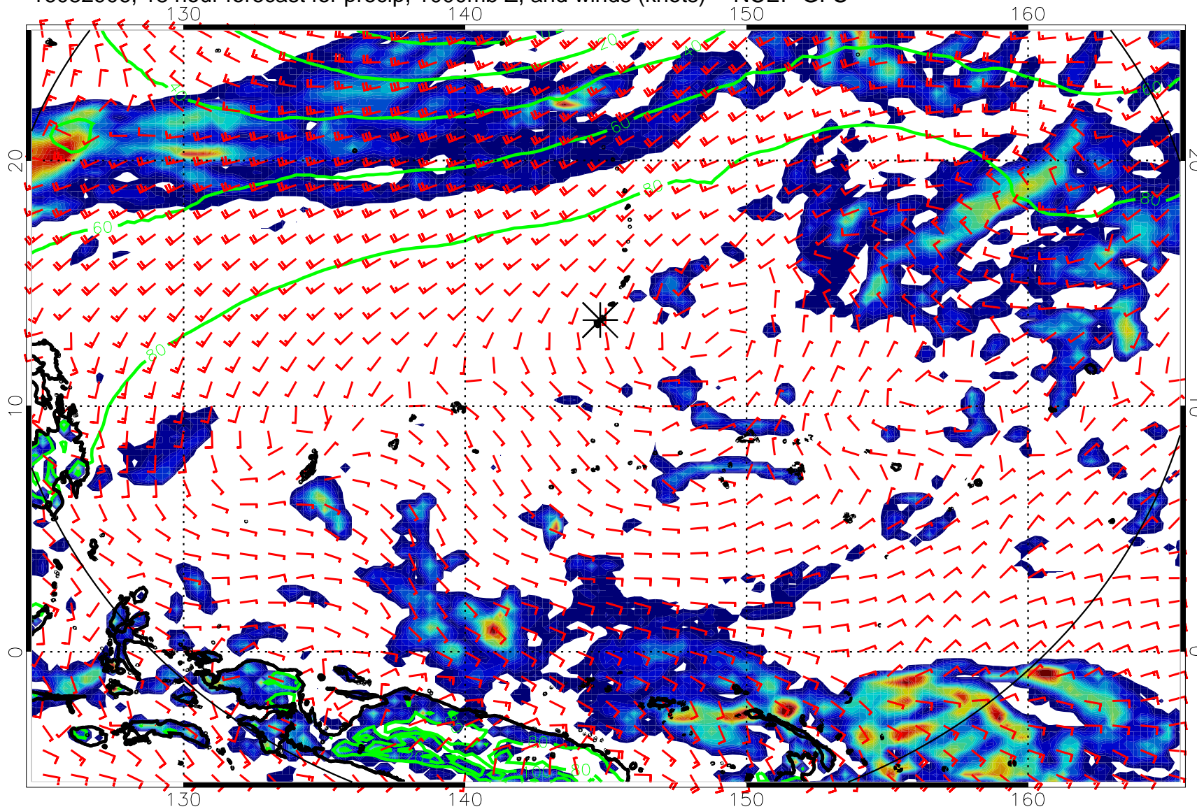
16082906, 18 hour forecast for precip, 1000mb Z, and winds (knots) -- NCEP GFS
