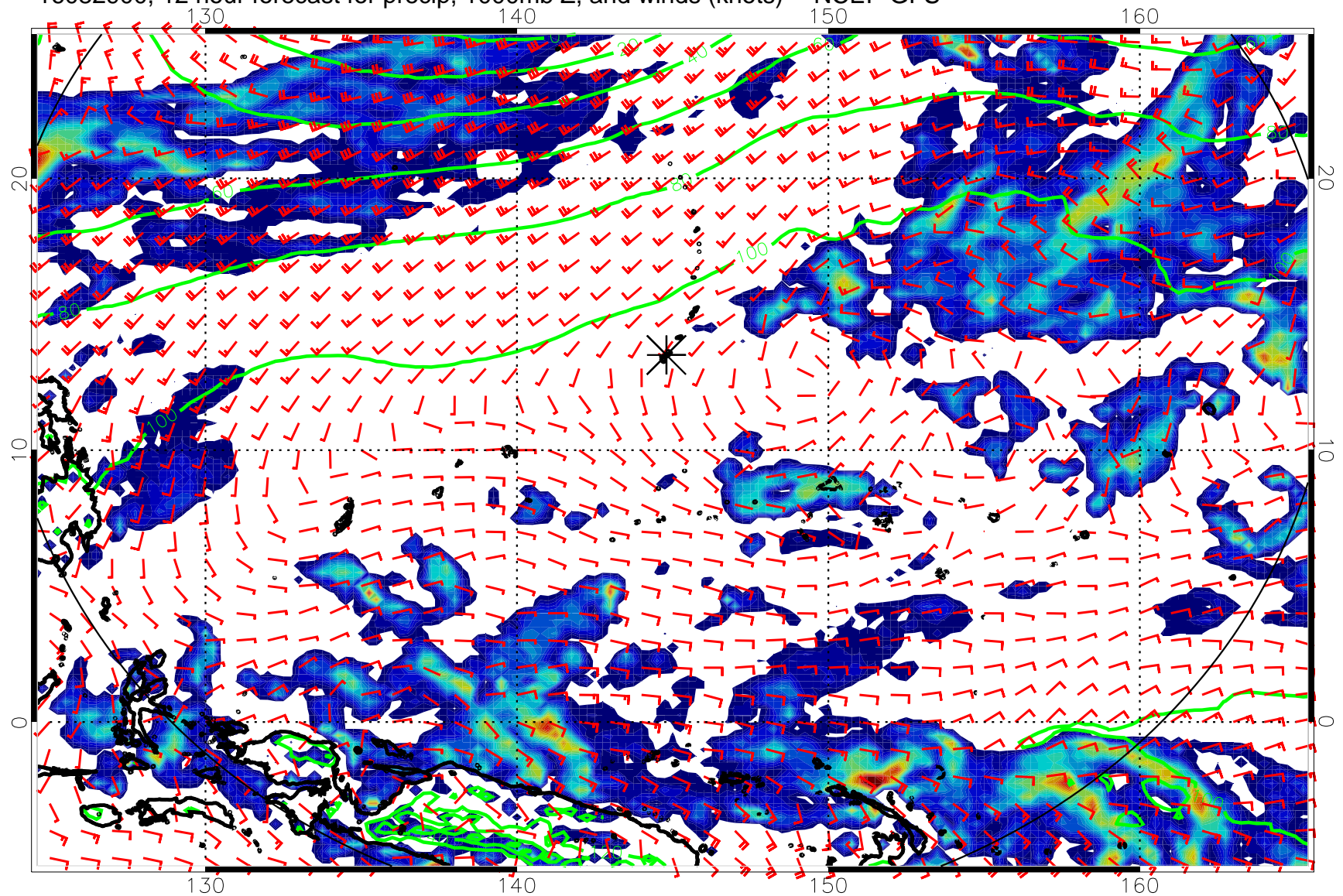
16082900, 12 hour forecast for precip, 1000mb Z, and winds (knots) -- NCEP GFS
