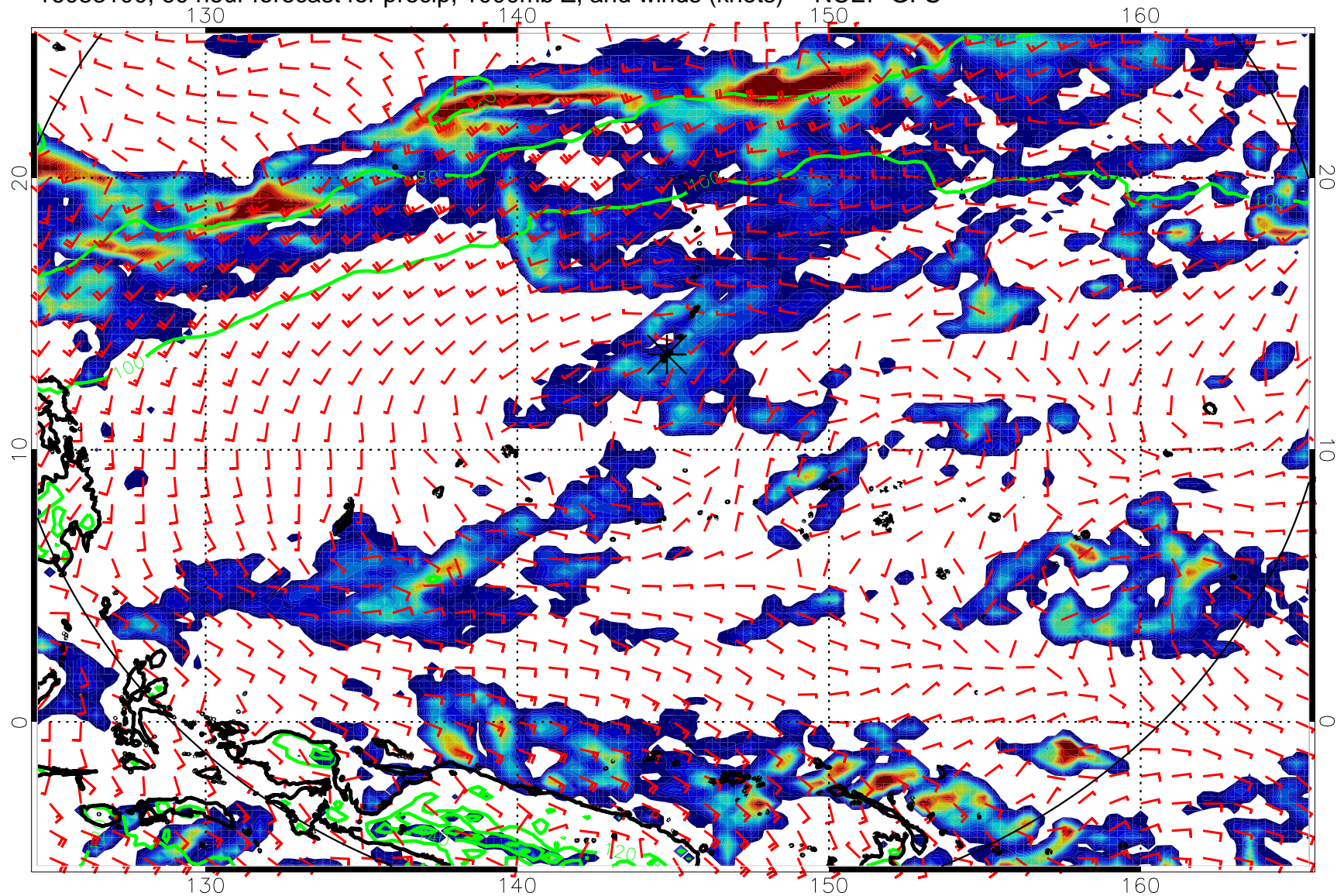
16083100, 60 hour forecast for precip, 1000mb Z, and winds (knots) -- NCEP GFS
