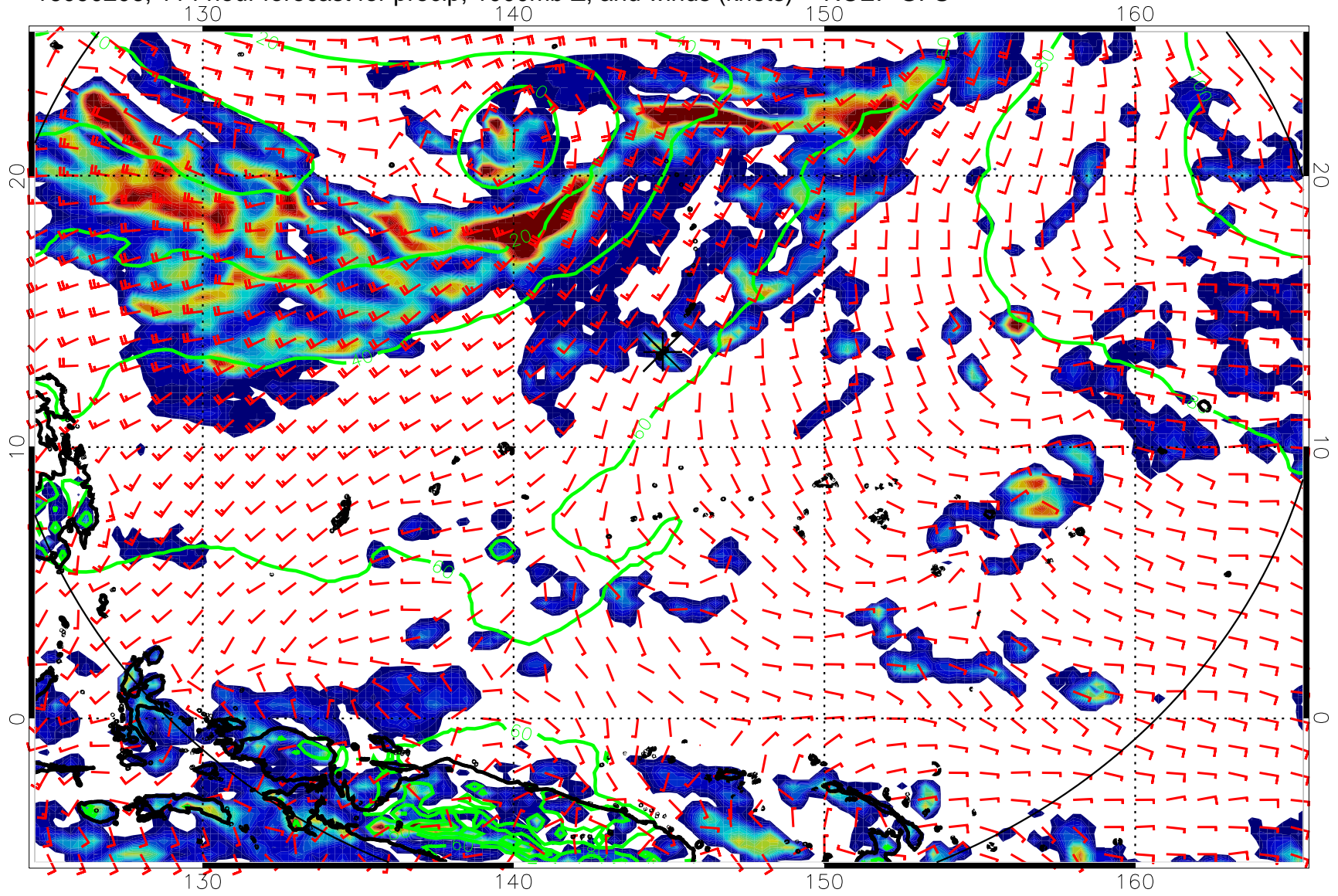
16090206, 114 hour forecast for precip, 1000mb Z, and winds (knots) -- NCEP GFS
