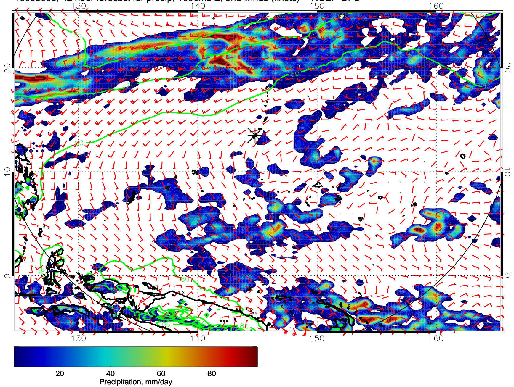
16083006, 42 hour forecast for precip, 1000mb Z, and winds (knots) -- NCEP GFS
