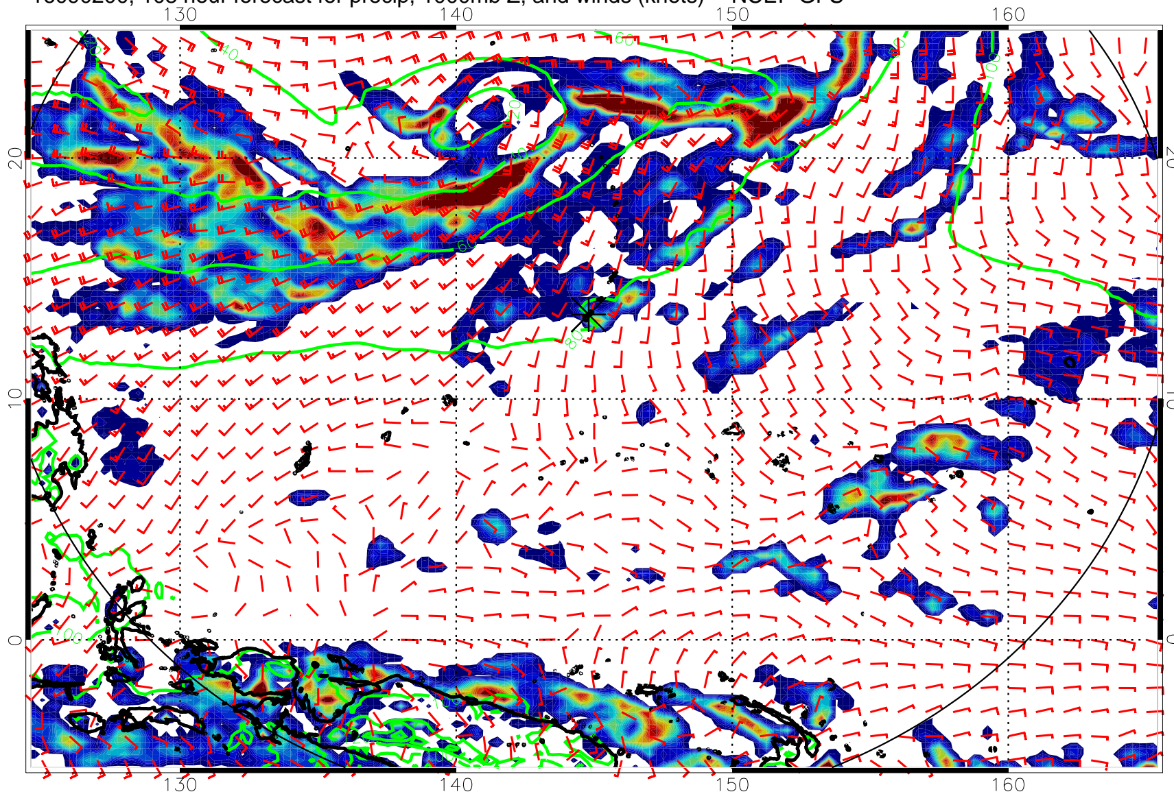
16090200, 108 hour forecast for precip, 1000mb Z, and winds (knots) -- NCEP GFS
