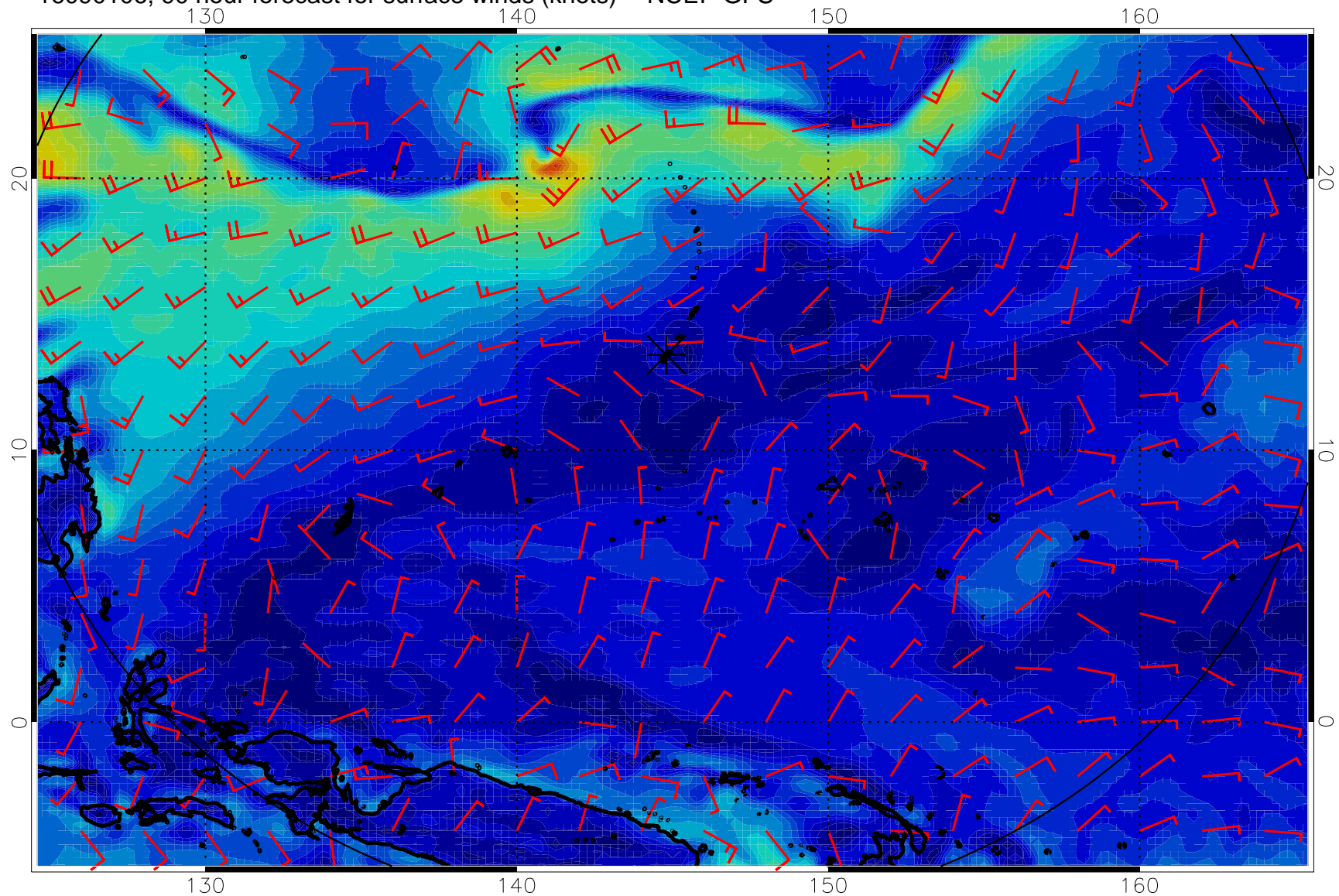
16090106, 90 hour forecast for surface winds (knots) -- NCEP GFS
