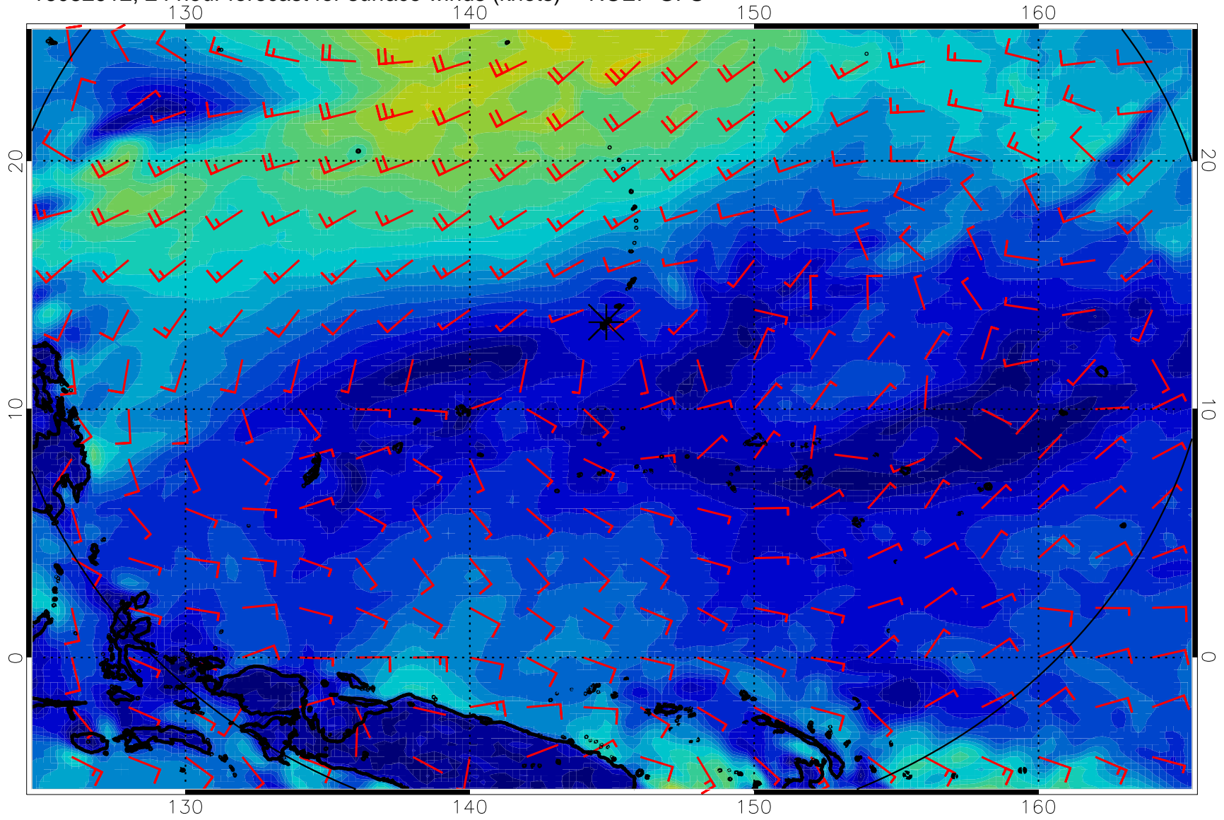
16082912, 24 hour forecast for surface winds (knots) -- NCEP GFS
