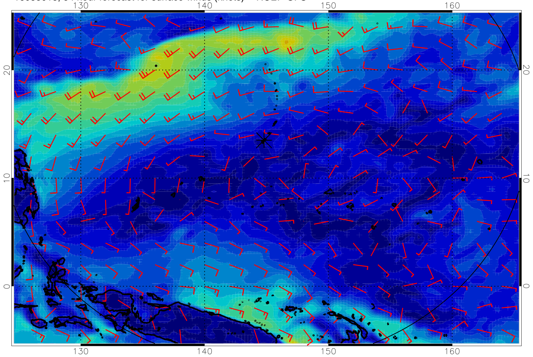
16083018, 54 hour forecast for surface winds (knots) -- NCEP GFS
