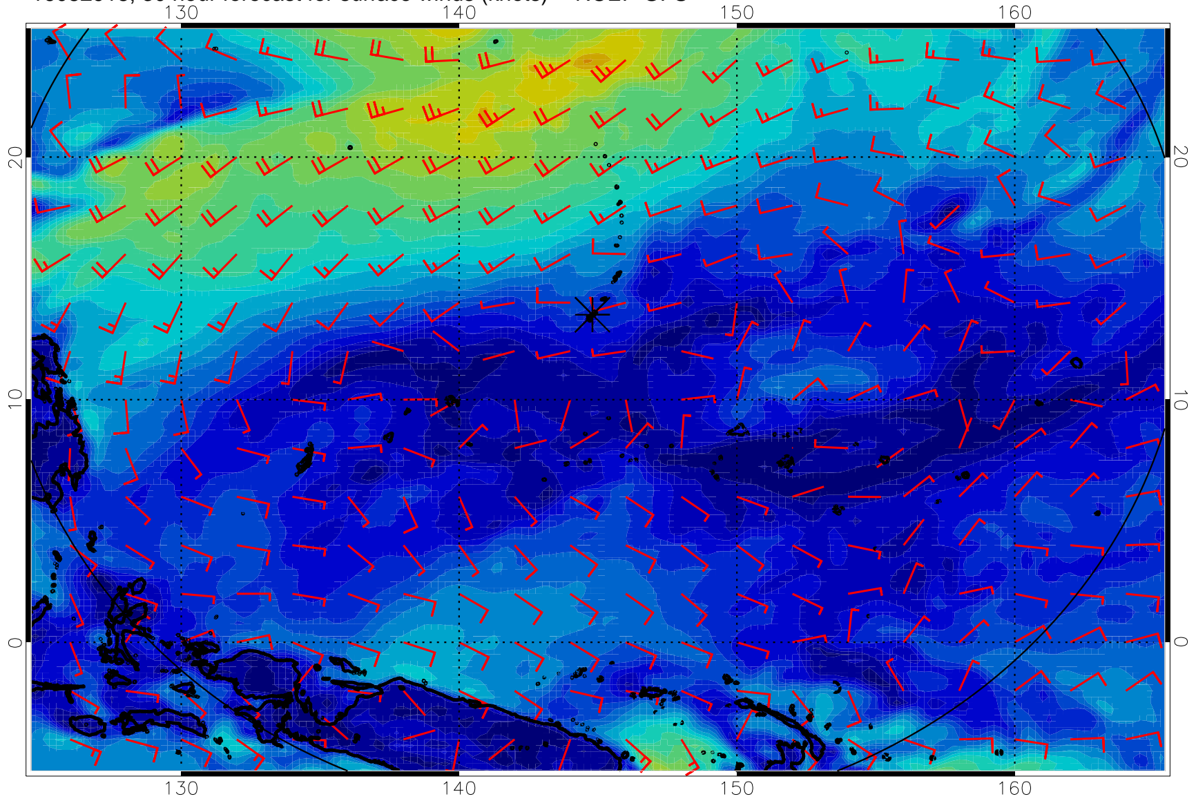
16082918, 30 hour forecast for surface winds (knots) -- NCEP GFS
