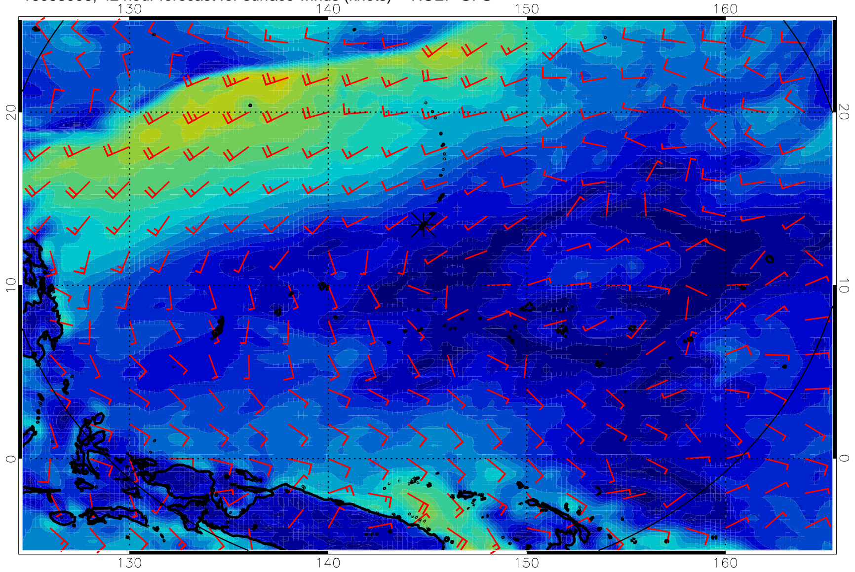
16083006, 42 hour forecast for surface winds (knots) -- NCEP GFS
