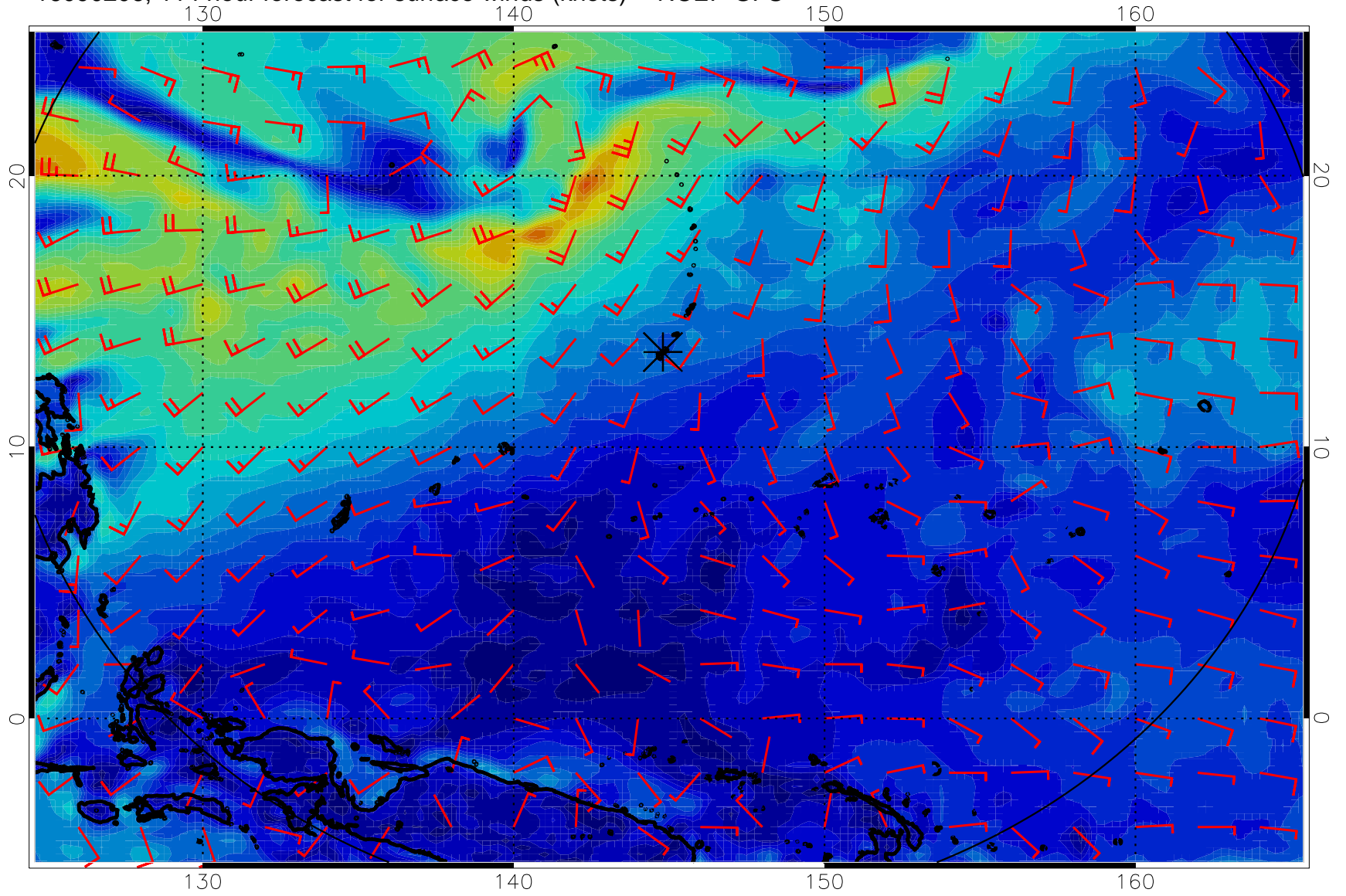
16090206, 114 hour forecast for surface winds (knots) -- NCEP GFS
