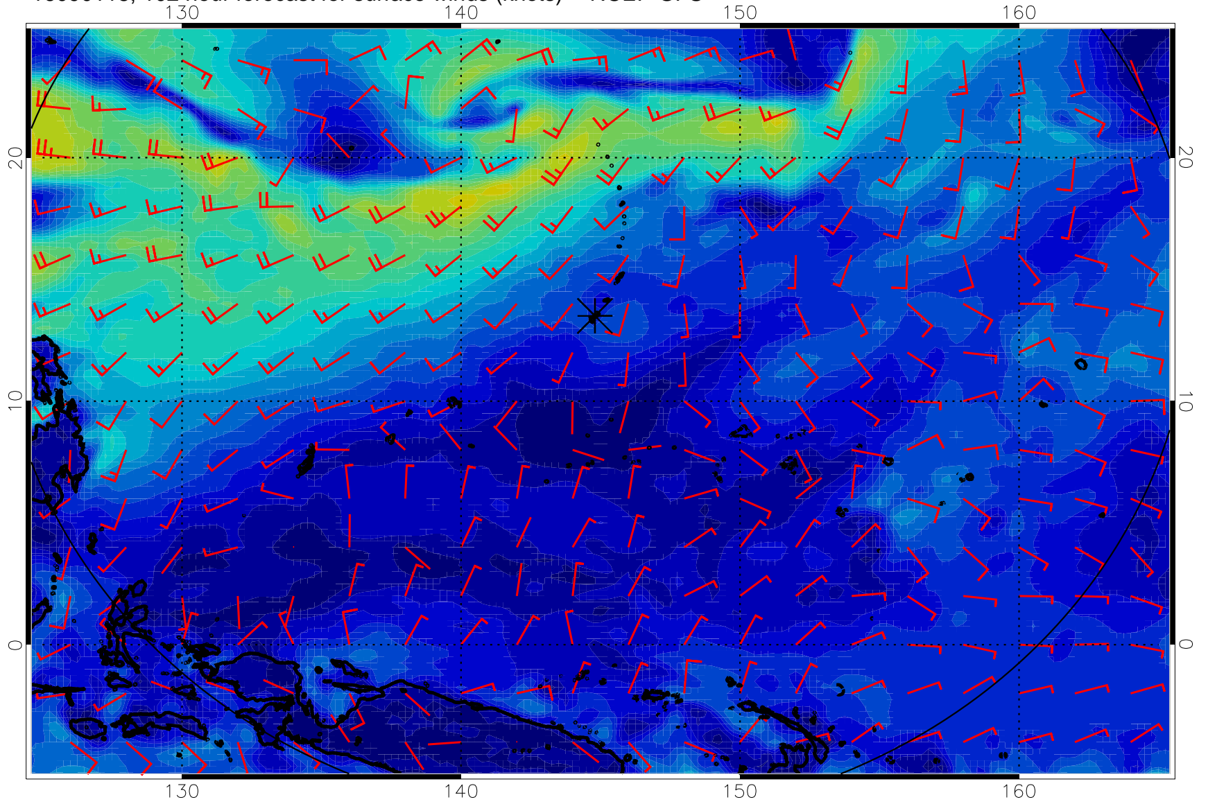
16090118, 102 hour forecast for surface winds (knots) -- NCEP GFS
