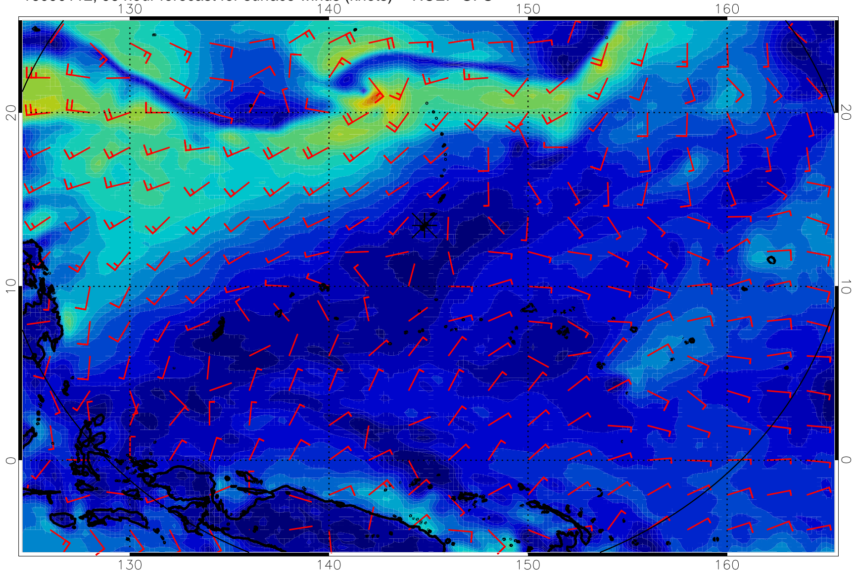
16090112, 96 hour forecast for surface winds (knots) -- NCEP GFS
