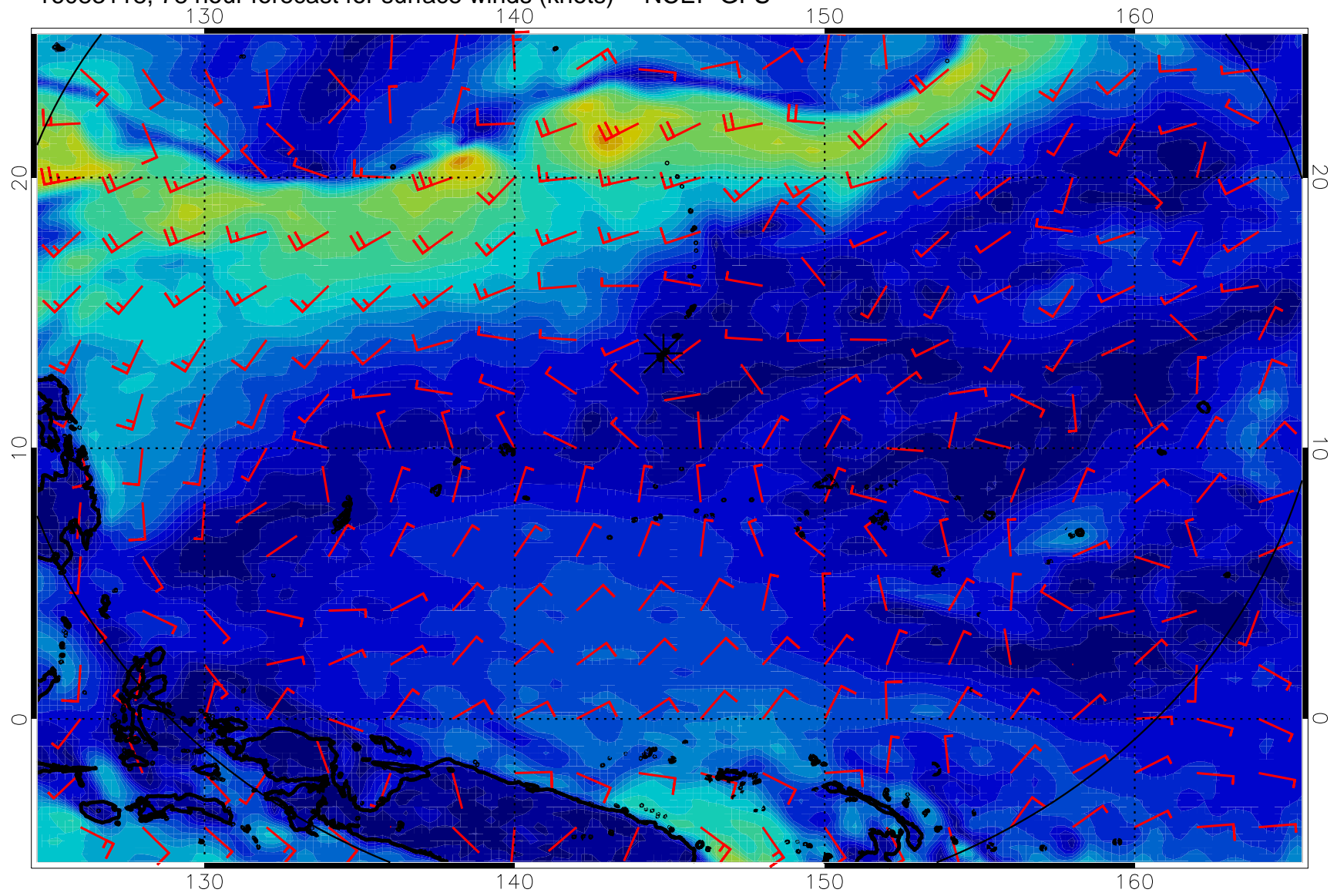
16083118, 78 hour forecast for surface winds (knots) -- NCEP GFS
