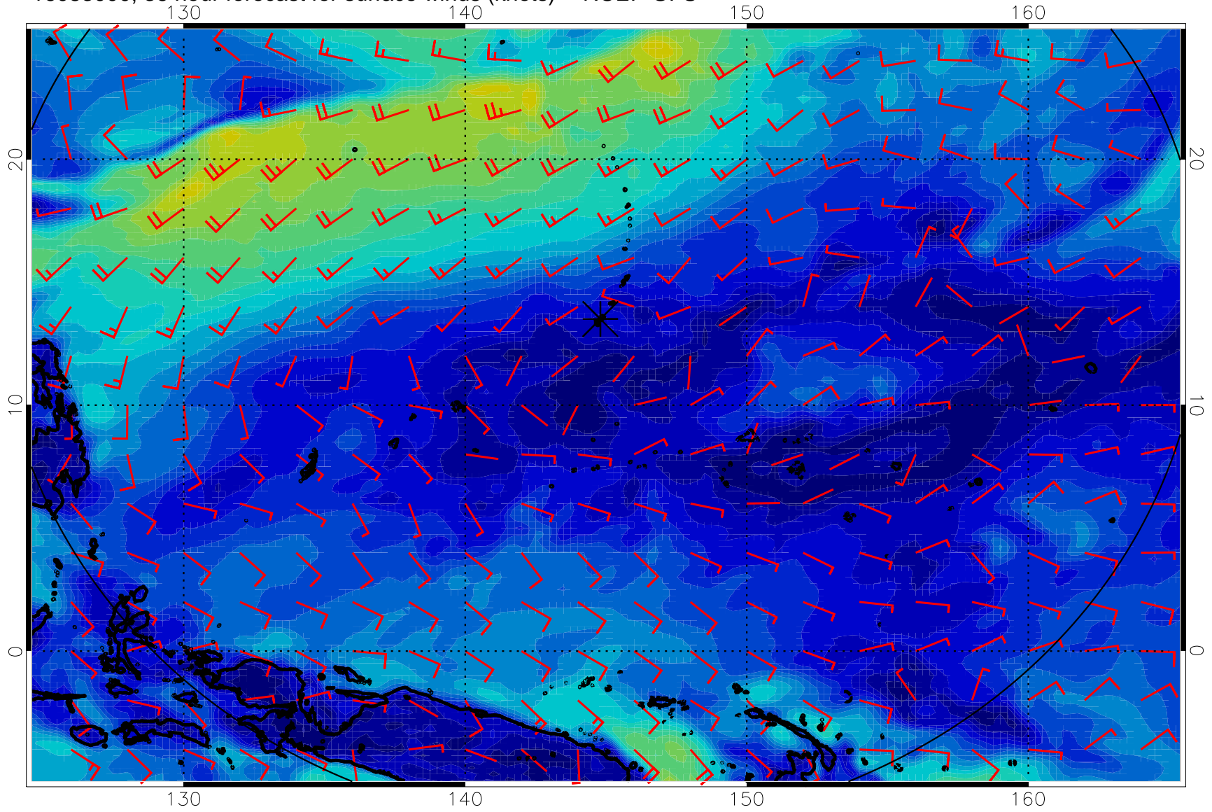
16083000, 36 hour forecast for surface winds (knots) -- NCEP GFS
