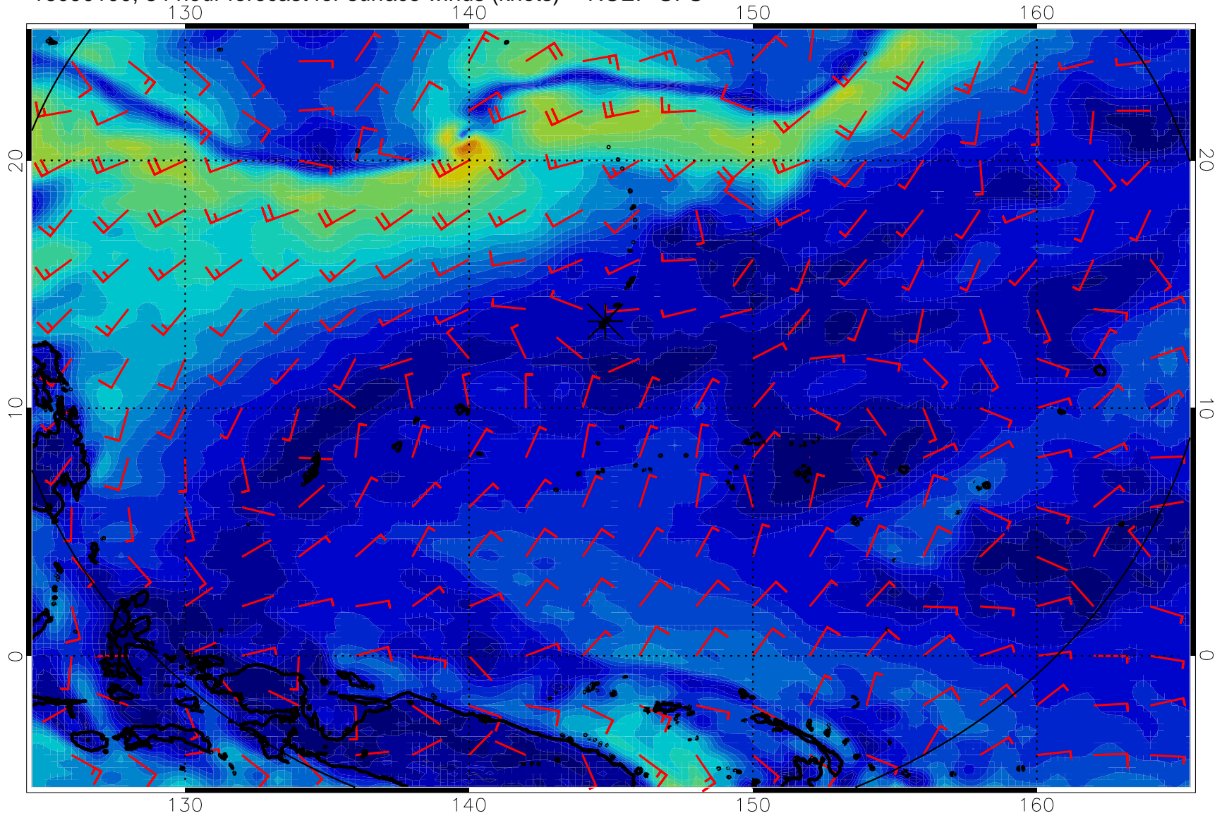
16090100, 84 hour forecast for surface winds (knots) -- NCEP GFS
