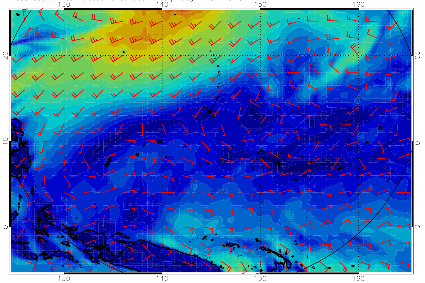
16082900, 12 hour forecast for surface winds (knots) -- NCEP GFS
