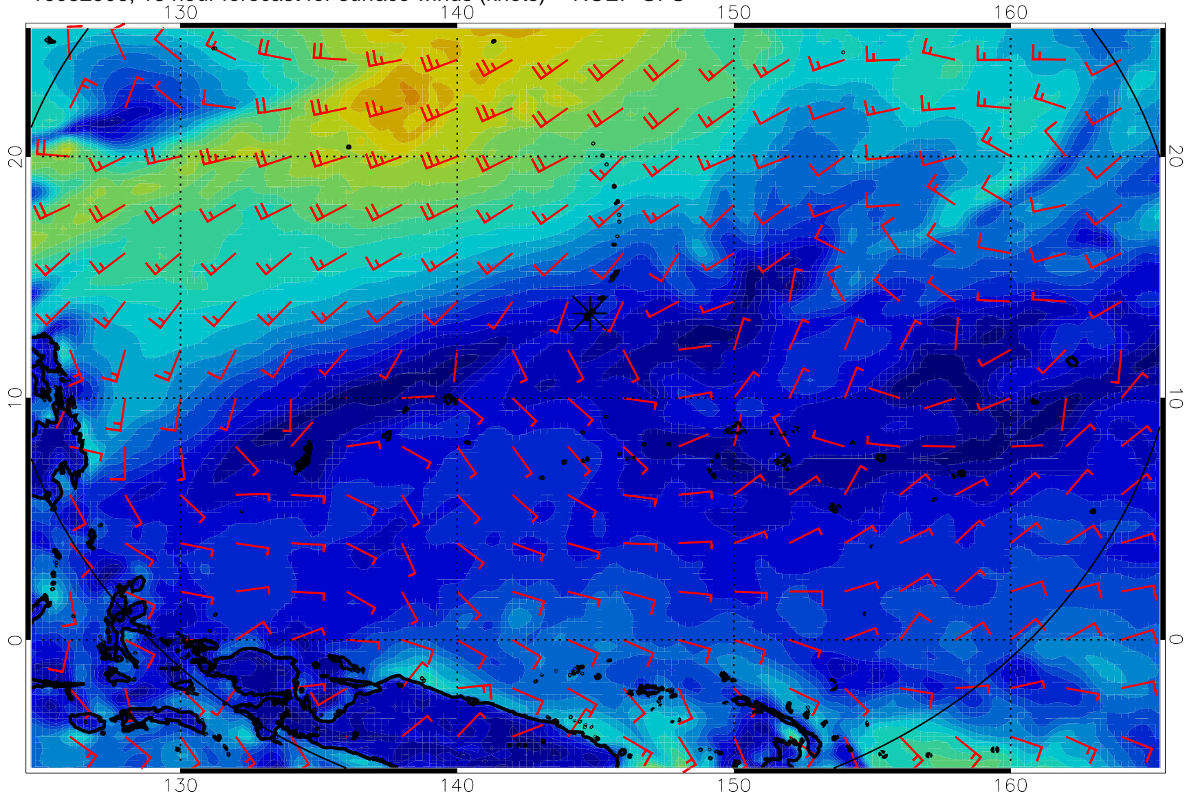
16082906, 18 hour forecast for surface winds (knots) -- NCEP GFS
