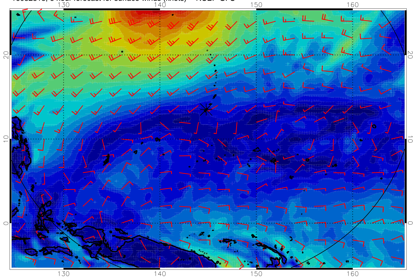
16082818, 6 hour forecast for surface winds (knots) -- NCEP GFS
