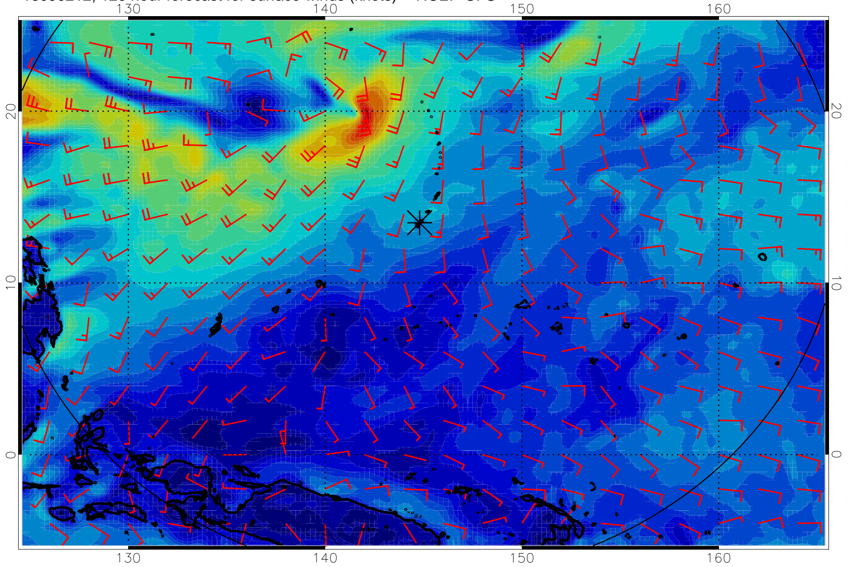
16090212, 120 hour forecast for surface winds (knots) -- NCEP GFS
