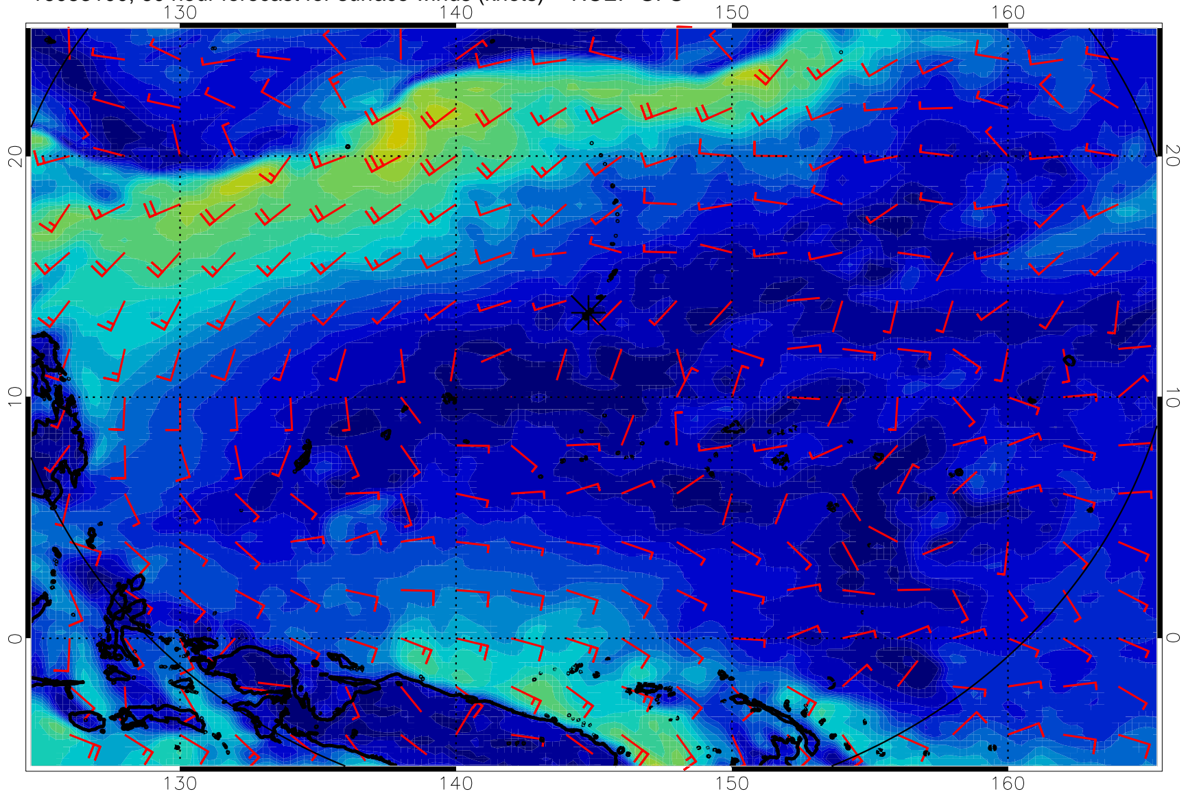
16083100, 60 hour forecast for surface winds (knots) -- NCEP GFS
