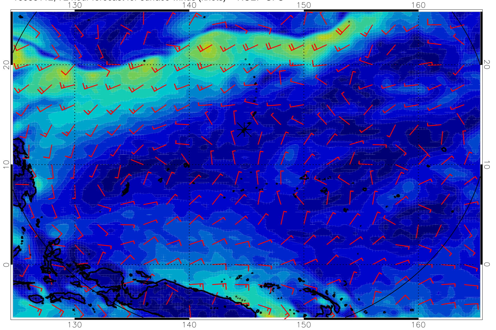
16083112, 72 hour forecast for surface winds (knots) -- NCEP GFS
