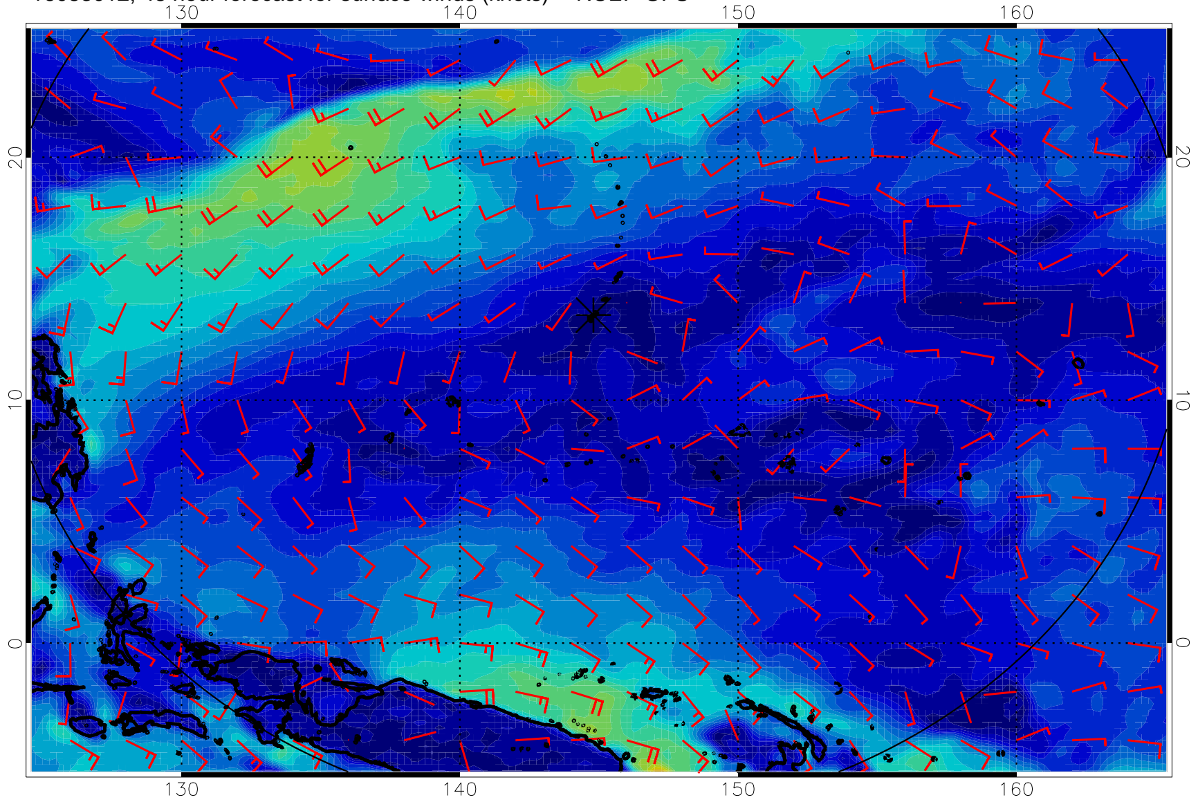
16083012, 48 hour forecast for surface winds (knots) -- NCEP GFS
