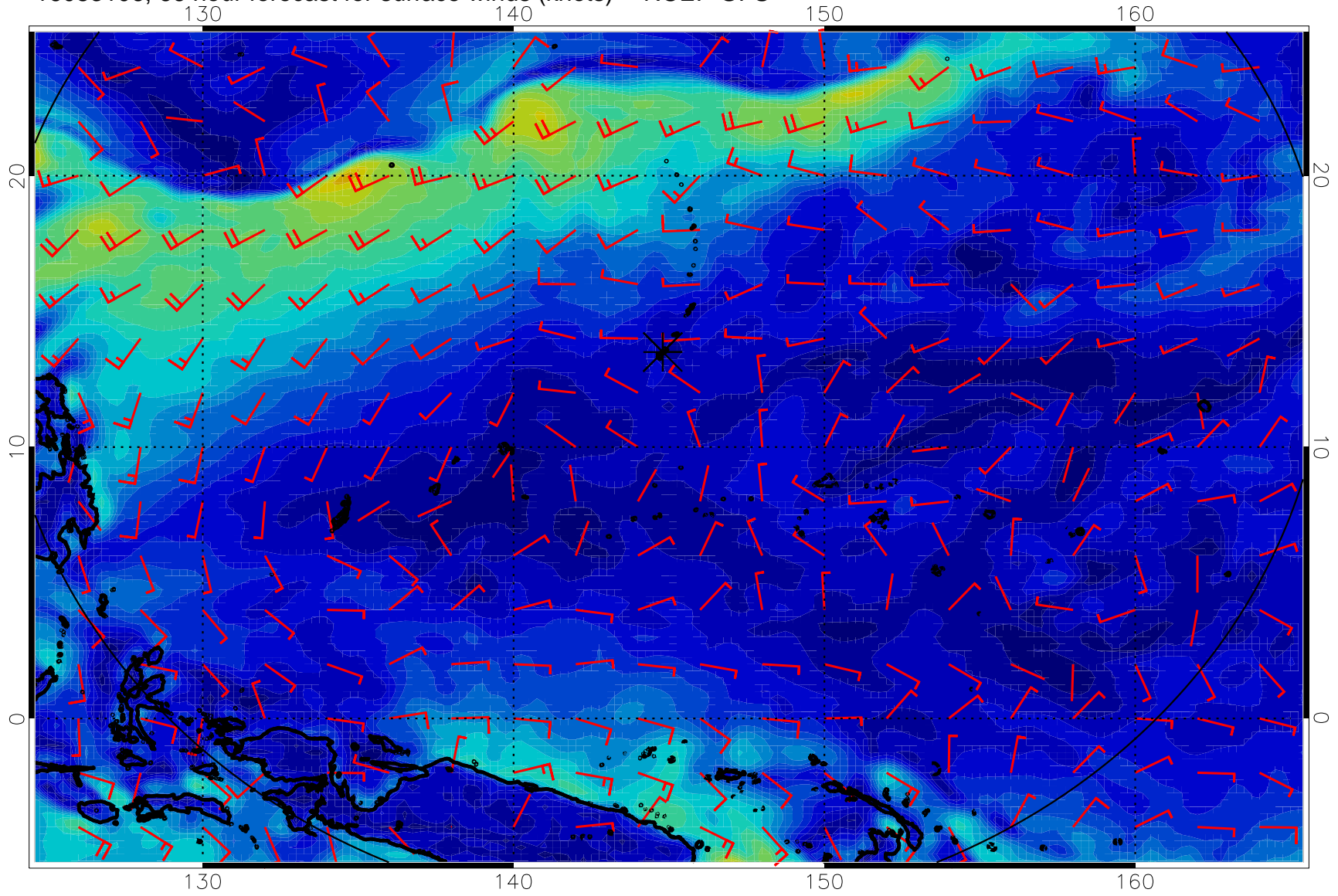
16083106, 66 hour forecast for surface winds (knots) -- NCEP GFS
