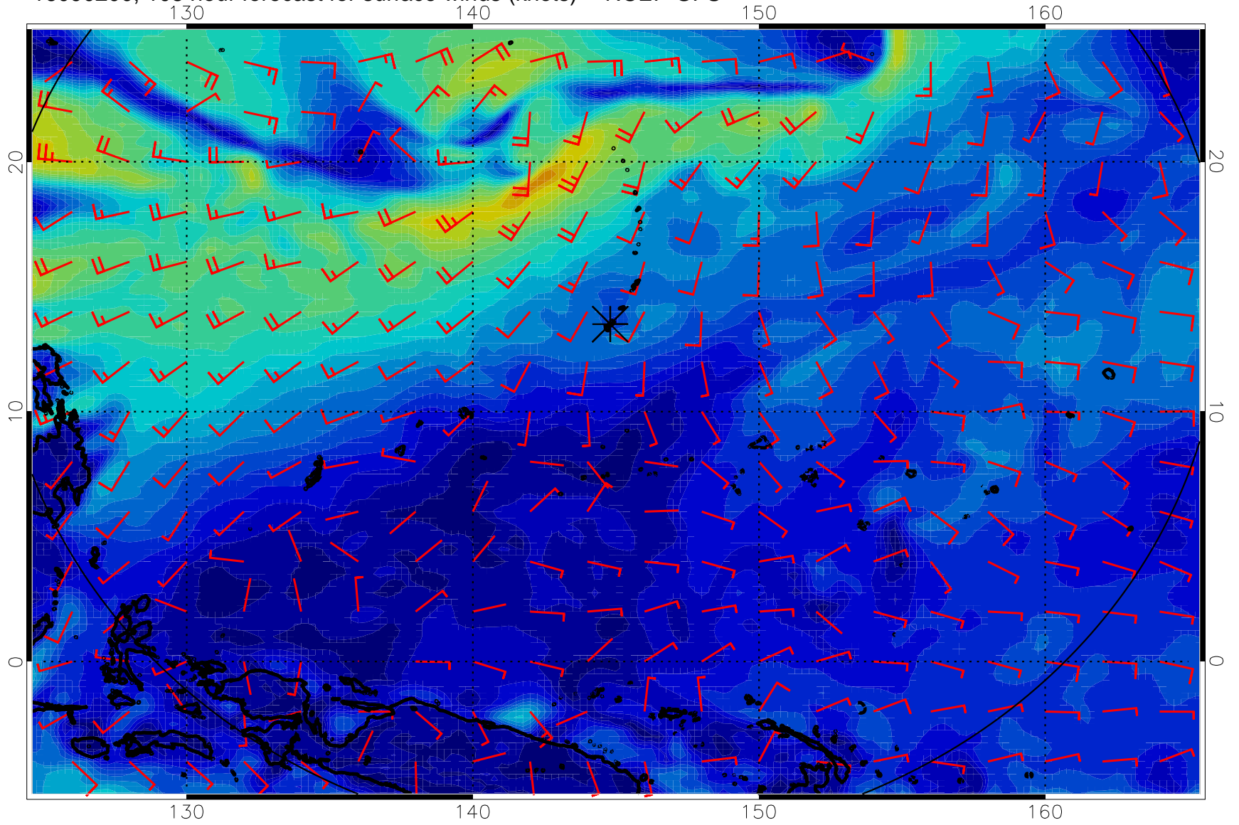
16090200, 108 hour forecast for surface winds (knots) -- NCEP GFS
