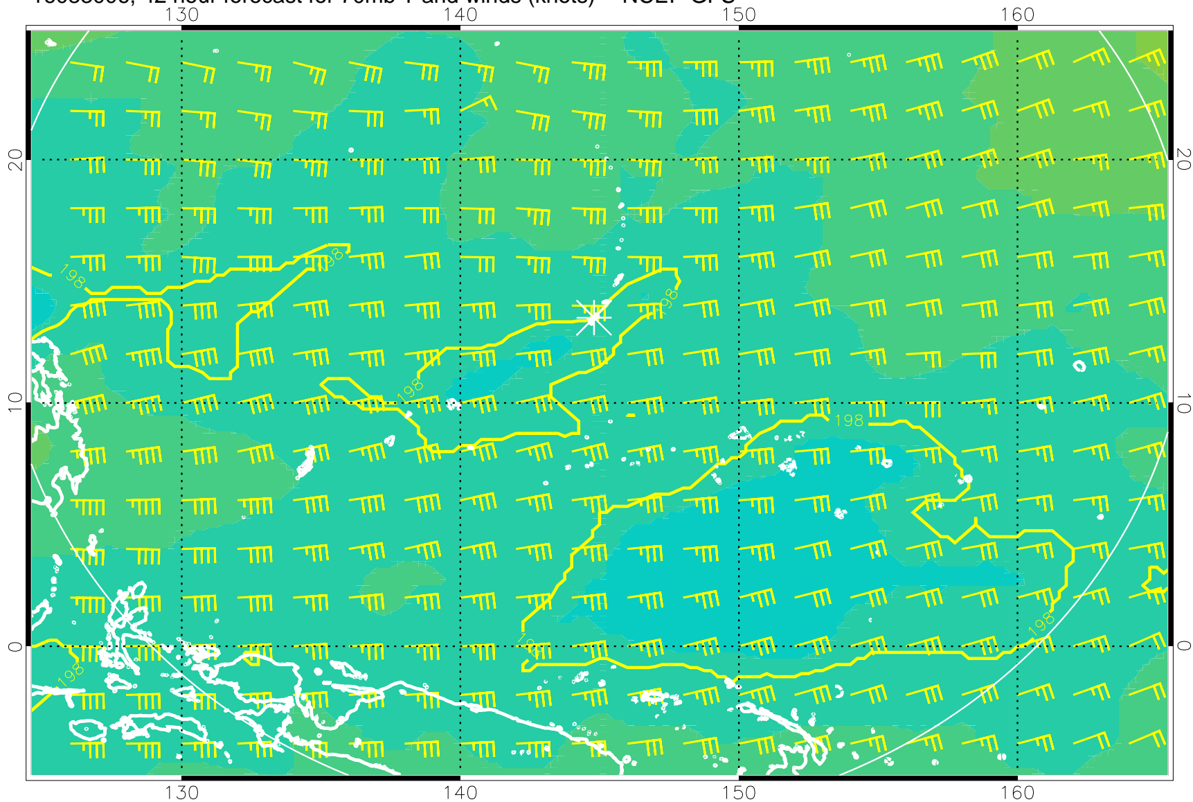
16083006, 42 hour forecast for 70mb T and winds (knots) -- NCEP GFS
