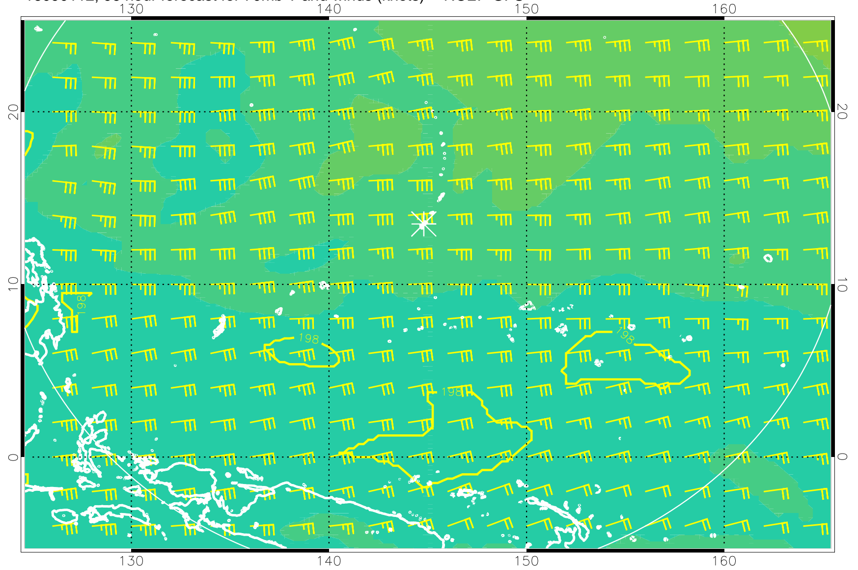
16090112, 96 hour forecast for 70mb T and winds (knots) -- NCEP GFS
