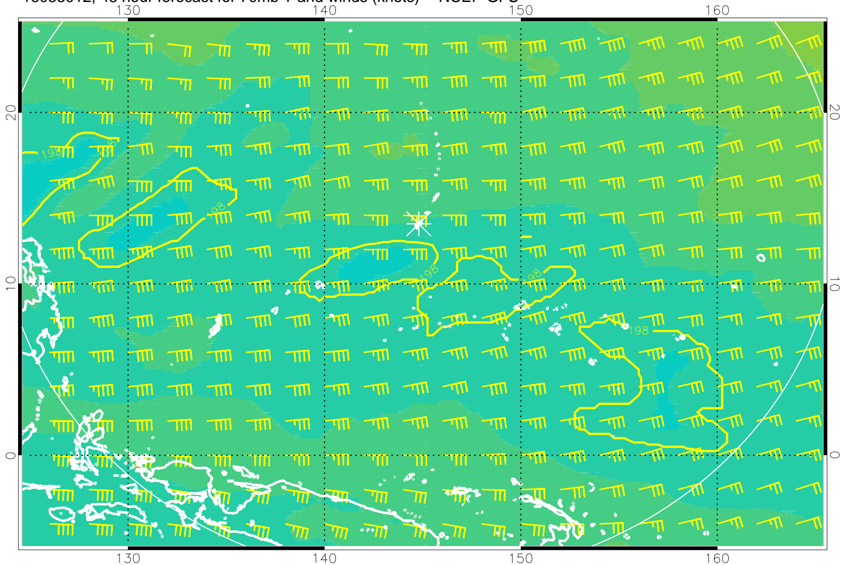
16083012, 48 hour forecast for 70mb T and winds (knots) -- NCEP GFS
