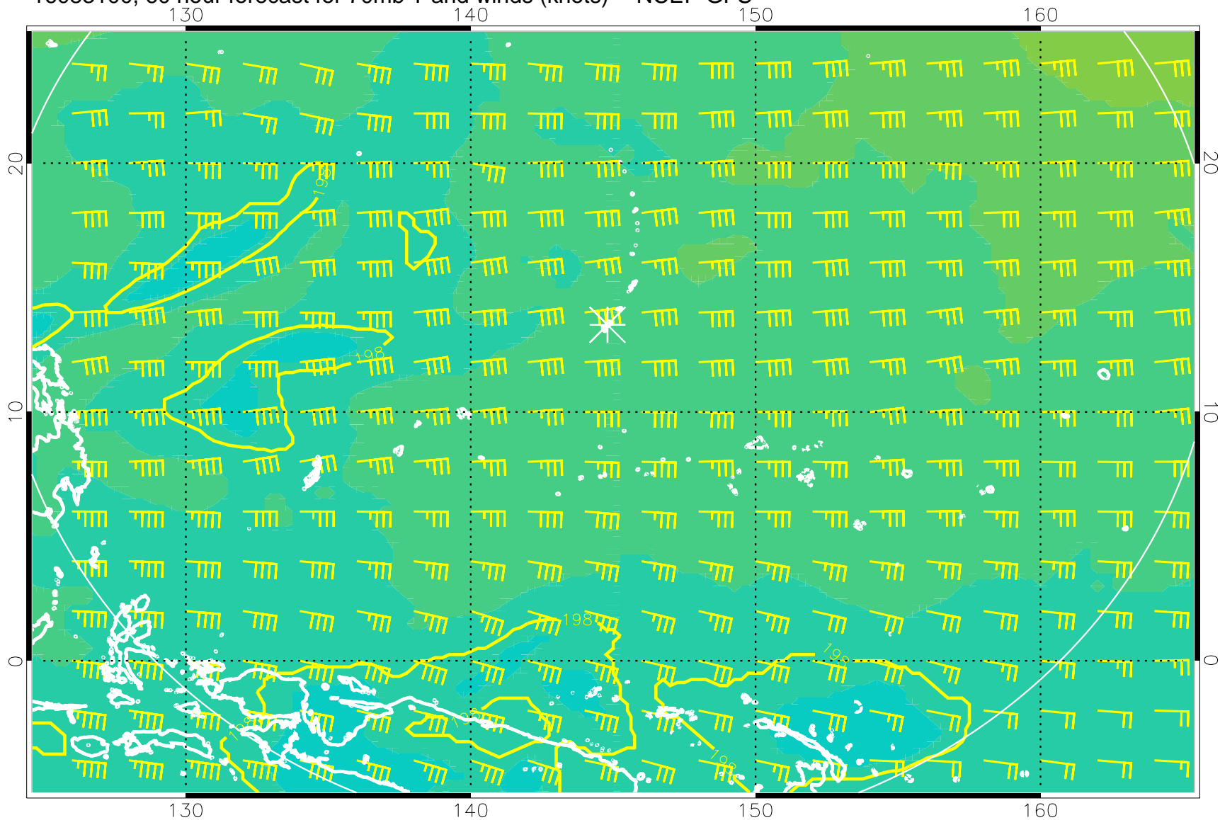
16083100, 60 hour forecast for 70mb T and winds (knots) -- NCEP GFS
