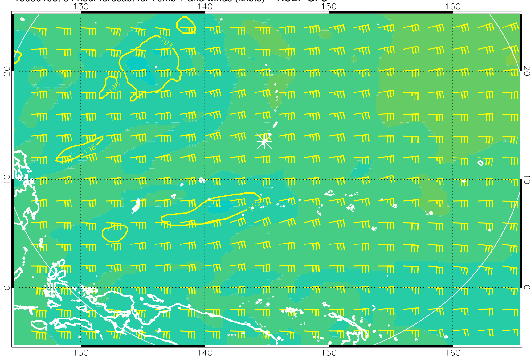
16090100, 84 hour forecast for 70mb T and winds (knots) -- NCEP GFS
