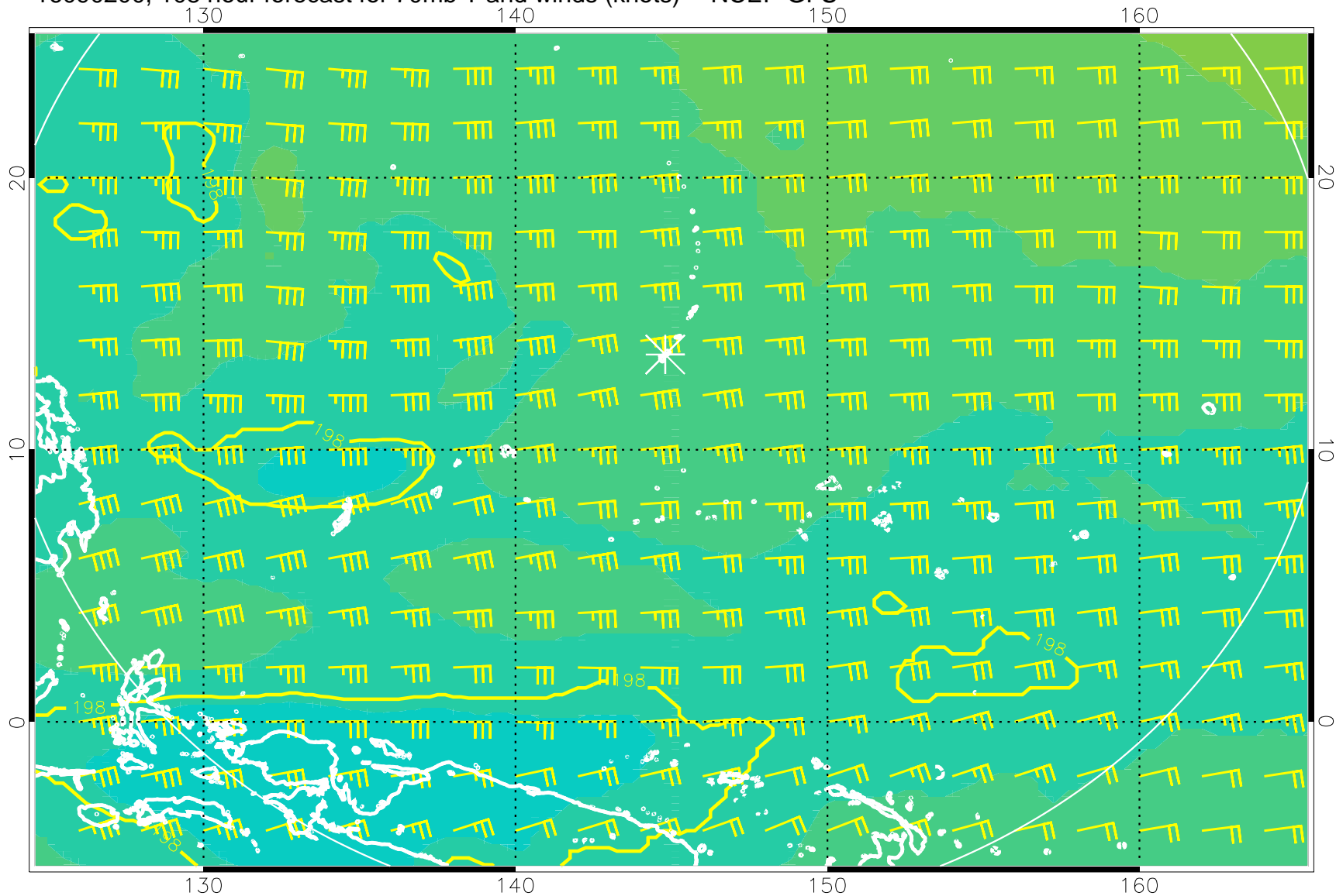
16090200, 108 hour forecast for 70mb T and winds (knots) -- NCEP GFS
