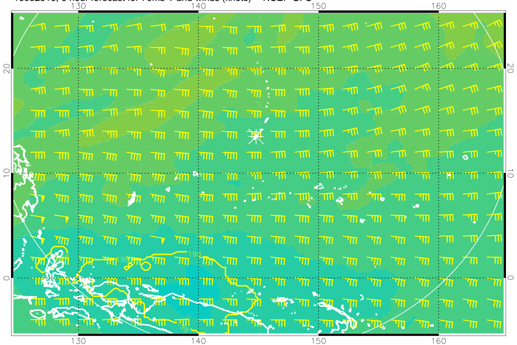
16082818, 6 hour forecast for 70mb T and winds (knots) -- NCEP GFS
