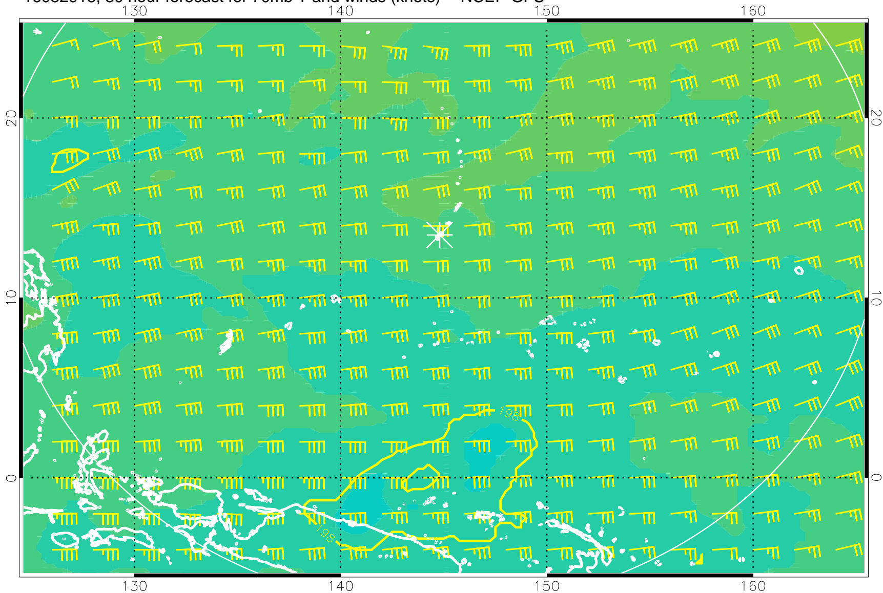
16082918, 30 hour forecast for 70mb T and winds (knots) -- NCEP GFS
