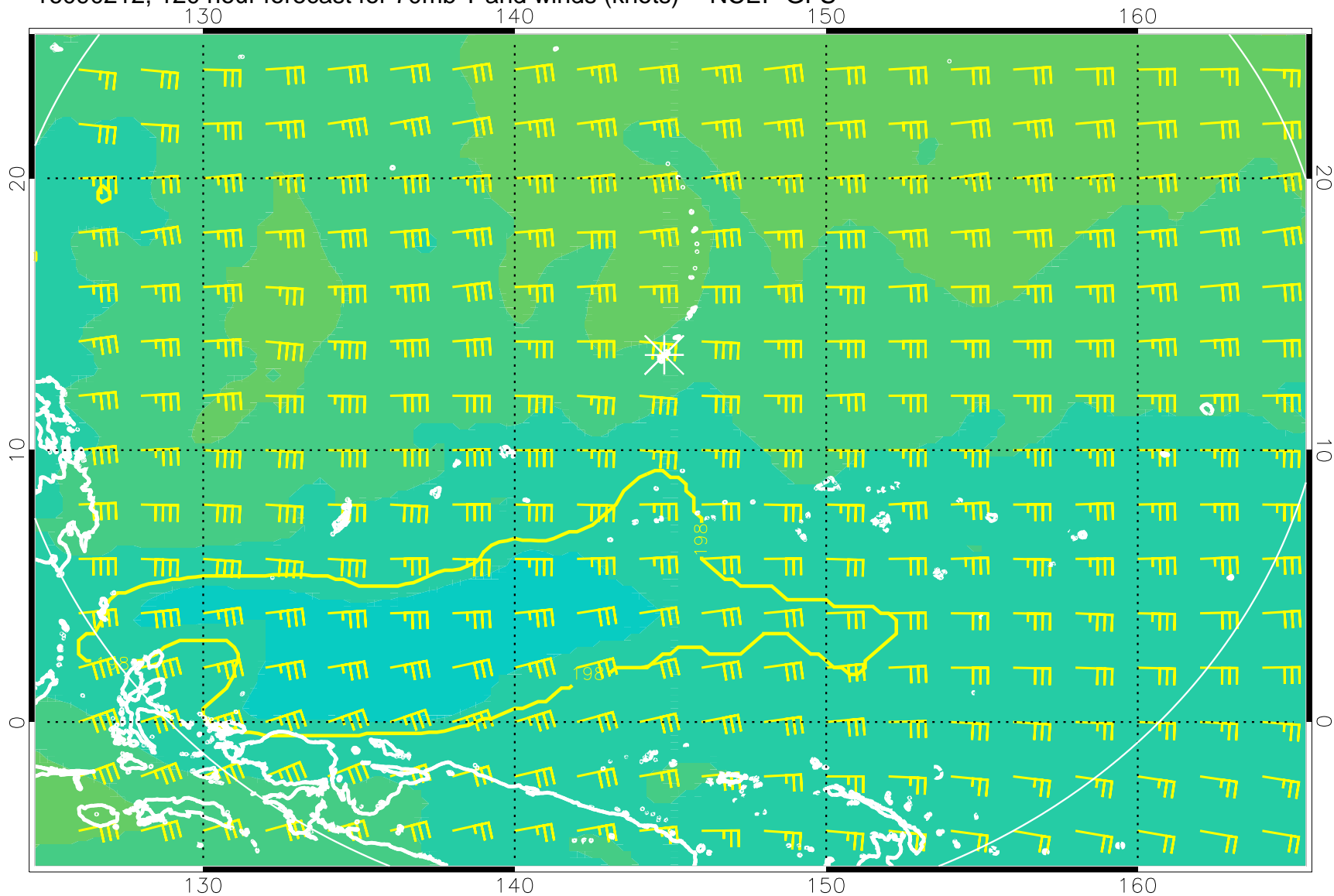
16090212, 120 hour forecast for 70mb T and winds (knots) -- NCEP GFS
