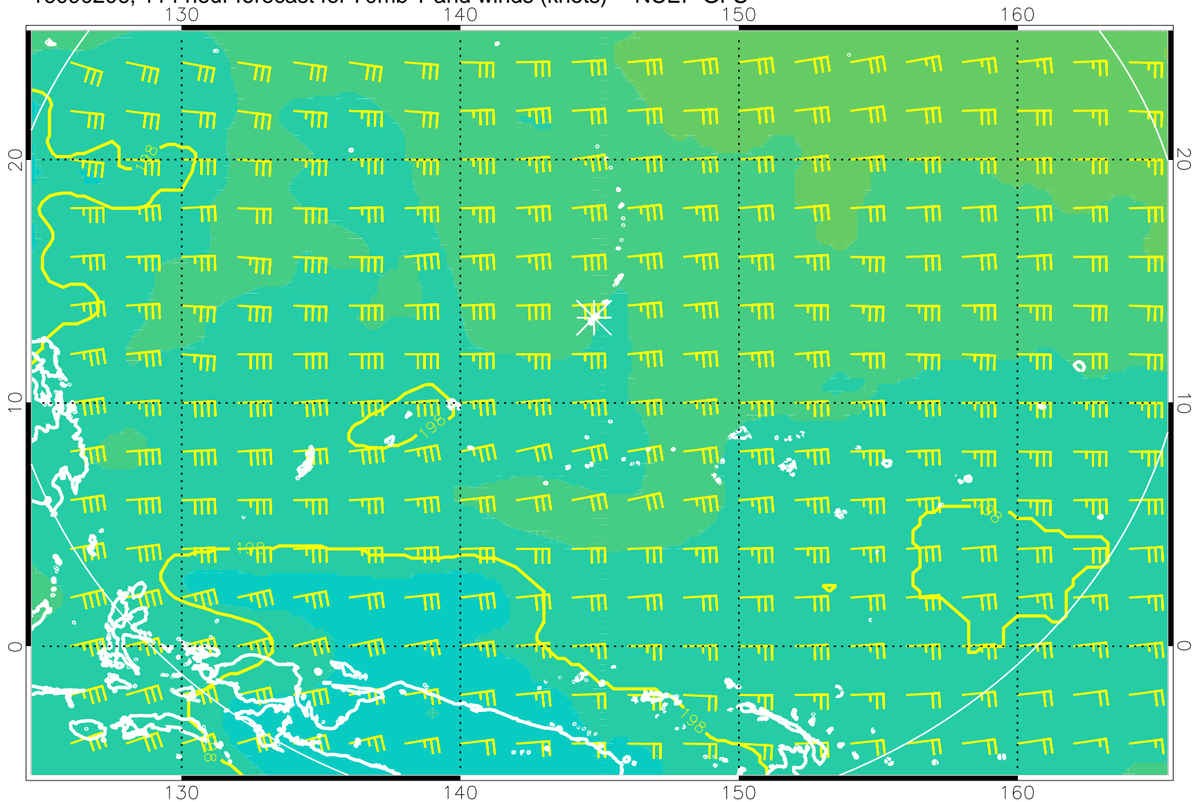
16090206, 114 hour forecast for 70mb T and winds (knots) -- NCEP GFS
