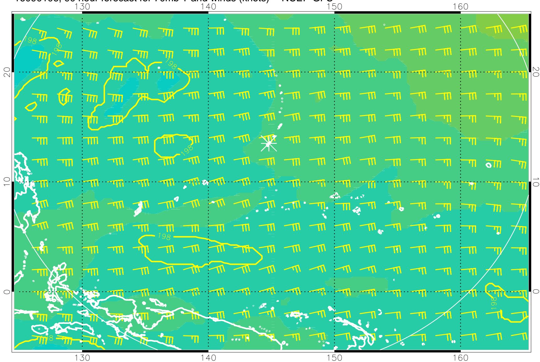
16090106, 90 hour forecast for 70mb T and winds (knots) -- NCEP GFS
