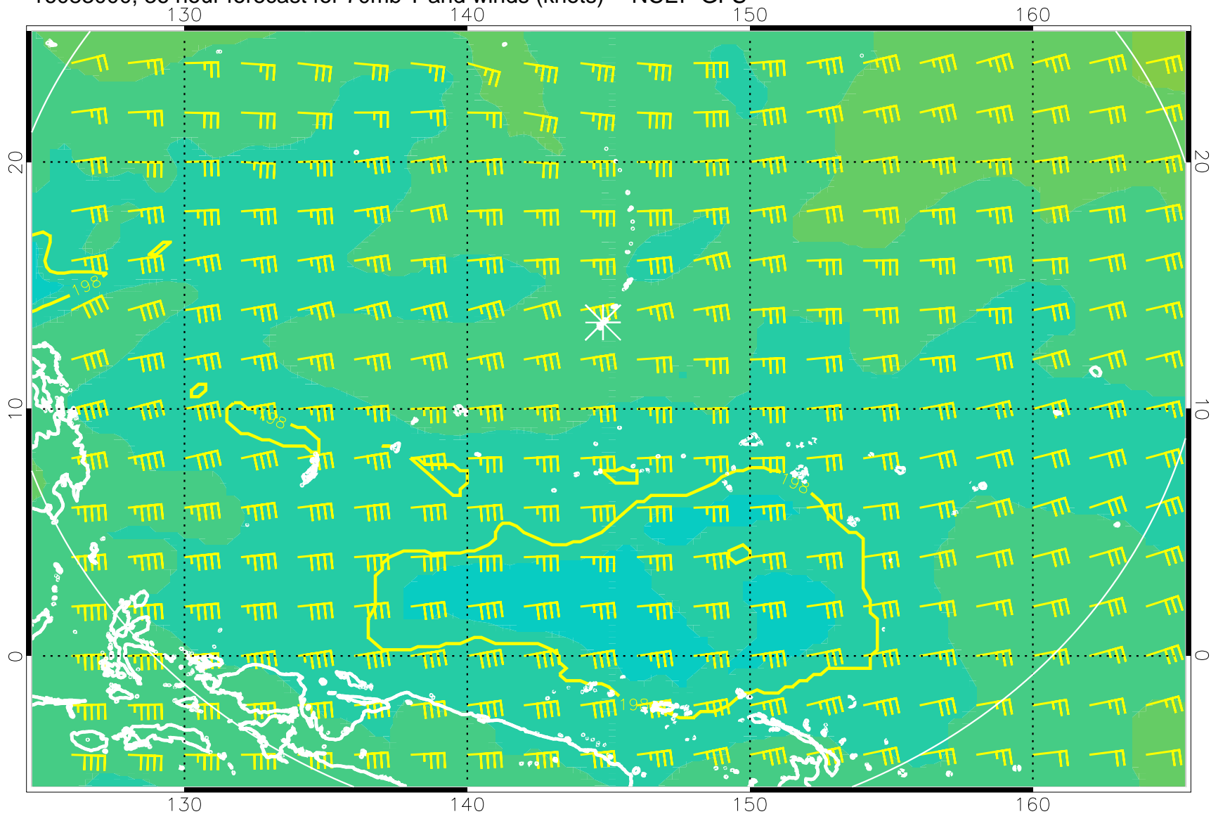
16083000, 36 hour forecast for 70mb T and winds (knots) -- NCEP GFS
