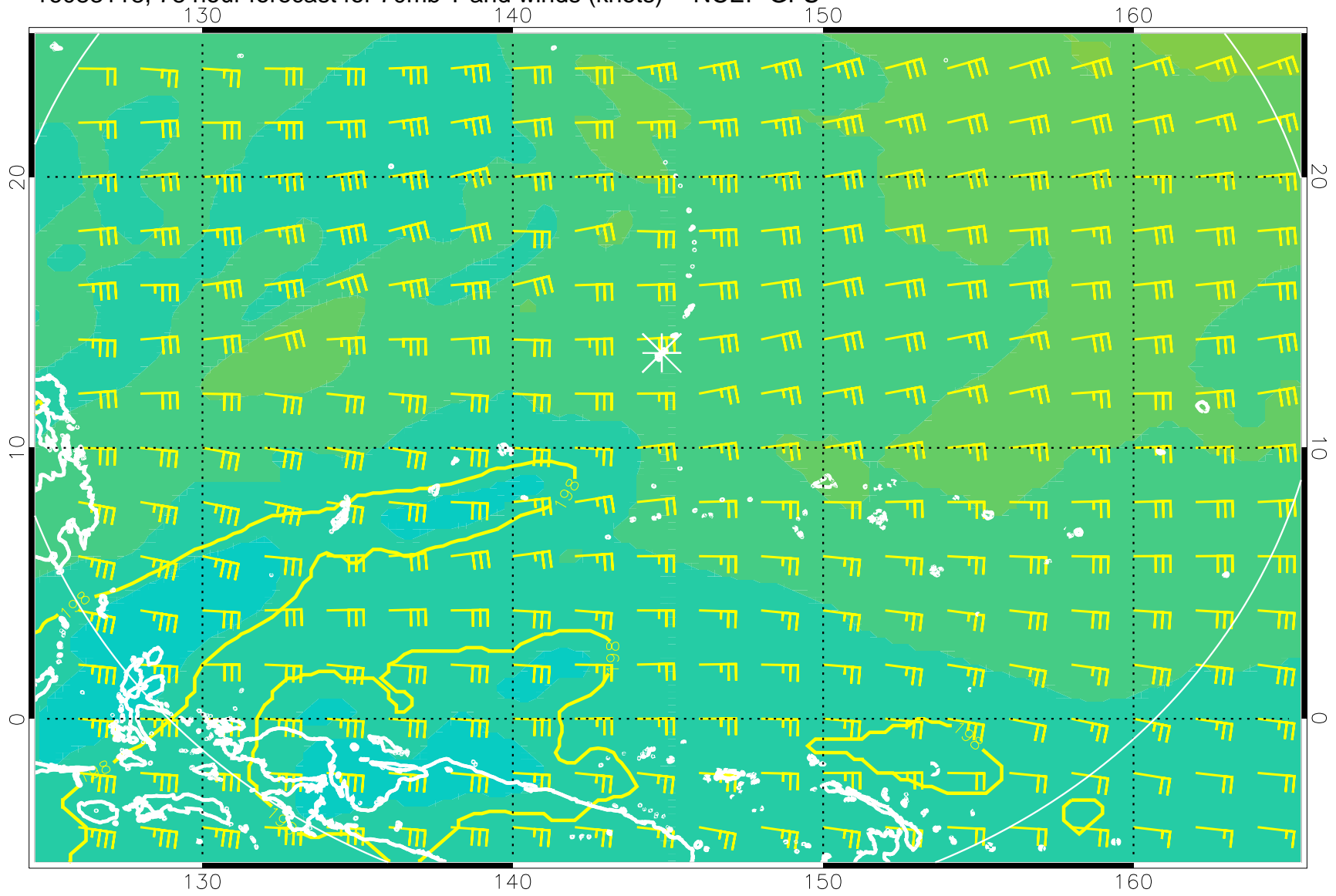
16083118, 78 hour forecast for 70mb T and winds (knots) -- NCEP GFS
