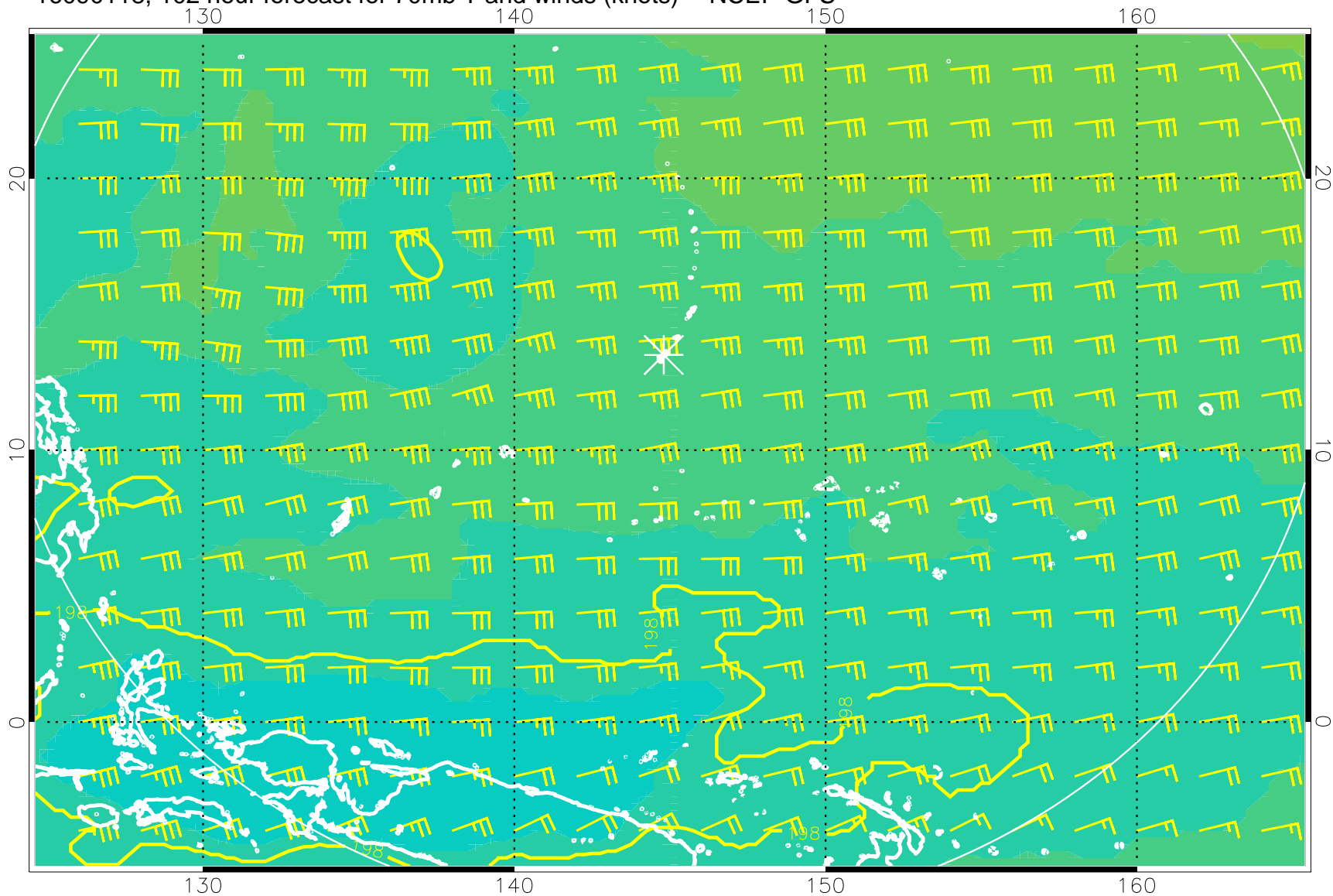
16090118, 102 hour forecast for 70mb T and winds (knots) -- NCEP GFS
