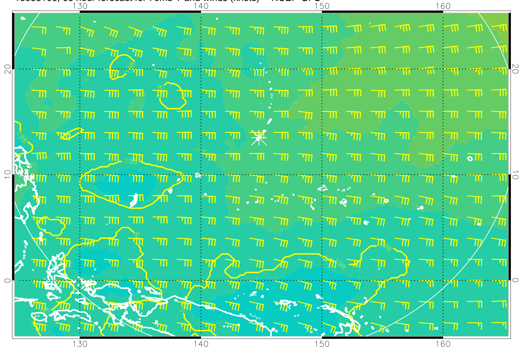
16083106, 66 hour forecast for 70mb T and winds (knots) -- NCEP GFS
