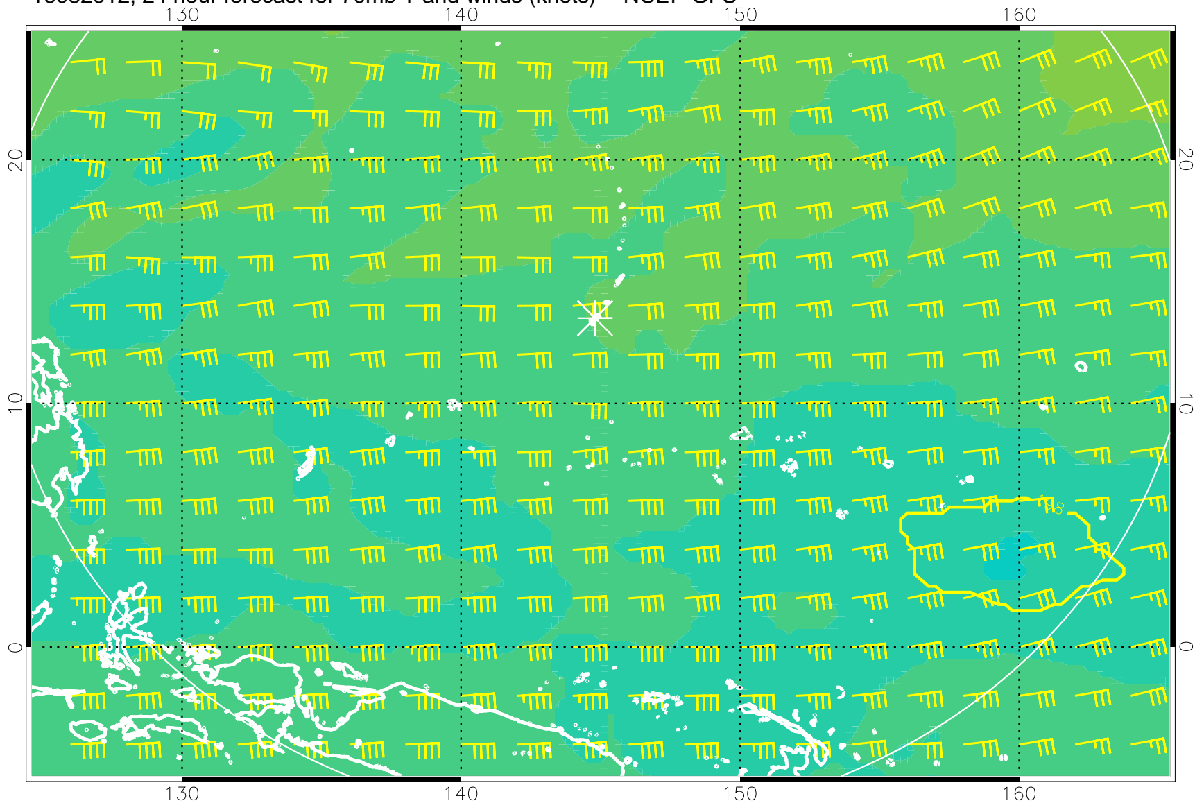
16082912, 24 hour forecast for 70mb T and winds (knots) -- NCEP GFS
