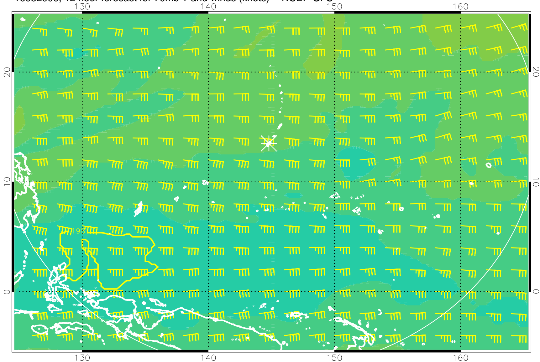
16082900, 12 hour forecast for 70mb T and winds (knots) -- NCEP GFS
