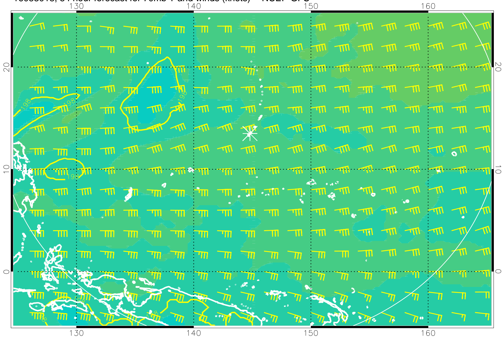
16083018, 54 hour forecast for 70mb T and winds (knots) -- NCEP GFS
