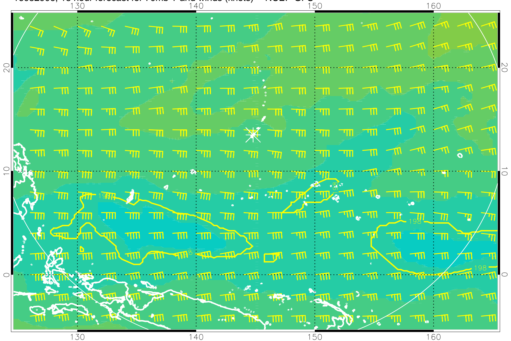
16082906, 18 hour forecast for 70mb T and winds (knots) -- NCEP GFS
