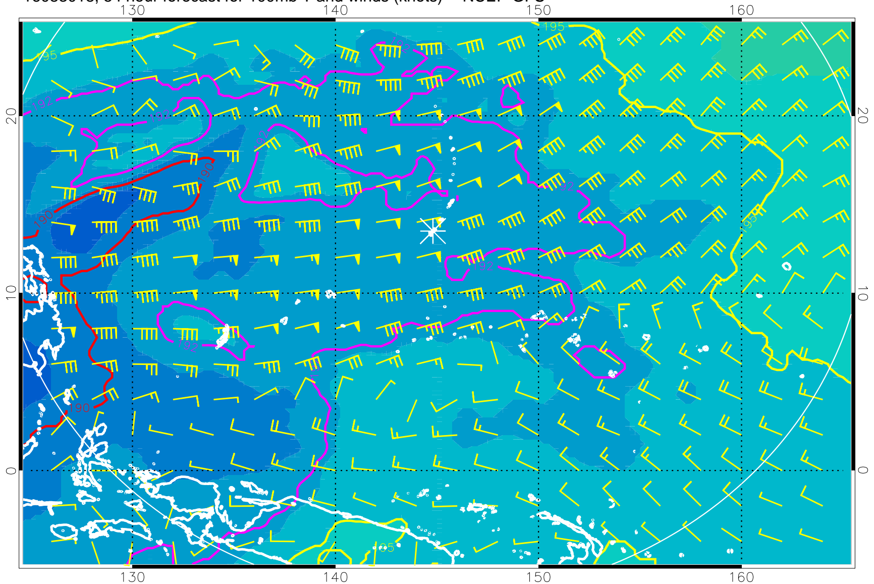
16083018, 54 hour forecast for 100mb T and winds (knots) -- NCEP GFS
