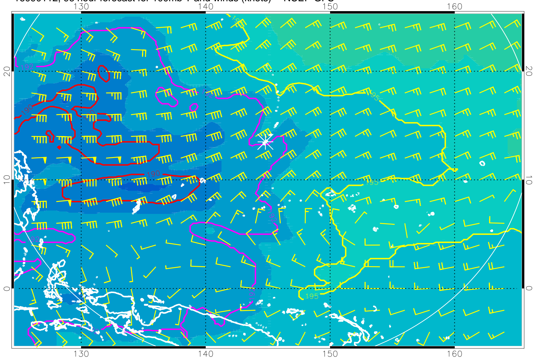
16090112, 96 hour forecast for 100mb T and winds (knots) -- NCEP GFS
