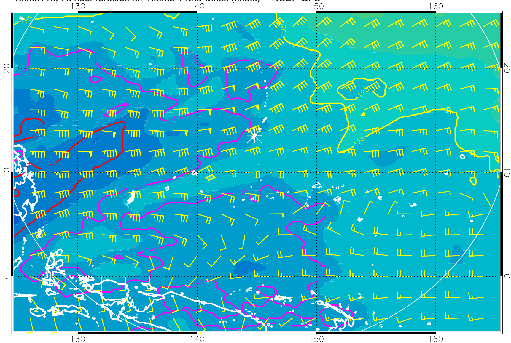
16083118, 78 hour forecast for 100mb T and winds (knots) -- NCEP GFS
