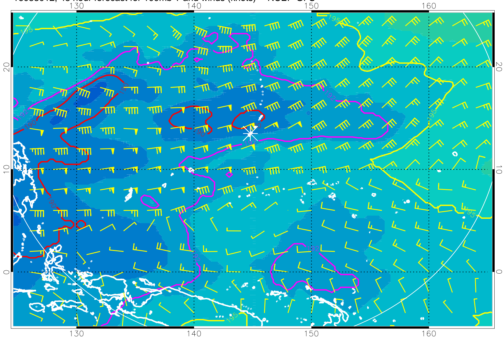
16083012, 48 hour forecast for 100mb T and winds (knots) -- NCEP GFS
