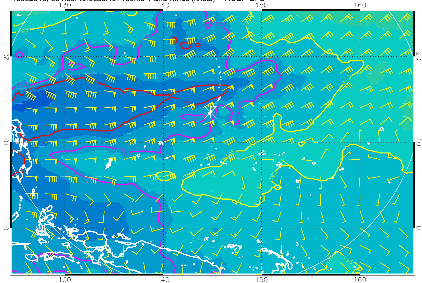
16082918, 30 hour forecast for 100mb T and winds (knots) -- NCEP GFS
