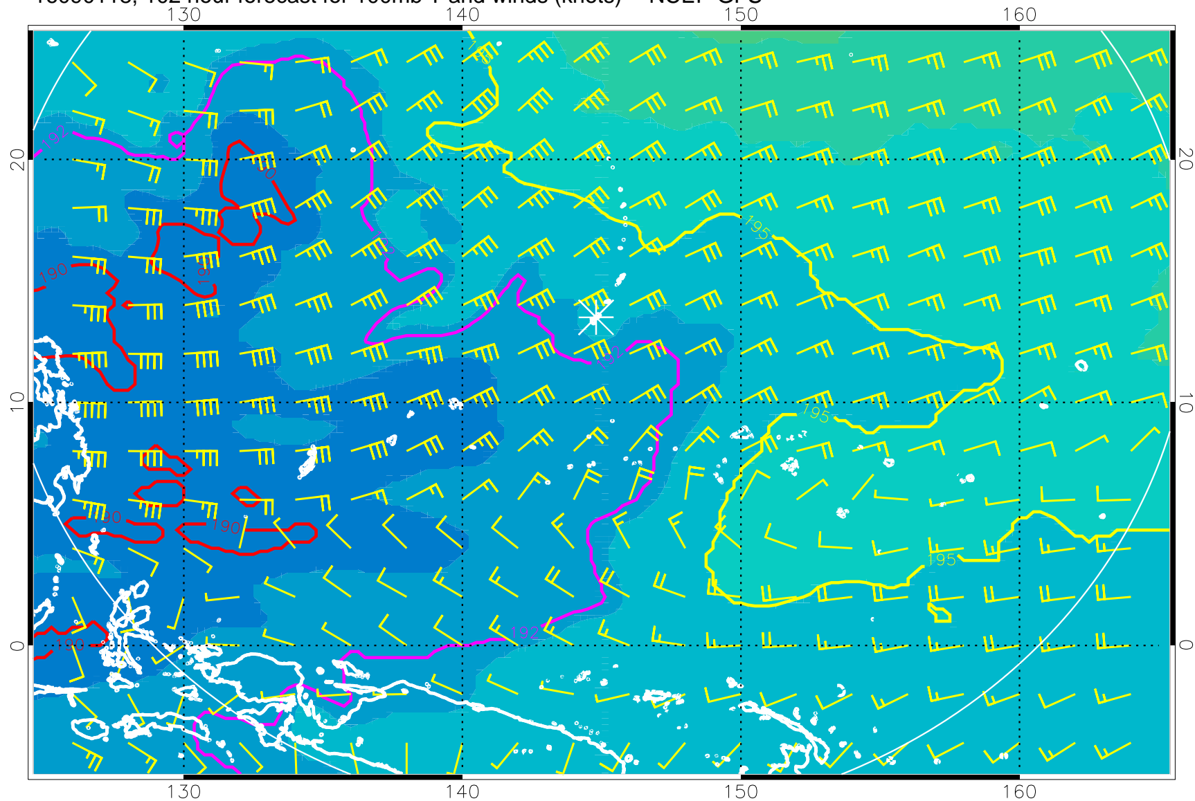
16090118, 102 hour forecast for 100mb T and winds (knots) -- NCEP GFS
