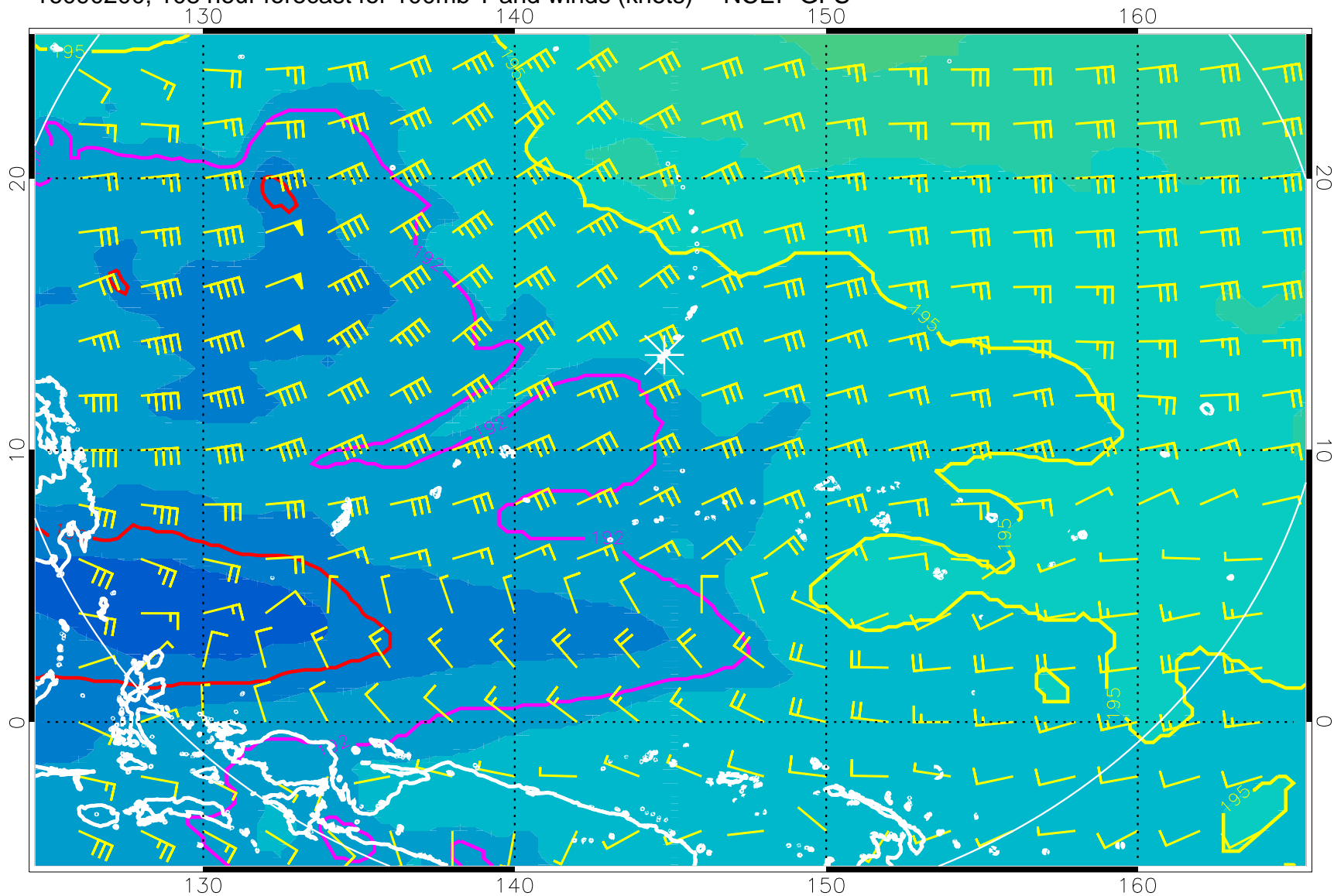
16090200, 108 hour forecast for 100mb T and winds (knots) -- NCEP GFS
