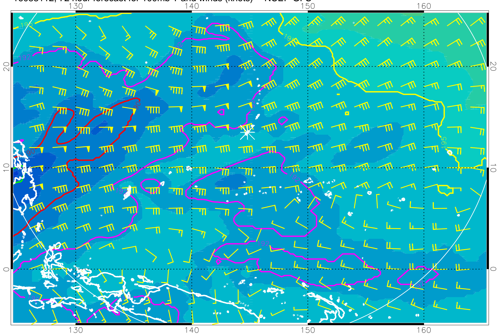
16083112, 72 hour forecast for 100mb T and winds (knots) -- NCEP GFS
