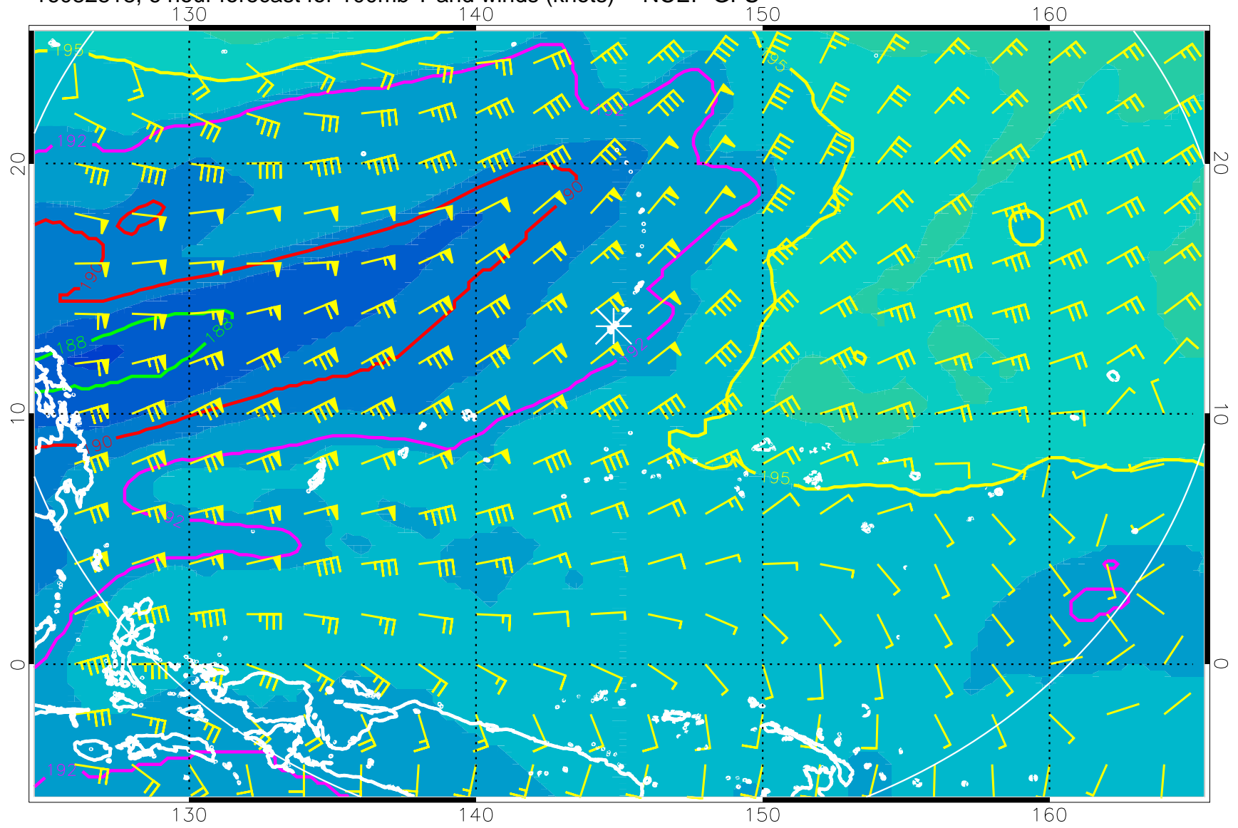
16082818, 6 hour forecast for 100mb T and winds (knots) -- NCEP GFS
