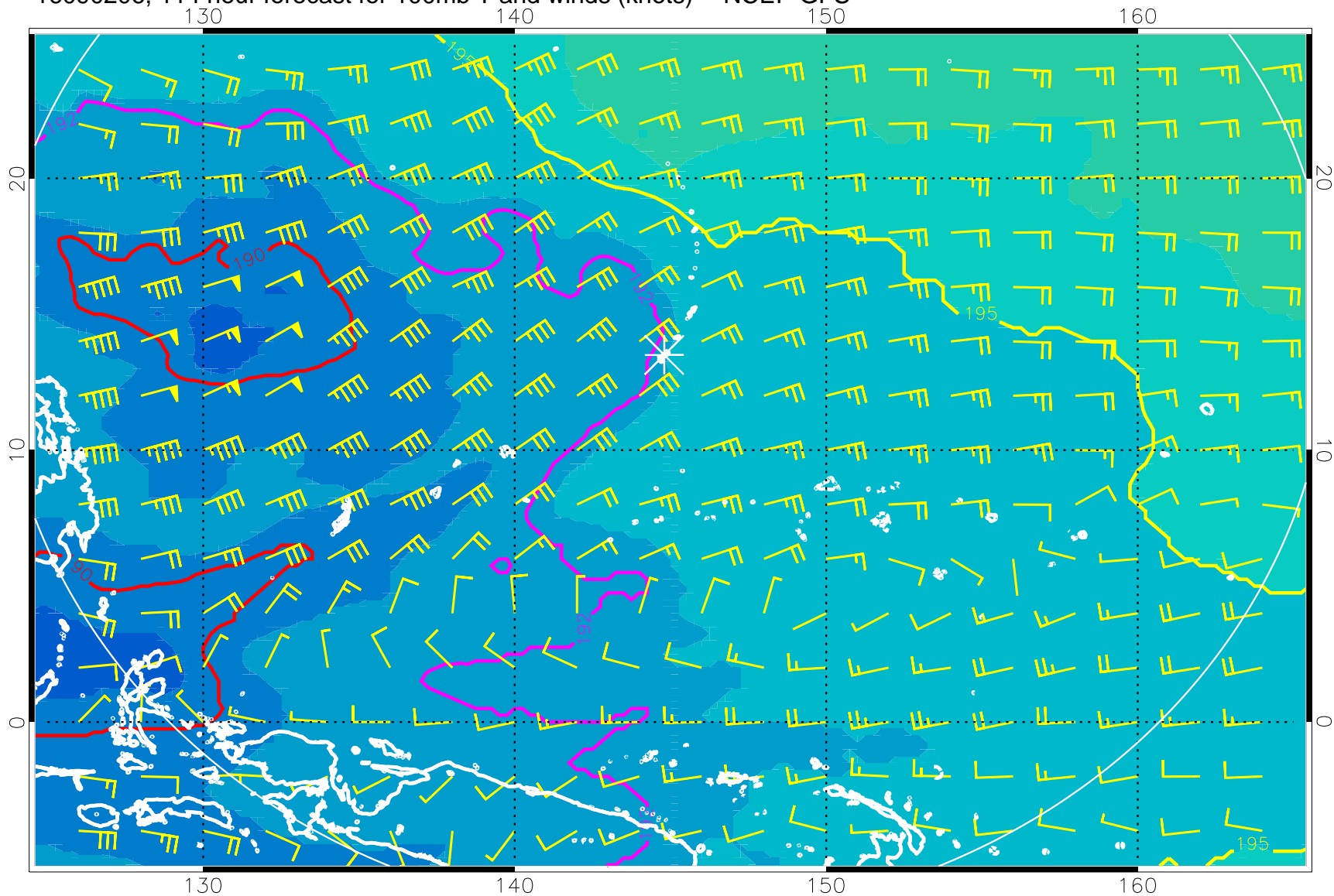
16090206, 114 hour forecast for 100mb T and winds (knots) -- NCEP GFS
