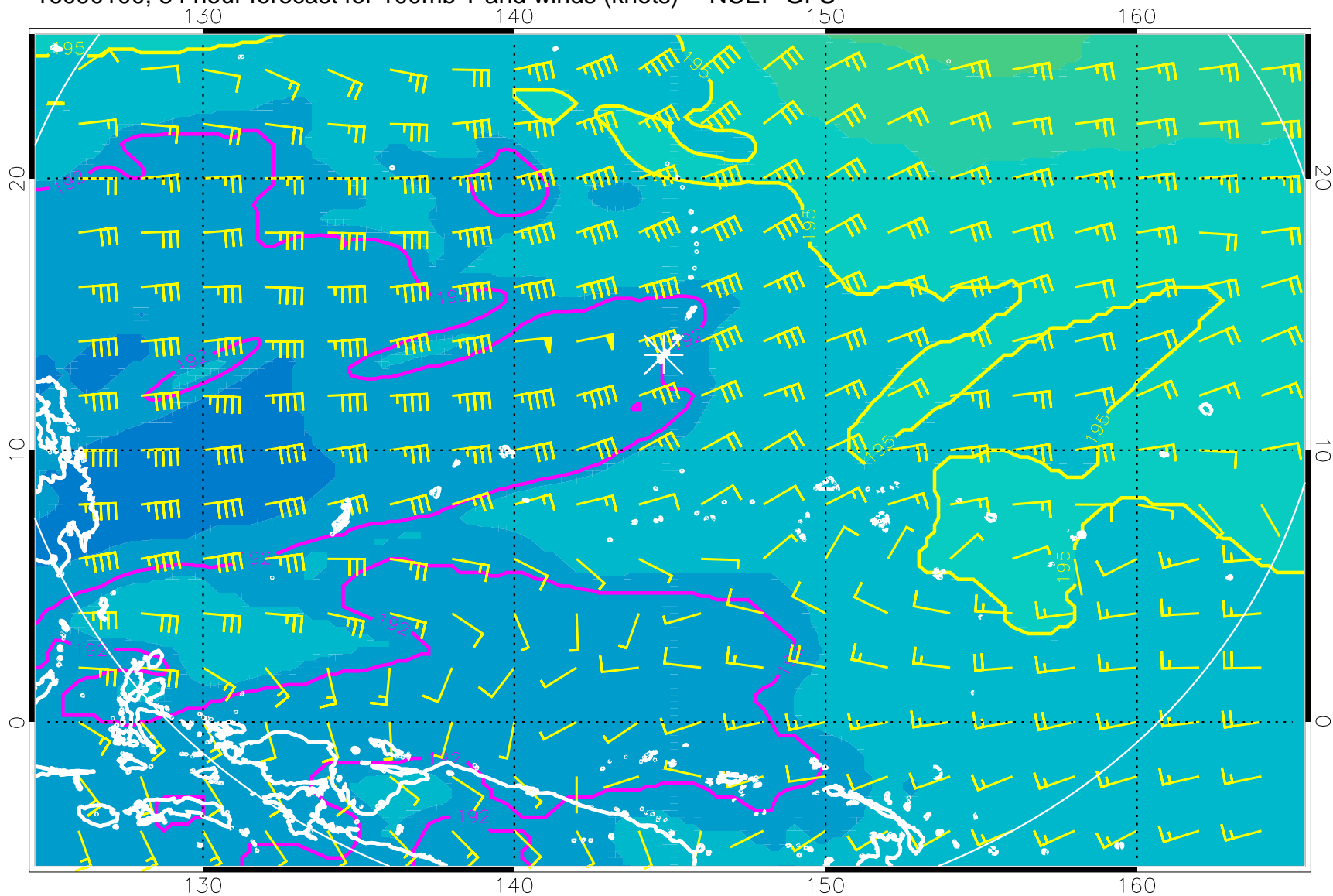
16090100, 84 hour forecast for 100mb T and winds (knots) -- NCEP GFS
