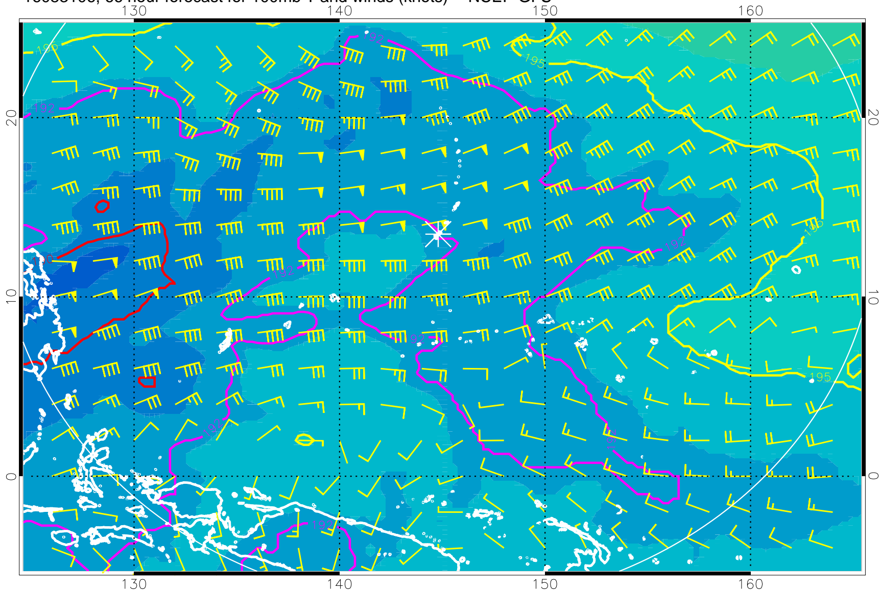
16083106, 66 hour forecast for 100mb T and winds (knots) -- NCEP GFS
