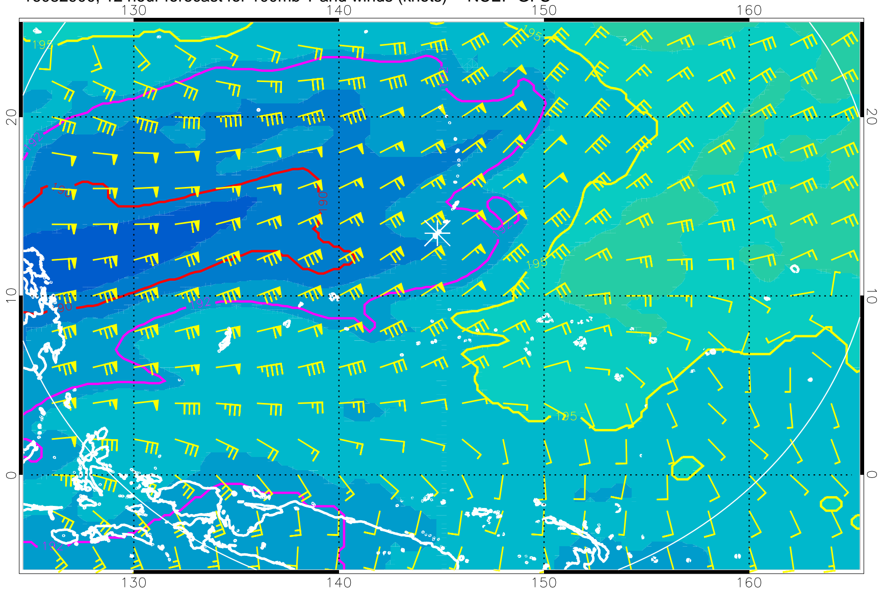
16082900, 12 hour forecast for 100mb T and winds (knots) -- NCEP GFS
