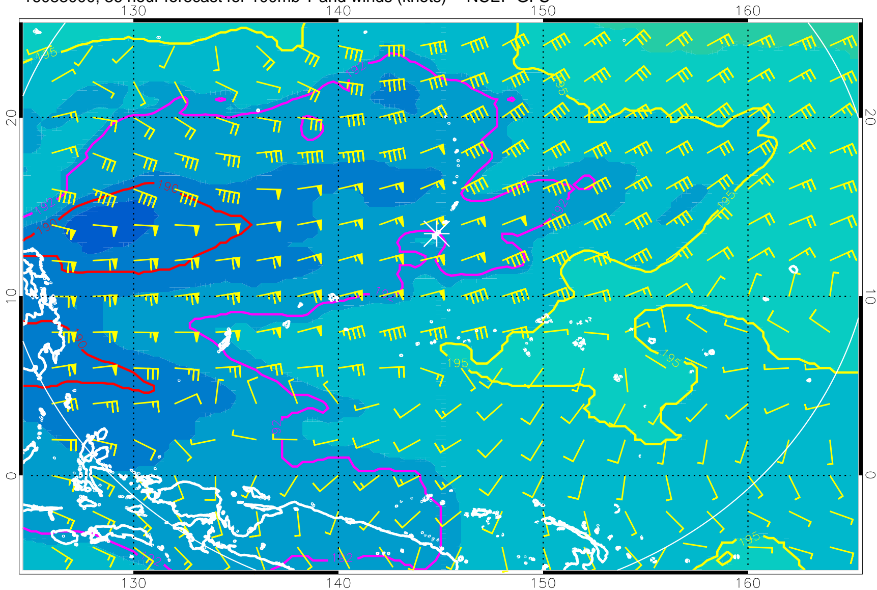
16083000, 36 hour forecast for 100mb T and winds (knots) -- NCEP GFS
