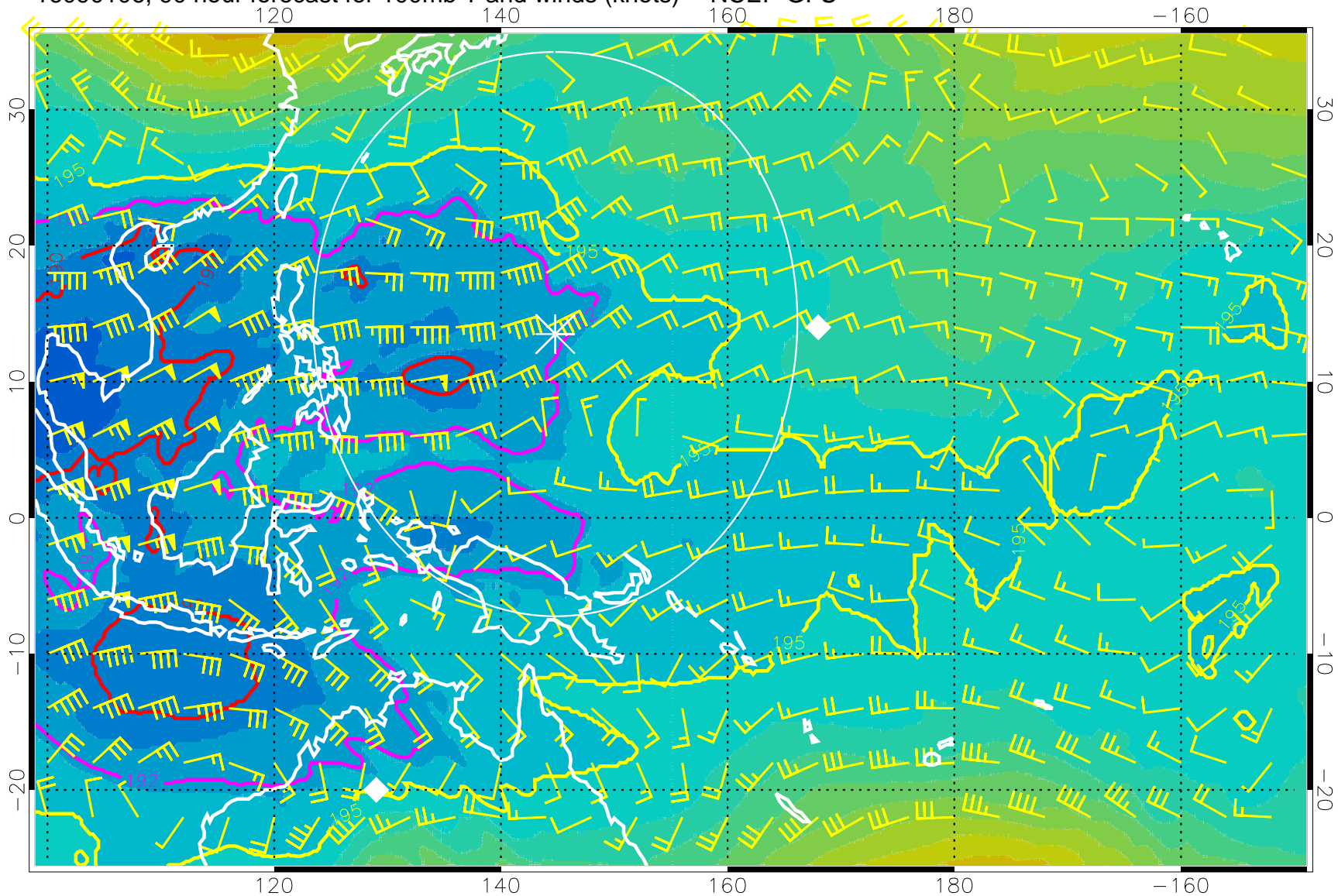
16090106, 90 hour forecast for 100mb T and winds (knots) -- NCEP GFS
