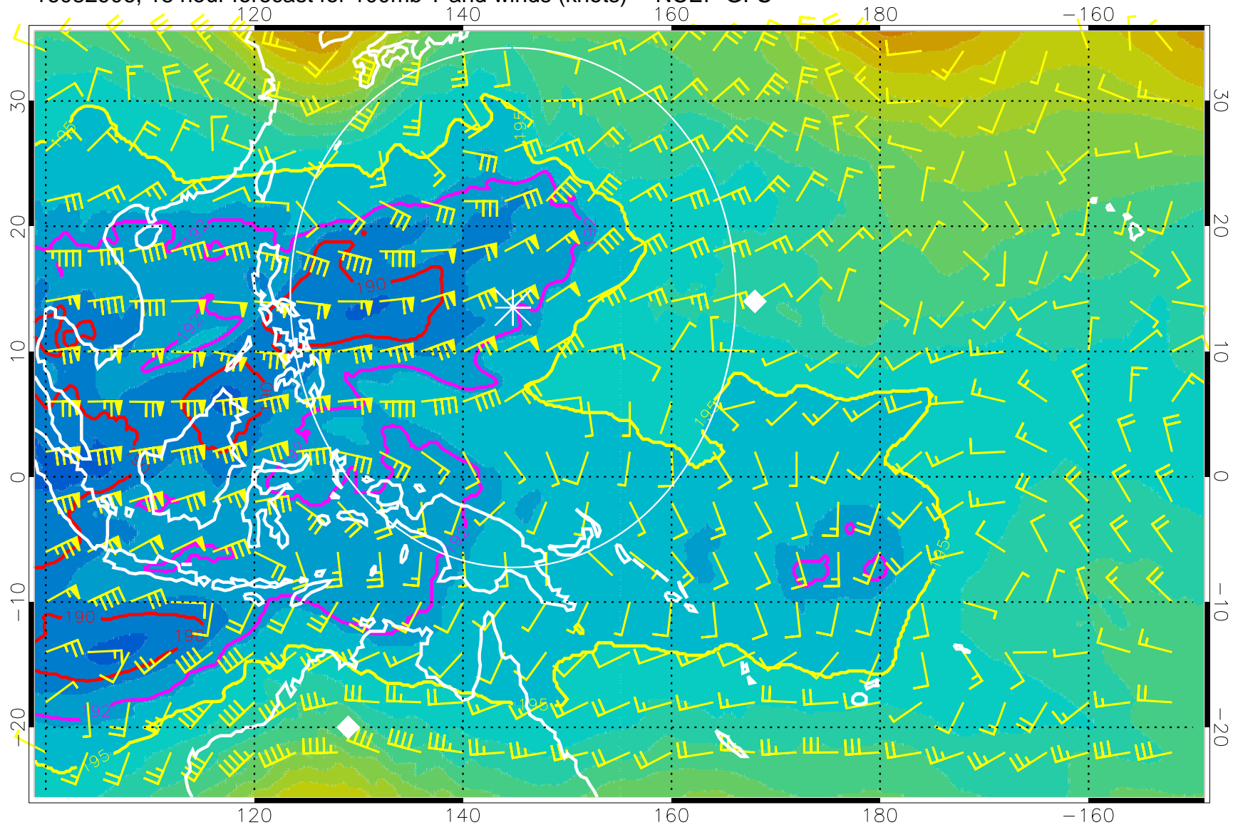
16082906, 18 hour forecast for 100mb T and winds (knots) -- NCEP GFS
