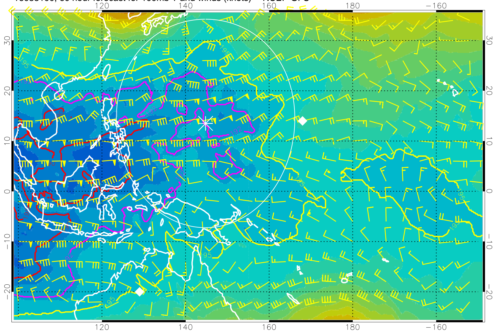
16083100, 60 hour forecast for 100mb T and winds (knots) -- NCEP GFS
