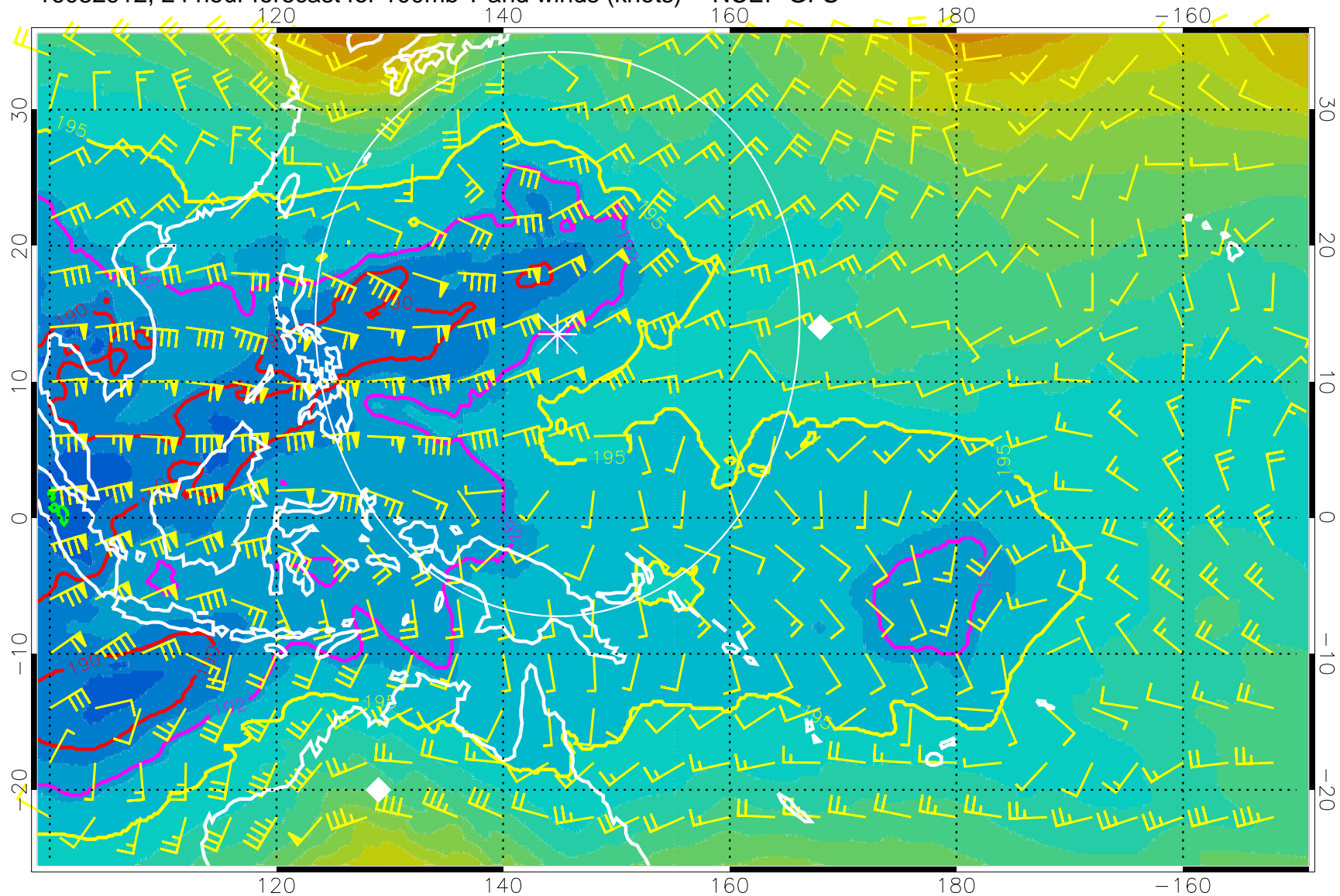
16082912, 24 hour forecast for 100mb T and winds (knots) -- NCEP GFS
