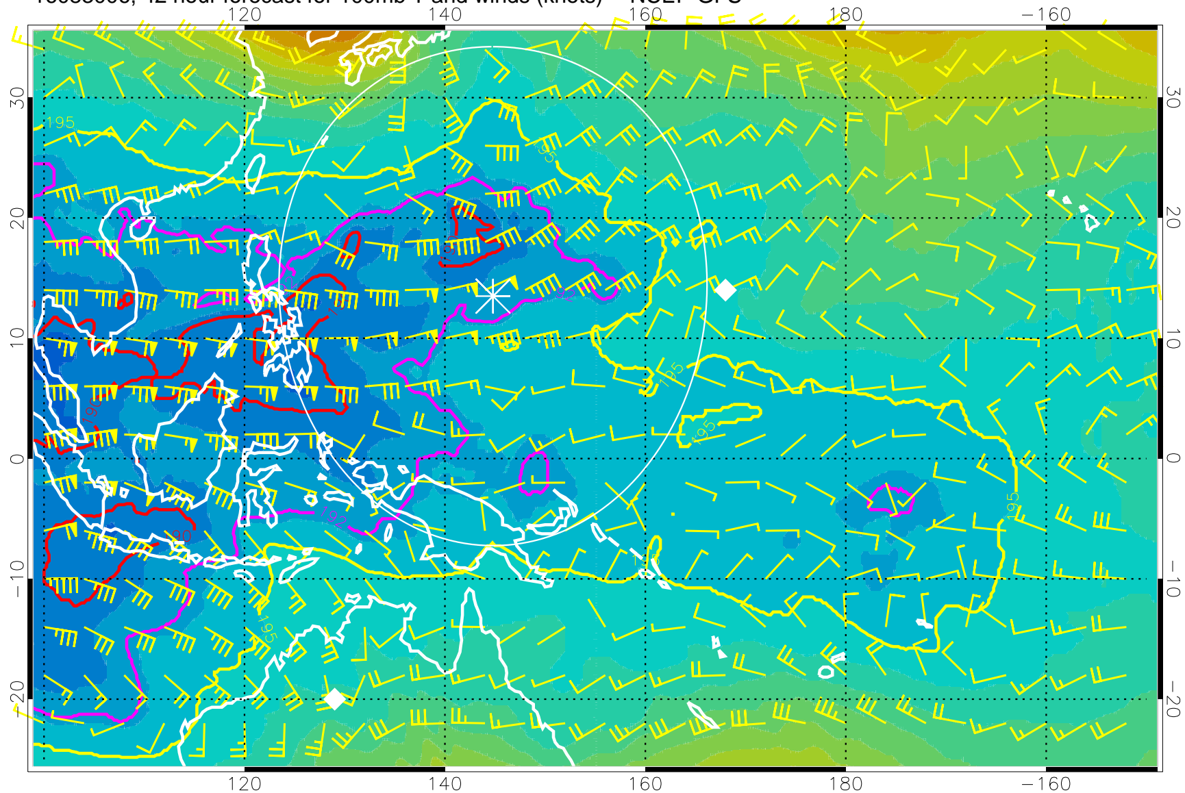
16083006, 42 hour forecast for 100mb T and winds (knots) -- NCEP GFS
