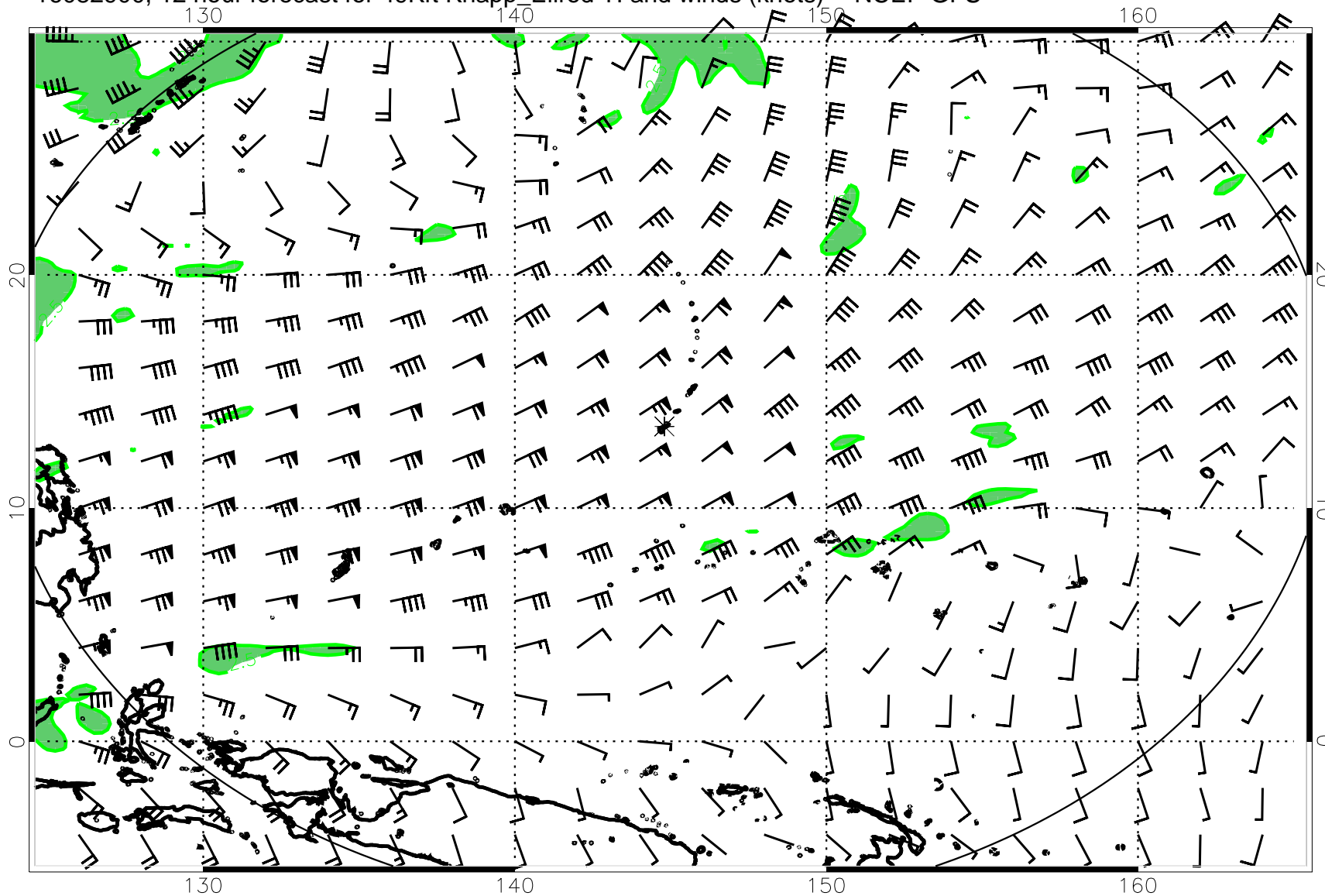
16082900, 12 hour forecast for 49Kft Knapp_Ellrod TI and winds (knots) -- NCEP GFS
