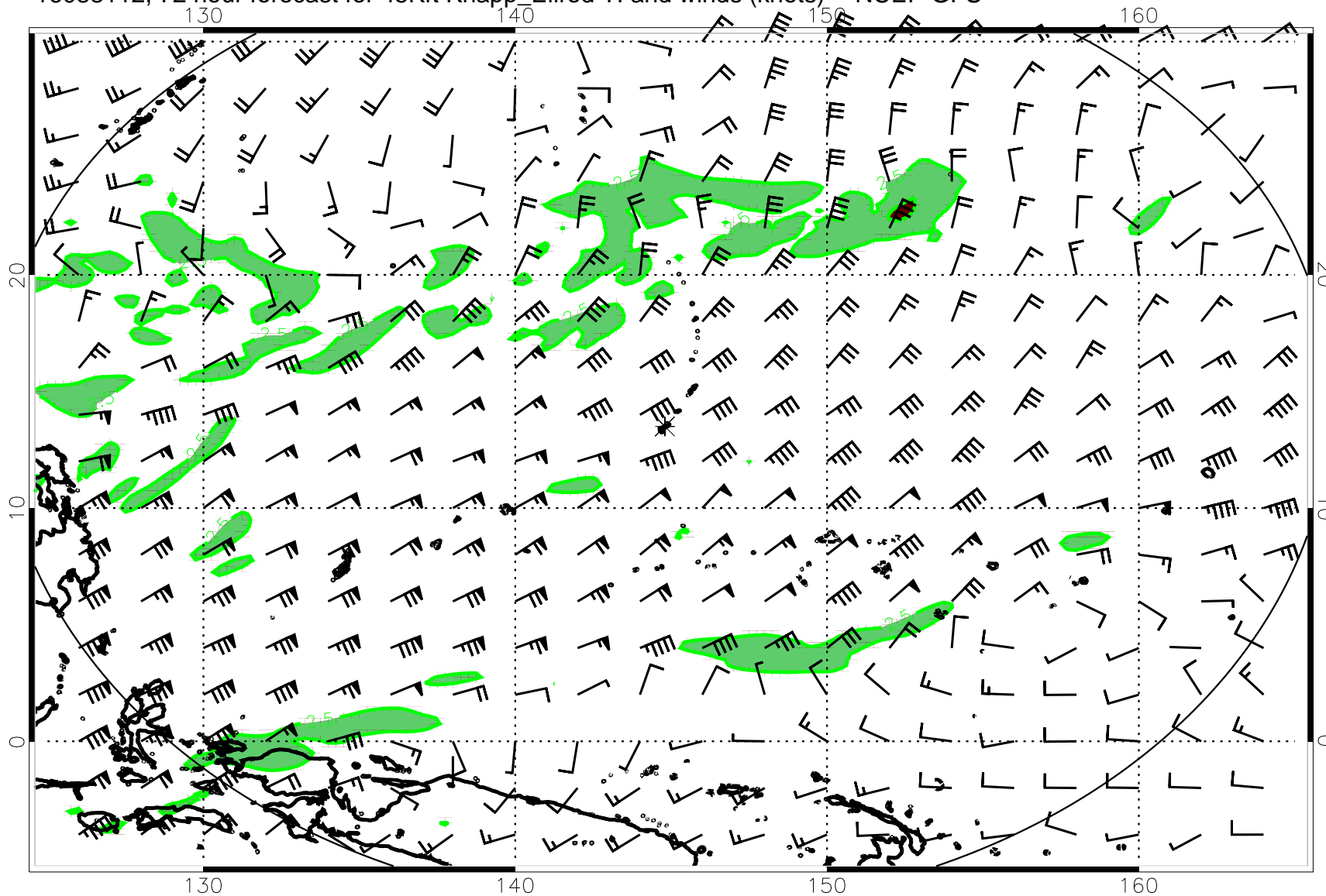
16083112, 72 hour forecast for 45Kft Knapp_Ellrod TI and winds (knots) -- NCEP GFS
