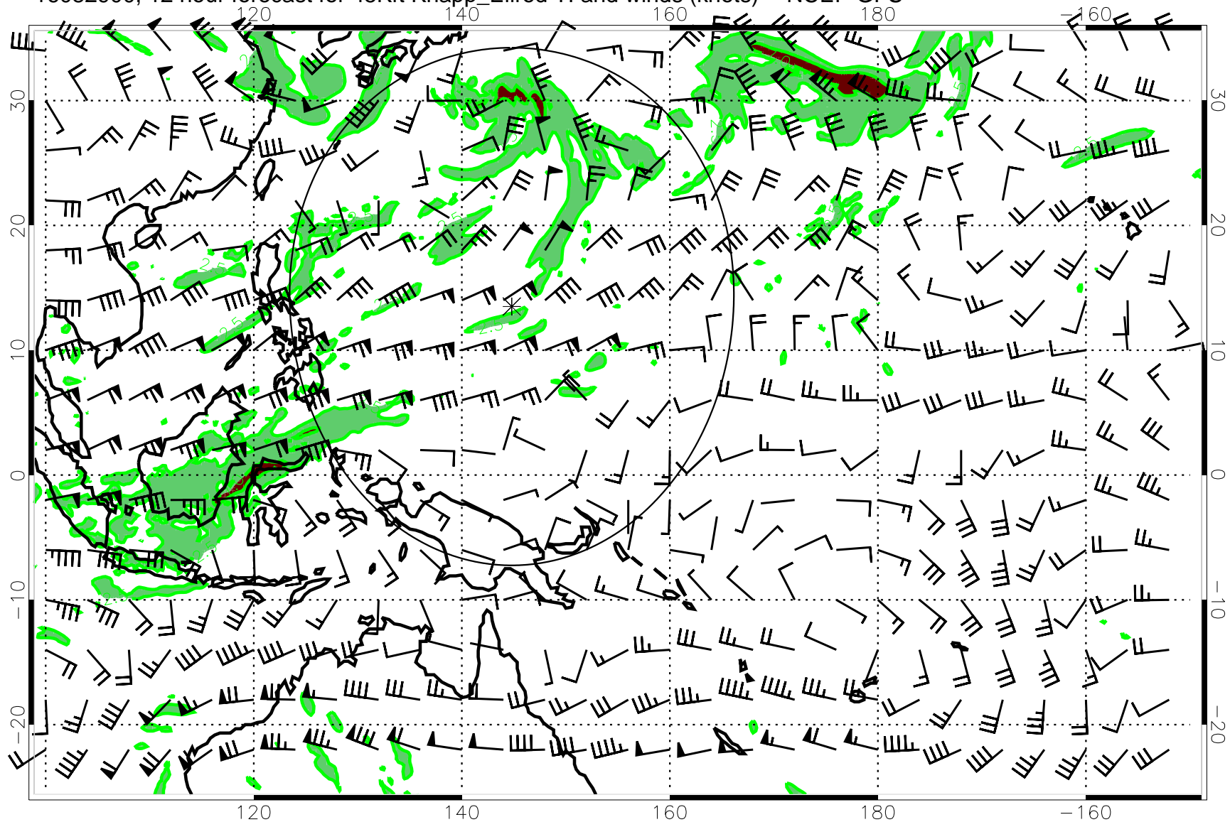
16082900, 12 hour forecast for 45Kft Knapp_Ellrod TI and winds (knots) -- NCEP GFS
