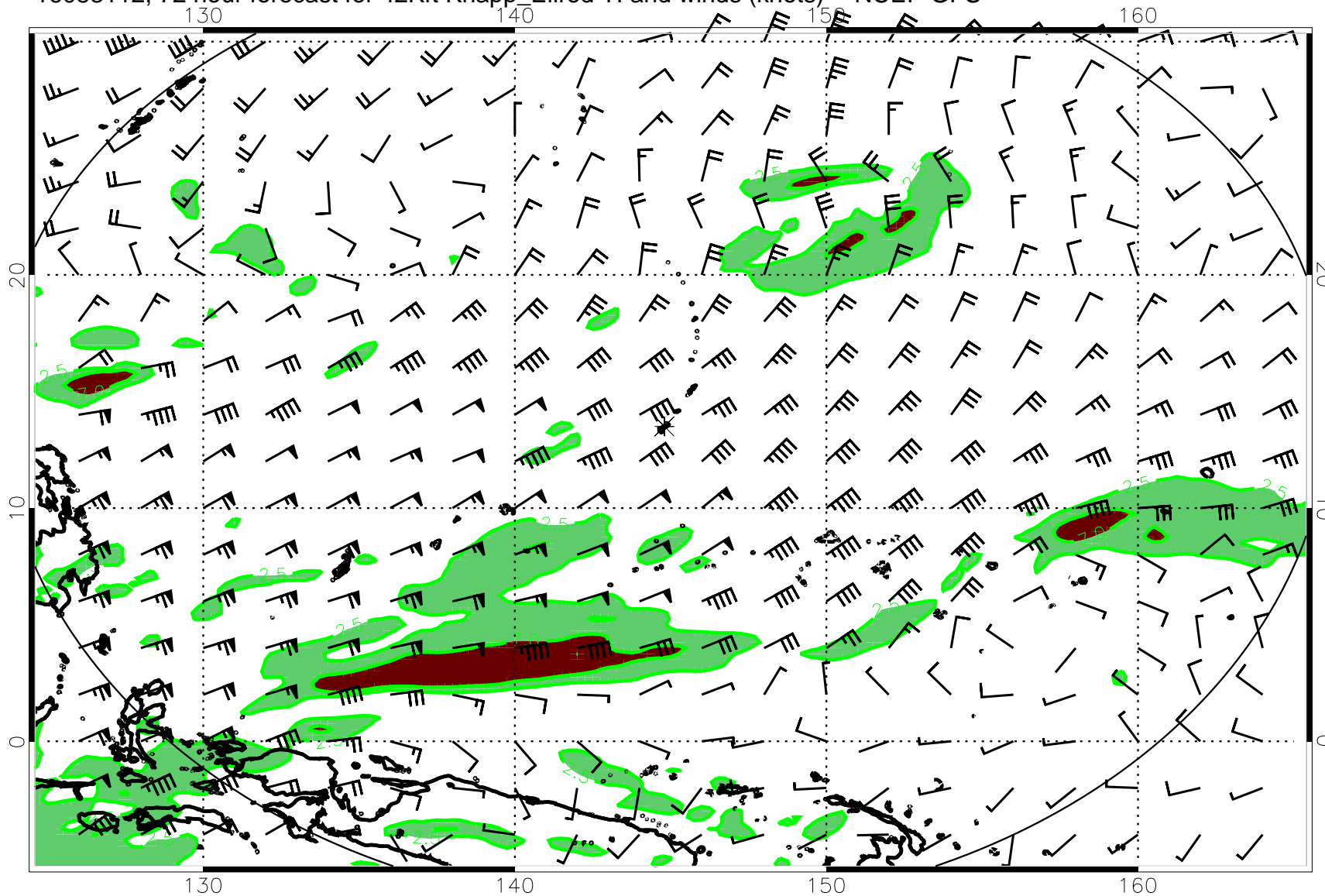
16083112, 72 hour forecast for 42Kft Knapp_Ellrod TI and winds (knots) -- NCEP GFS
