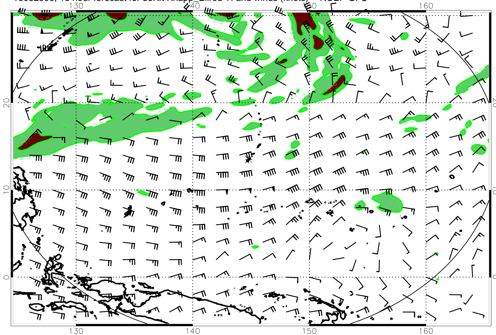
16082906, 18 hour forecast for 36Kft Knapp_Ellrod TI and winds (knots) -- NCEP GFS
