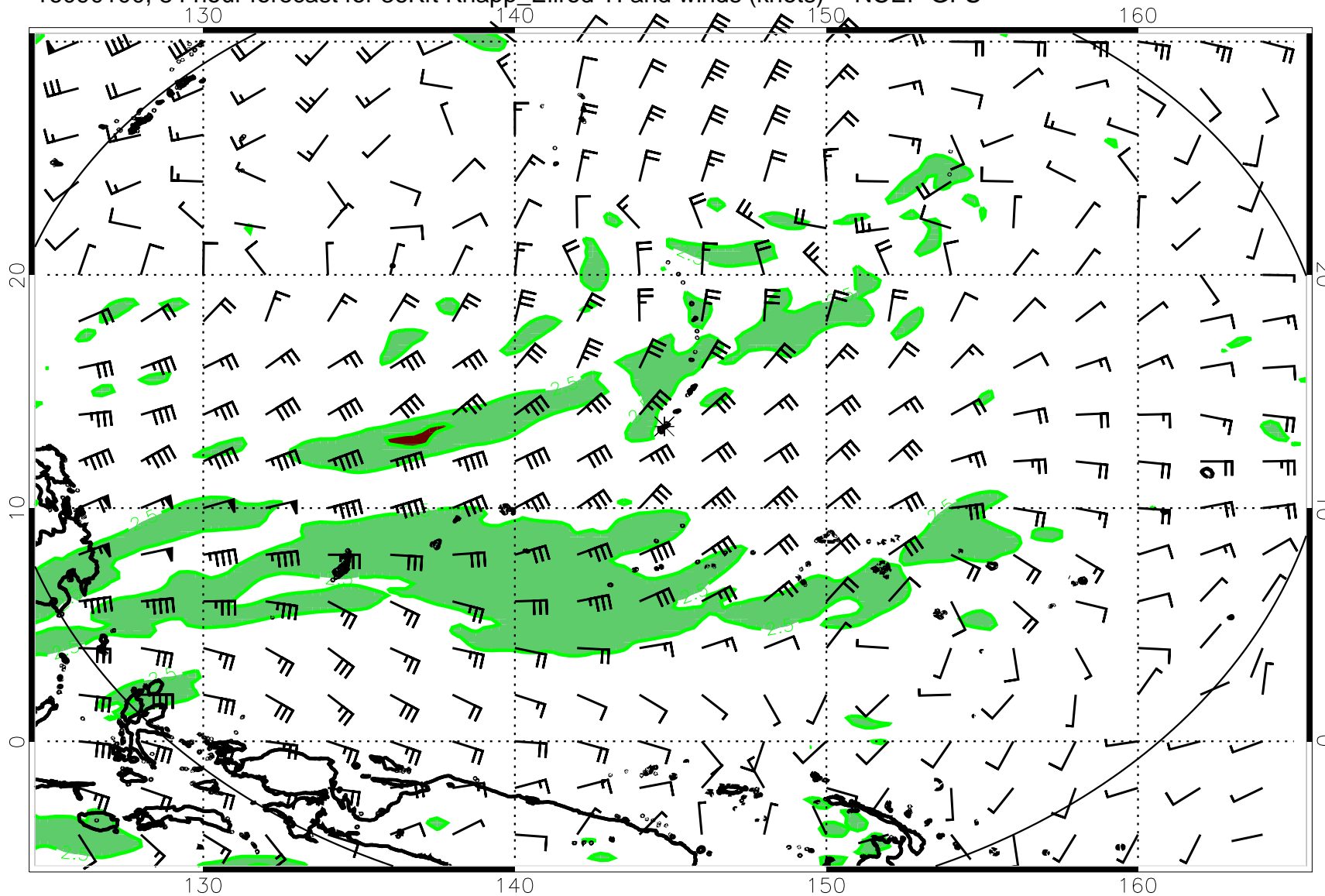
16090100, 84 hour forecast for 36Kft Knapp_Ellrod TI and winds (knots) -- NCEP GFS
